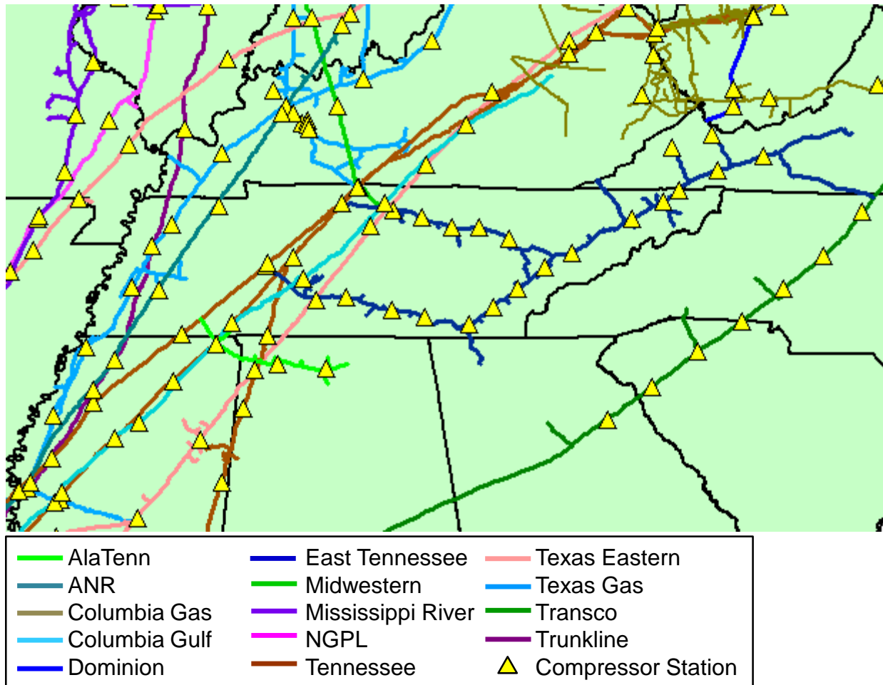
Figure 25. TVA Pipeline Map
