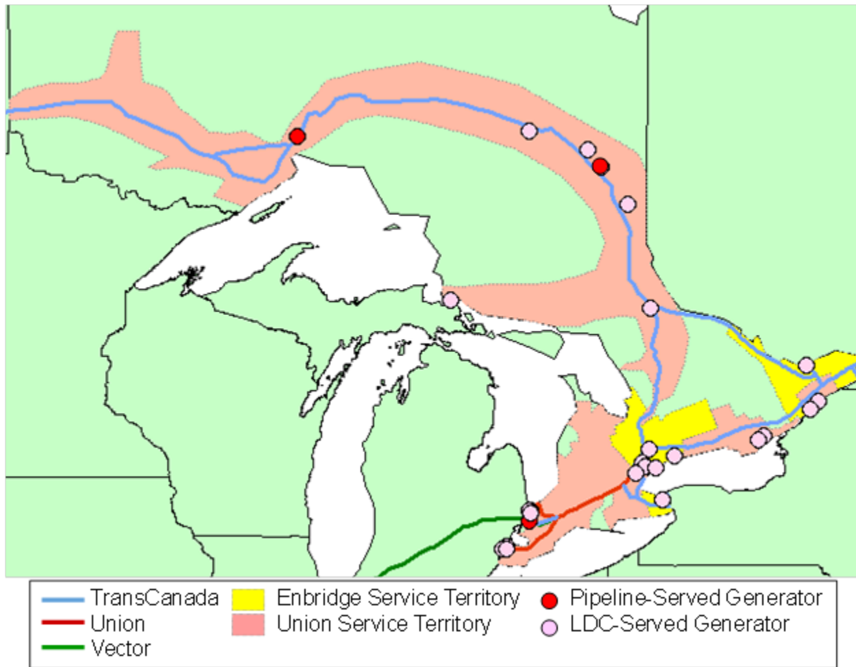
Figure 10. Ontario Natural Gas Infrastructure
