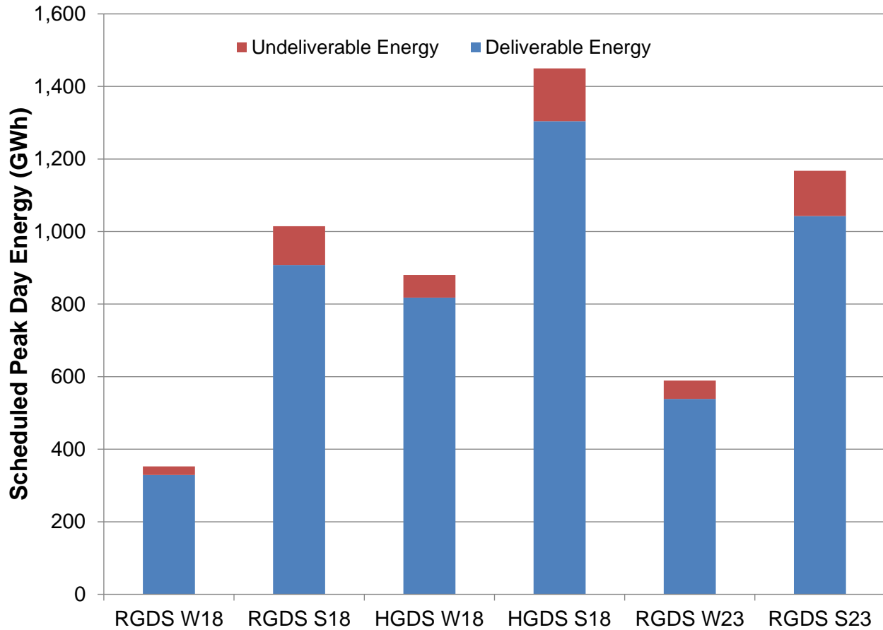
Figure 24. PJM Baseline Energy Deliverability
