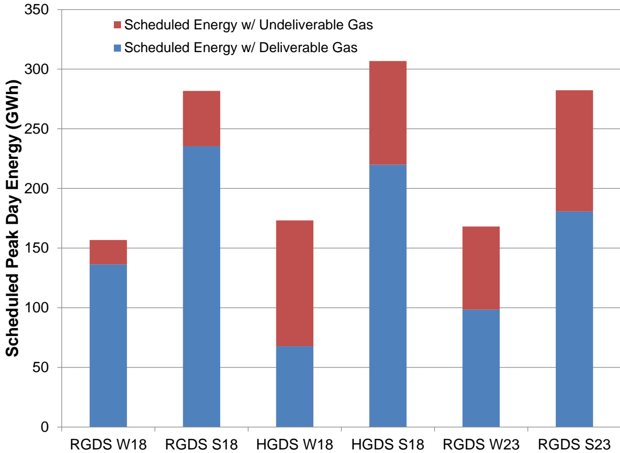
Figure 13. ISO-NE Baseline Energy Deliverability
