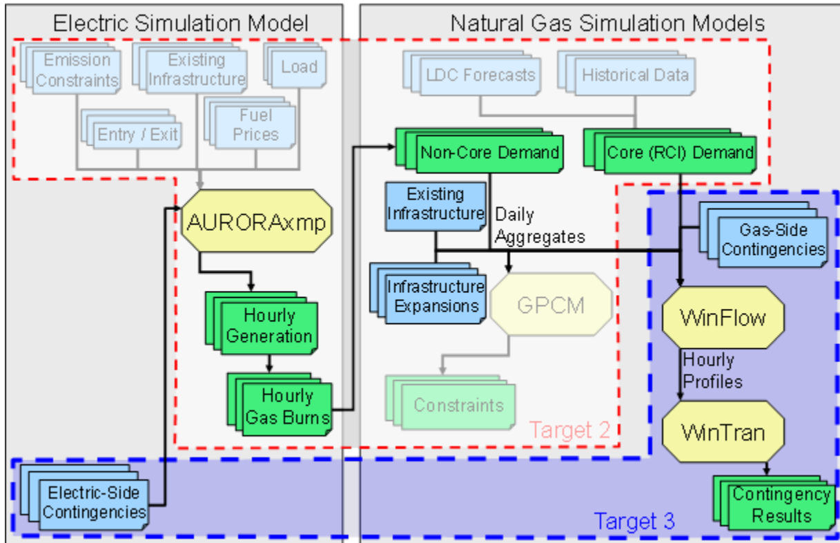
Figure 2. Target 3 Model Components
