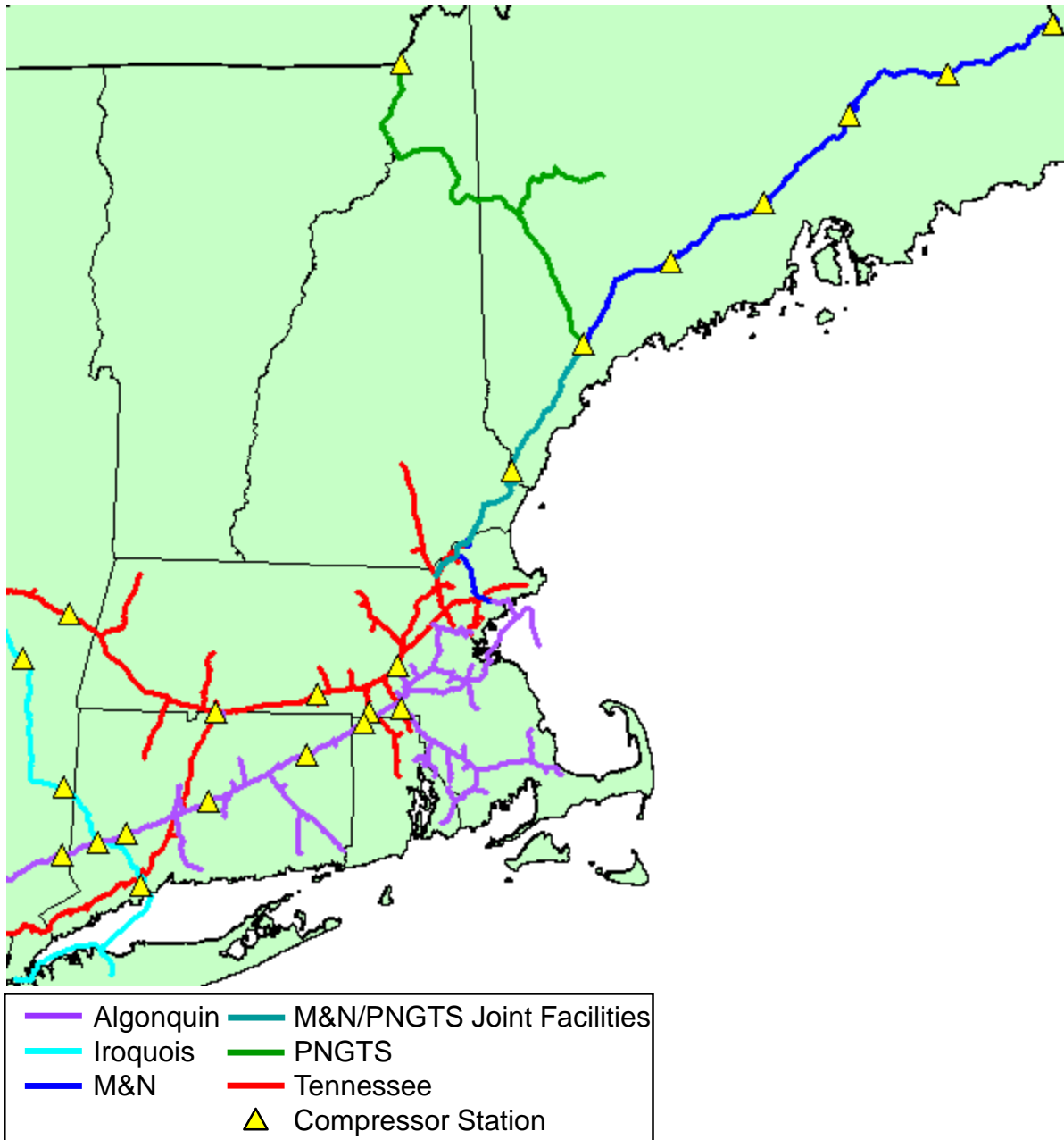
Figure 11. New England Gas Pipeline Map
