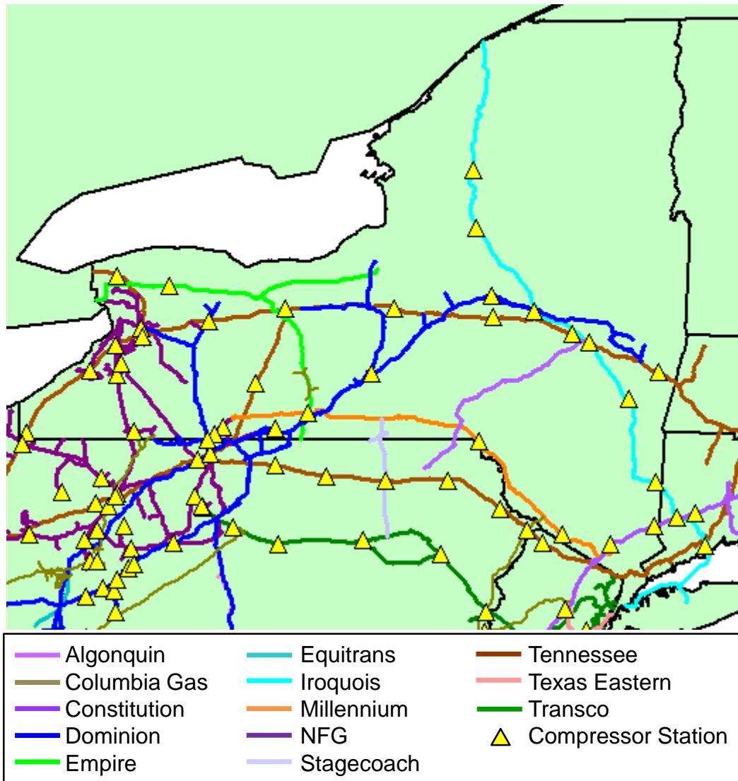
Figure 19. NYISO Pipeline Map 49
