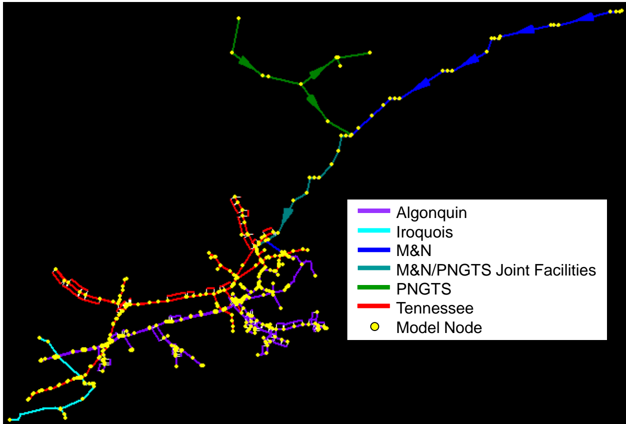
Figure 12. Consolidated New England Hydraulic Model
