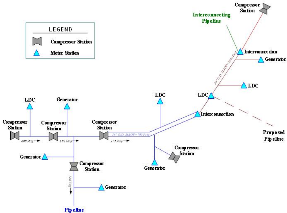
Figure 3. Example Hydraulic Model Schematic
