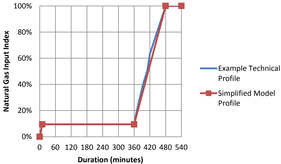
Figure 9. Steam Generator Start-Up Fuel Input Profile
