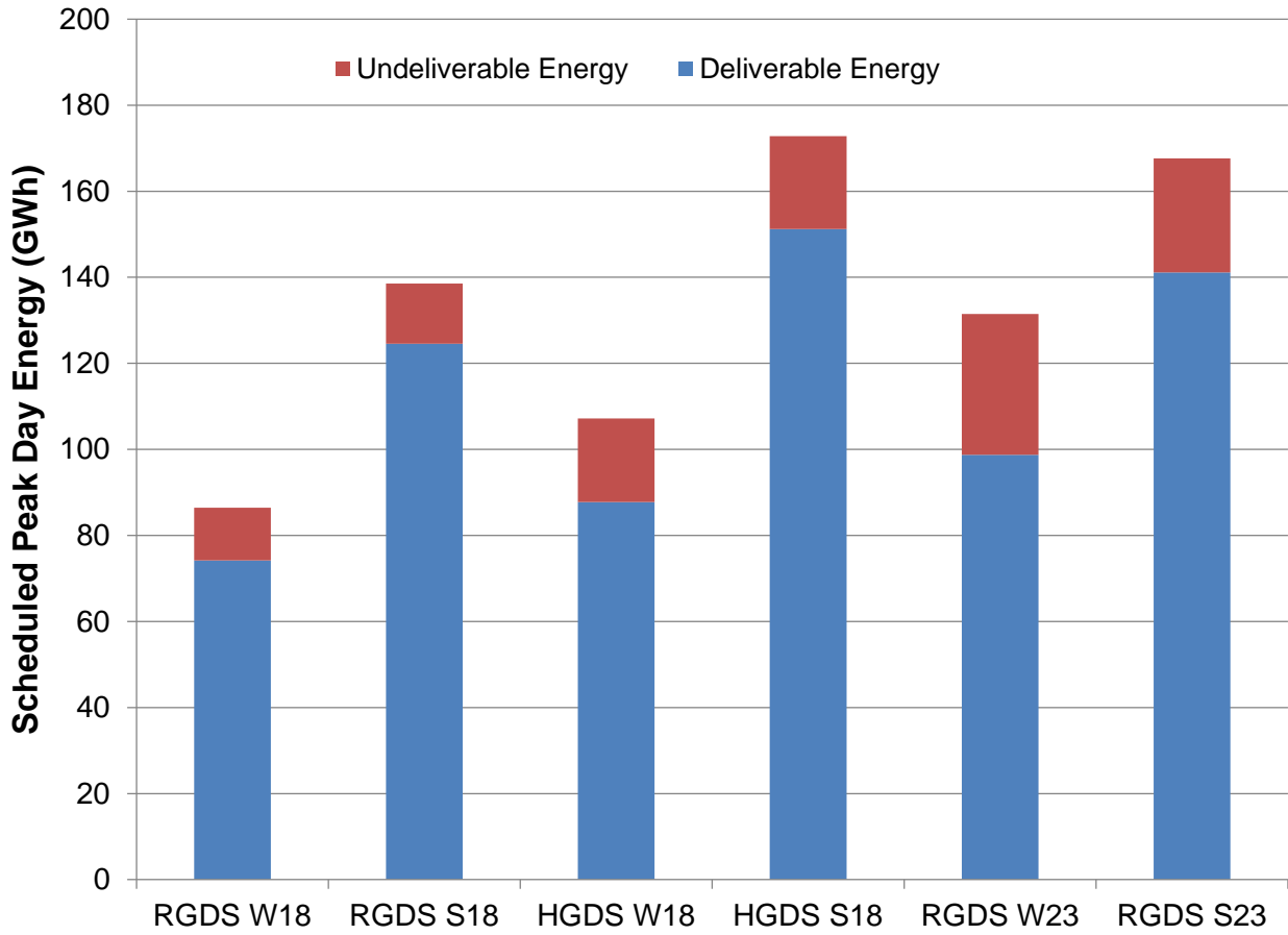
Figure 21. NYISO Baseline Energy Deliverability
