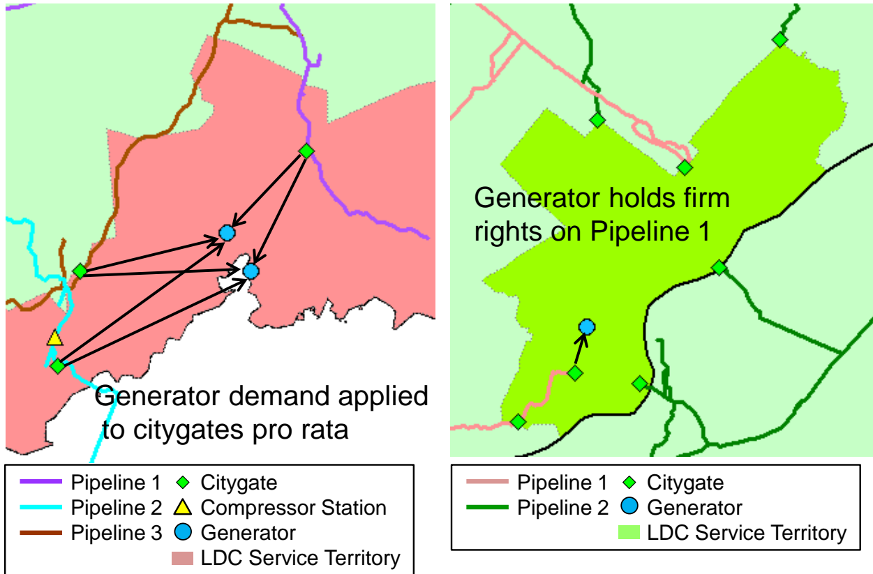
Figure 4. LDC-Served Generator Demand Allocation Examples
