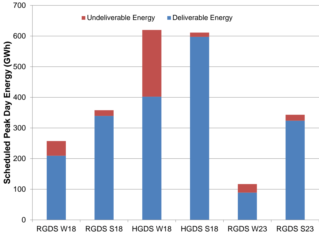
Figure 18. MISO Baseline Energy Deliverability
