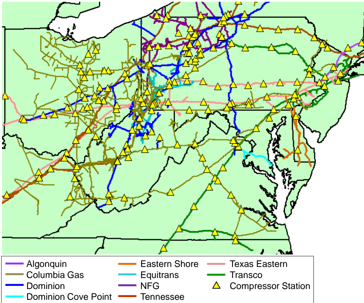
Figure 22. PJM Pipeline Map
