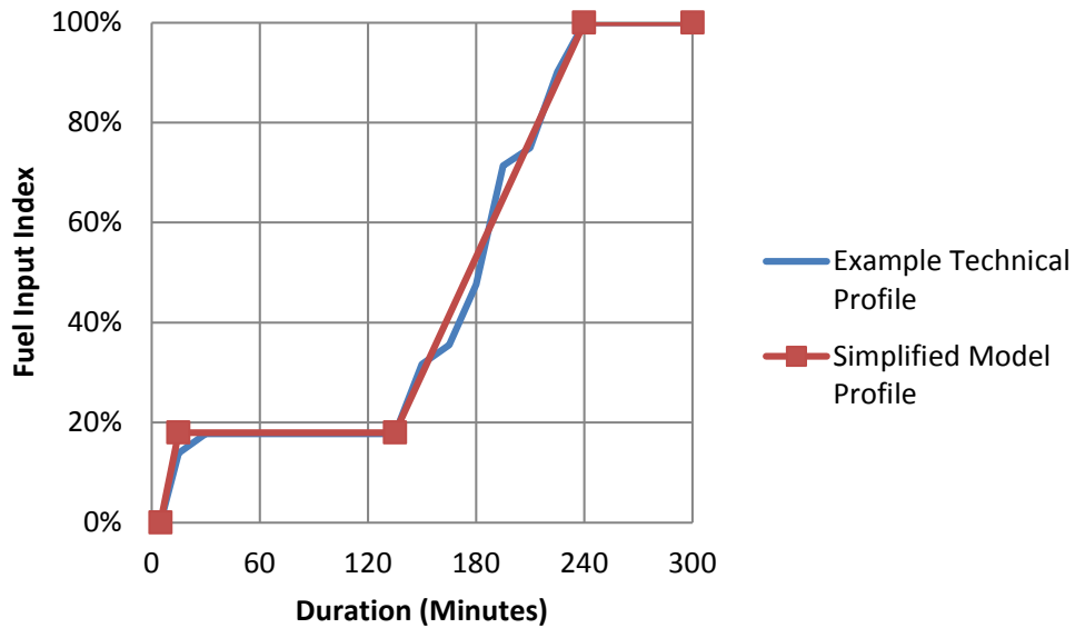
Figure 8. CCGT Generator Start-Up Fuel Input Profile
