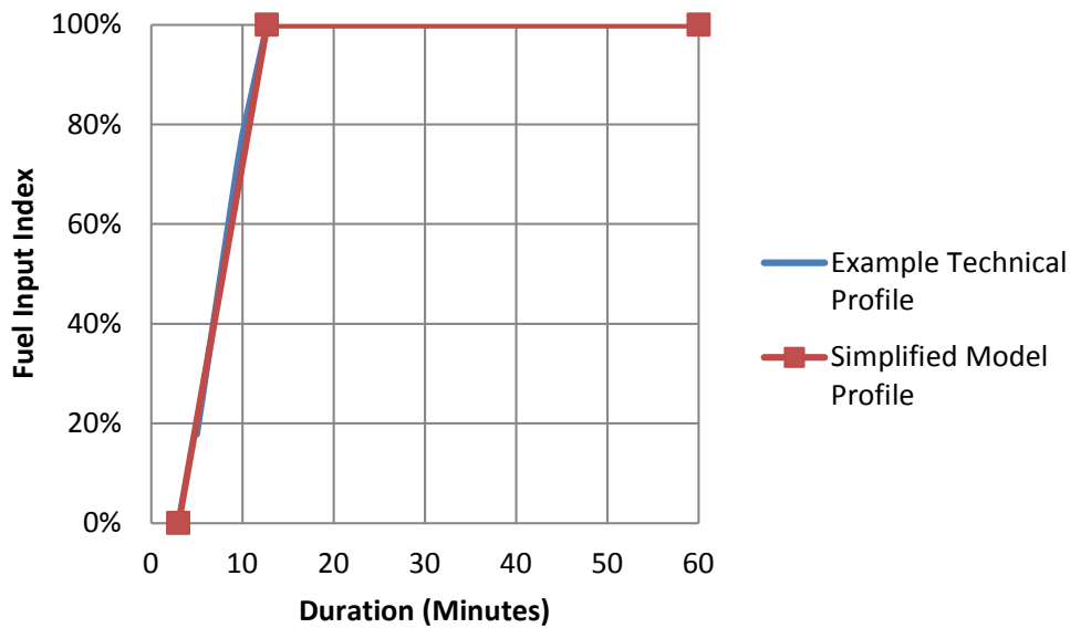
Figure 6. Small SCGT Generator Start-Up Fuel Input Profile
