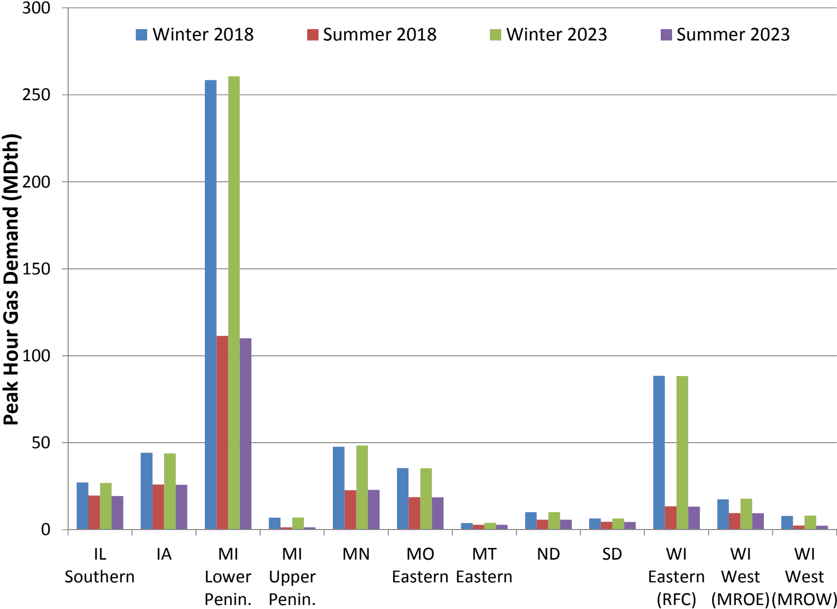
Figure E14-3. RGDS S0 RCI Peak Hour Gas Demand – MISO North/Central
