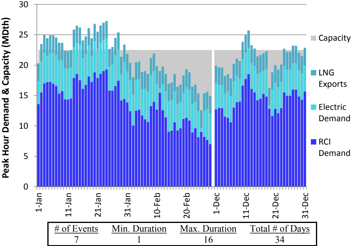
Figure U354. LGDS Roll-Up Winter 2023 – Dominion Southeast – Descending Demand
