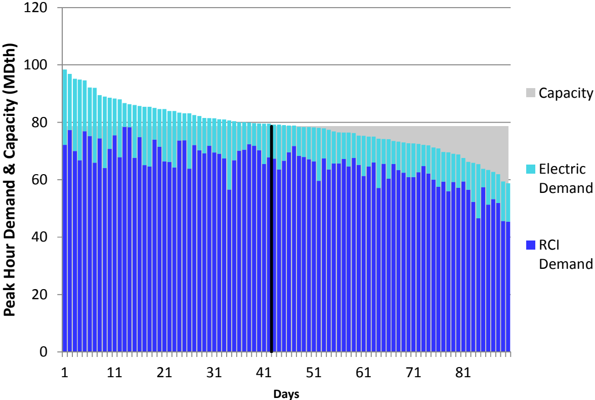
Figure U88. RGDS Roll-Up Winter 2023 – Tennessee Z4 PA – Descending Demand
