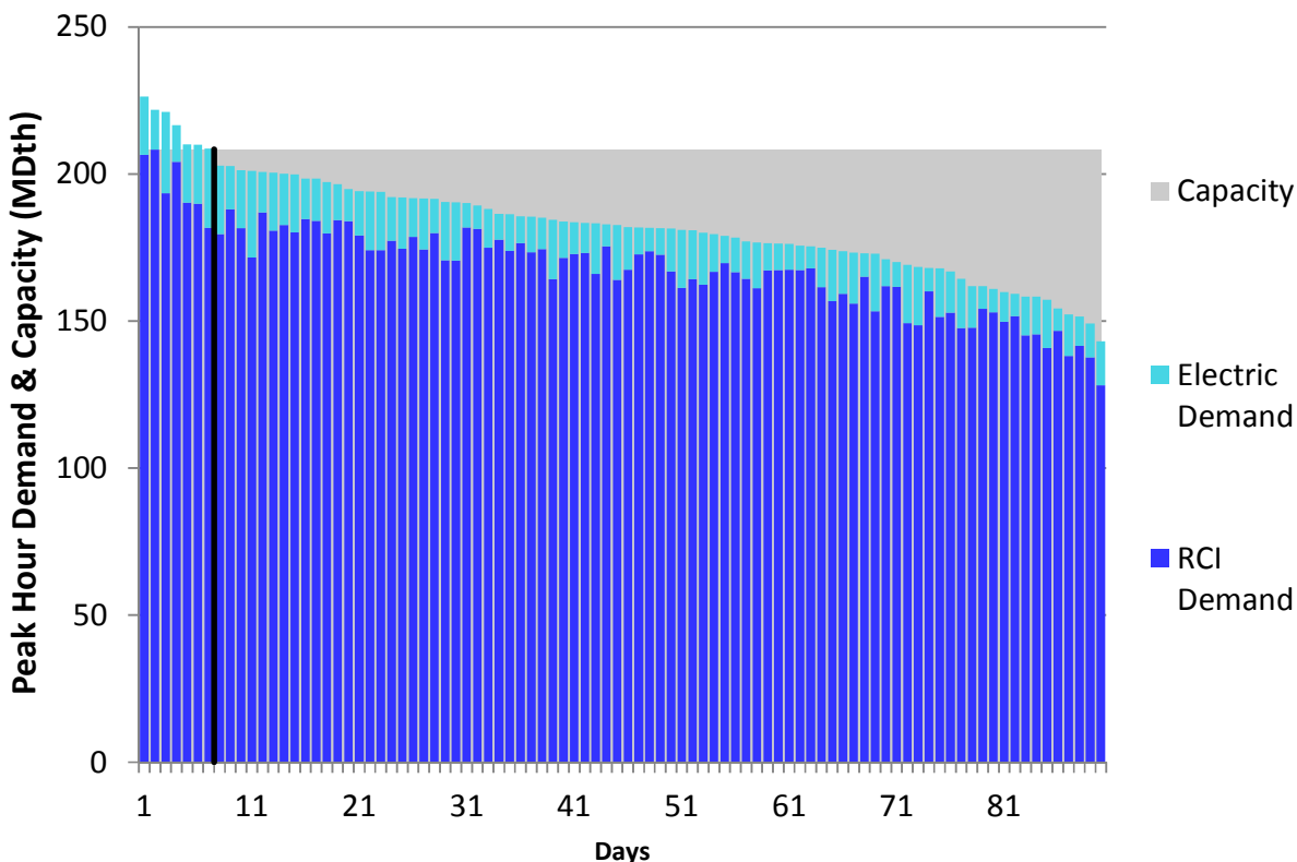
Figure U188. HGDS Roll-Up Winter 2018 – Union Gas Dawn – Descending Demand
