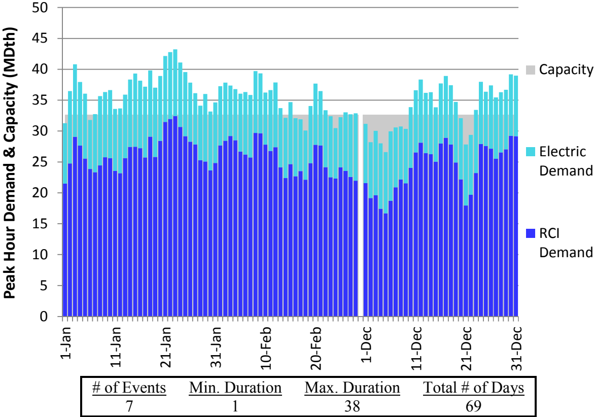
Figure U20. RGDS Roll-Up Winter 2018 – Millennium – Descending Demand
