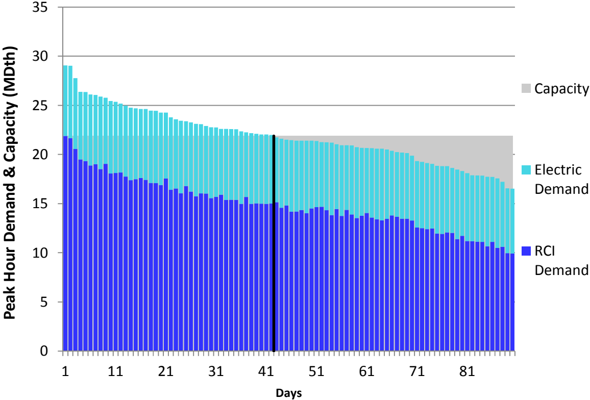
Figure U238. HGDS Roll-Up Winter 2023 – Empire – Descending Demand
