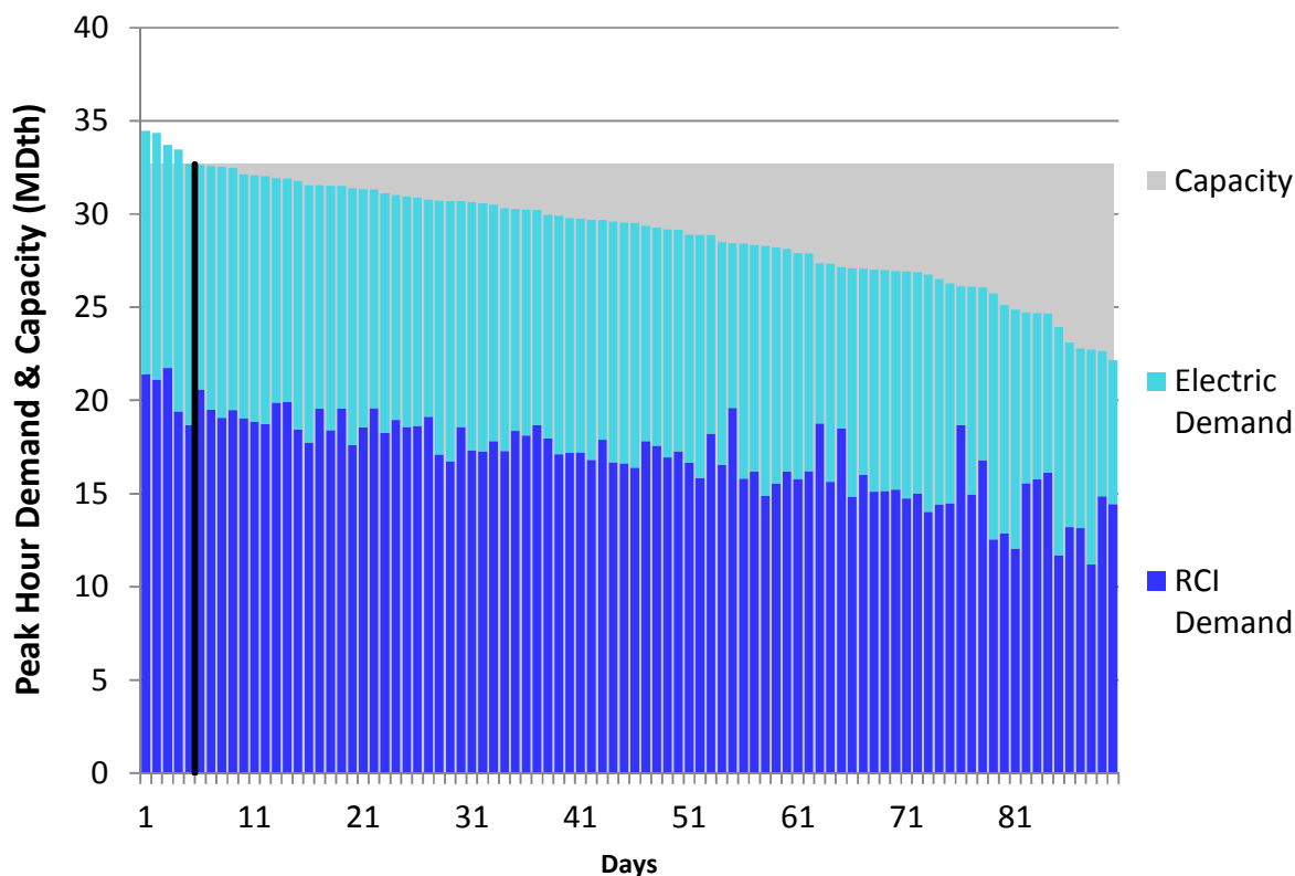
Figure U314. LGDS Roll-Up Winter 2018 – Millennium – Descending Demand
