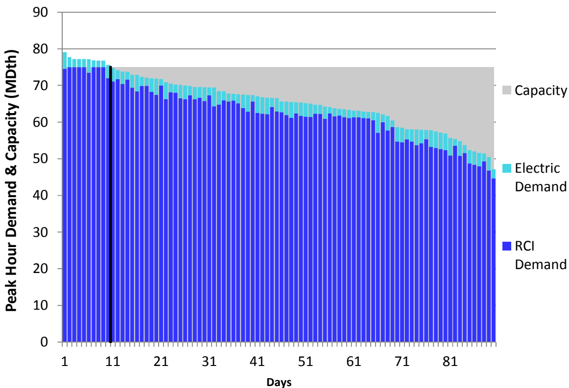
Figure U218. HGDS Roll-Up Winter 2023 – Alliance – Descending Demand
