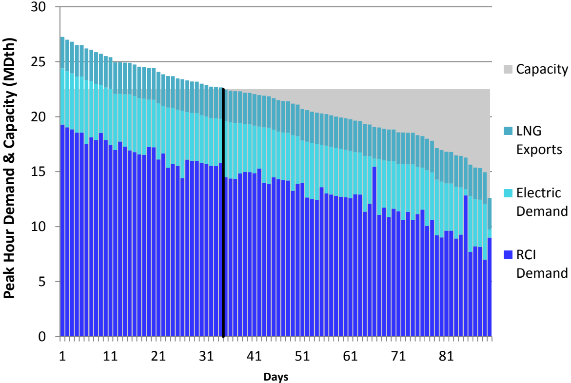
Figure U354. LGDS Roll-Up Winter 2023 – Dominion Southeast – Descending Demand
