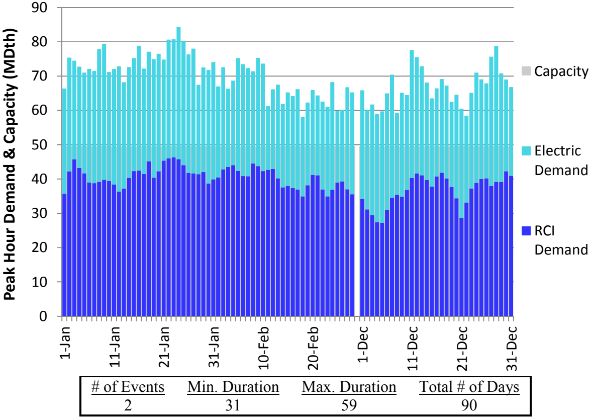
Figure U90. RGDS Roll-Up Winter 23 – Tennessee Z5 NY – Descending Demand
