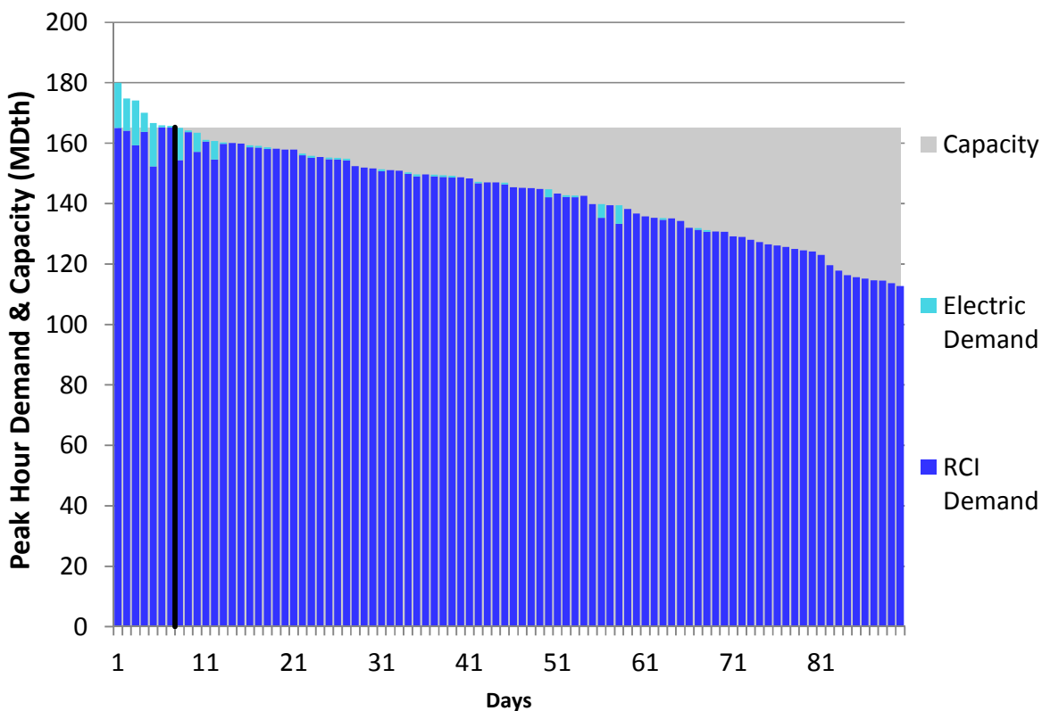
Figure U38. RGDS Roll-Up Winter 2018 – Transco Z5 – Descending Demand
