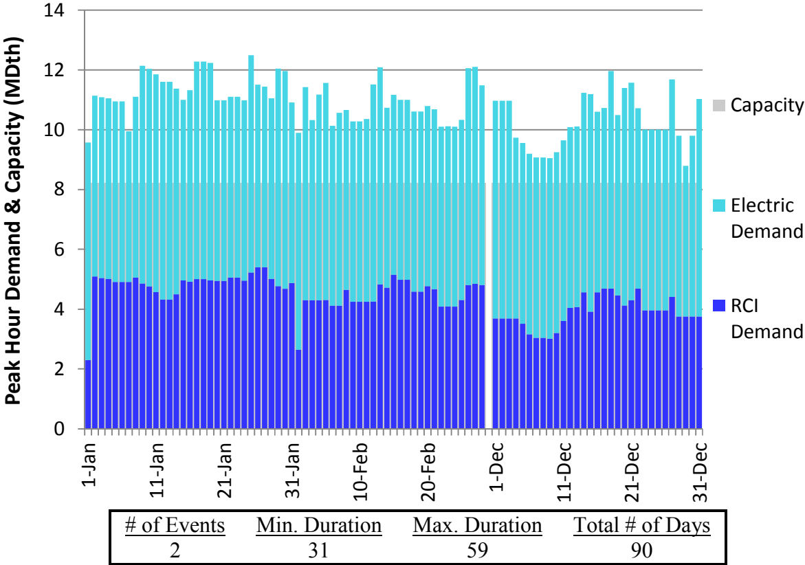
Figure U130. HGDS Roll-Up Winter 2018 – AlaTenn – Descending Demand
