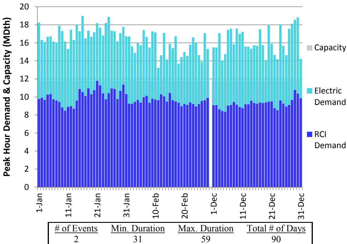
Figure U86. RGDS Roll-Up Winter 2023 – NB/NS – Descending Demand
