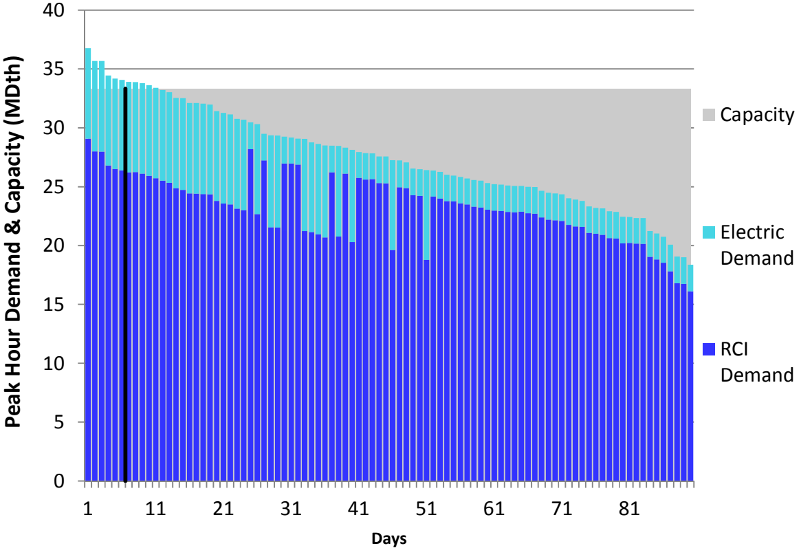
Figure U78. RGDS Roll-Up Winter 2023 – East Tennessee – Descending Demand
