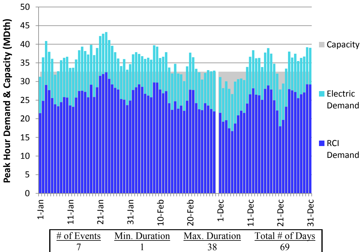
Figure U84. RGDS Roll-Up Winter 2023 – Millennium – Descending Demand
