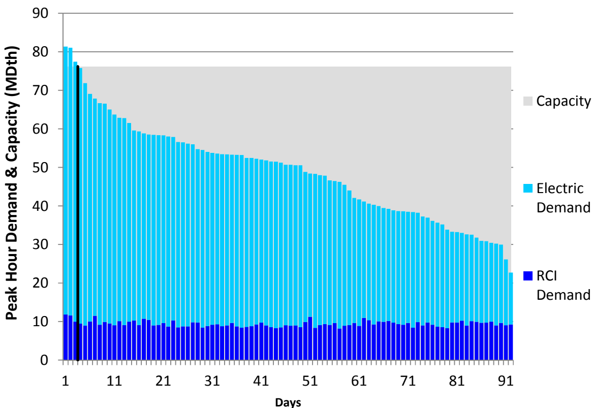
Figure U44. RGDS Roll-Up Summer 2018 – Algonquin CT – Descending Demand
