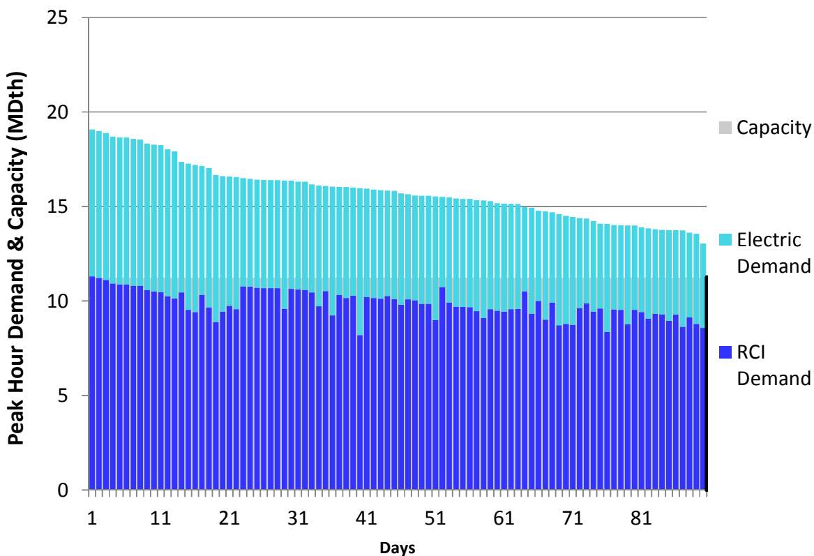
Figure U270. HGDS Roll-Up Winter 2023 – TransCanada Quebec to PNGTS – Descending Demand
