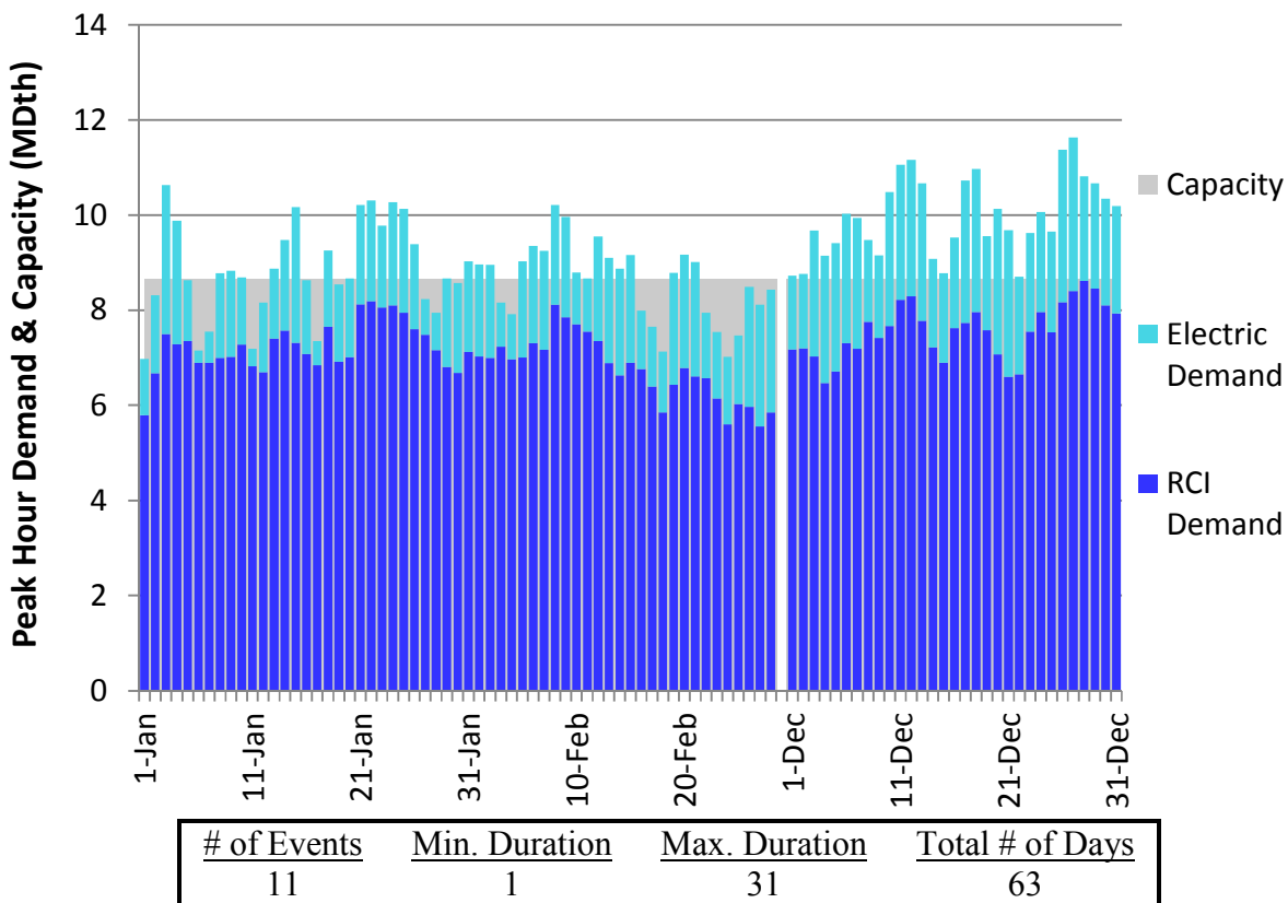
Figure U150. HGDS Roll-Up Winter 2018 – Eastern Shore – Descending Demand
