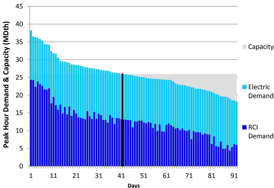
Figure U304. HGDS Roll-Up Summer 2023 – Texas Eastern ETX – Descending Demand
