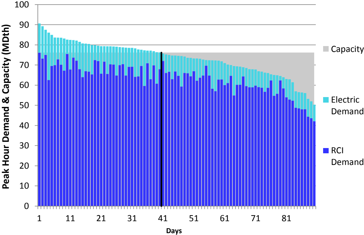
Figure U344. LGDS Roll-Up Winter 2023 – Algonquin CT – Descending Demand
