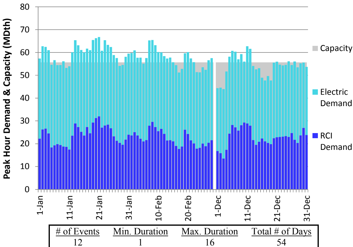
Figure U220. HGDS Roll-Up Winter 2023 – ANR Northern IL – Descending Demand
