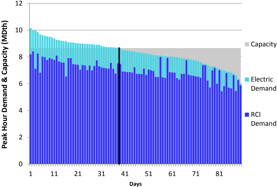
Figure U356. LGDS Roll-Up Winter 2023 – Eastern Shore – Descending Demand
