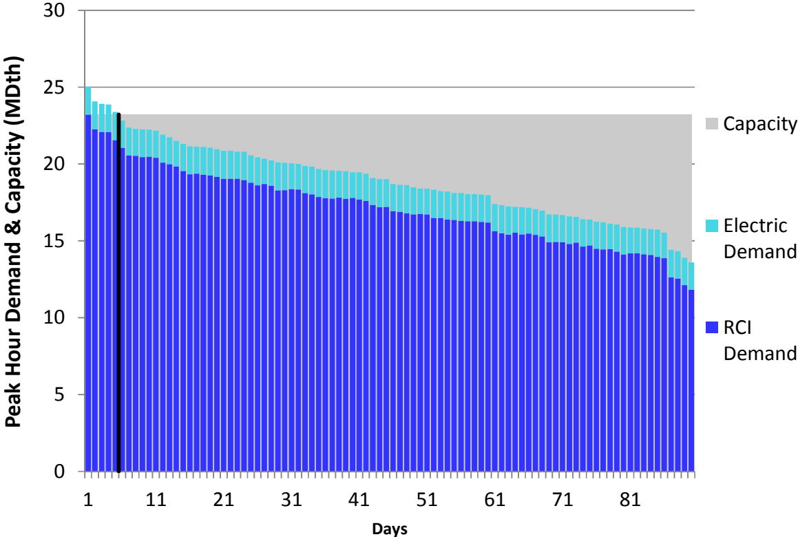
Figure U74. RGDS Roll-Up Winter 2023 – Dominion Western NY– Descending Demand
