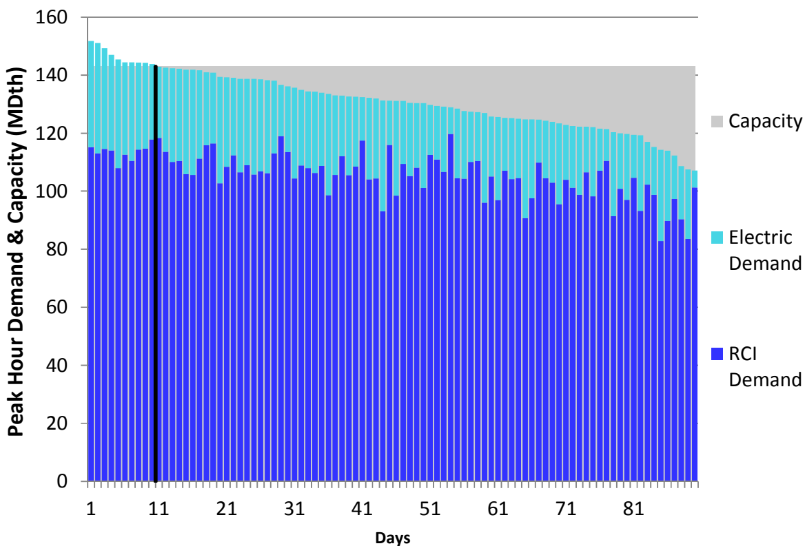
Figure U376. LGDS Roll-Up Winter 2023 – Transco Leidy to Station 210 – Descending Demand
