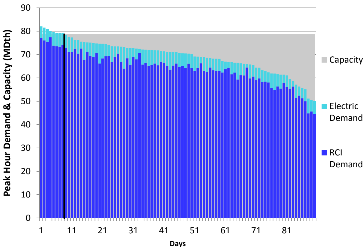
Figure U362. LGDS Roll-Up Winter 2023 – Tennessee Z4 PA – Descending Demand
