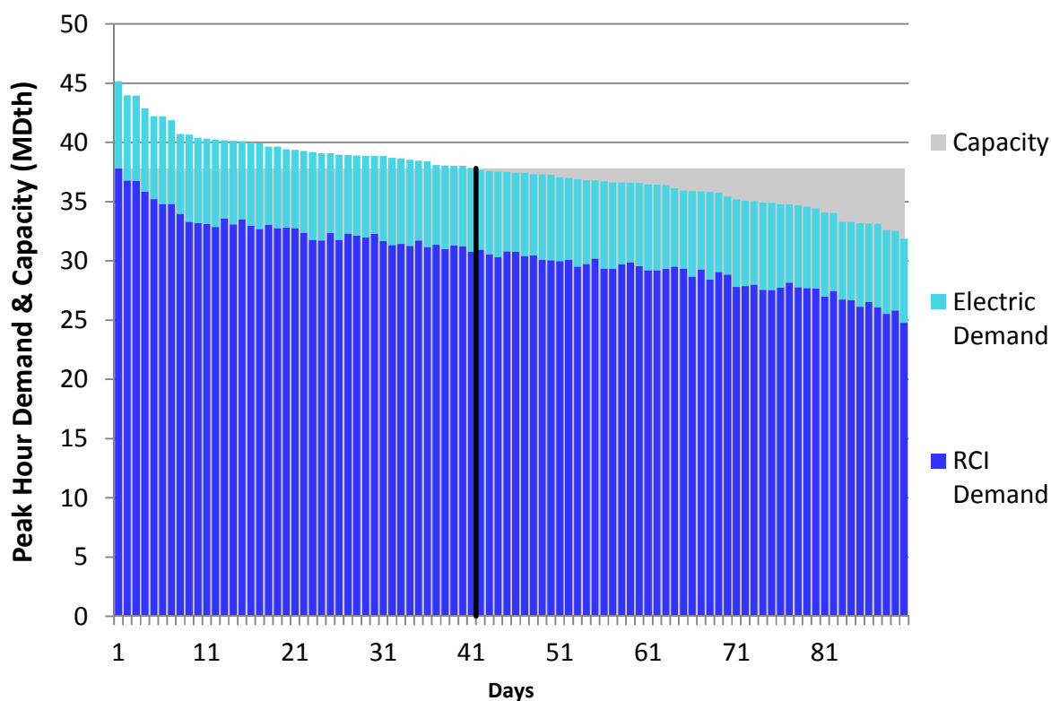
Figure U228. HGDS Roll-Up Winter 2023 – Dominion Eastern NY– Descending Demand
