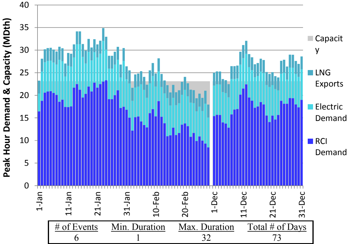
Figure U76. RGDS Roll-Up Winter 2023 – Dominion Southeast – Descending Demand
