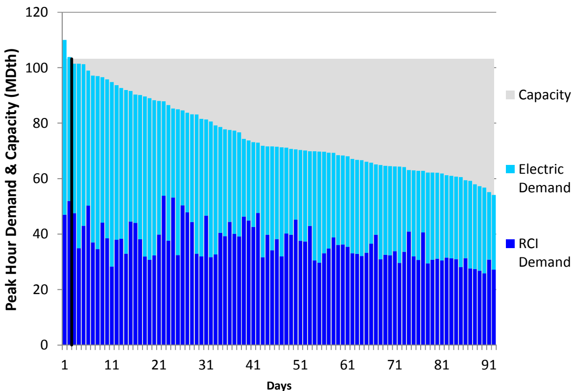
Figure U46. RGDS Roll-Up Summer 2018 – Columbia Gas VA/MD – Descending Demand
