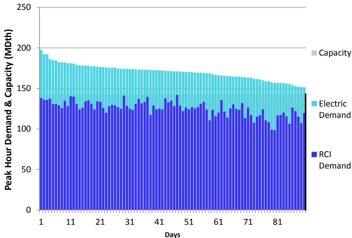
Figure U275. HGDS Roll-Up Winter 2023 – Transco Leidy to 210 – Chronological Demand
