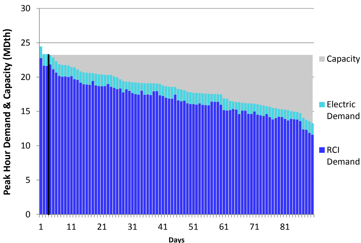
Figure U352. LGDS Roll-Up Winter 2023 – Dominion Western NY– Descending Demand
