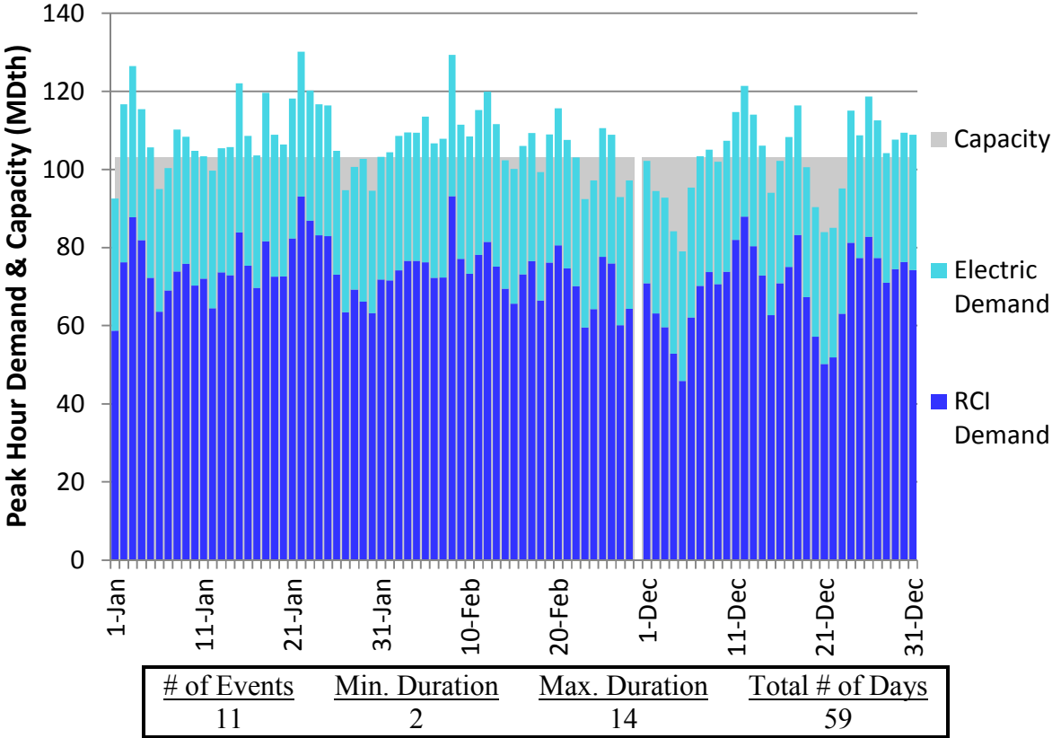
Figure U136. HGDS Roll-Up Winter 2018 – Columbia Gas VA/MD – Descending Demand
