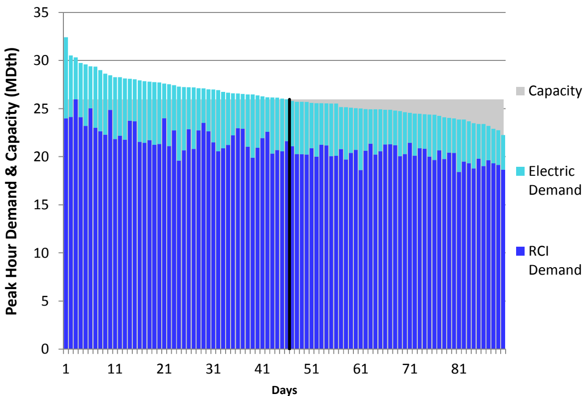
Figure U316. LGDS Roll-Up Winter 2018 – NB/NS – Descending Demand
