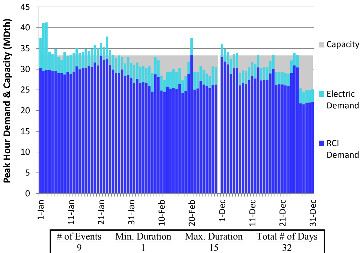
Figure U258. HGDS S34 Winter 2023 – Northern Natural Zone D – Descending Demand
