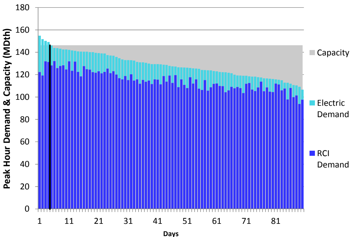
Figure U268. HGDS Roll-Up Winter 2023 – TransCanada Ontario West – Descending Demand
