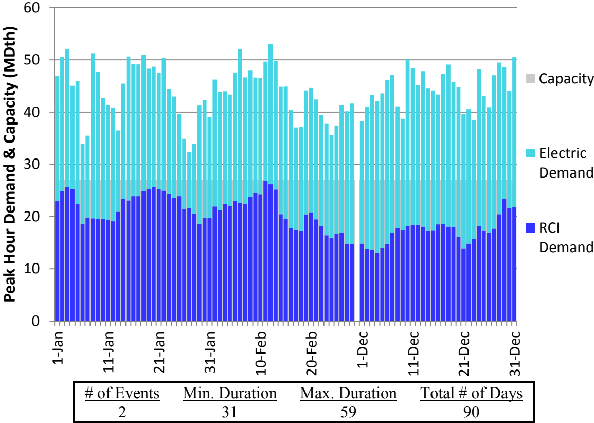
Figure U6. RGDS Roll-Up Winter 2018 – Constitution – Descending Demand
