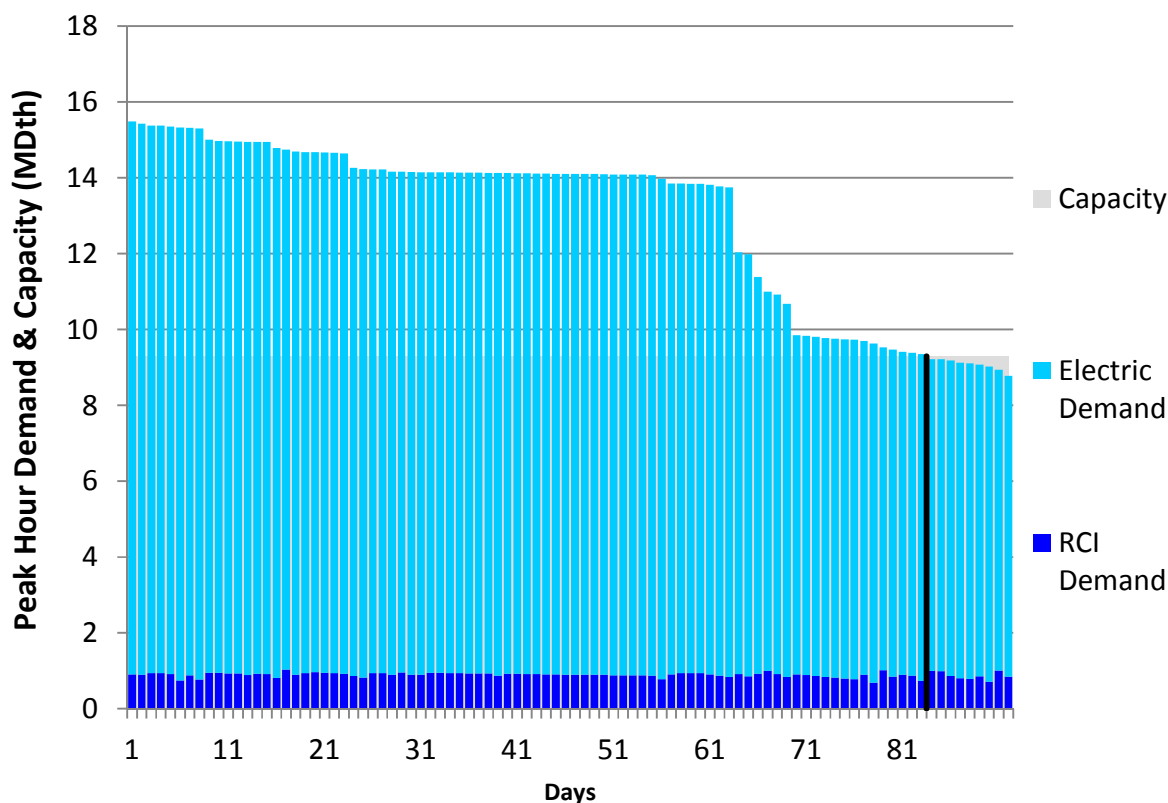
Figure U298. HGDS Roll-Up Summer 2023 – PNGTS N of Westbrook – Descending Demand
