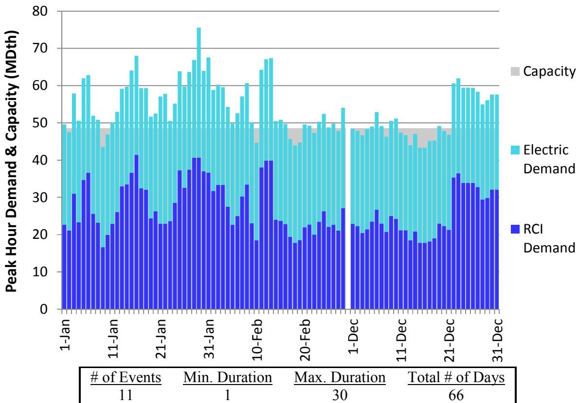
Figure U154. HGDS Roll-Up Winter 2018 – Great Lakes East – Descending Demand
