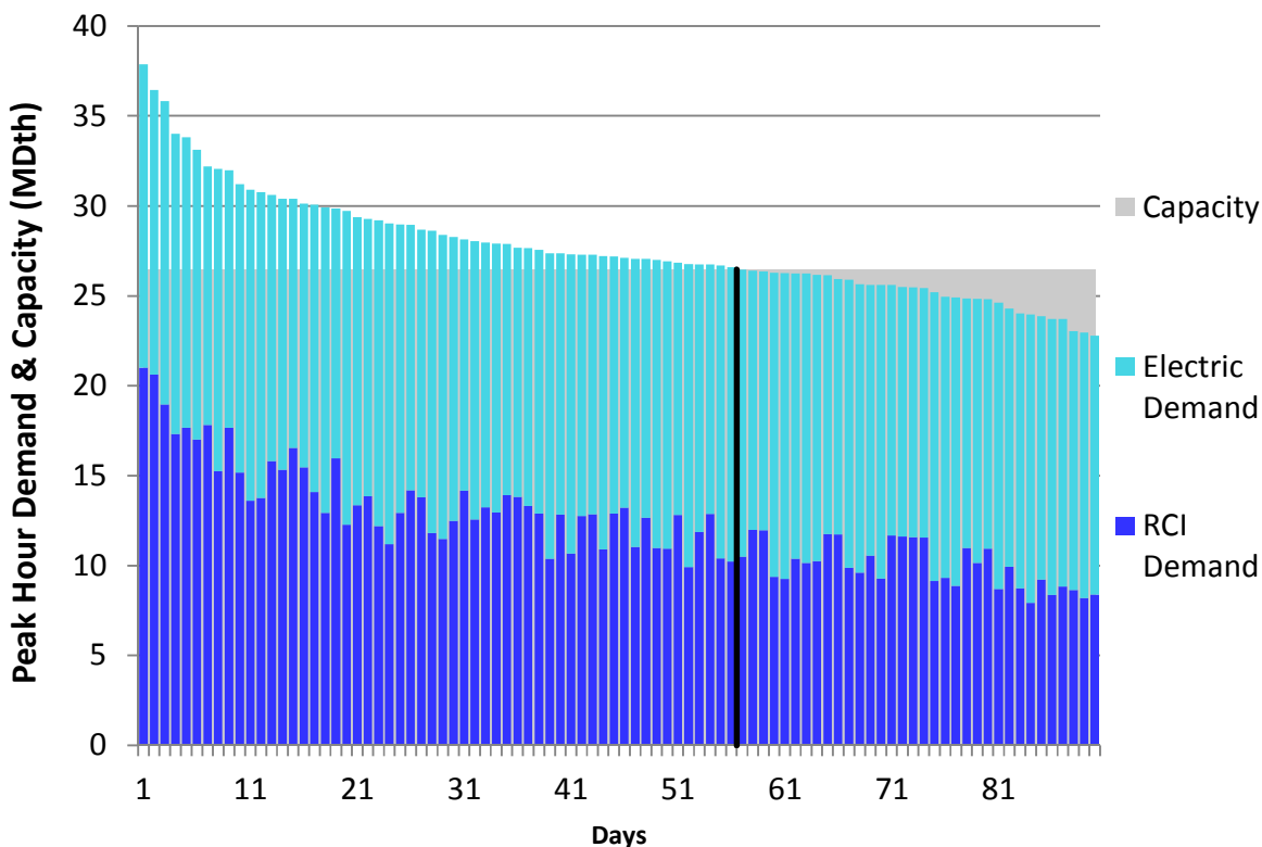
Figure U244. HGDS Roll-Up Winter 2023 – Midwestern – Descending Demand
