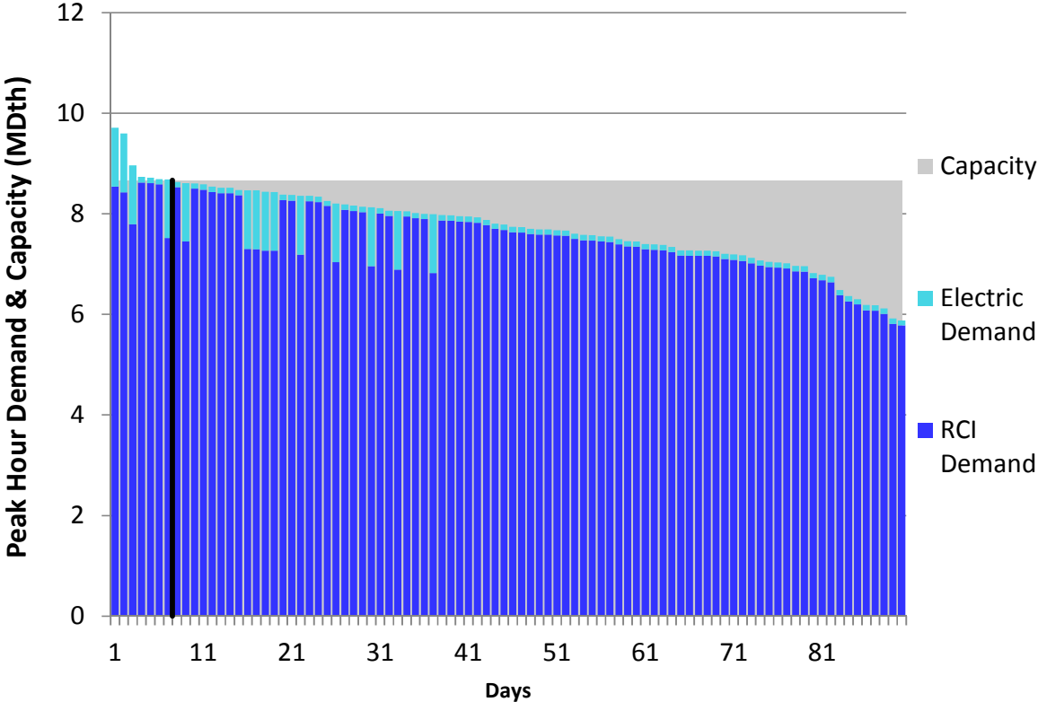
Figure U236. HGDS Roll-Up Winter 2023 – Eastern Shore – Descending Demand
