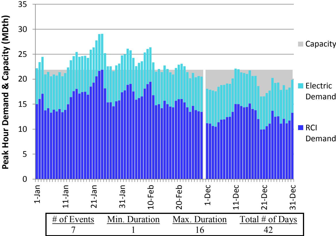
Figure U238. HGDS Roll-Up Winter 2023 – Empire – Descending Demand
