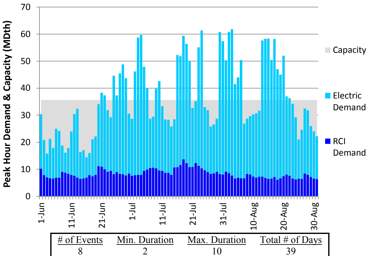
Figure U52. RGDS Roll-Up Summer 2018 – Iroquois Z1 → Z2 – Descending Demand
