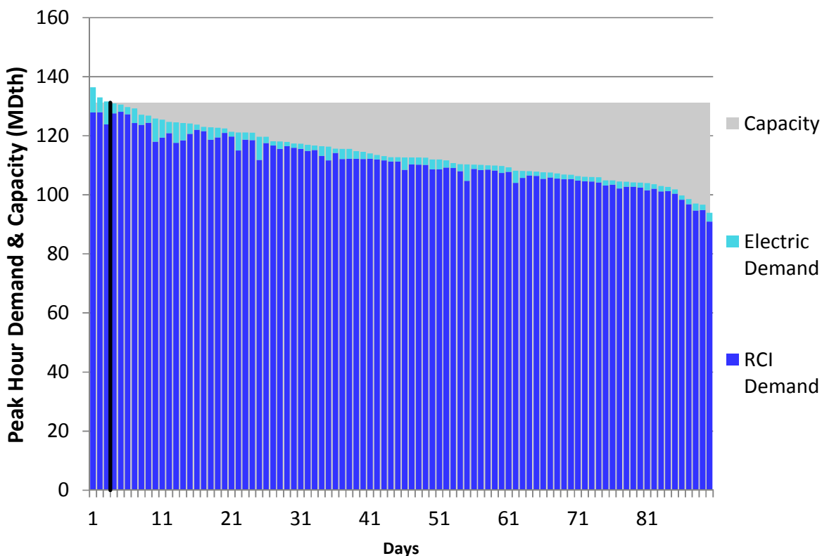
Figure U326. LGDS Roll-Up Winter 2018 – TransCanada Ontario West – Descending Demand
