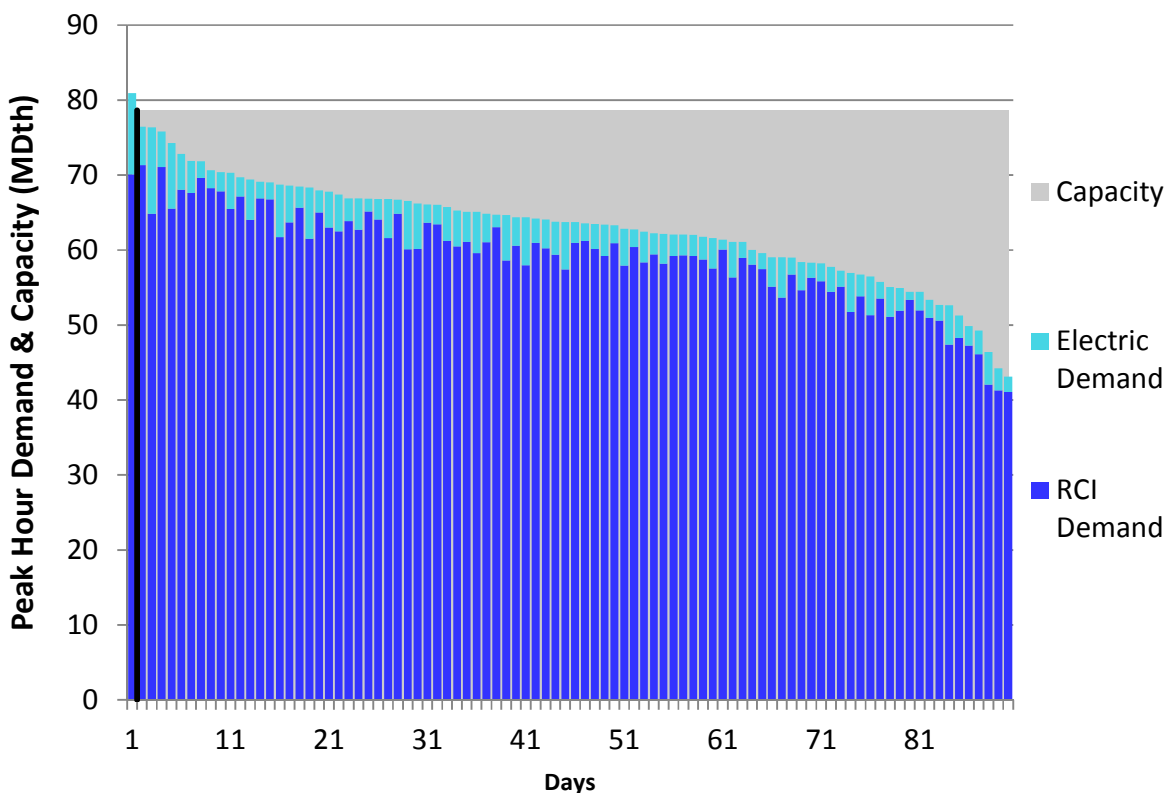
Figure U318. LGDS Roll-Up Winter 2018 – Tennessee Z4 PA – Descending Demand
