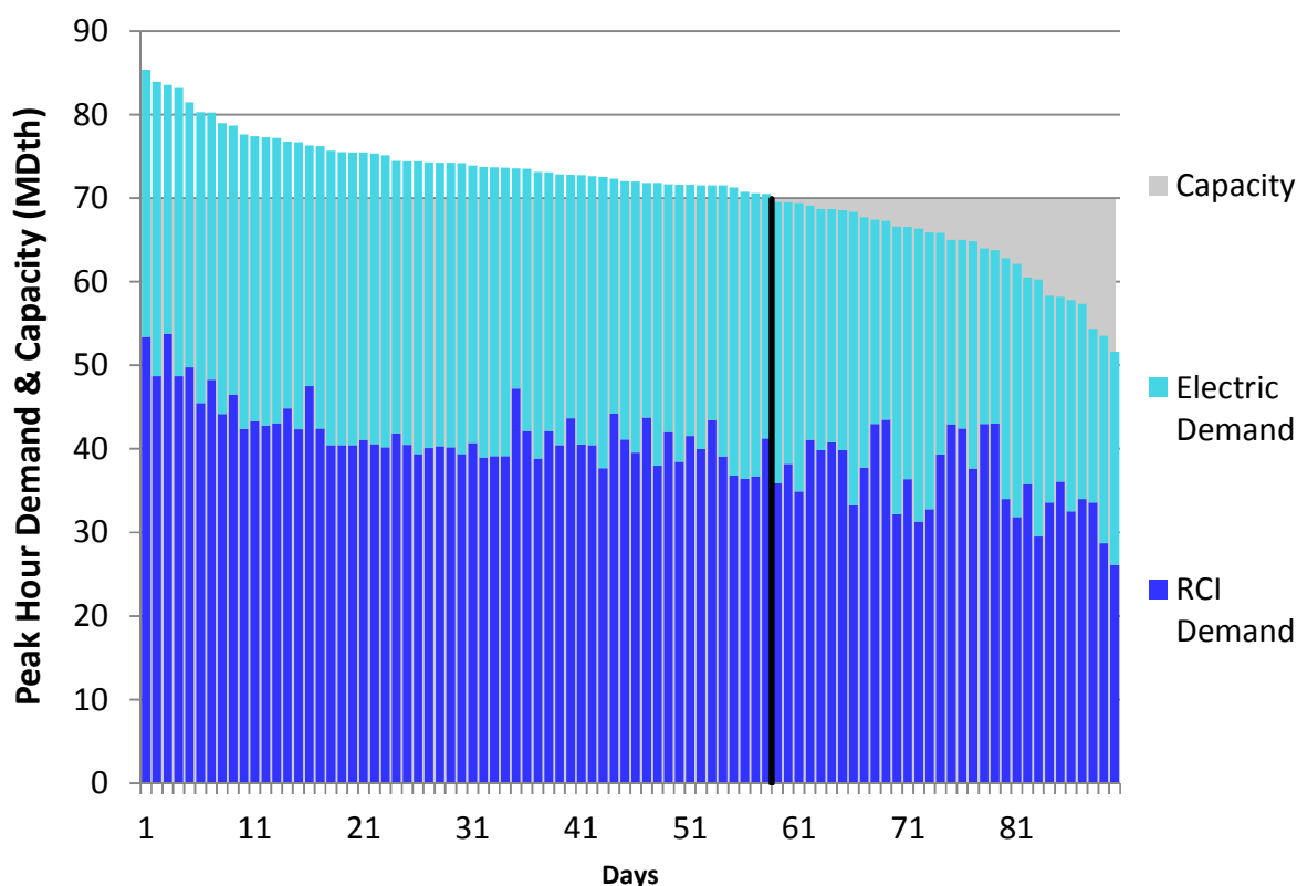
Figure U162. HGDS Roll-Up Winter 2018 – NGPL IA/IL North – Descending Demand
