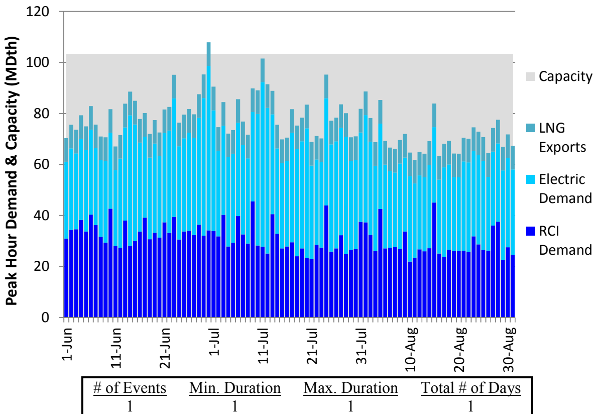
Figure U382. LGDS Roll-Up Summer 2023 – Columbia Gas VA/MD – Descending Demand
