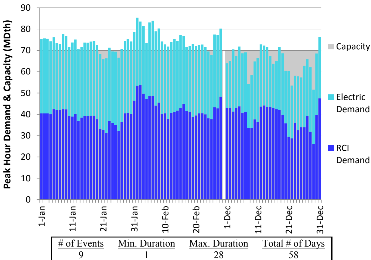
Figure U162. HGDS Roll-Up Winter 2018 – NGPL IA/IL North – Descending Demand
