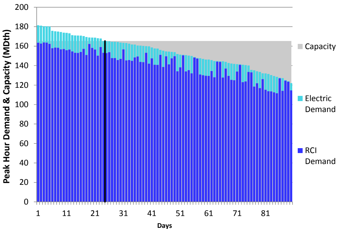
Figure U184. HGDS Roll-Up Winter 2018 – Transco Z5 – Descending Demand
