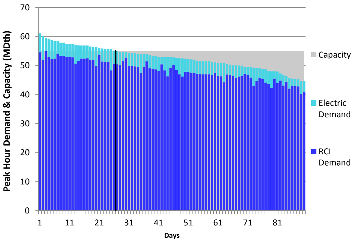
Figure U180. HGDS Roll-Up Winter 2018 – TransCanada Quebec – Descending Demand
