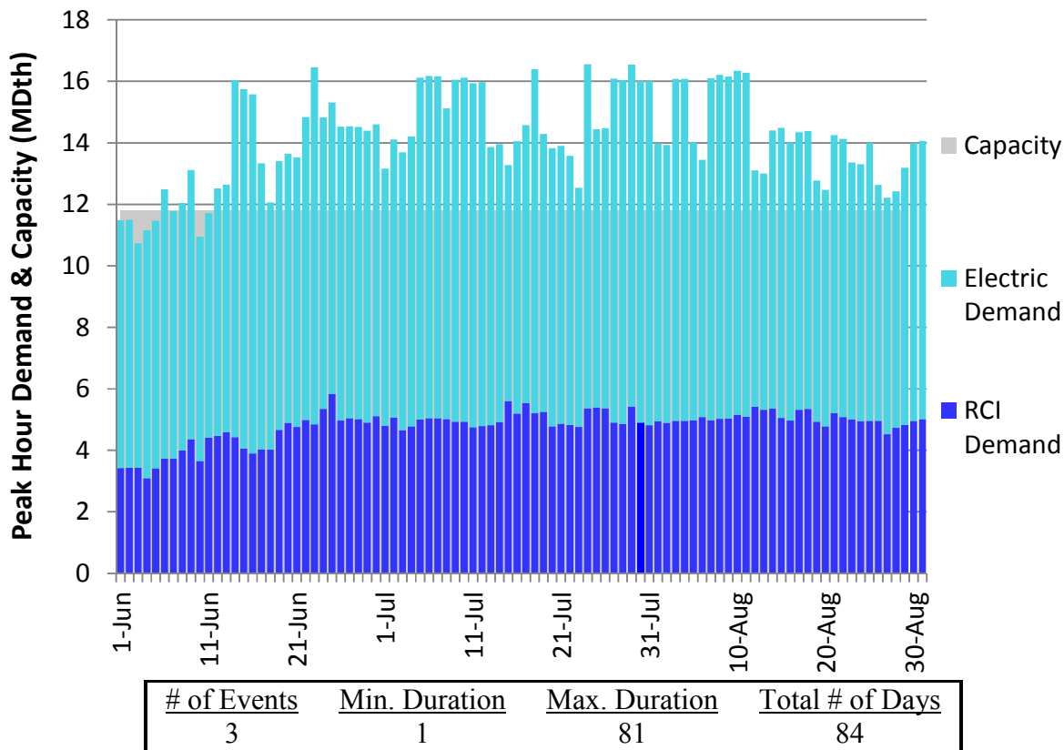
Figure U118. RGDS Roll-Up Summer 2023 – NB/NS Supply – Descending Demand
