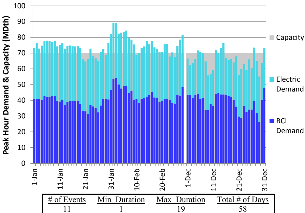
Figure U250. HGDS Roll-Up Winter 2023 – NGPL IA/IL North – Descending Demand
