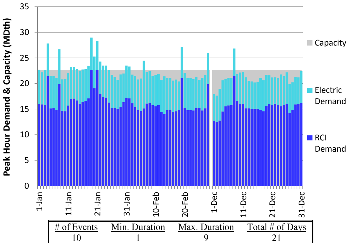
Figure U190. HGDS Roll-Up Winter 2018 – Viking Zone 1 – Descending Demand
