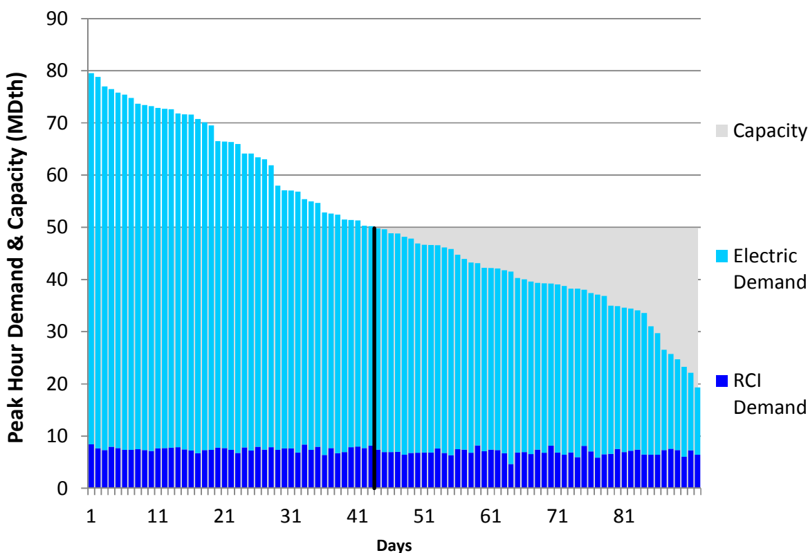
Figure U116. RGDS Roll-Up Summer 2018 – Iroquois Zone 1 – Descending Demand
