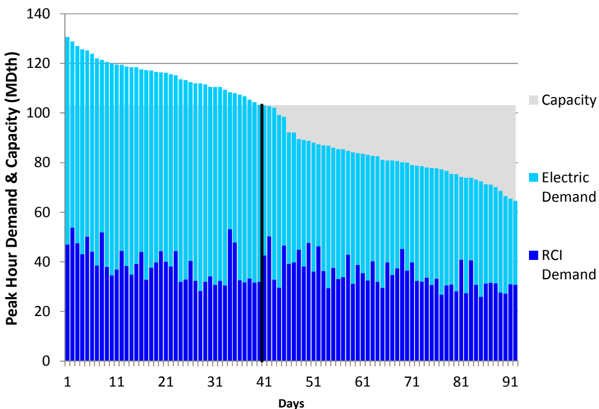
Figure U196. HGDS Roll-Up Summer 2018 – Columbia Gas VA/MD – Descending Demand
