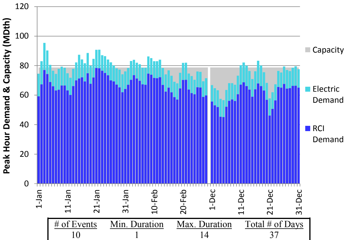
Figure U170. HGDS Roll-Up Winter 2018 – Tennessee Z4 PA – Descending Demand
