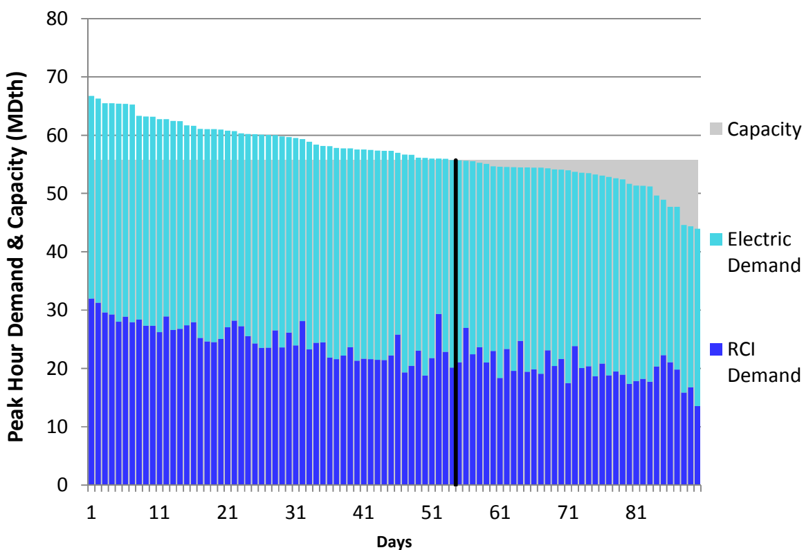
Figure U220. HGDS Roll-Up Winter 2023 – ANR Northern IL – Descending Demand
