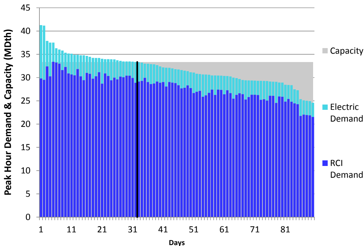
Figure U258. HGDS S34 Winter 2023 – Northern Natural Zone D – Descending Demand
