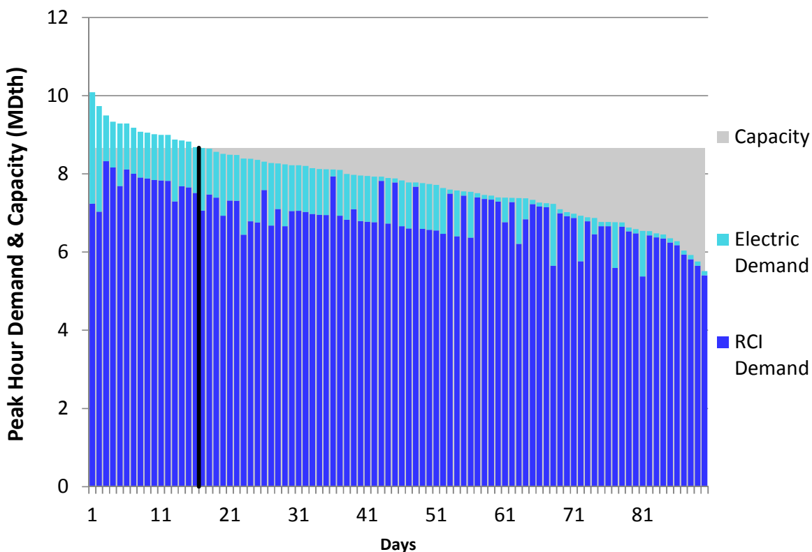
Figure U312. LGDS Roll-Up Winter 2018 – Eastern Shore – Descending Demand
