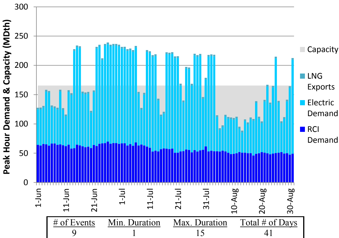
Figure U306. HGDS Roll-Up Summer 2023 – Transco Z5 – Descending Demand
