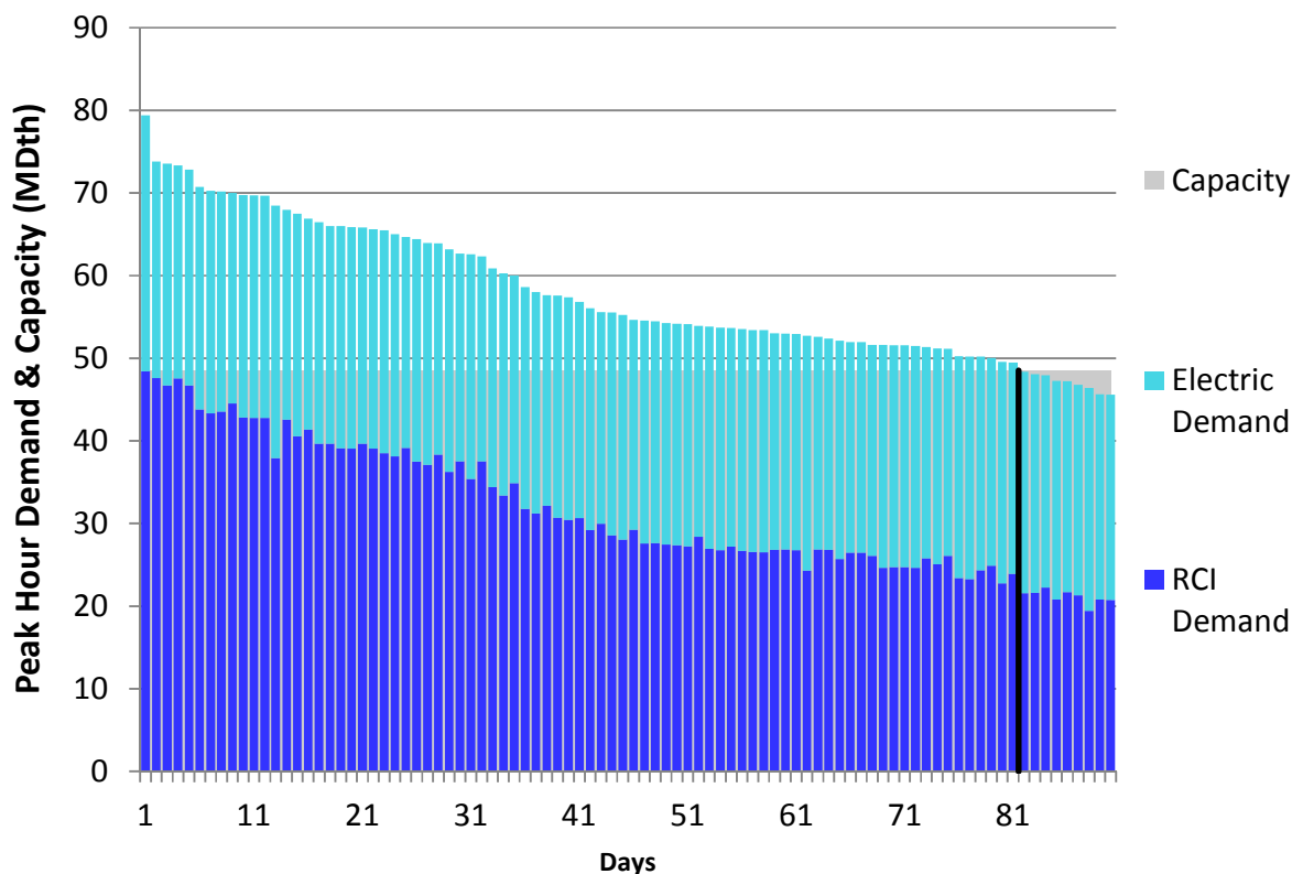
Figure U240. HGDS Roll-Up Winter 2023 – Great Lakes East – Descending Demand
