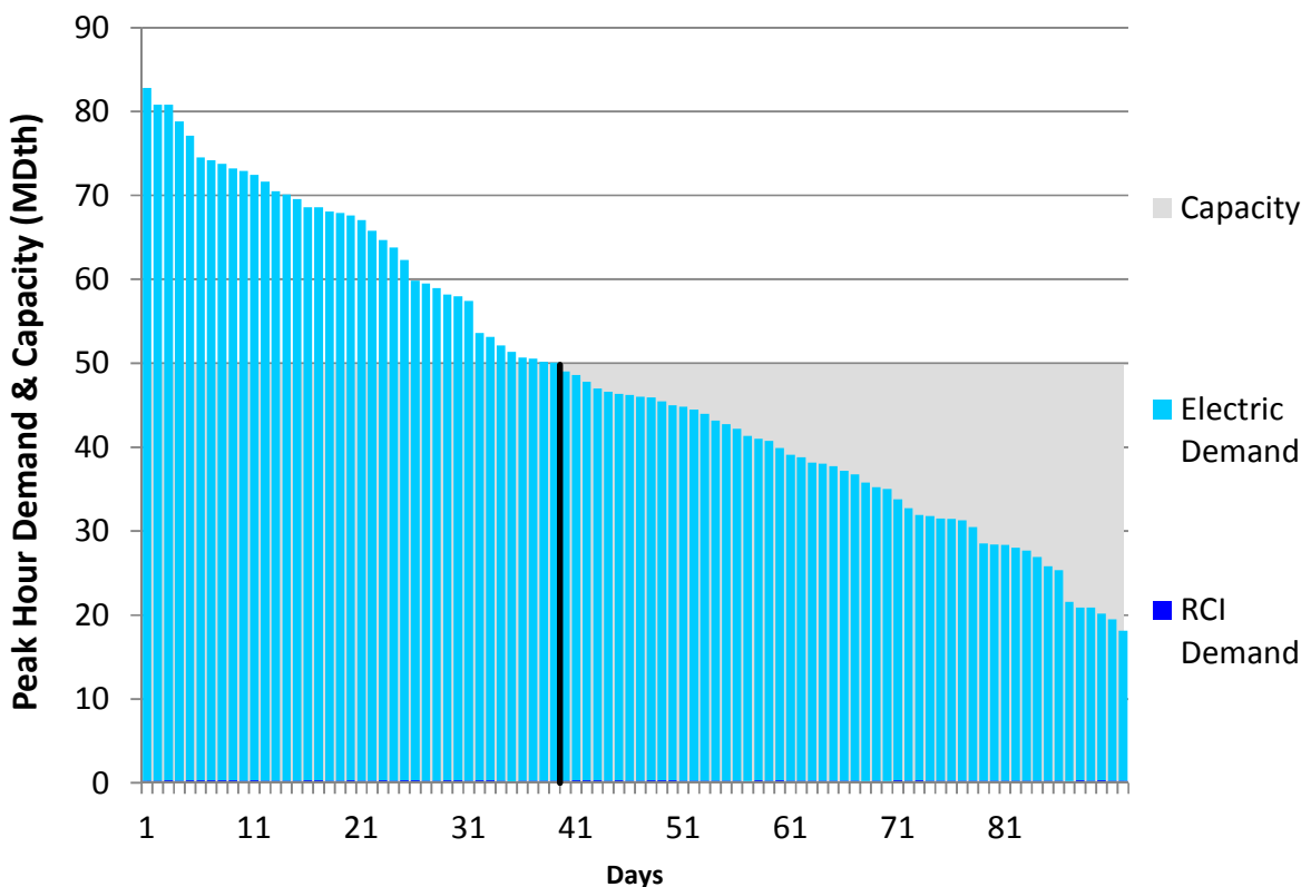
Figure U294. HGDS Roll-Up Summer 2023 – Iroquois Zone 1 – Descending Demand
