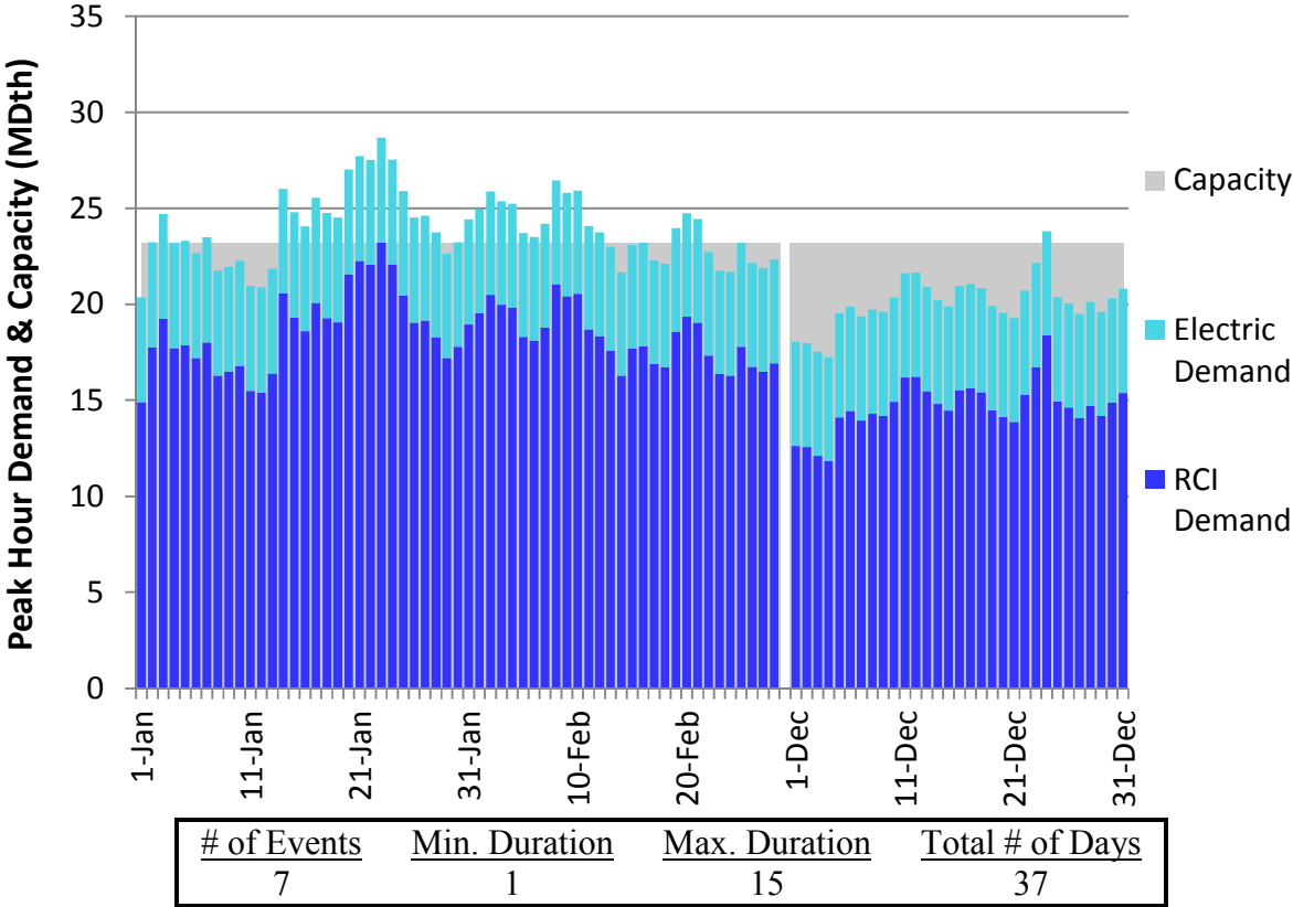
Figure U230. HGDS Roll-Up Winter 2023 – Dominion Western NY– Descending Demand
