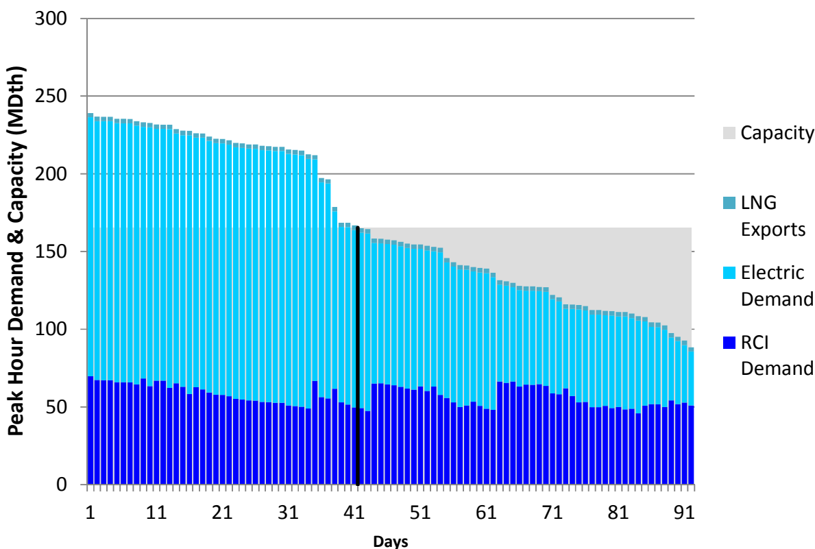
Figure U306. HGDS Roll-Up Summer 2023 – Transco Z5 – Descending Demand
