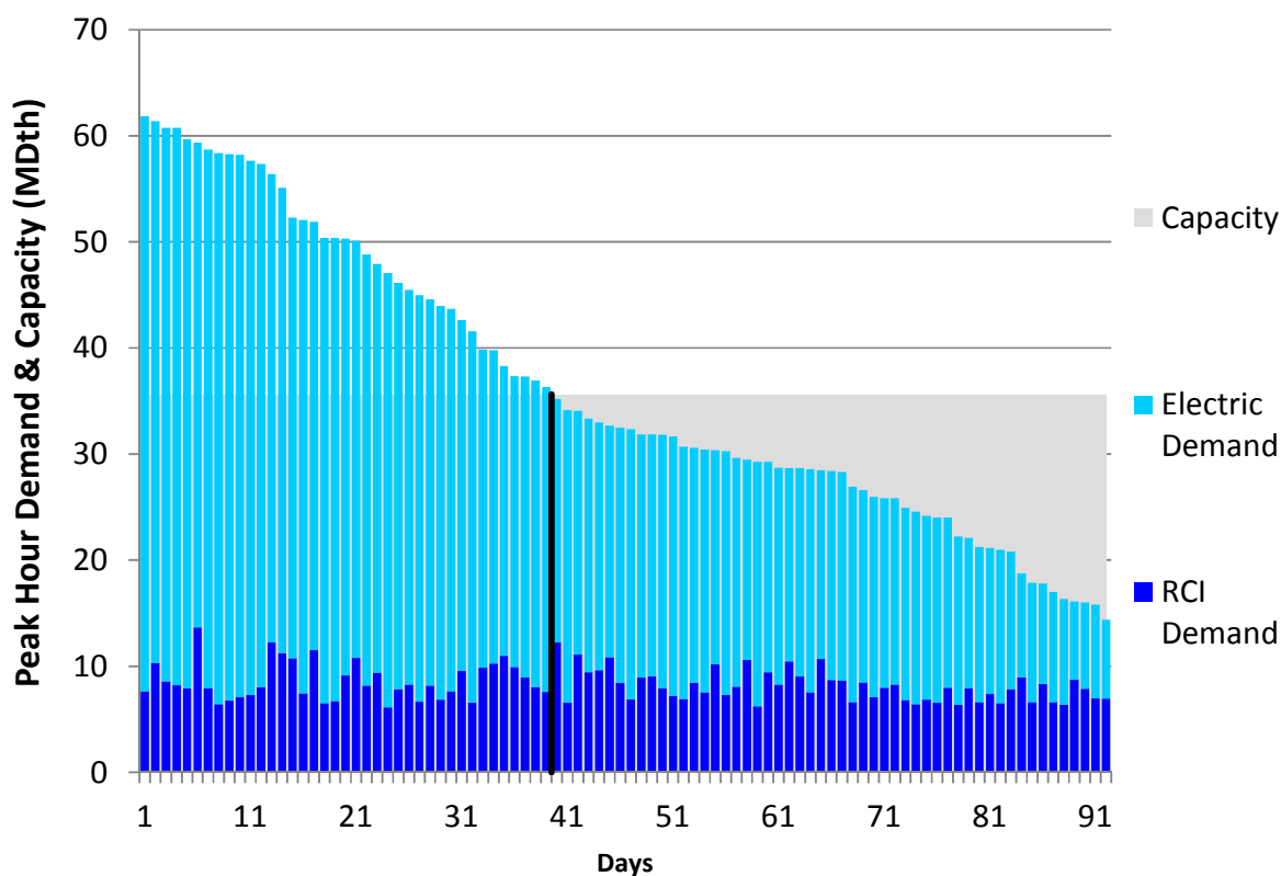
Figure U52. RGDS Roll-Up Summer 2018 – Iroquois Z1 → Z2 – Descending Demand
