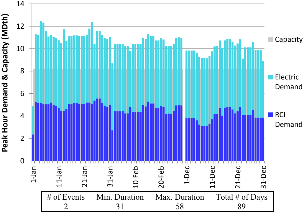
Figure U216. HGDS Roll-Up Winter 2023 – AlaTenn – Descending Demand
