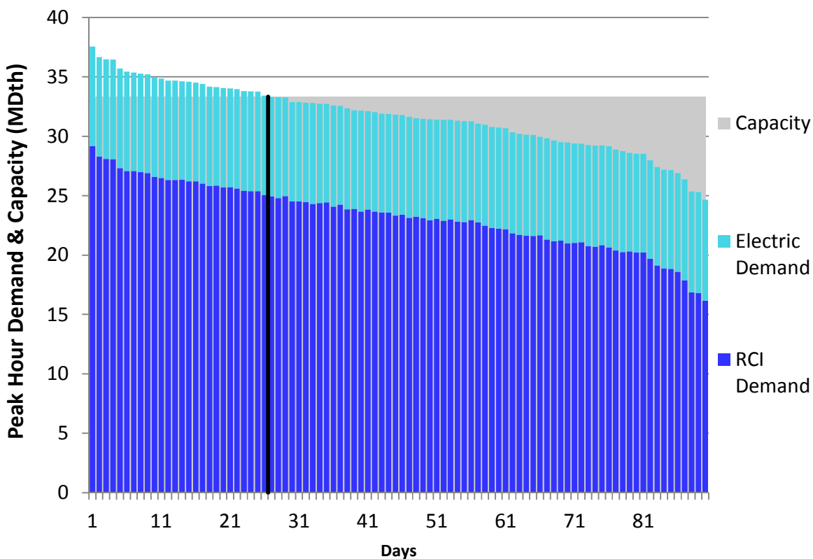
Figure U234. HGDS Roll-Up Winter 2023 – East Tennessee – Descending Demand
