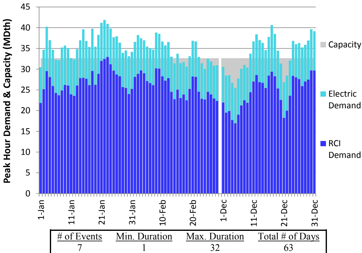
Figure U158. HGDS Roll-Up Winter 2018 – Millennium – Descending Demand
