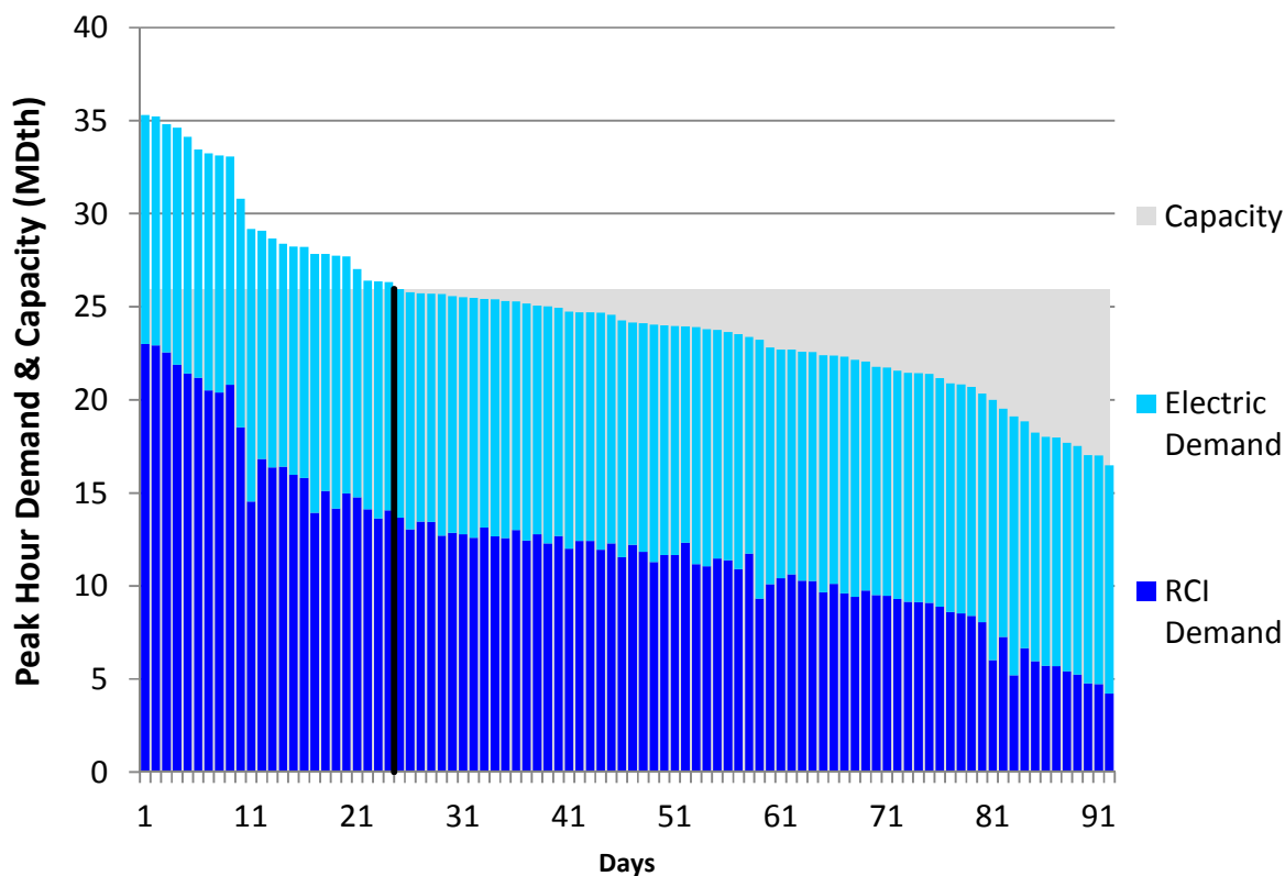
Figure U212. HGDS Roll-Up Summer 2018 – Texas Eastern ETX – Descending Demand
