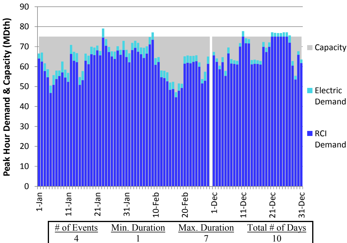
Figure U218. HGDS Roll-Up Winter 2023 – Alliance – Descending Demand
