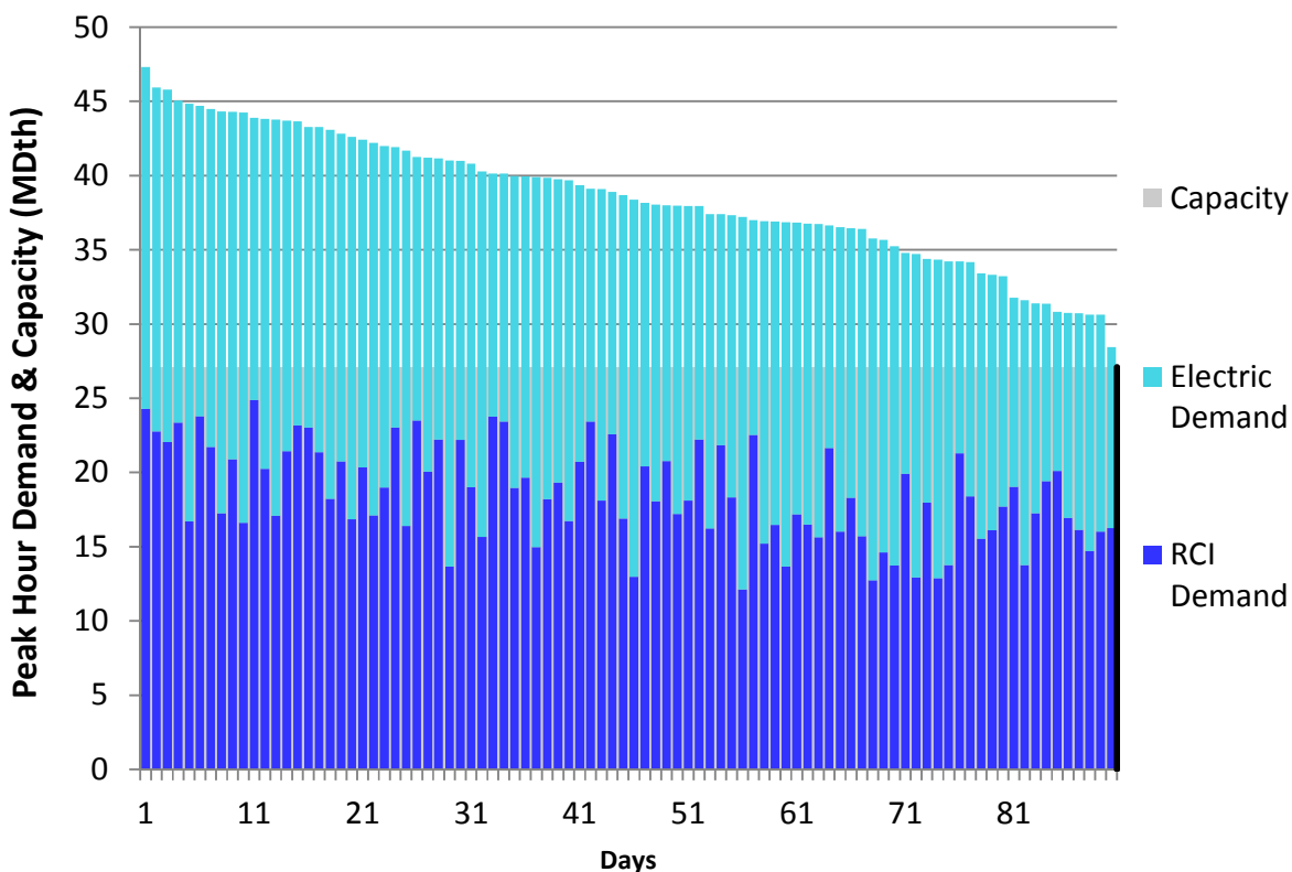
Figure U310. LGDS Roll-Up Winter 2018 – Constitution – Descending Demand
