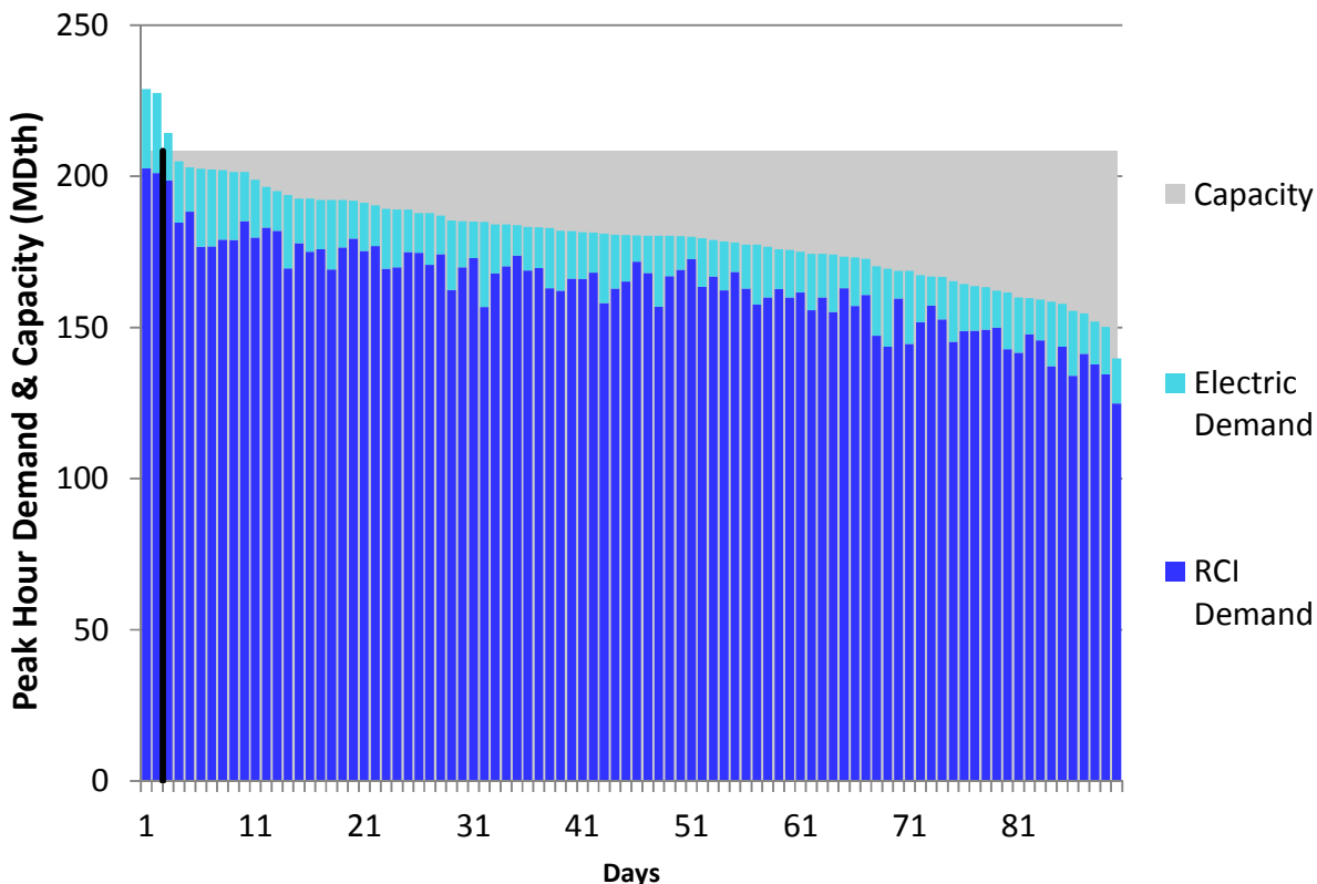
Figure U106. RGDS Roll-Up Winter 2023 – Union Gas Dawn – Descending Demand
