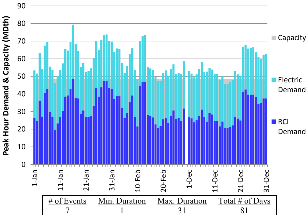
Figure U240. HGDS Roll-Up Winter 2023 – Great Lakes East – Descending Demand
