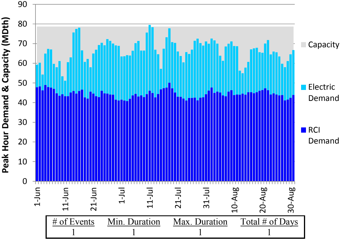
Figure U58. RGDS Roll-Up Summer 2018 – Tennessee Z4 PA – Descending Demand
