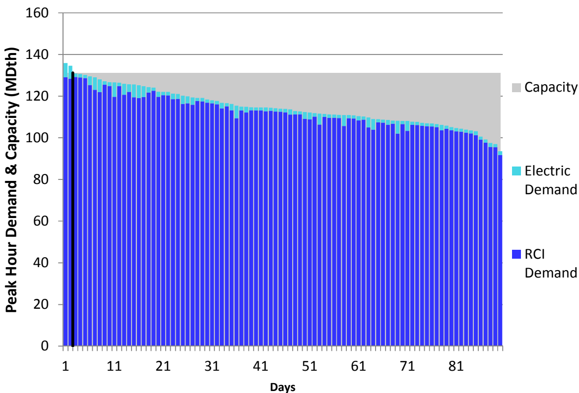
Figure U370. LGDS Roll-Up Winter 2023 – TransCanada Ontario West – Descending Demand
