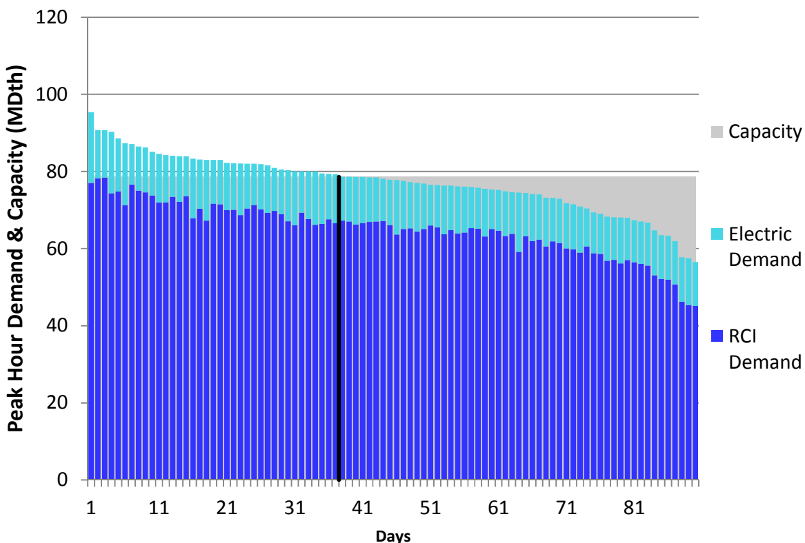
Figure U170. HGDS Roll-Up Winter 2018 – Tennessee Z4 PA – Descending Demand
