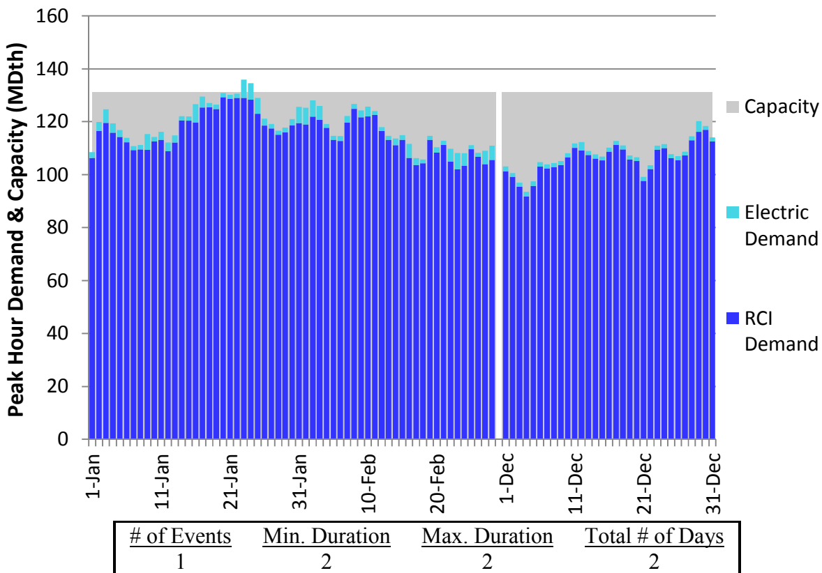
Figure U370. LGDS Roll-Up Winter 2023 – TransCanada Ontario West – Descending Demand
