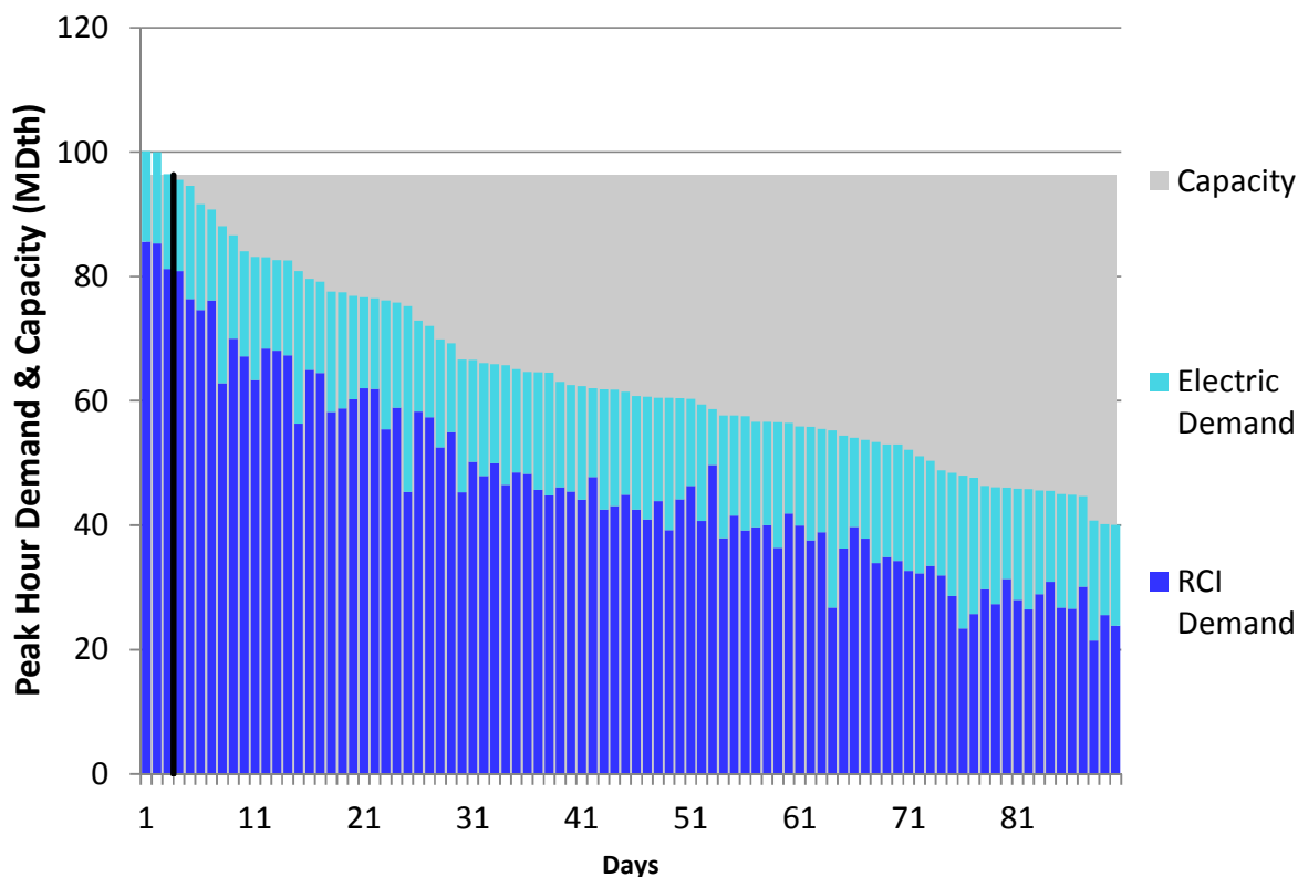
Figure U254. HGDS Roll-Up Winter 2023 – Northern Border Mainline – Descending Demand
