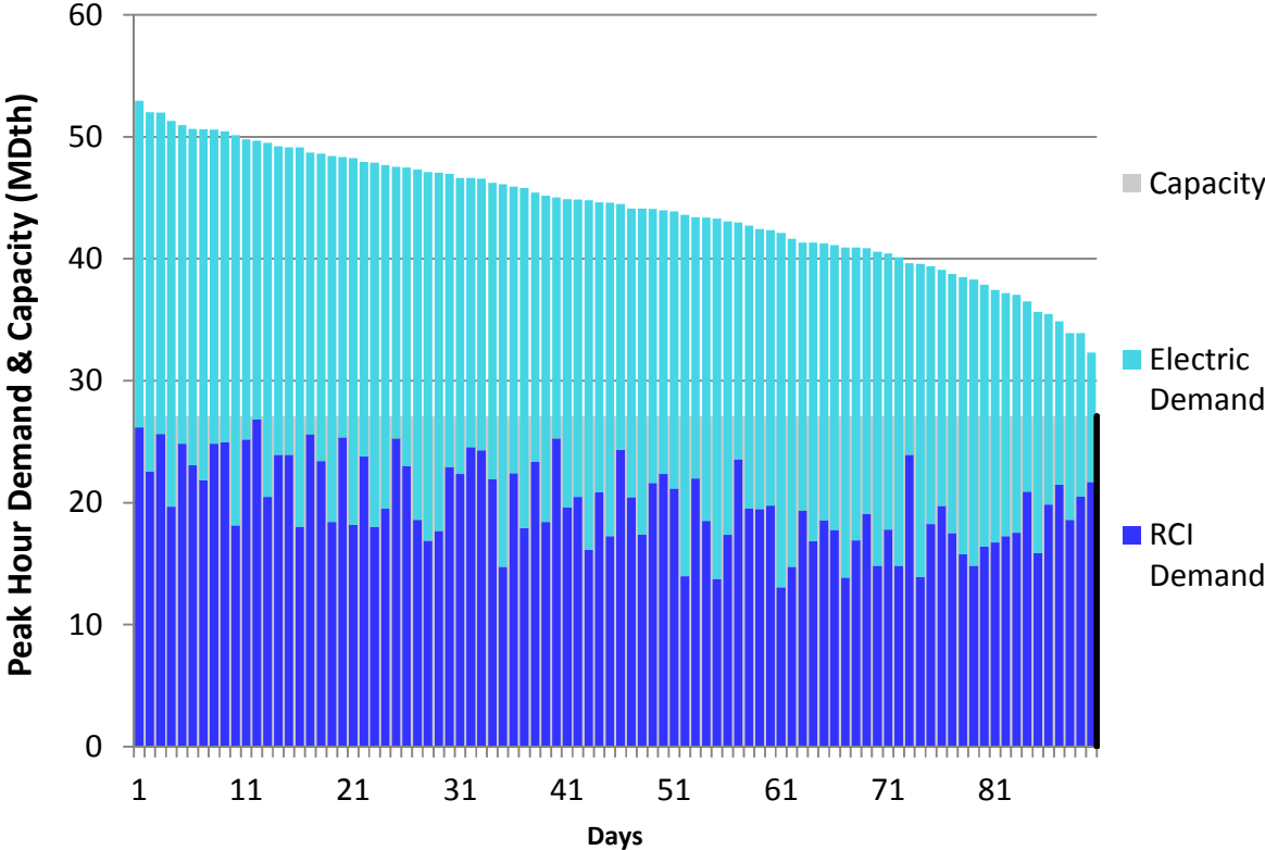
Figure U6. RGDS Roll-Up Winter 2018 – Constitution – Descending Demand
