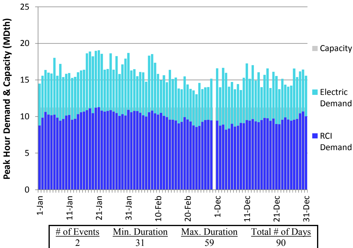
Figure U270. HGDS Roll-Up Winter 2023 – TransCanada Quebec to PNGTS – Descending Demand
