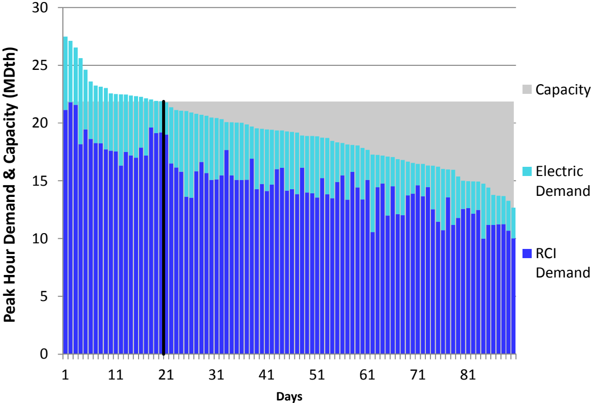
Figure U18. RGDS Roll-Up Winter 2018 – Empire – Descending Demand
