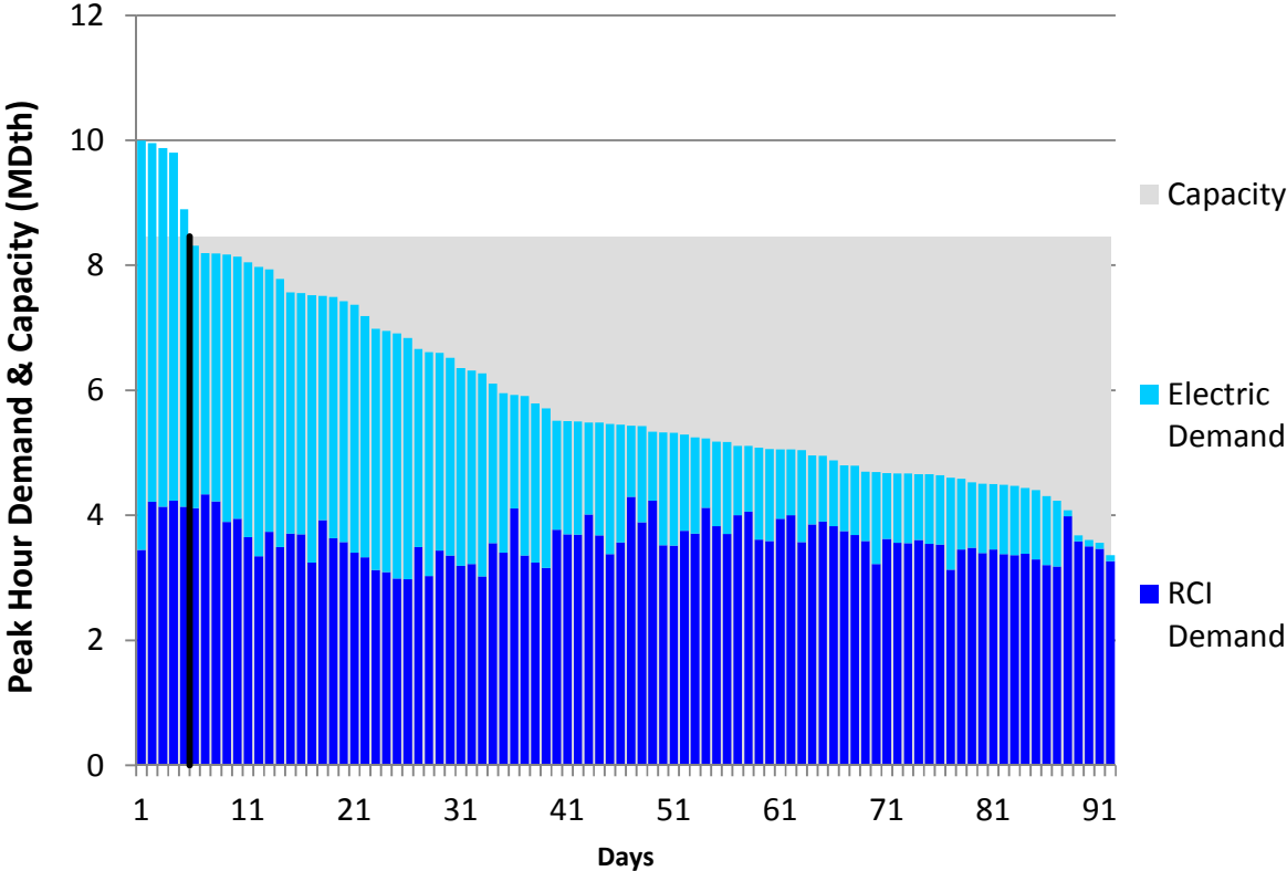
Figure U50. RGDS Roll-Up Summer 2018 – Eastern Shore – Descending Demand
