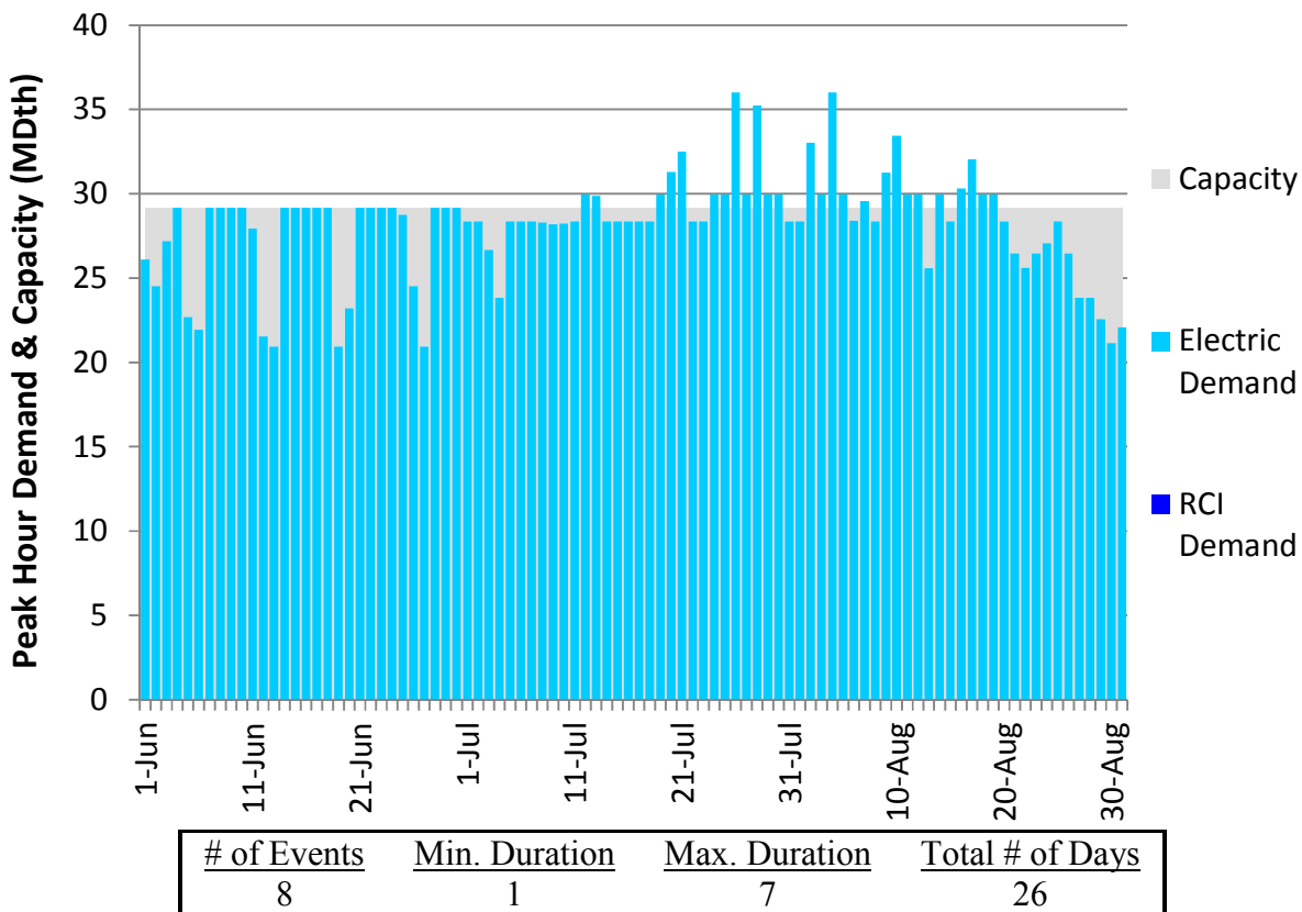
Figure U292. HGDS Roll-Up Summer 23 – Gulf South Z2 HH – Descending Demand
