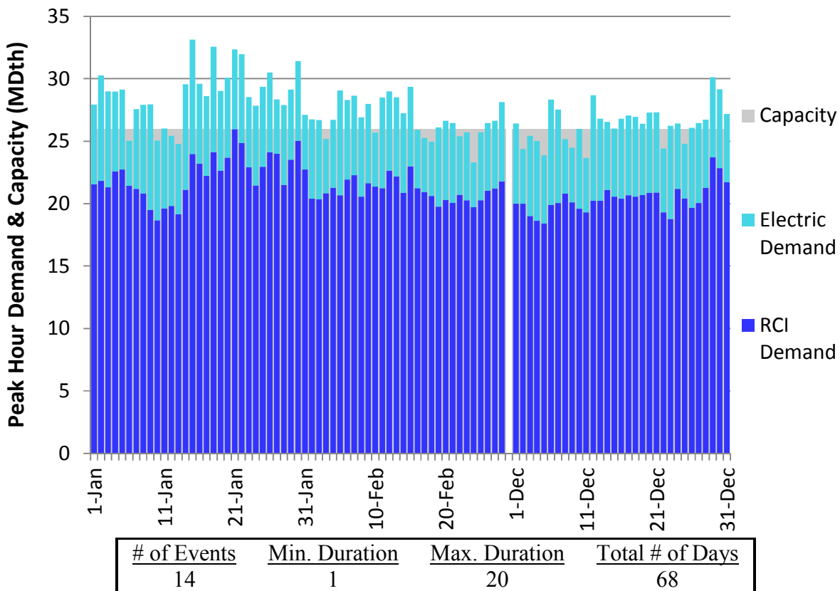
Figure U160. HGDS Roll-Up Winter 2018 – NB/NS Supply – Descending Demand
