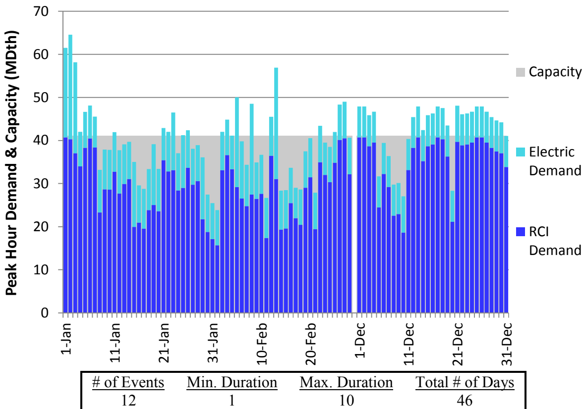
Figure U166. HGDS Roll-Up Winter 2018 – Northern Border Chicago – Descending Demand
