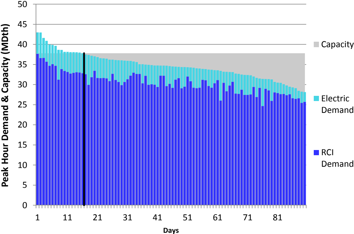
Figure U8. RGDS Roll-Up Winter 2018 – Dominion Eastern NY– Descending Demand
