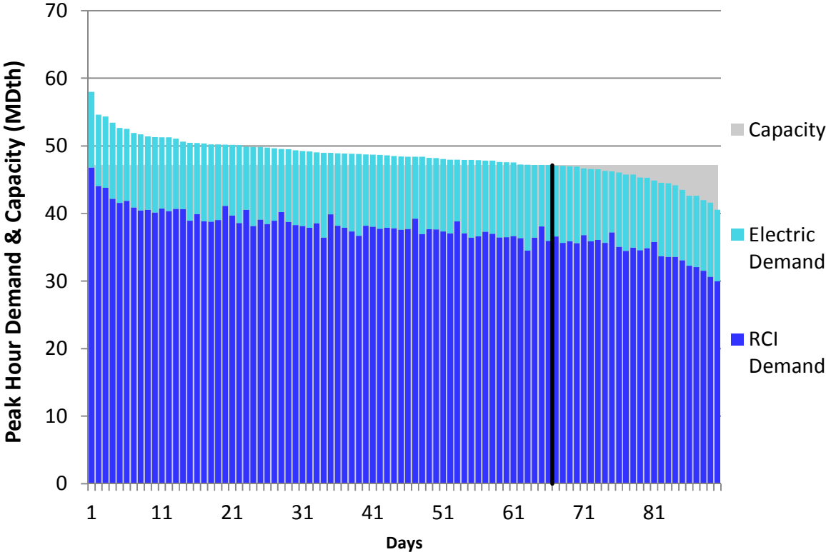
Figure U224. HGDS Roll-Up Winter 2023 – Columbia Gas W PA/NY – Descending Demand
