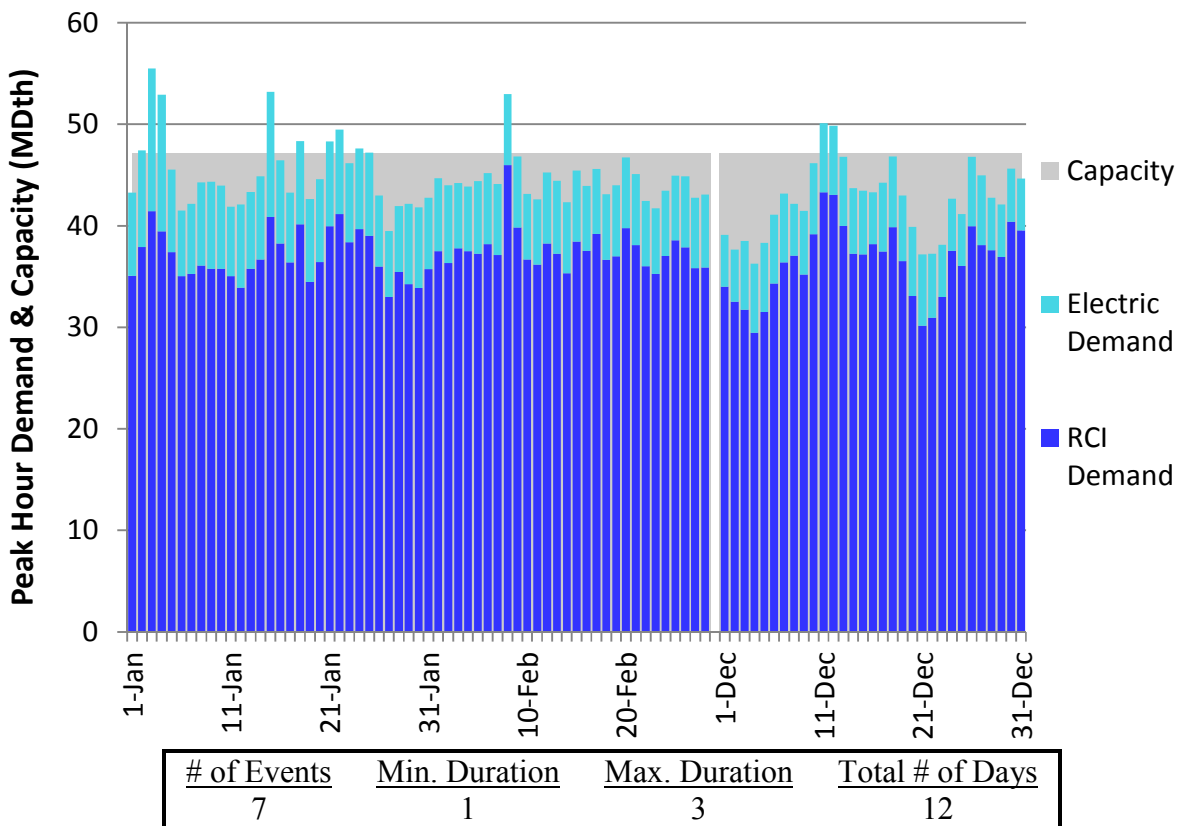
Figure U138. HGDS Roll-Up Winter 2018 – Columbia Gas W PA/NY – Descending Demand
