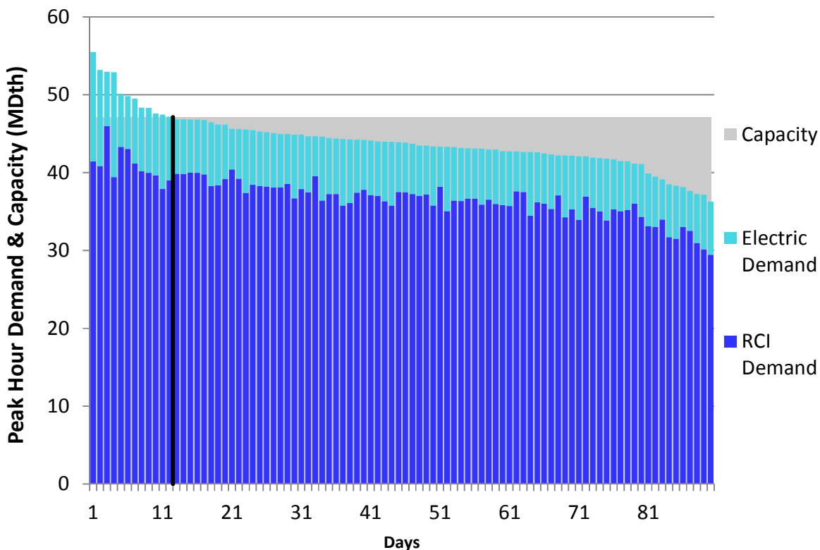
Figure U138. HGDS Roll-Up Winter 2018 – Columbia Gas W PA/NY – Descending Demand
