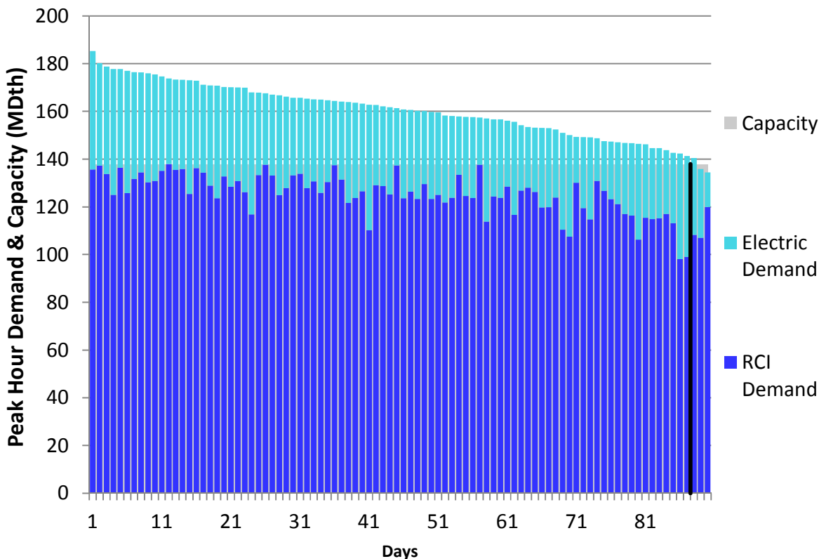
Figure U104. RGDS Roll-Up Winter 2023 – Transco Leidy to Station 210 – Descending Demand
