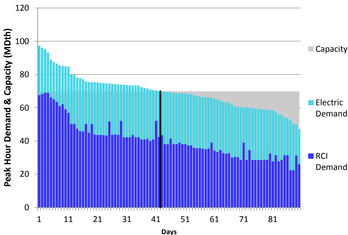
Figure U252. HGDS Roll-Up Winter 2023 – NGPL IA/IL South – Descending Demand
