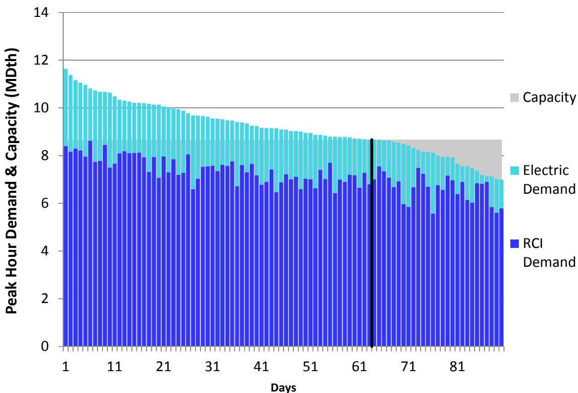
Figure U150. HGDS Roll-Up Winter 2018 – Eastern Shore – Descending Demand
