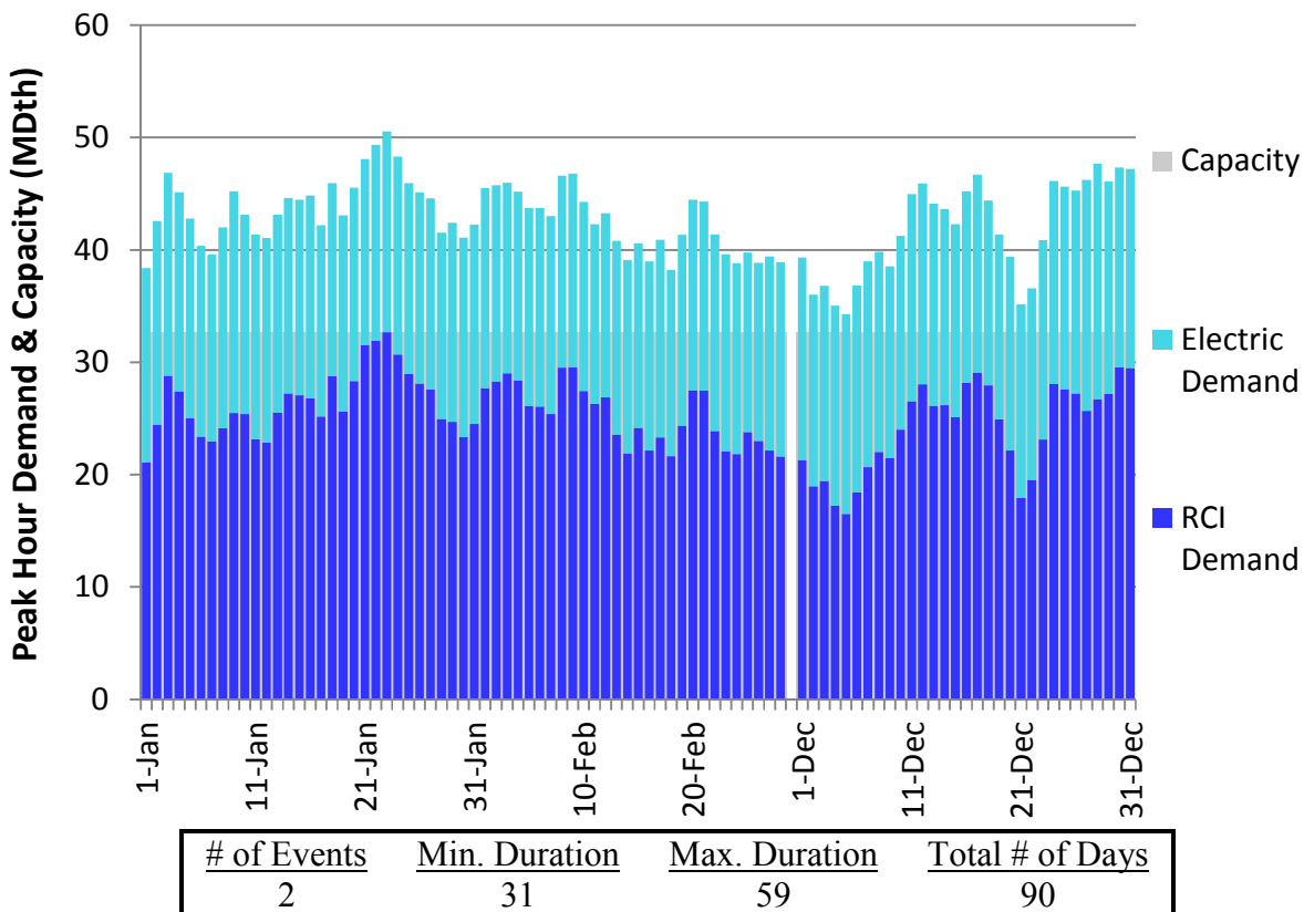
Figure U246. HGDS Roll-Up Winter 2023 – Millennium – Descending Demand
