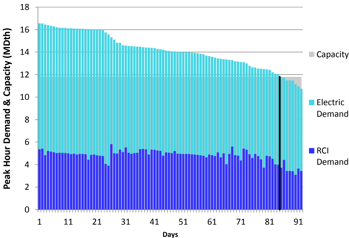
Figure U118. RGDS Roll-Up Summer 2023 – NB/NS Supply – Descending Demand
