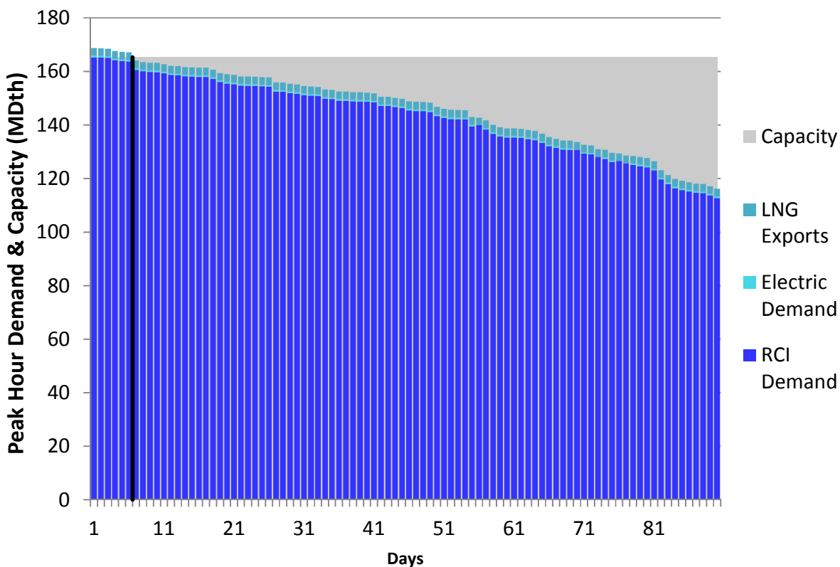
Figure U374. LGDS Roll-Up Winter 2023 – Transco Z5 – Descending Demand
