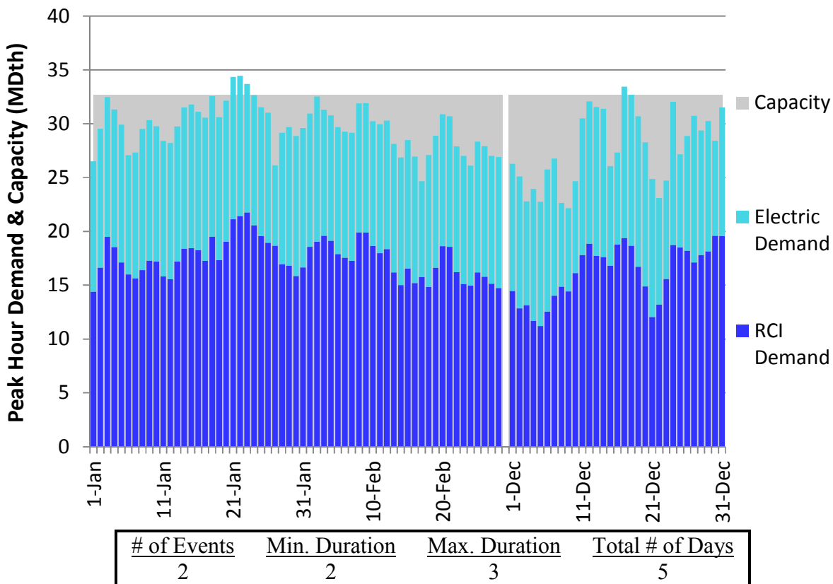
Figure U314. LGDS Roll-Up Winter 2018 – Millennium – Descending Demand
