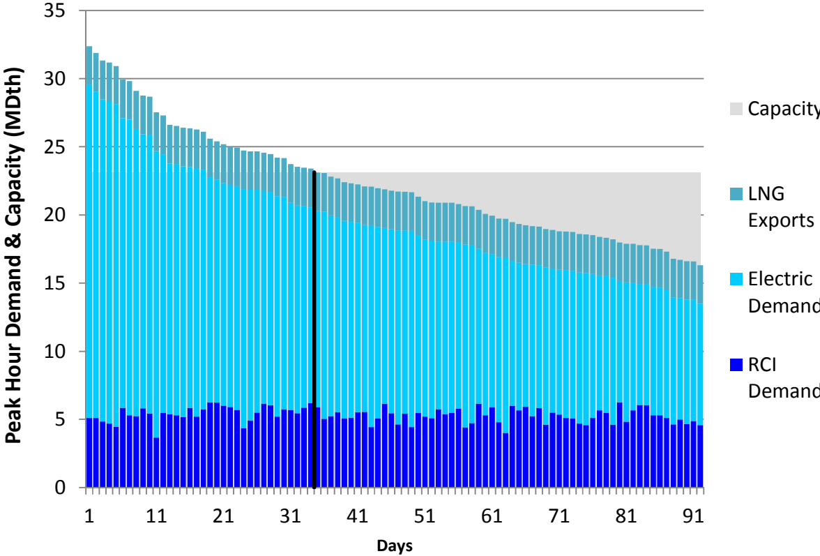
Figure U112. RGDS Roll-Up Summer 2023 – Dominion Southeast – Descending Demand
