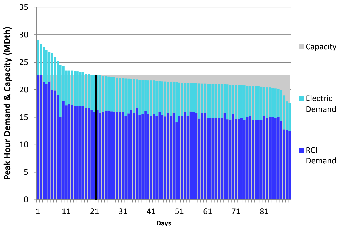
Figure U190. HGDS Roll-Up Winter 2018 – Viking Zone 1 – Descending Demand
