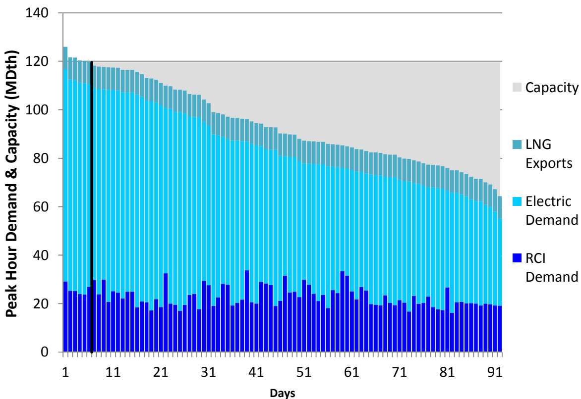
Figure U286. HGDS Roll-Up Summer 2023 – Columbia Gas VA/MD – Descending Demand
