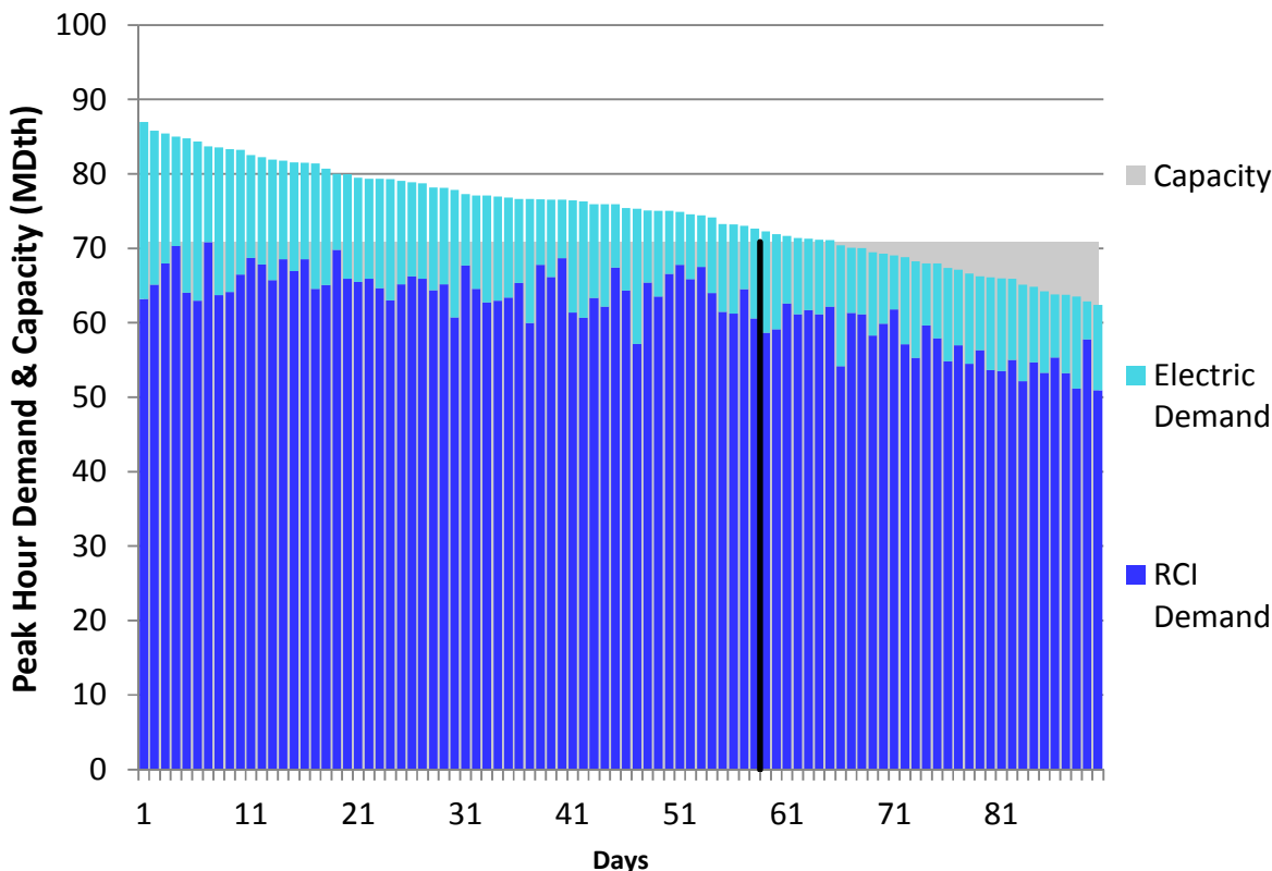
Figure U100. RGDS Roll-Up Winter 2023 – Transco Leidy Atlantic – Descending Demand
