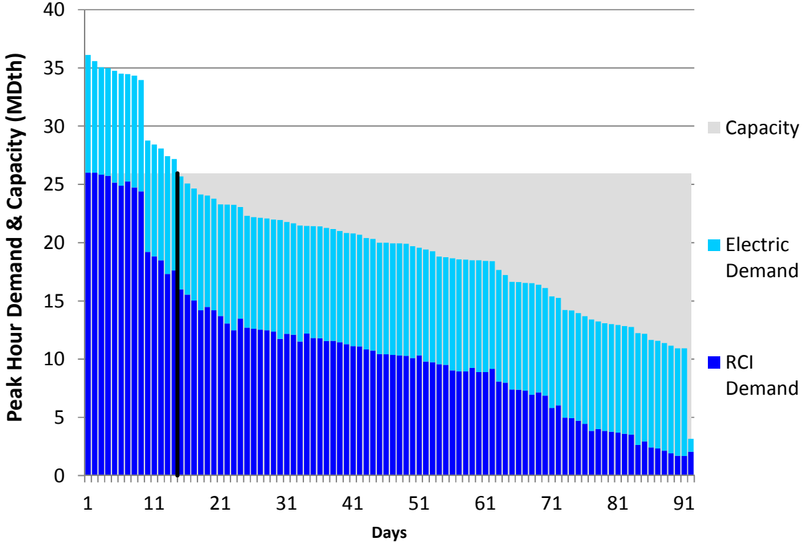
Figure U340. LGDS Roll-Up Summer 2018 – Texas Eastern ETX – Descending Demand
