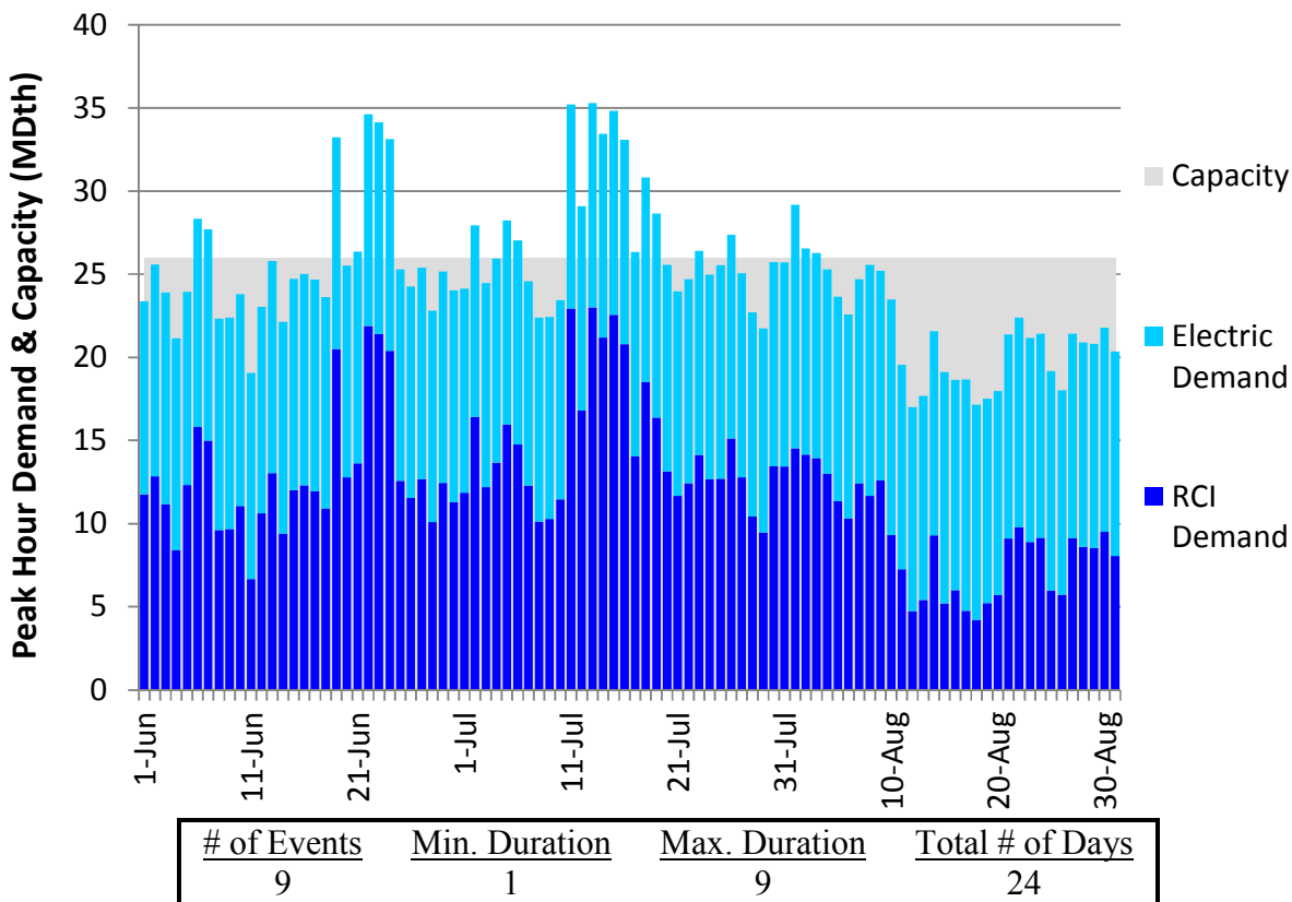
Figure U212. HGDS Roll-Up Summer 2018 – Texas Eastern ETX – Descending Demand
