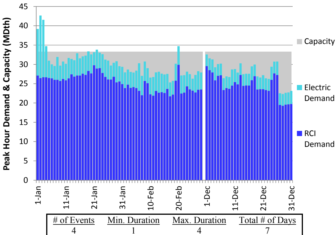
Figure U168. HGDS Roll-Up Winter 2018 – Northern Natural Zone D – Descending Demand
