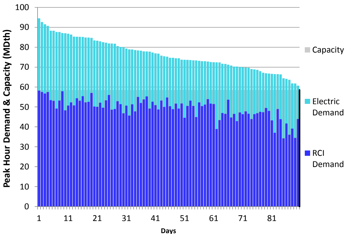
Figure U262. HGDS Roll-Up Winter 2023 – Tennessee Z5 NY – Descending Demand
