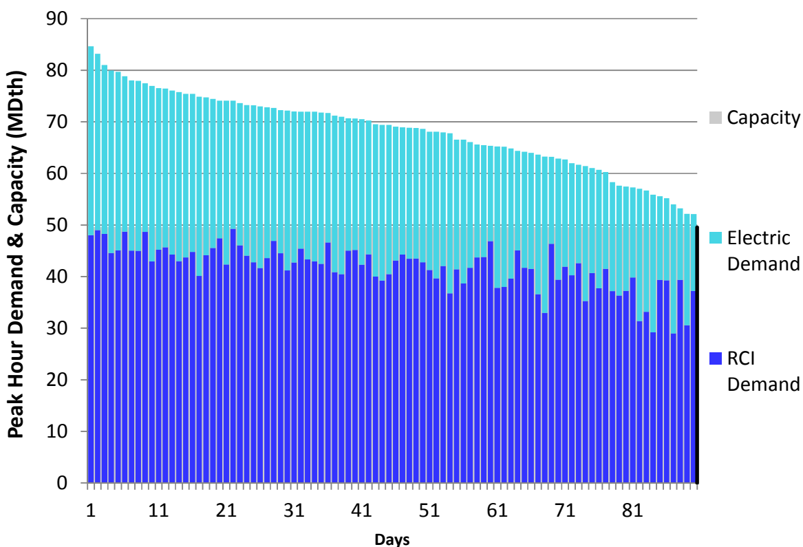
Figure U26. RGDS Roll-Up Winter 2018 – Tennessee Z5 NY – Descending Demand
