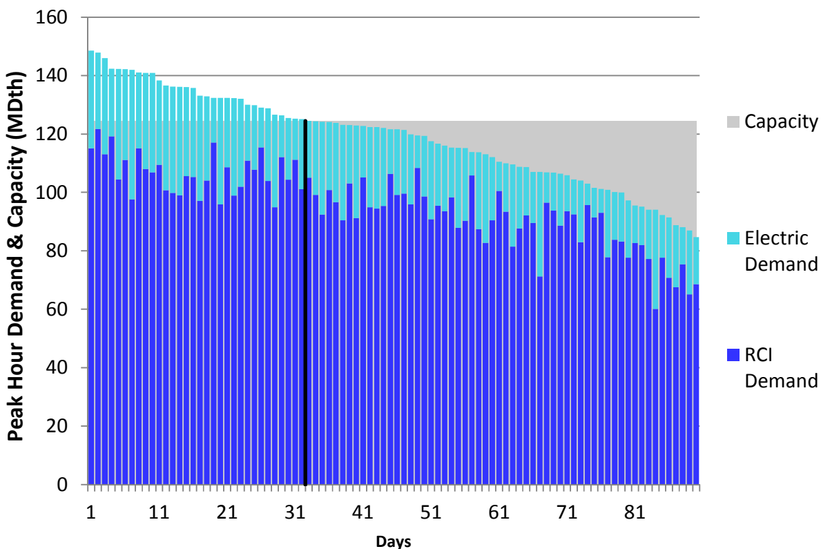
Figure U30. RGDS Roll-Up Winter 2018 – Texas Eastern M3 North – Descending Demand
