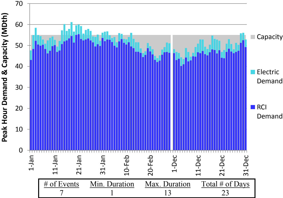
Figure U34. RGDS Roll-Up Winter 2018 – TransCanada Quebec – Descending Demand
