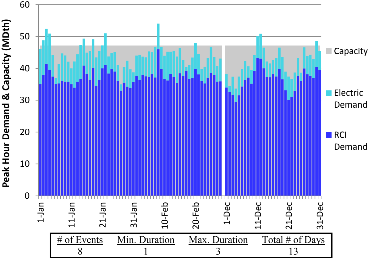
Figure U4. RGDS Roll-Up Winter 2018 – Columbia Gas W PA/NY – Descending Demand
