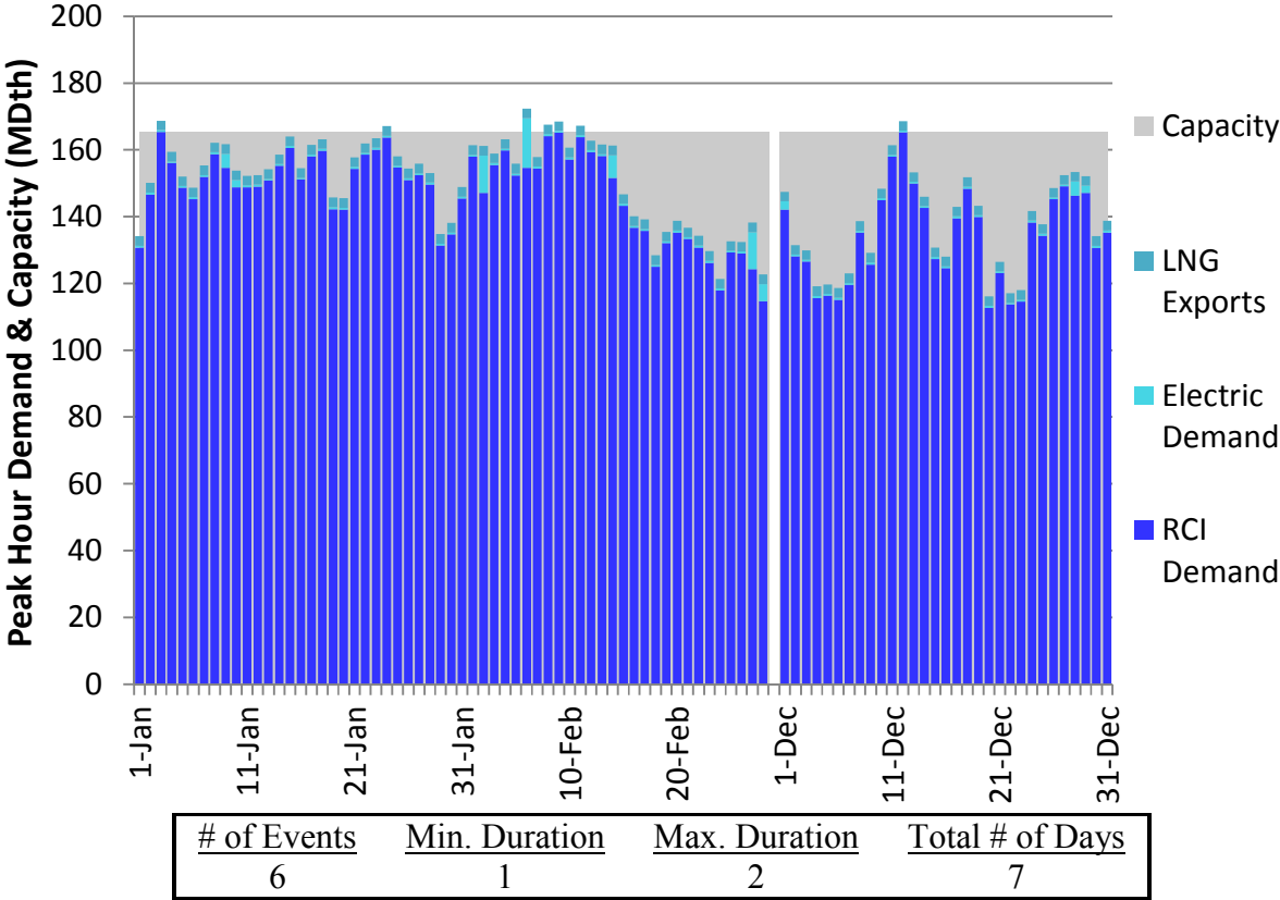
Figure U102. RGDS Roll-Up Winter 2023 – Transco Z5 – Descending Demand
