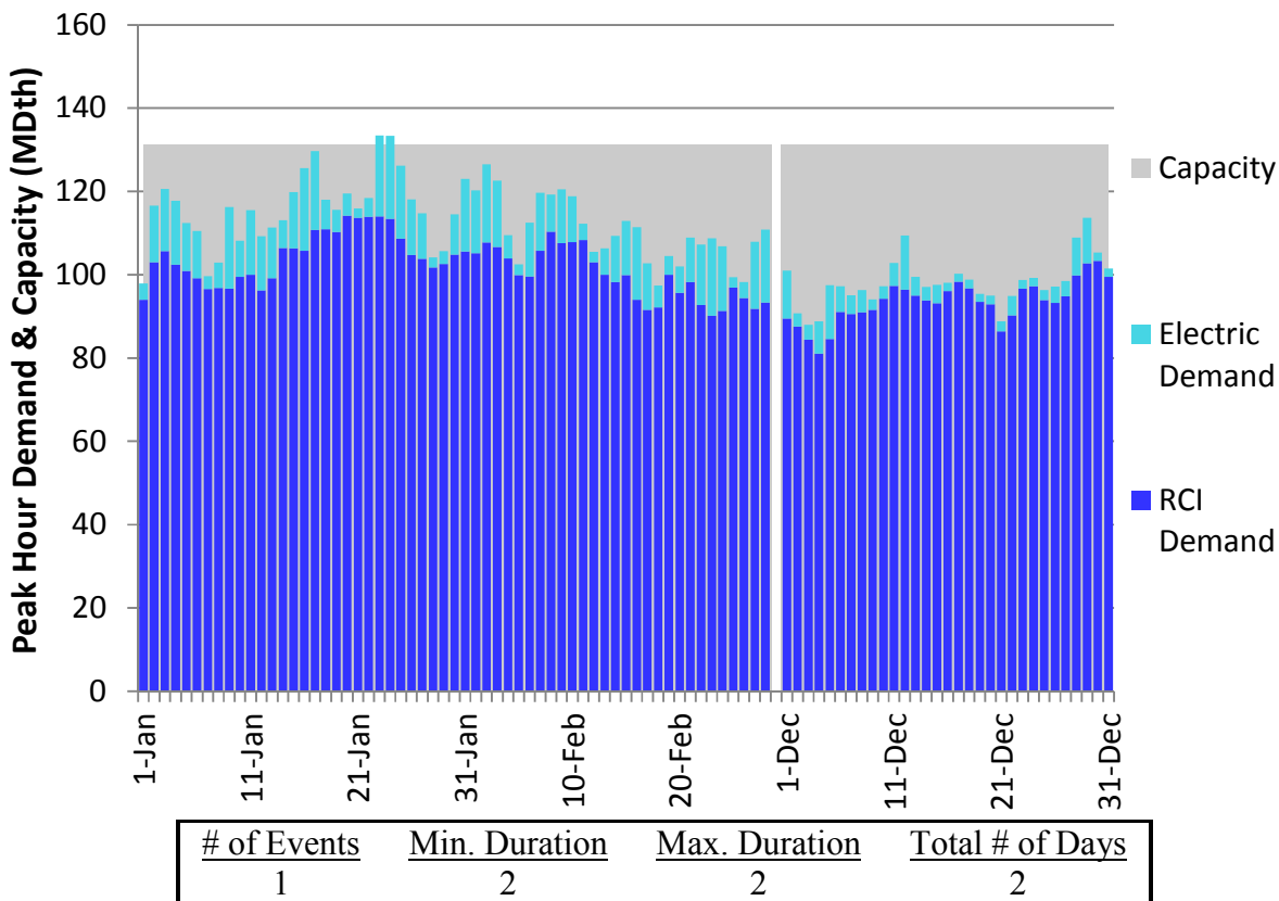
Figure U96. RGDS Roll-Up Winter 2023 – TransCanada Ontario West – Descending Demand
