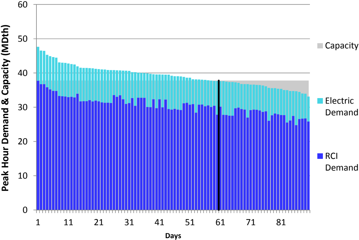
Figure U72. RGDS Roll-Up Winter 2023 – Dominion Eastern NY– Descending Demand
