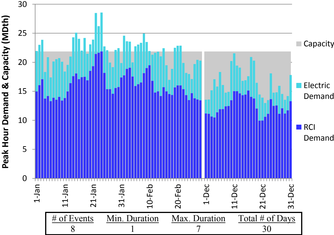
Figure U152. HGDS Roll-Up Winter 2018 – Empire – Descending Demand
