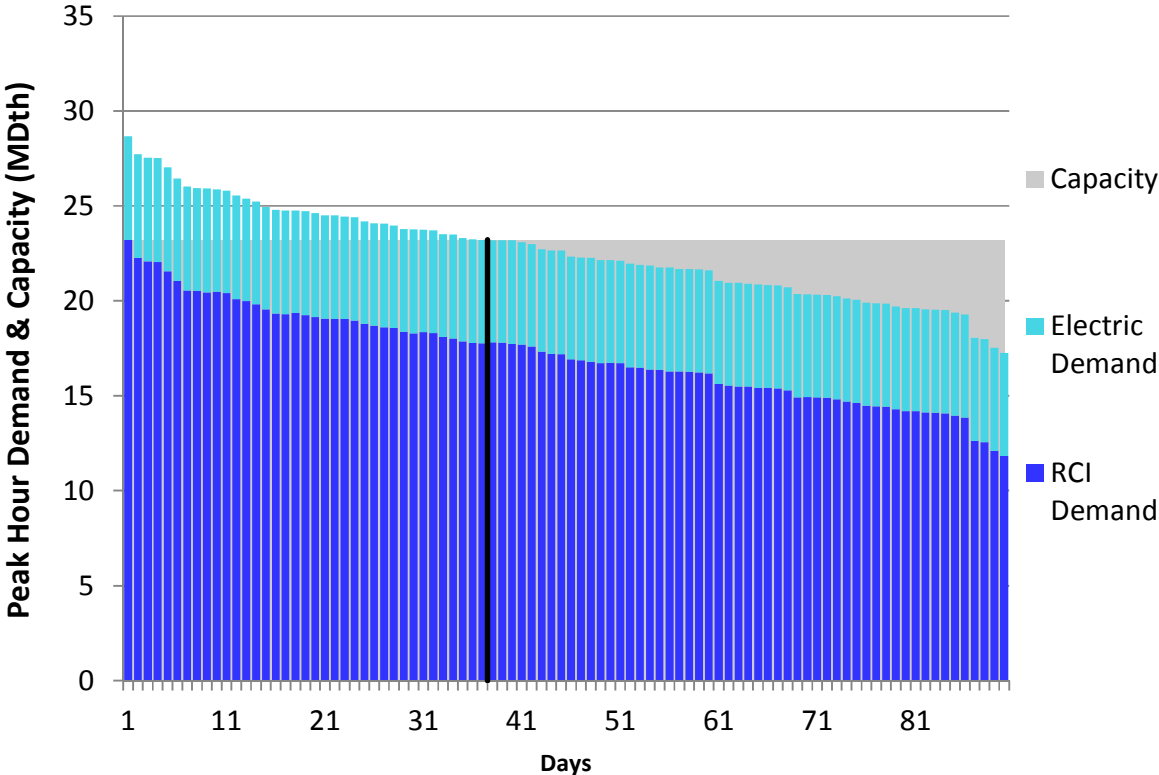
Figure U230. HGDS Roll-Up Winter 2023 – Dominion Western NY– Descending Demand
