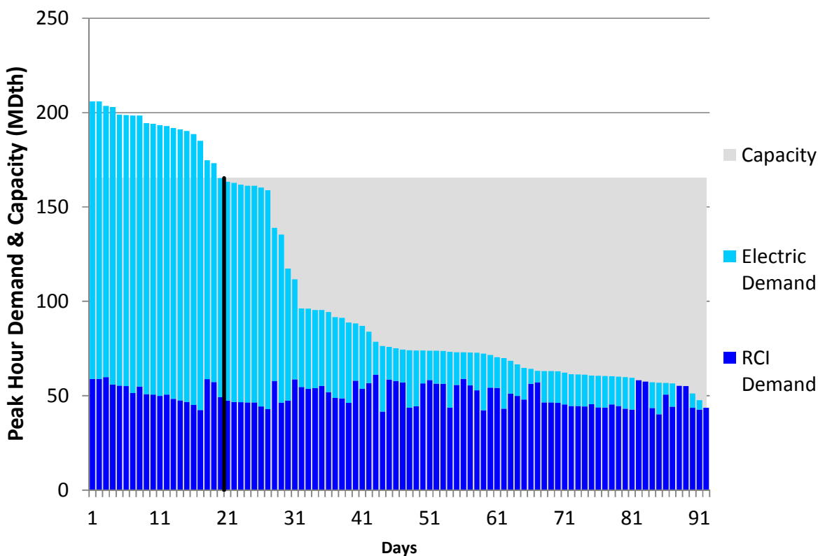
Figure U64. RGDS Roll-Up Summer 2018 – Transco Z5 – Descending Demand
