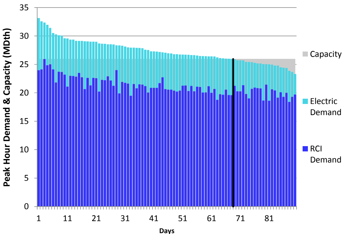
Figure U160. HGDS Roll-Up Winter 2018 – NB/NS Supply – Descending Demand
