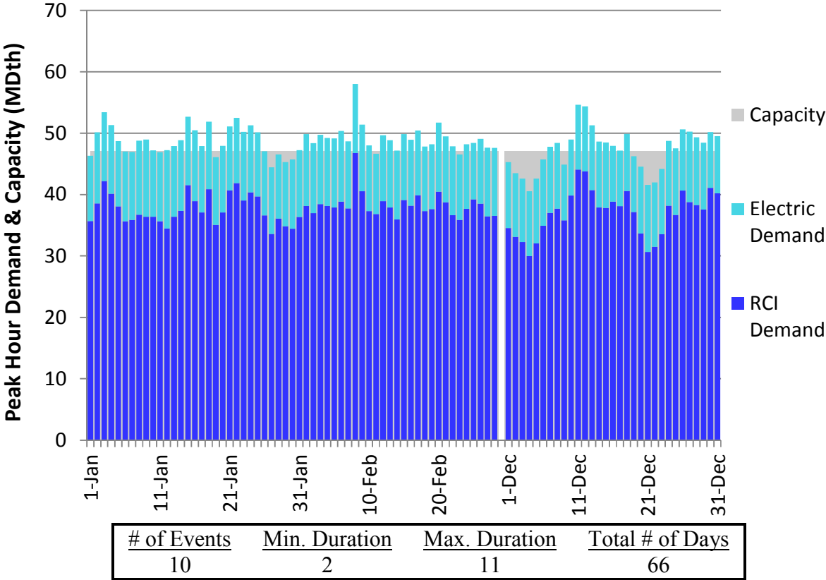
Figure U224. HGDS Roll-Up Winter 2023 – Columbia Gas W PA/NY – Descending Demand
