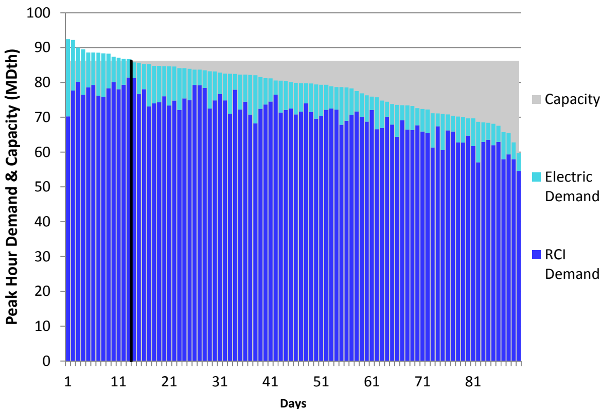
Figure U322. LGDS Roll-Up Winter 2018 – Texas Eastern M2 PA South – Descending Demand
