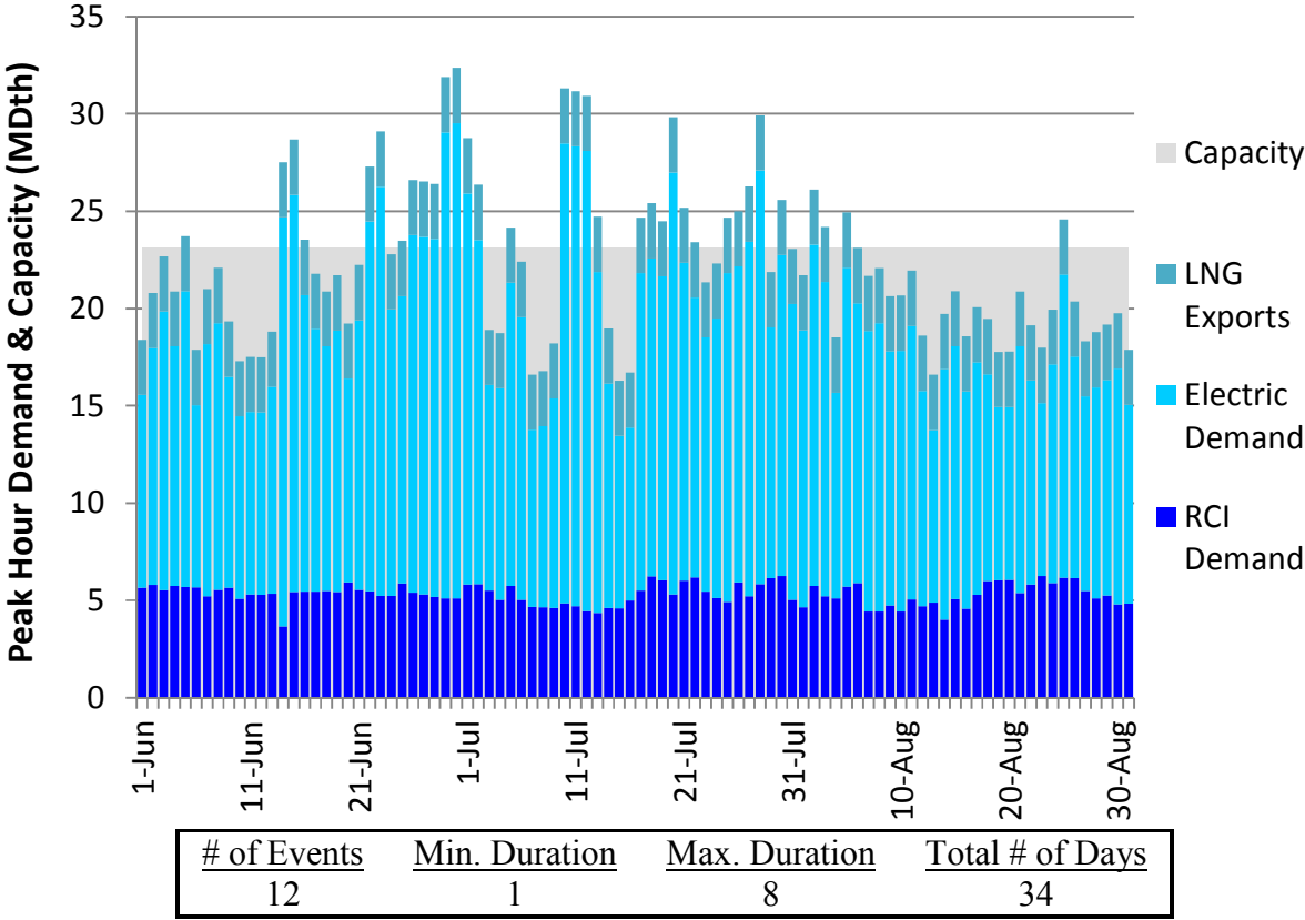
Figure U112. RGDS Roll-Up Summer 2023 – Dominion Southeast – Descending Demand
