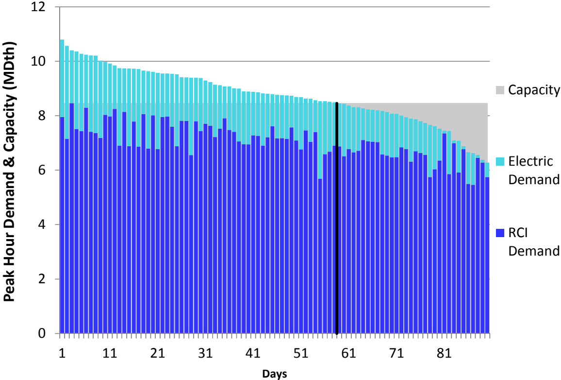
Figure U16. RGDS Roll-Up Winter 2018 – Eastern Shore – Descending Demand
