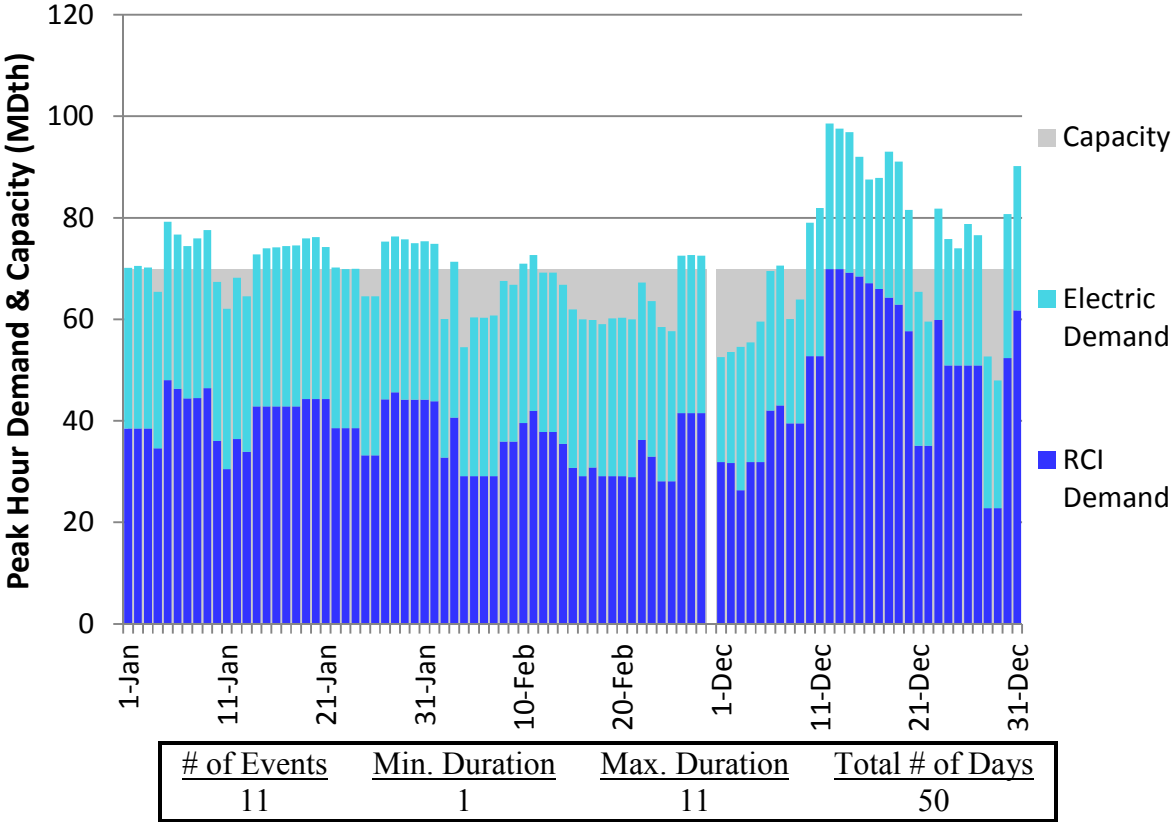
Figure U164. HGDS Roll-Up Winter 2018 – NGPL IA/IL South – Descending Demand
