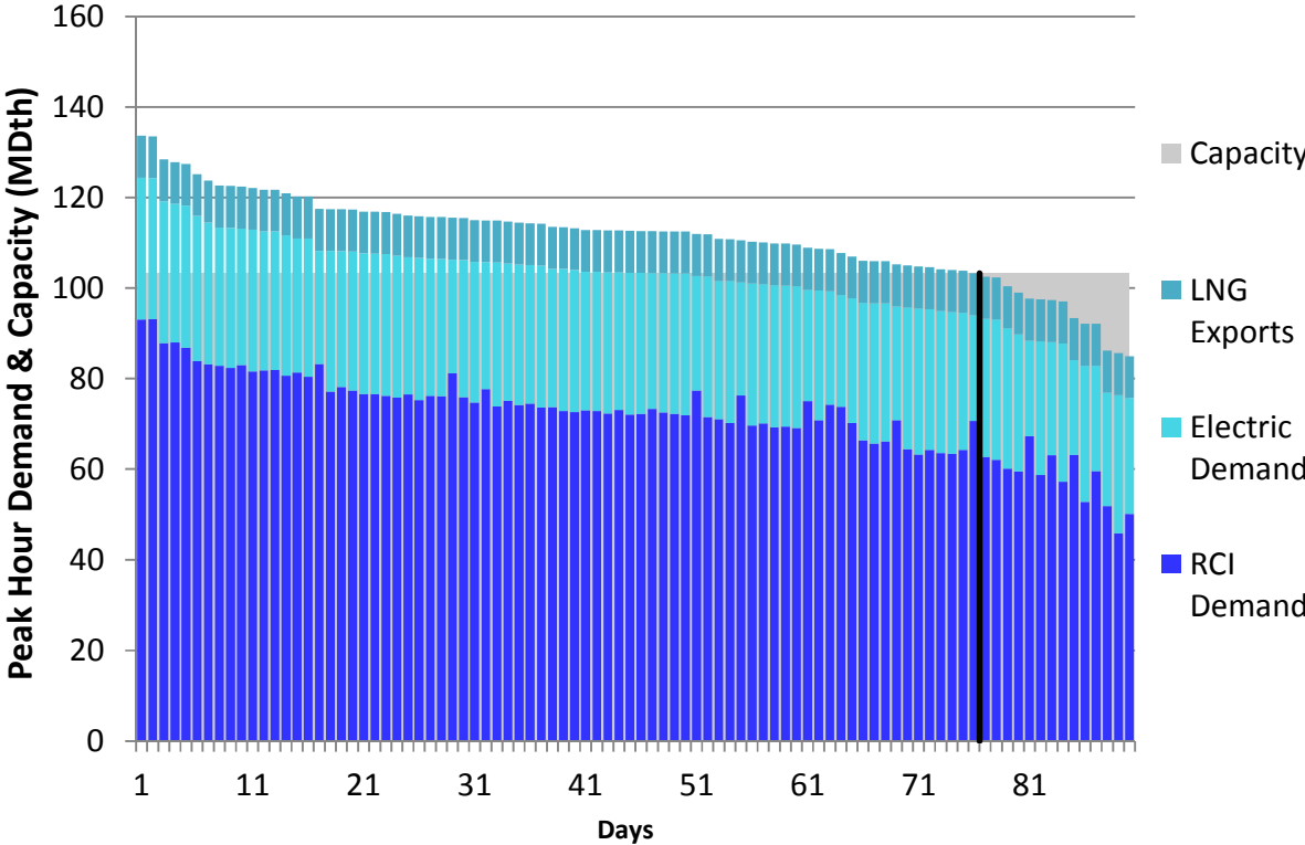
Figure U346. LGDS Roll-Up Winter 2023 – Columbia Gas VA/MD – Descending Demand
