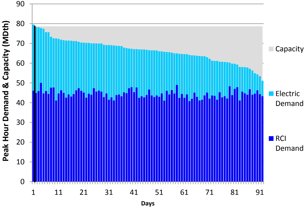
Figure U58. RGDS Roll-Up Summer 2018 – Tennessee Z4 PA – Descending Demand
