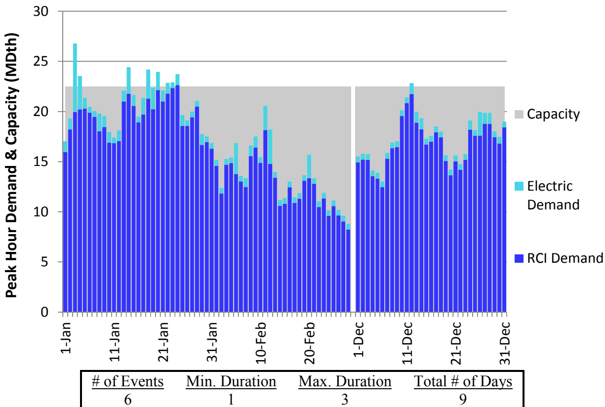
Figure U12. RGDS Roll-Up Winter 2018 – Dominion Southeast – Descending Demand
