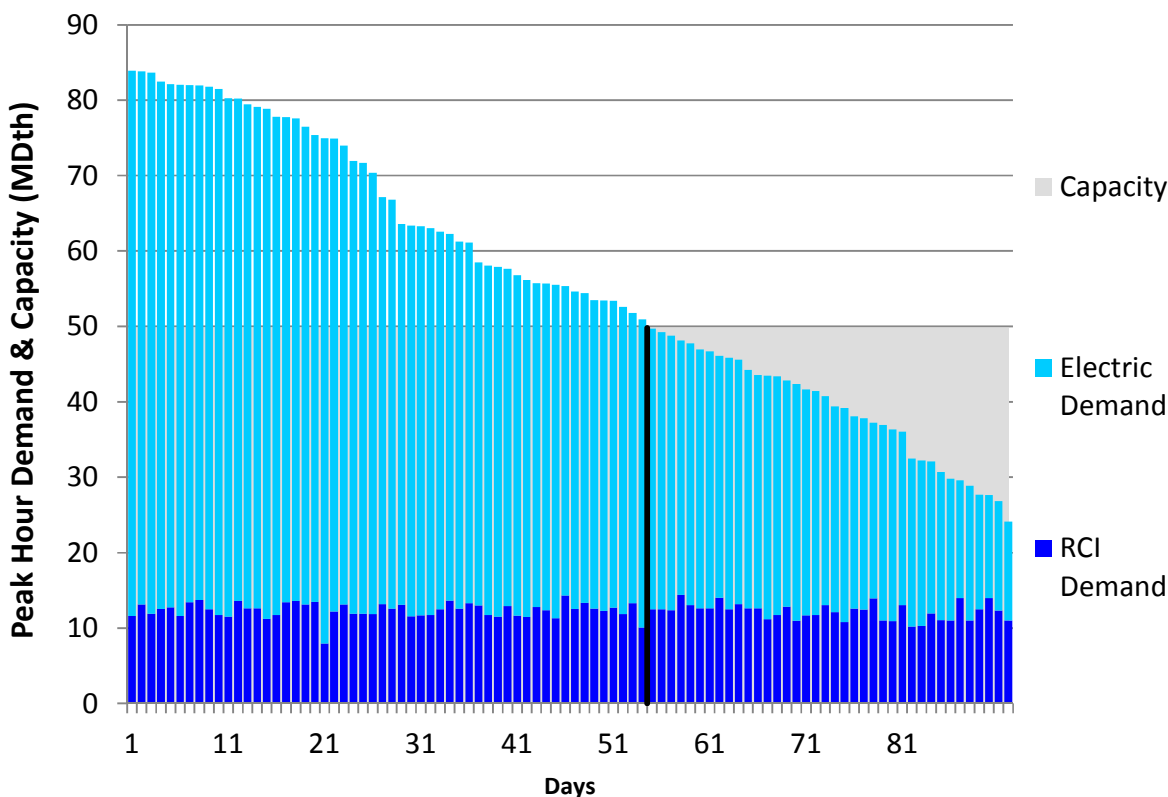
Figure U202. HGDS Roll-Up Summer 2018 – Iroquois Zone 1 – Descending Demand
