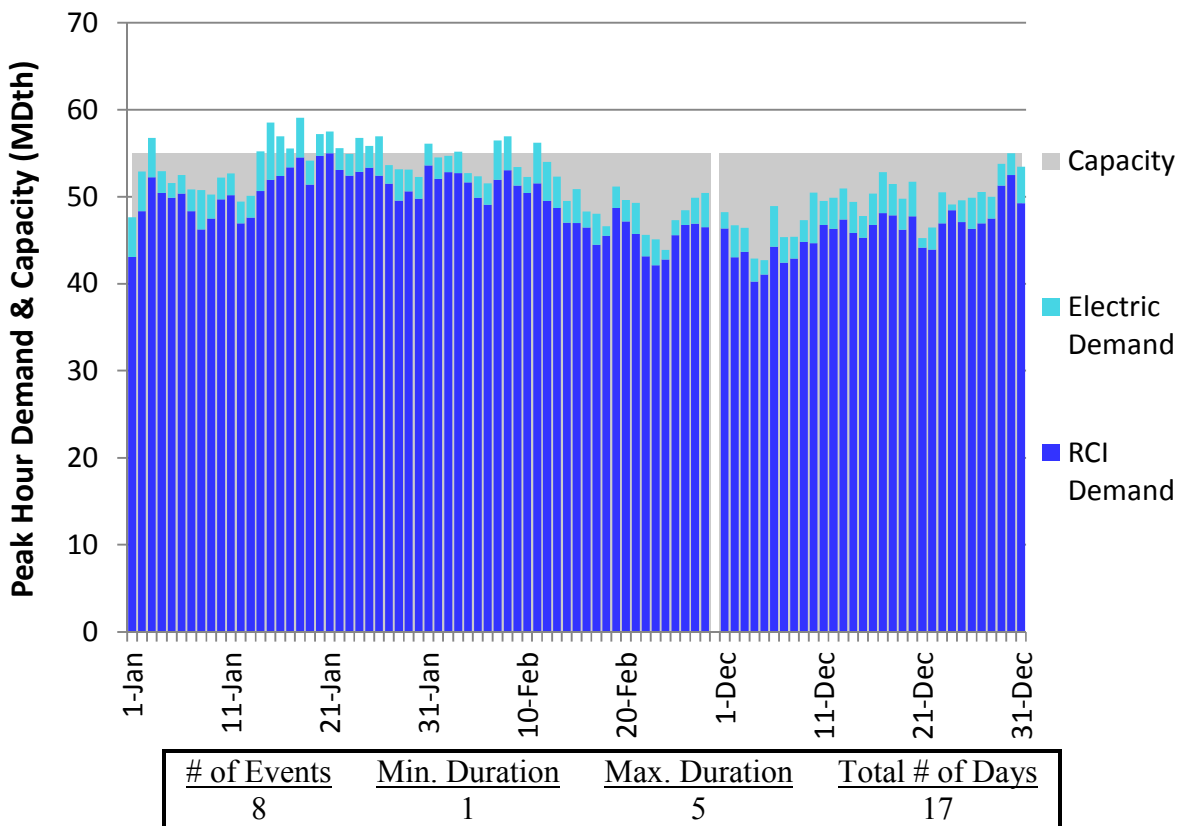
Figure U328. LGDS Roll-Up Winter 2018 – TransCanada Quebec – Descending Demand
