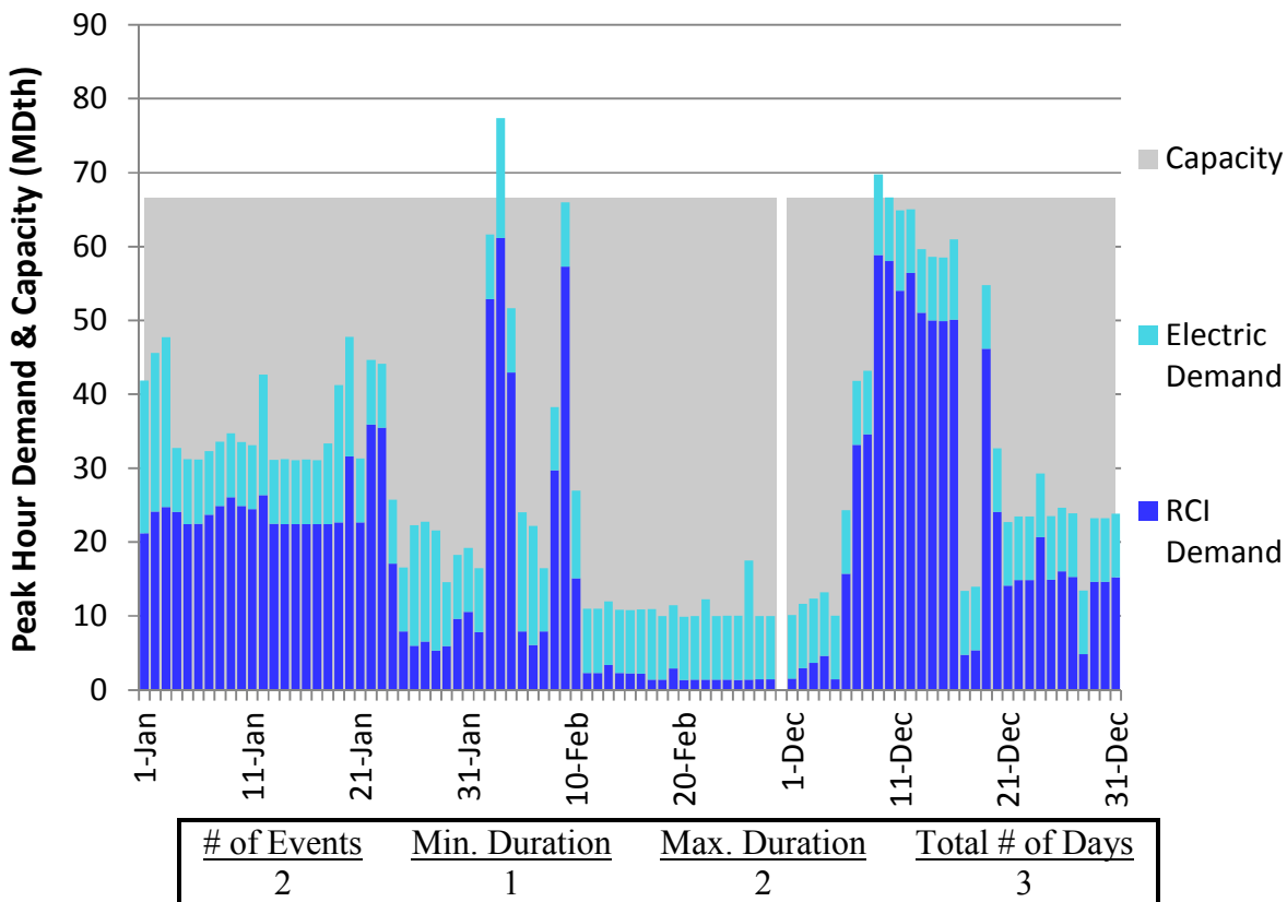
Figure U280. HGDS Roll-Up Winter 2023 – Vector Zone 1 – Descending Demand
