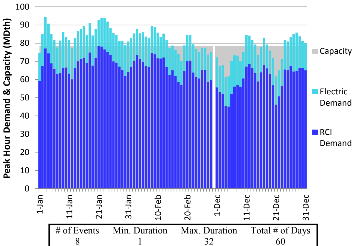
Figure U260. HGDS Roll-Up Winter 2023 – Tennessee Z4 PA – Descending Demand
