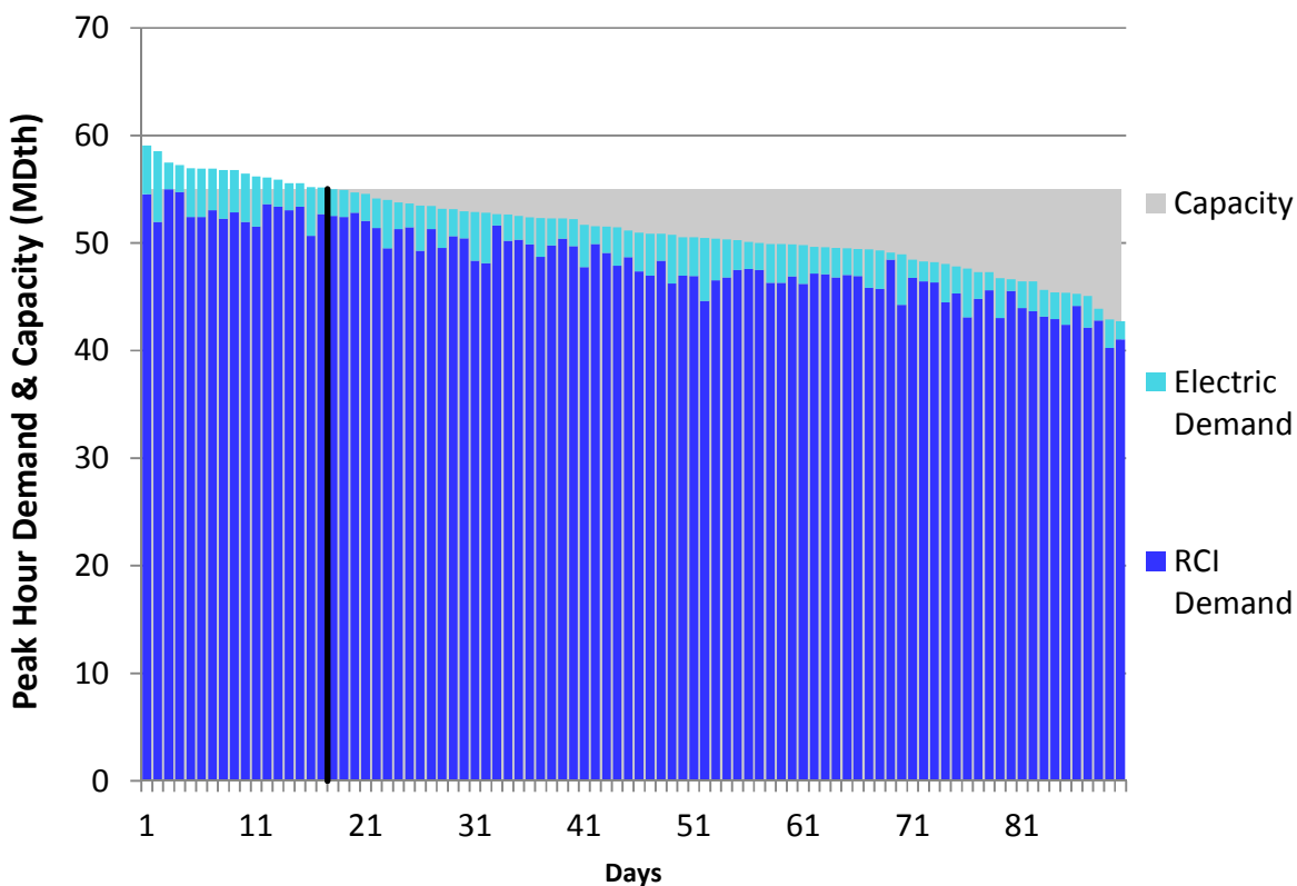
Figure U328. LGDS Roll-Up Winter 2018 – TransCanada Quebec – Descending Demand
