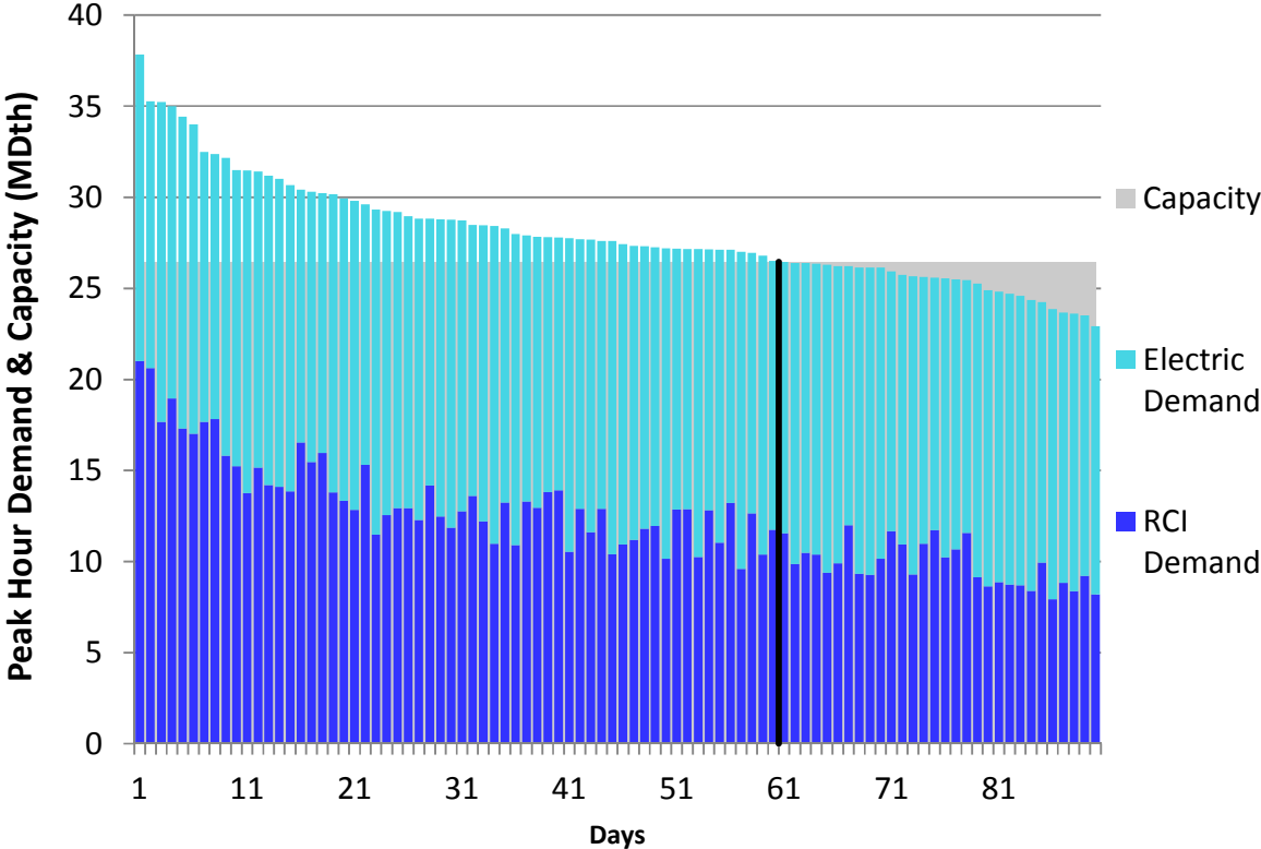
Figure U156. HGDS Roll-Up Winter 2018 – Midwestern – Descending Demand
