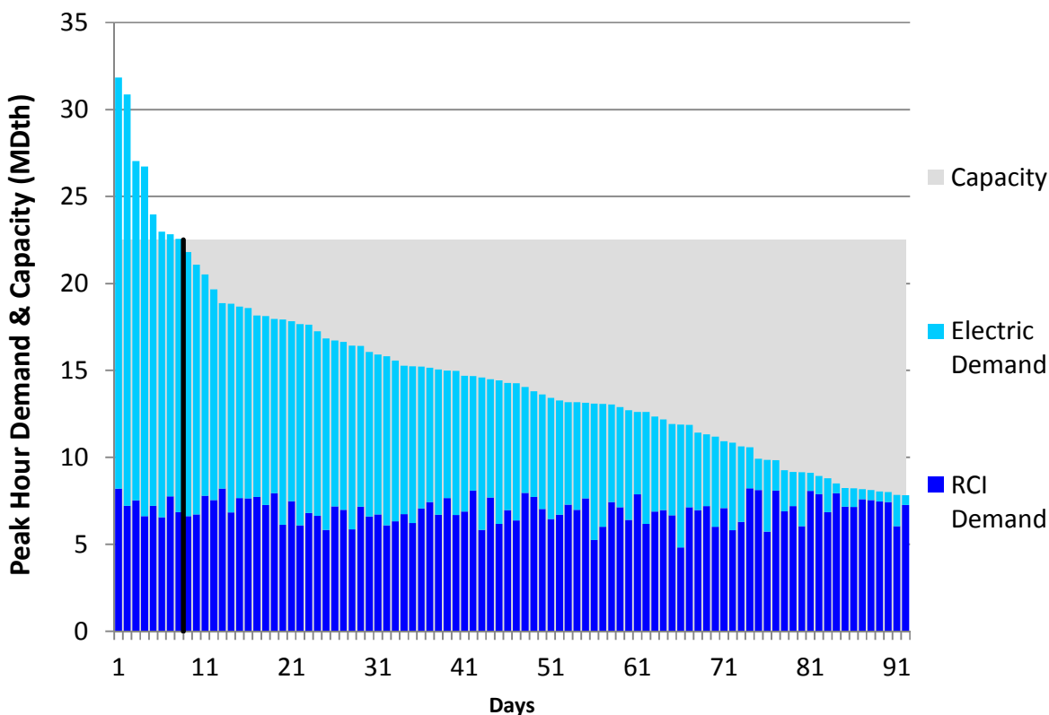
Figure U48. RGDS Roll-Up Summer 2018 – Dominion Southeast – Descending Demand
