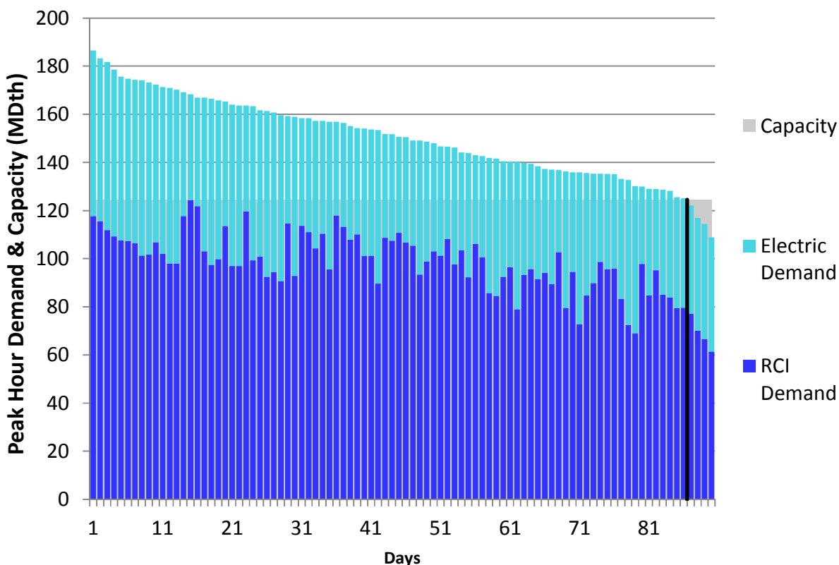
Figure U176. HGDS Roll-Up Winter 2018 – Texas Eastern M3 North – Descending Demand
