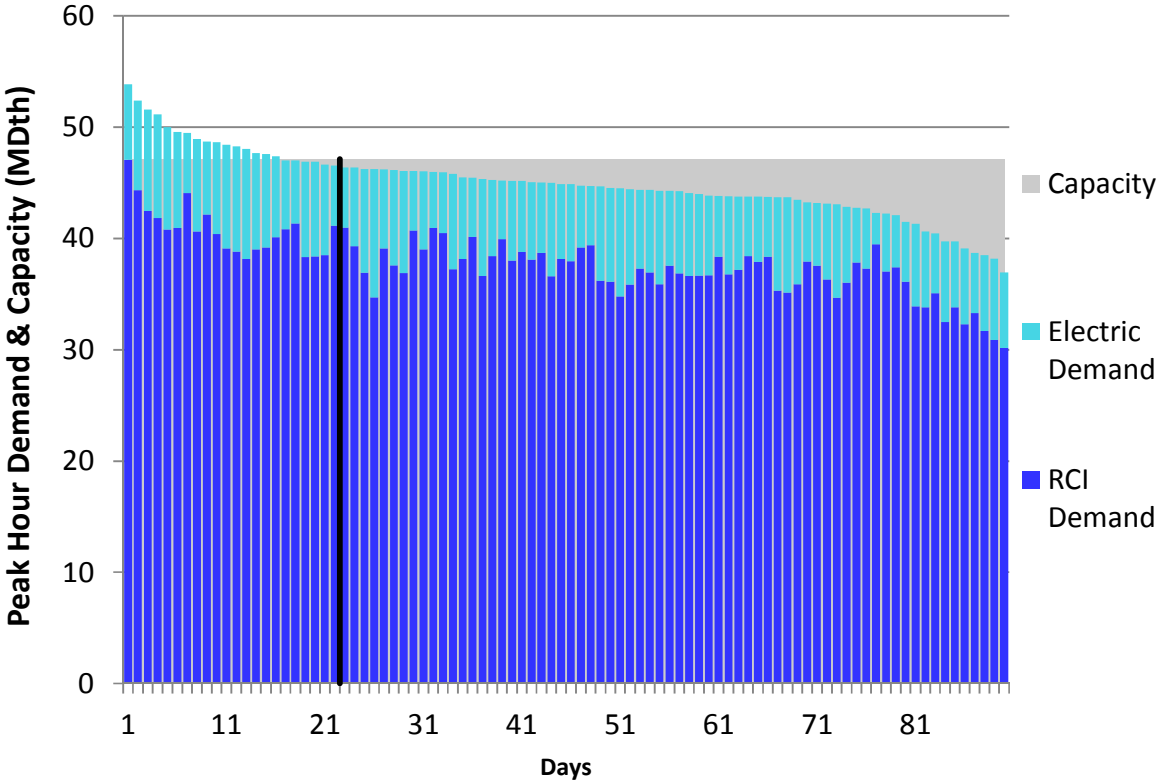
Figure U68. RGDS Roll-Up Winter 2023 – Columbia Gas W PA/NY – Descending Demand
