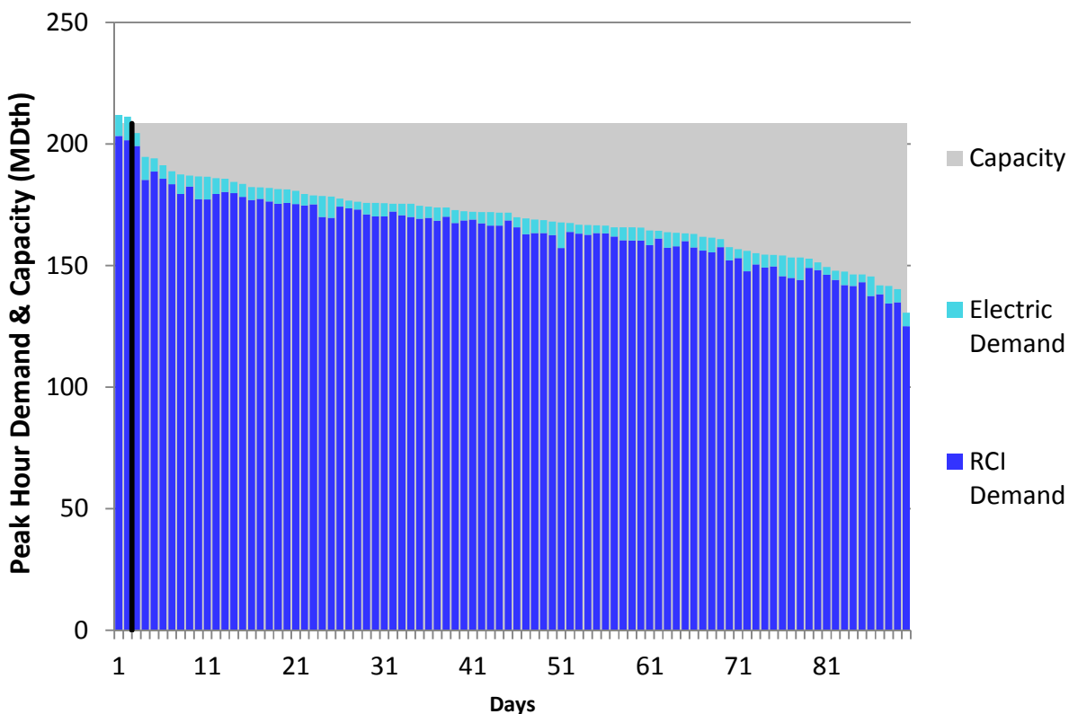
Figure U378. LGDS Roll-Up Winter 2023 – Union Gas Dawn – Descending Demand
