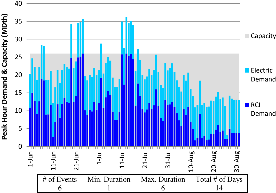
Figure U340. LGDS Roll-Up Summer 2018 – Texas Eastern ETX – Descending Demand
