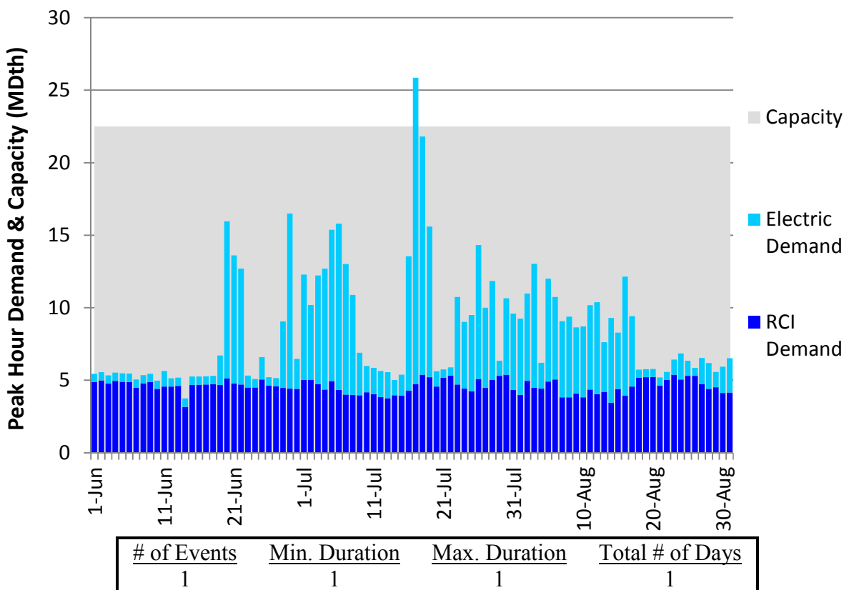
Figure U336. LGDS Roll-Up Summer 2018 – Dominion Southeast – Descending Demand
