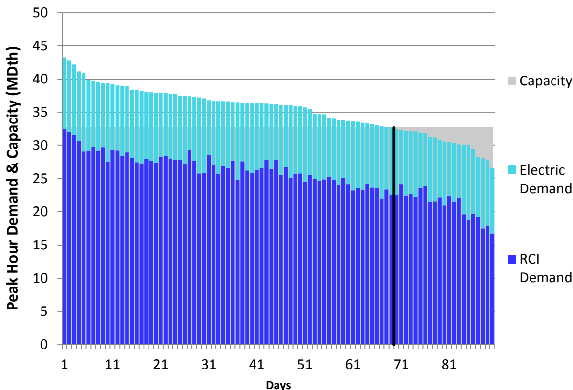
Figure U84. RGDS Roll-Up Winter 2023 – Millennium – Descending Demand
