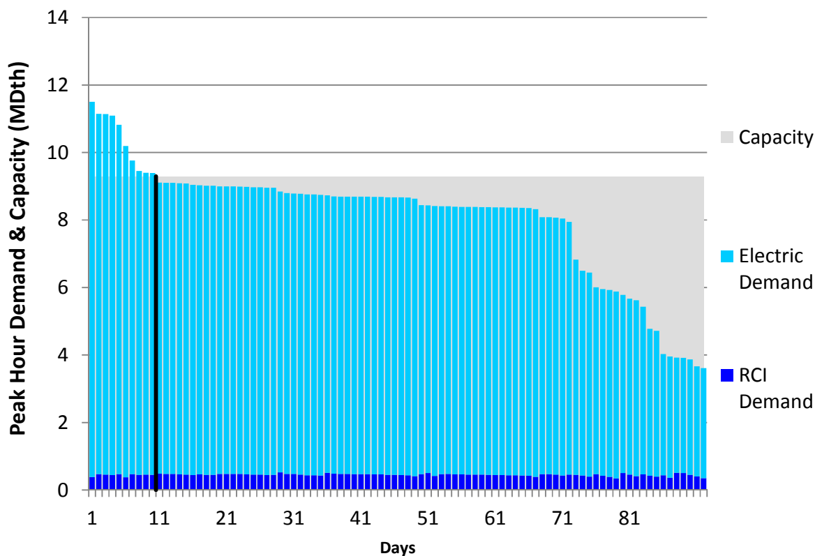
Figure U390. LGDS Roll-Up Summer 2023 – PNGTS N of Westbrook – Descending Demand
