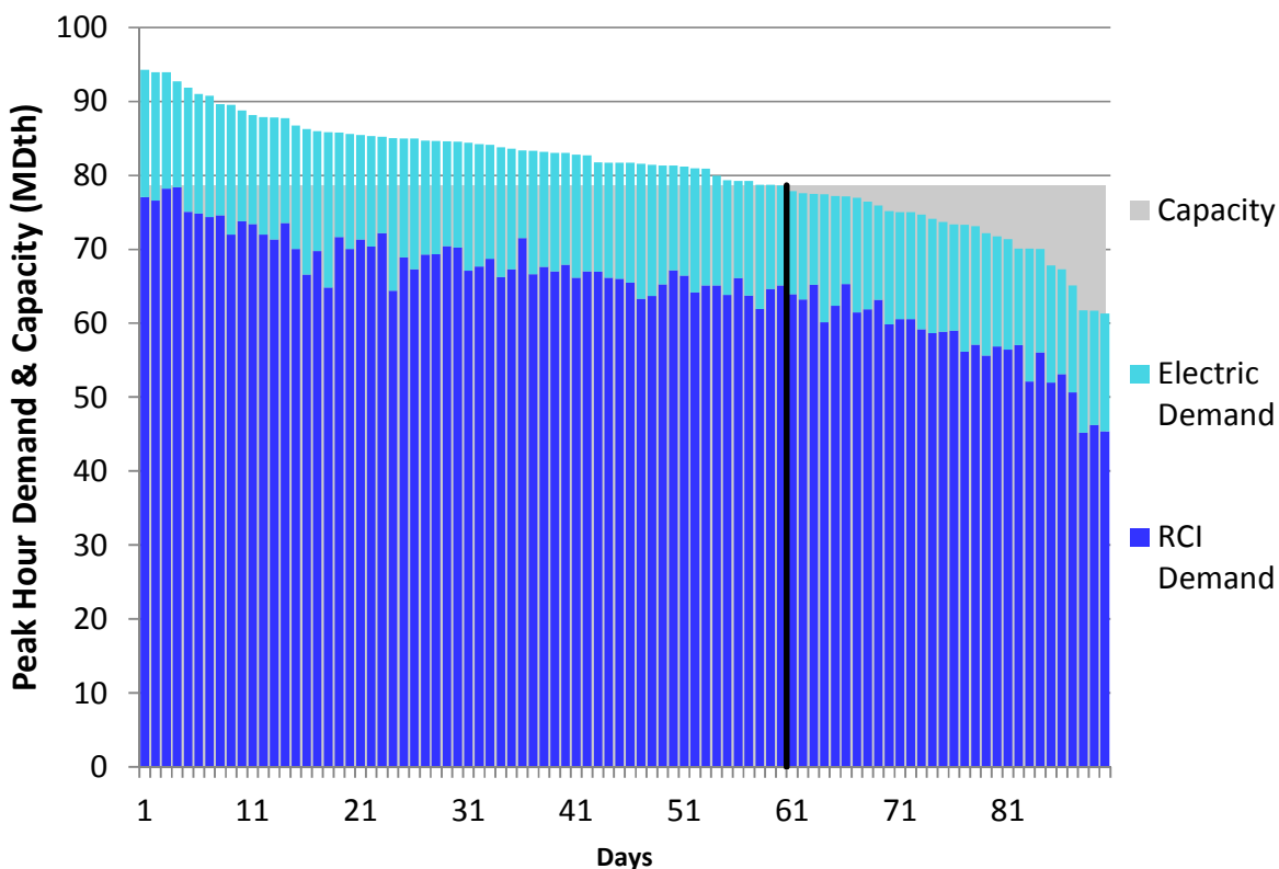
Figure U260. HGDS Roll-Up Winter 2023 – Tennessee Z4 PA – Descending Demand
