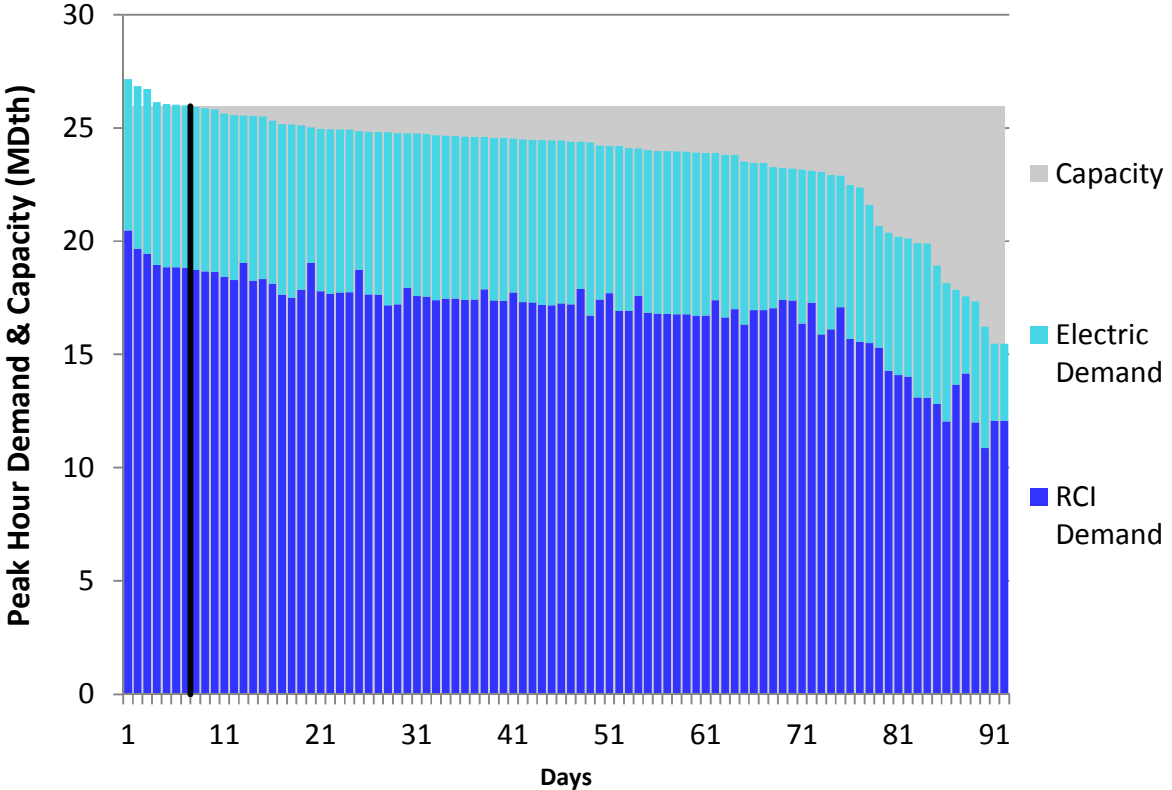
Figure U54. RGDS Roll-Up Summer 2018 – NB/NS Supply – Descending Demand
