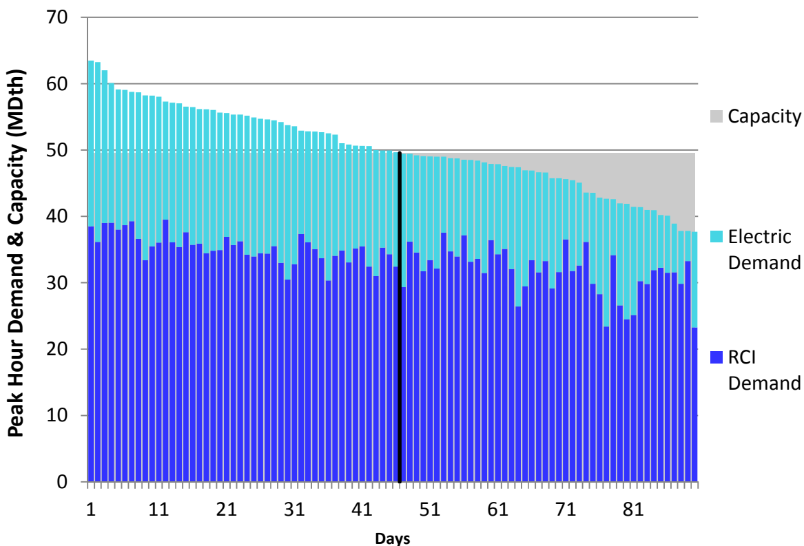
Figure U320. LGDS Roll-Up Winter 2018 – Tennessee Z5 NY – Descending Demand
