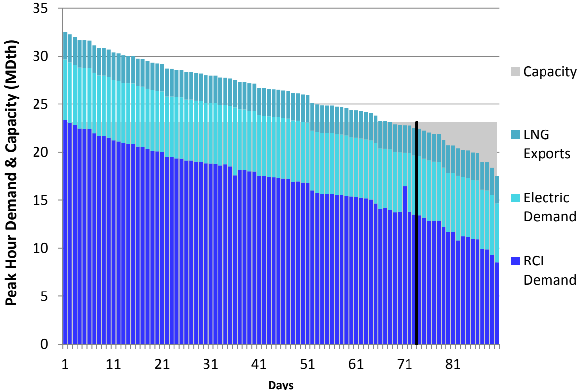
Figure U76. RGDS Roll-Up Winter 2023 – Dominion Southeast – Descending Demand
