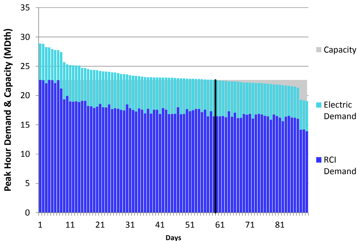
Figure U282. HGDS Roll-Up Winter 2023 – Viking Zone 1 – Descending Demand
