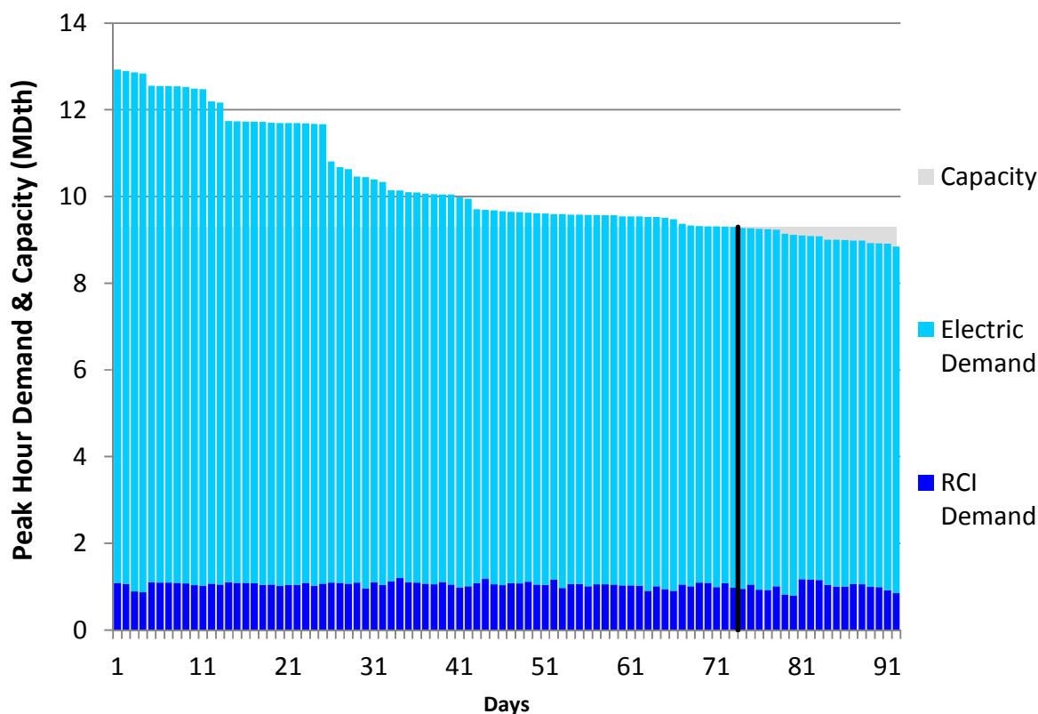
Figure U120. RGDS Roll-Up Summer 2023 – PNGTS N of Westbrook – Descending Demand
