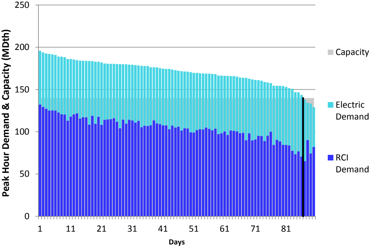
Figure U266. HGDS Roll-Up Winter 2023 – Texas Eastern M3 North – Descending Demand
