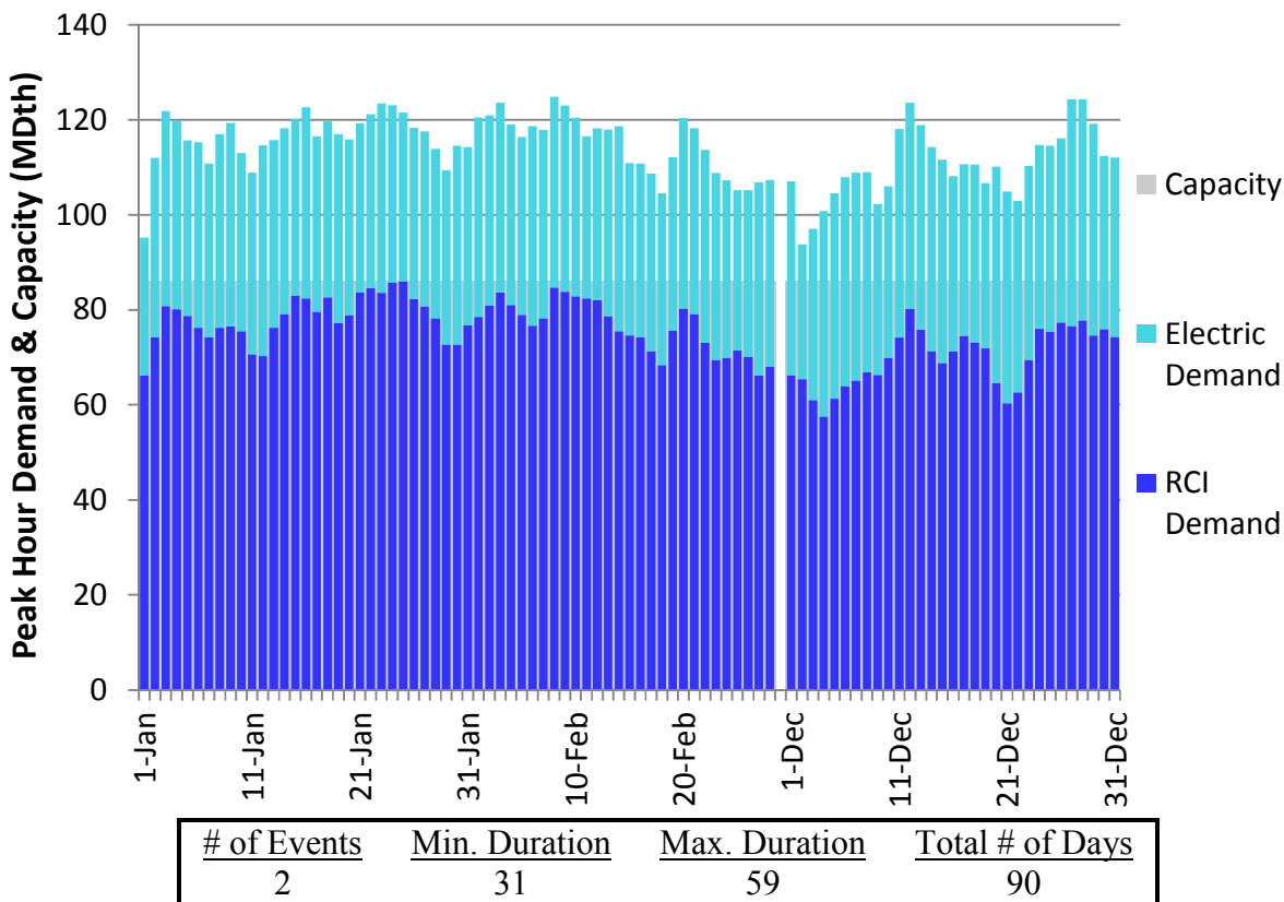
Figure U264. HGDS Roll-Up Winter 2023 – Texas Eastern M2 PA South – Descending Demand
