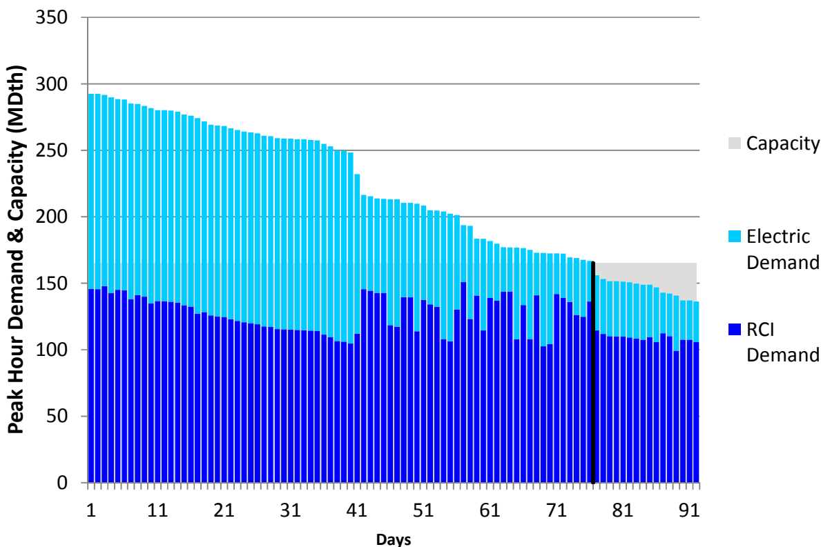
Figure U214. HGDS Roll-Up Summer 2018 – Transco Z5 – Descending Demand
