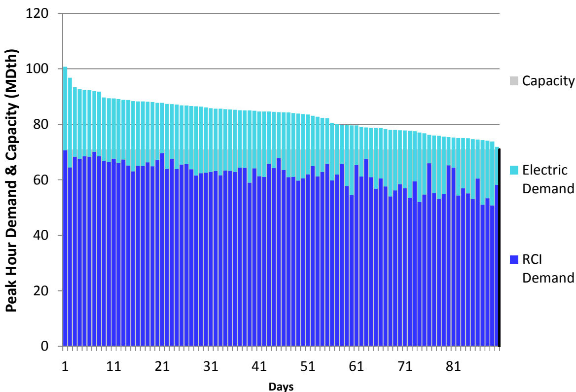
Figure U182. HGDS Roll-Up Winter 2018 – Transco Leidy Atlantic – Descending Demand
