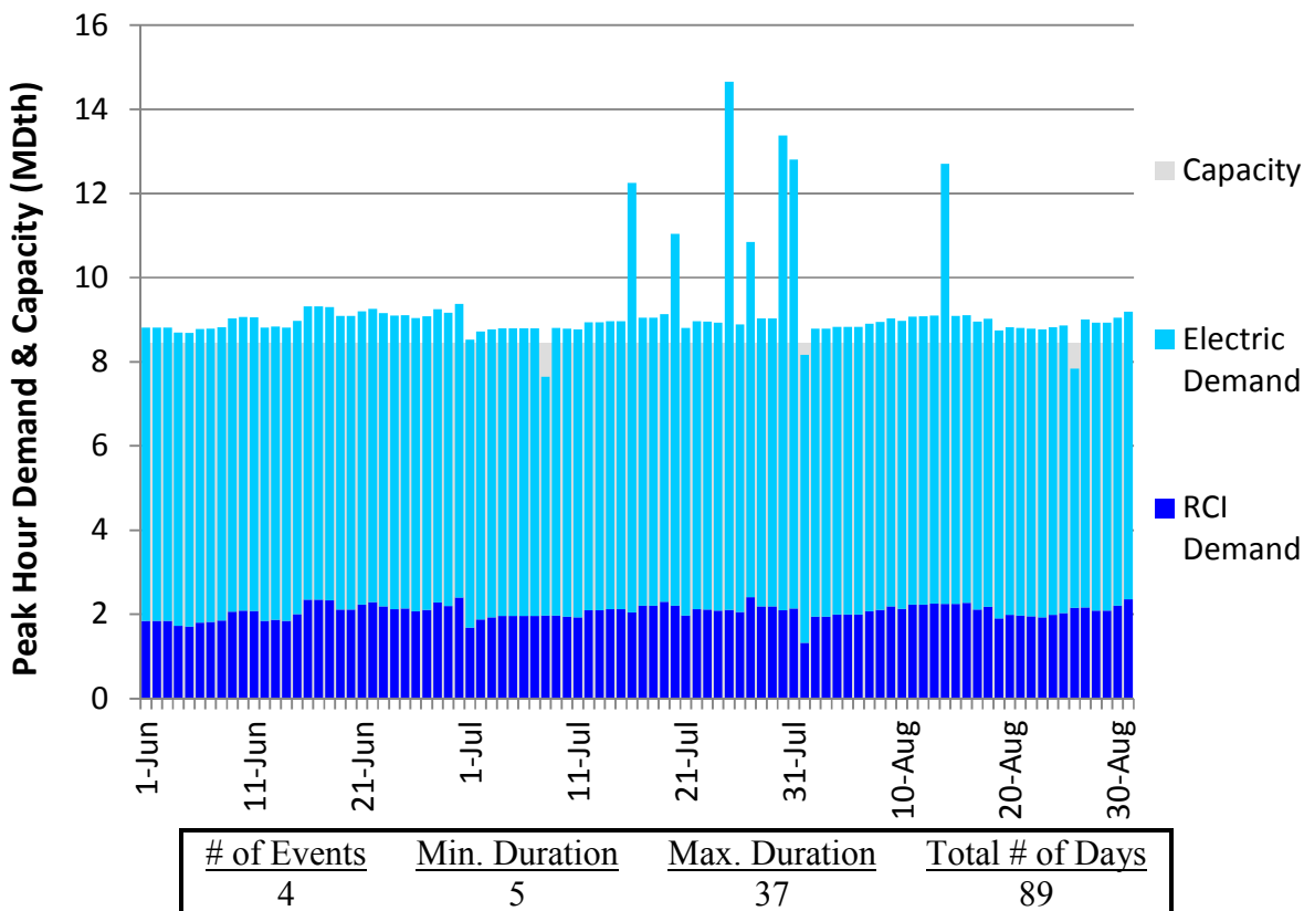
Figure U192. HGDS Roll-Up Summer 2018 – AlaTenn – Descending Demand
