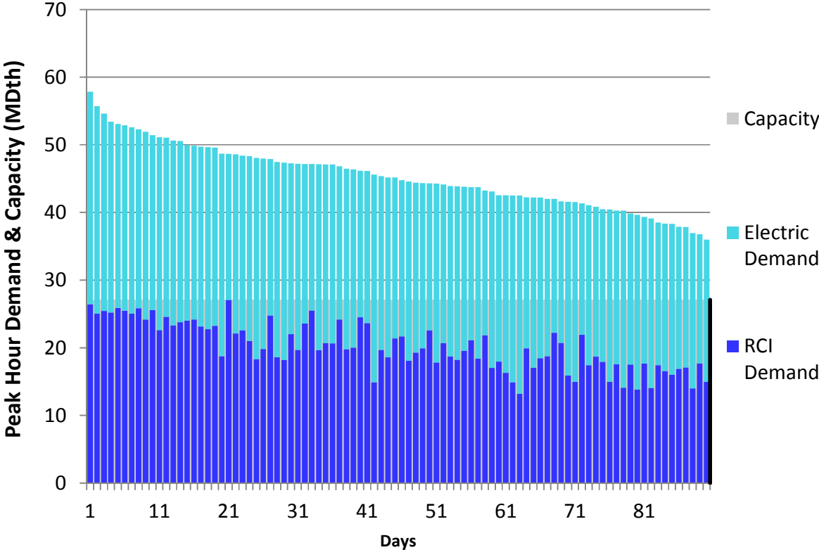
Figure U140. HGDS Roll-Up Winter 2018 – Constitution – Descending Demand
