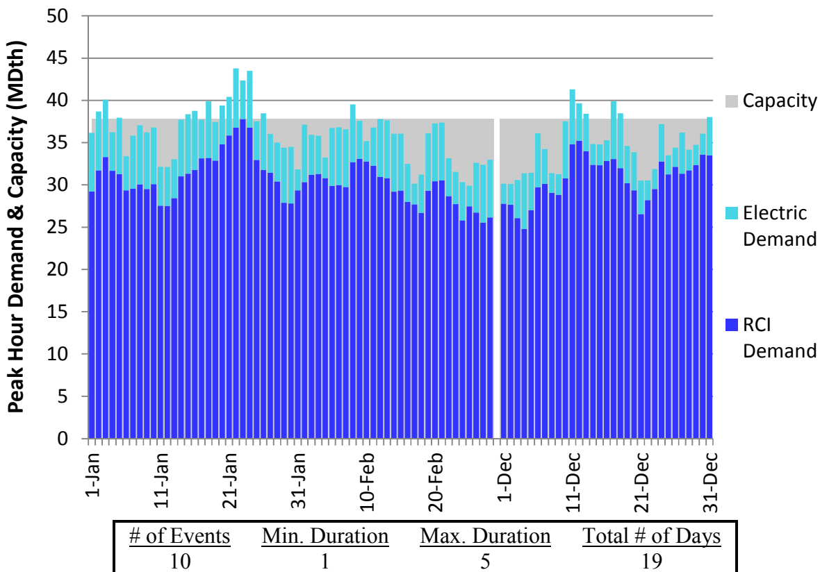
Figure U142. HGDS Roll-Up Winter 2018 – Dominion Eastern NY– Descending Demand
