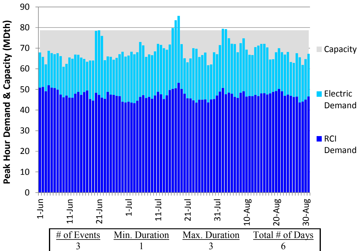
Figure U208. HGDS Roll-Up Summer 2018 – Tennessee Z4 PA – Descending Demand
