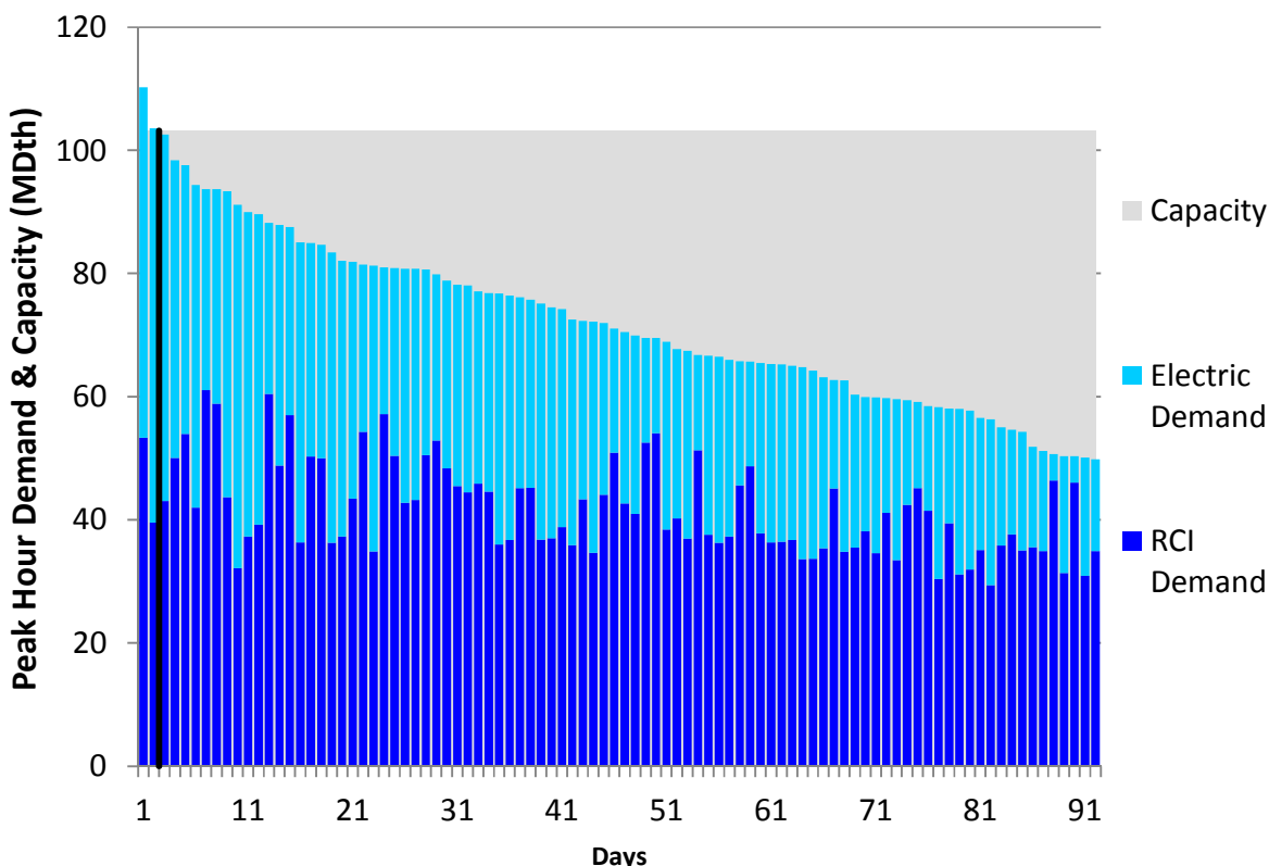
Figure U334. LGDS Roll-Up Summer 2018 – Columbia Gas VA/MD – Descending Demand
