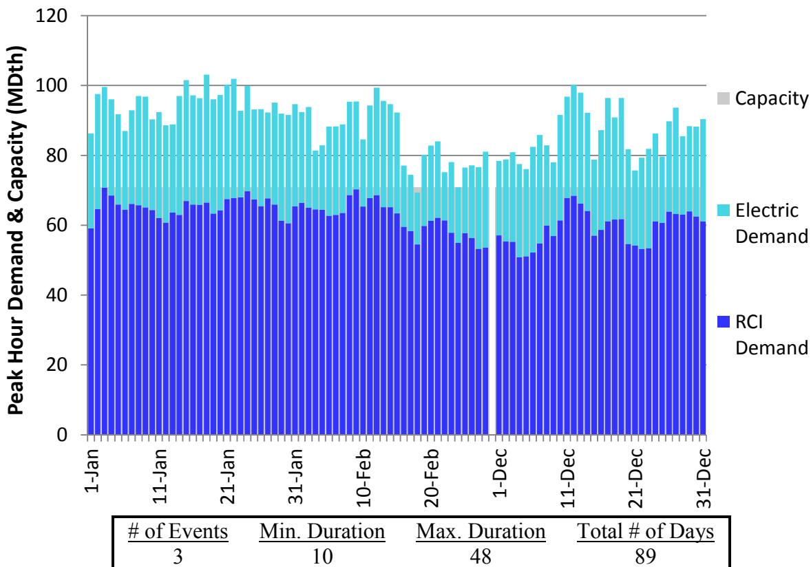
Figure U36. RGDS Roll-Up Winter 2018 – Transco Leidy Atlantic – Descending Demand
