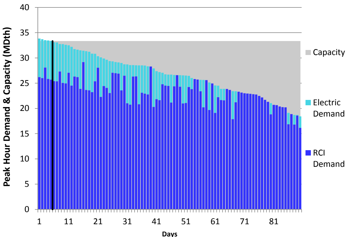
Figure U14. RGDS Roll-Up Winter 2018 – East Tennessee – Descending Demand
