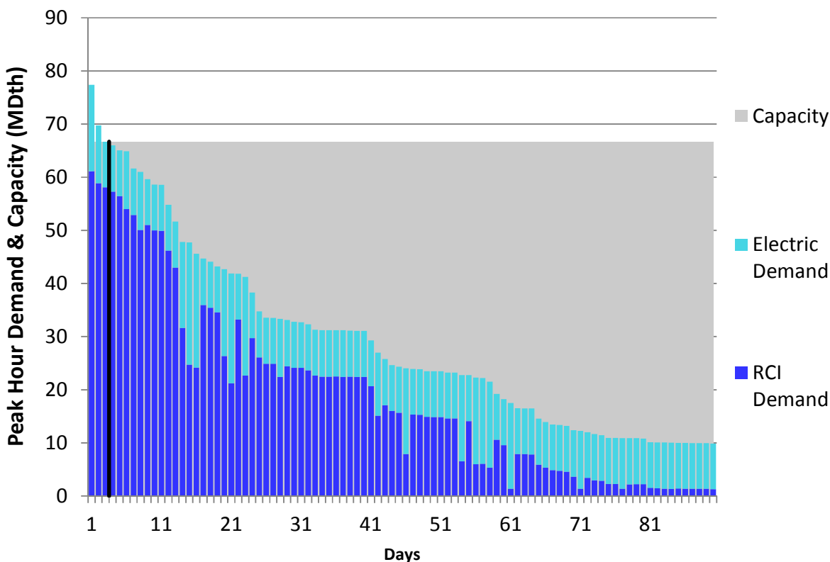
Figure U280. HGDS Roll-Up Winter 2023 – Vector Zone 1 – Descending Demand
