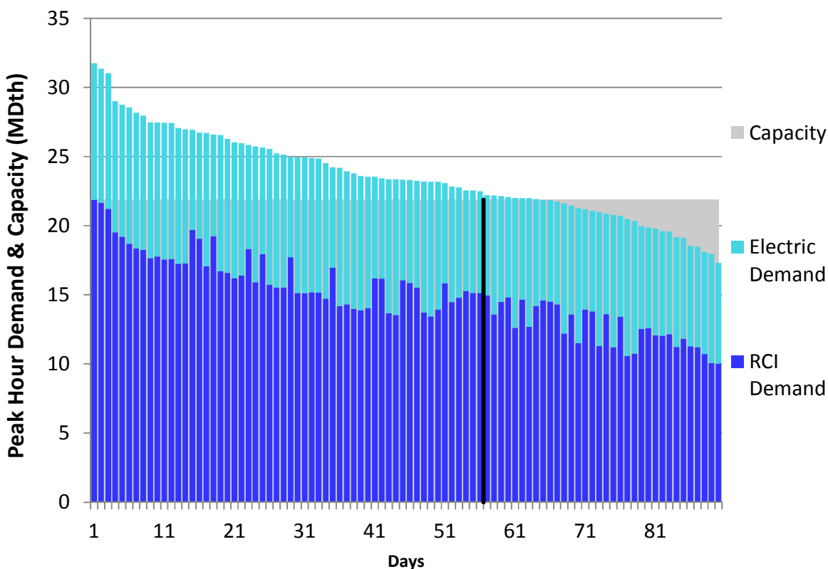
Figure U82. RGDS Roll-Up Winter 2023 – Empire – Descending Demand
