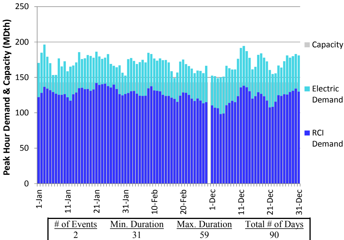
Figure U186. HGDS Roll-Up Winter 2018 – Transco Leidy to Station 210 – Descending Demand
