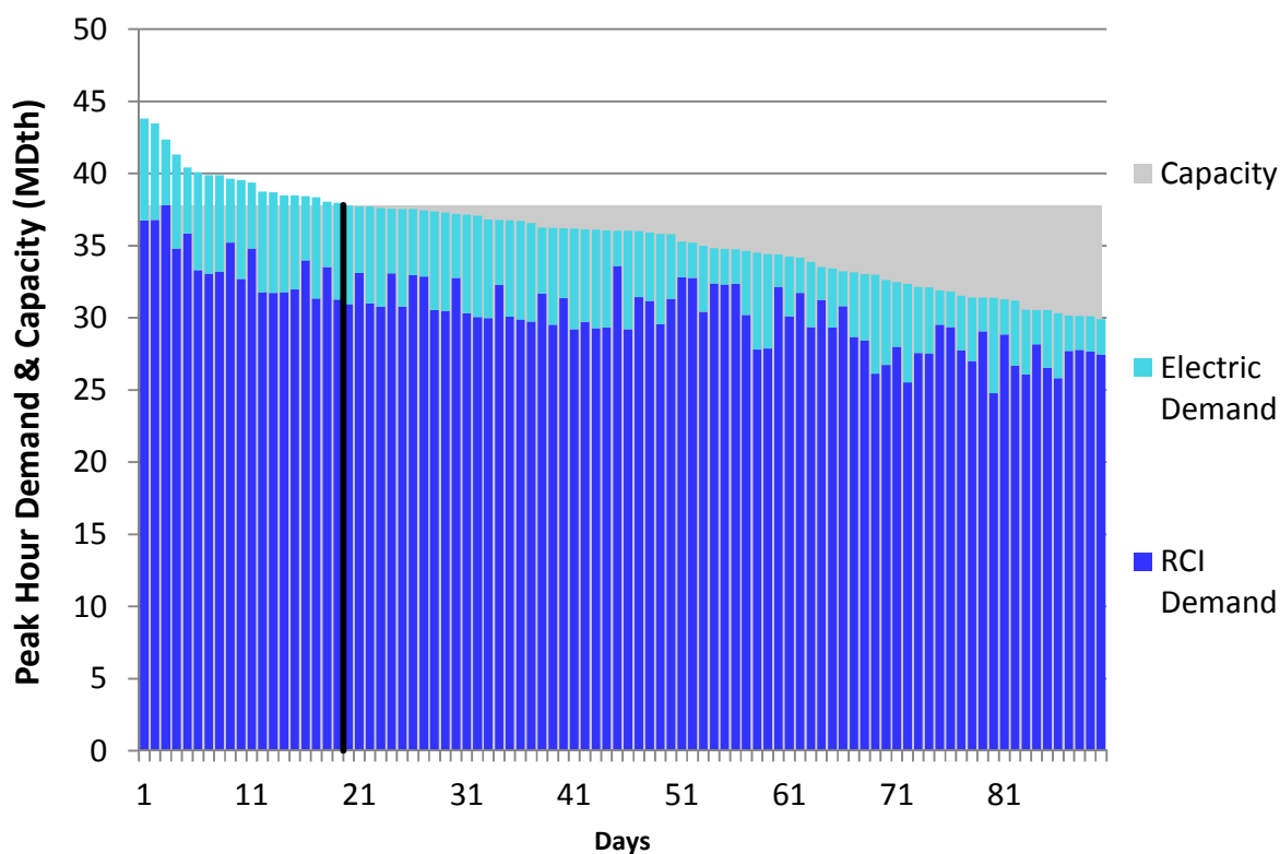
Figure U142. HGDS Roll-Up Winter 2018 – Dominion Eastern NY– Descending Demand
