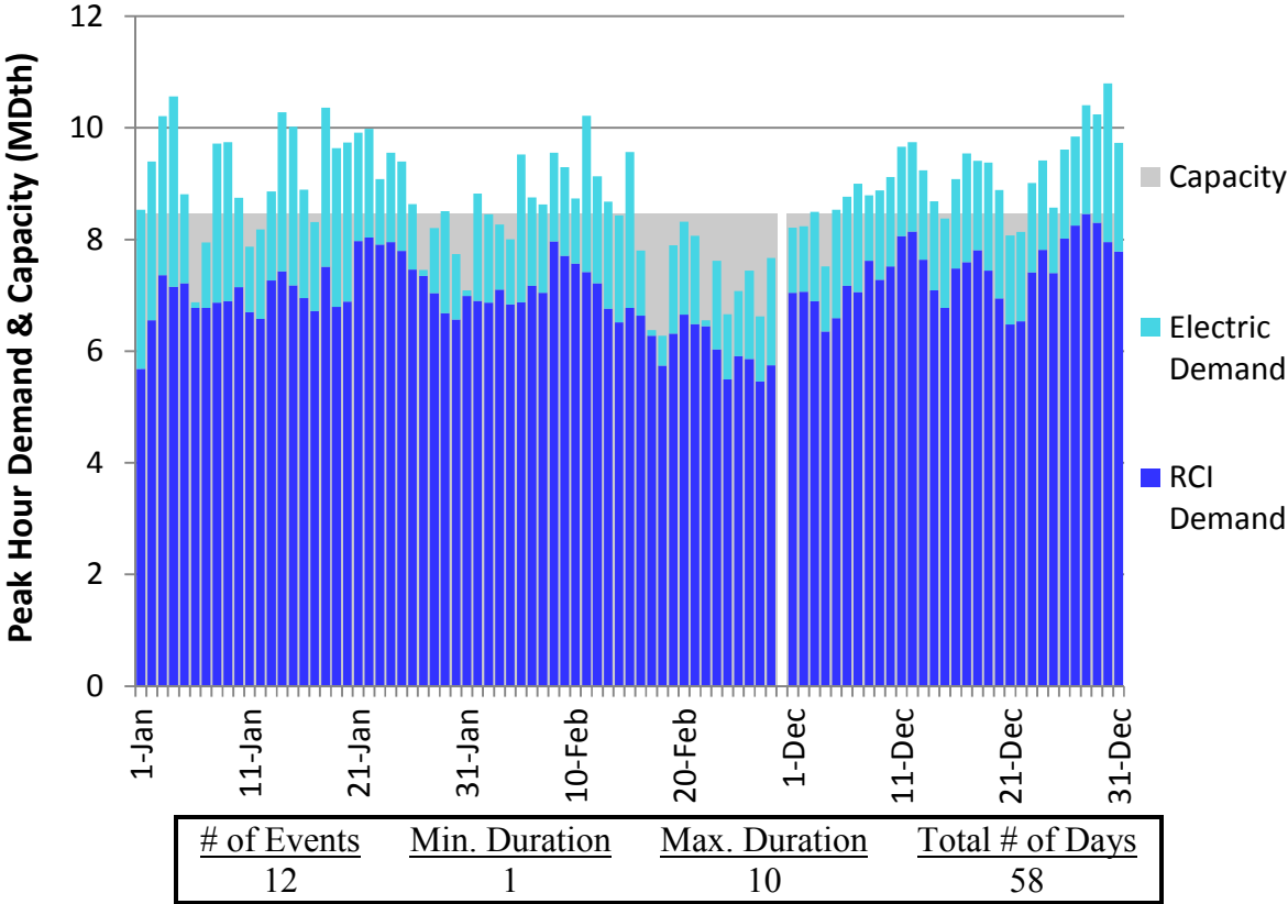
Figure U16. RGDS Roll-Up Winter 2018 – Eastern Shore – Descending Demand
