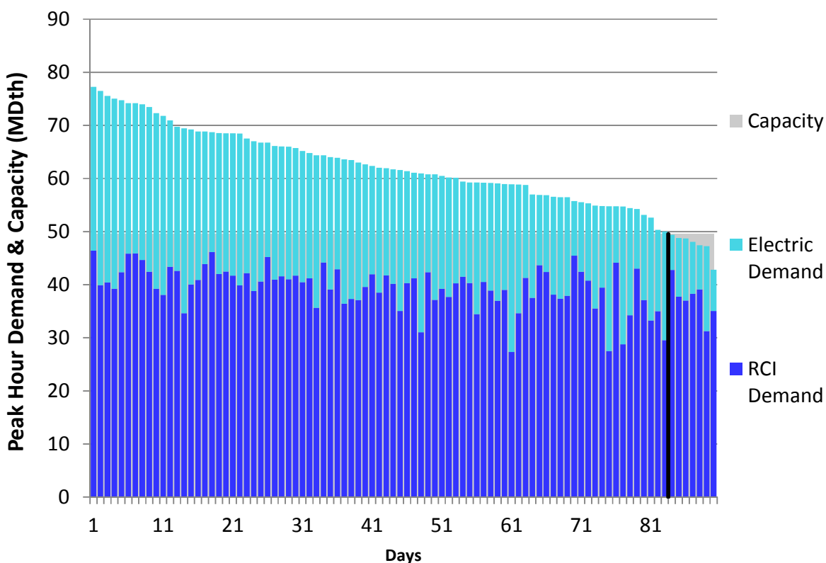
Figure U364. LGDS Roll-Up Winter 2023 – Tennessee Z5 NY – Descending Demand
