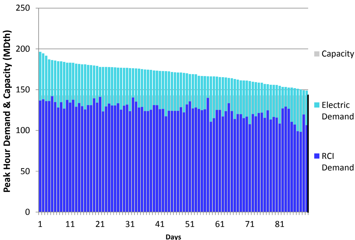
Figure U186. HGDS Roll-Up Winter 2018 – Transco Leidy to Station 210 – Descending Demand
