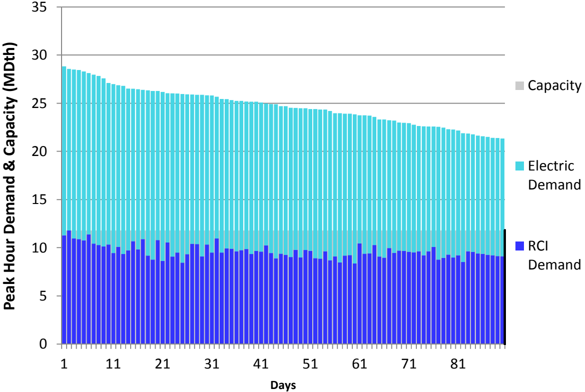
Figure U248. HGDS Roll-Up Winter 2023 – NB/NS Supply – Descending Demand
