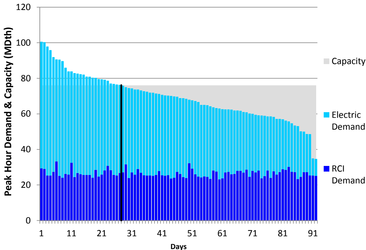
Figure U108. RGDS Roll-Up Summer 2023 – Algonquin CT – Descending Demand
