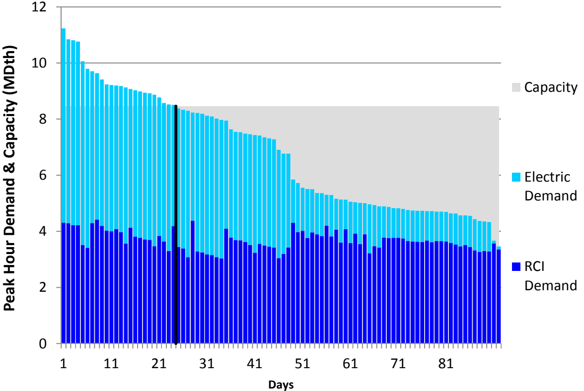
Figure U200. HGDS Roll-Up Summer 2018 – Eastern Shore – Descending Demand
