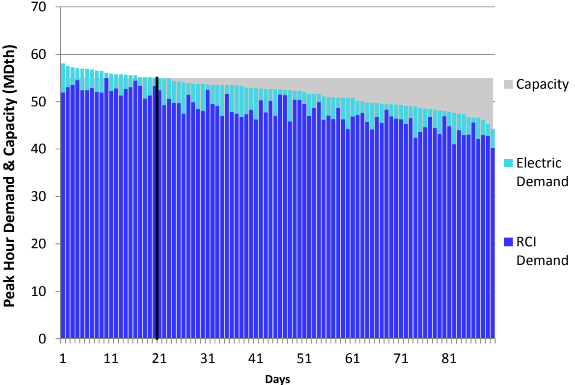
Figure U372. LGDS Roll-Up Winter 2023 – TransCanada Quebec – Descending Demand
