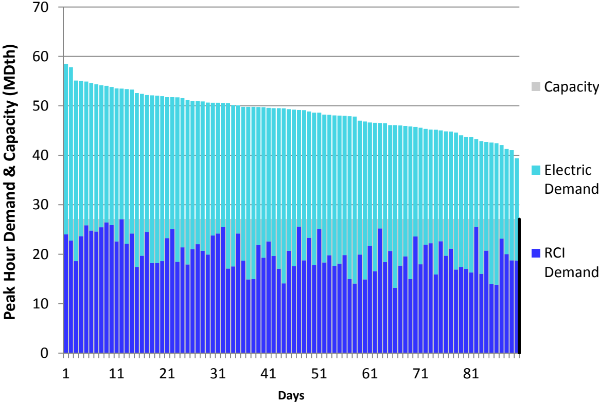
Figure U70. RGDS Roll-Up Winter 2023 – Constitution – Descending Demand
