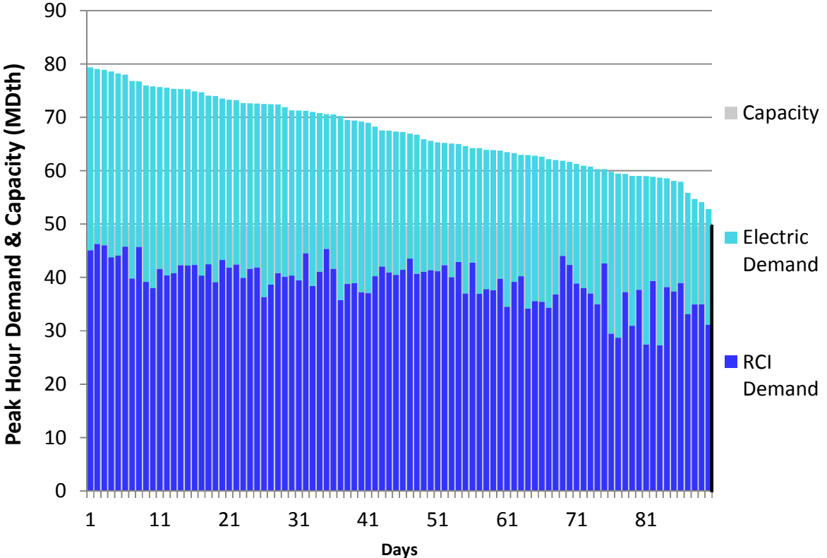
Figure U90. RGDS Roll-Up Winter 23 – Tennessee Z5 NY – Descending Demand
