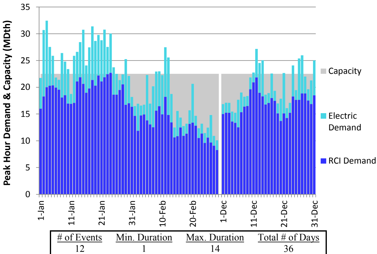
Figure U146. HGDS Roll-Up Winter 2018 – Dominion Southeast – Descending Demand
