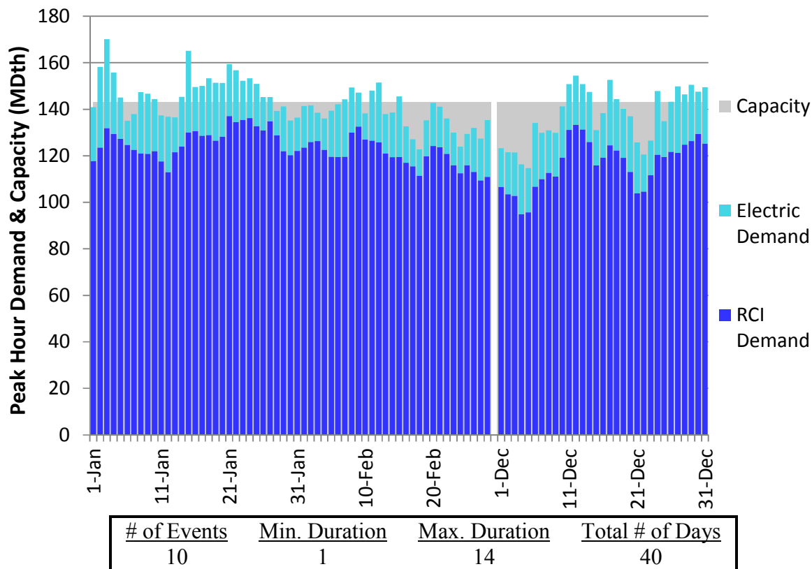
Figure U330. LGDS Roll-Up Winter 2018 – Transco Leidy to Station 210 – Descending Demand
