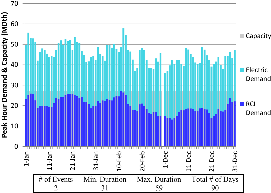
Figure U140. HGDS Roll-Up Winter 2018 – Constitution – Descending Demand
