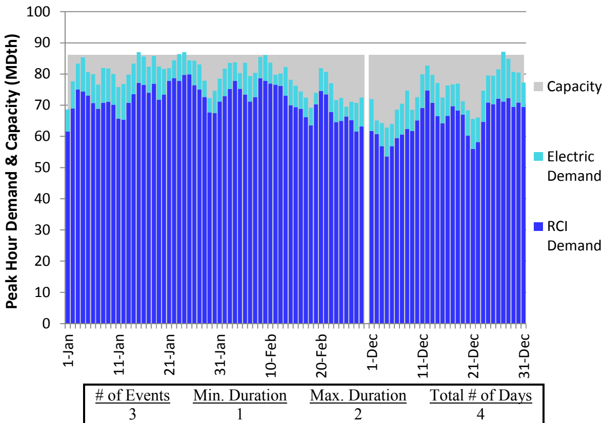
Figure U366. LGDS Roll-Up Winter 2023 – Texas Eastern M2 PA South – Descending Demand
