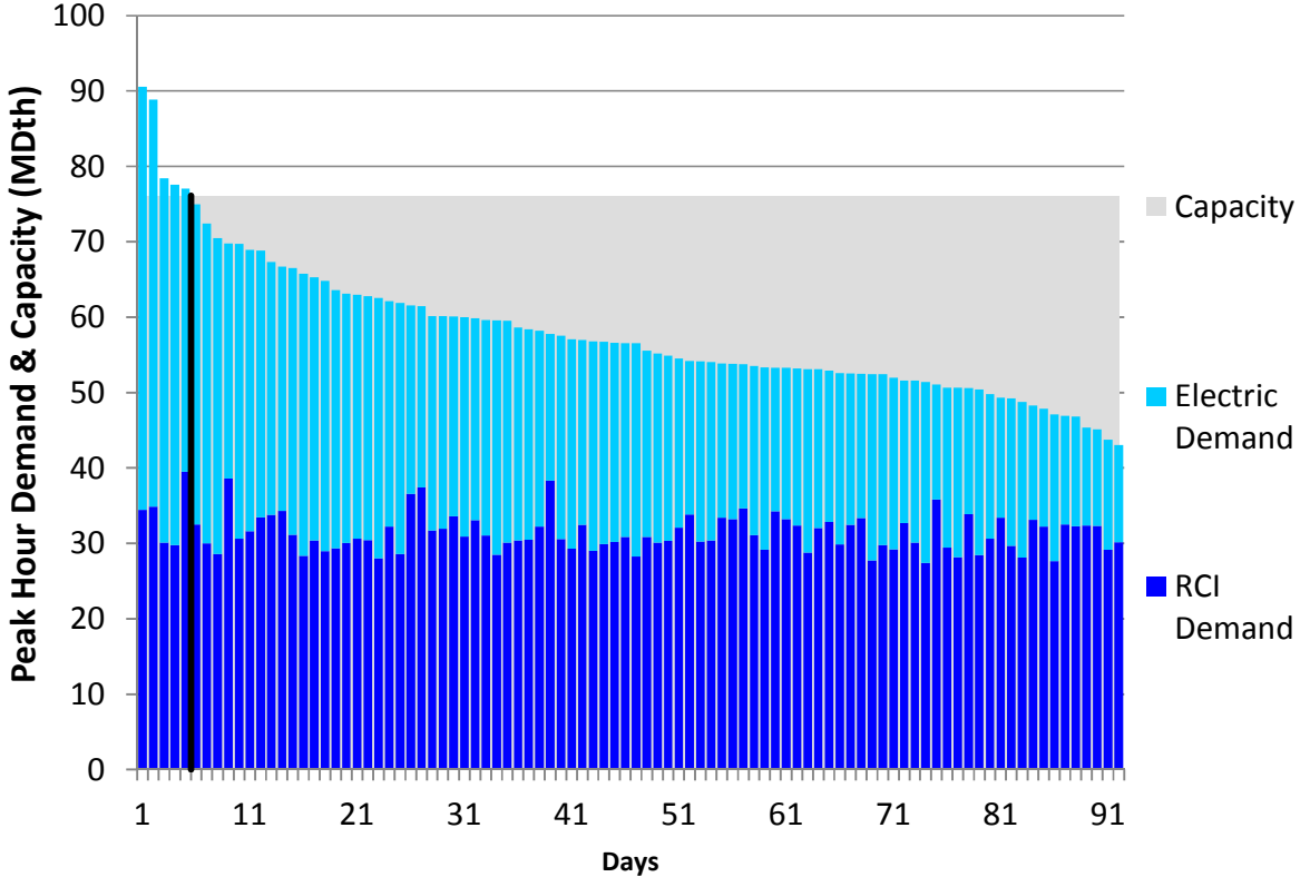
Figure U380. LGDS Roll-Up Summer 23 – Algonquin CT – Descending Demand
