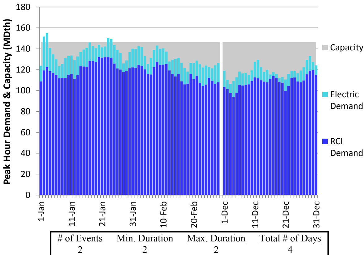
Figure U268. HGDS Roll-Up Winter 2023 – TransCanada Ontario West – Descending Demand
