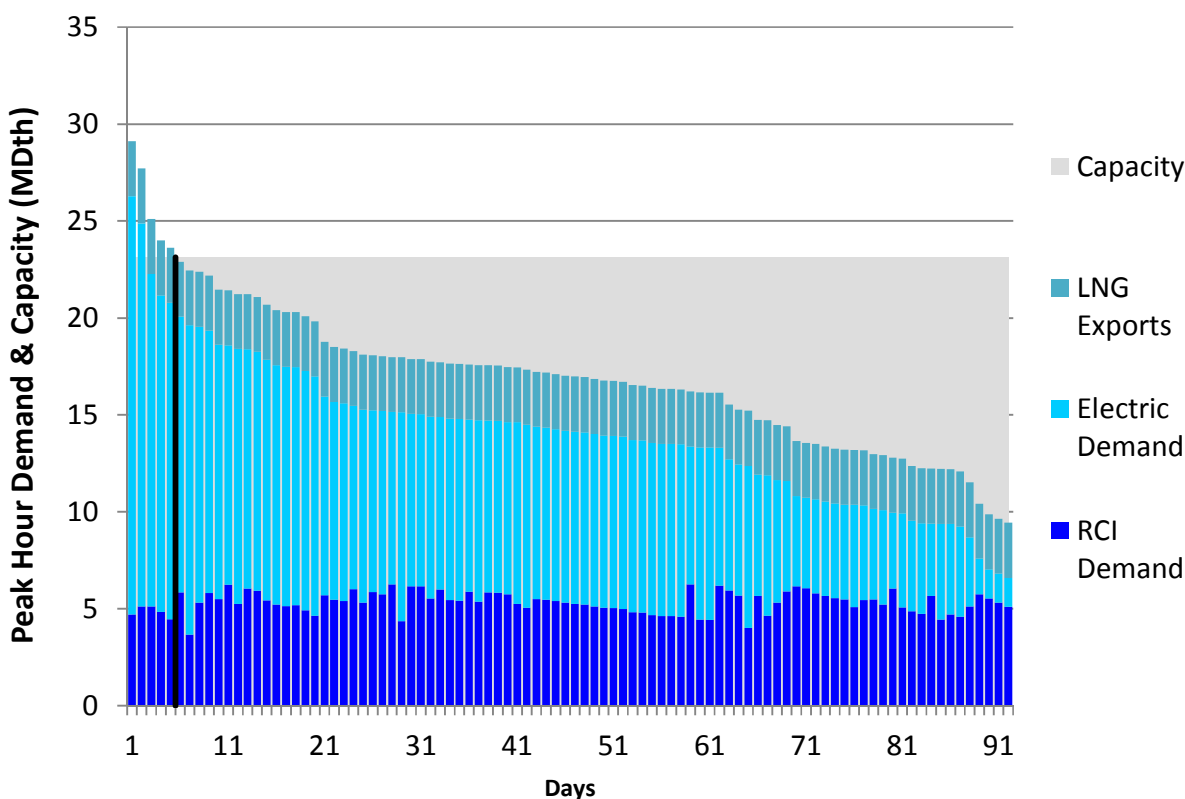
Figure U384. LGDS Roll-Up Summer 2023 – Dominion Southeast – Descending Demand
