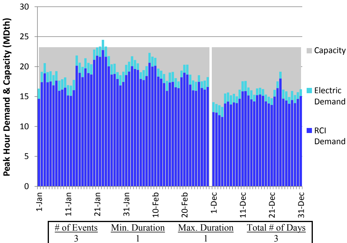
Figure U352. LGDS Roll-Up Winter 2023 – Dominion Western NY– Descending Demand
