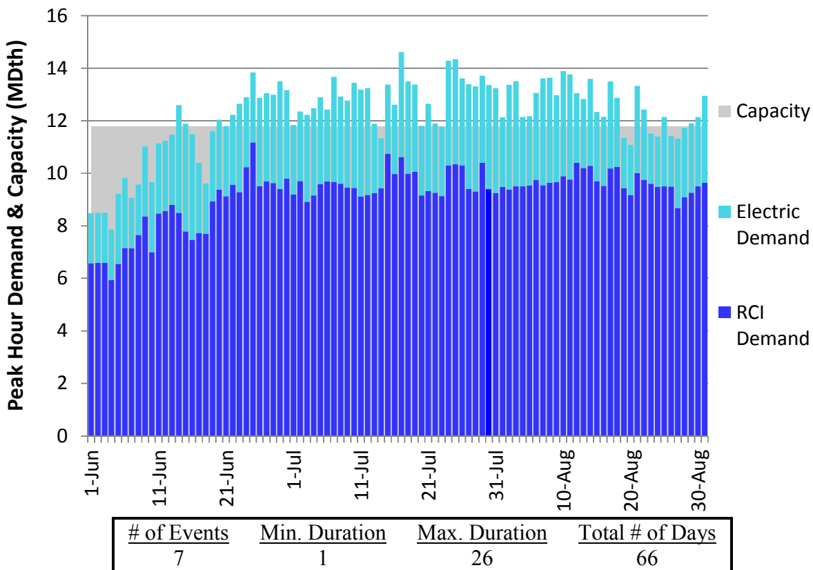
Figure U388. LGDS Roll-Up Summer 23 – NB/NS Supply – Descending Demand
