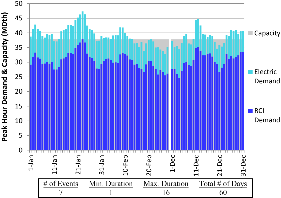
Figure U72. RGDS Roll-Up Winter 2023 – Dominion Eastern NY– Descending Demand
