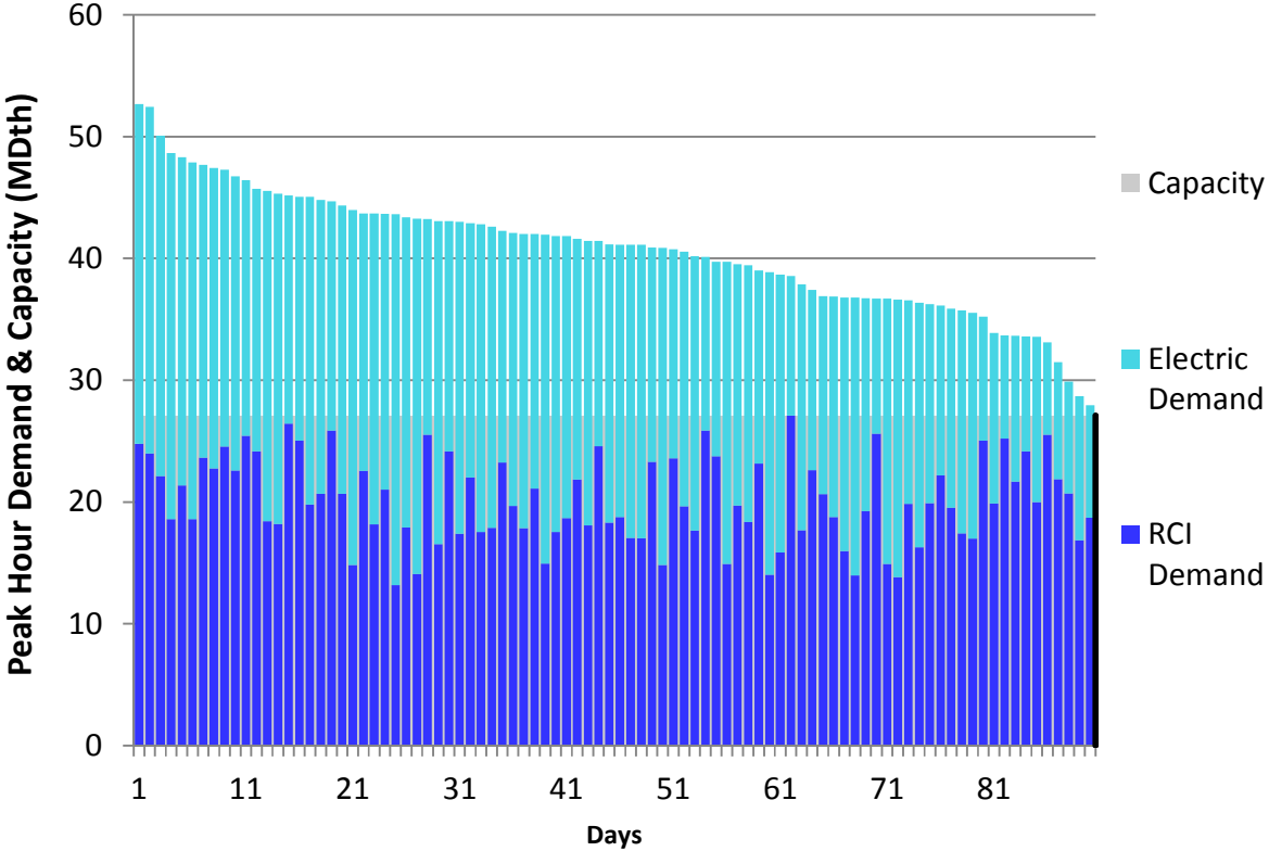
Figure U348. LGDS Roll-Up Winter 2023 – Constitution – Descending Demand
