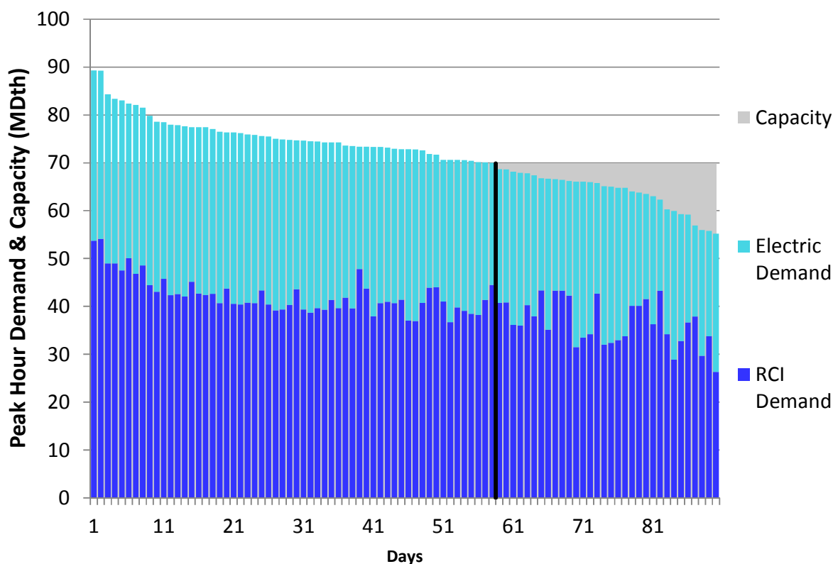
Figure U250. HGDS Roll-Up Winter 2023 – NGPL IA/IL North – Descending Demand
