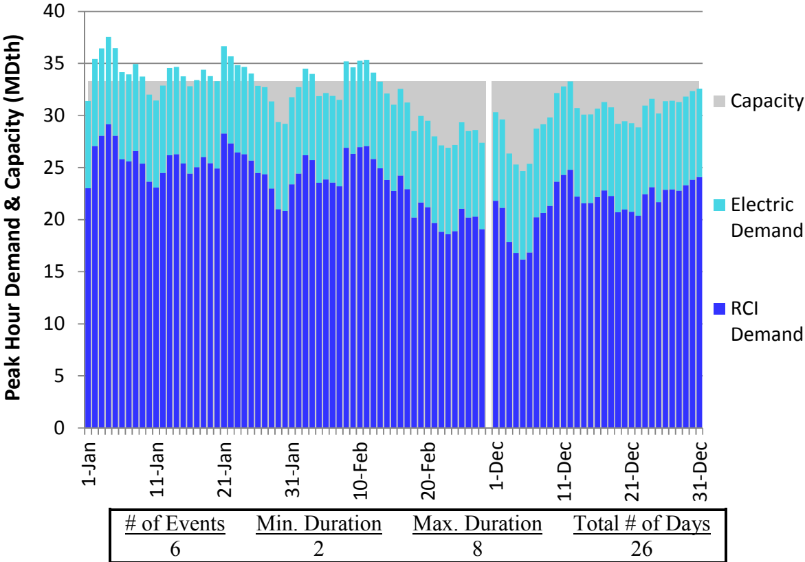
Figure U148. HGDS Roll-Up Winter 2018 – East Tennessee – Descending Demand
