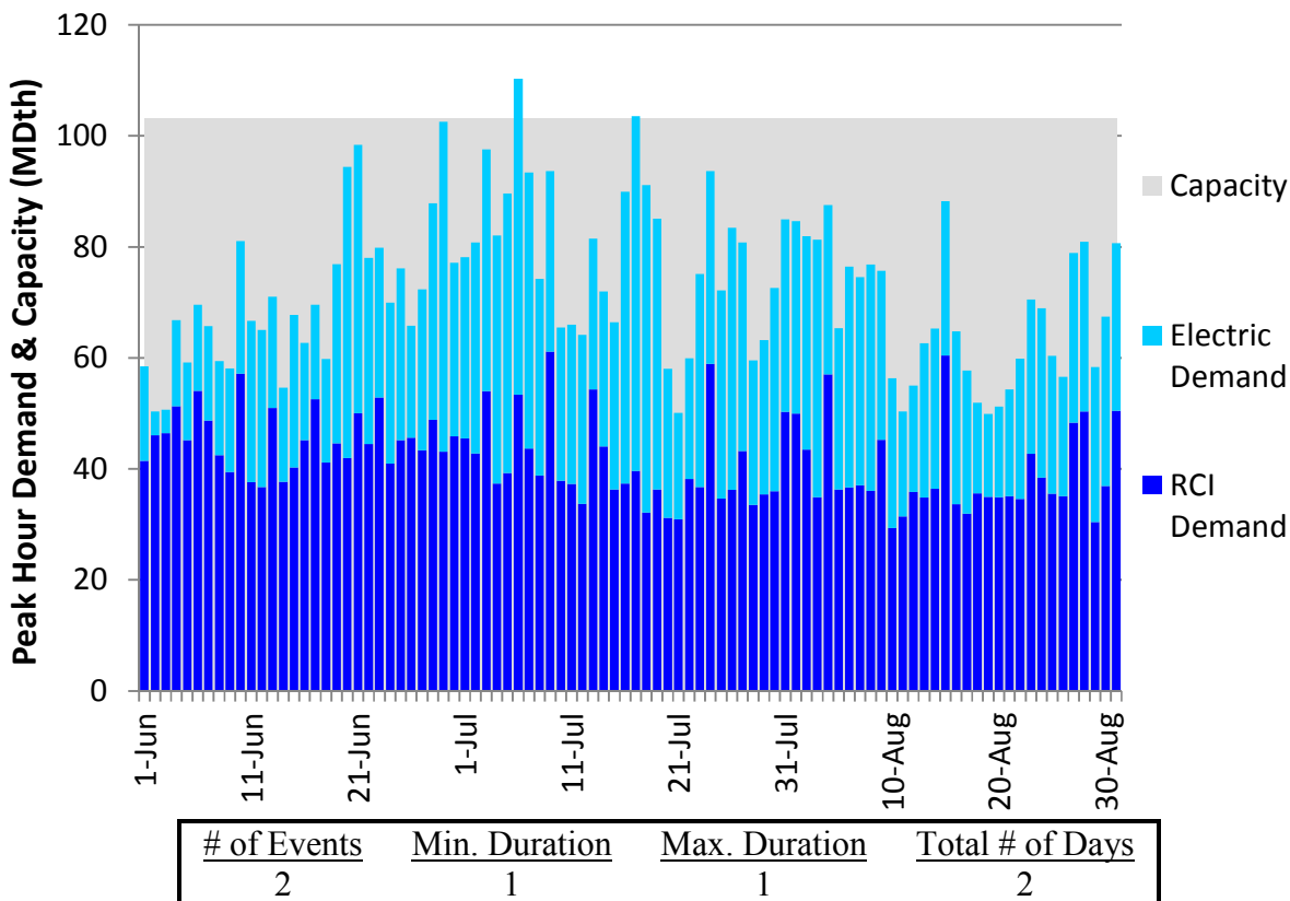
Figure U334. LGDS Roll-Up Summer 2018 – Columbia Gas VA/MD – Descending Demand
