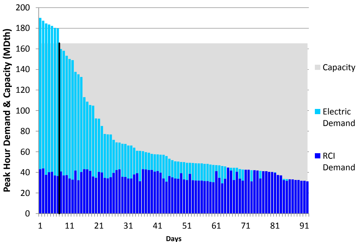
Figure U342. LGDS Roll-Up Summer 2018 – Transco Z5 – Descending Demand
