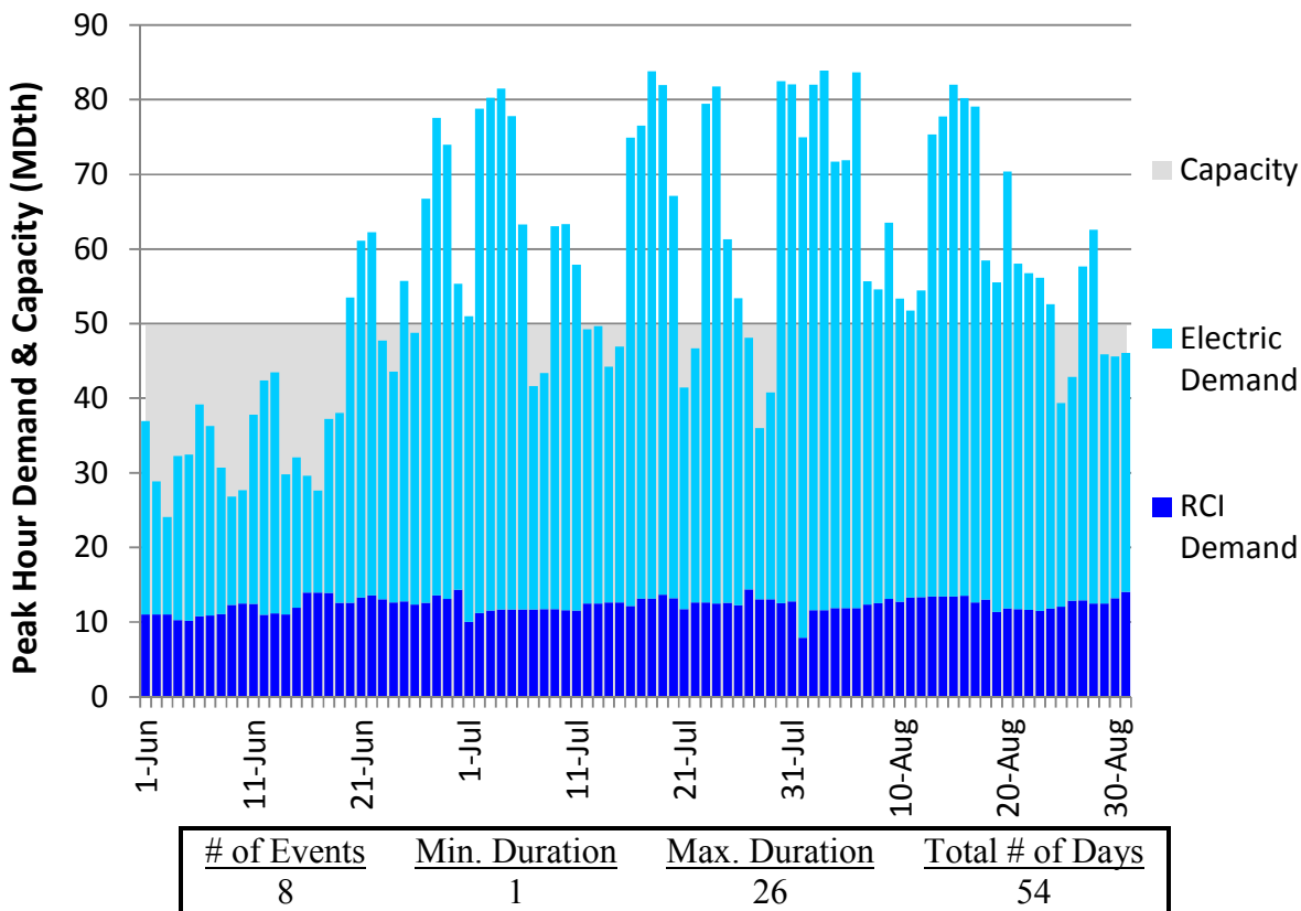
Figure U202. HGDS Roll-Up Summer 2018 – Iroquois Zone 1 – Descending Demand
