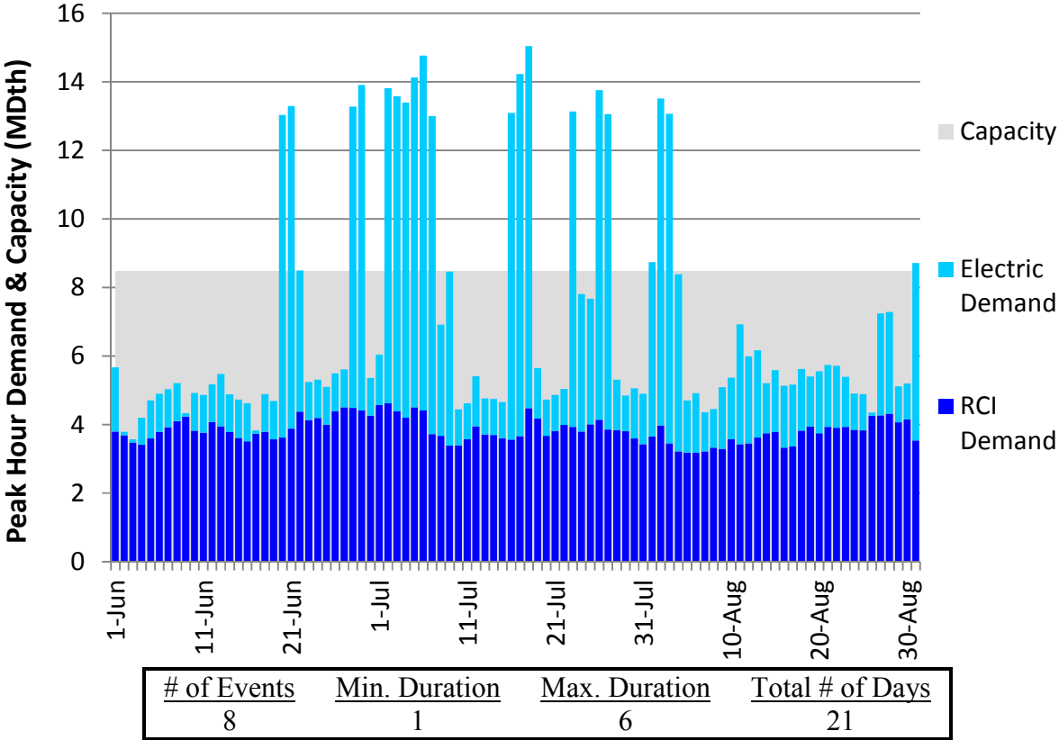
Figure N160. RGDS S19 Summer 2018 – Eastern Shore – Descending Demand
