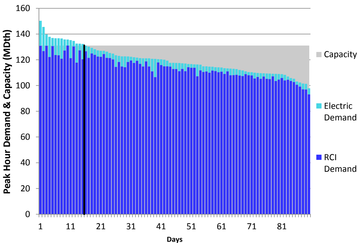
Figure N144. RGDS S19 Winter 2018 – TransCanada Ontario West – Descending Demand
