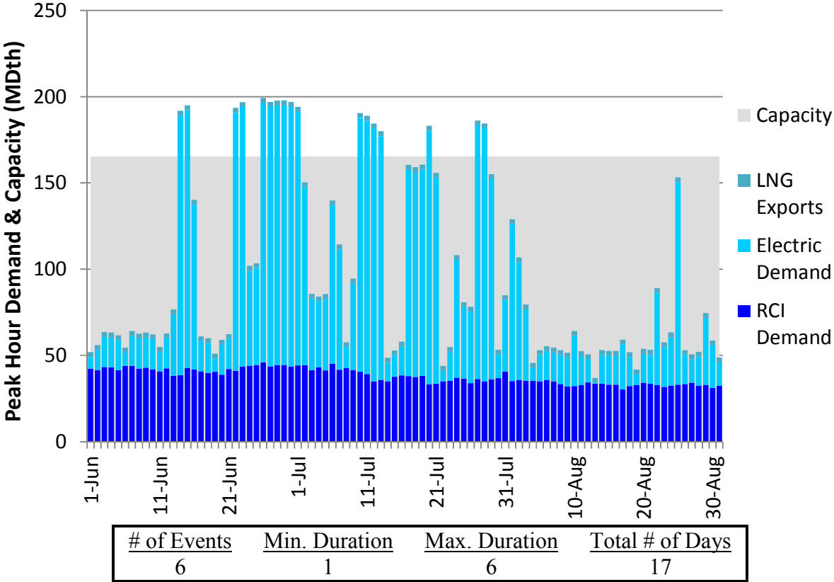
Figure N112. RGDS S18 Summer 2023 – Transco Z5 – Descending Demand
