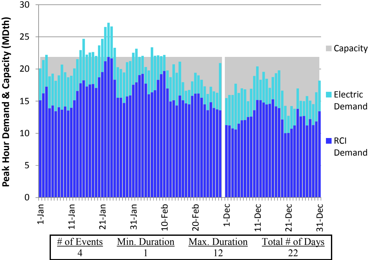
Figure N130. RGDS S19 Winter 2018 – Empire – Descending Demand
