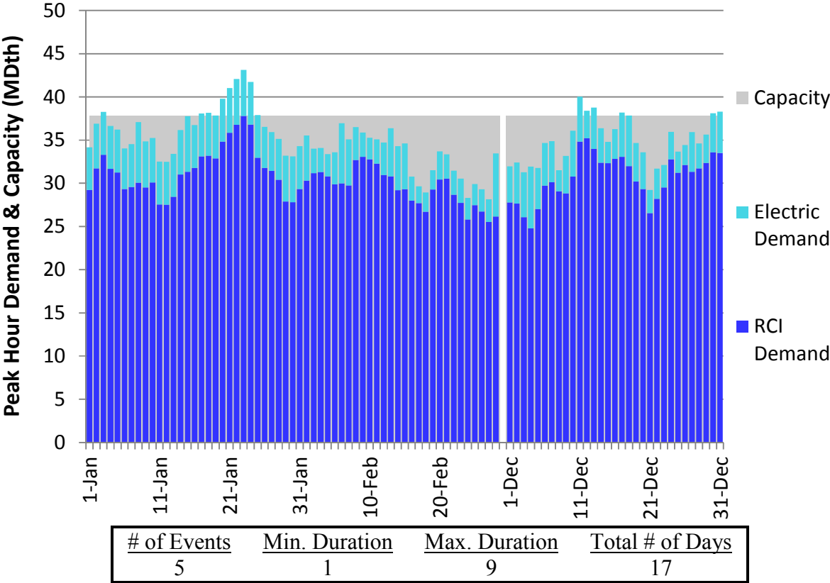
Figure N120. RGDS S19 Winter 2018 – Dominion Eastern NY– Descending Demand
