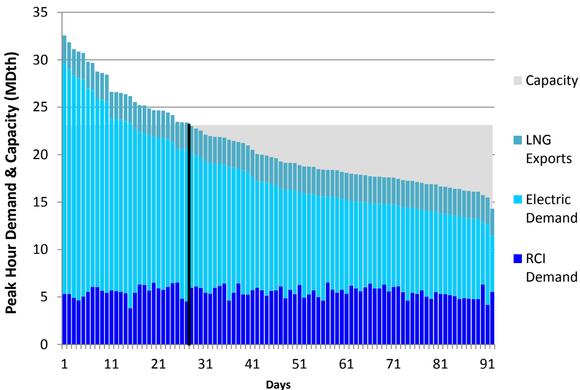
Figure N210. RGDS S19 Summer 2023 – Dominion Southeast – Descending Demand
