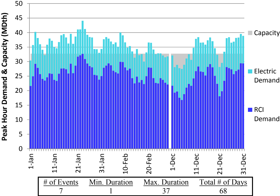
Figure N184. RGDS S19 Winter 2023 – Millennium – Descending Demand
