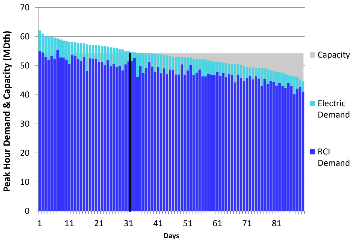
Figure N34. RGDS S18 Winter 2018 – TransCanada Quebec – Descending Demand
