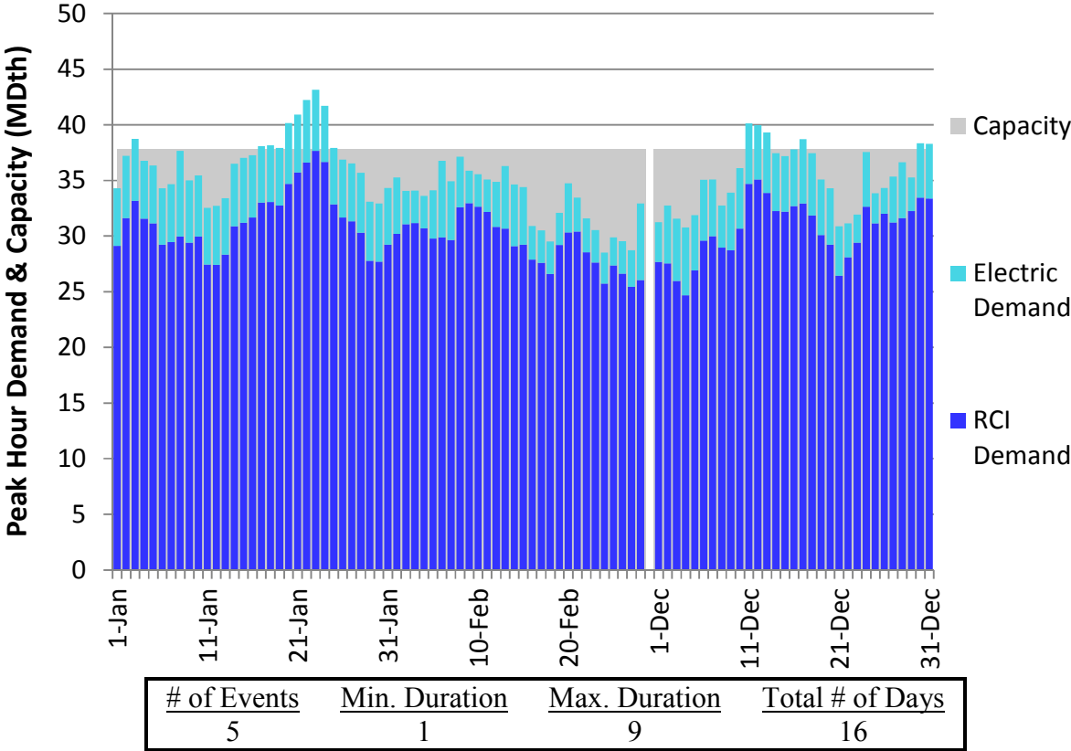
Figure N8. RGDS S18 Winter 2018 – Dominion Eastern NY– Descending Demand
