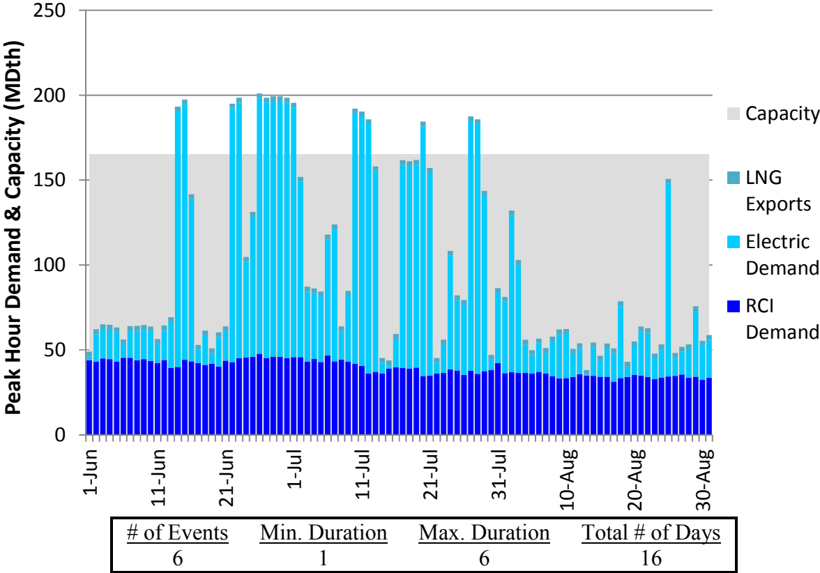
Figure N230. RGDS S19 Summer 2023 – Transco Z5 – Descending Demand
