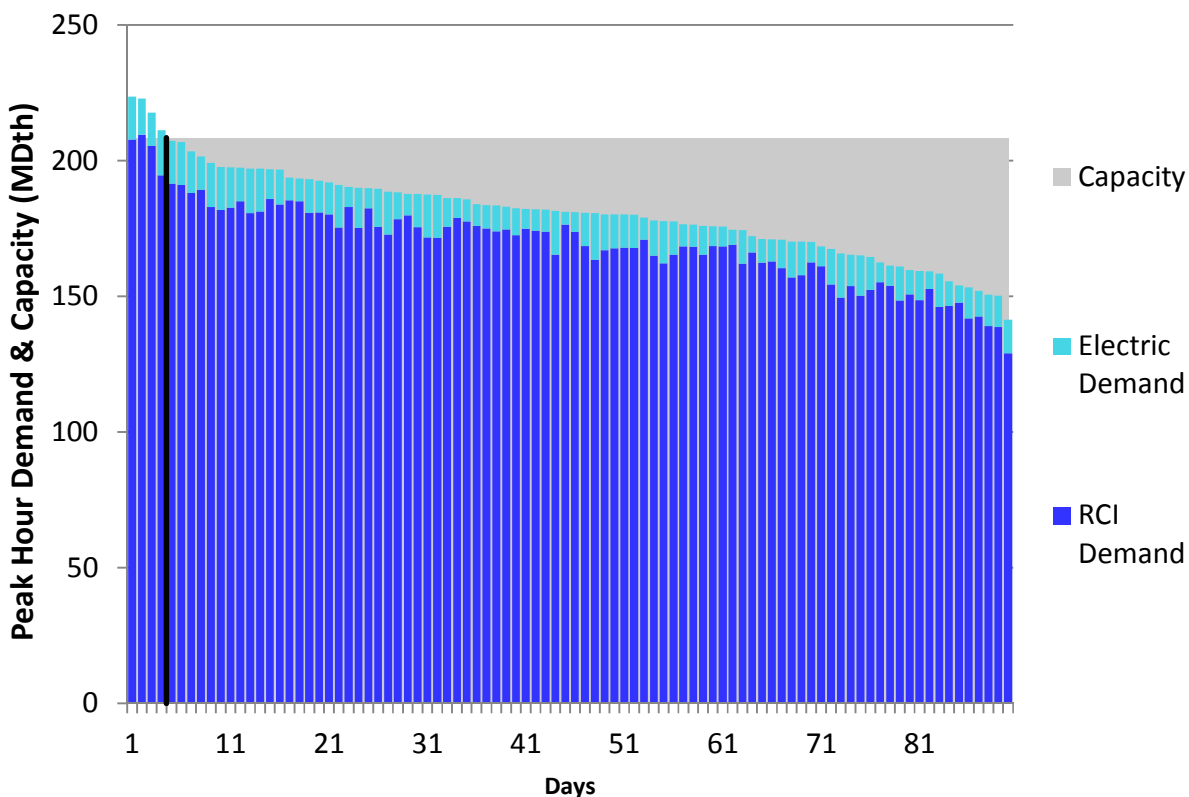
Figure N42. RGDS S18 Winter 2018 – Union Gas Dawn – Descending Demand
