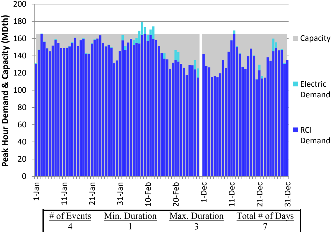
Figure N38. RGDS S18 Winter 2018 – Transco Z5 – Descending Demand
