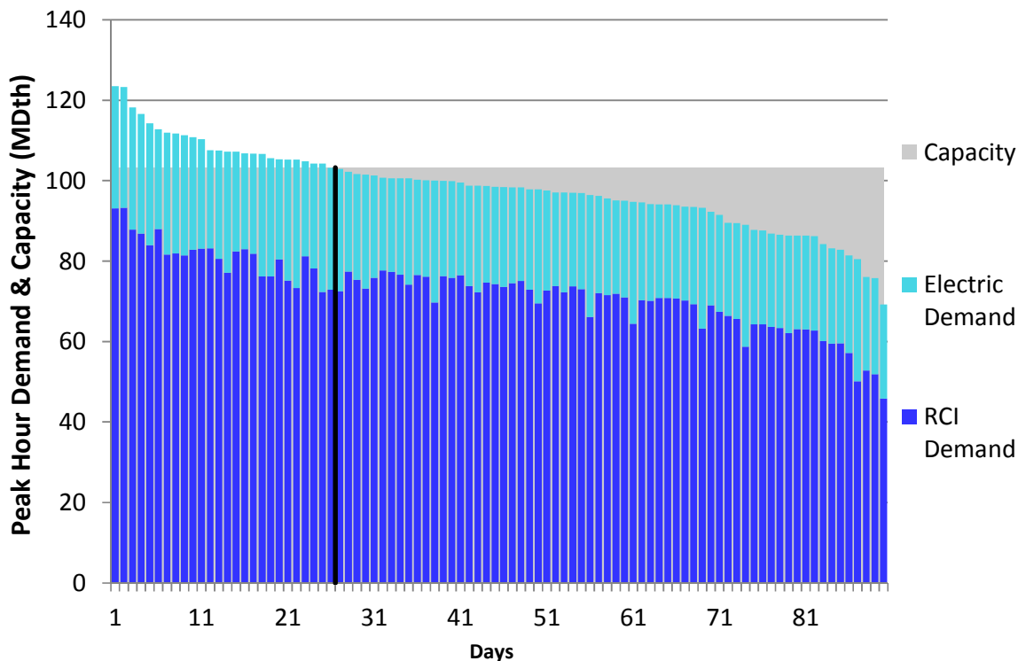
Figure N114. RGDS S19 Winter 2018 – Columbia Gas VA/MD – Descending Demand
