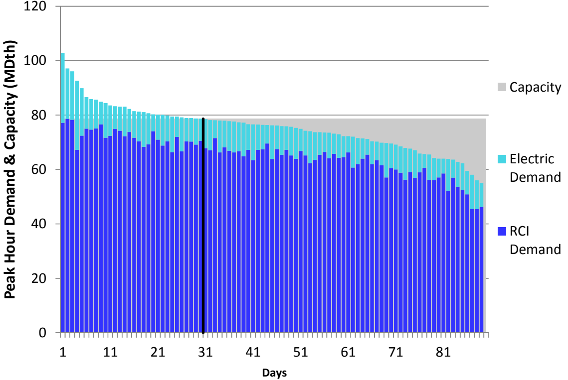
Figure N136. RGDS S19 Winter 2018 – Tennessee Z4 PA – Descending Demand
