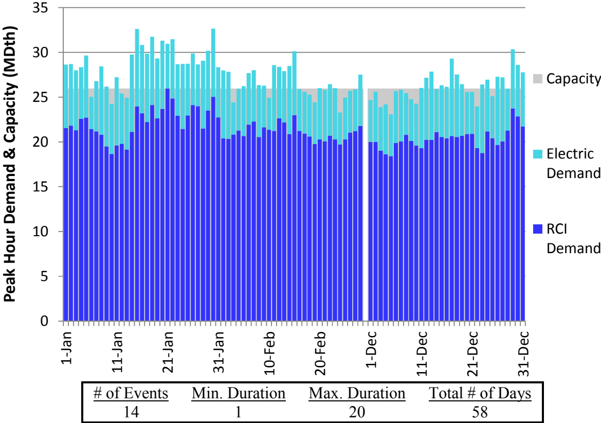
Figure N22. RGDS S18 Winter 2018 – NB/NS – Descending Demand
