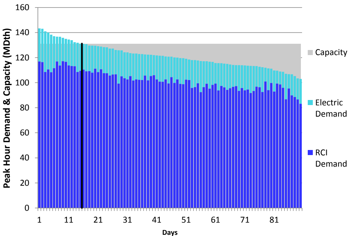
Figure N196. RGDS S19 Winter 2023 – TransCanada Ontario West – Descending Demand
