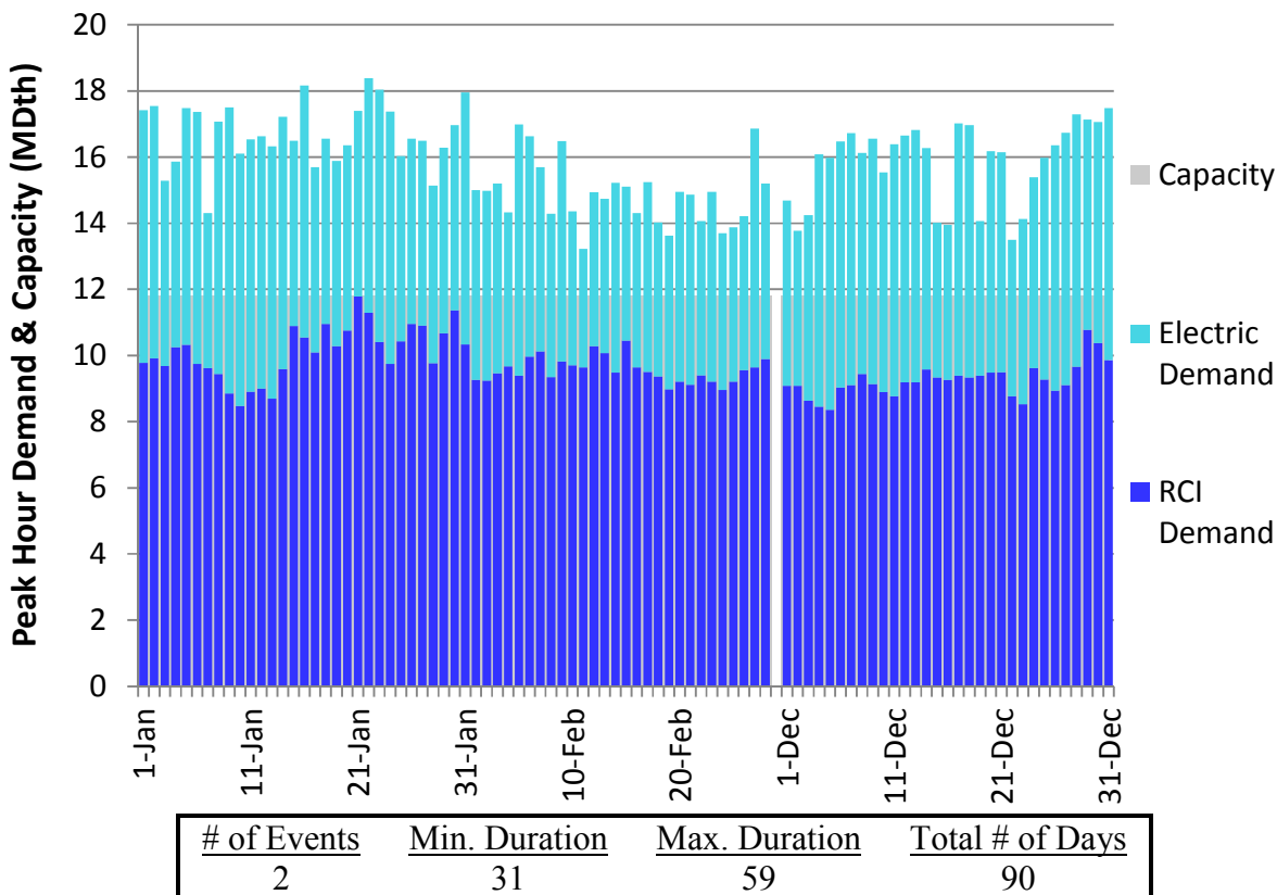
Figure N74. RGDS S18 Winter 2023 – NB/NS – Descending Demand
