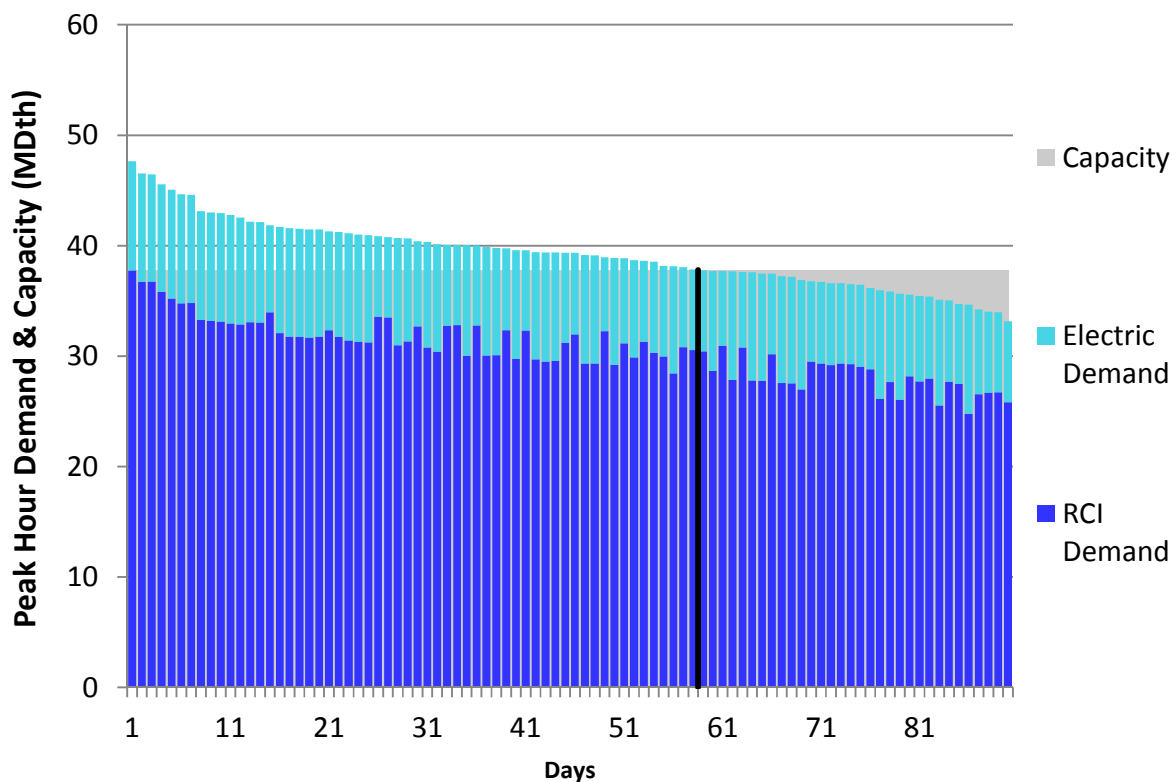
Figure N60. RGDS S18 Winter 2023 – Dominion Eastern NY– Descending Demand
