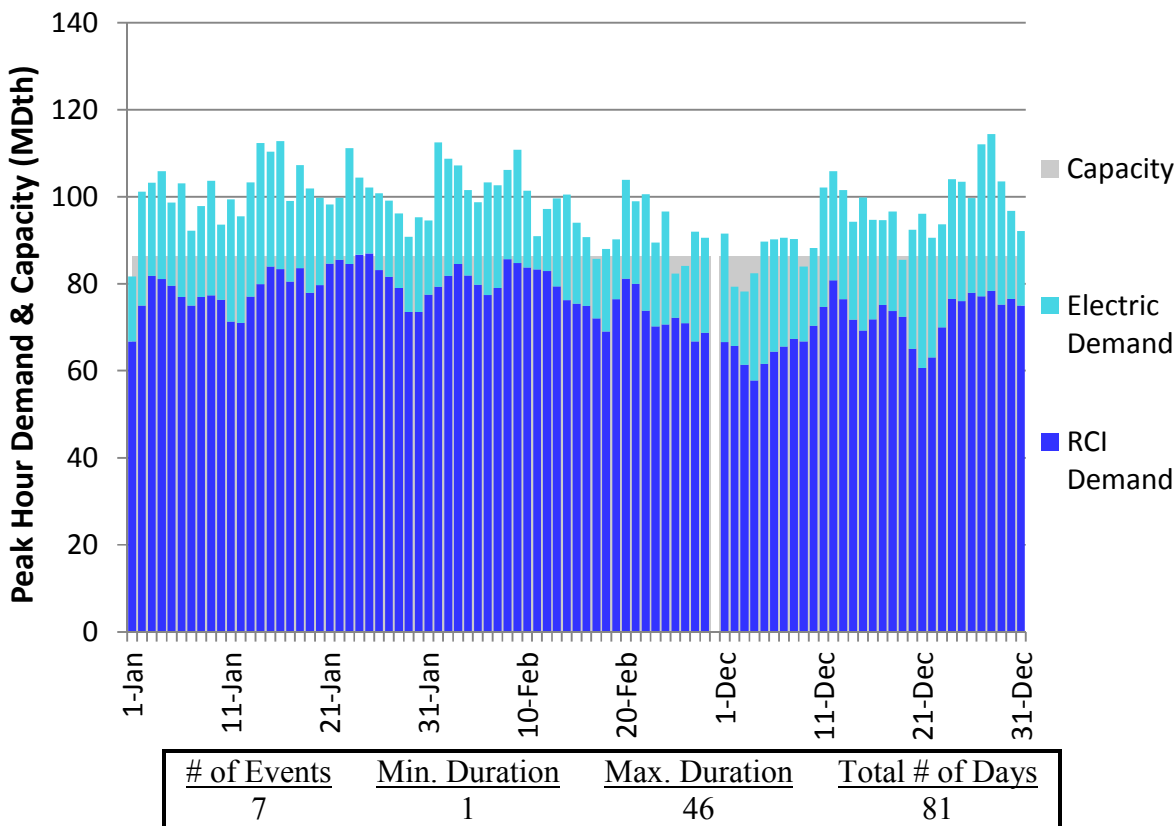
Figure N192. RGDS S19 Winter 2023 – Texas Eastern M2 PA South – Descending Demand
