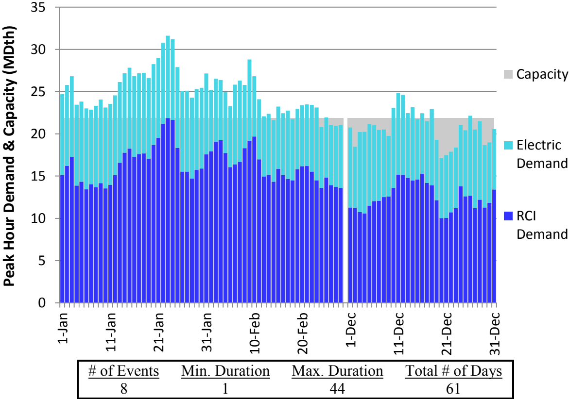
Figure N182. RGDS S19 Winter 23 – Empire – Descending Demand
