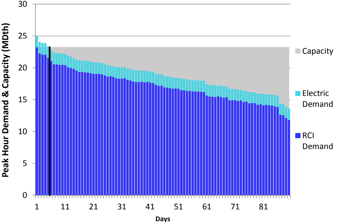
Figure N62. RGDS S18 Winter 2023 – Dominion Western NY– Descending Demand
