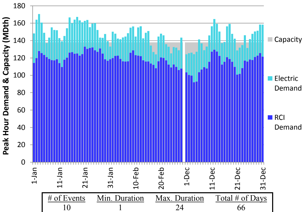
Figure N152. RGDS S19 Winter 2018 – Transco Leidy to Station 210 – Descending Demand
