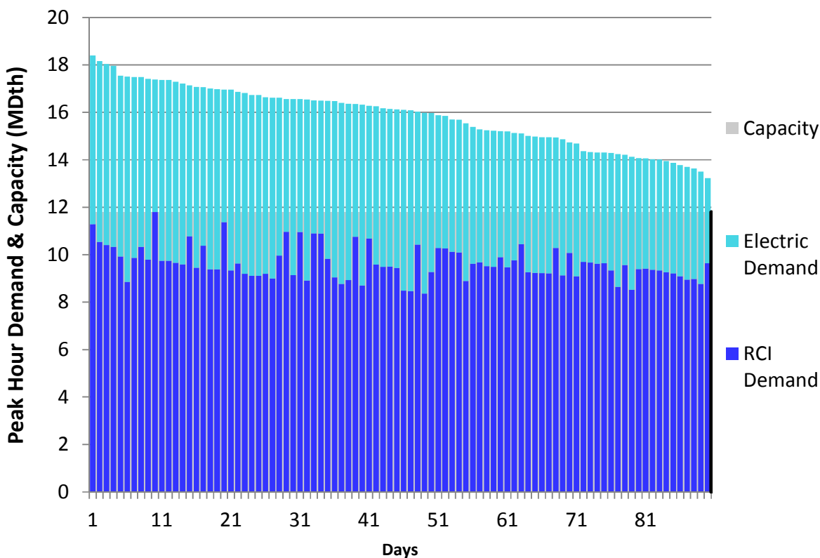
Figure N74. RGDS S18 Winter 2023 – NB/NS – Descending Demand
