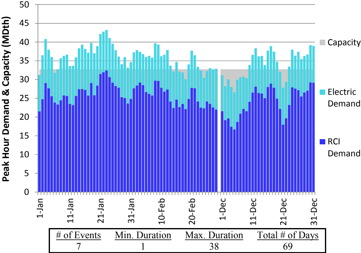
Figure N20. RGDS S18 Winter 2018 – Millennium – Descending Demand
