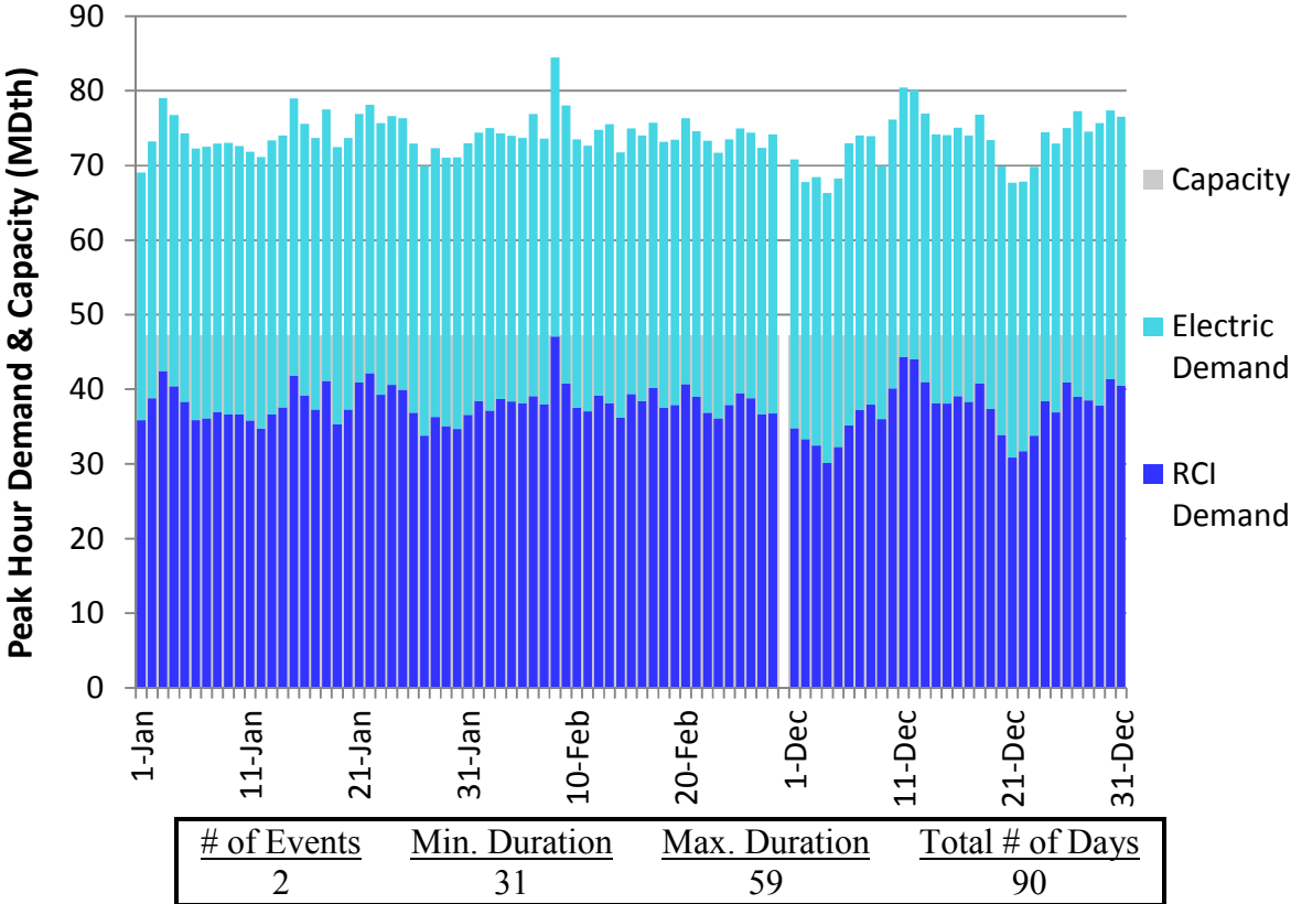
Figure N56. RGDS S18 Winter 2023 – Columbia Gas W PA/NY – Descending Demand
