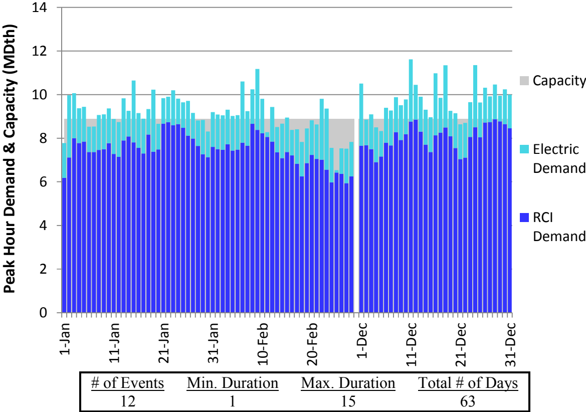
Figure N180. RGDS S19 Winter 2023 – Eastern Shore – Descending Demand
