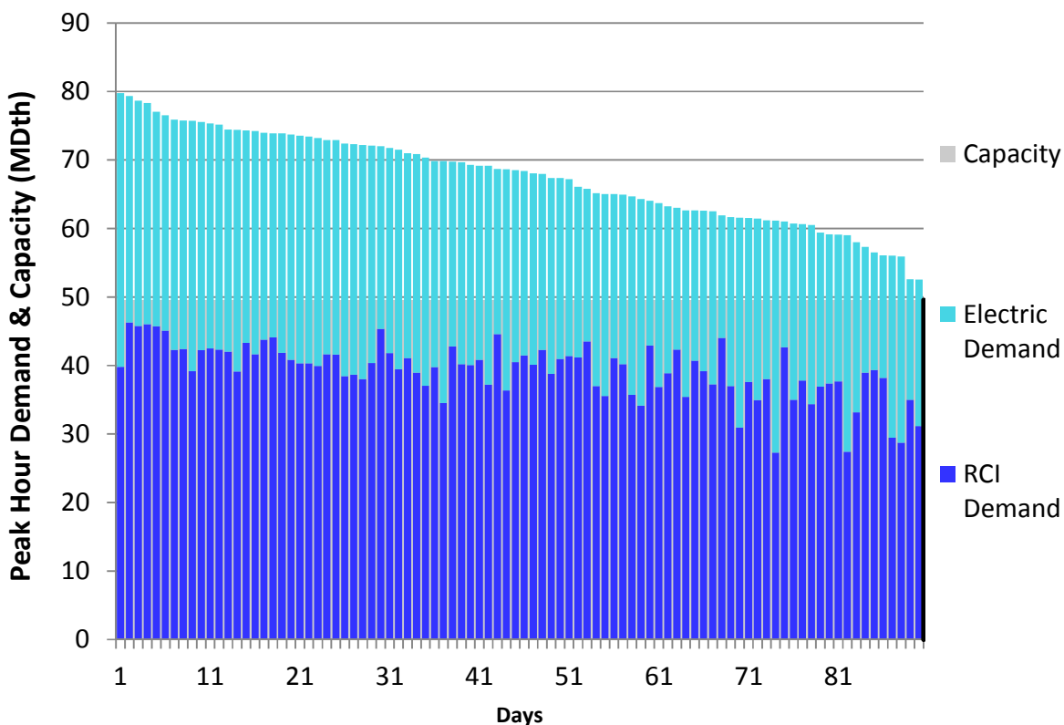
Figure N78. RGDS S18 Winter 2023 – Tennessee Z5 NY – Descending Demand
