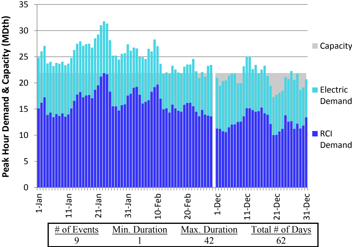
Figure N70. RGDS S18 Winter 2023 – Empire – Descending Demand
