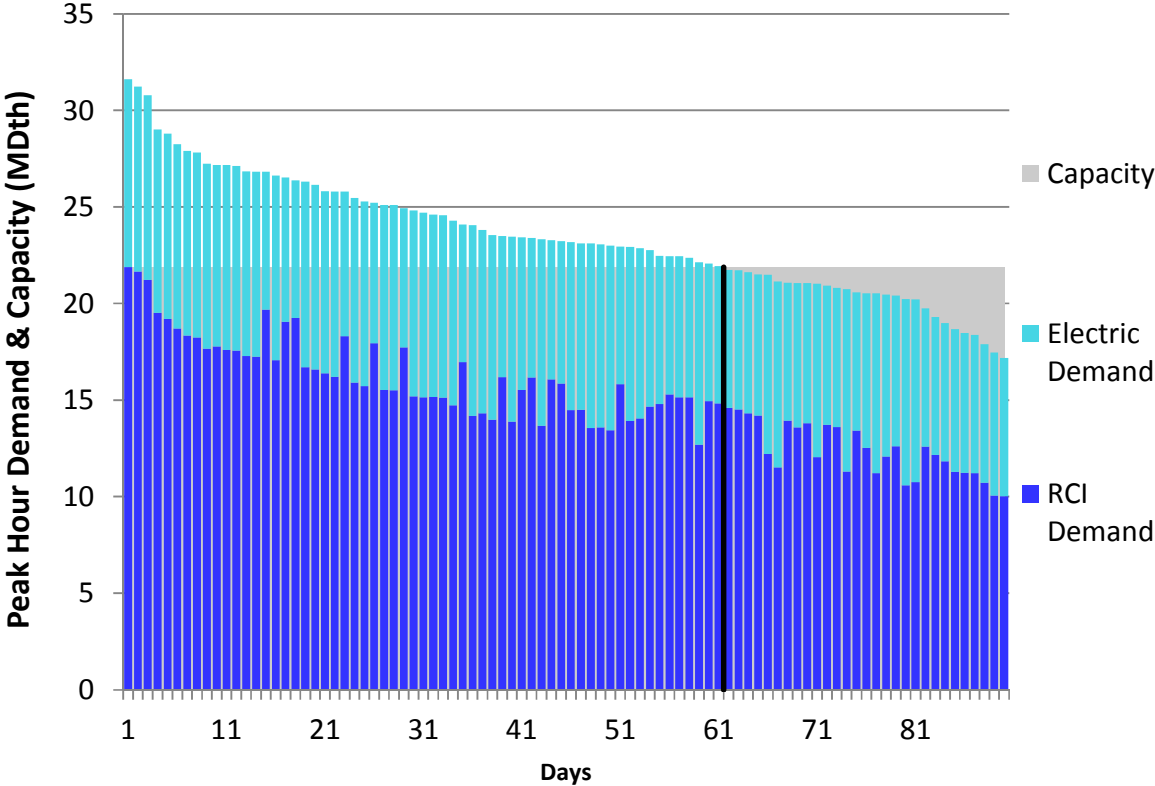
Figure N182. RGDS S19 Winter 23 – Empire – Descending Demand
