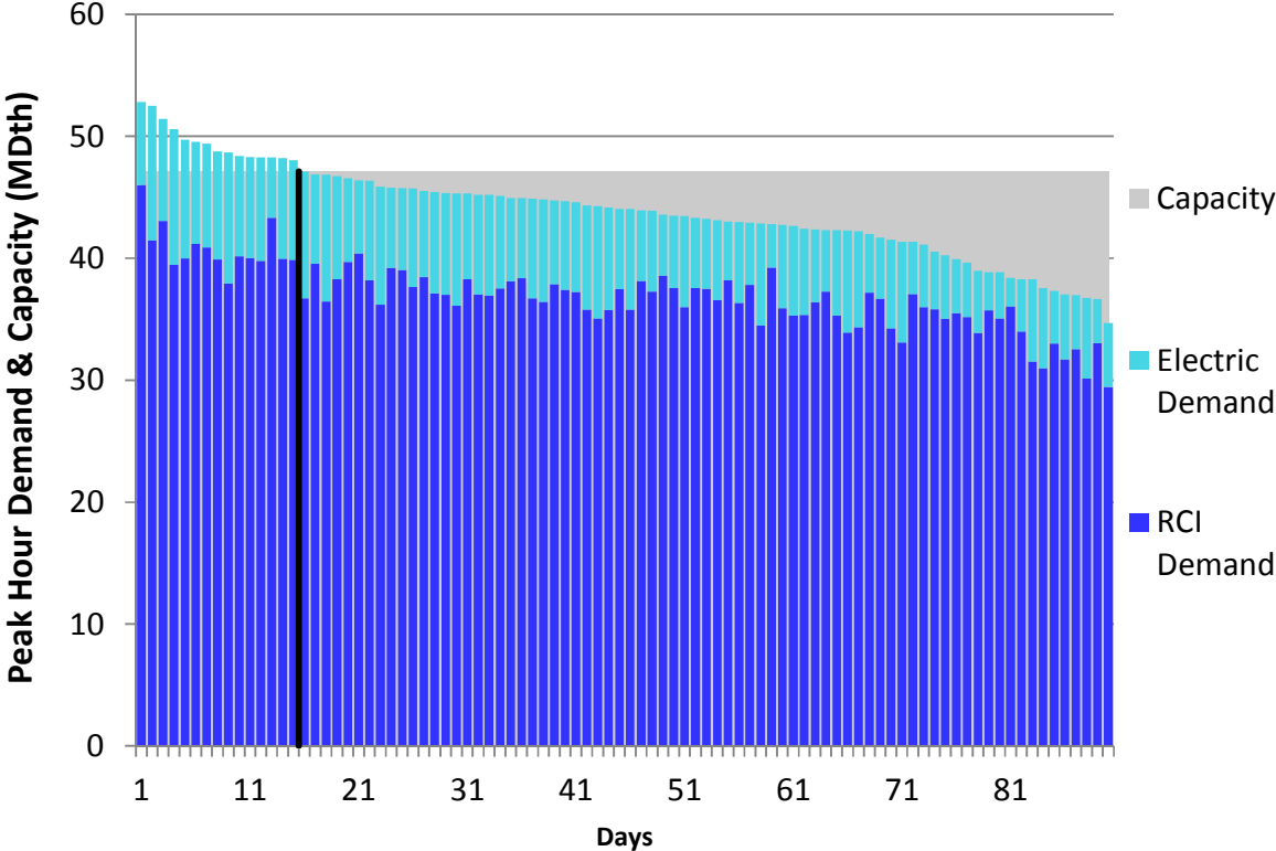
Figure N4. RGDS S18 Winter 2018 – Columbia Gas W PA/NY – Descending Demand
