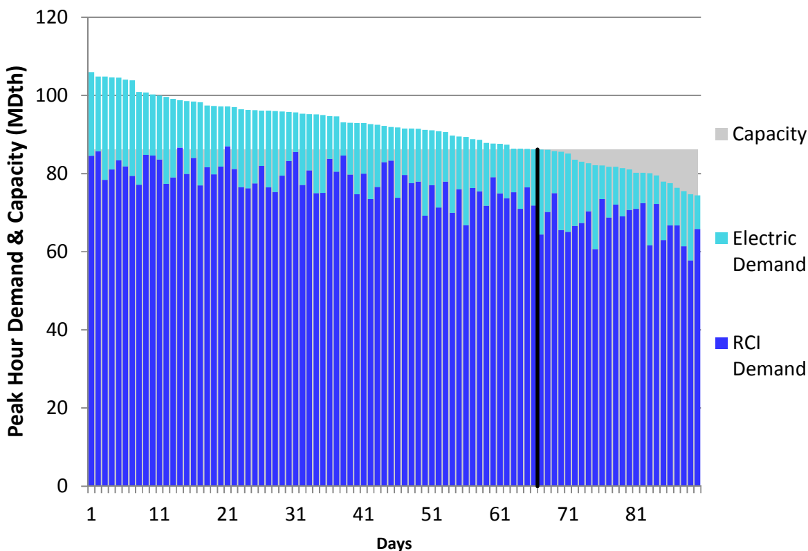
Figure N80. RGDS S18 Winter 2023 – Texas Eastern M2 PA South – Descending Demand
