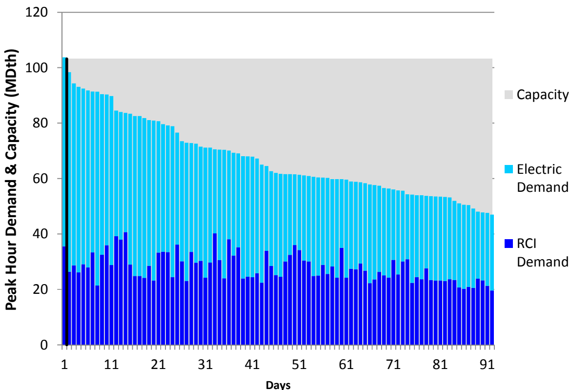
Figure N156. RGDS S19 Summer 2018 – Columbia Gas VA/MD – Descending Demand
