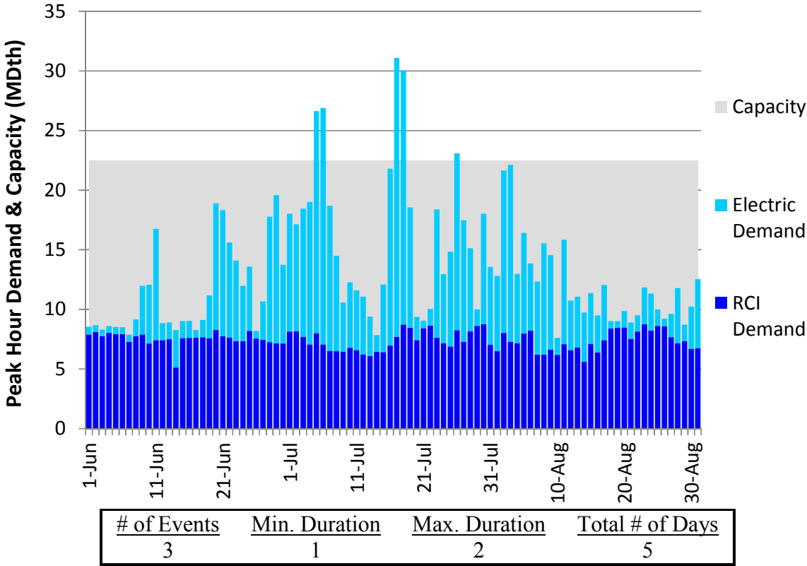
Figure N158. RGDS S19 Summer 2018 – Dominion Southeast – Descending Demand
