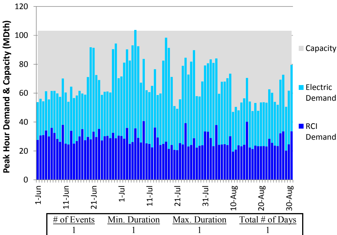
Figure N156. RGDS S19 Summer 2018 – Columbia Gas VA/MD – Descending Demand
