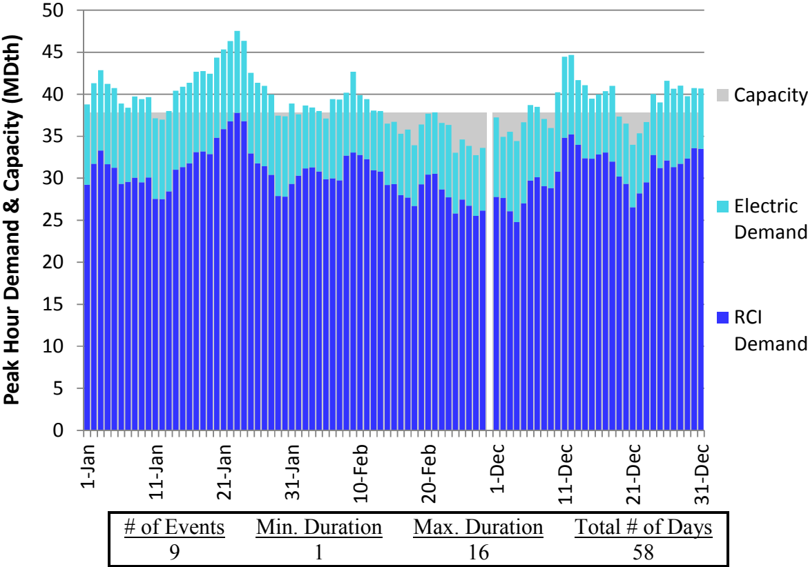
Figure N172. RGDS S19 Winter 2023 – Dominion Eastern NY– Descending Demand
