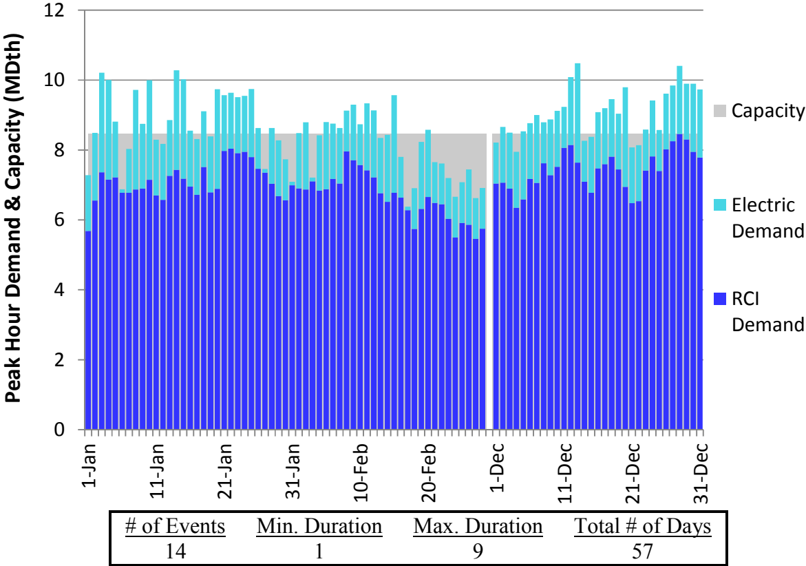
Figure N16. RGDS S18 Winter 2018 – Eastern Shore – Descending Demand
