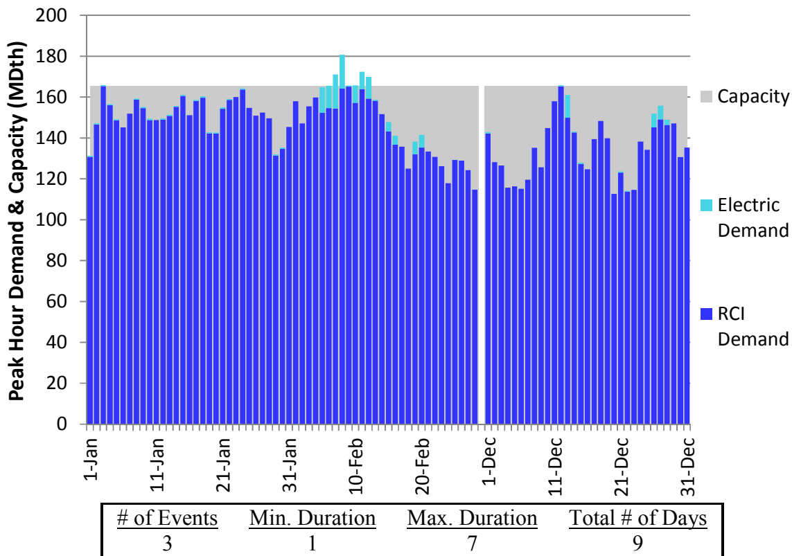
Figure N150. RGDS S19 Winter 2018 – Transco Z5 – Descending Demand
