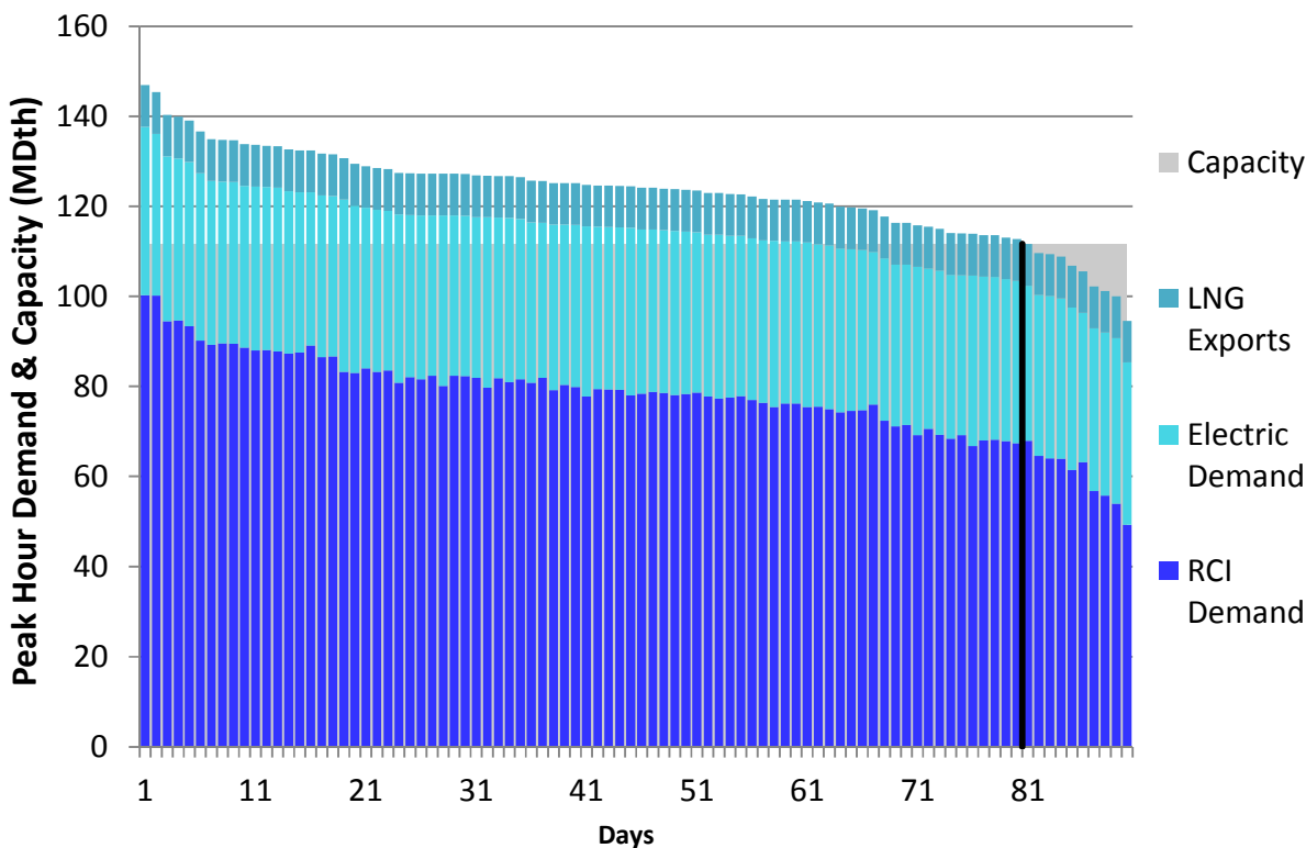
Figure N54. RGDS S18 Winter 2023 – Columbia Gas VA/MD – Descending Demand
