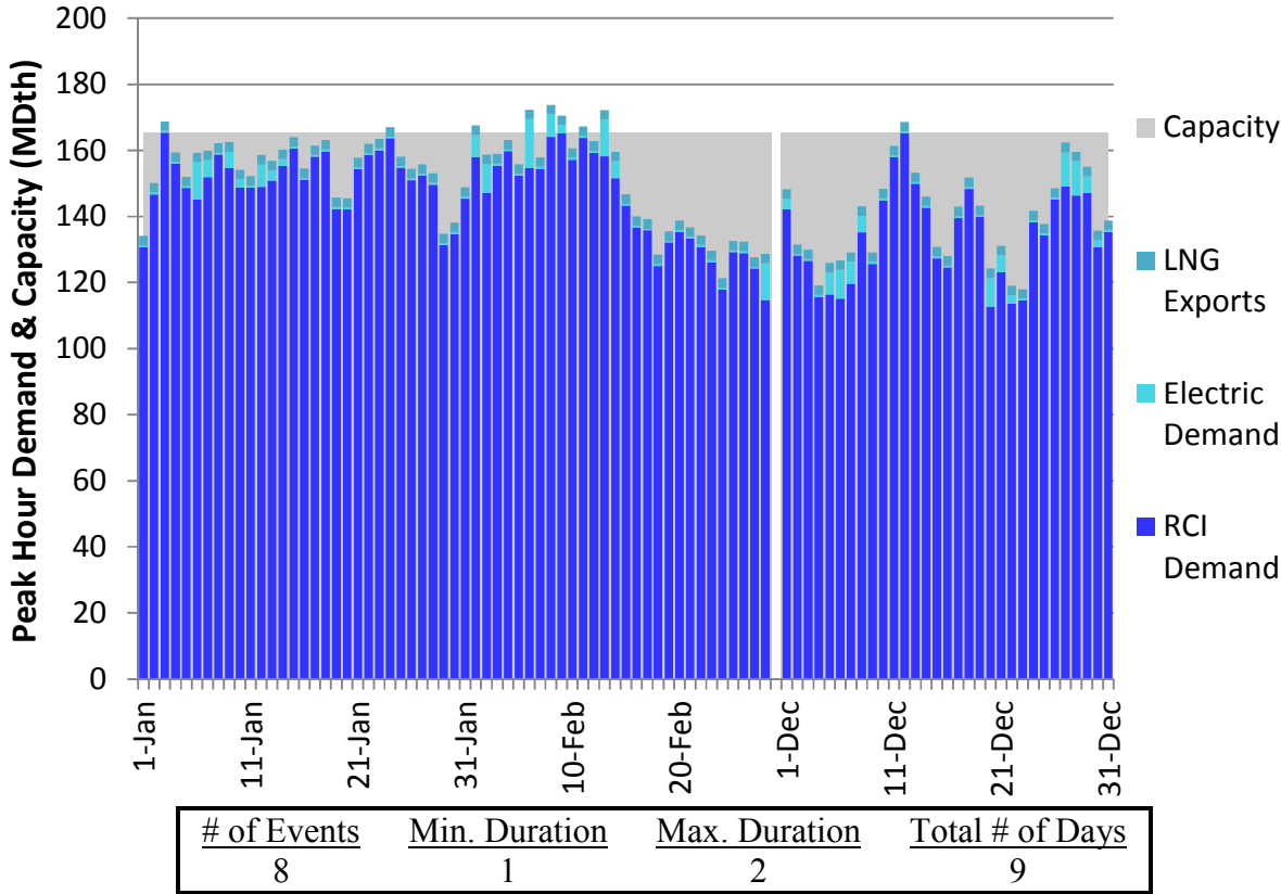
Figure N90. RGDS S18 Winter 2023 – Transco Z5 – Descending Demand
