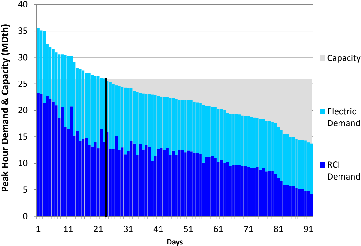
Figure N110. RGDS S18 Summer 2023 – Texas Eastern ETX – Descending Demand
