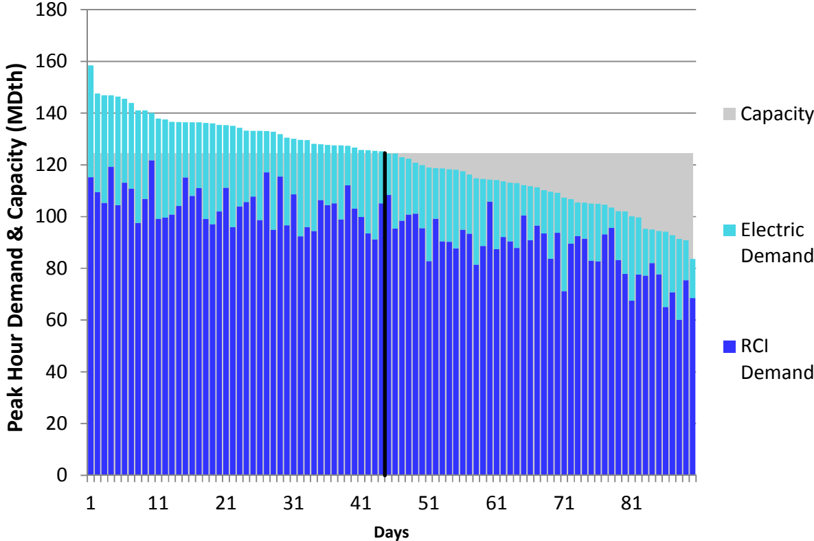
Figure N30. RGDS S18 Winter 2018 – Texas Eastern M3 North – Descending Demand
