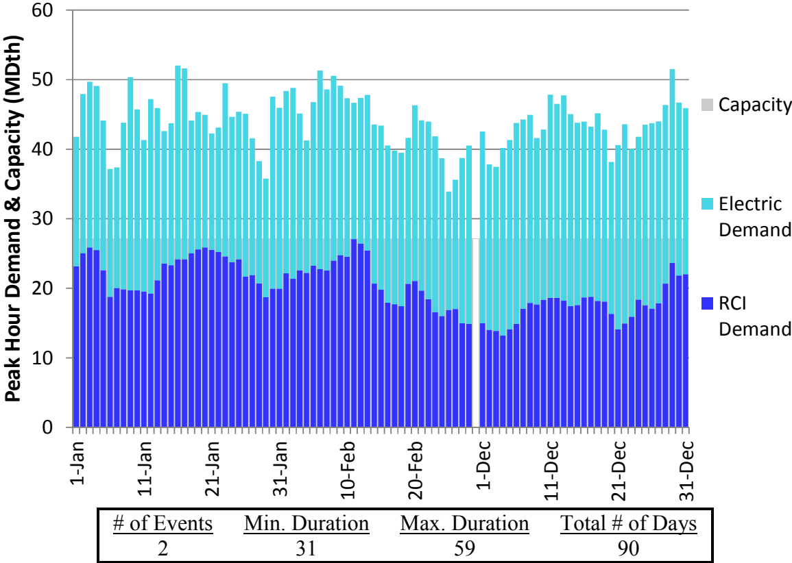
Figure N170. RGDS S19 Winter 2023 – Constitution – Descending Demand
