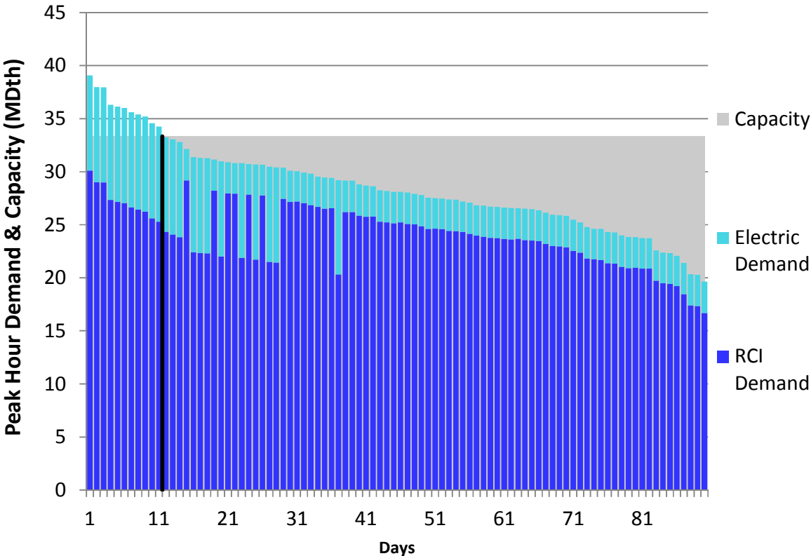
Figure N178. RGDS S19 Winter 2023 – East Tennessee – Descending Demand
