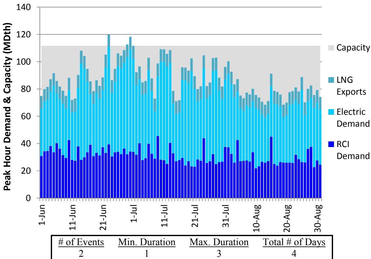
Figure N98. RGDS S18 Summer 2023 – Columbia Gas VA/MD – Descending Demand
