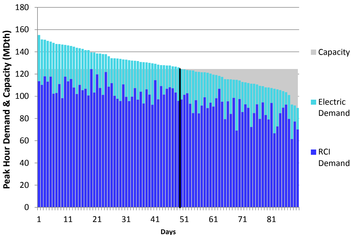
Figure N194. RGDS S19 Winter 2023 – Texas Eastern M3 North – Descending Demand
