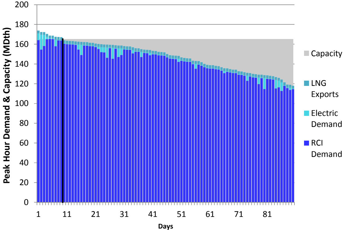
Figure N90. RGDS S18 Winter 2023 – Transco Z5 – Descending Demand
