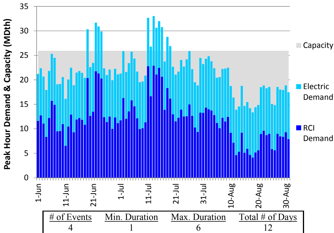
Figure N162. RGDS S19 Summer 2018 – Texas Eastern ETX – Descending Demand
