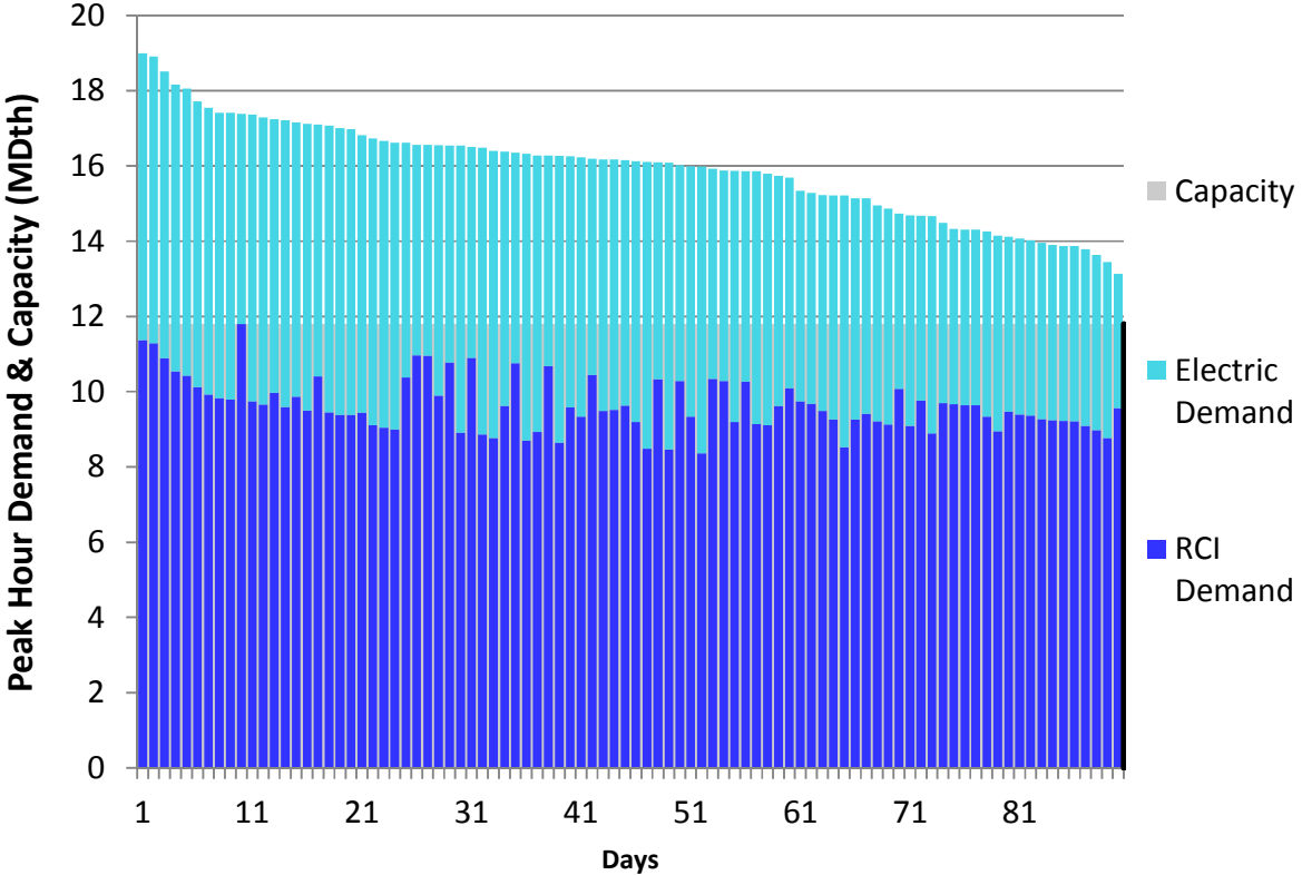
Figure N186. RGDS S19 Winter 2023 – NB/NS Supply – Descending Demand
