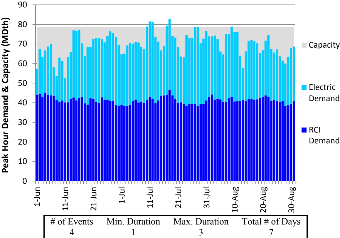
Figure N218. RGDS S19 Summer 2023 – Tennessee Z4 PA – Descending Demand
