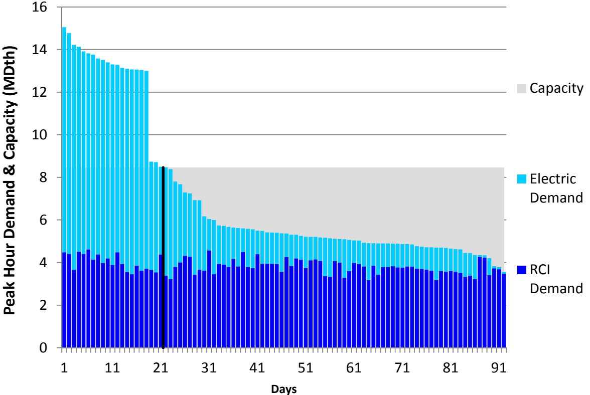
Figure N160. RGDS S19 Summer 2018 – Eastern Shore – Descending Demand
