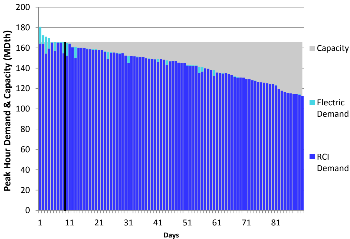
Figure N150. RGDS S19 Winter 2018 – Transco Z5 – Descending Demand
