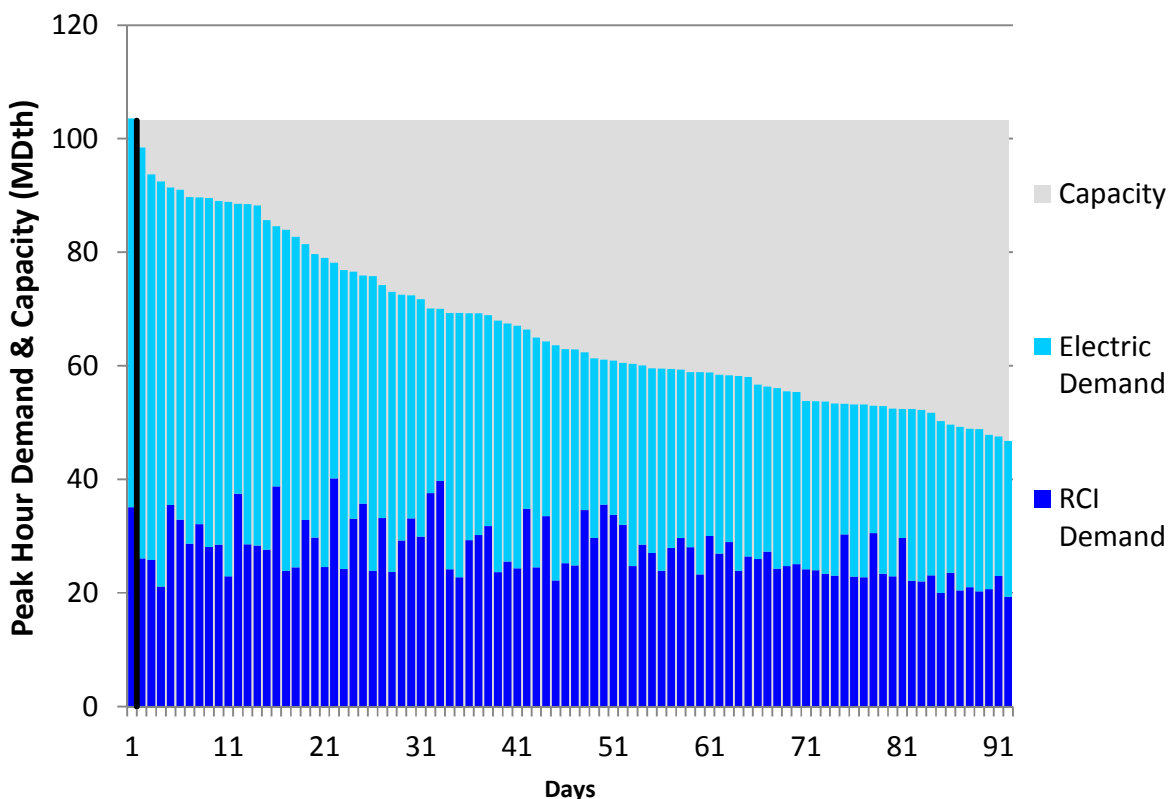
Figure N44. RGDS S18 Summer 2018 – Columbia Gas VA/MD – Descending Demand
