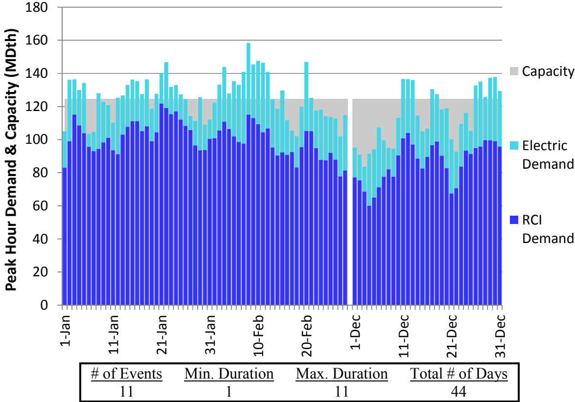
Figure N30. RGDS S18 Winter 2018 – Texas Eastern M3 North – Descending Demand
