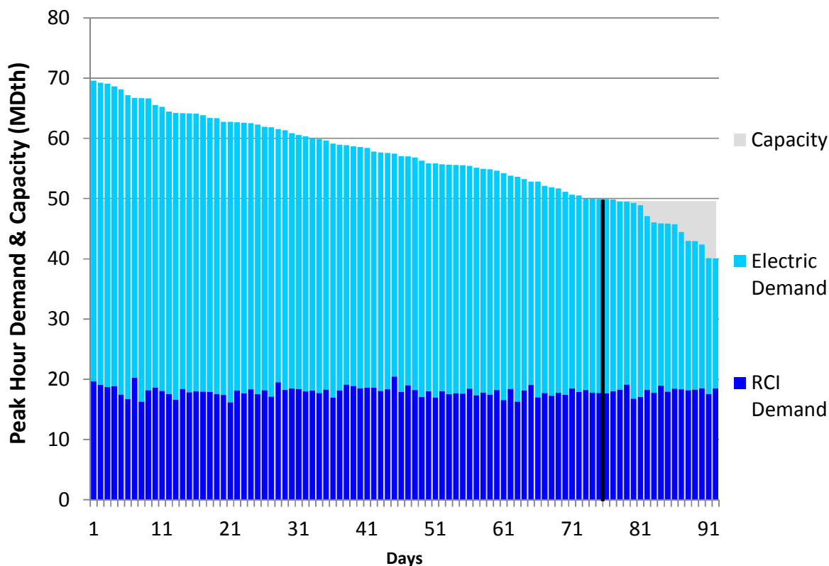
Figure N220. RGDS S19 Summer 2023 – Tennessee Z5 NY – Descending Demand
