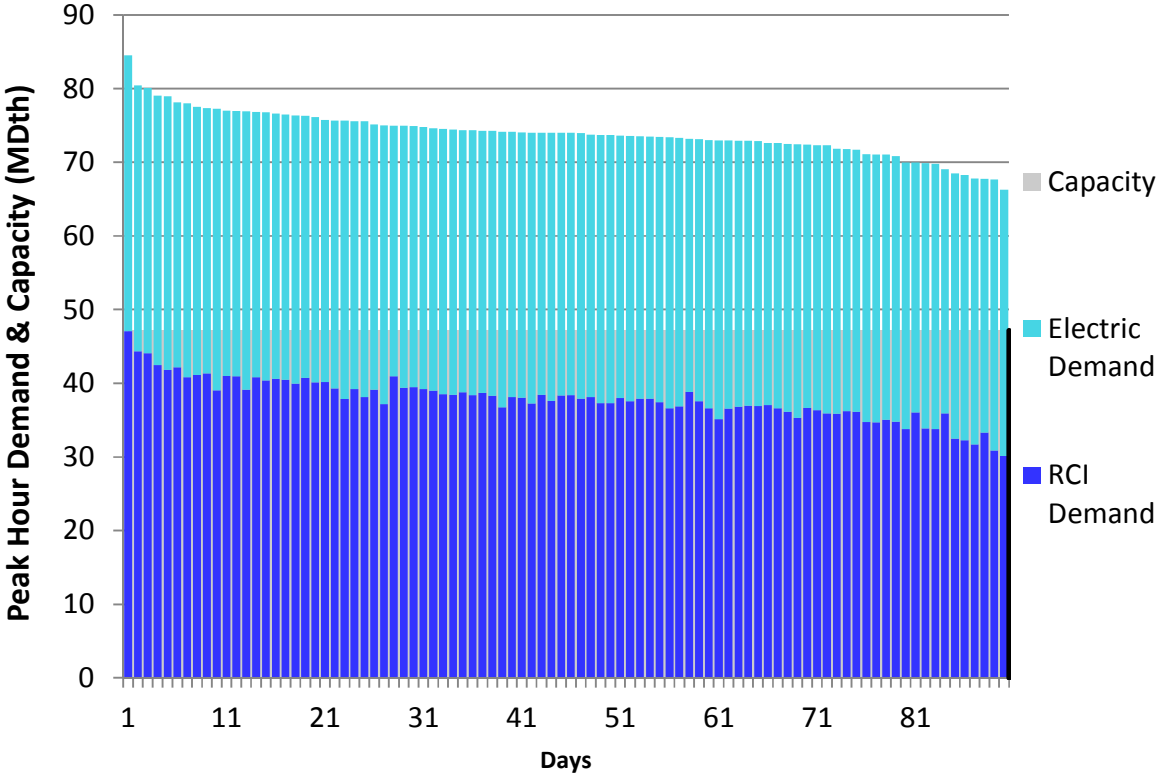
Figure N56. RGDS S18 Winter 2023 – Columbia Gas W PA/NY – Descending Demand
