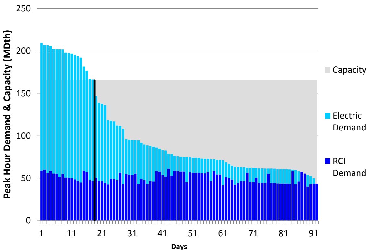
Figure N52. RGDS S18 Summer 2018 – Transco Z5 – Descending Demand
