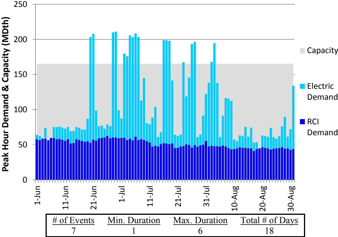
Figure N164. RGDS S19 Summer 2018 – Transco Z5 – Descending Demand
