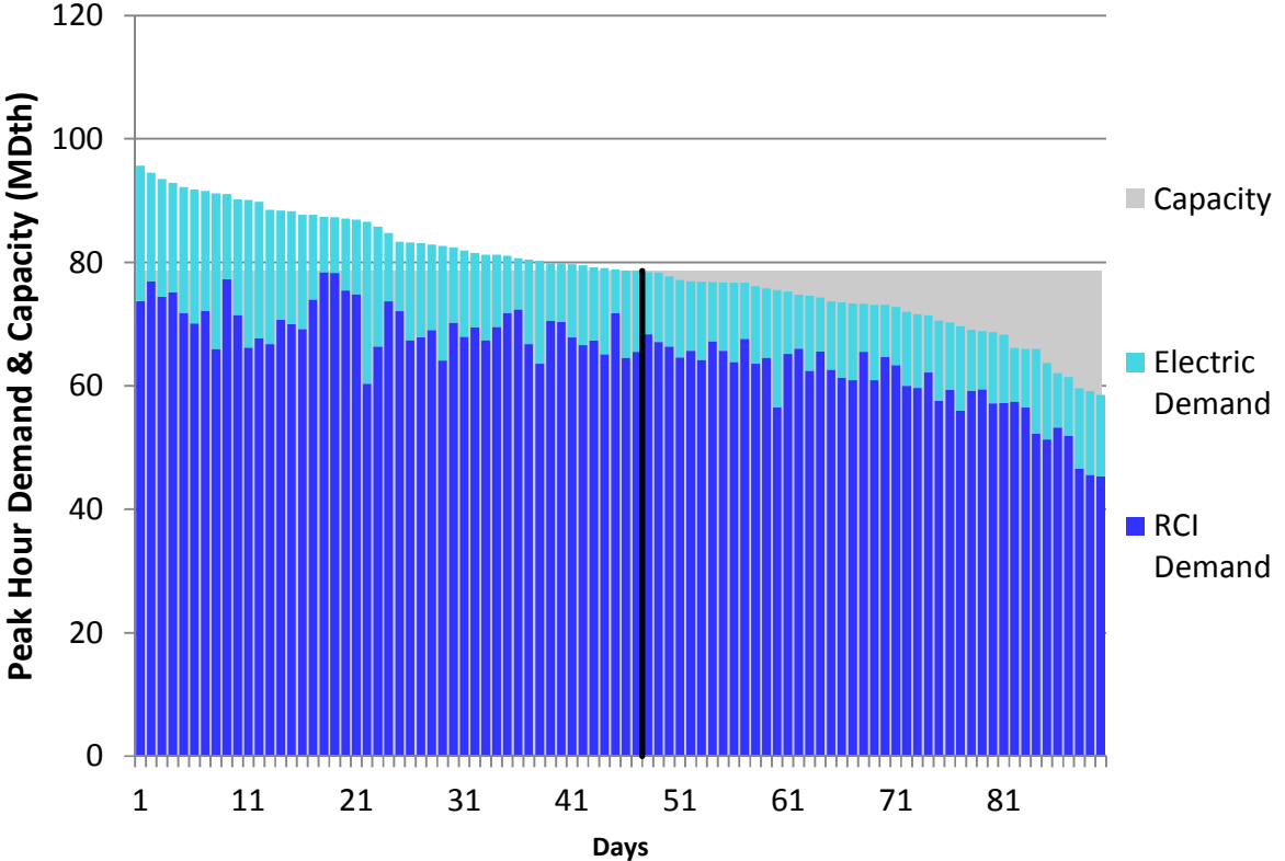
Figure N76. RGDS S18 Winter 2023 – Tennessee Z4 PA – Descending Demand
