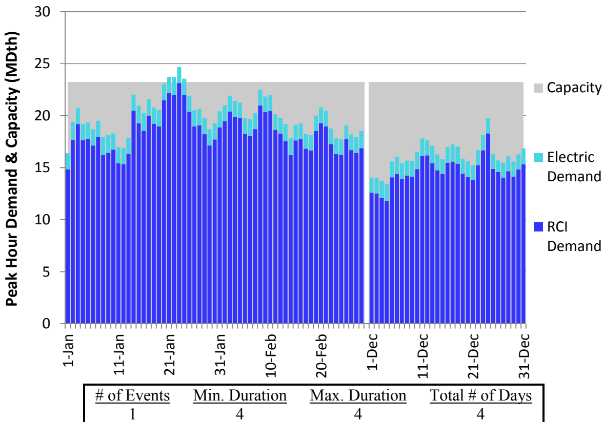
Figure N10. RGDS S18 Winter 2018 – Dominion Western NY– Descending Demand
