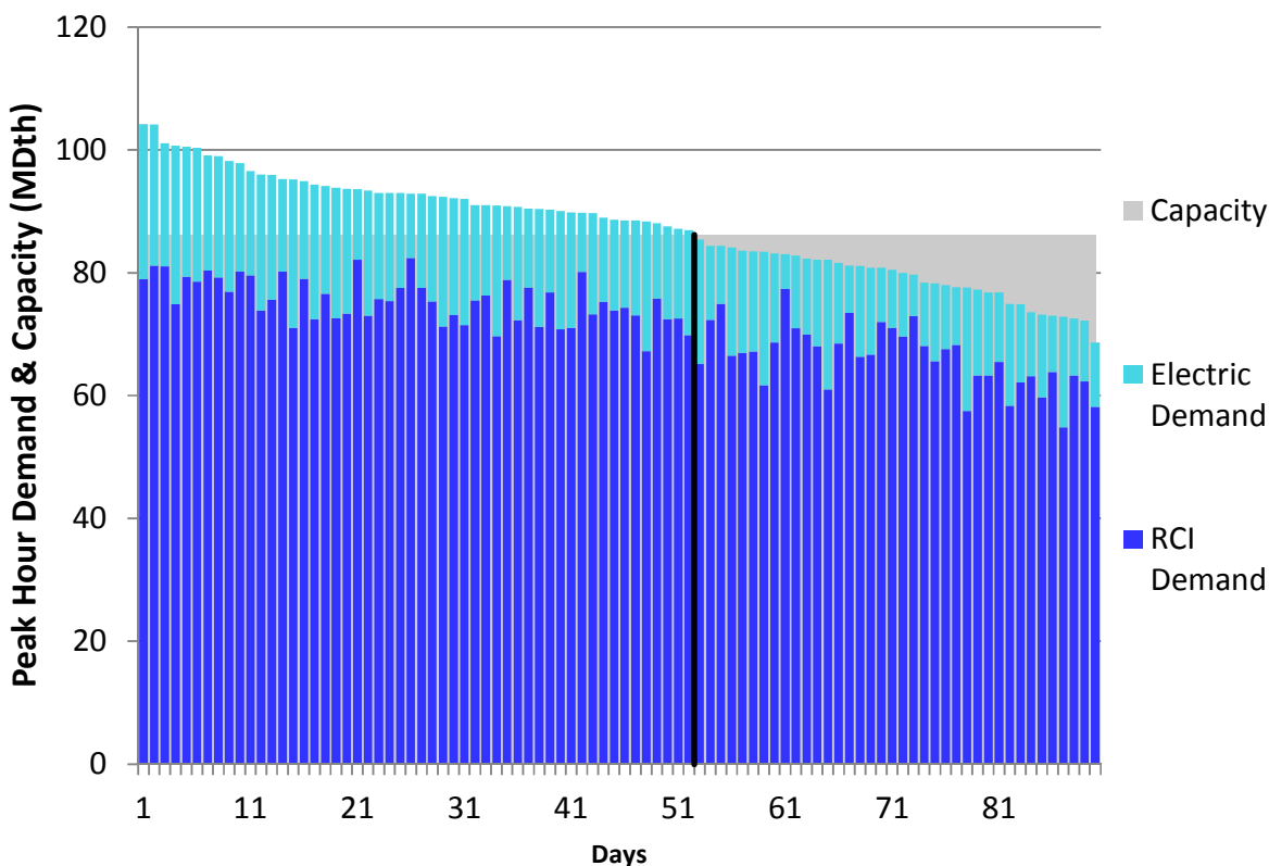
Figure N28. RGDS S18 Winter 2018 – Texas Eastern M2 PA South – Descending Demand
