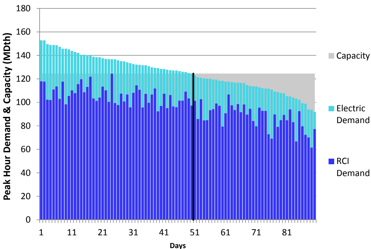
Figure N82. RGDS S18 Winter 2023 – Texas Eastern M3 North – Descending Demand
