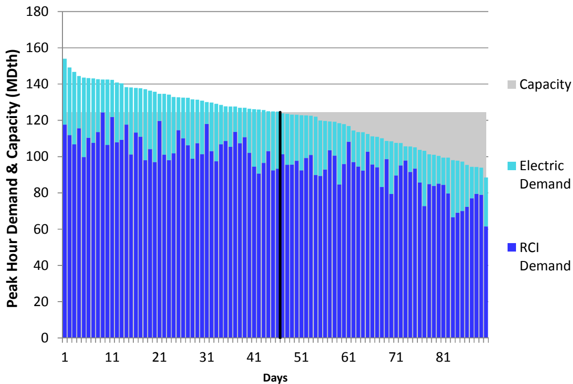
Figure N142. RGDS S19 Winter 2018 – Texas Eastern M3 North – Descending Demand
