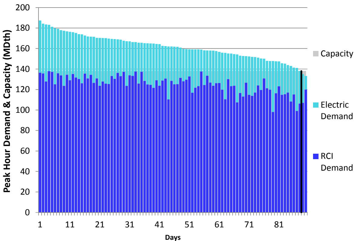
Figure N92. RGDS S18 Winter 2023 – Transco Leidy to Station 210 – Descending Demand
