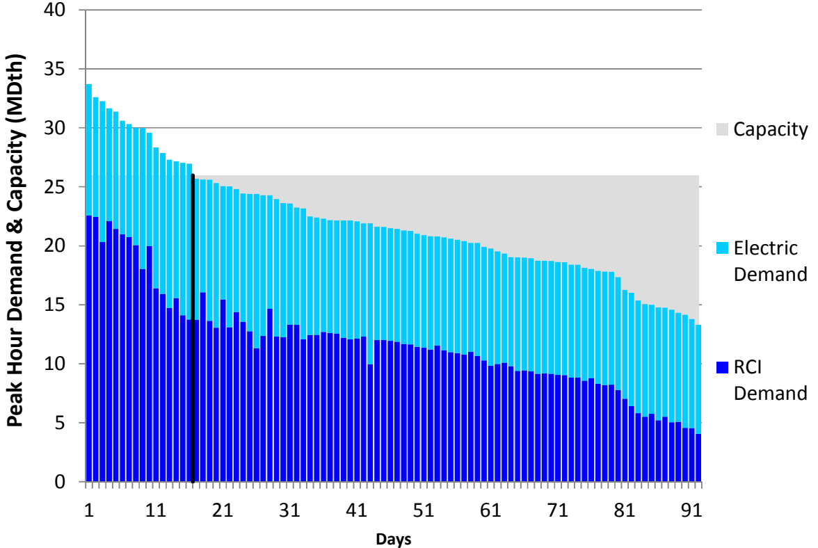
Figure N50. RGDS S18 Summer 2018 – Texas Eastern ETX – Descending Demand
