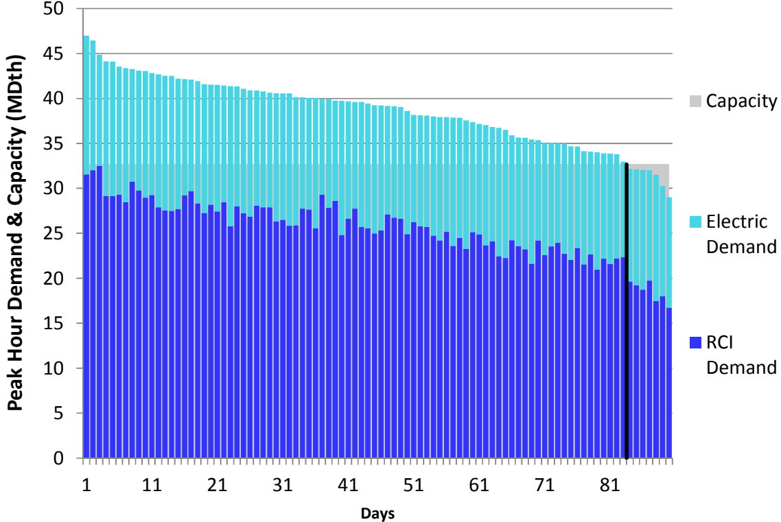
Figure N132. RGDS S19 Winter 2018 – Millennium – Descending Demand
