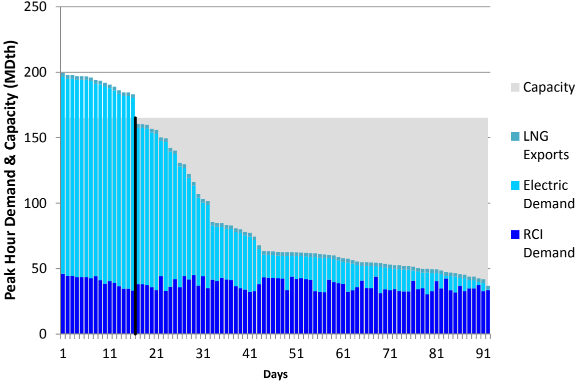
Figure L84. RGDS S13 Summer 2023 – Transco Z5 – Descending Demand
