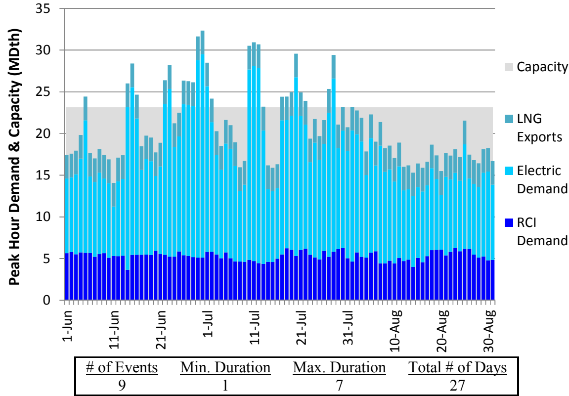
Figure L184. RGDS S14 Summer 2023 – Dominion Southeast – Descending Demand
