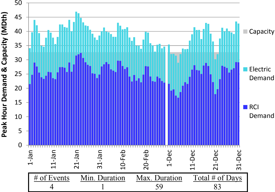
Figure L104. RGDS S14 Winter 2018 – Millennium – Descending Demand
