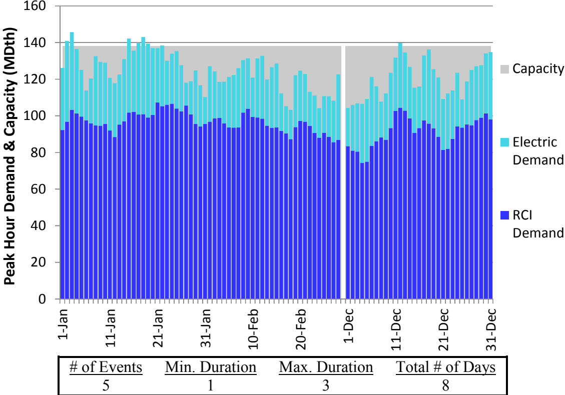
Figure L32. RGDS S13 Winter 2018 – Transco Leidy to Station 210 – Descending Demand
