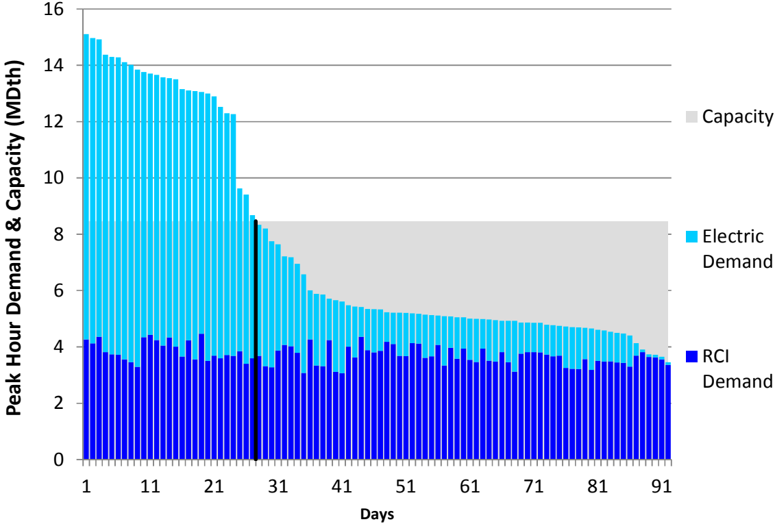
Figure L290. RGDS S16 Summer 2023 – Eastern Shore – Descending Demand
