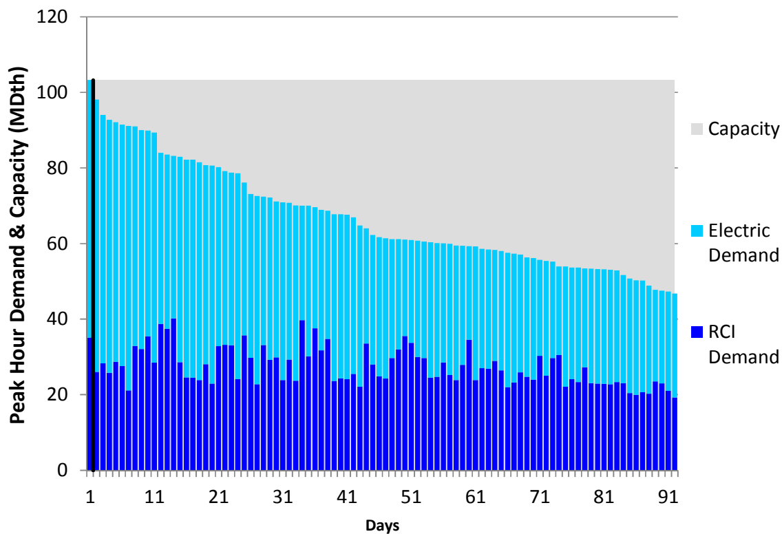
Figure L128. RGDS S14 Summer 2018 – Columbia Gas VA/MD – Descending Demand
