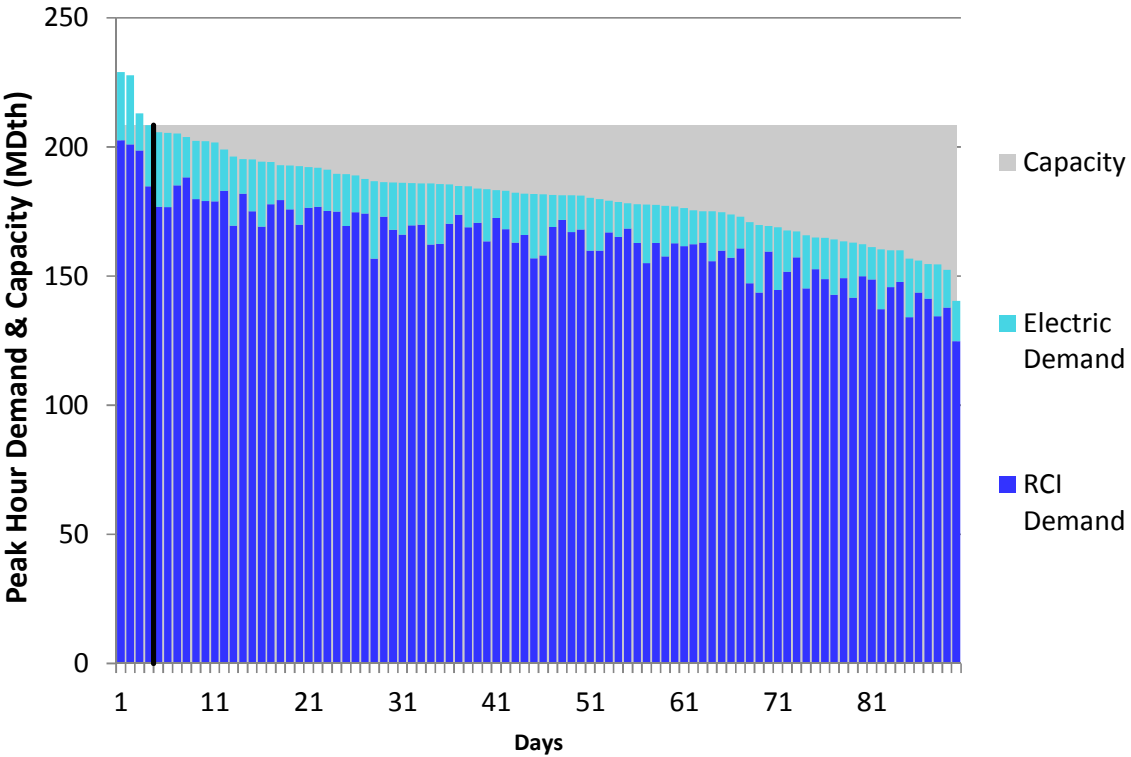
Figure L284. RGDS S16 Winter 2023 – Union Gas Dawn – Descending Demand
