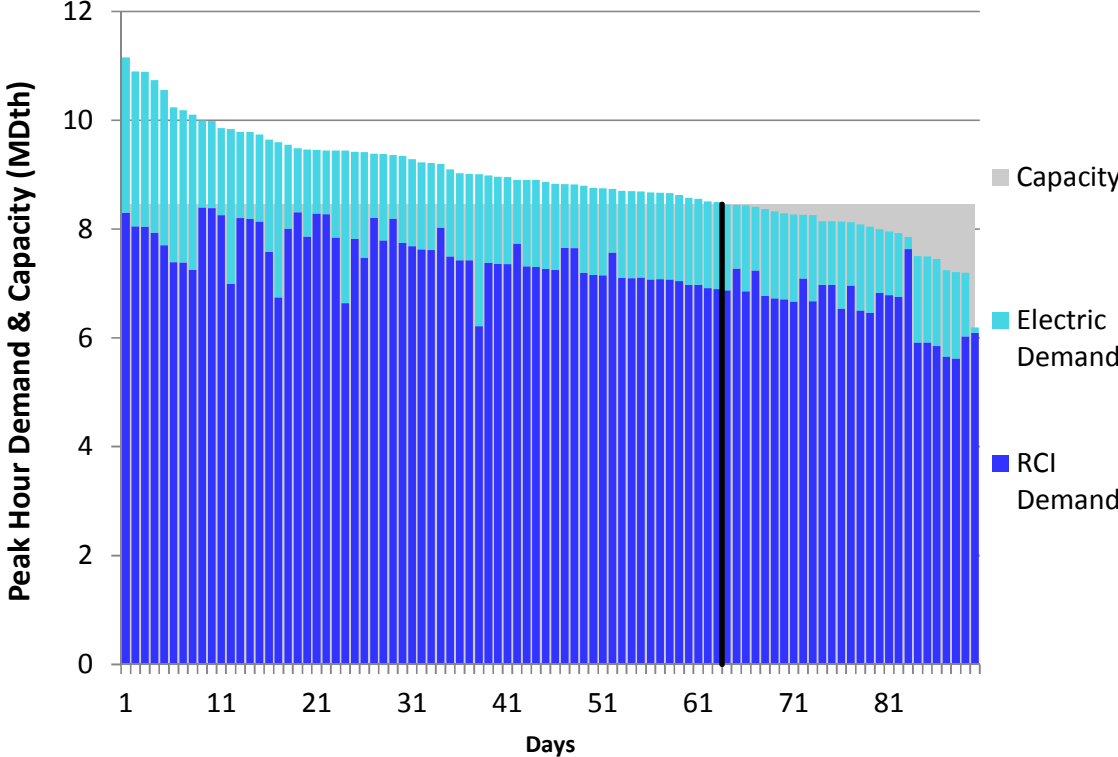
Figure L152. RGDS S14 Winter 2023 – Eastern Shore – Descending Demand
