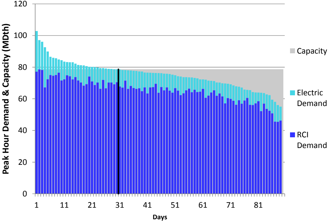
Figure L108. RGDS S14 Winter 2018 – Tennessee Z4 PA – Descending Demand
