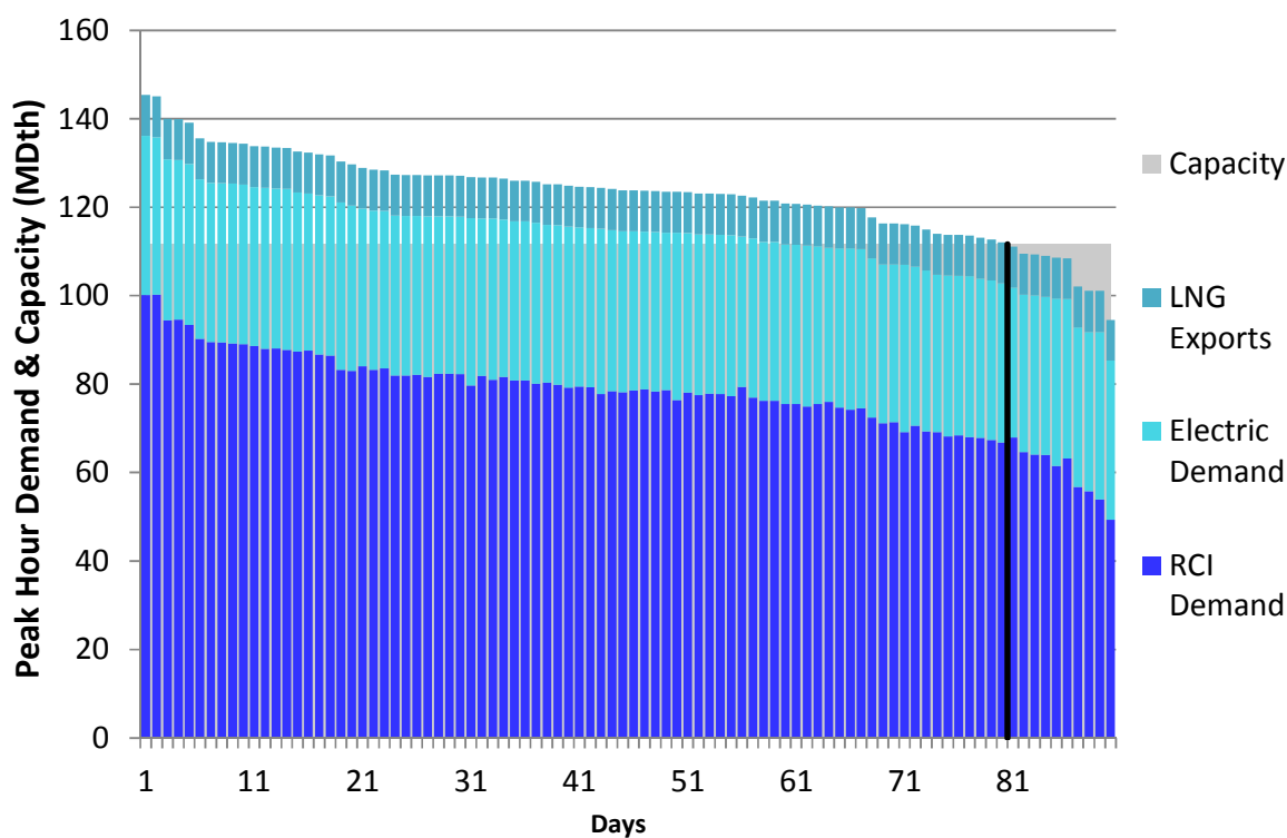
Figure L246. RGDS S16 Winter 2023 – Columbia Gas VA/MD – Descending Demand
