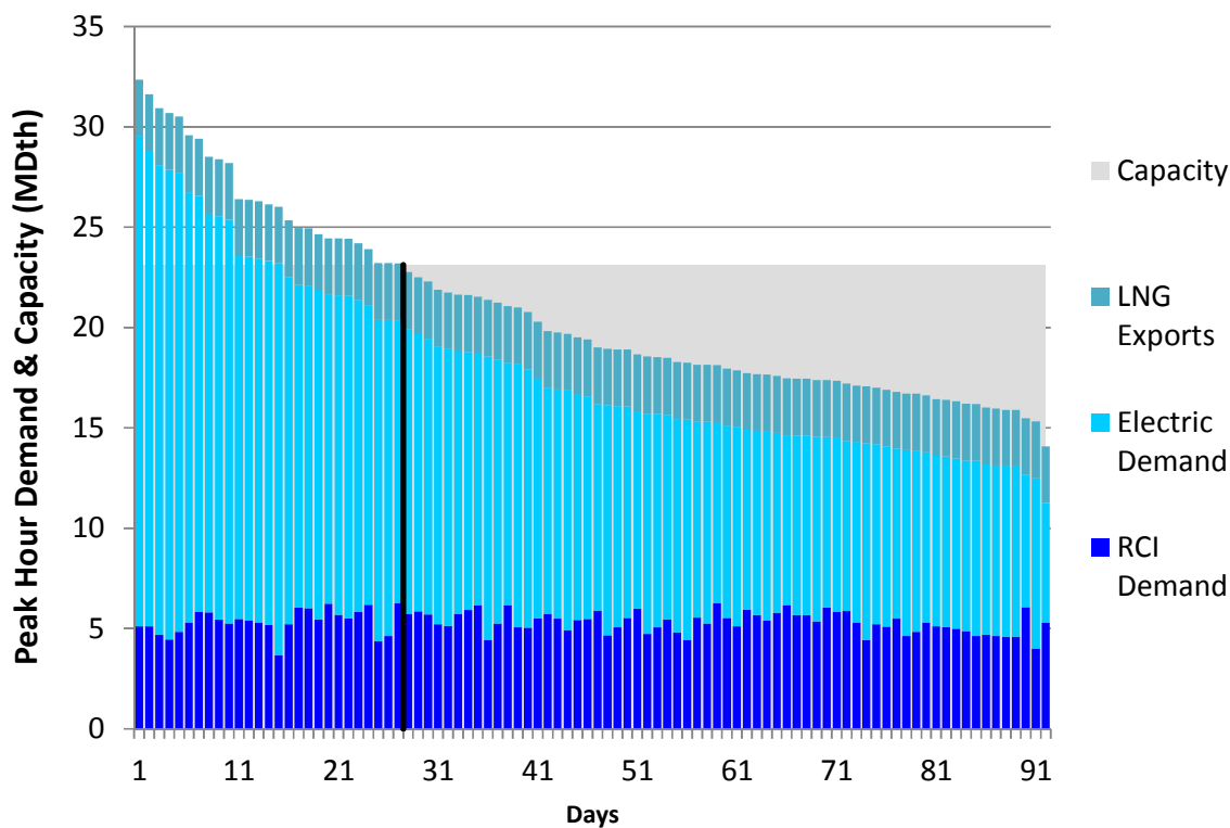
Figure L288. RGDS S16 Summer 2023 – Dominion Southeast – Descending Demand
