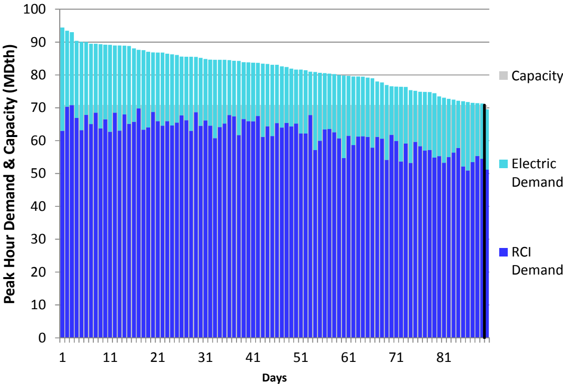
Figure L172. RGDS S14 Winter 2023 – Transco Leidy Atlantic – Descending Demand
