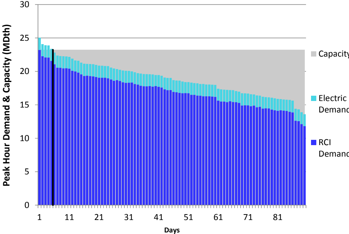
Figure L254. RGDS S16 Winter 2023 – Dominion Western NY– Descending Demand
