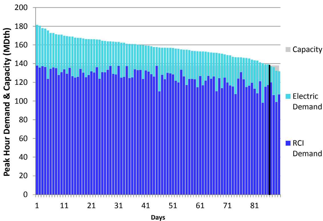
Figure L176. RGDS S14 Winter 2023 – Transco Leidy to Station 210 – Descending Demand
