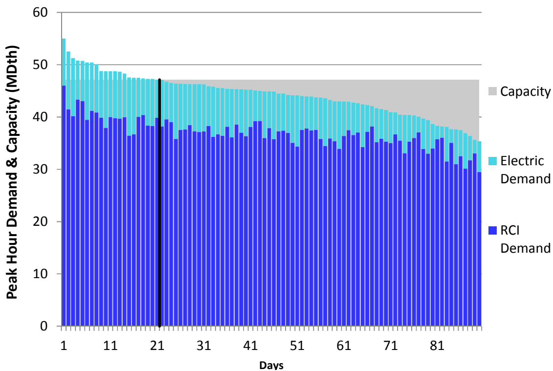
Figure L88. RGDS S14 Winter 2018 – Columbia Gas W PA/NY – Descending Demand
