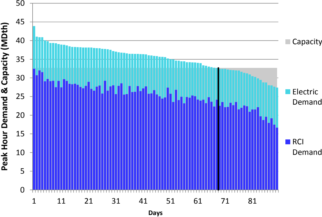
Figure L56. RGDS S13 Winter 2023 – Millennium – Descending Demand
