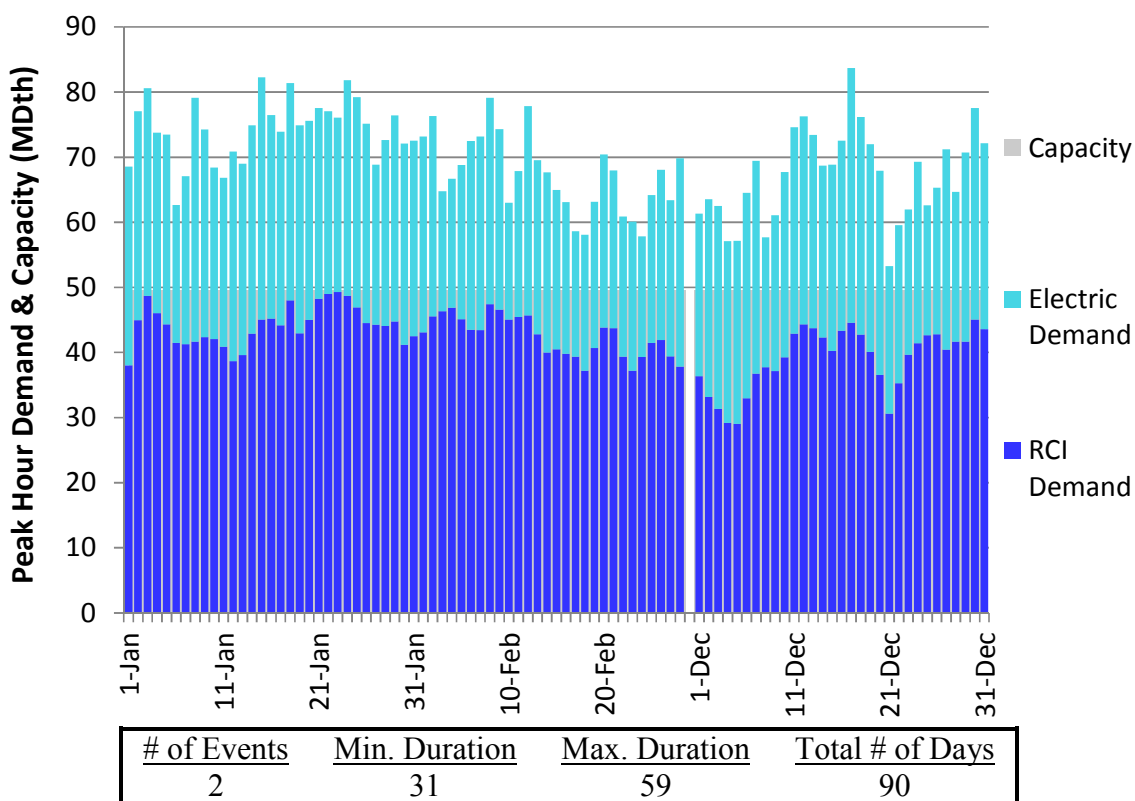
Figure L21. RGDS S13 Winter 2018 – Tennessee Z5 NY – Chronological Demand
