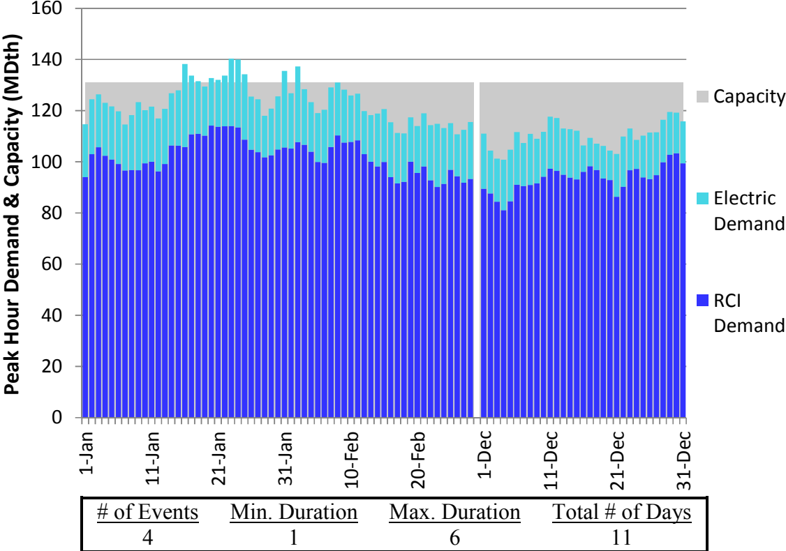
Figure L274. RGDS S16 Winter 2023 – TransCanada Ontario West – Descending Demand
