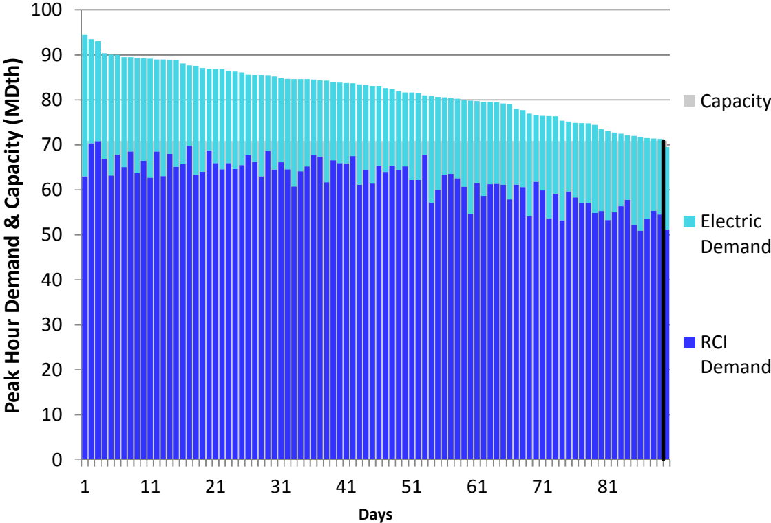
Figure L68. RGDS S13 Winter 2023 – Transco Leidy Atlantic – Descending Demand
