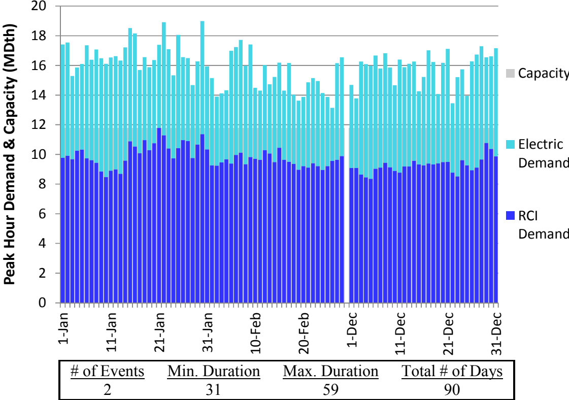
Figure L58. RGDS S13 Winter 2023 – NB/NS Supply – Descending Demand
