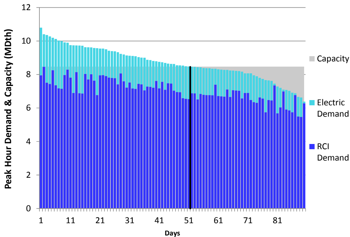
Figure L210. RGDS S16 Winter 2018 – Eastern Shore – Descending Demand
