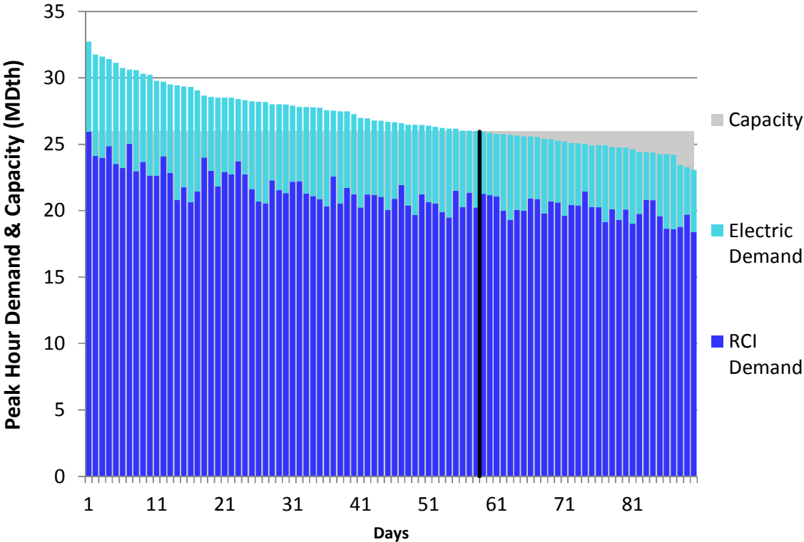
Figure L16. RGDS S13 Winter 2018 – NB/NS Supply – Descending Demand
