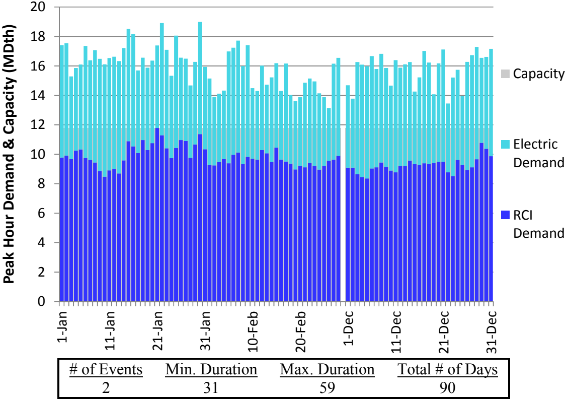
Figure L158. RGDS S14 Winter 2023 – NB/NS – Descending Demand
