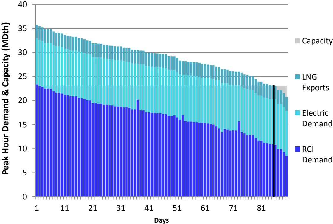
Figure L256. RGDS S16 Winter 2023 – Dominion Southeast – Descending Demand
