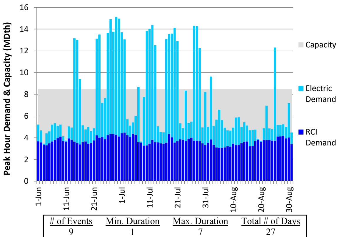
Figure L186. RGDS S14 Summer 2023 – Eastern Shore – Descending Demand
