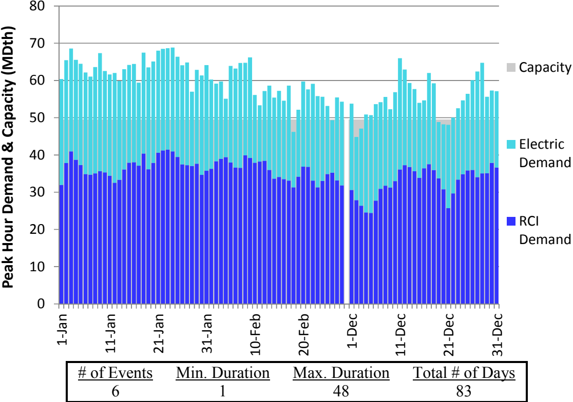
Figure L268. RGDS S16 Winter 2023 – Tennessee Z5 NY – Descending Demand
