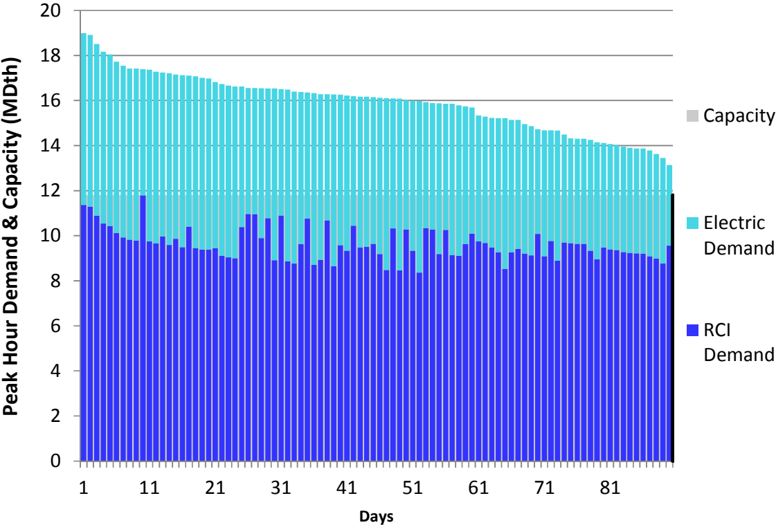
Figure L58. RGDS S13 Winter 2023 – NB/NS Supply – Descending Demand
