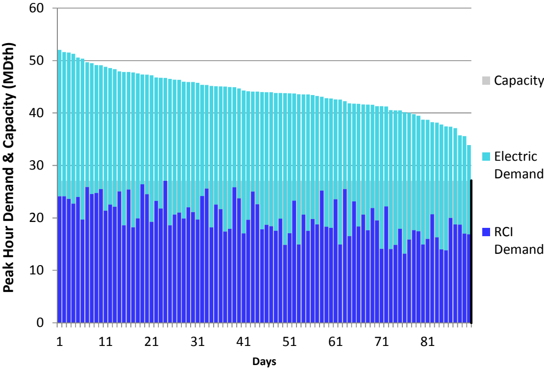
Figure L250. RGDS S16 Winter 2023 – Constitution – Descending Demand
