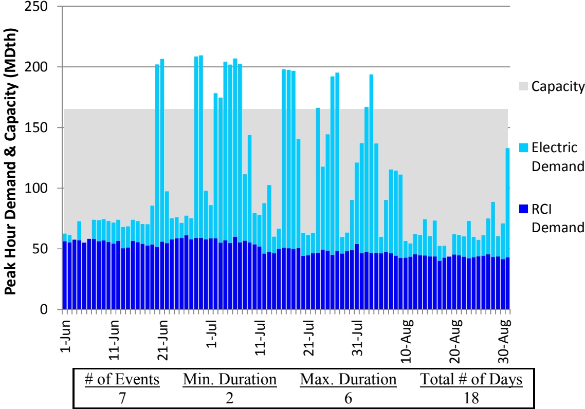
Figure L244. RGDS S16 Summer 2018 – Transco Z5 – Descending Demand
