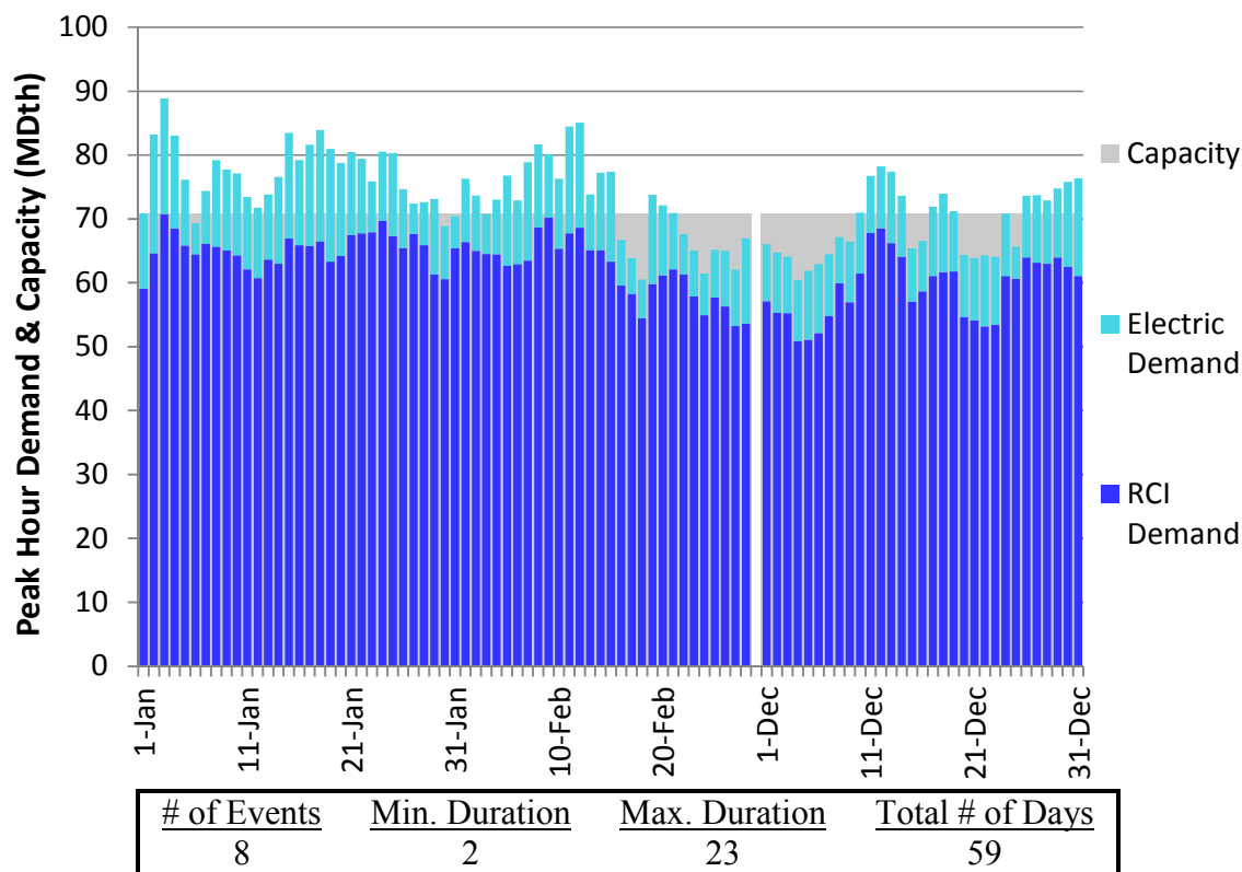
Figure L228. RGDS S16 Winter 2018 – Transco Leidy Atlantic – Descending Demand
