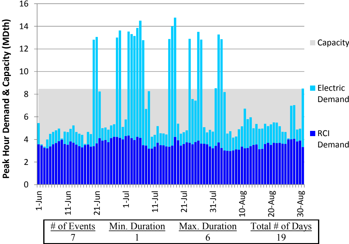
Figure L38. RGDS S13 Summer 2018 – Eastern Shore – Descending Demand
