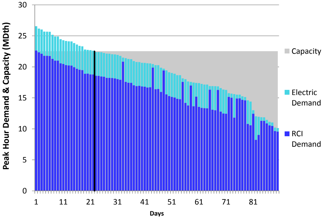
Figure L6. RGDS S13 Winter 2018 – Dominion Southeast – Descending Demand
