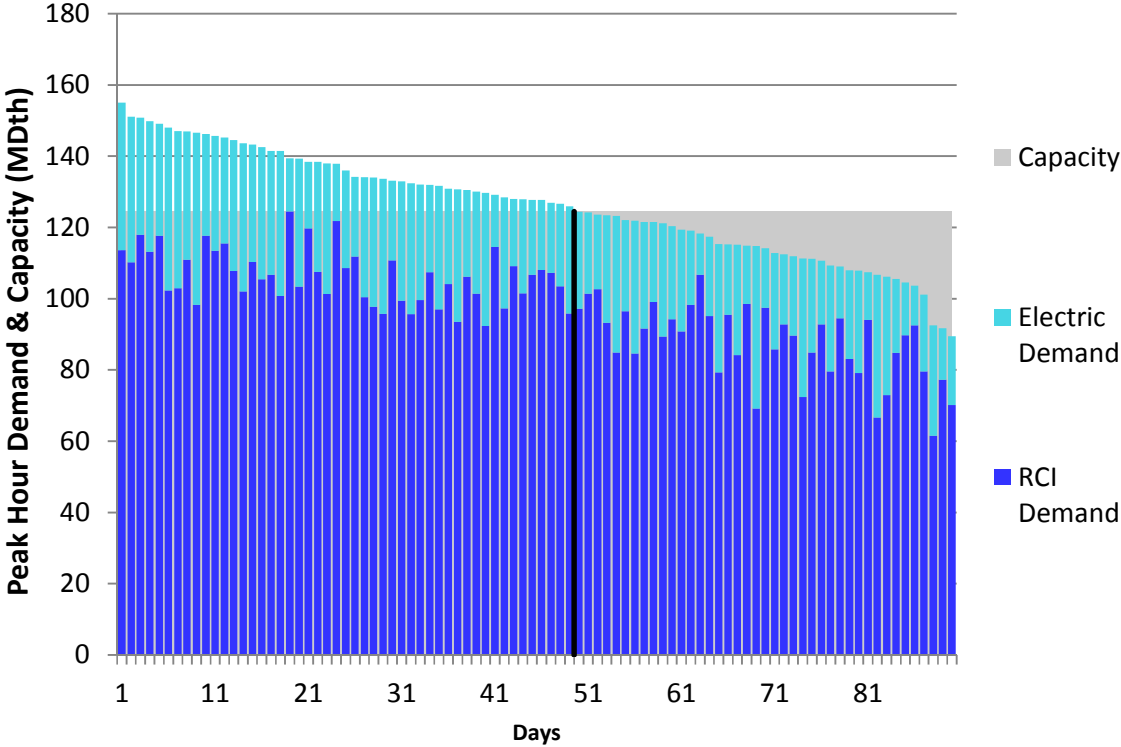
Figure L64. RGDS S13 Winter 2023 – Texas Eastern M3 North – Descending Demand
