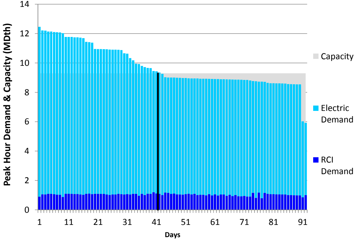
Figure L190. RGDS S14 Summer 2023 – PNGTS N of Westbrook – Descending Demand
