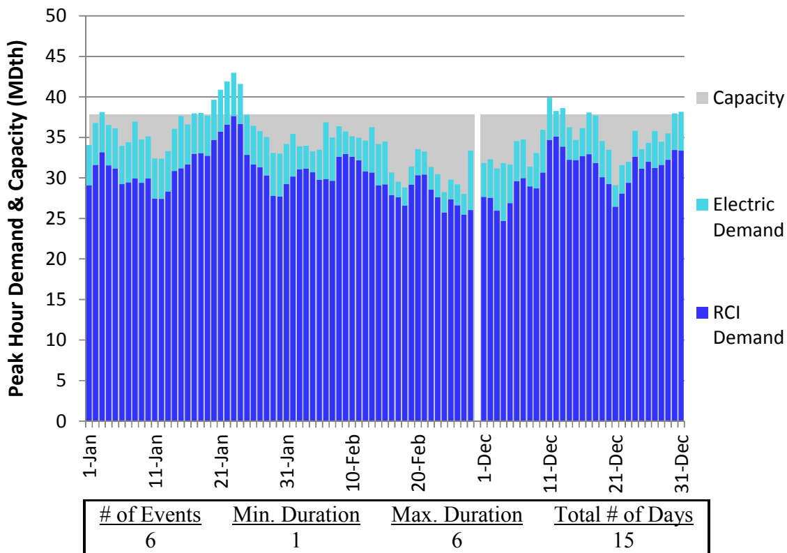
Figure L92. RGDS S14 Winter 2018 – Dominion Eastern NY– Descending Demand
