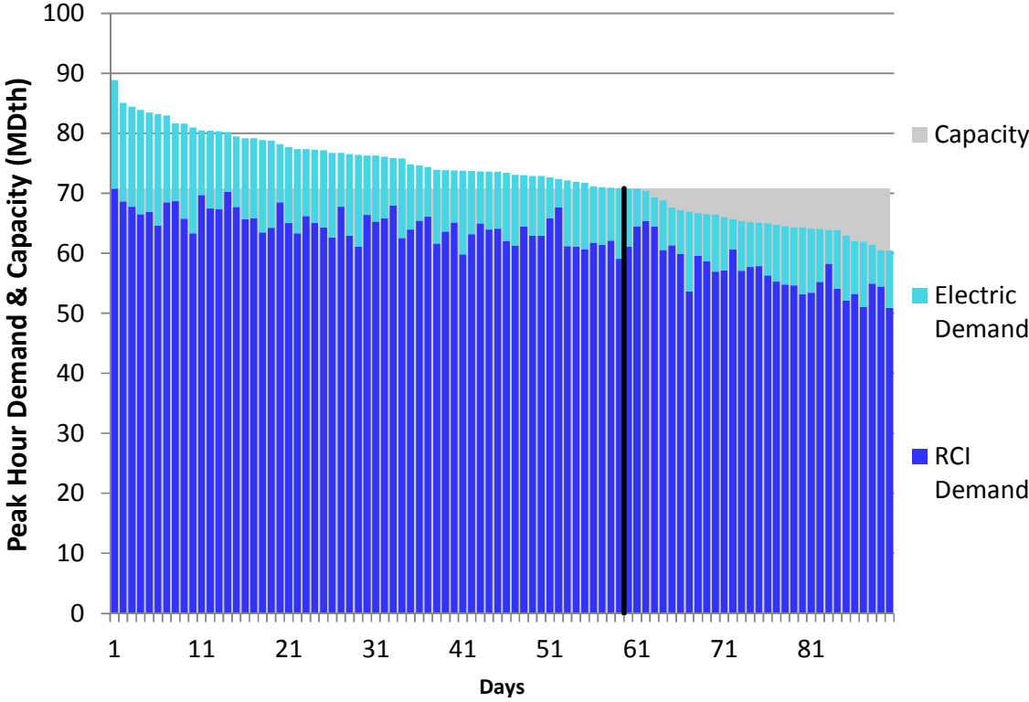
Figure L28. RGDS S13 Winter 2018 – Transco Leidy Atlantic – Descending Demand
