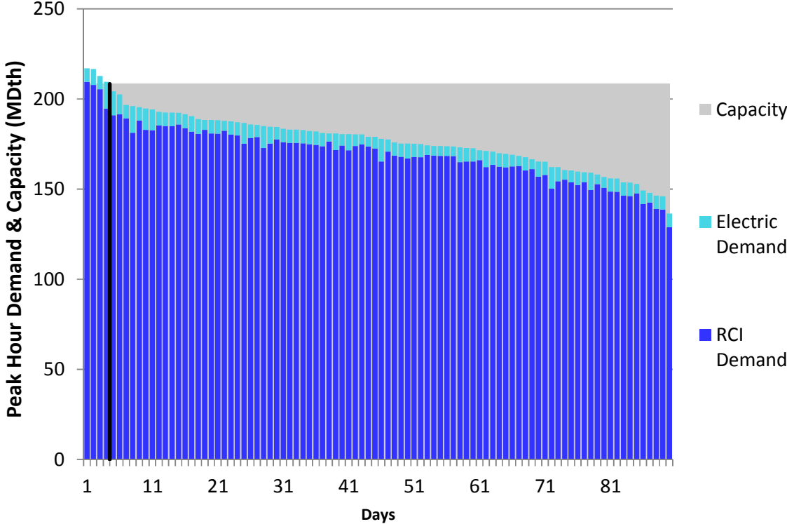
Figure L234. RGDS S16 Winter 2018 – Union Gas Dawn – Descending Demand
