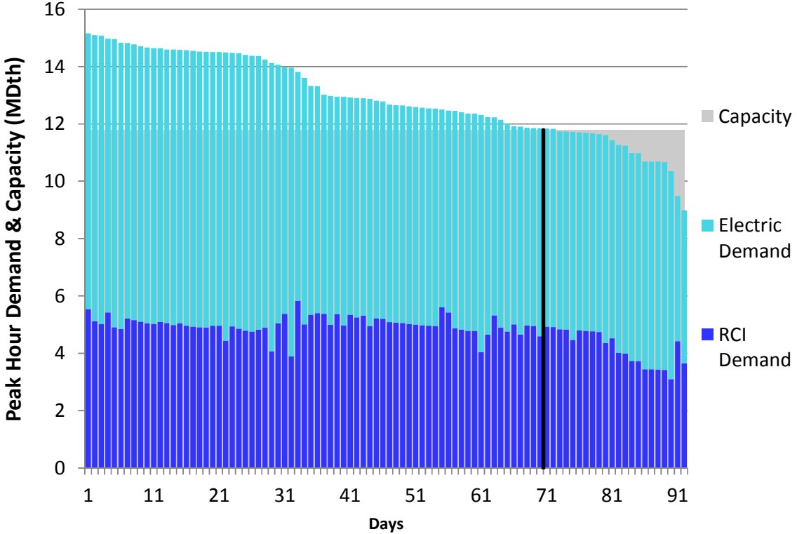
Figure L188. RGDS S14 Summer 2023 – NB/NS – Descending Demand
