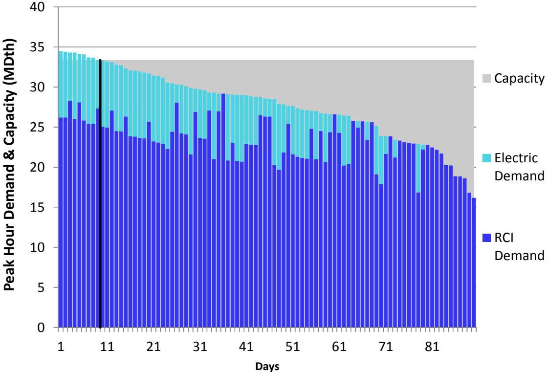
Figure L98. RGDS S14 Winter 2018 – East Tennessee – Descending Demand
