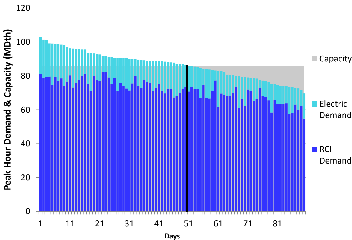
Figure L112. RGDS S14 Winter 2018 – Texas Eastern M2 PA South – Descending Demand
