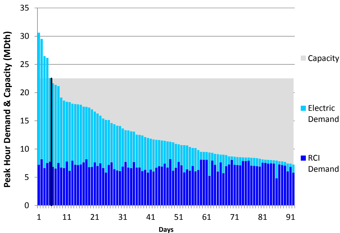
Figure L36. RGDS S13 Summer 2018 – Dominion Southeast – Descending Demand
