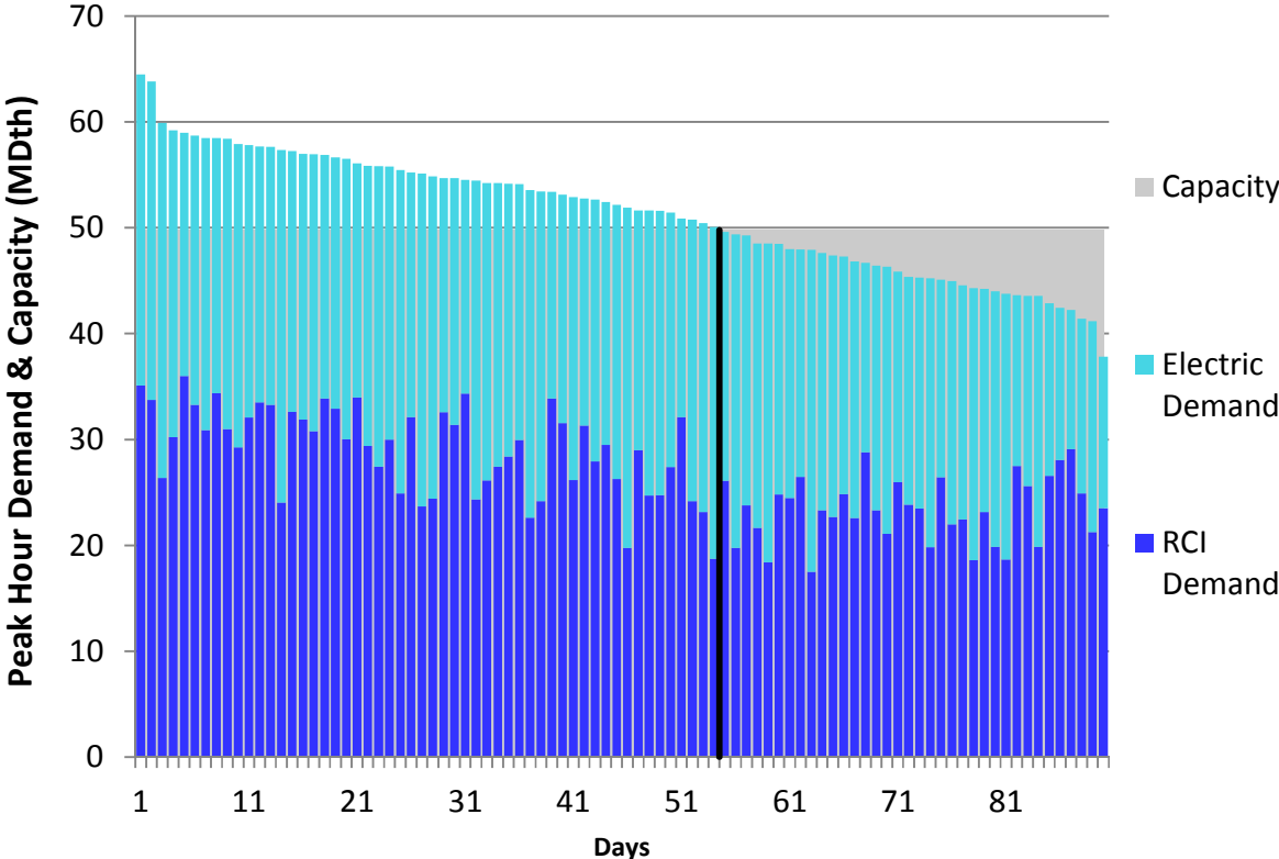
Figure L12. RGDS S13 Winter 2018 – Iroquois Zone 1 – Descending Demand
