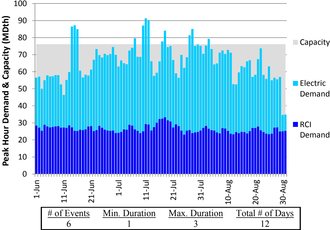
Figure L180. RGDS S14 Summer 2023 – Algonquin CT – Descending Demand
