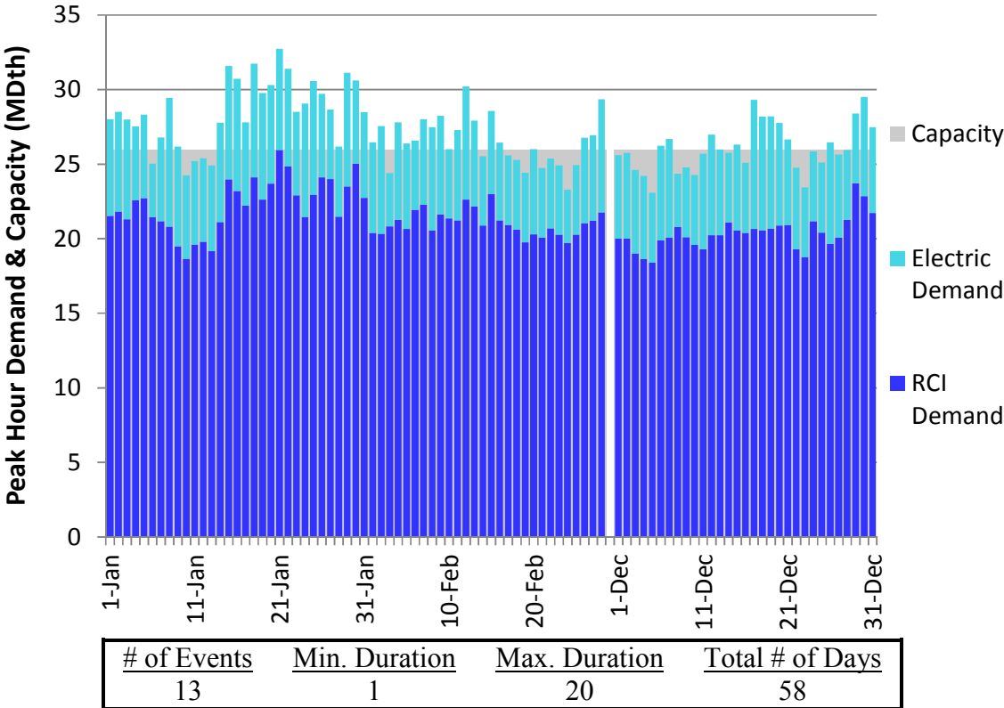
Figure L16. RGDS S13 Winter 2018 – NB/NS Supply – Descending Demand
