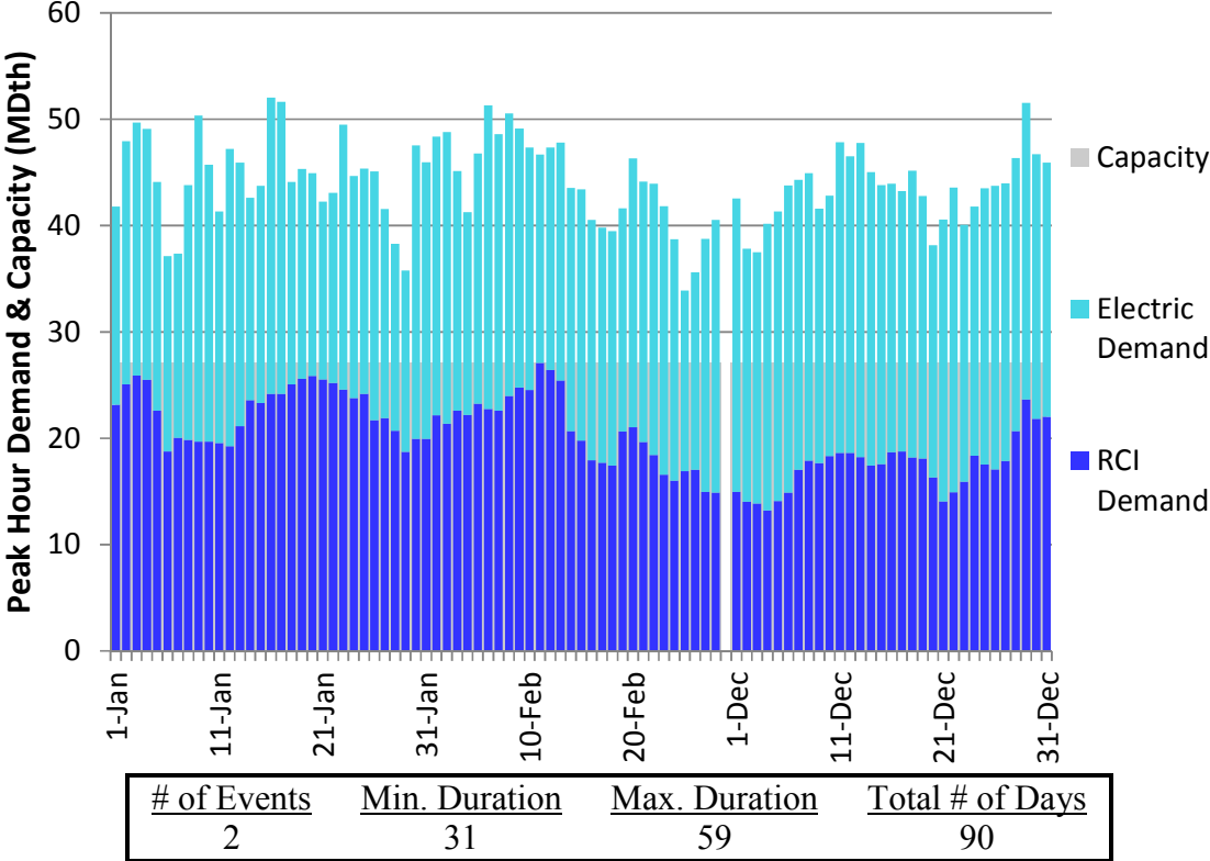
Figure L142. RGDS S14 Winter 2023 – Constitution – Descending Demand
