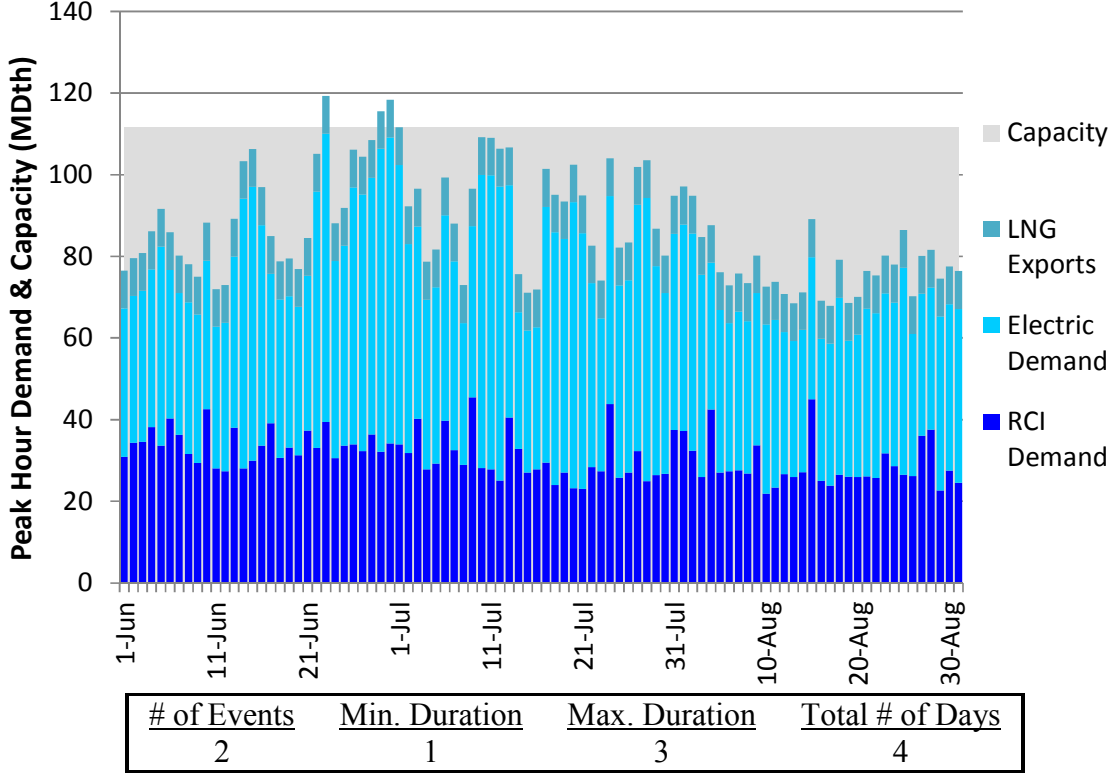
Figure L182. RGDS S14 Summer 2023 – Columbia Gas VA/MD – Descending Demand
