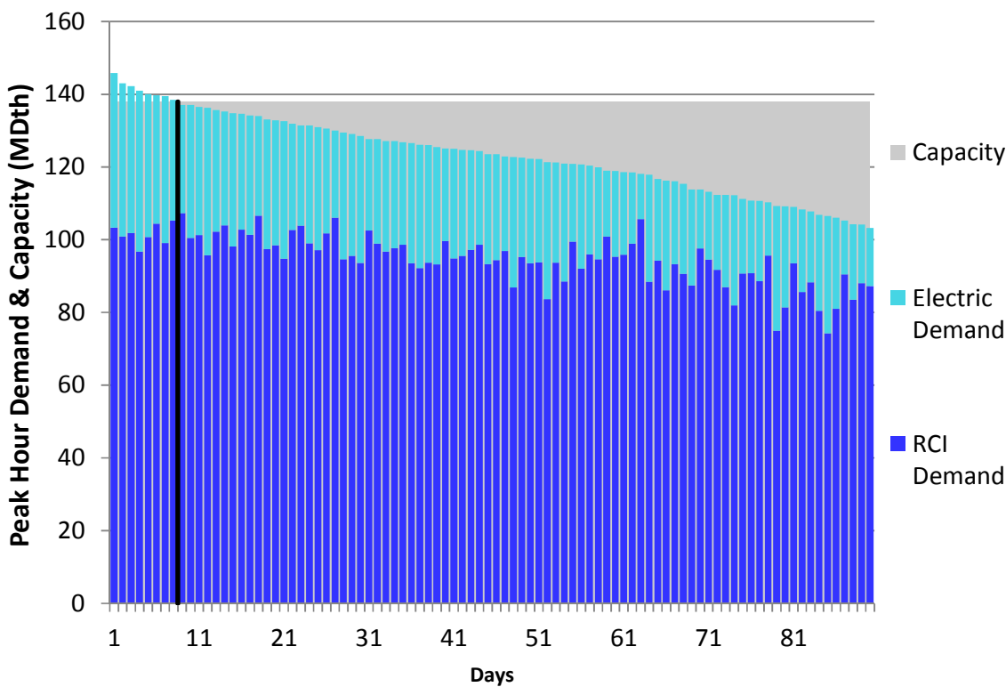
Figure L124. RGDS S14 Winter 2018 – Transco Leidy to Station 210 – Descending Demand
