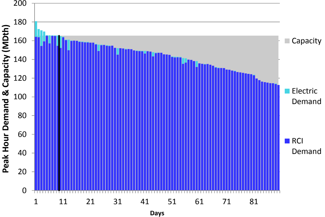
Figure L122. RGDS S14 Winter 2018 – Transco Z5 – Descending Demand
