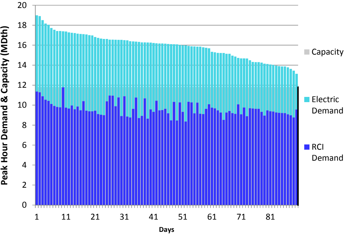
Figure L158. RGDS S14 Winter 2023 – NB/NS – Descending Demand
