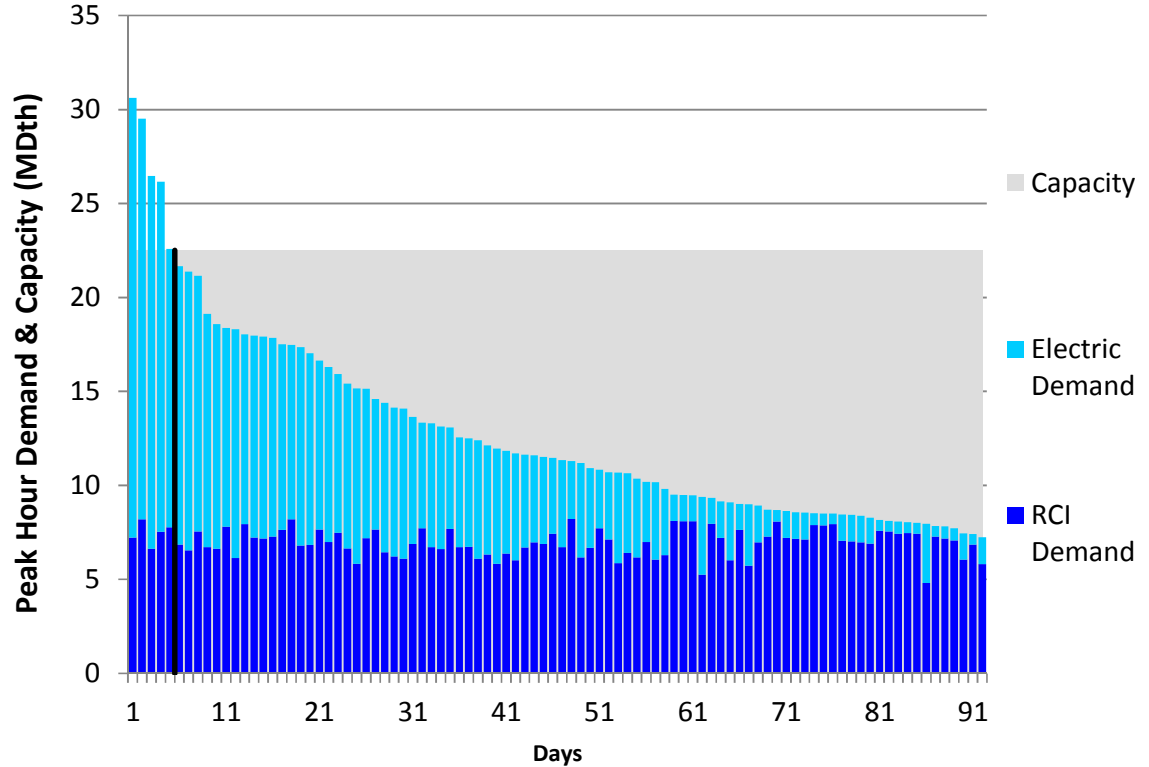
Figure L130. RGDS S14 Summer 2018 – Dominion Southeast – Descending Demand
