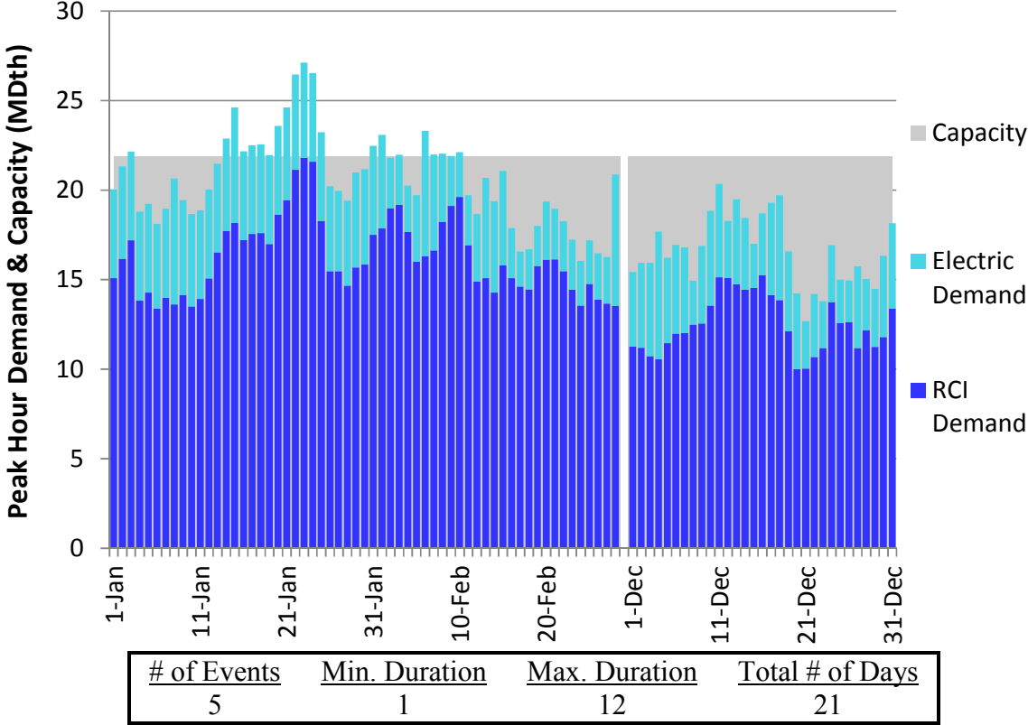
Figure L102. RGDS S14 Winter 2018 – Empire – Descending Demand
