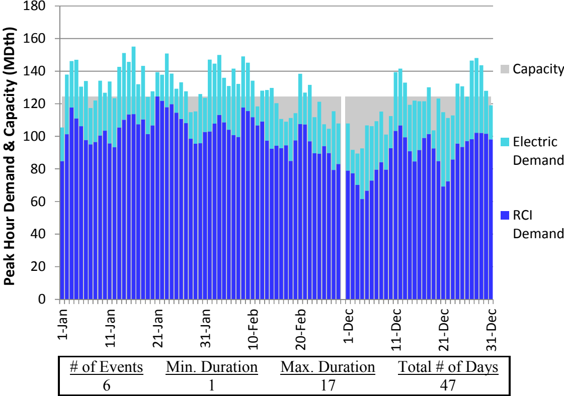
Figure L166. RGDS S14 Winter 2023 – Texas Eastern M3 North – Descending Demand
