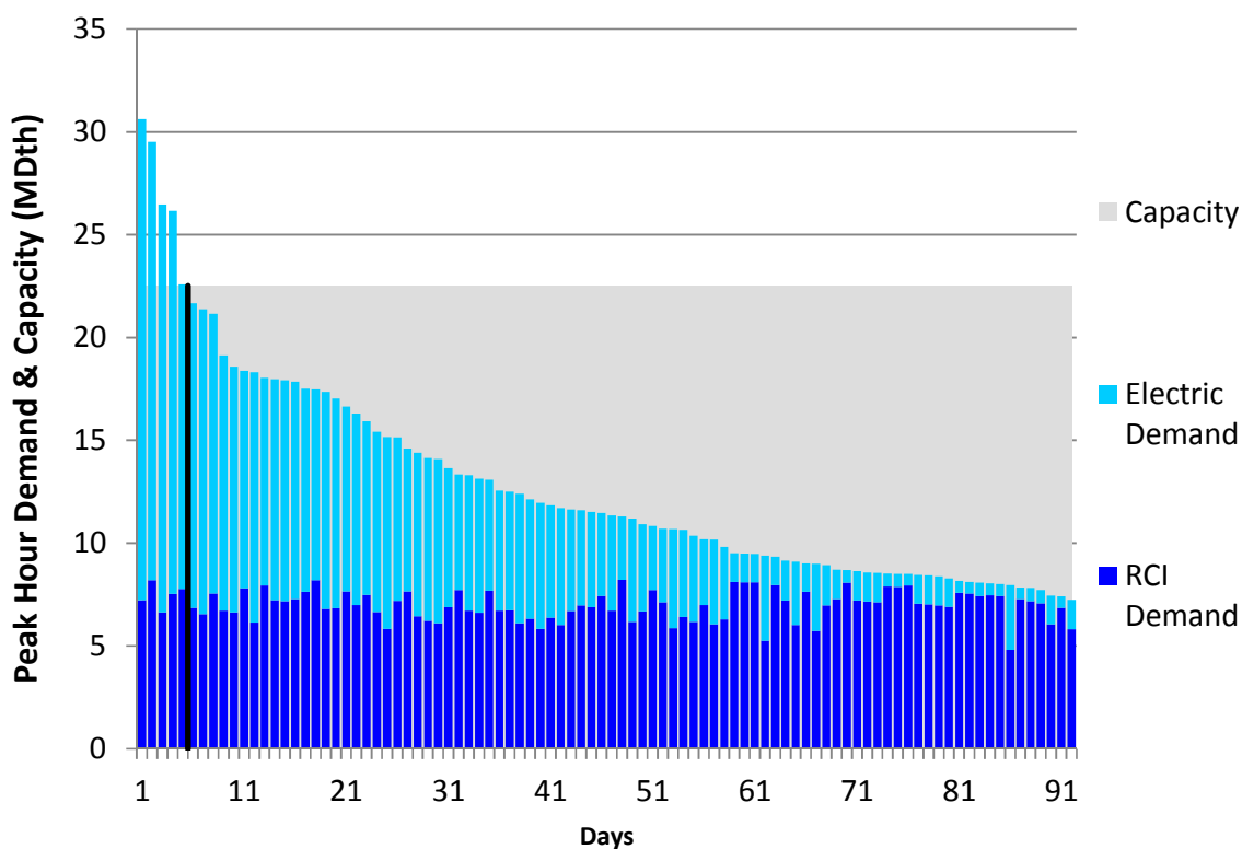
Figure L238. RGDS S16 Summer 2018 – Dominion Southeast – Descending Demand
