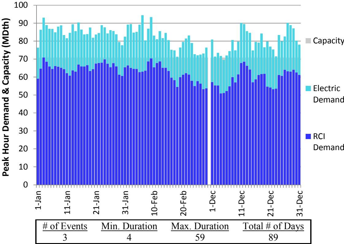
Figure L172. RGDS S14 Winter 2023 – Transco Leidy Atlantic – Descending Demand
