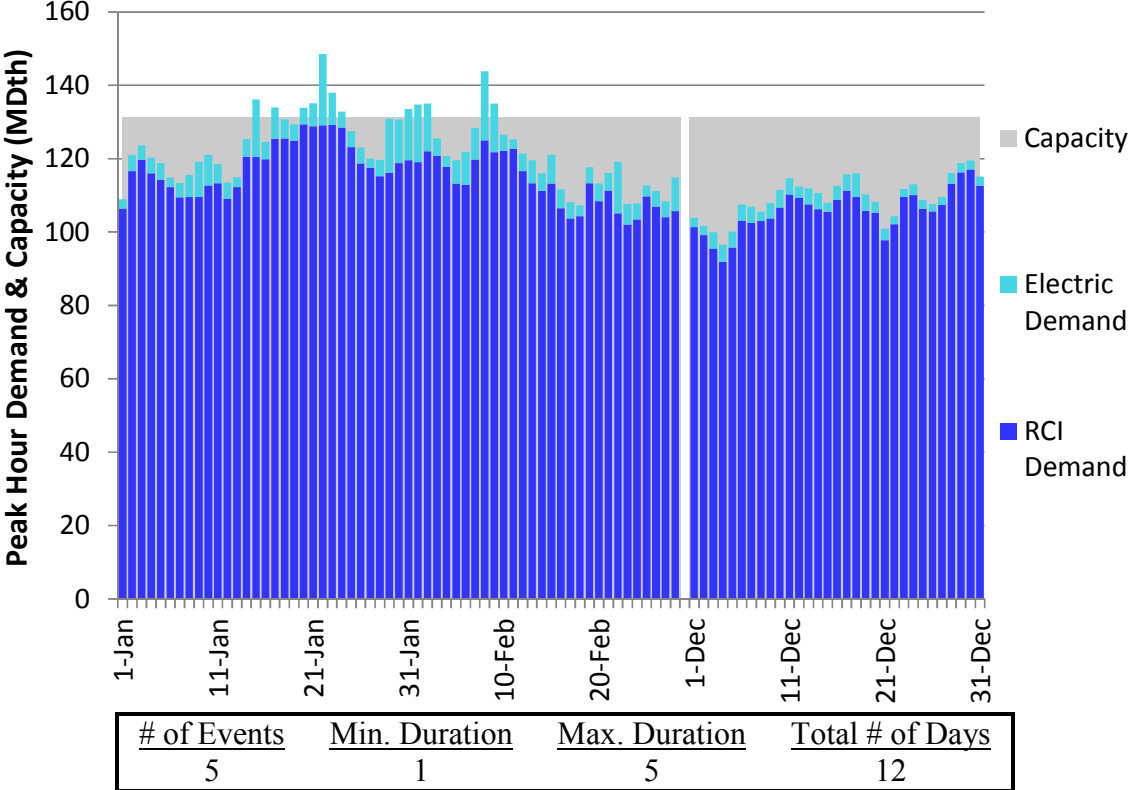
Figure L224. RGDS S16 Winter 2018 – TransCanada Ontario West – Descending Demand
