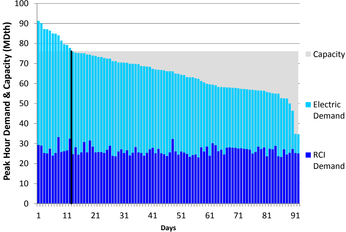
Figure L180. RGDS S14 Summer 2023 – Algonquin CT – Descending Demand
