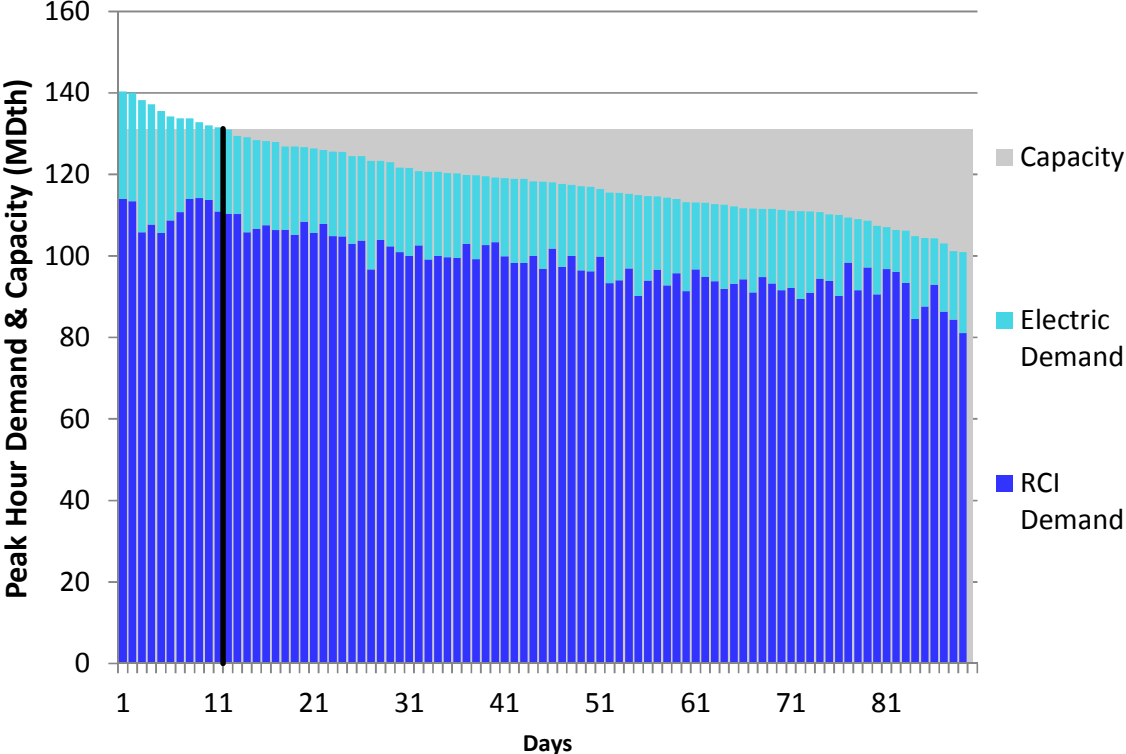
Figure L274. RGDS S16 Winter 2023 – TransCanada Ontario West – Descending Demand
