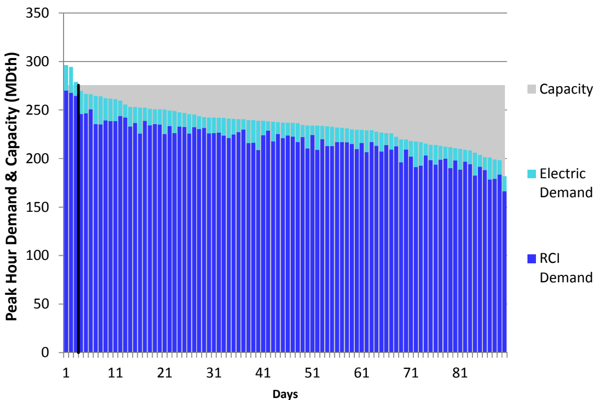
Figure L74. RGDS S13 Winter 2023 – Union Gas Dawn – Descending Demand
