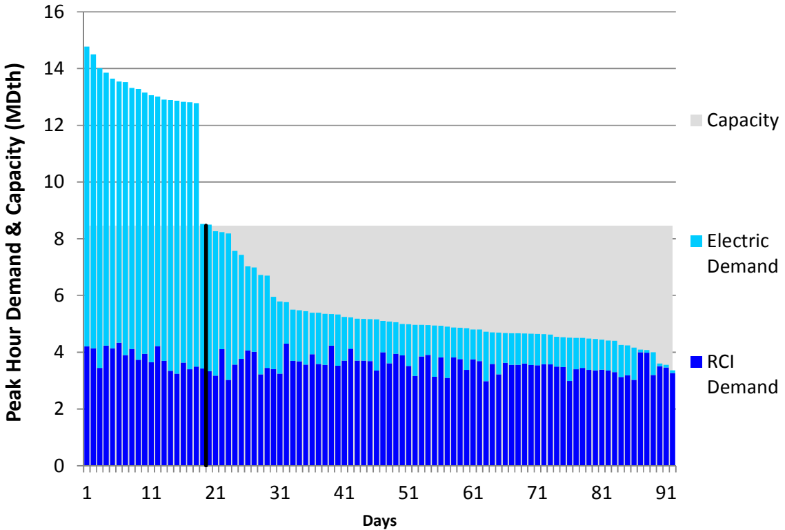
Figure L38. RGDS S13 Summer 2018 – Eastern Shore – Descending Demand
