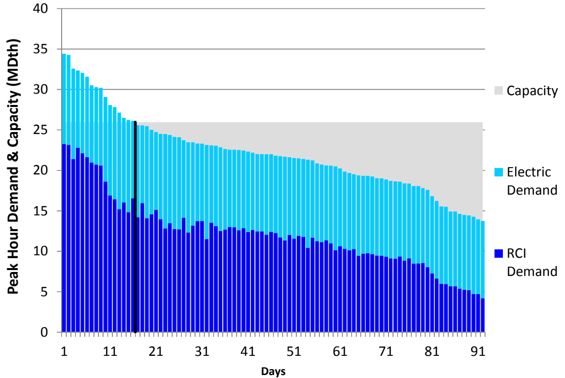
Figure L192. RGDS S14 Summer 2023 – Texas Eastern ETX – Descending Demand
