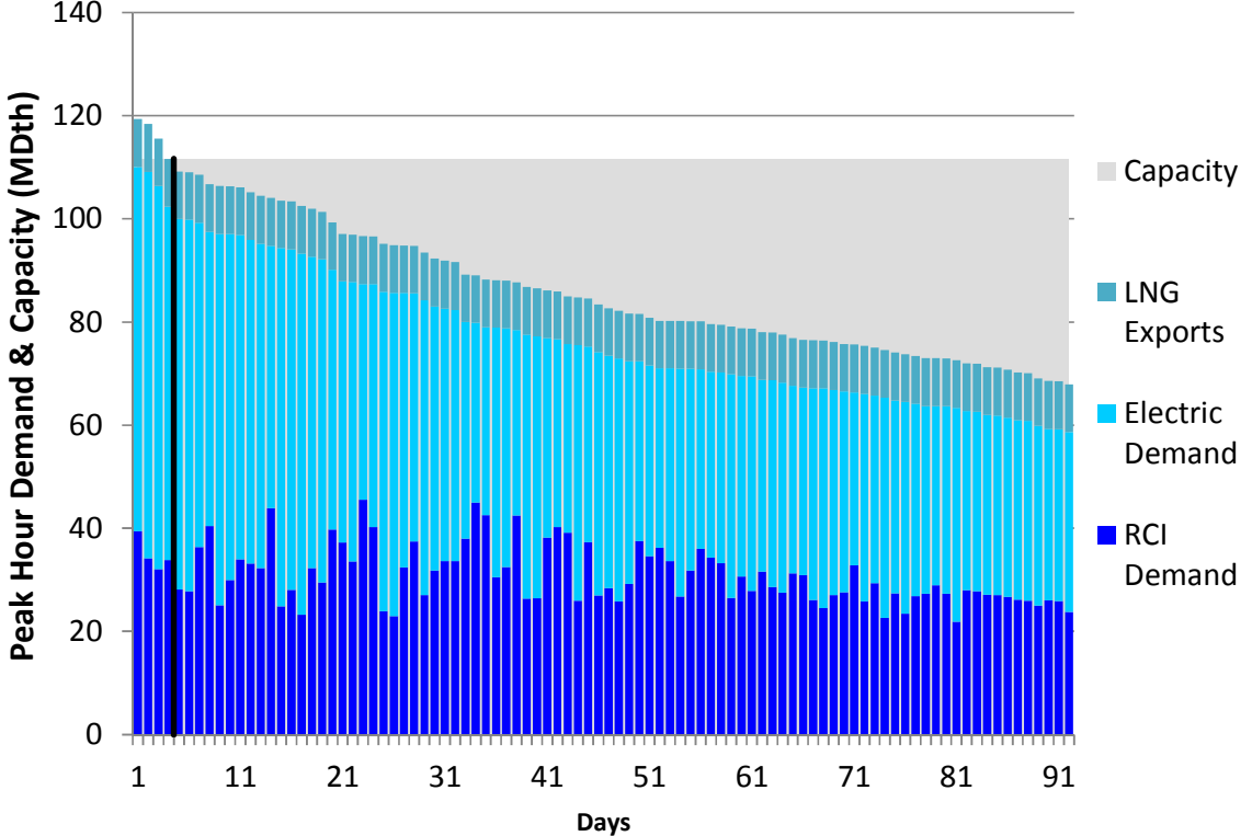
Figure L76. RGDS S13 Summer 2023 – Columbia Gas VA/MD – Descending Demand
