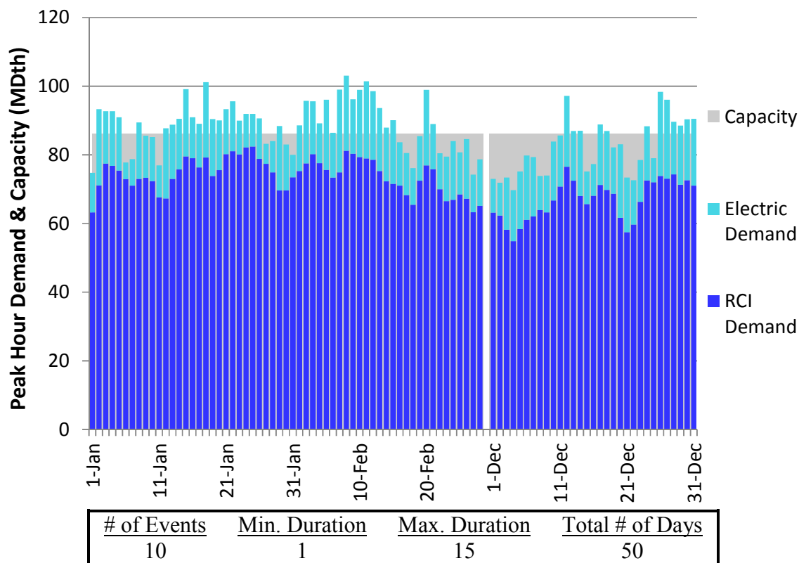
Figure L112. RGDS S14 Winter 2018 – Texas Eastern M2 PA South – Descending Demand
