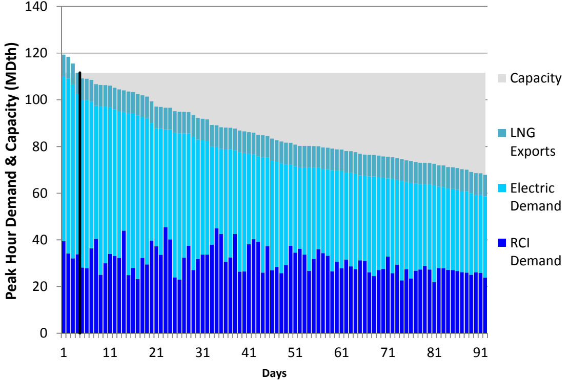
Figure L182. RGDS S14 Summer 2023 – Columbia Gas VA/MD – Descending Demand
