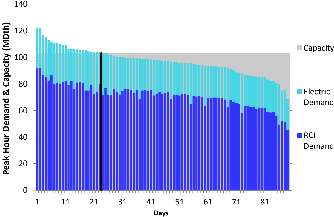
Figure L86. RGDS S14 Winter 2018 – Columbia Gas VA/MD – Descending Demand
