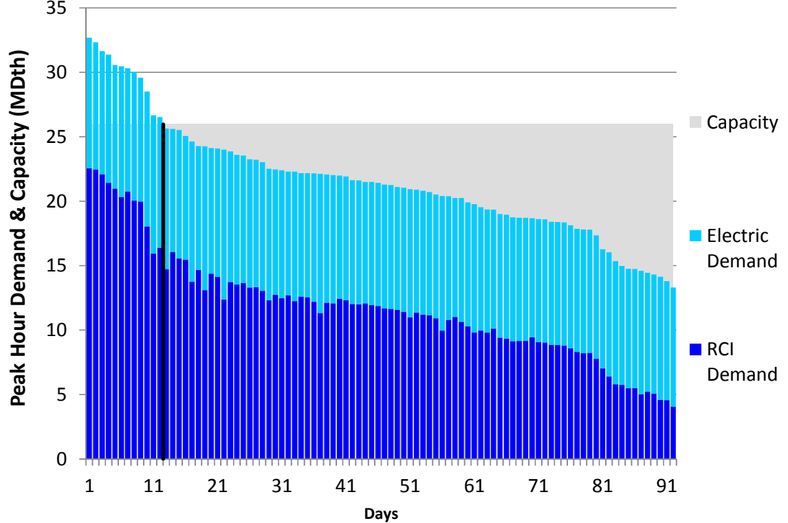
Figure L134. RGDS S14 Summer 2018 – Texas Eastern ETX – Descending Demand
