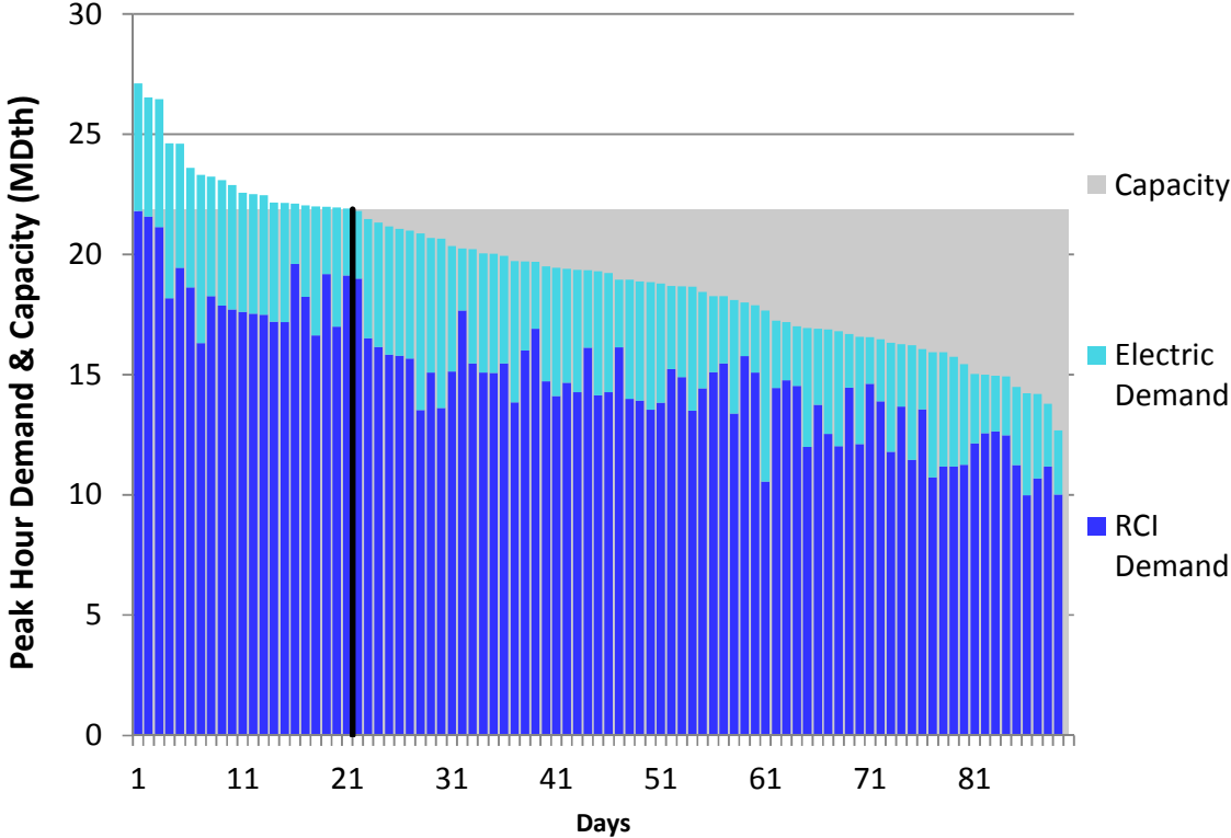
Figure L102. RGDS S14 Winter 2018 – Empire – Descending Demand
