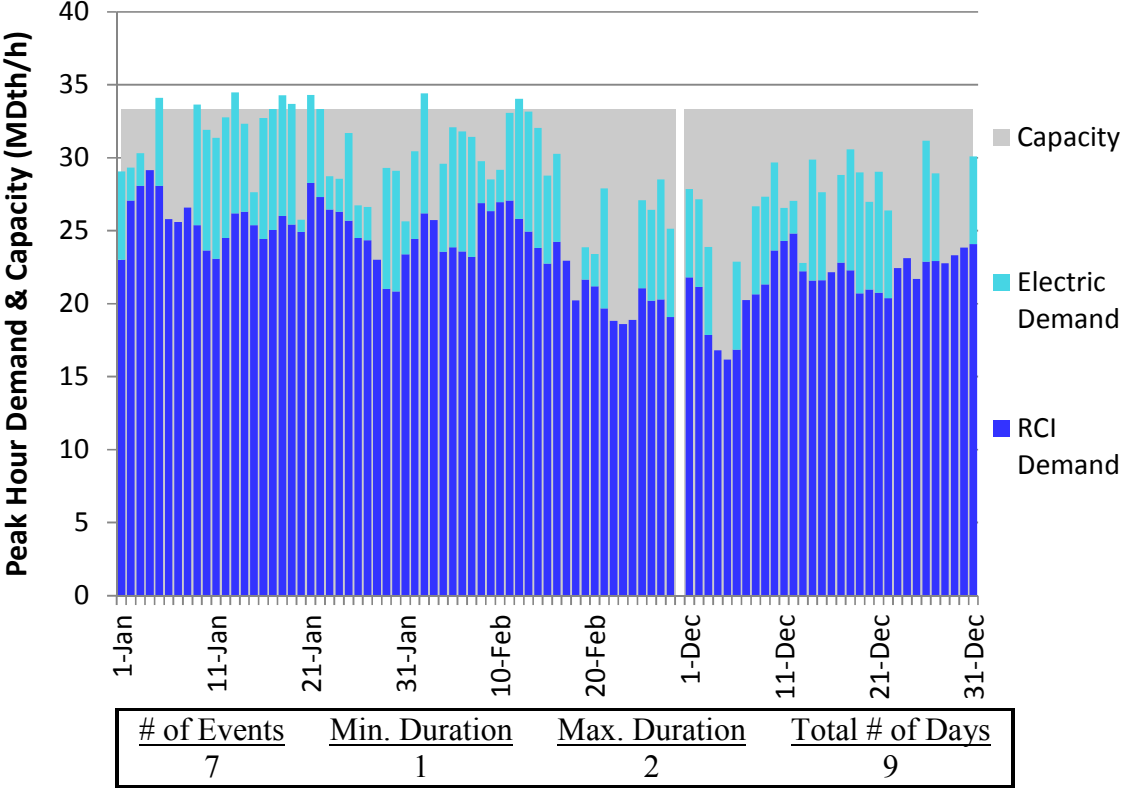
Figure L208. RGDS S16 Winter 2018 – East Tennessee – Descending Demand
