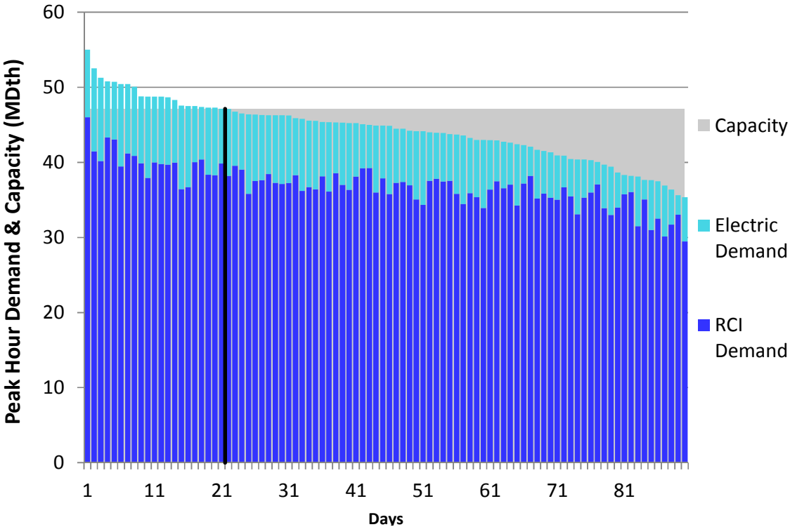
Figure L198. RGDS S16 Winter 2018 – Columbia Gas W PA/NY – Descending Demand
