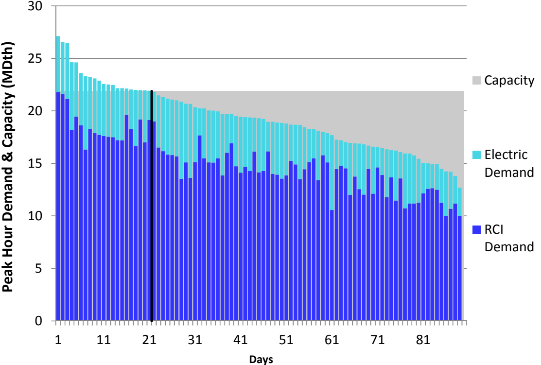
Figure L212. RGDS S16 Winter 2018 – Empire – Descending Demand
