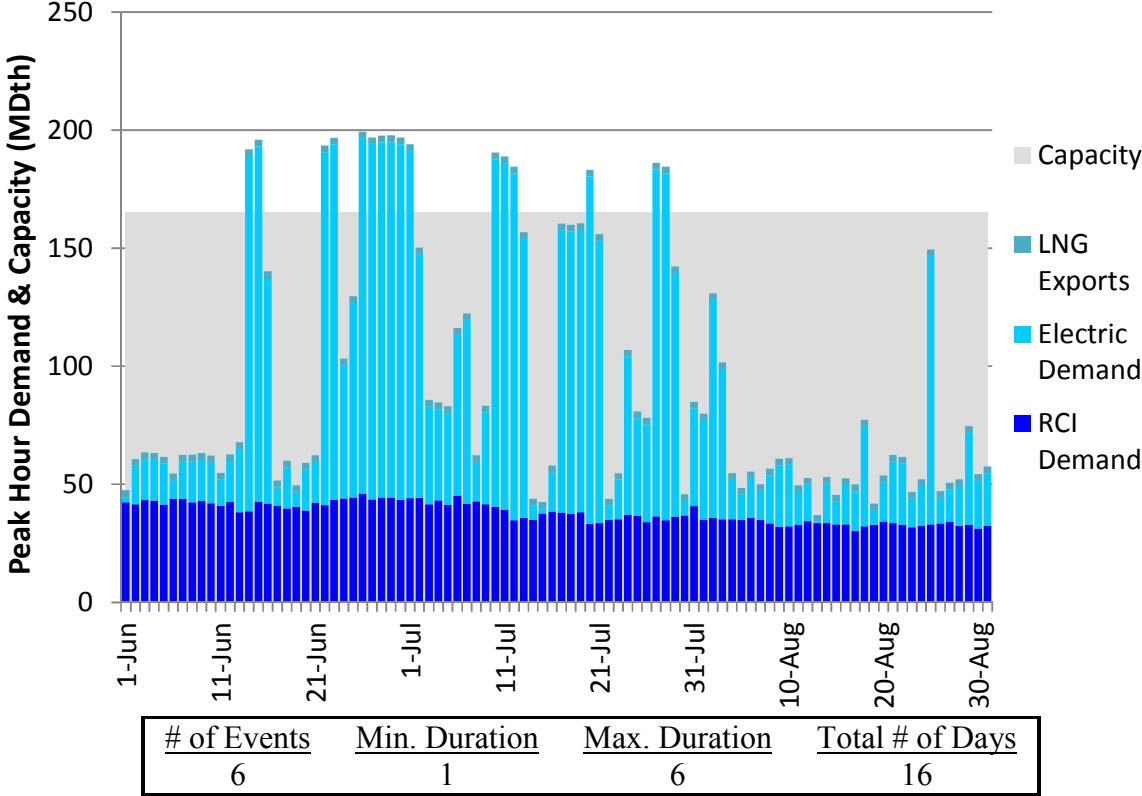
Figure L294. RGDS S16 Summer 2023 – Transco Z5 – Descending Demand
