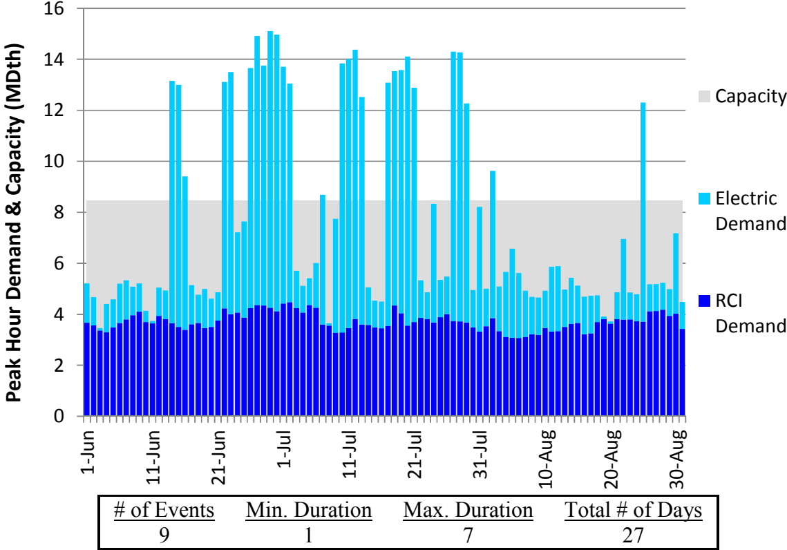
Figure L290. RGDS S16 Summer 2023 – Eastern Shore – Descending Demand
