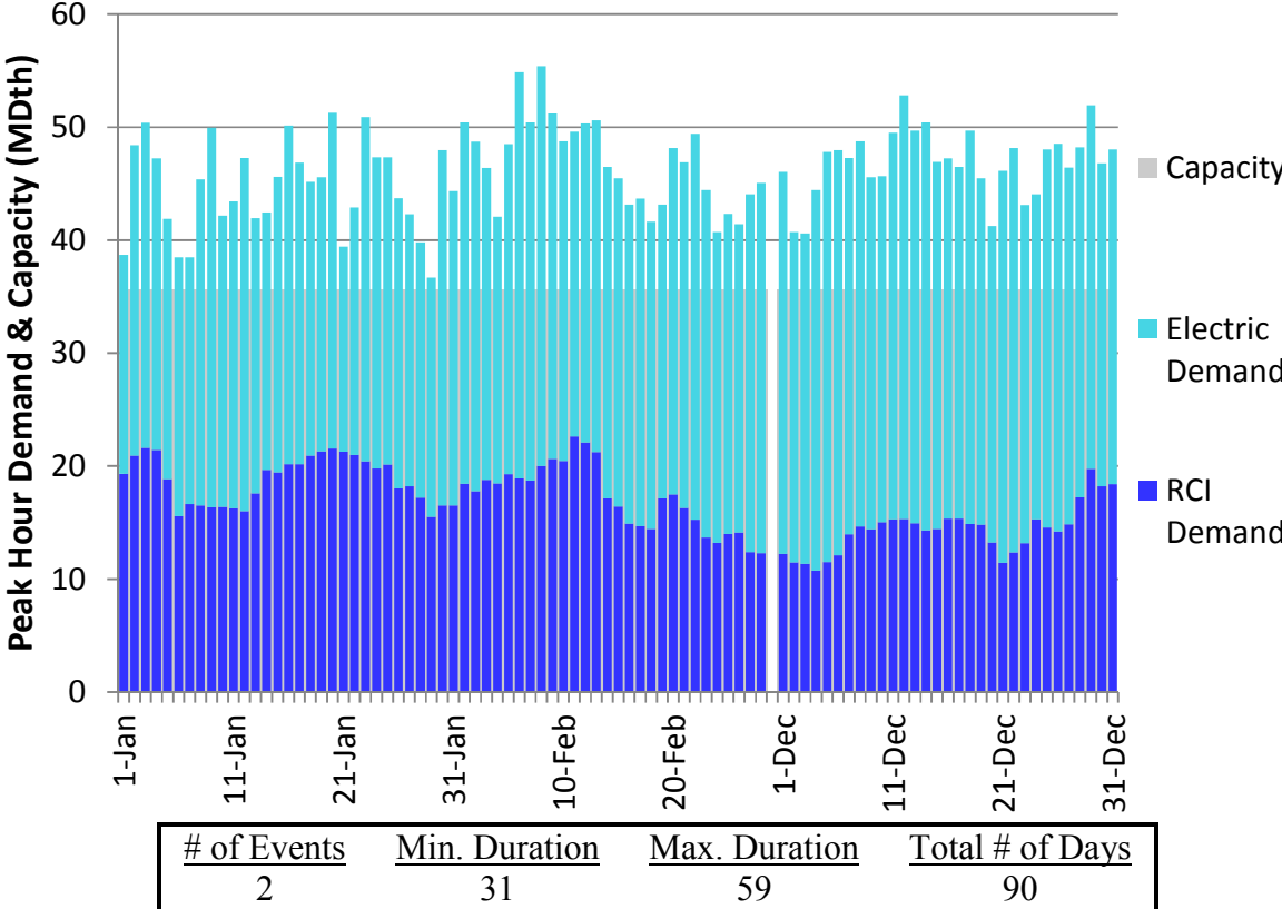
Figure L54. RGDS S13 Winter 2023 – Iroquois Z1 → Z2 – Descending Demand
