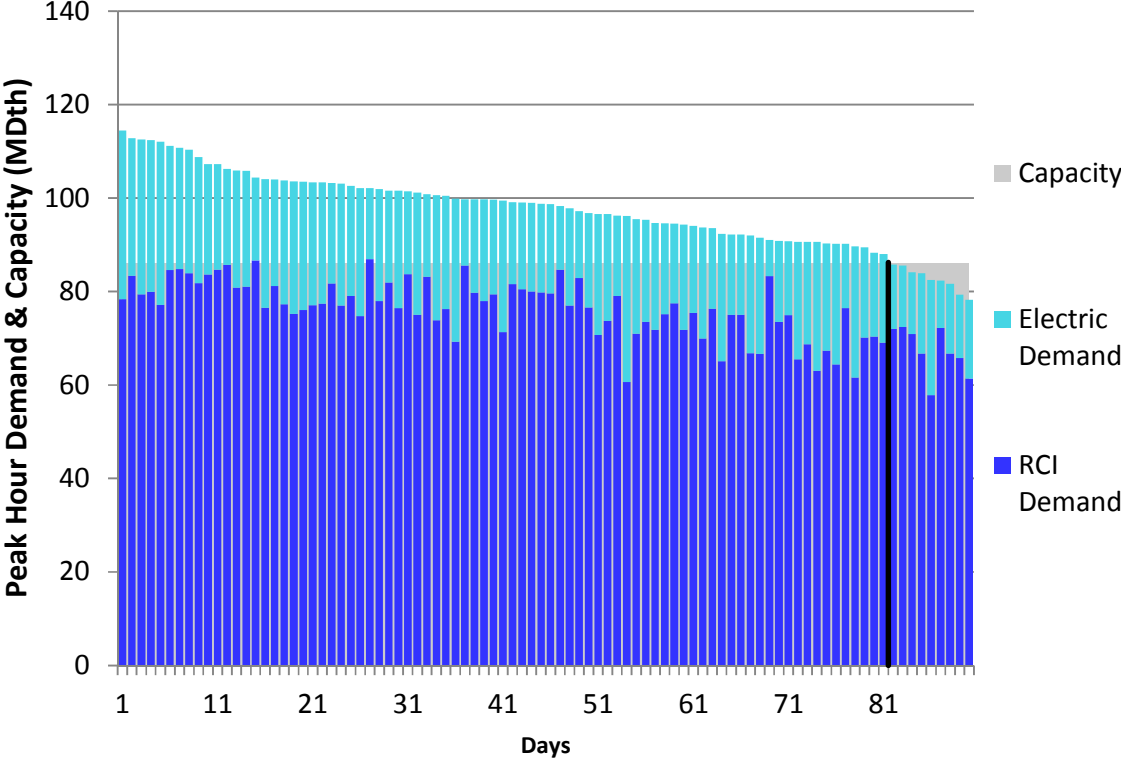
Figure L164. RGDS S14 Winter 2023 – Texas Eastern M2 PA South – Descending Demand
