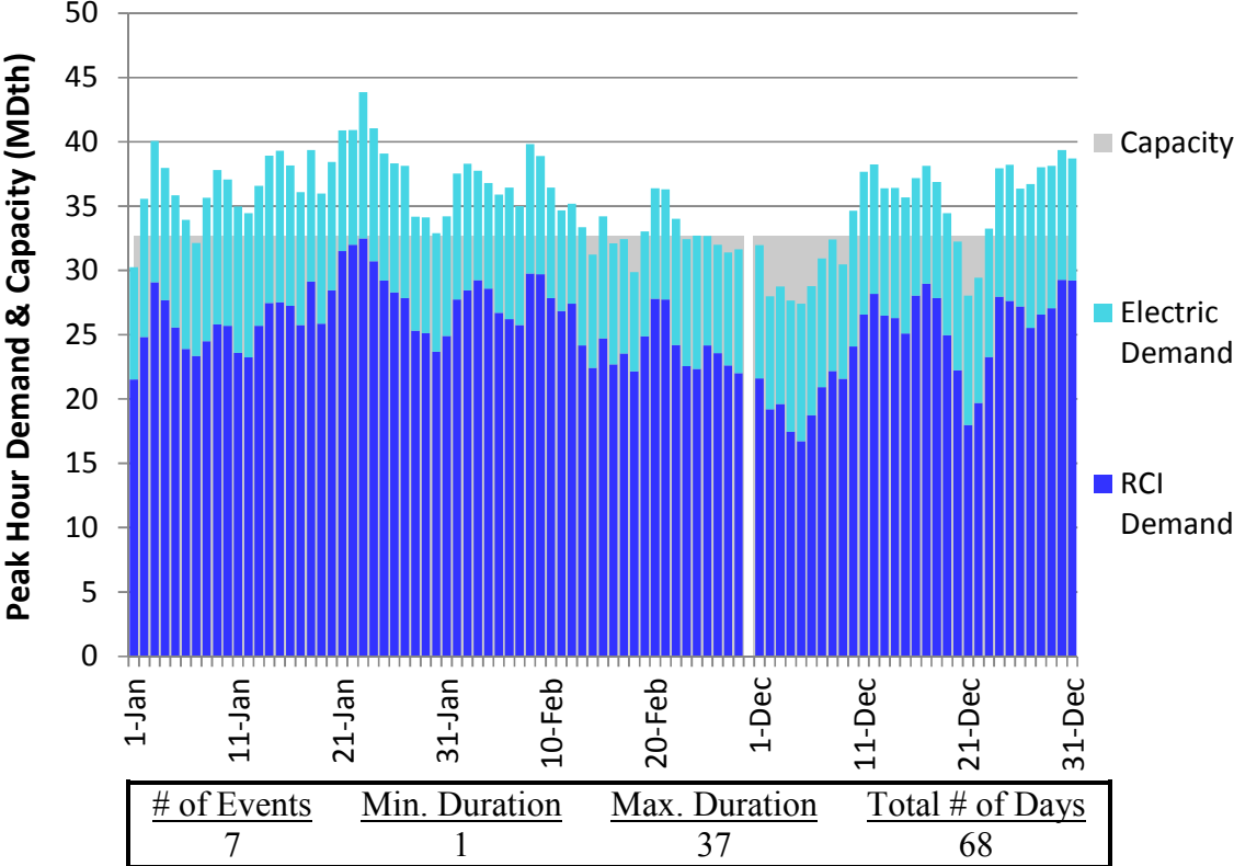
Figure L56. RGDS S13 Winter 2023 – Millennium – Descending Demand
