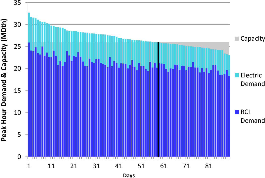
Figure L106. RGDS S14 Winter 2018 – NB/NS – Descending Demand
