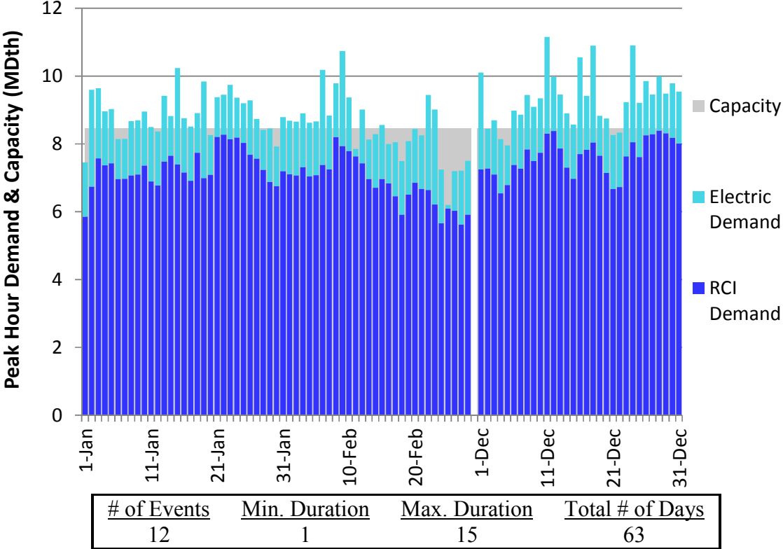
Figure L260. RGDS S16 Winter 2023 – Eastern Shore – Descending Demand
