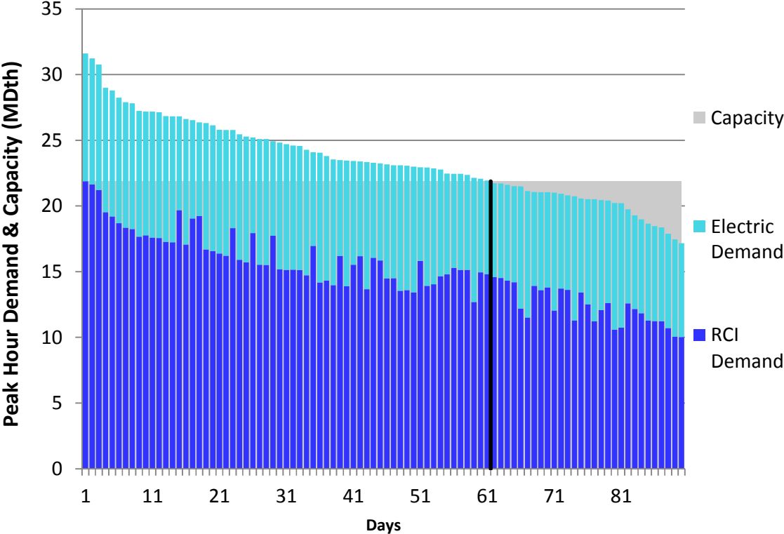
Figure L262. RGDS S16 Winter 2023 – Empire – Descending Demand
