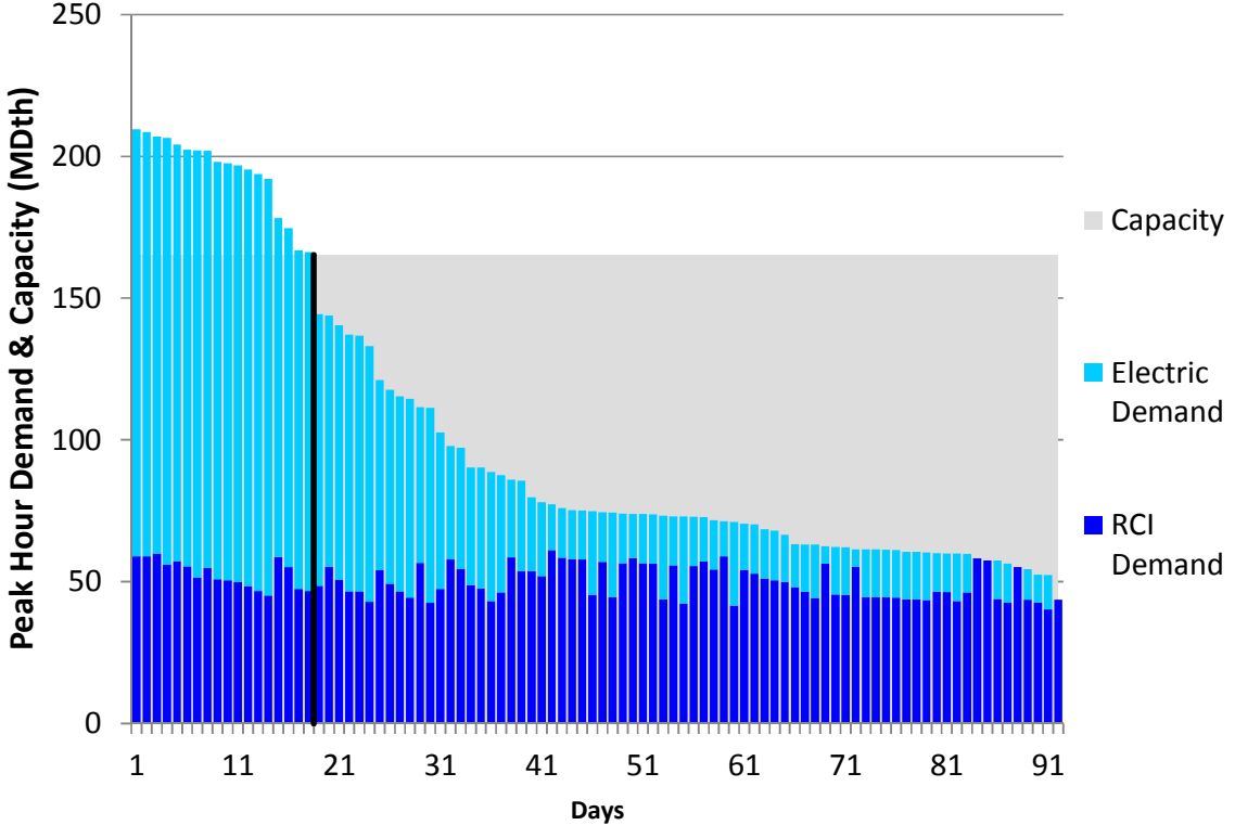
Figure L244. RGDS S16 Summer 2018 – Transco Z5 – Descending Demand
