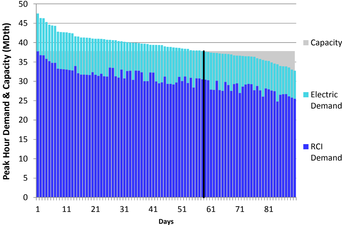
Figure L144. RGDS S14 Winter 2023 – Dominion Eastern NY– Descending Demand
