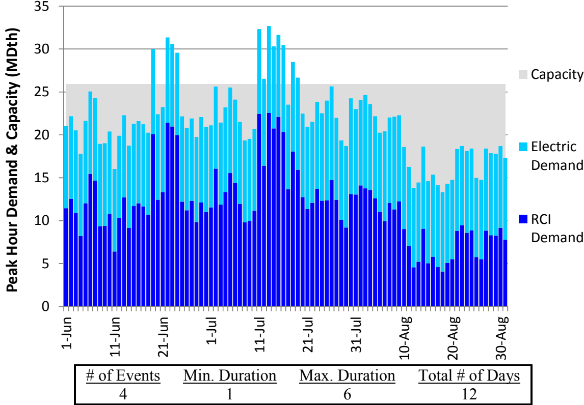
Figure L134. RGDS S14 Summer 2018 – Texas Eastern ETX – Descending Demand
