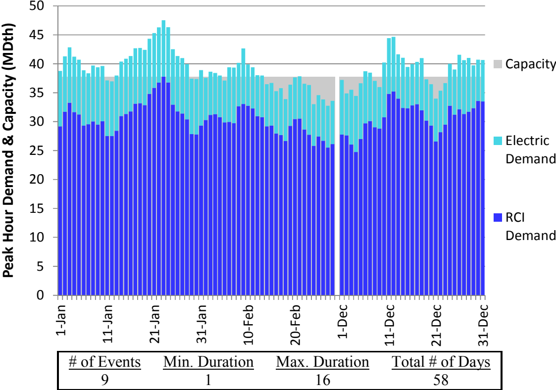
Figure L144. RGDS S14 Winter 2023 – Dominion Eastern NY– Descending Demand
