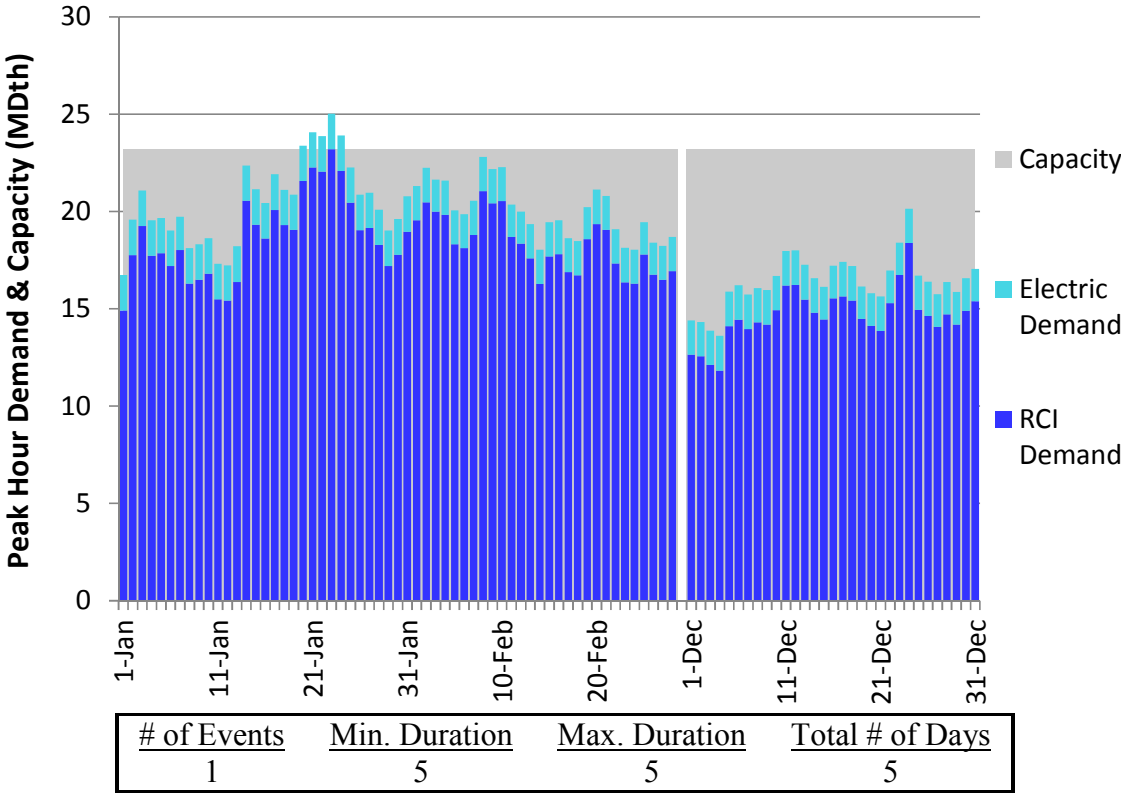
Figure L146. RGDS S14 Winter 2023 – Dominion Western NY– Descending Demand
