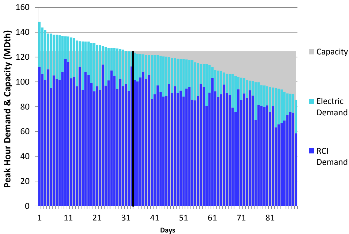
Figure L222. RGDS S16 Winter 2018 – Texas Eastern M3 North – Descending Demand
