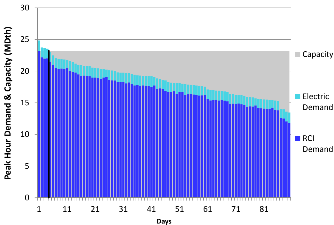
Figure L204. RGDS S16 Winter 2018 – Dominion Western NY– Descending Demand
