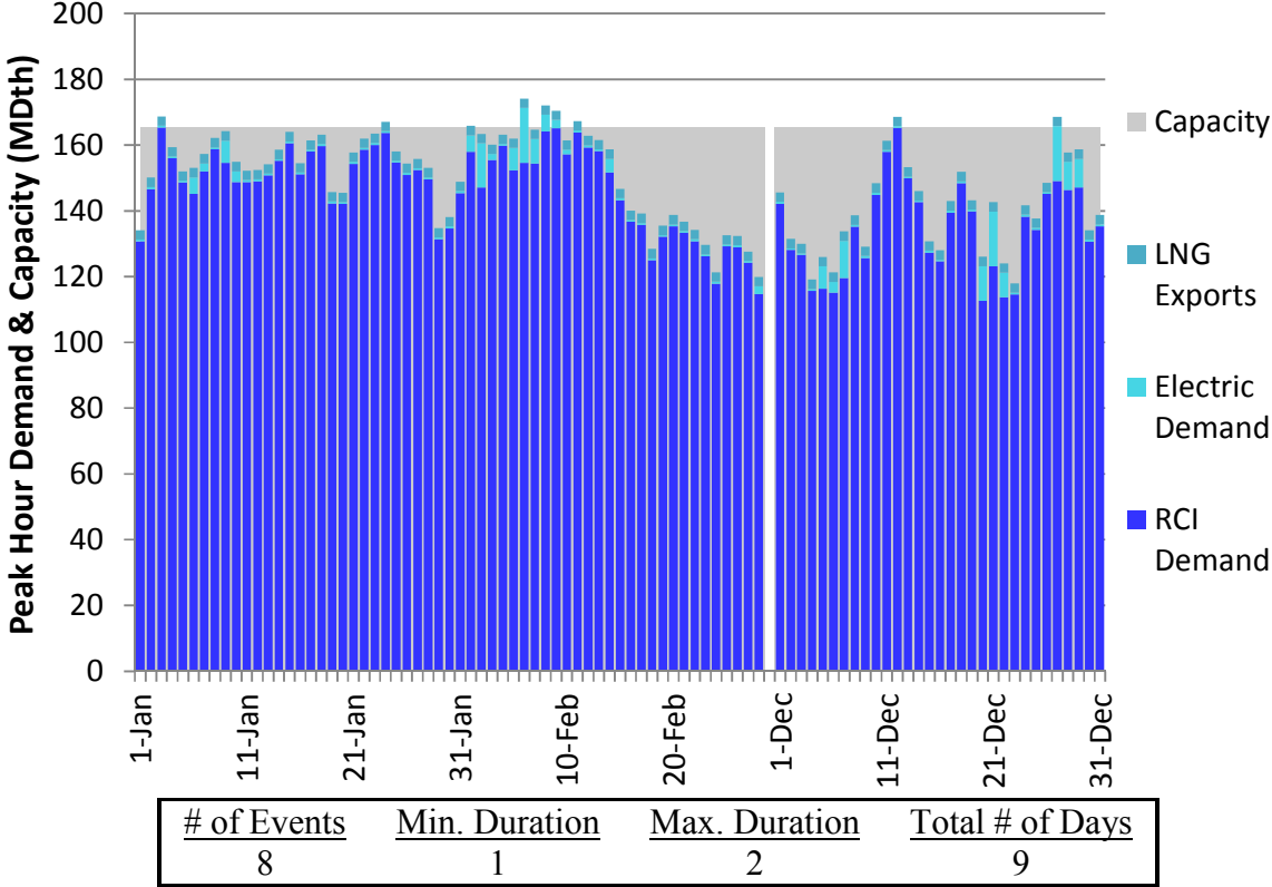
Figure L70. RGDS S13 Winter 2023 – Transco Z5 – Descending Demand
