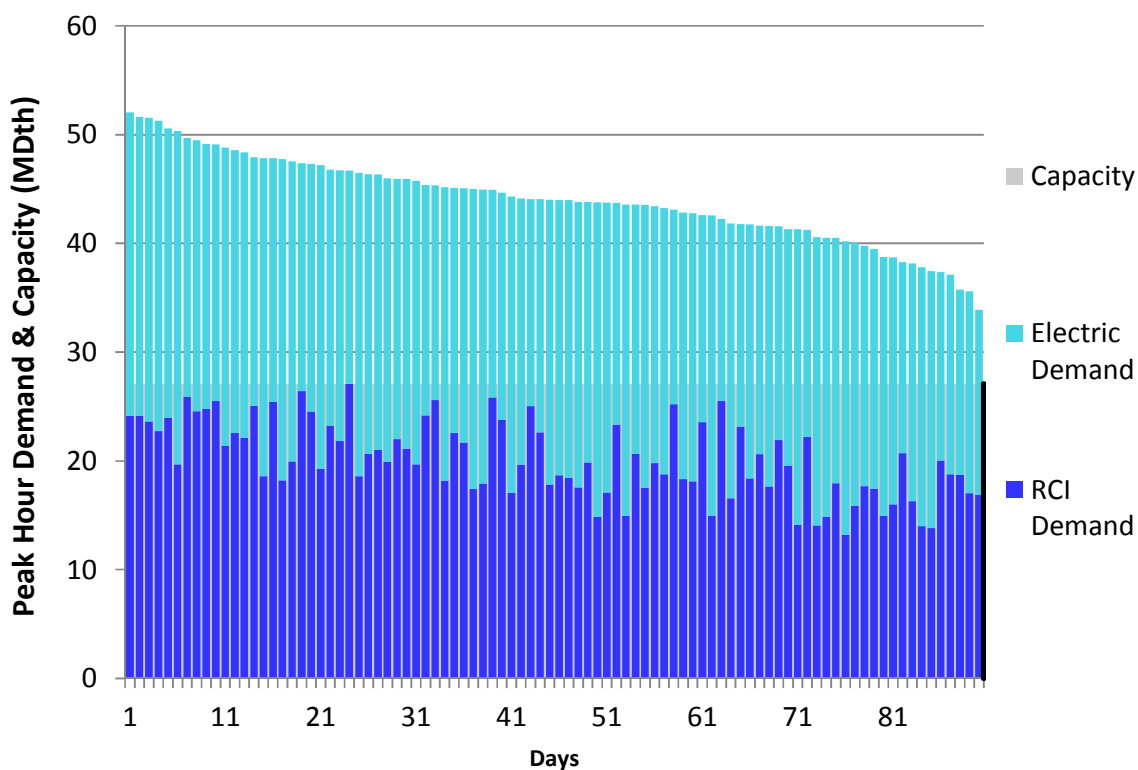
Figure L46. RGDS S13 Winter 2023 – Constitution – Descending Demand
