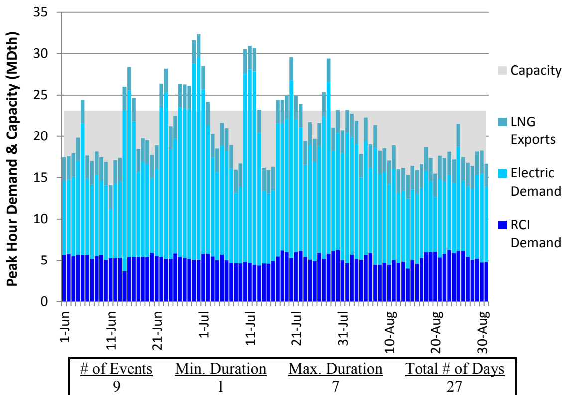
Figure L288. RGDS S16 Summer 2023 – Dominion Southeast – Descending Demand
