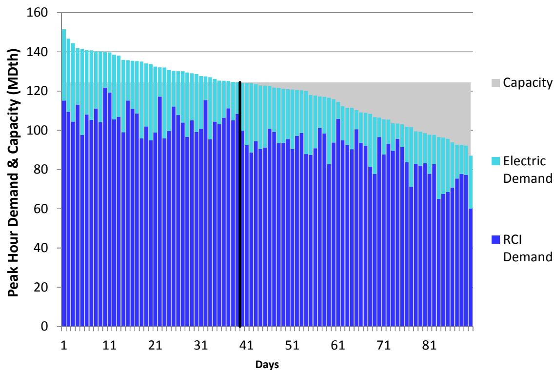
Figure L114. RGDS S14 Winter 2018 – Texas Eastern M3 North – Descending Demand
