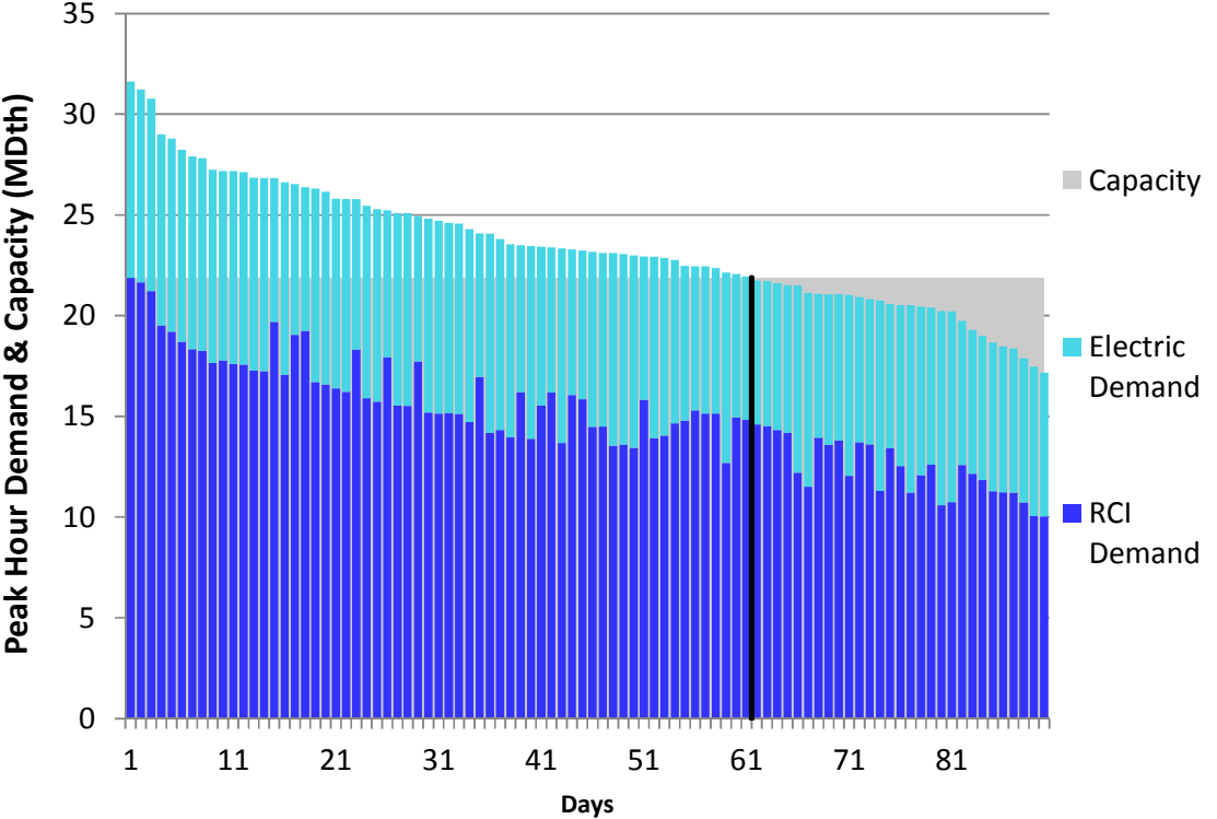
Figure L154. RGDS S14 Winter 2023 – Empire – Descending Demand
