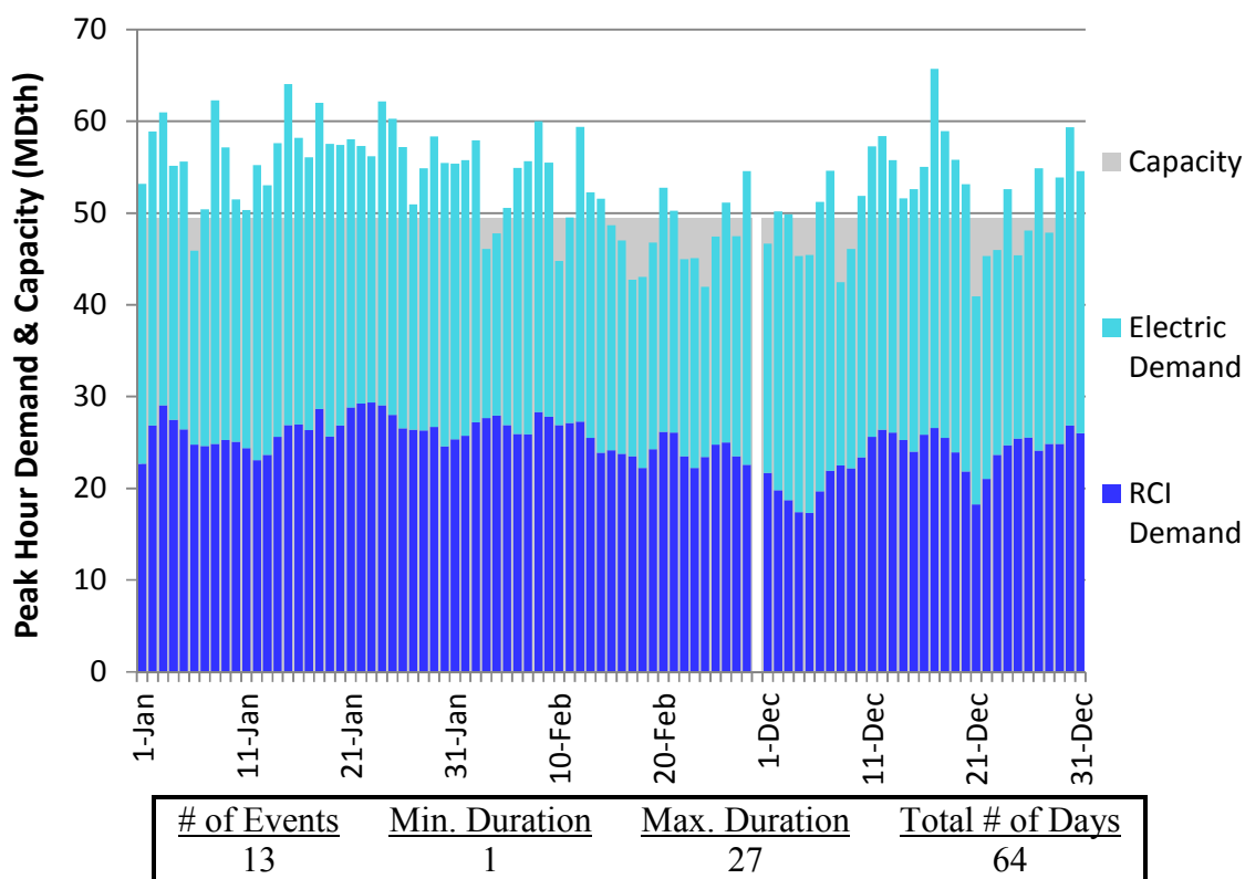
Figure L218. RGDS S16 Winter 2018 – Tennessee Z5 NY – Descending Demand
