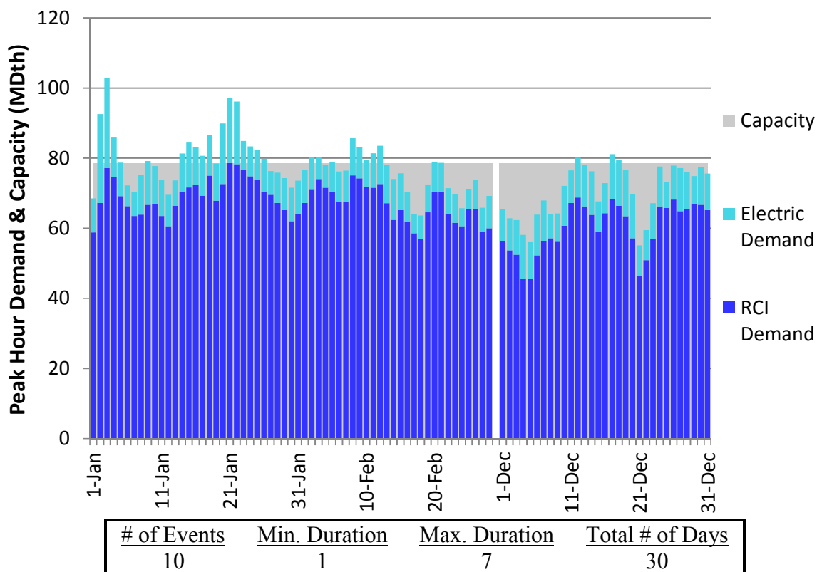
Figure L20. RGDS S13 Winter 2018 – Tennessee Z4 PA – Descending Demand
