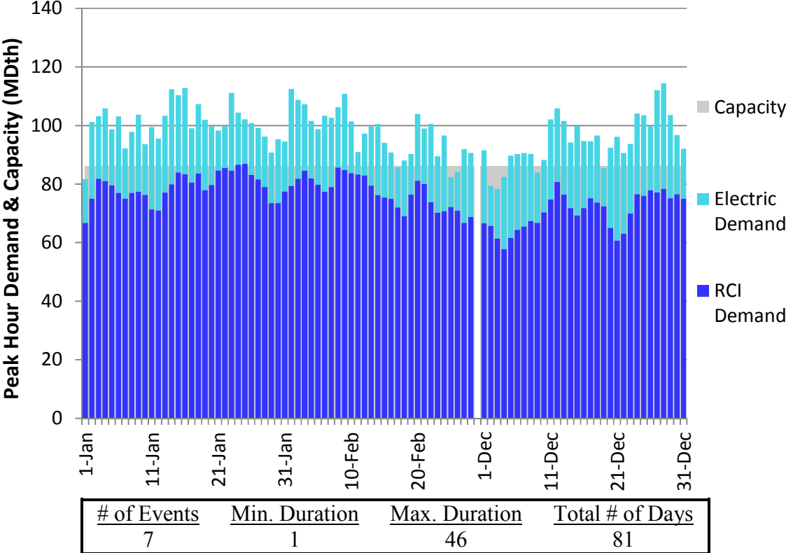
Figure L62. RGDS S13 Winter 2023 – Texas Eastern M2 PA South – Descending Demand
