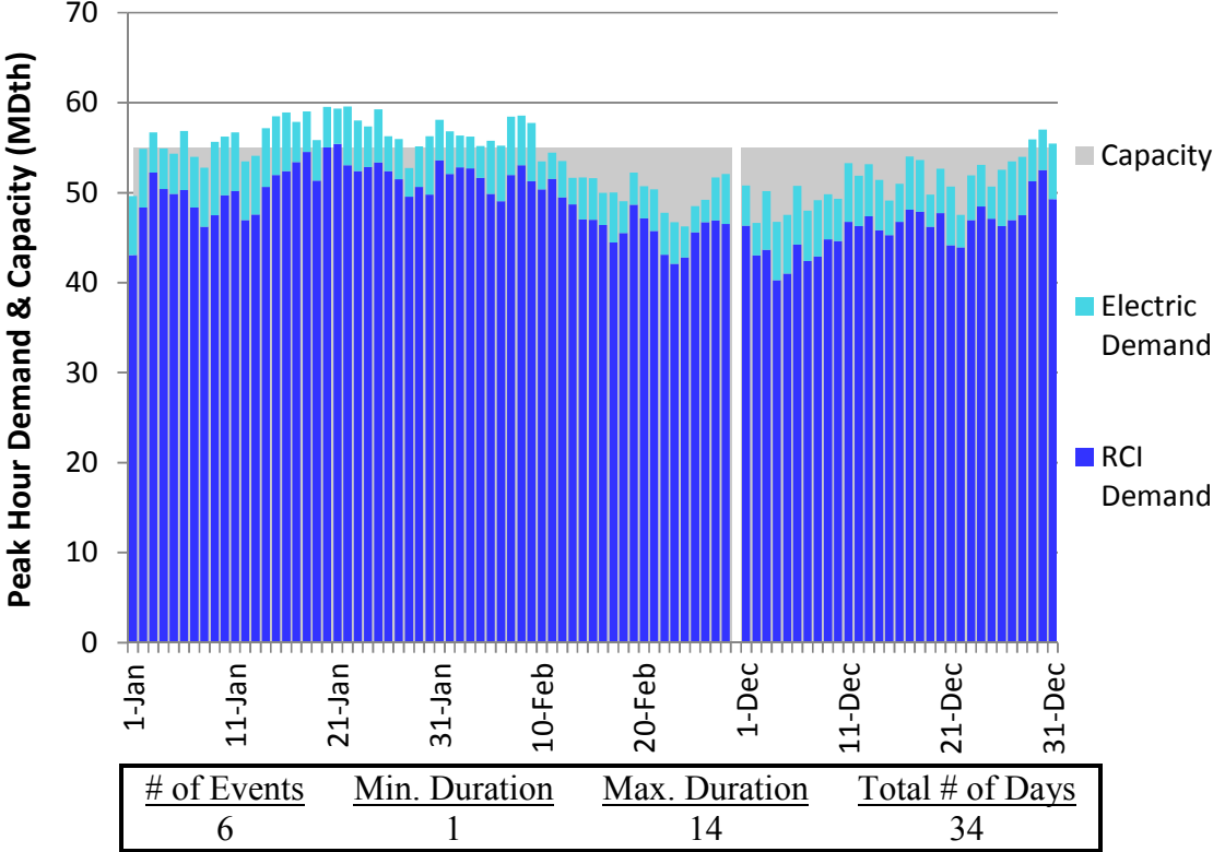
Figure L170. RGDS S14 Winter 2023 – TransCanada Quebec – Descending Demand
