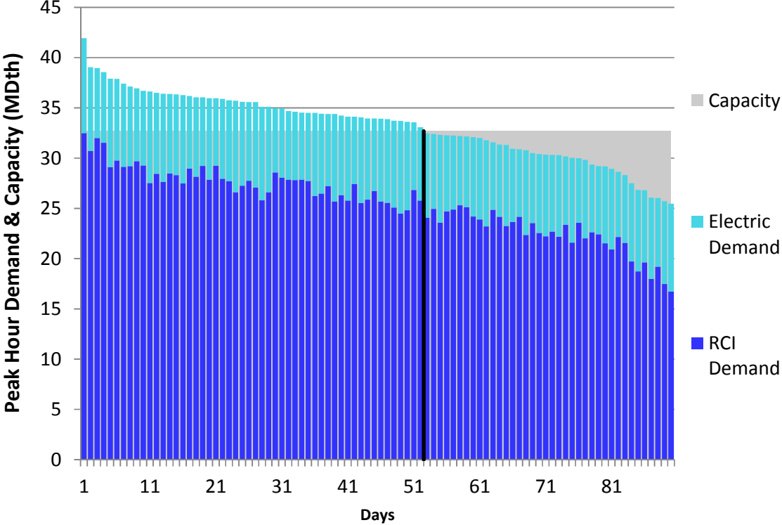
Figure L264. RGDS S16 Winter 2023 – Millennium – Descending Demand
