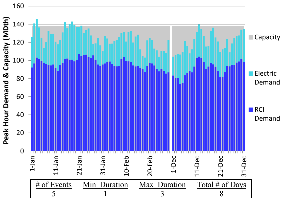
Figure L232. RGDS S16 Winter 2018 – Transco Leidy to Station 210 – Descending Demand
