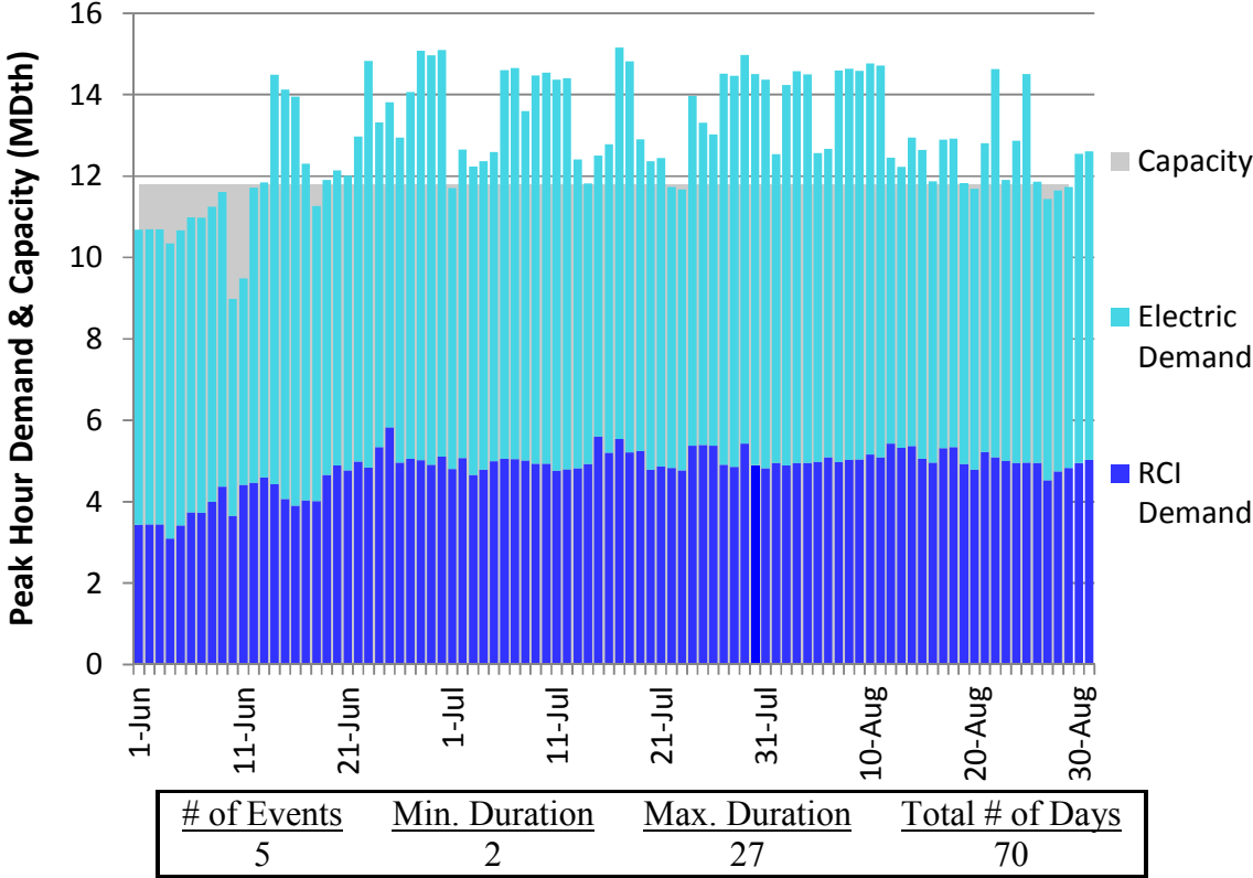
Figure L188. RGDS S14 Summer 2023 – NB/NS – Descending Demand
