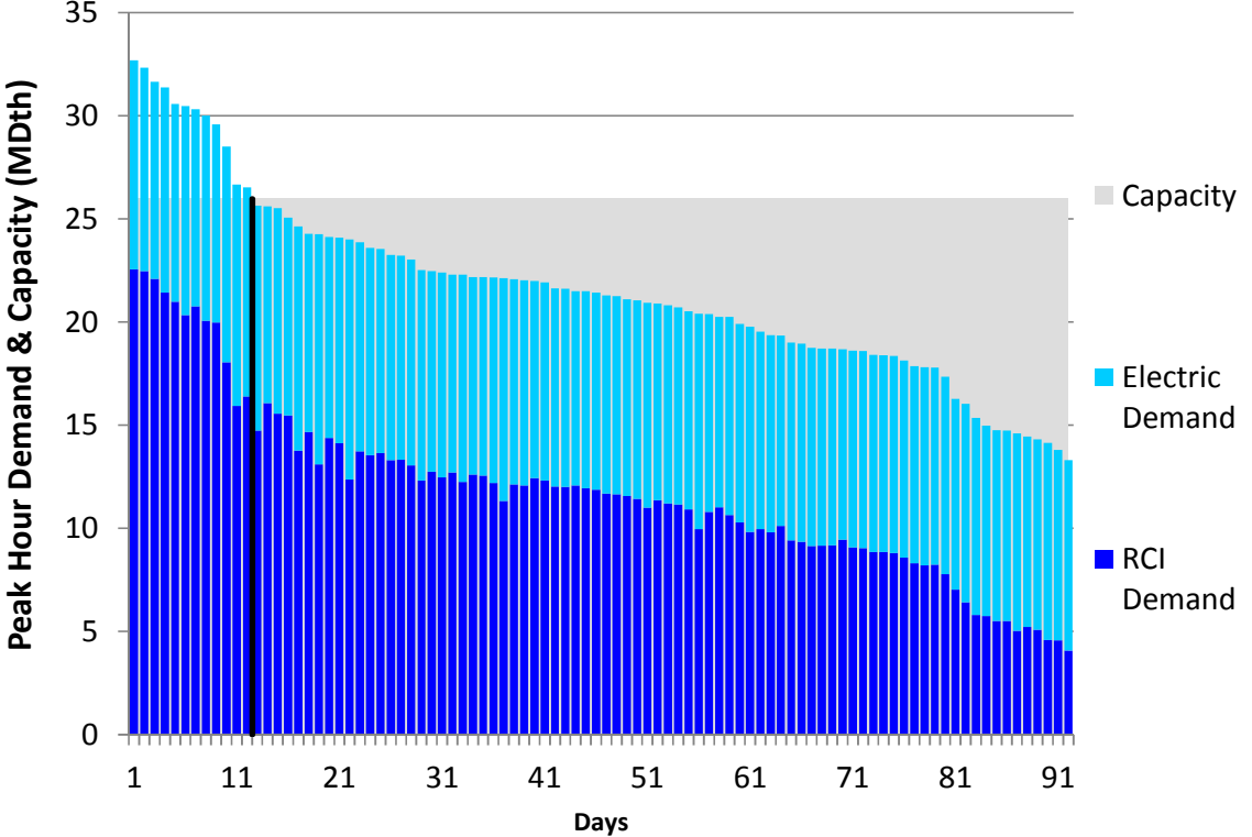
Figure L40. RGDS S13 Summer 2018 – Texas Eastern ETX – Descending Demand
