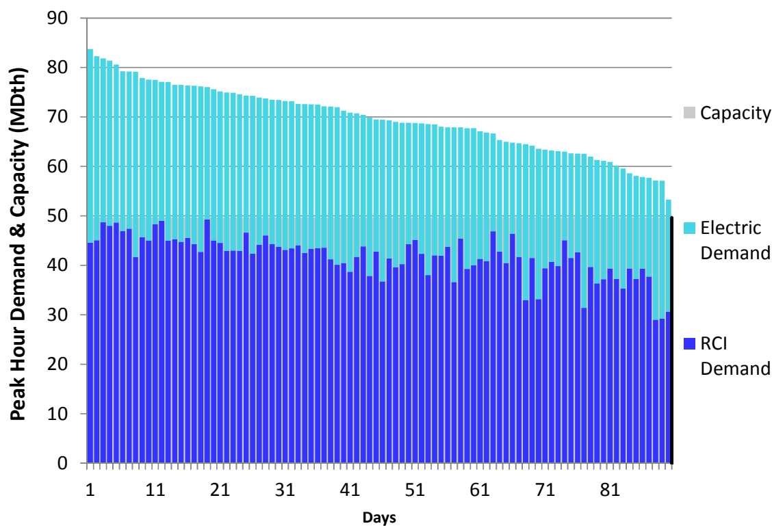
Figure L110. RGDS S14 Winter 2018 – Tennessee Z5 NY – Descending Demand
