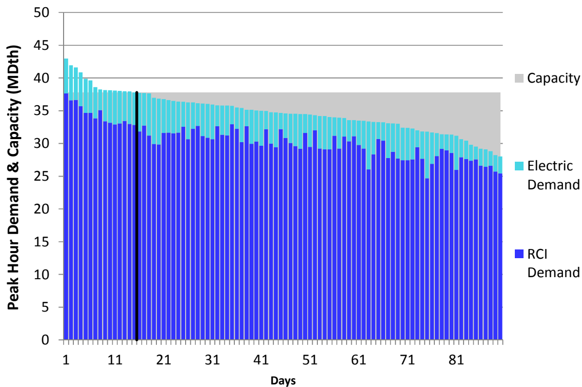
Figure L92. RGDS S14 Winter 2018 – Dominion Eastern NY– Descending Demand
