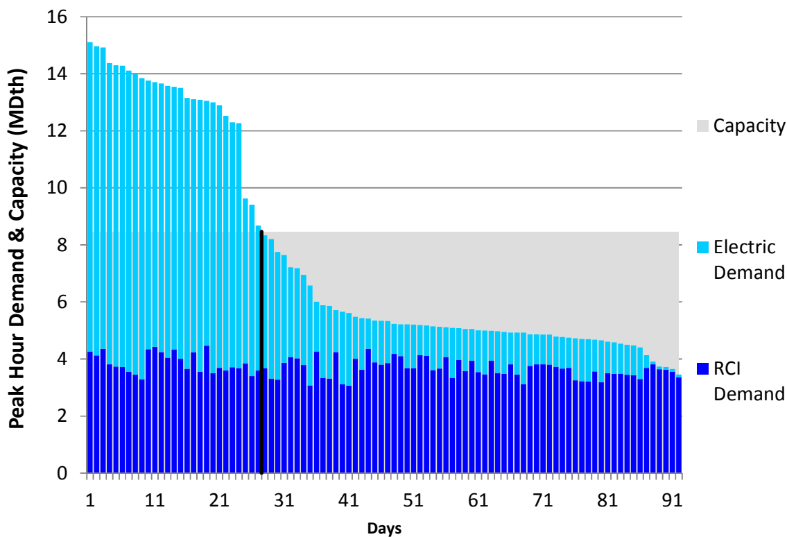
Figure L186. RGDS S14 Summer 2023 – Eastern Shore – Descending Demand
