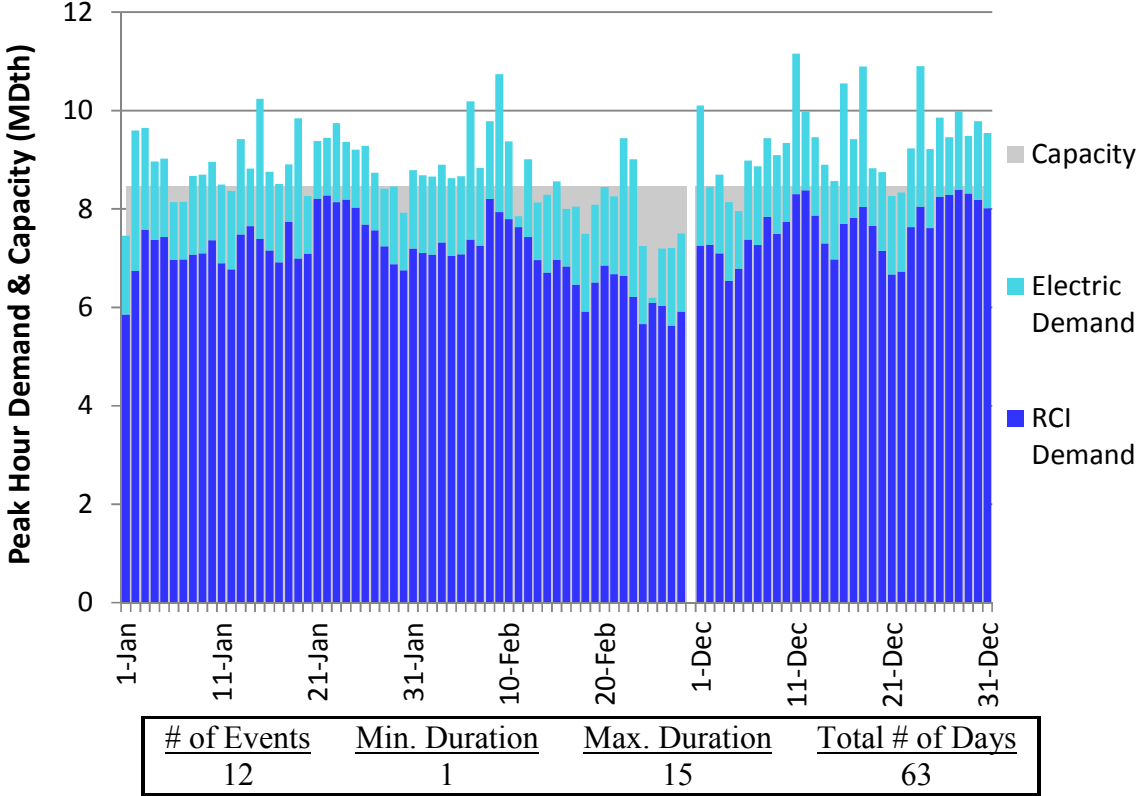
Figure L152. RGDS S14 Winter 2023 – Eastern Shore – Descending Demand
