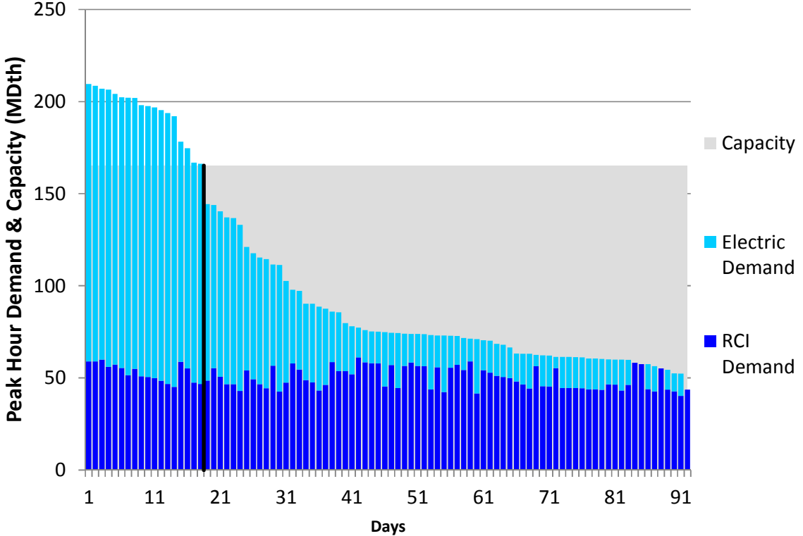
Figure L42. RGDS S13 Summer 2018 – Transco Z5 – Descending Demand
