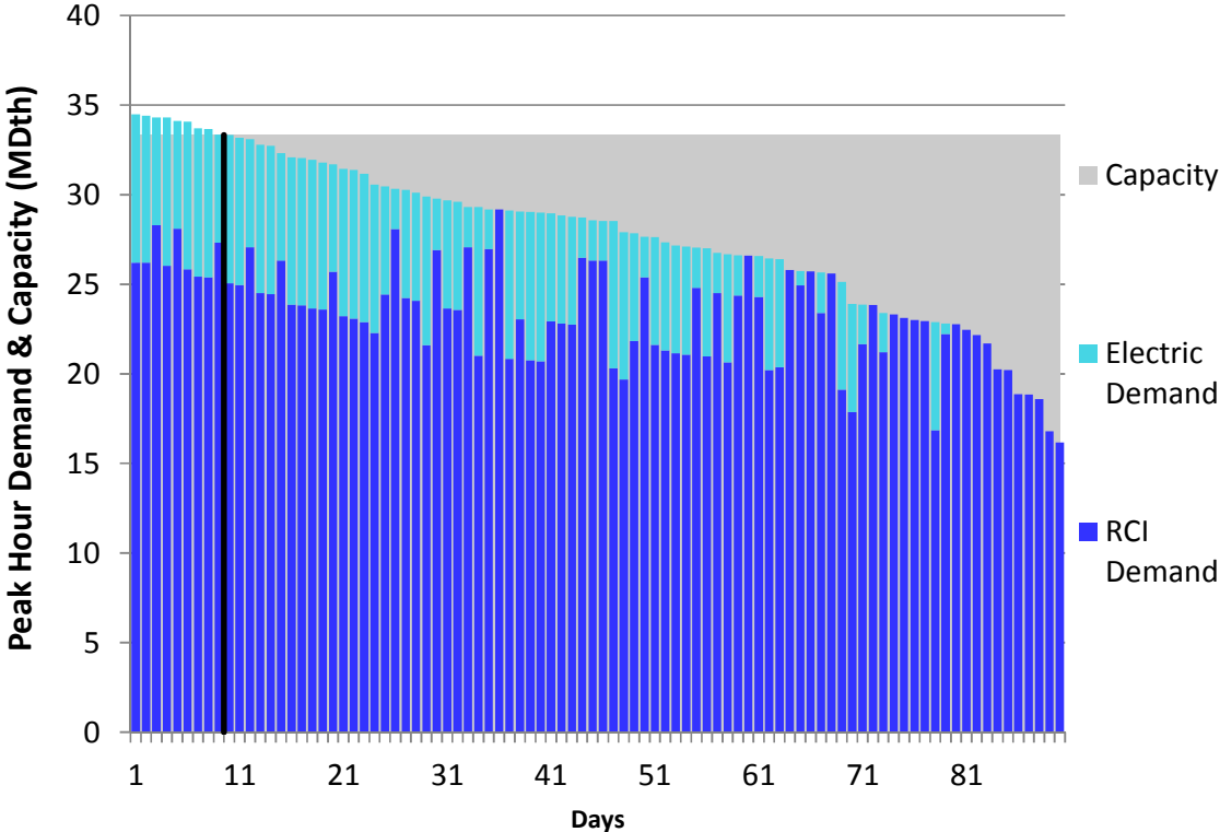
Figure L208. RGDS S16 Winter 2018 – East Tennessee – Descending Demand
