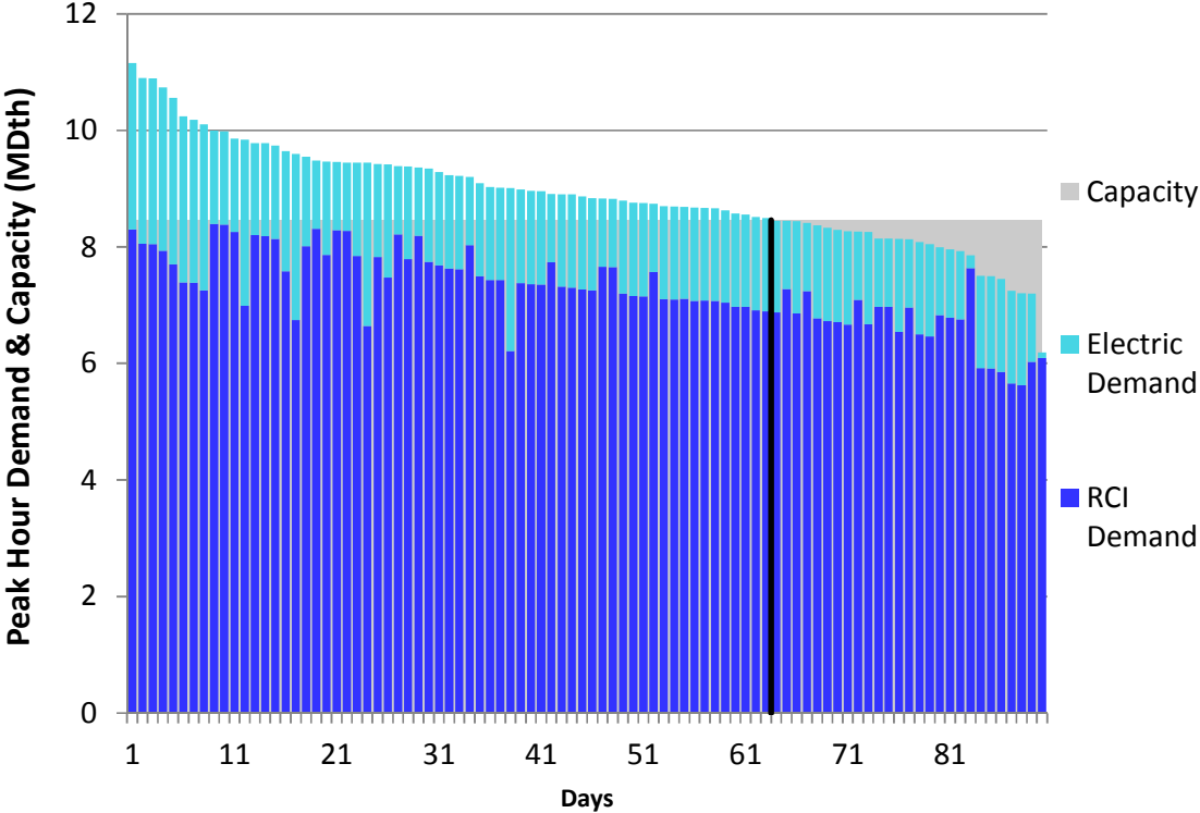
Figure L260. RGDS S16 Winter 2023 – Eastern Shore – Descending Demand
