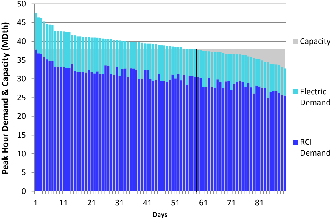
Figure L252. RGDS S16 Winter 2023 – Dominion Eastern NY– Descending Demand
