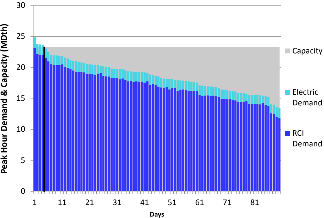
Figure L94. RGDS S14 Winter 2018 – Dominion Western NY– Descending Demand
