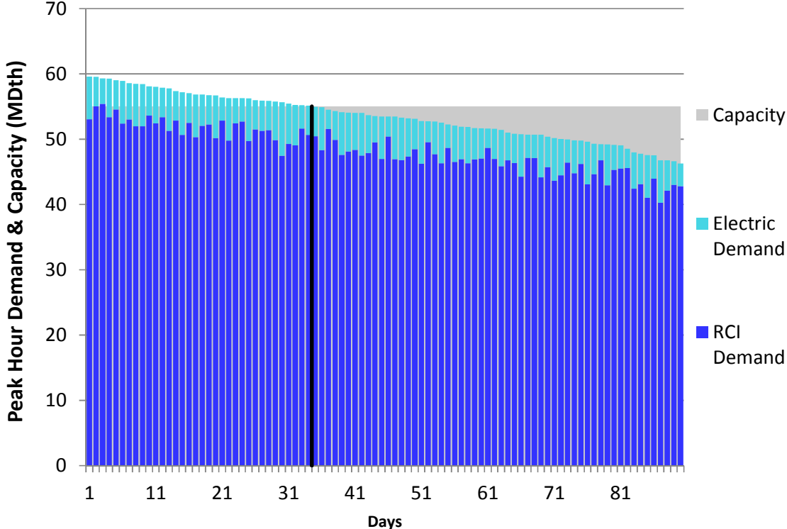
Figure L170. RGDS S14 Winter 2023 – TransCanada Quebec – Descending Demand
