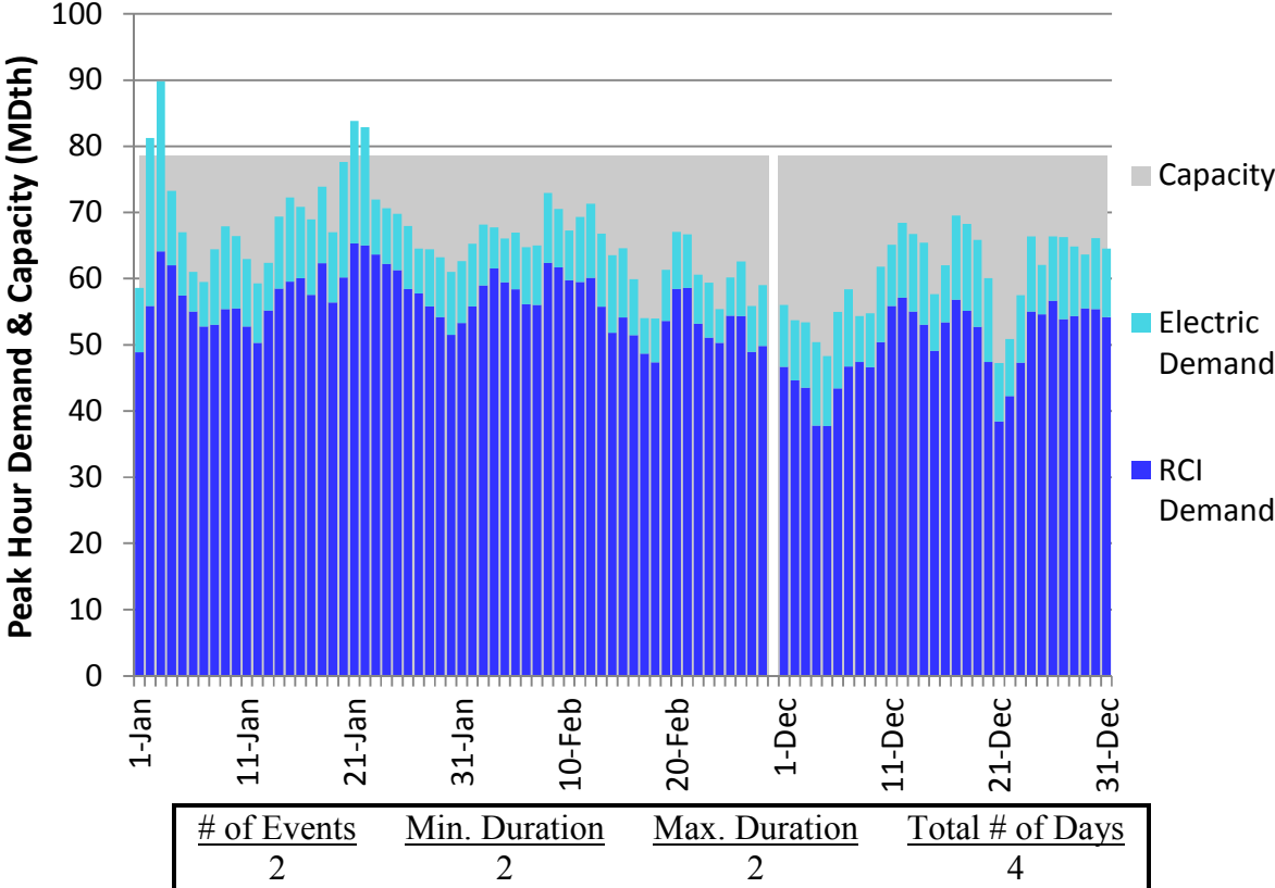
Figure L216. RGDS S16 Winter 2018 – Tennessee Z4 PA – Descending Demand
