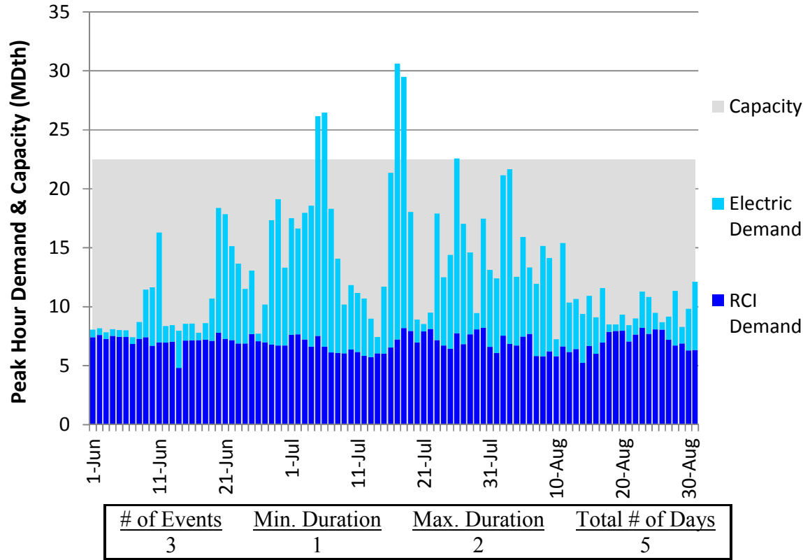
Figure L130. RGDS S14 Summer 2018 – Dominion Southeast – Descending Demand
