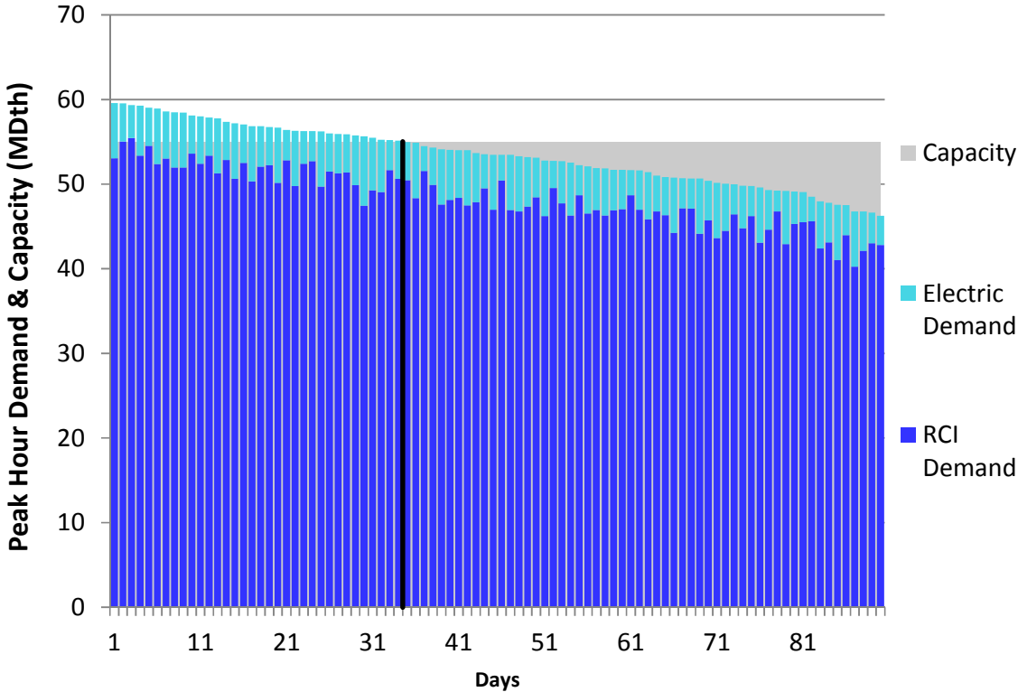
Figure L276. RGDS S16 Winter 2023 – TransCanada Quebec – Descending Demand
