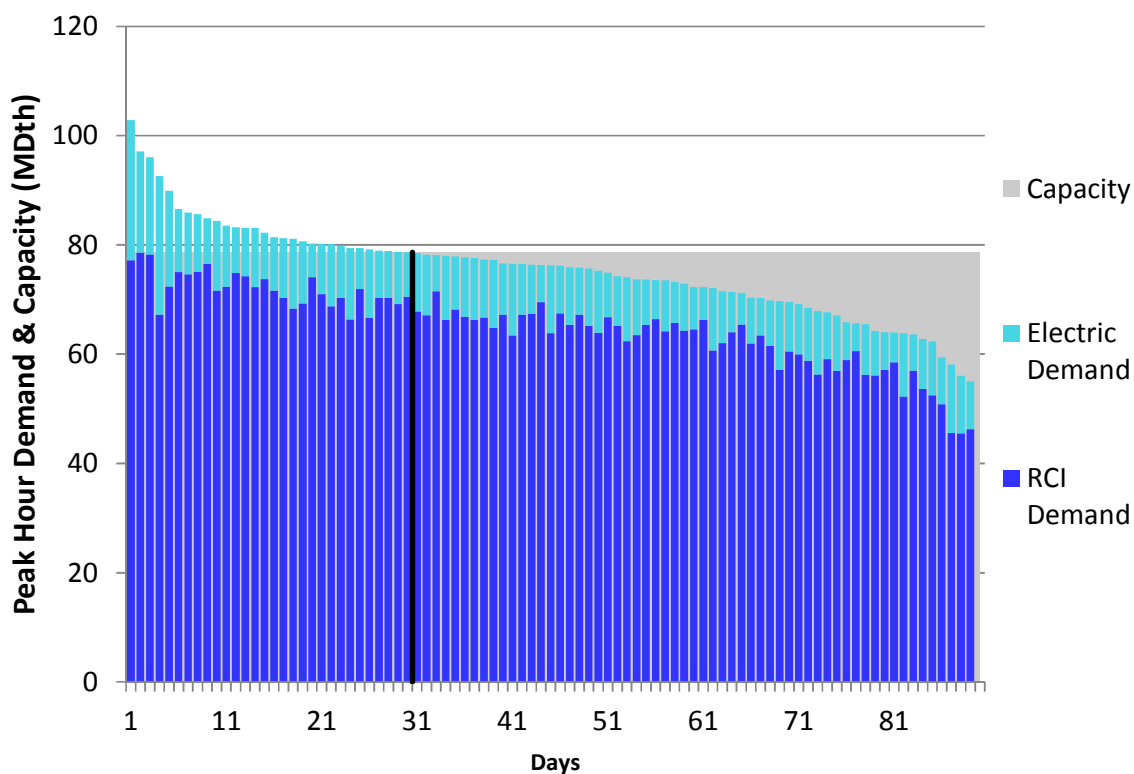
Figure L20. RGDS S13 Winter 2018 – Tennessee Z4 PA – Descending Demand
