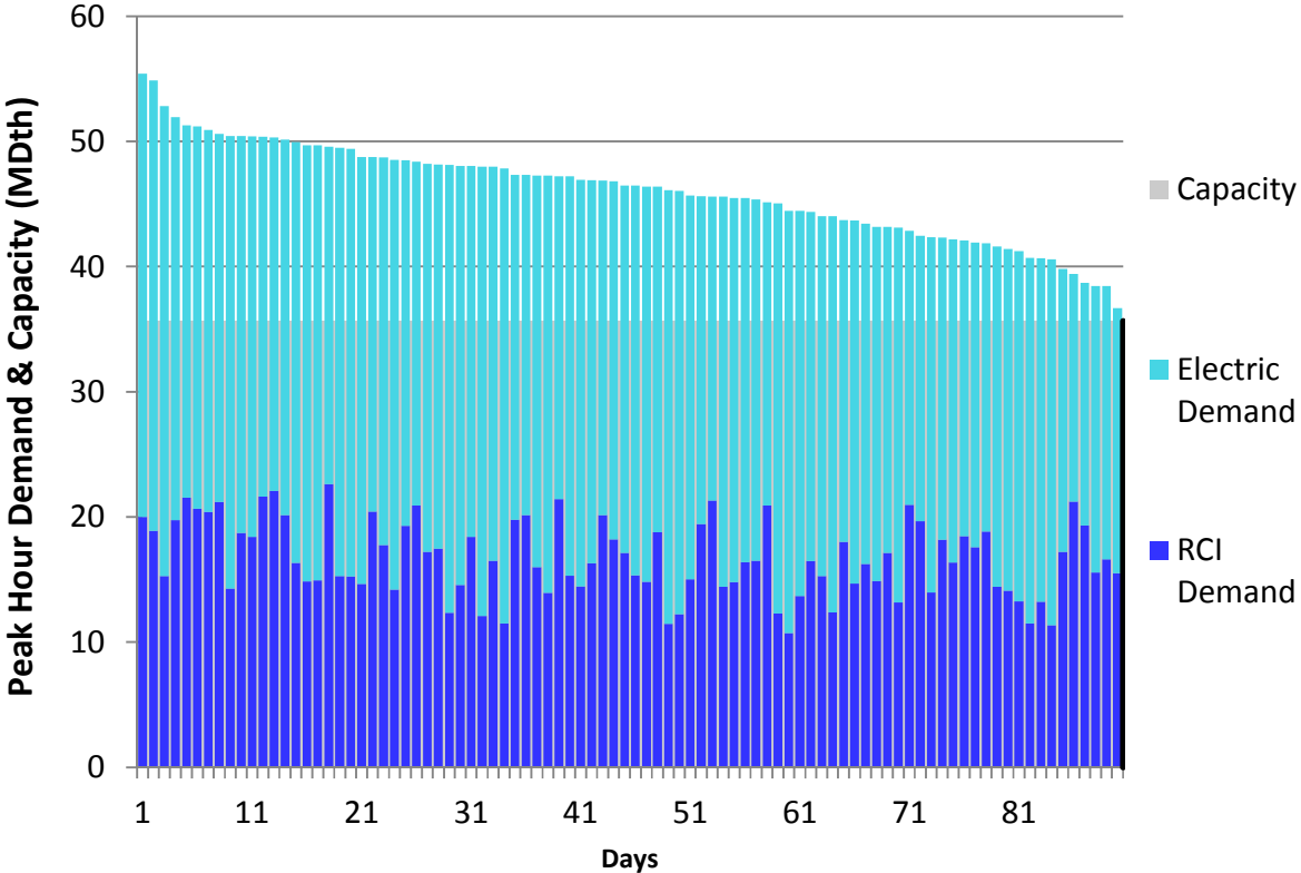
Figure L54. RGDS S13 Winter 2023 – Iroquois Z1 → Z2 – Descending Demand
