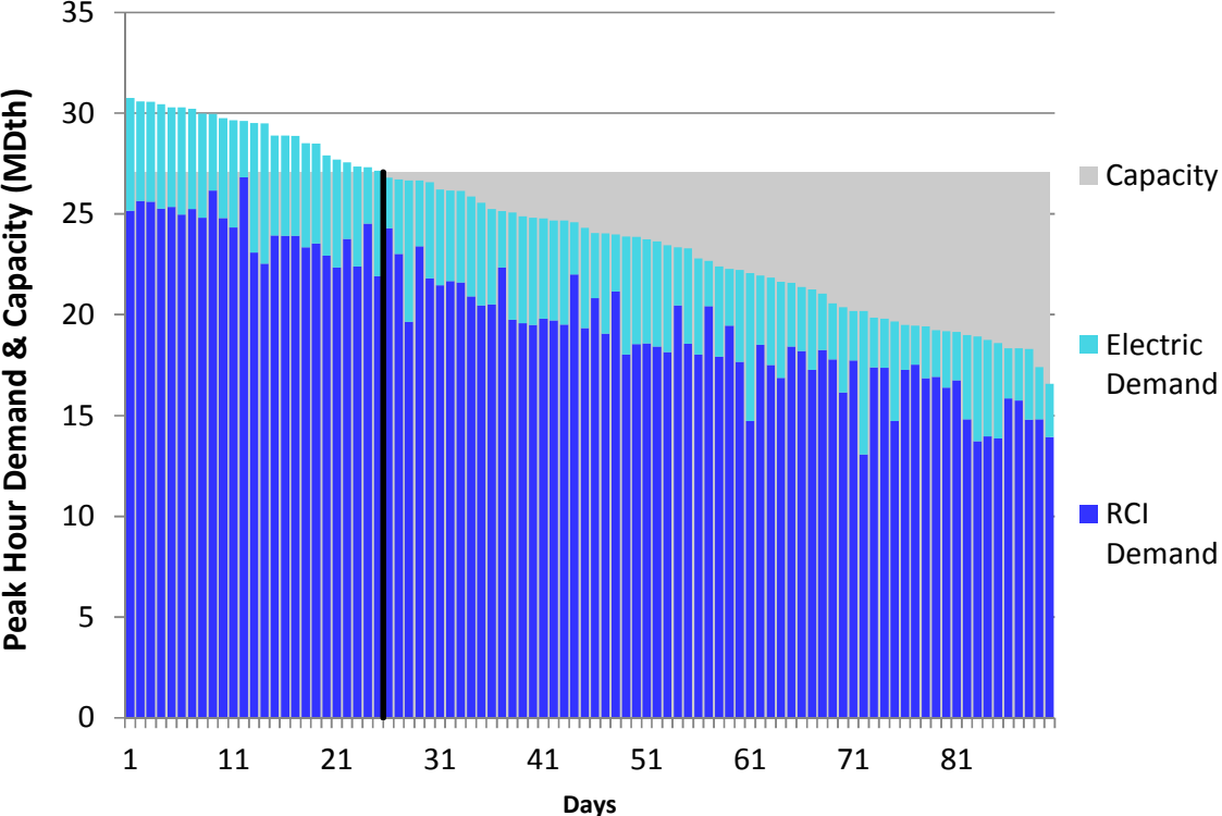
Figure L4. RGDS S13 Winter 2018 – Constitution – Descending Demand
