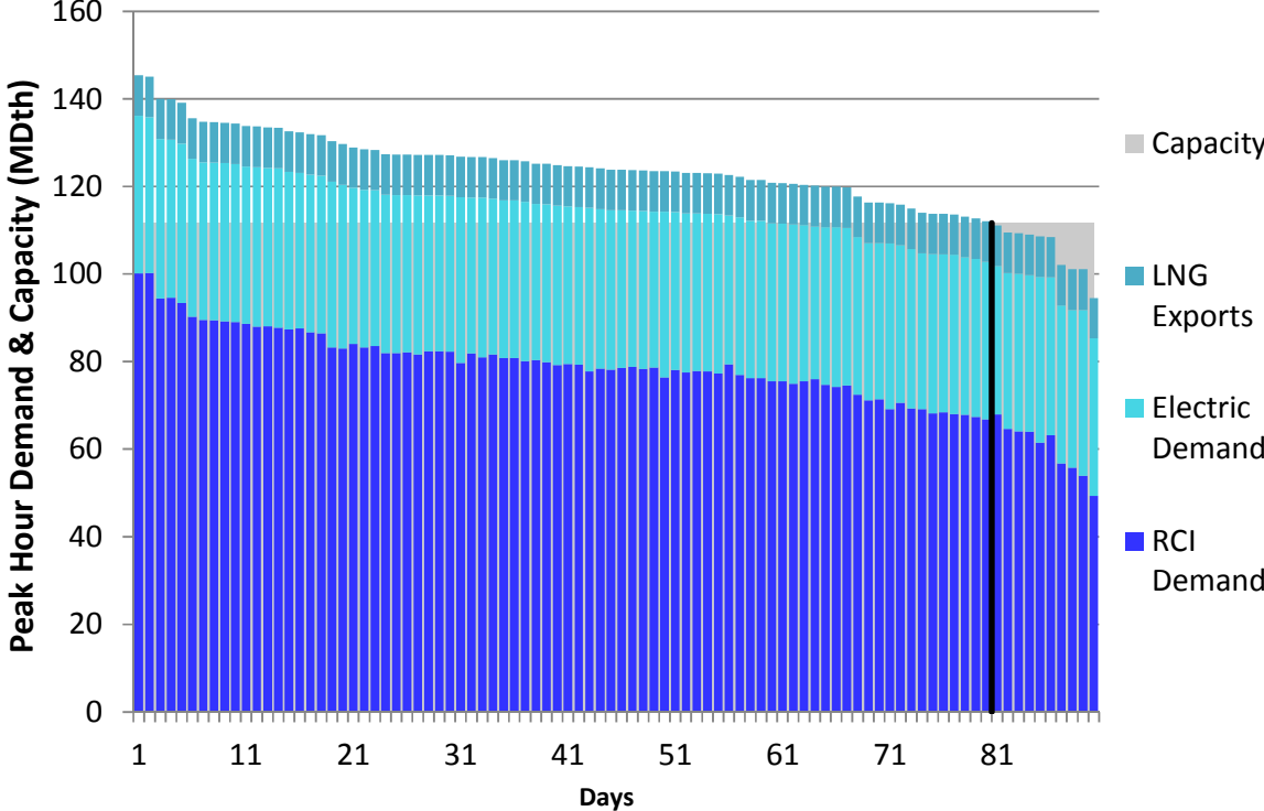
Figure L138. RGDS S14 Winter 2023 – Columbia Gas VA/MD – Descending Demand
