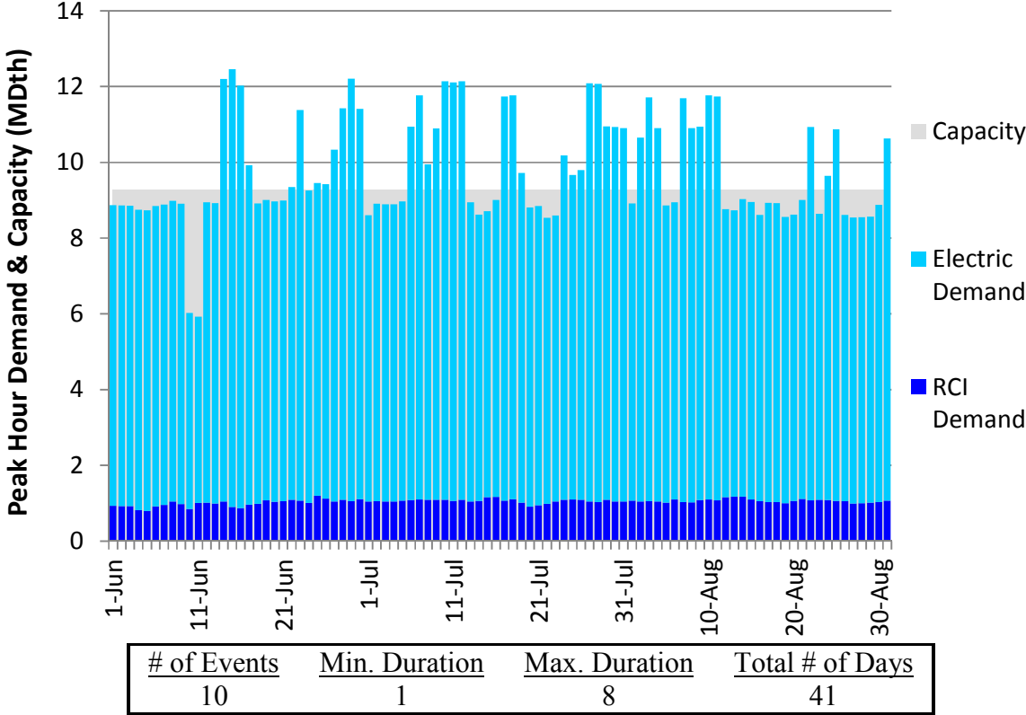
Figure L190. RGDS S14 Summer 2023 – PNGTS N of Westbrook – Descending Demand
