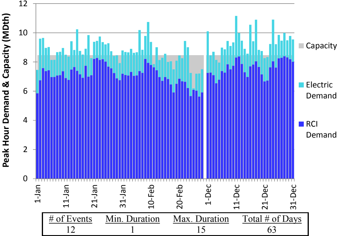
Figure L52. RGDS S13 Winter 2023 – Eastern Shore – Descending Demand
