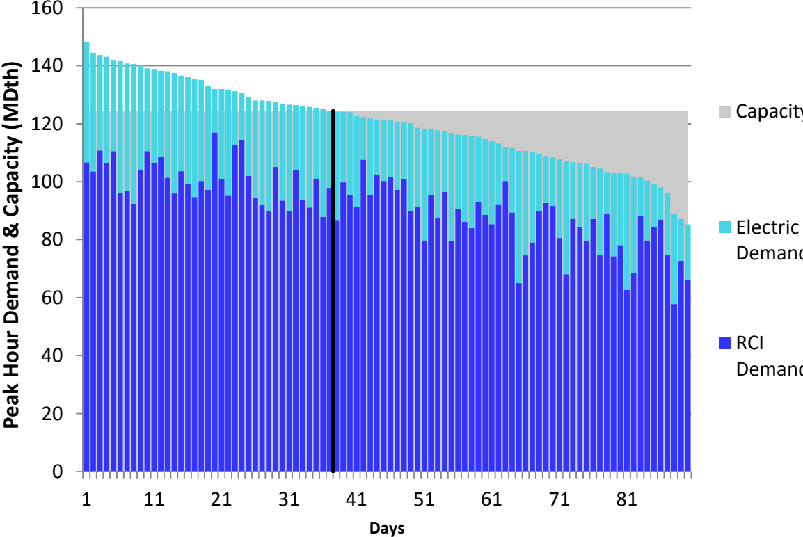
Figure L272. RGDS S16 Winter 2023 – Texas Eastern M3 North – Descending Demand
