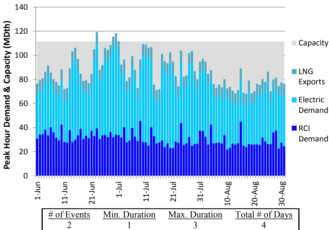
Figure L286. RGDS S16 Summer 2023 – Columbia Gas VA/MD – Descending Demand
