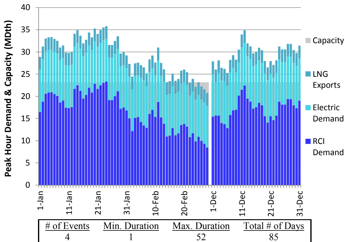
Figure L147. RGDS S14 Winter 2023 – Dominion Southeast – Chronological Demand
