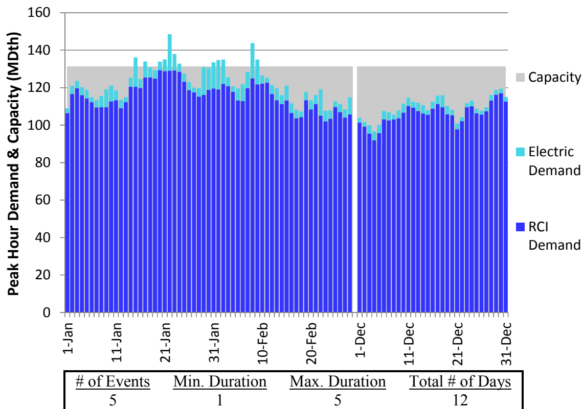
Figure L116. RGDS S14 Winter 2018 – TransCanada Ontario West – Descending Demand
