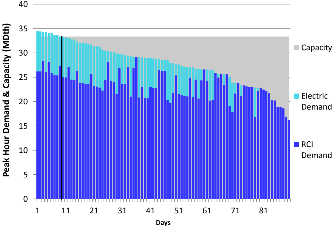
Figure L8. RGDS S13 Winter 2018 – East Tennessee – Descending Demand
