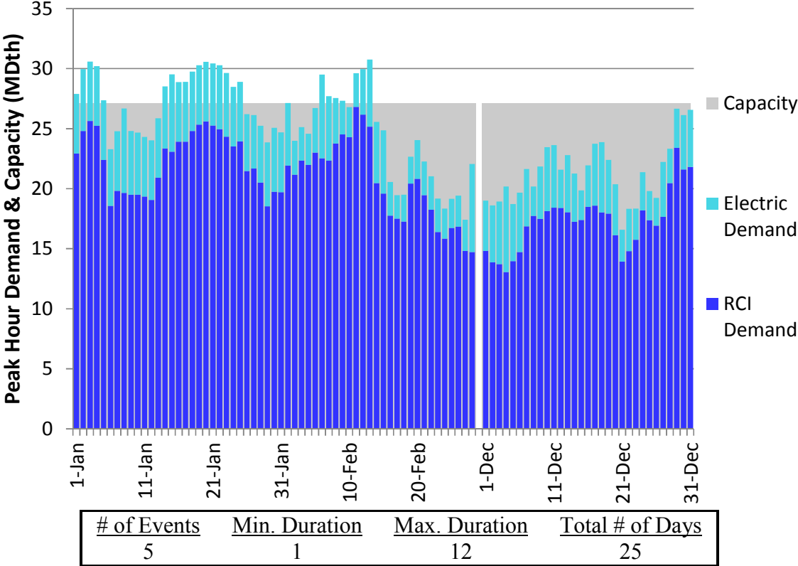
Figure L90. RGDS S14 Winter 2018 – Constitution – Descending Demand
