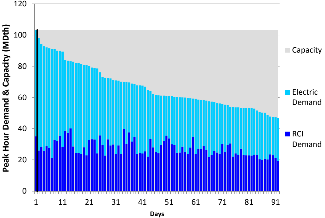
Figure L236. RGDS S16 Summer 2018 – Columbia Gas VA/MD – Descending Demand
