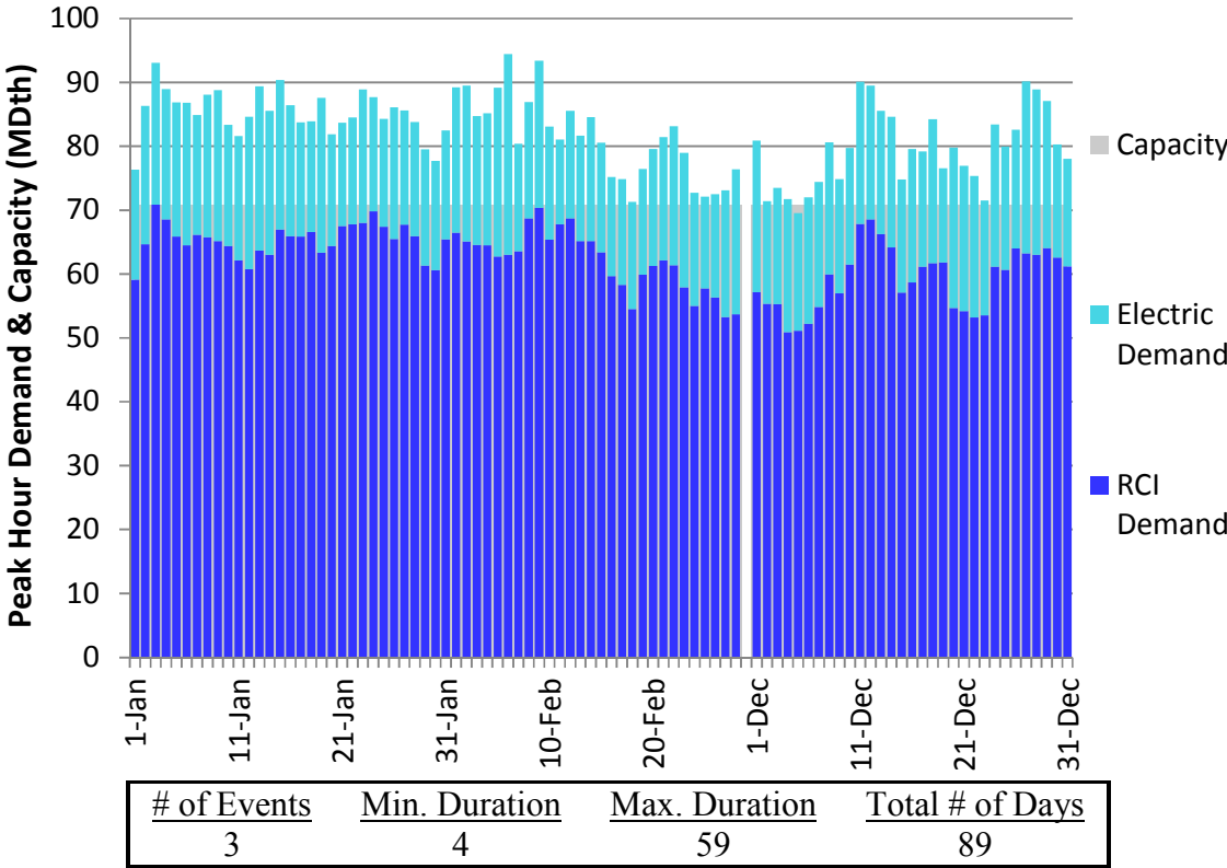
Figure L278. RGDS S16 Winter 2023 – Transco Leidy Atlantic – Descending Demand
