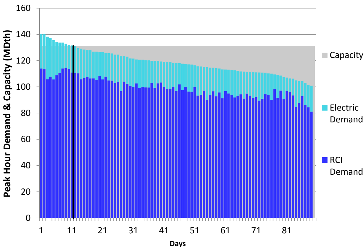
Figure L66. RGDS S13 Winter 2023 – TransCanada Ontario West – Descending Demand
