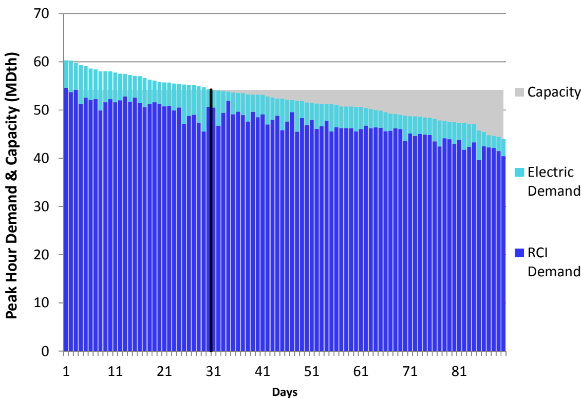
Figure L118. RGDS S14 Winter 2018 – TransCanada Quebec – Descending Demand
