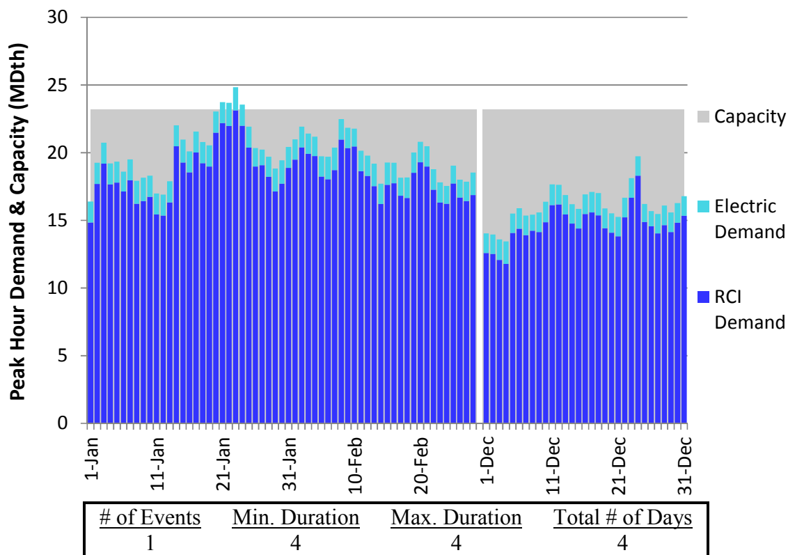
Figure L204. RGDS S16 Winter 2018 – Dominion Western NY– Descending Demand
