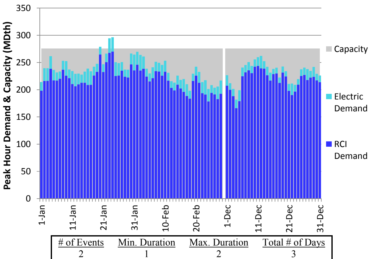
Figure L74. RGDS S13 Winter 2023 – Union Gas Dawn – Descending Demand
