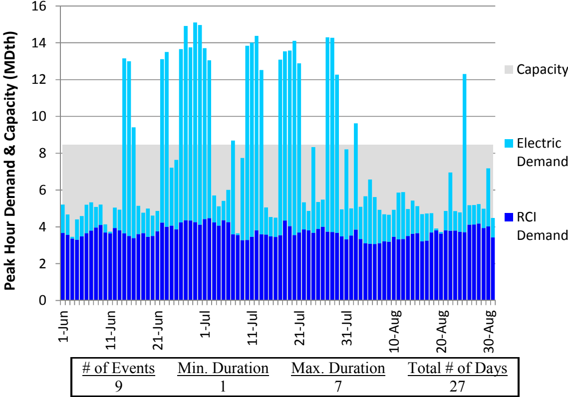
Figure L80. RGDS S13 Summer 2023 – Eastern Shore – Descending Demand
