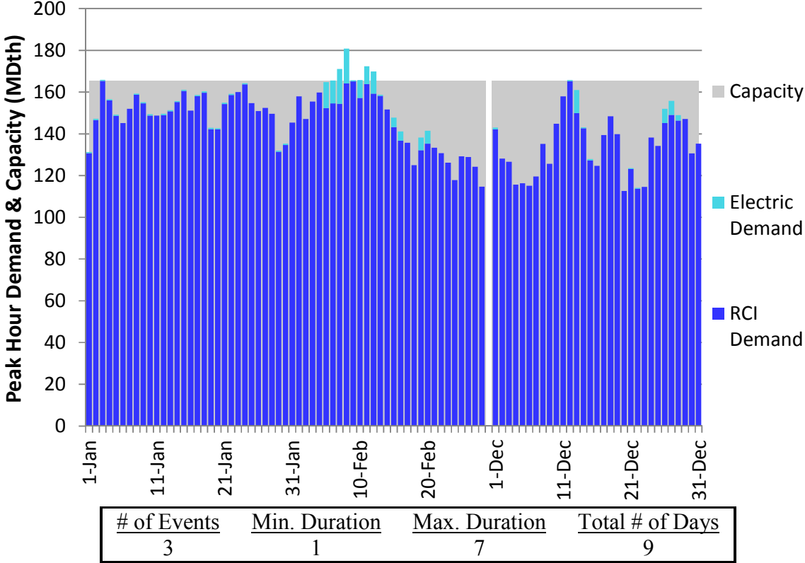
Figure L230. RGDS S16 Winter 2018 – Transco Z5 – Descending Demand
