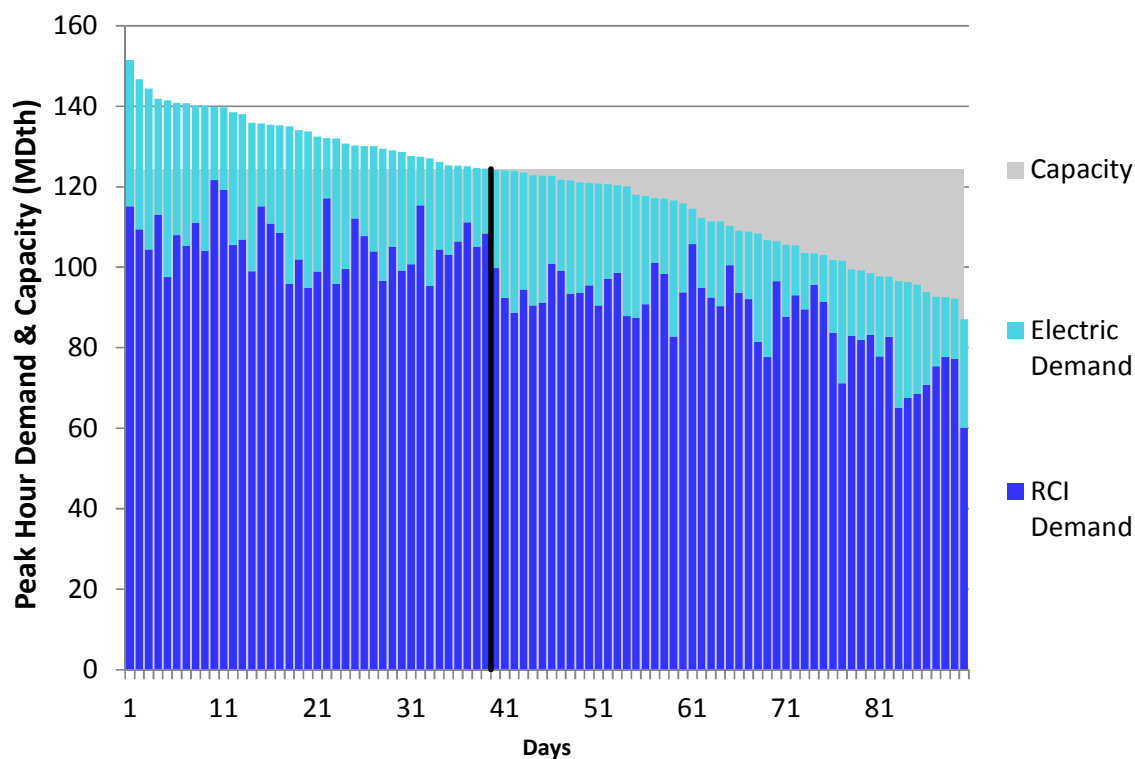
Figure L26. RGDS S13 Winter 2018 – Texas Eastern M3 North – Descending Demand
