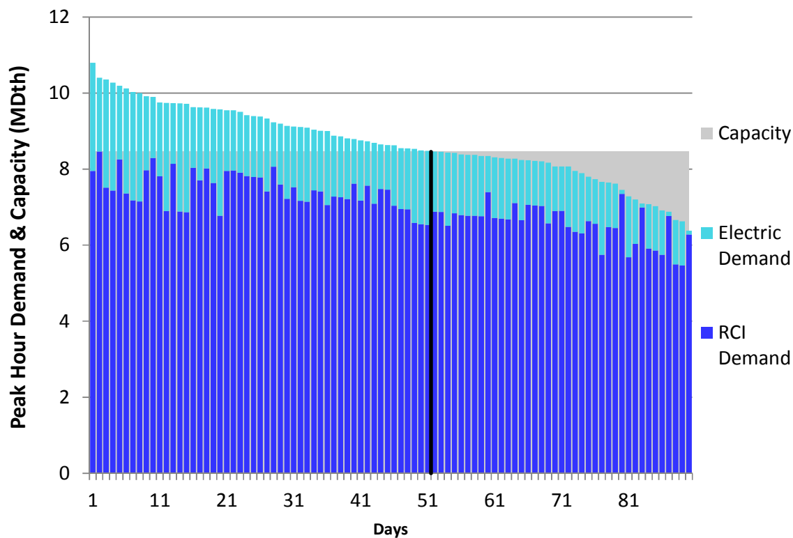
Figure L10. RGDS S13 Winter 2018 – Eastern Shore – Descending Demand
