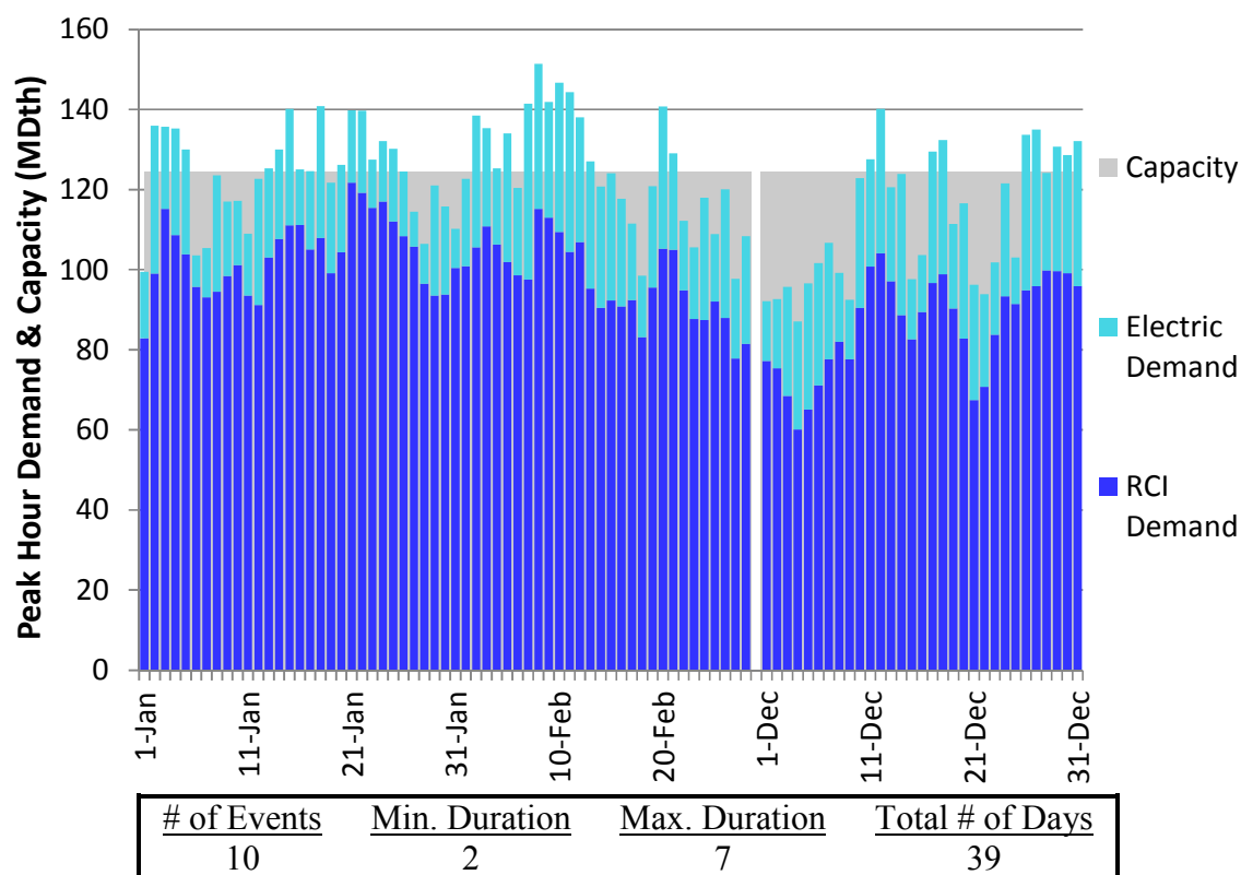
Figure L114. RGDS S14 Winter 2018 – Texas Eastern M3 North – Descending Demand
