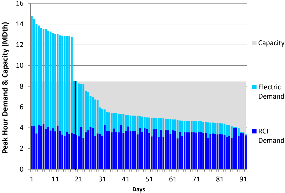
Figure L132. RGDS S14 Summer 2018 – Eastern Shore – Descending Demand
