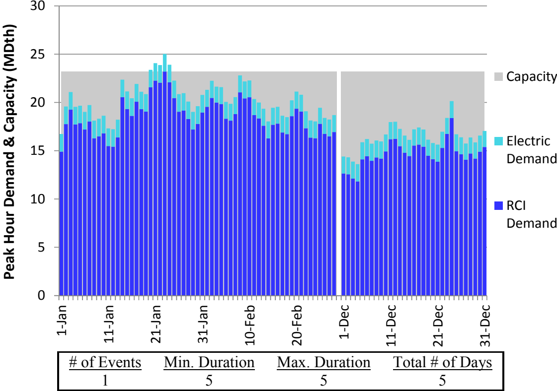
Figure L254. RGDS S16 Winter 2023 – Dominion Western NY– Descending Demand
