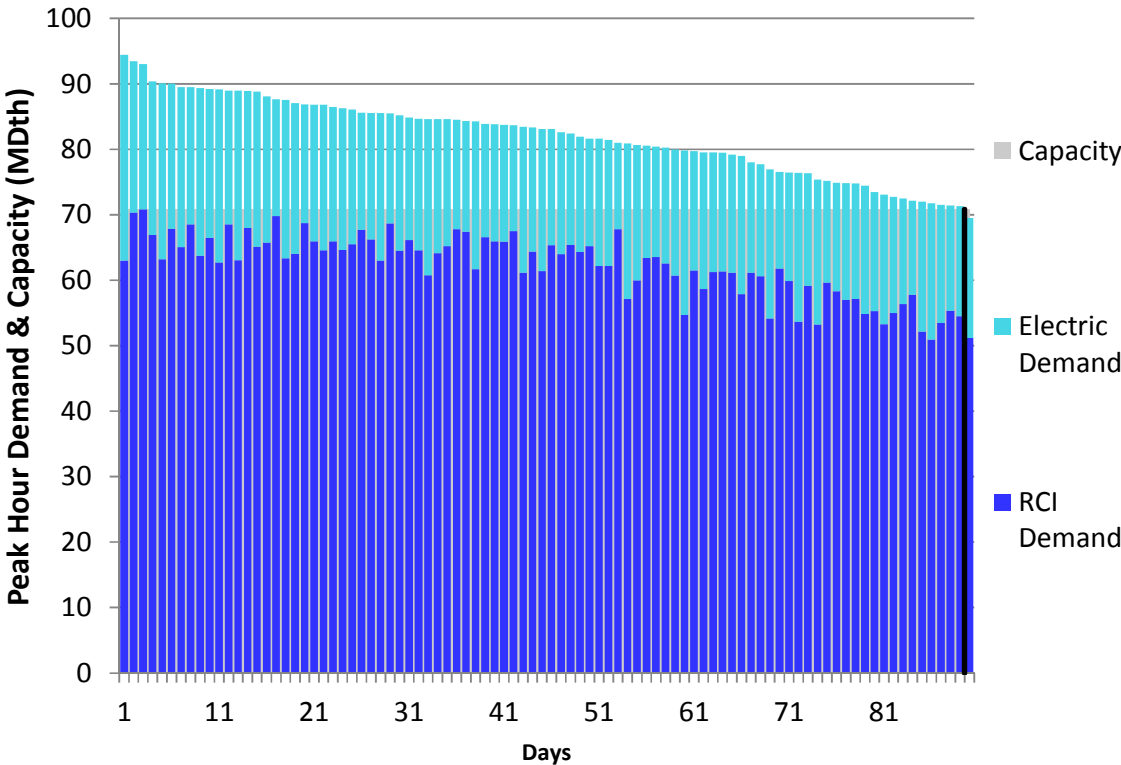
Figure L278. RGDS S16 Winter 2023 – Transco Leidy Atlantic – Descending Demand
