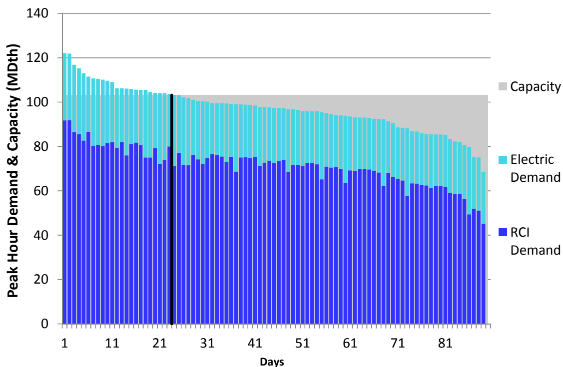
Figure L2. RGDS S13 Winter 2018 – Columbia Gas VA/MD – Descending Demand
