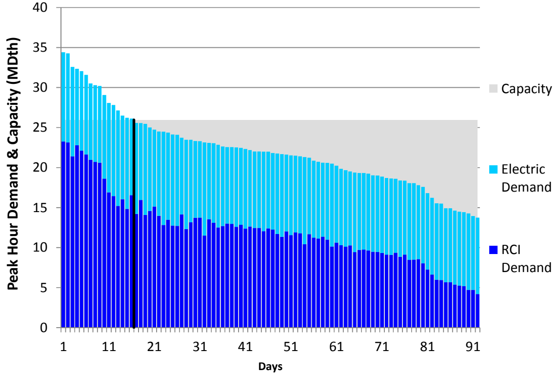
Figure L292. RGDS S16 Summer 2023 – Texas Eastern ETX – Descending Demand
