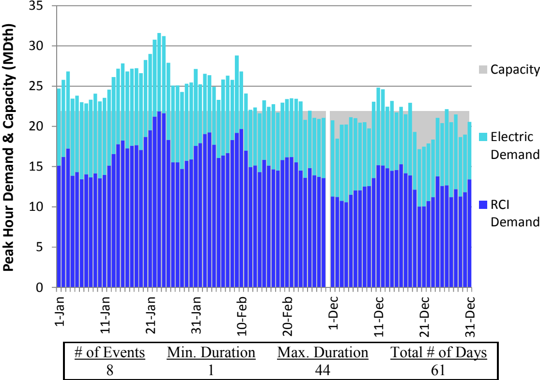
Figure L262. RGDS S16 Winter 2023 – Empire – Descending Demand
