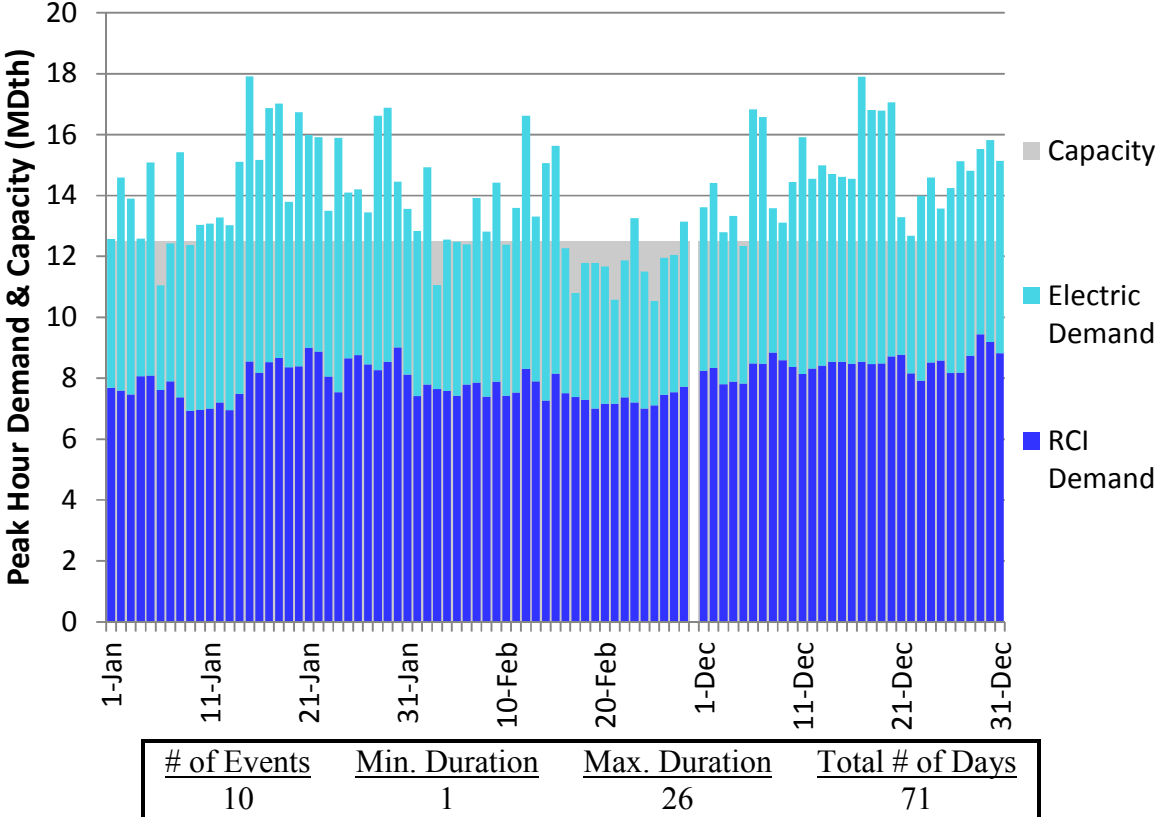
Figure L18. RGDS S13 Winter 2018 – PNGTS N of Westbrook – Descending Demand
