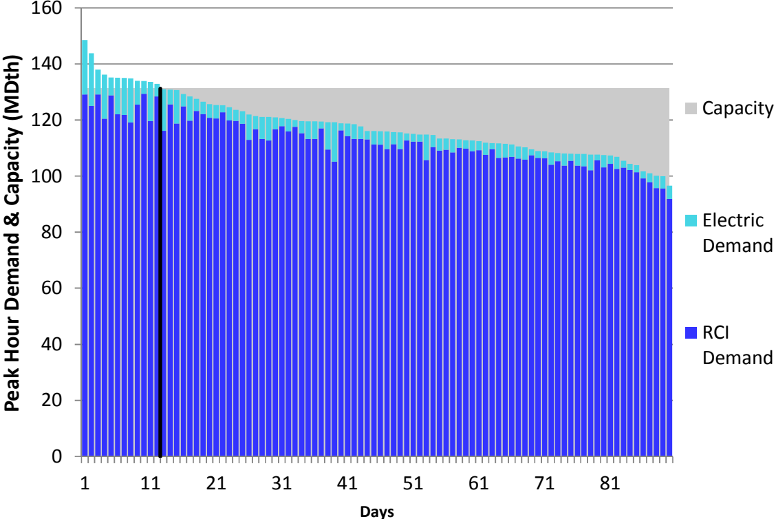
Figure L224. RGDS S16 Winter 2018 – TransCanada Ontario West – Descending Demand
