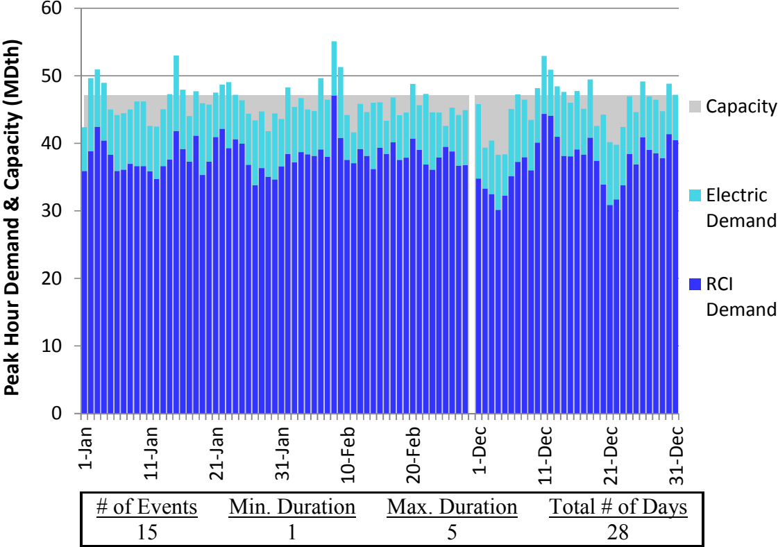
Figure L248. RGDS S16 Winter 2023 – Columbia Gas W PA/NY – Descending Demand
