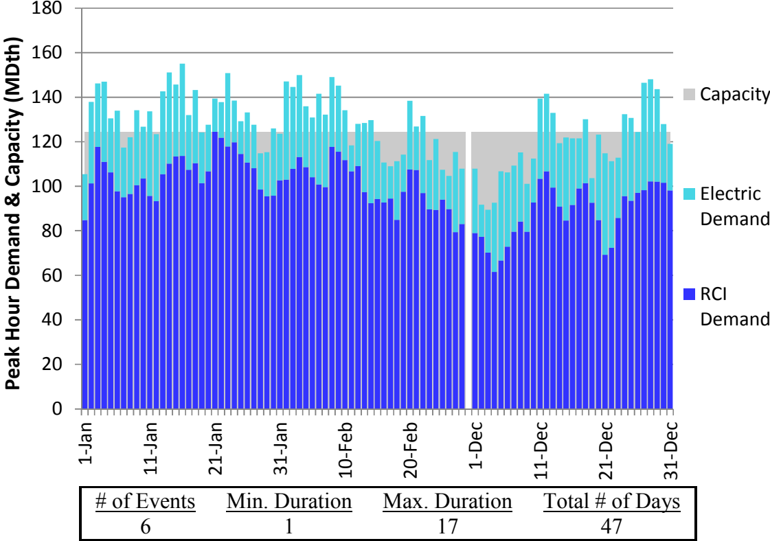
Figure L64. RGDS S13 Winter 2023 – Texas Eastern M3 North – Descending Demand
