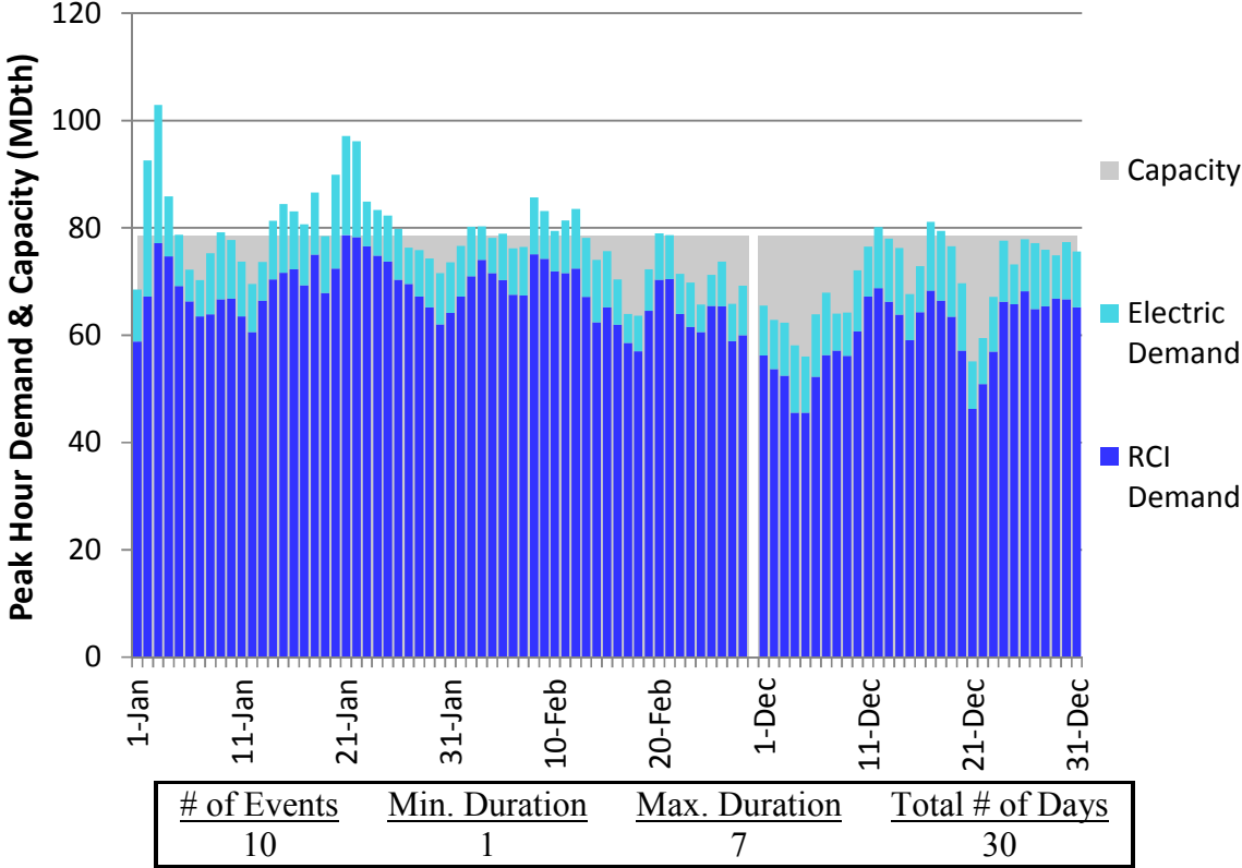
Figure L108. RGDS S14 Winter 2018 – Tennessee Z4 PA – Descending Demand
