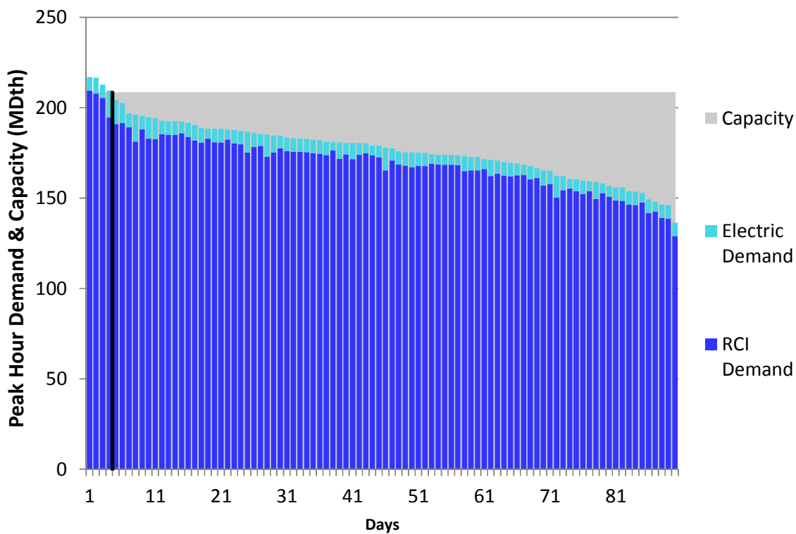
Figure L126. RGDS S14 Winter 2018 – Union Gas Dawn – Descending Demand
