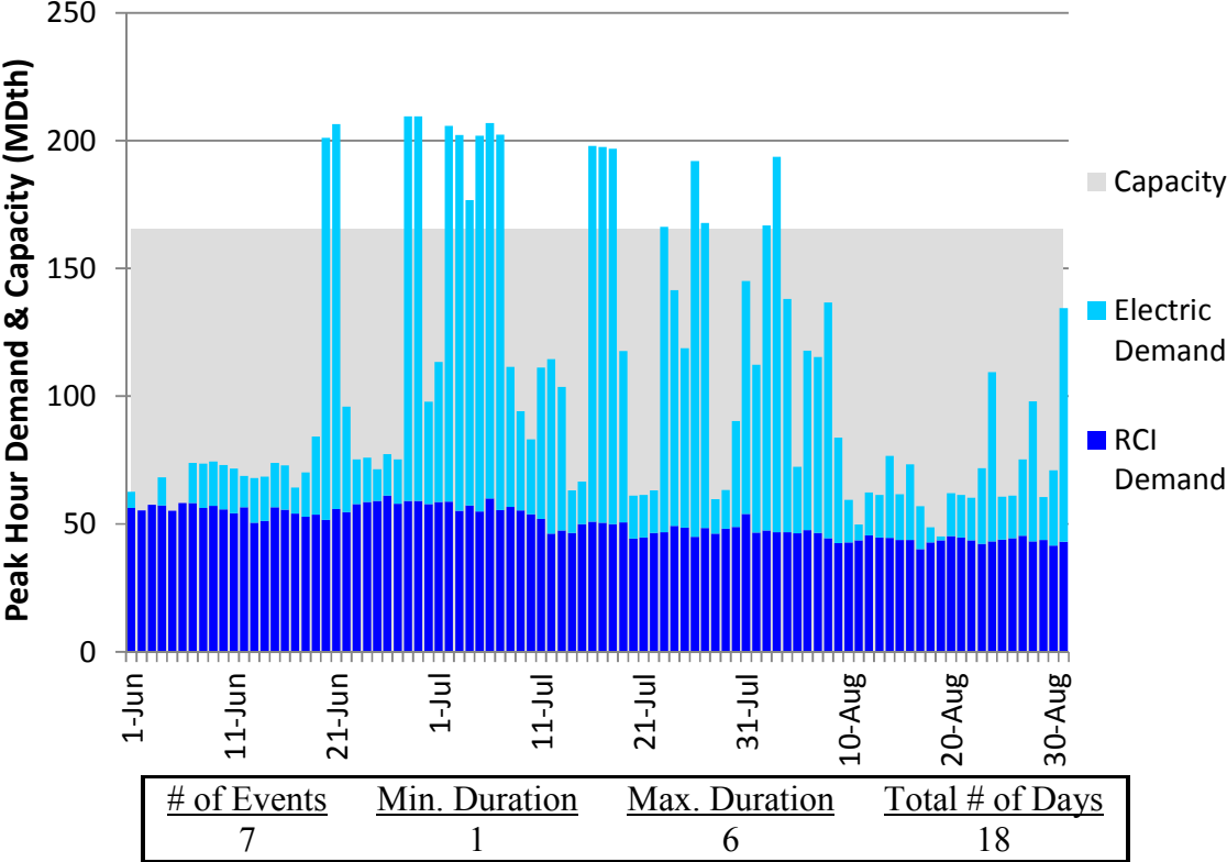
Figure J52. RGDS S5a Summer 2018 – Transco Z5 – Descending Demand
