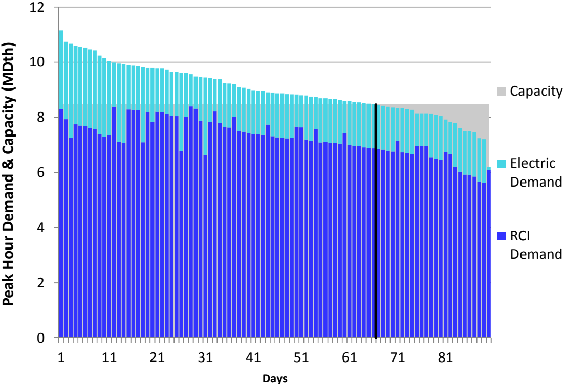
Figure J236. RGDS S5c Winter 2023 – Eastern Shore – Descending Demand
