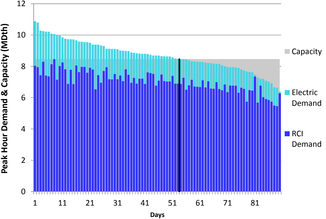
Figure J16. RGDS S5a Winter 2018 – Eastern Shore – Descending Demand
