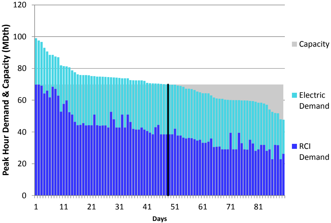
Figure J312. HGDS S9 Winter 2018 – NGPL IA/IL South – Descending Demand
