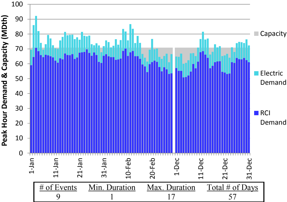
Figure J36. RGDS S5a Winter 2018 – Transco Leidy Atlantic – Descending Demand
