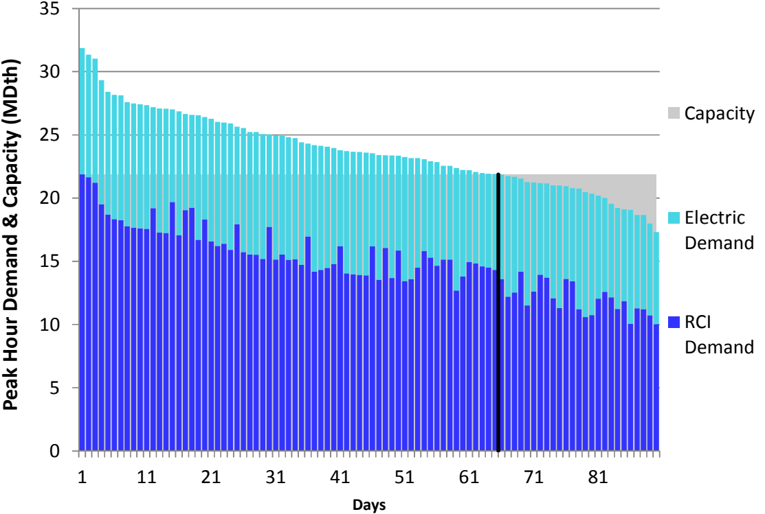
Figure J128. RGDS S5b Winter 23 – Empire – Descending Demand
