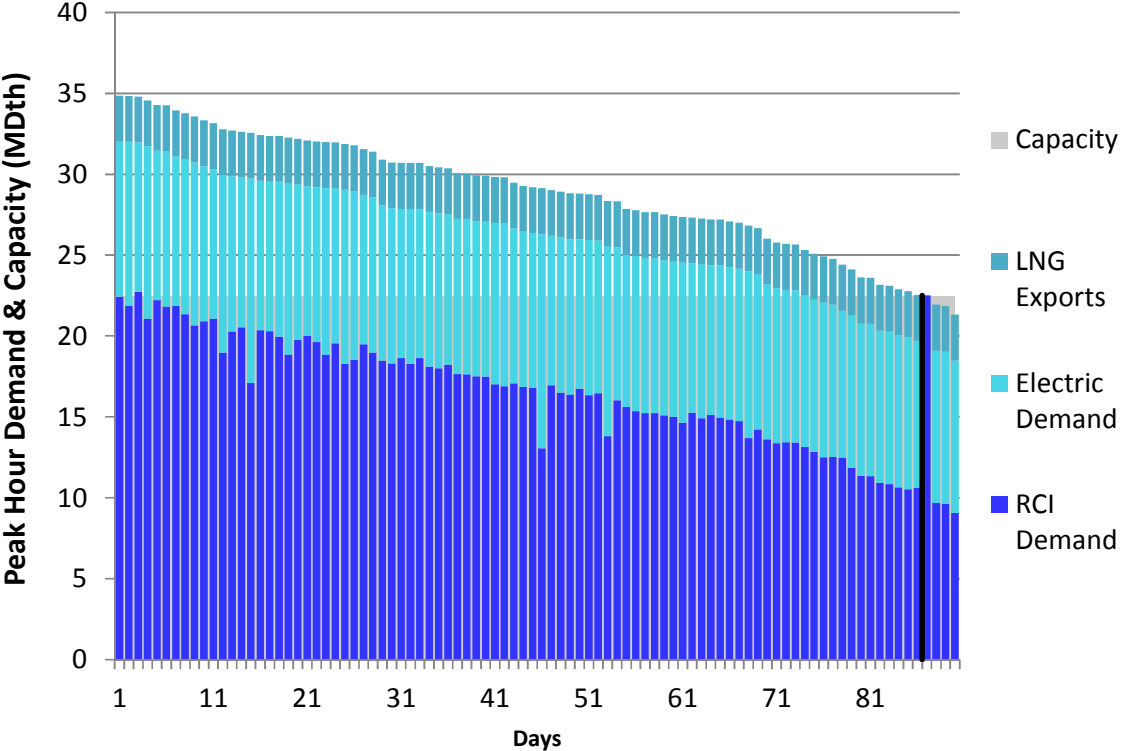
Figure J370. HGDS S0 Winter 2023 – Dominion Southeast – Descending Demand
