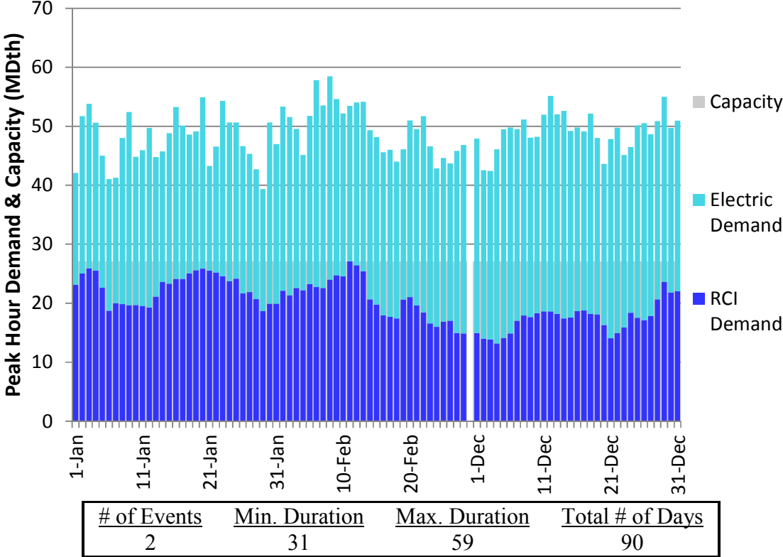
Figure J226. RGDS S5c Winter 23 – Constitution – Descending Demand
