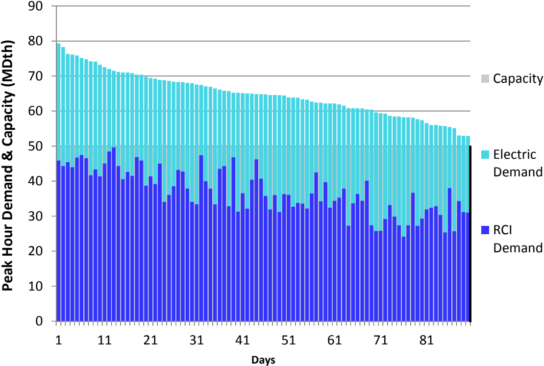
Figure J380. HGDS S0 Winter 2018 – Iroquois Zone 1 – Descending Demand
