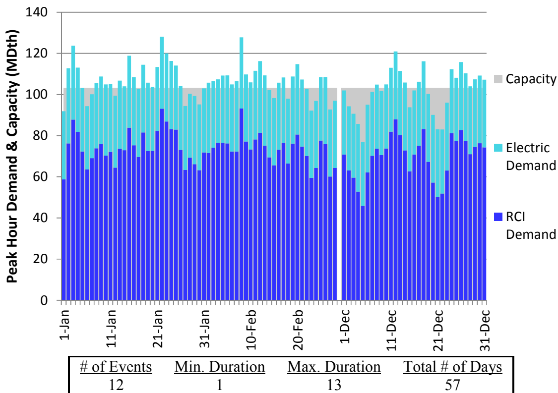
Figure J284. HGDS S9 Winter 2018 – Columbia Gas VA/MD – Descending Demand
