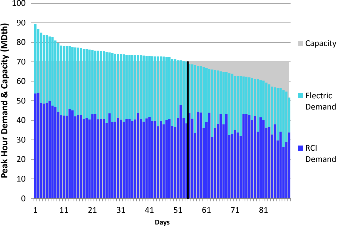
Figure J388. HGDS S0 Winter 2023 – NGPL IA/IL North – Descending Demand
