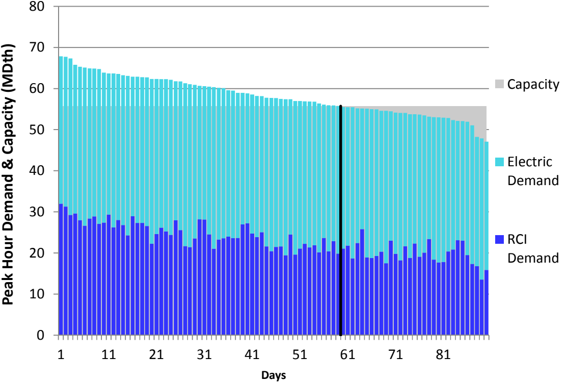
Figure J282. HGDS S9 Winter 2018 – ANR Northern IL – Descending Demand
