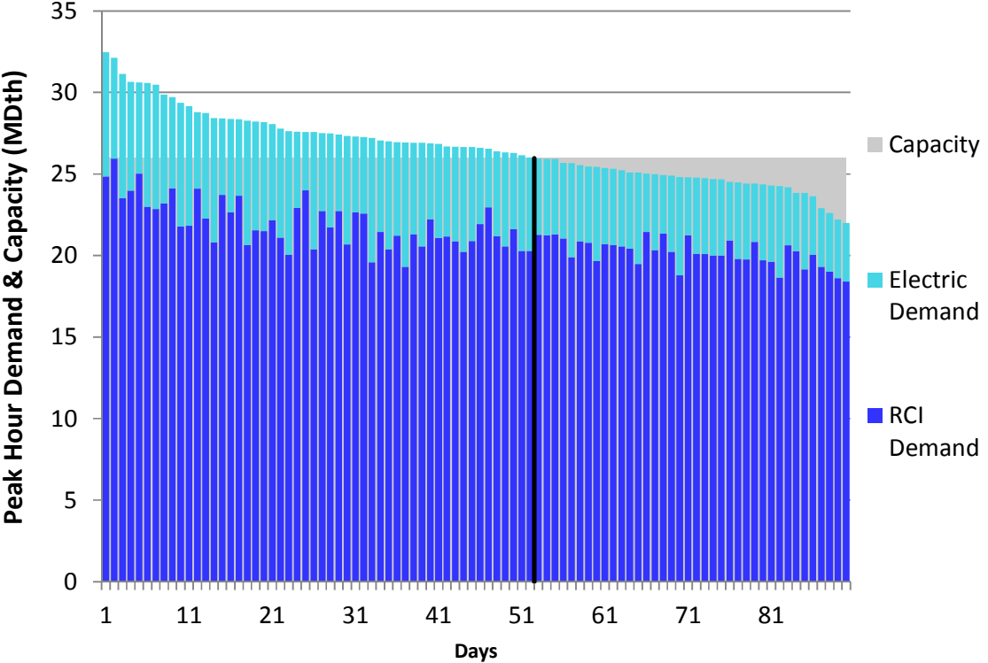
Figure J22. RGDS S5a Winter 2018 – NB/NS – Descending Demand
