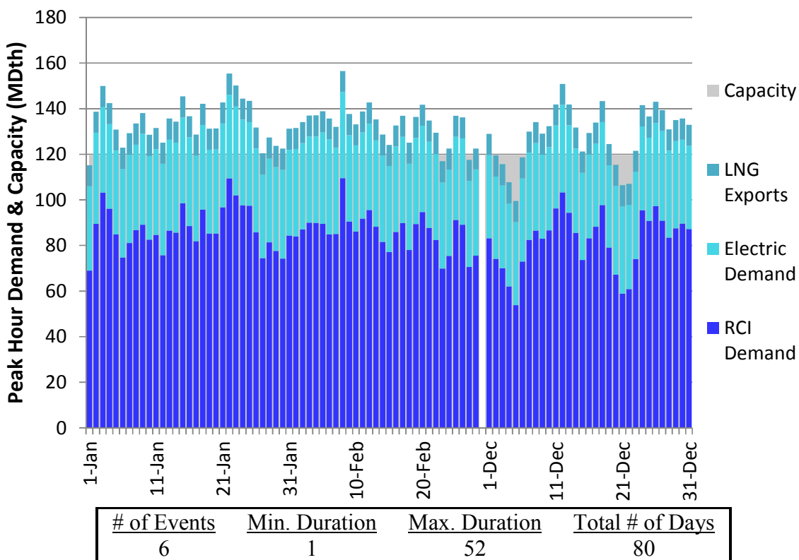
Figure J360. HGDS S0 Winter 2023 – Columbia Gas VA/MD – Descending Demand
