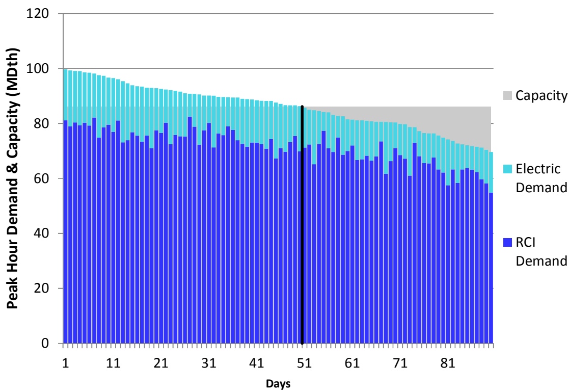
Figure J28. RGDS S5a Winter 2018 – Texas Eastern M2 PA South – Descending Demand
