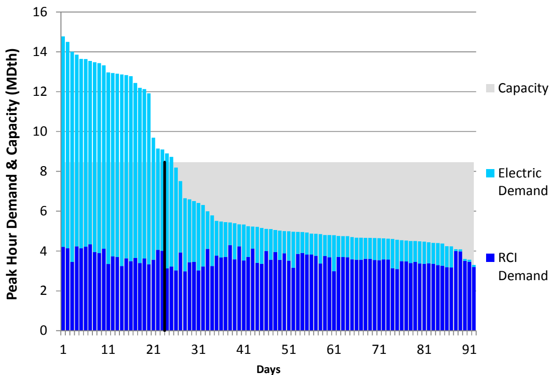
Figure J216. RGDS S5c Summer 2018 – Eastern Shore – Descending Demand
