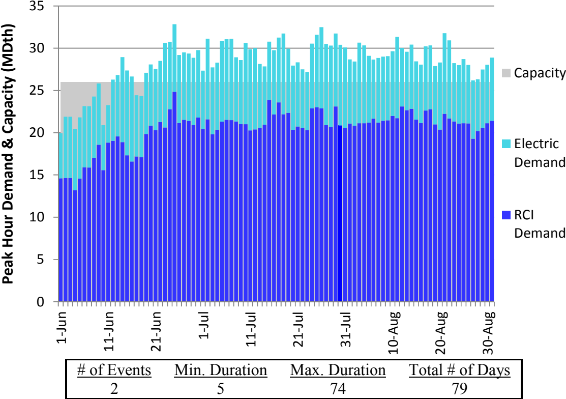
Figure J348. HGDS S9 Summer 2018 – NB/NS Supply – Descending Demand
