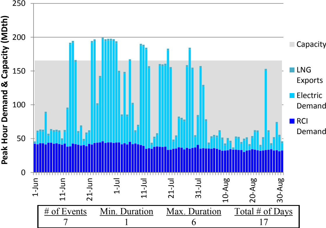
Figure J110. RGDS S5a Summer 2023 – Transco Z5 – Descending Demand
