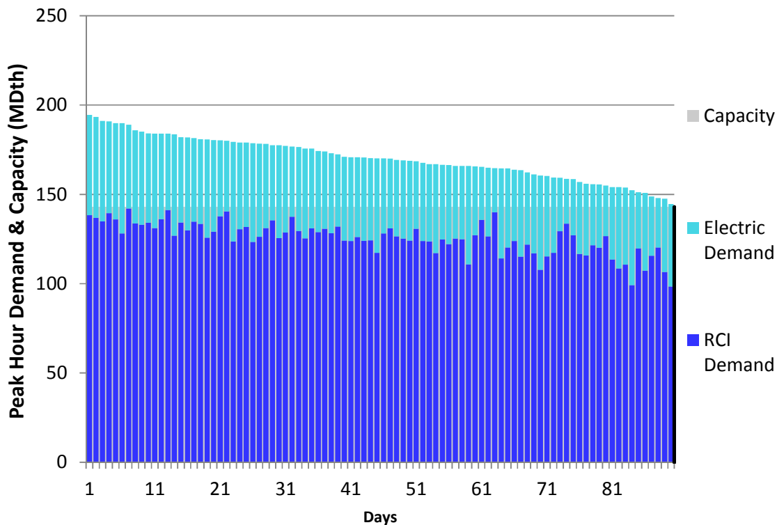
Figure J334. HGDS S9 Winter 2018 – Transco Leidy to Station 210 – Descending Demand
