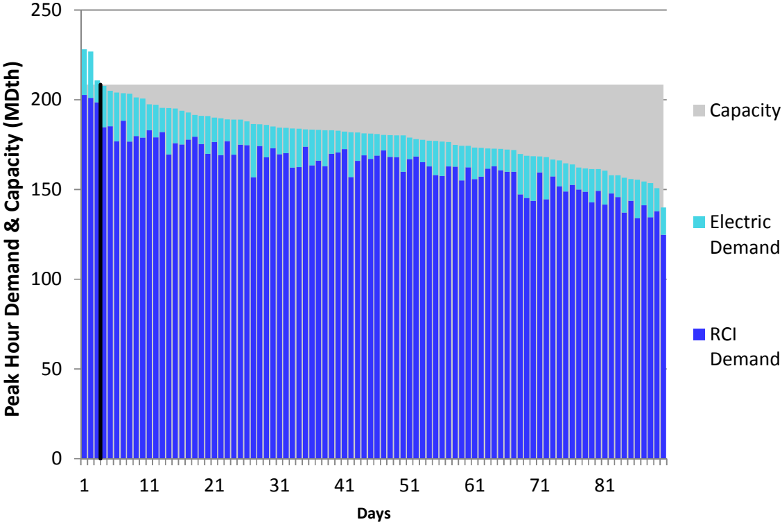
Figure J94. RGDS S5a Winter 2023 – Union Gas Dawn – Descending Demand
