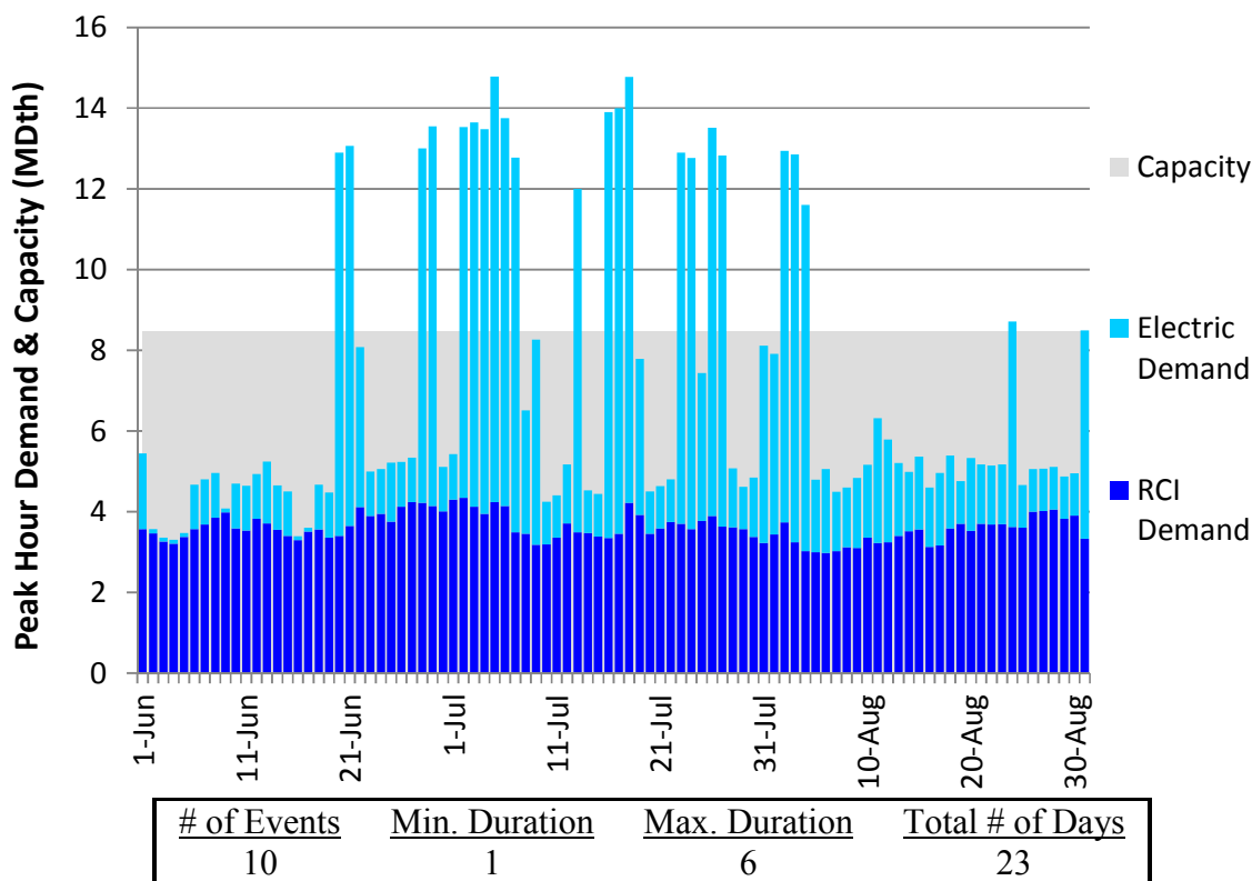
Figure J216. RGDS S5c Summer 2018 – Eastern Shore – Descending Demand
