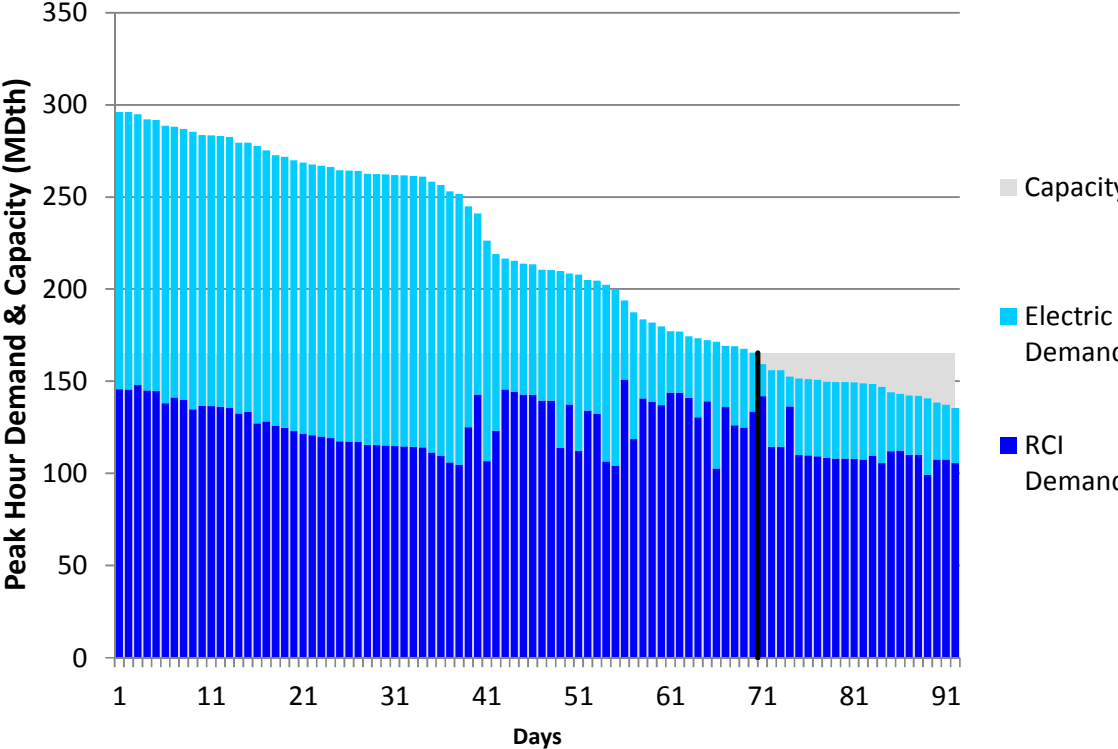
Figure J354. HGDS S9 Summer 2018 – Transco Z5 – Descending Demand
