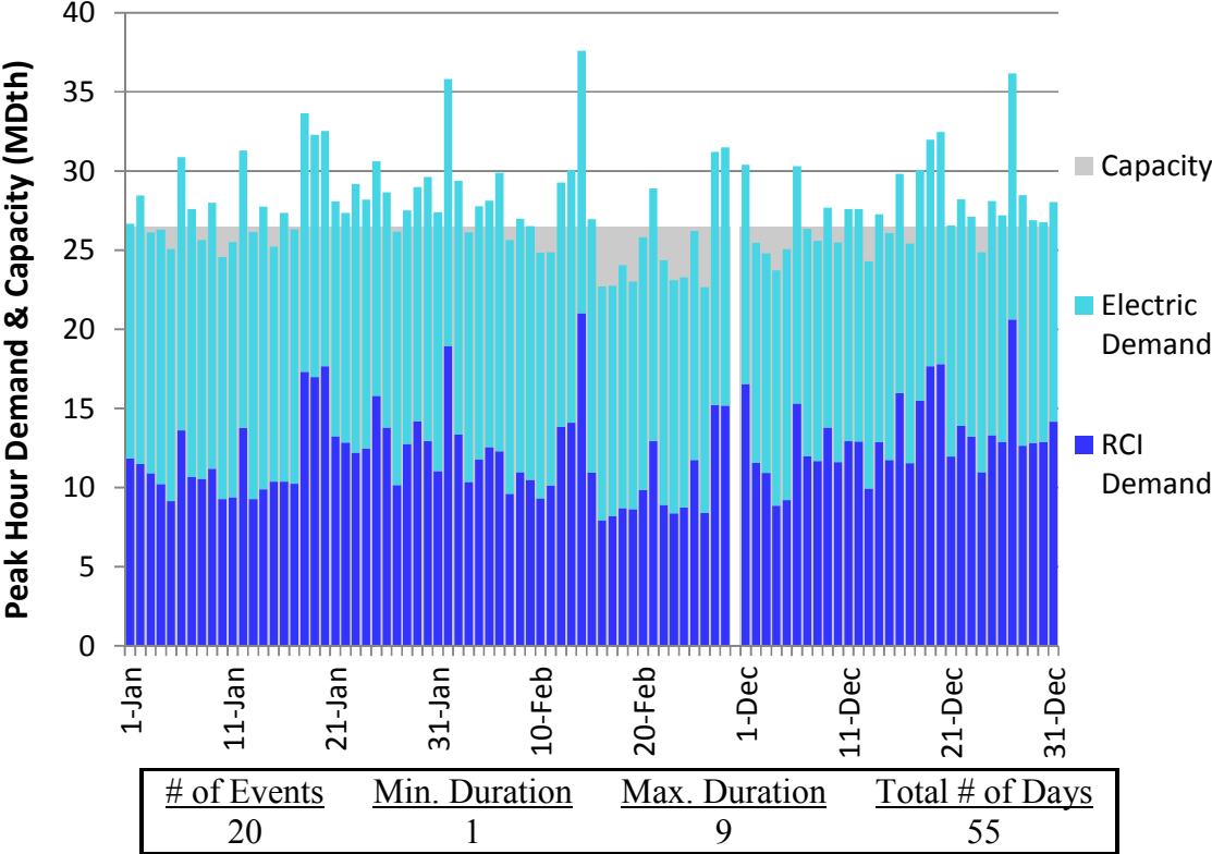
Figure J382. HGDS S0 Winter 2023 – Midwestern – Descending Demand
