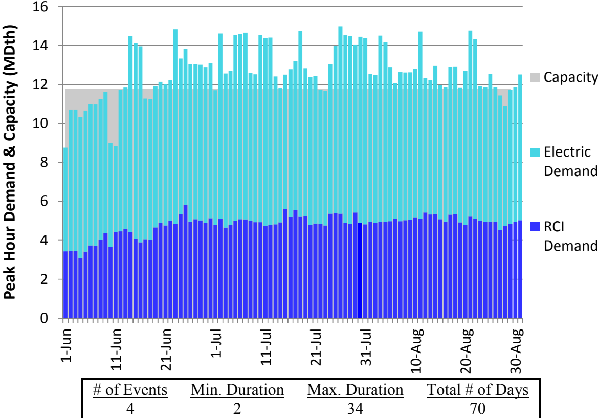
Figure J104. RGDS S5a Summer 2023 – NB/NS – Descending Demand
