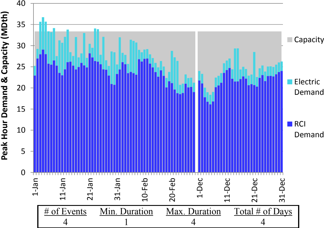
Figure J124. RGDS S5b Winter 2023 – East Tennessee – Descending Demand
