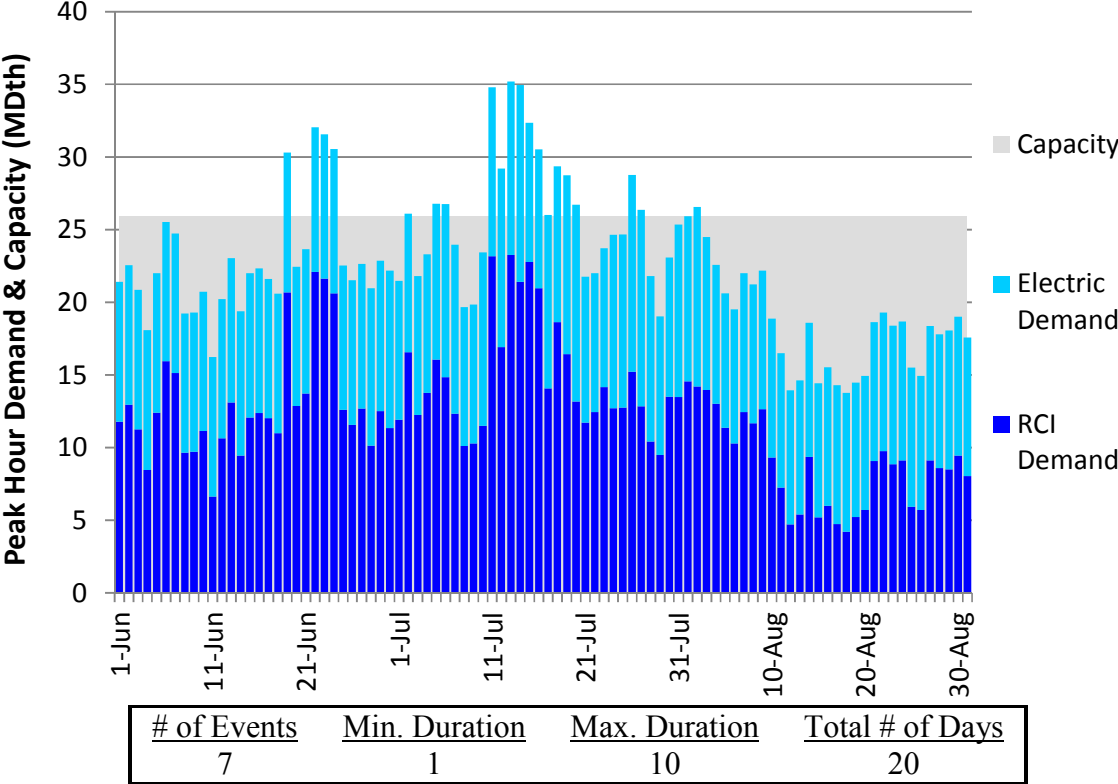
Figure J166. RGDS S5b Summer 2023 – Texas Eastern ETX – Descending Demand
