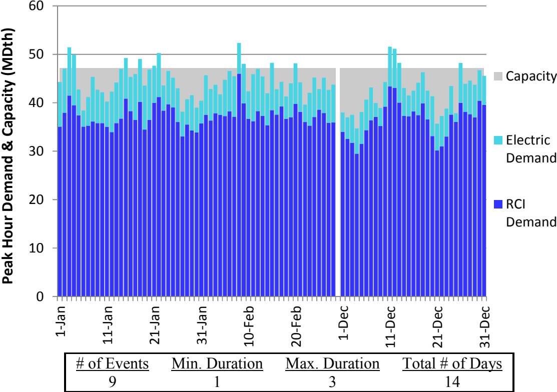
Figure J4. RGDS S5a Winter 2018 – Columbia Gas W PA/NY – Descending Demand
