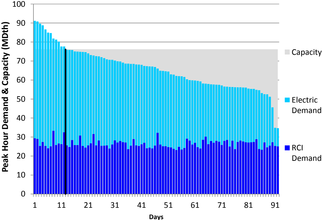
Figure J264. RGDS S5c Summer 2023 – Algonquin CT – Descending Demand
