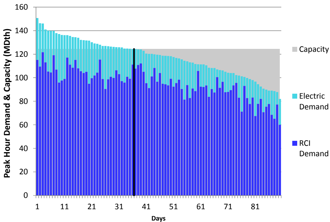
Figure J30. RGDS S5a Winter 2018 – Texas Eastern M3 North – Descending Demand
