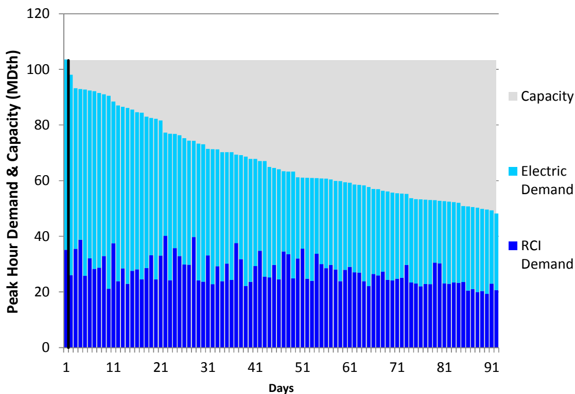
Figure J44. RGDS S5a Summer 2018 – Columbia Gas VA/MD – Descending Demand
