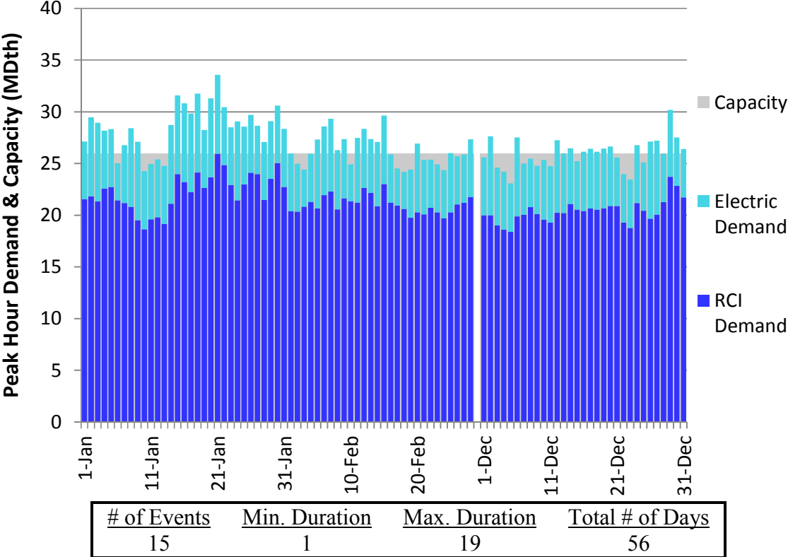
Figure J308. HGDS S9 Winter 2018 – NB/NS Supply – Descending Demand
