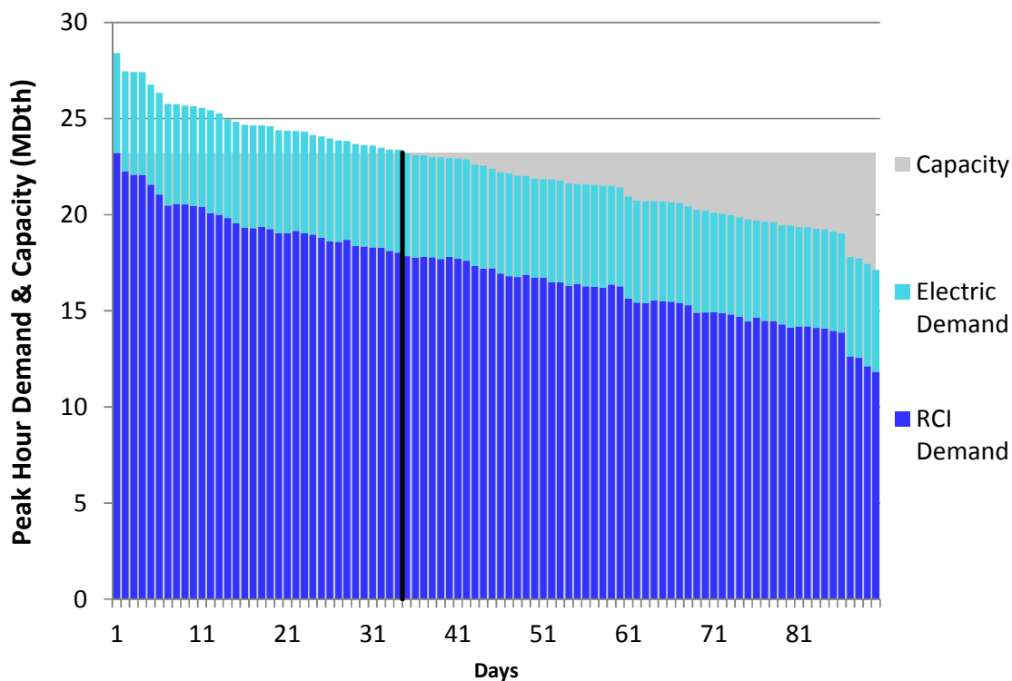
Figure J292. HGDS S9 Winter 2018 – Dominion Western NY– Descending Demand
