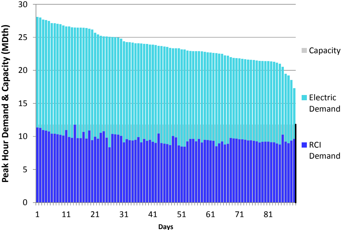
Figure J386. HGDS S0 Winter 2023 – NB/NS Supply – Descending Demand
