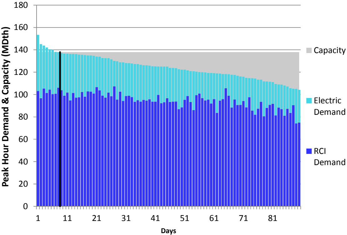
Figure J40. RGDS S5a Winter 2018 – Transco Leidy to Station 210 – Descending Demand
