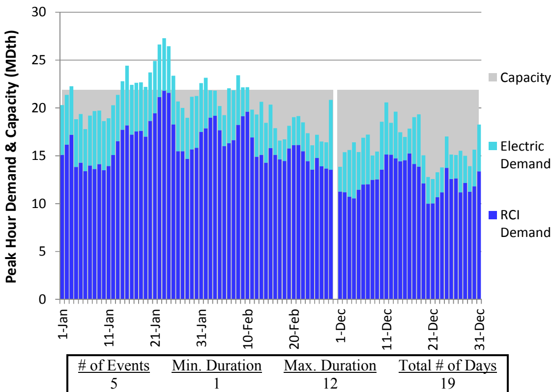
Figure J186. RGDS S5c Winter 2018 – Empire – Descending Demand
