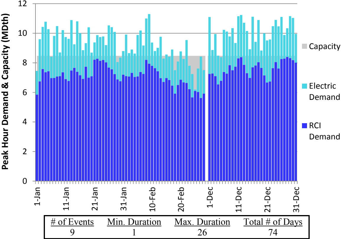
Figure J68. RGDS S5a Winter 2023 – Eastern Shore – Descending Demand
