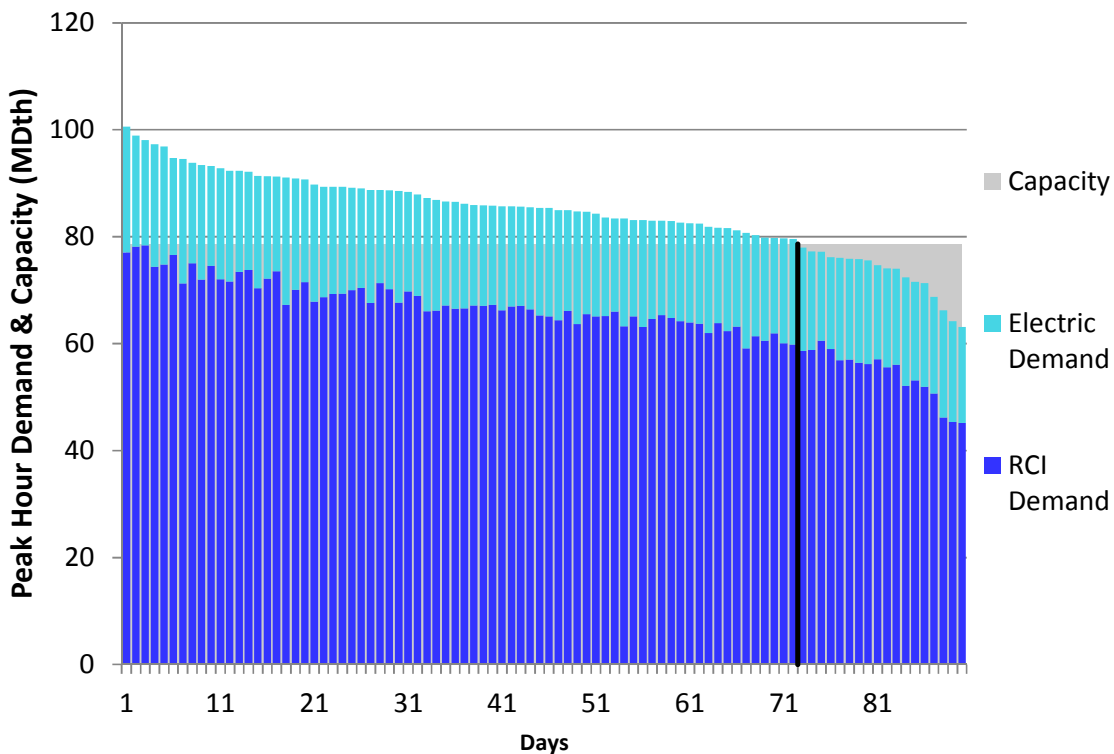
Figure J318. HGDS S9 Winter 2018 – Tennessee Z4 PA – Descending Demand
