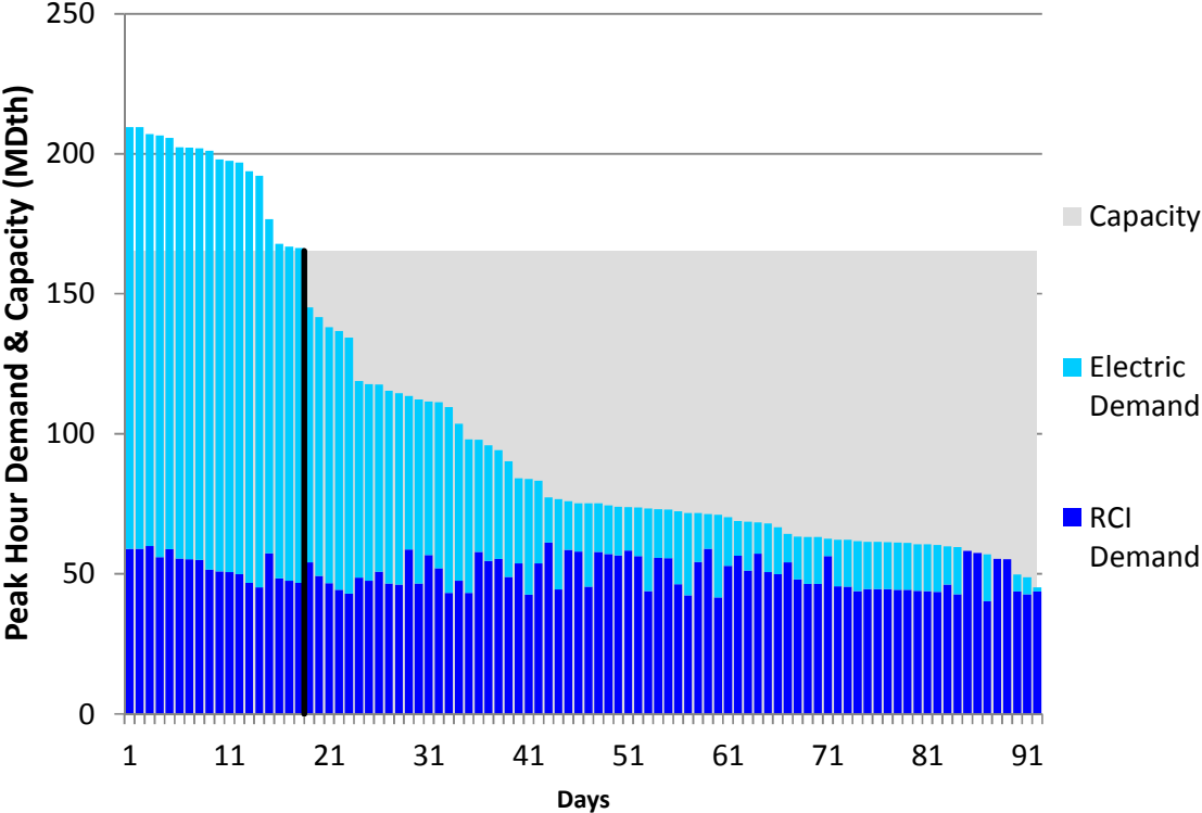
Figure J52. RGDS S5a Summer 2018 – Transco Z5 – Descending Demand
