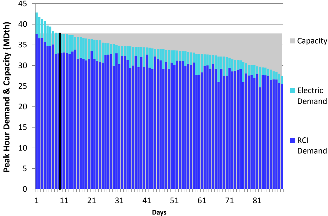
Figure J8. RGDS S5a Winter 2018 – Dominion Eastern NY– Descending Demand
