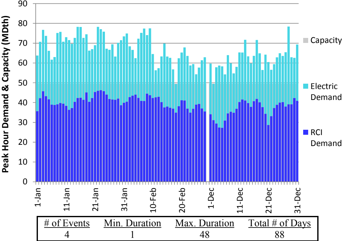
Figure J78. RGDS S5a Winter 2023 – Tennessee Z5 NY – Descending Demand
