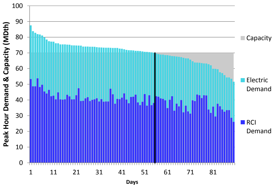
Figure J310. HGDS S9 Winter 2018 – NGPL IA/IL North – Descending Demand
