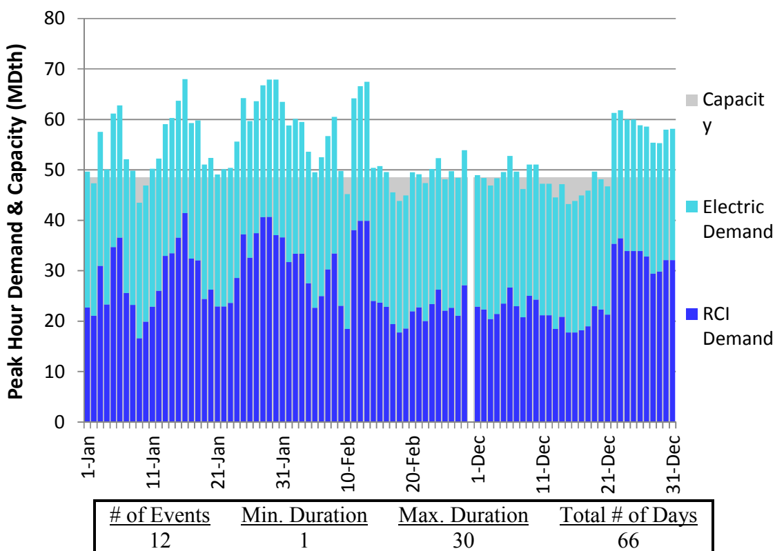
Figure J301. HGDS S9 Winter 2018 – Great Lakes East – Chronological Demand
