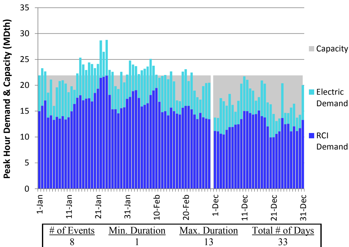
Figure J300. HGDS S9 Winter 2018 – Empire – Descending Demand
