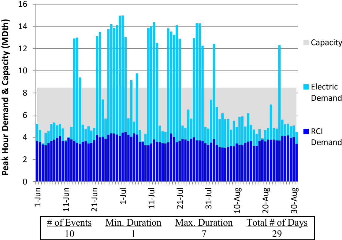
Figure J160. RGDS S5b Summer 2023 – Eastern Shore – Descending Demand
