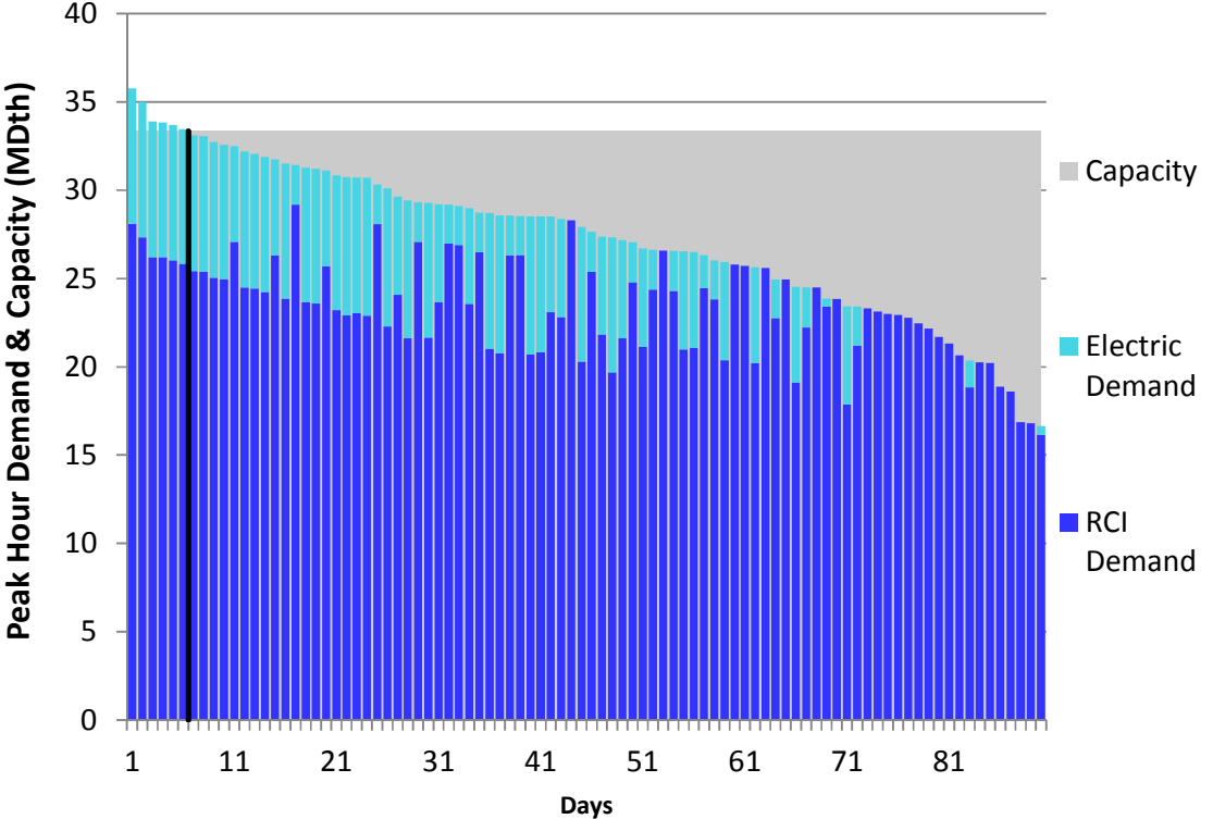
Figure J14. RGDS S5a Winter 2018 – East Tennessee – Descending Demand
