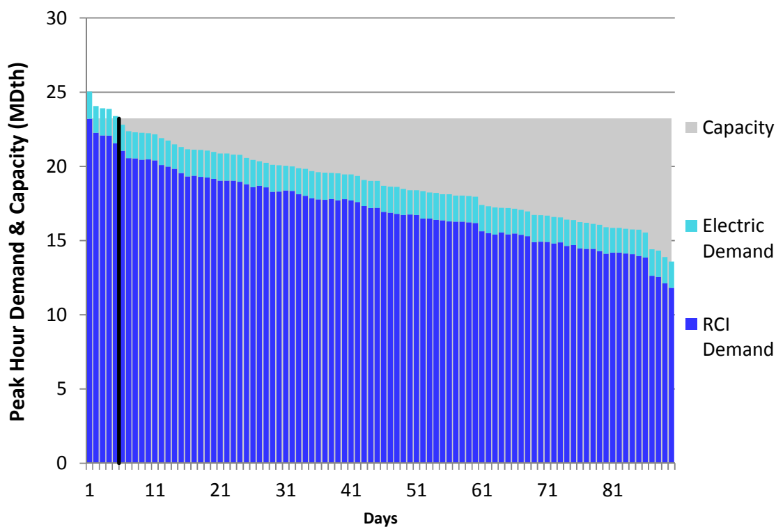
Figure J230. RGDS S5c Winter 2023 – Dominion Western NY– Descending Demand
