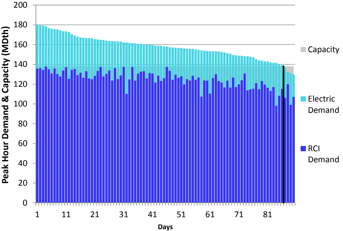
Figure J150. RGDS S5b Winter 2023 – Transco Leidy to Station 210 – Descending Demand
