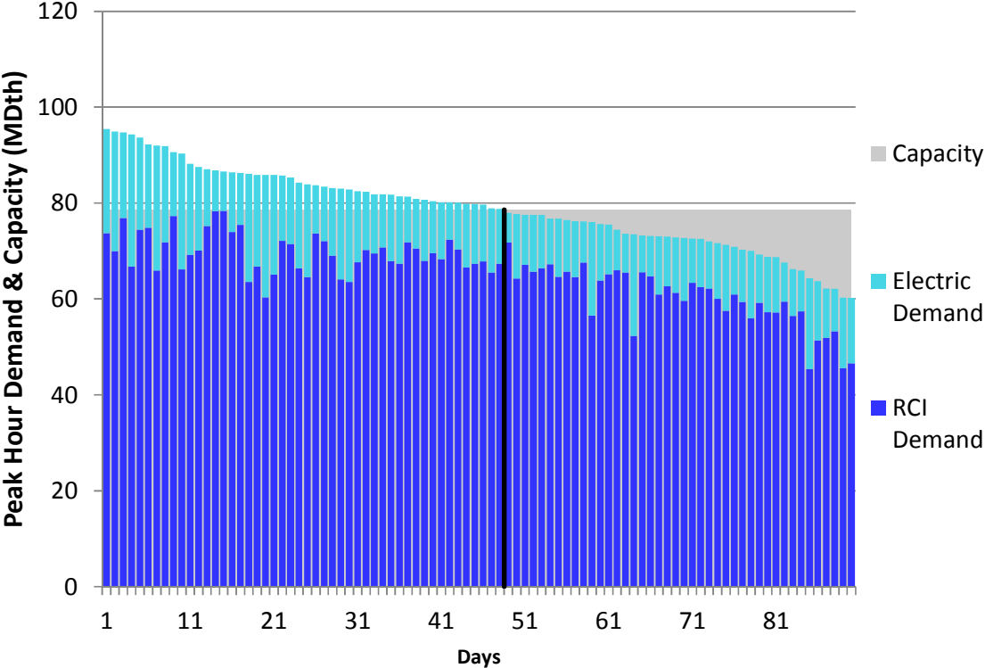
Figure J134. RGDS S5b Winter 2023 – Tennessee Z4 PA – Descending Demand
