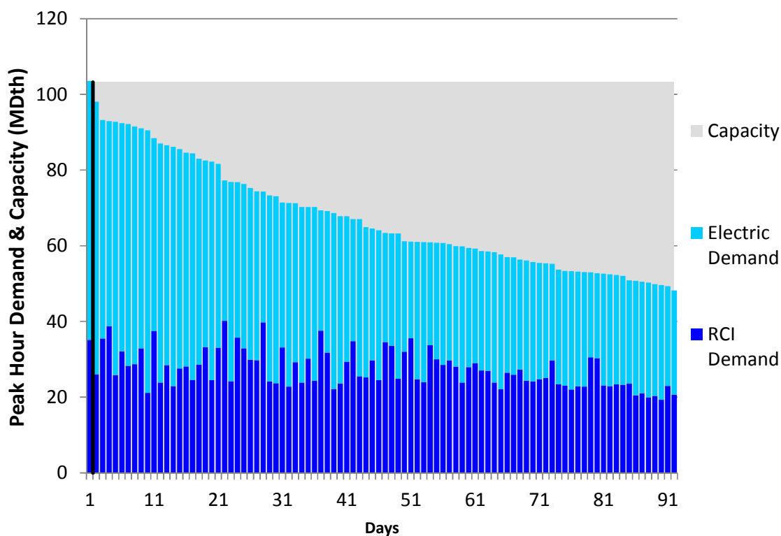
Figure J212. RGDS S5c Summer 2018 – Columbia Gas VA/MD – Descending Demand
