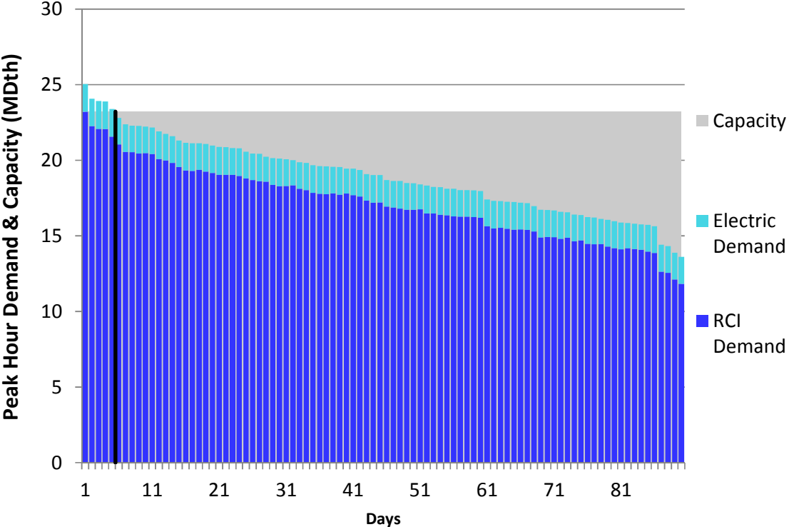
Figure J120. RGDS S5b Winter 2023 – Dominion Western NY– Descending Demand
