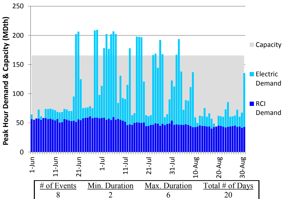
Figure J220. RGDS S5c Summer 2018 – Transco Z5 – Descending Demand
