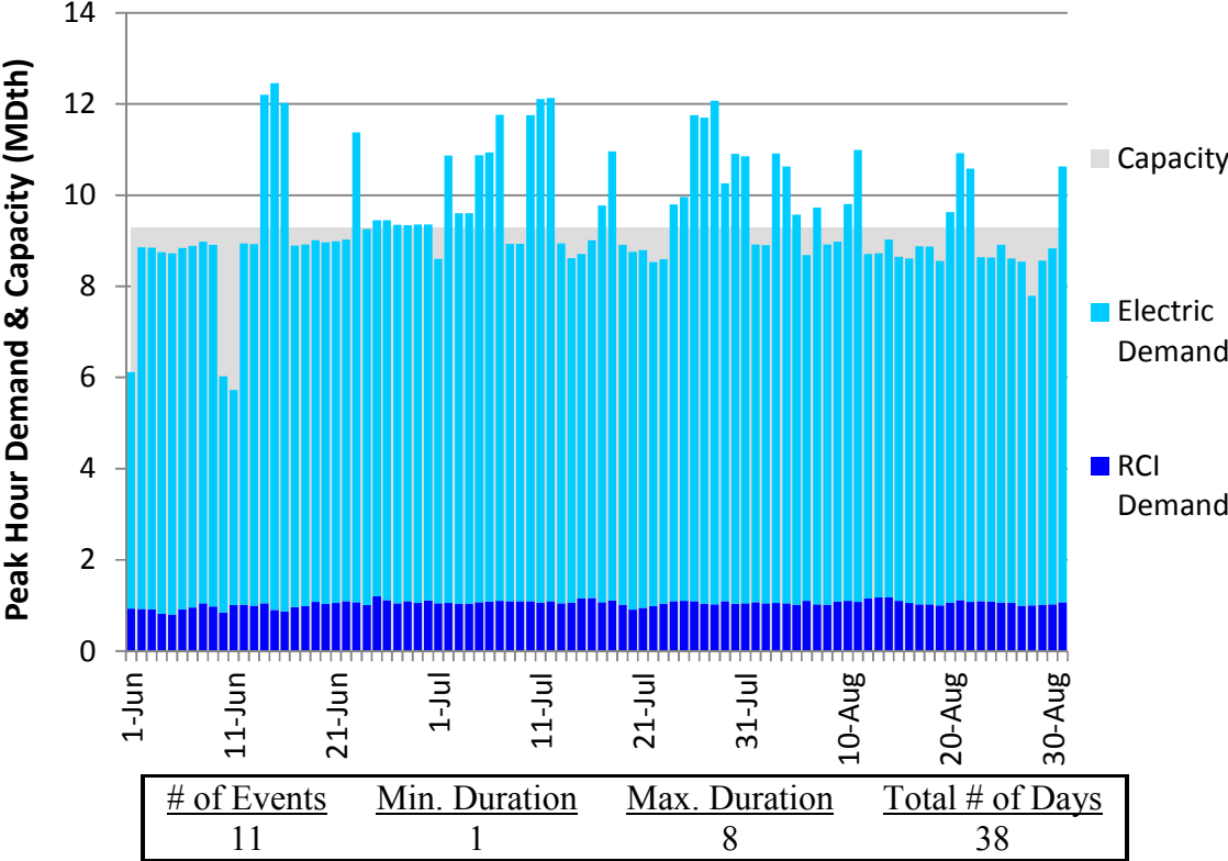
Figure J106. RGDS S5a Summer 2023 – PNGTS N of Westbrook – Descending Demand
