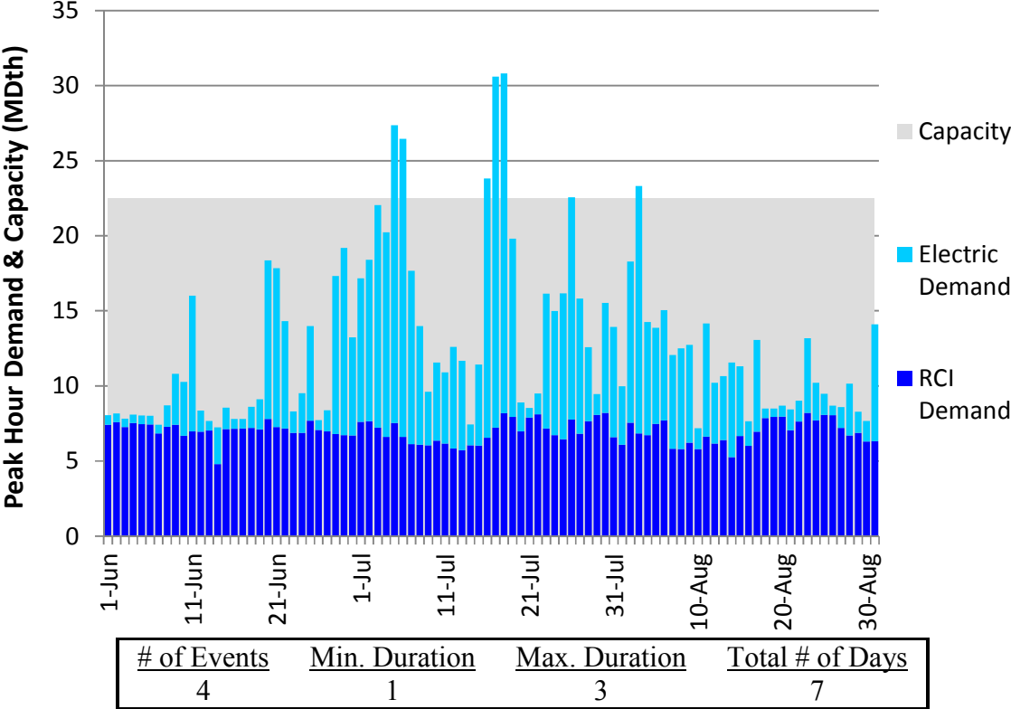
Figure J214. RGDS S5c Summer 2018 – Dominion Southeast – Descending Demand
