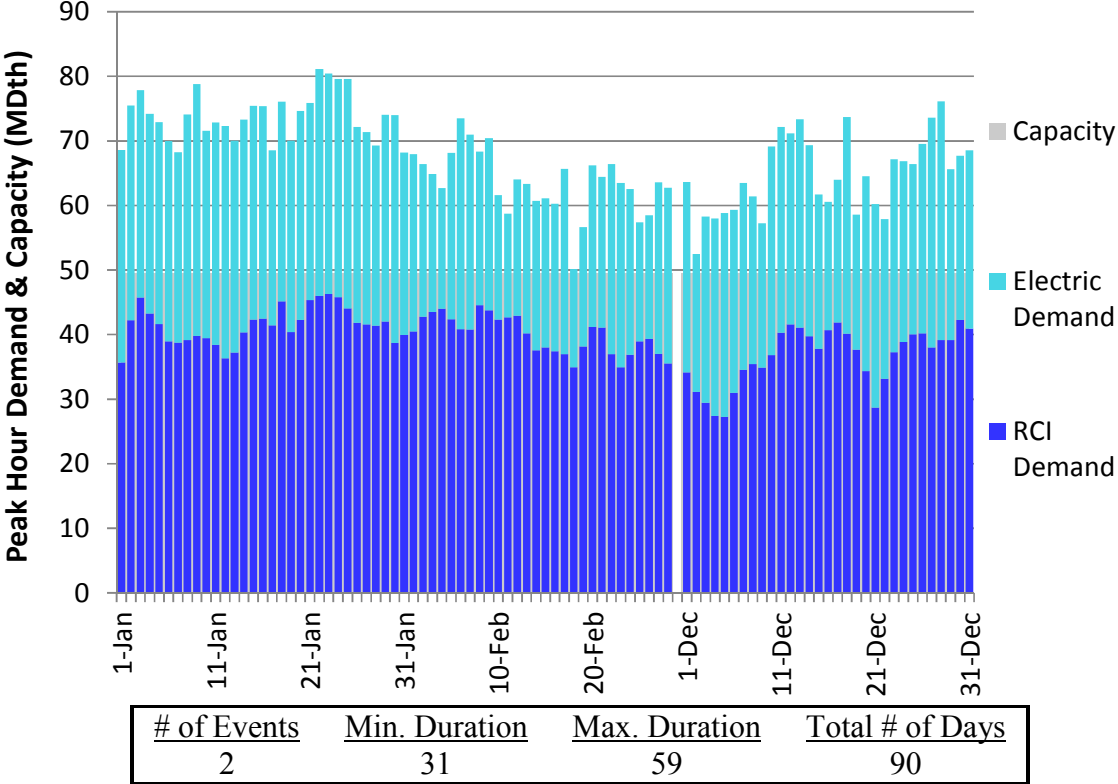
Figure J136. RGDS S5b Winter 23 – Tennessee Z5 NY – Descending Demand
