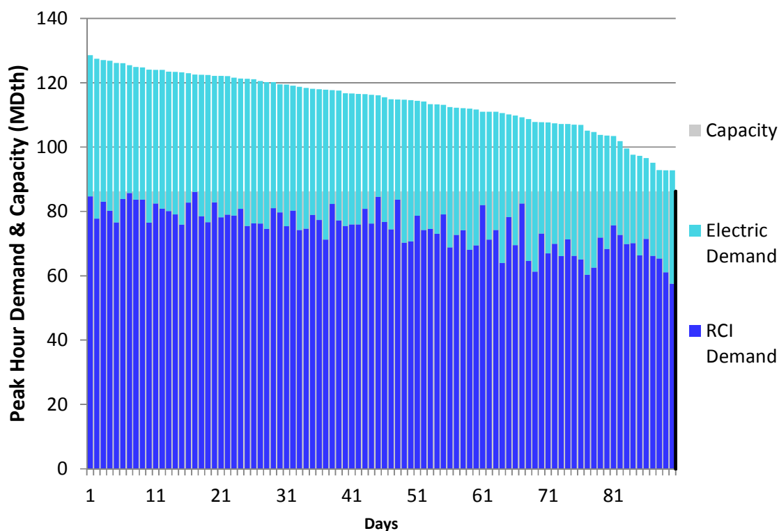
Figure J402. HGDS S0 Winter 2023 – Texas Eastern M2 PA South – Descending Demand
