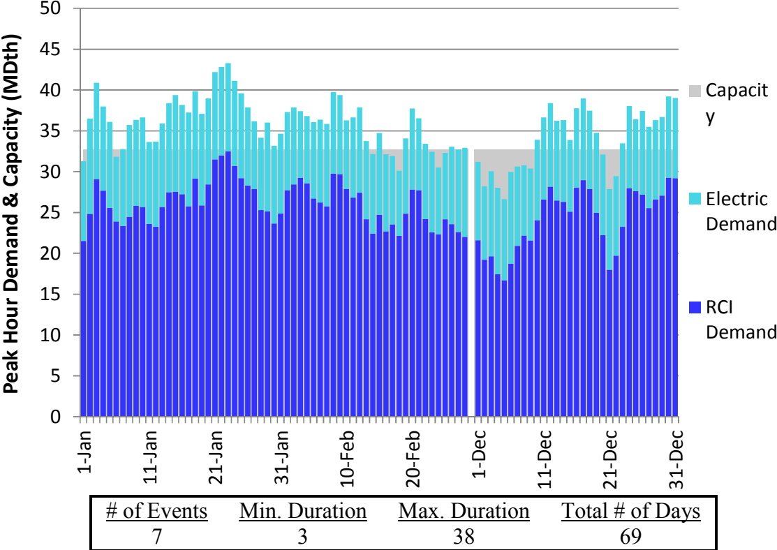
Figure J240. RGDS S5c Winter 2023 – Millennium – Descending Demand
