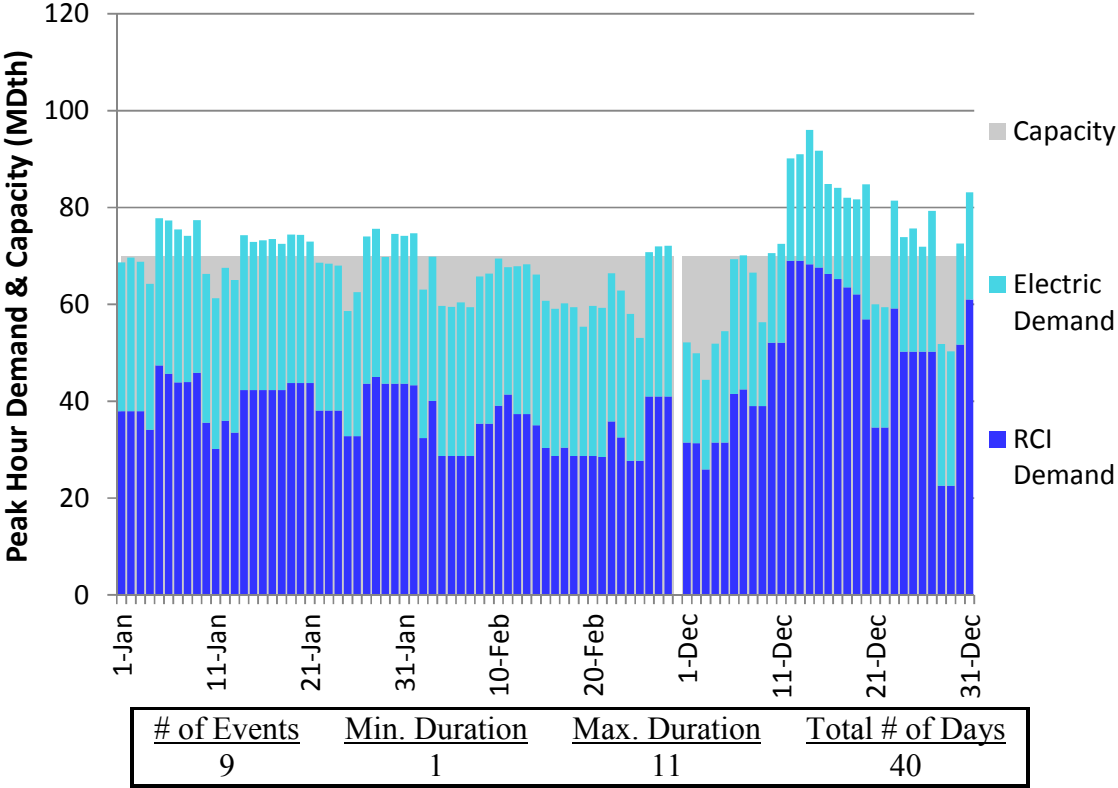
Figure J390. HGDS S0 Winter 2023 – NGPL IA/IL South – Descending Demand
