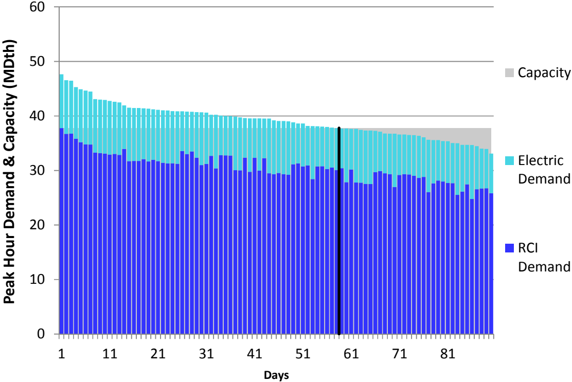
Figure J228. RGDS S5c Winter 2023 – Dominion Eastern NY– Descending Demand
