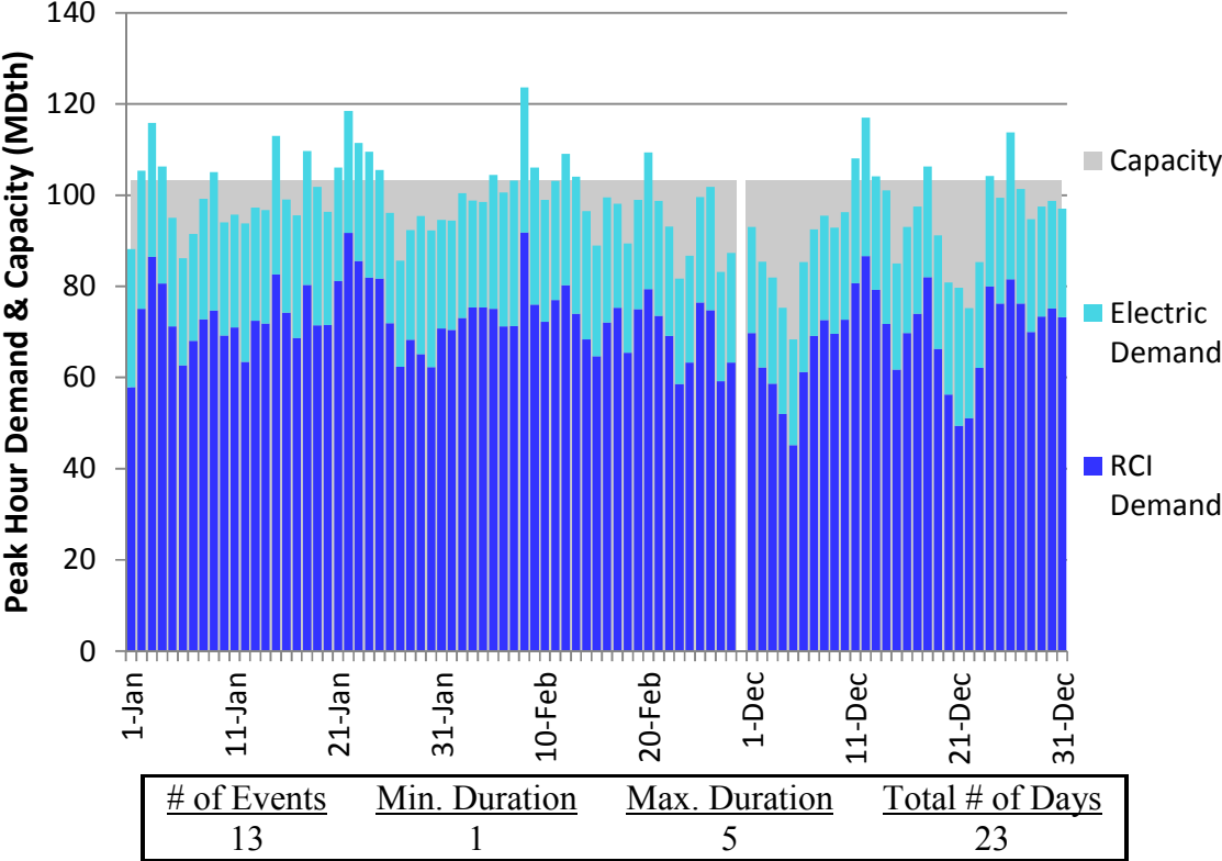
Figure J170. RGDS S5c Winter 2018 – Columbia Gas VA/MD – Descending Demand
