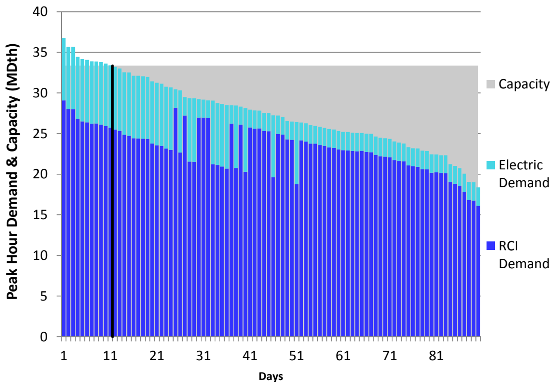
Figure J234. RGDS S5c Winter 2023 – East Tennessee – Descending Demand
