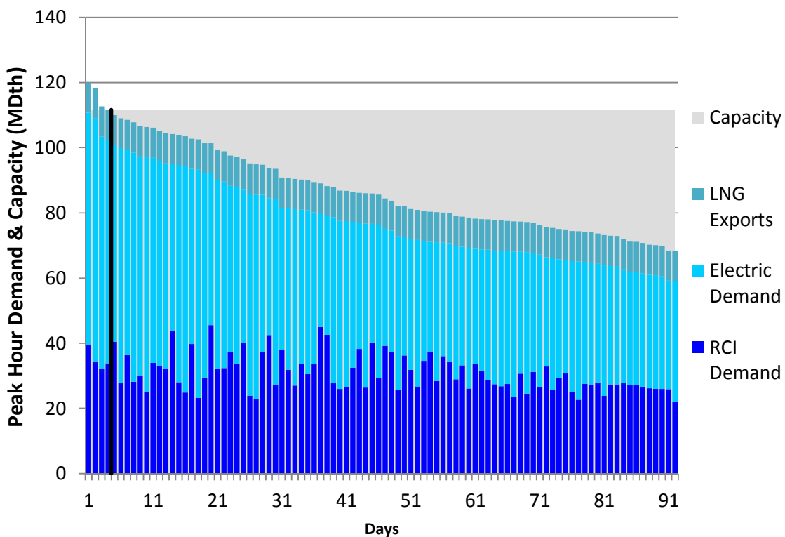
Figure J156. RGDS S5b Summer 2023 – Columbia Gas VA/MD – Descending Demand
