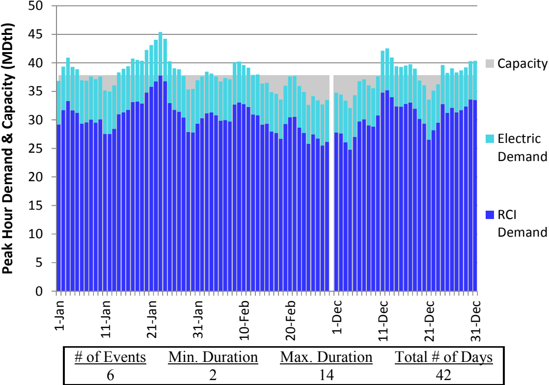
Figure J366. HGDS S0 Winter 2023 – Dominion Eastern NY– Descending Demand
