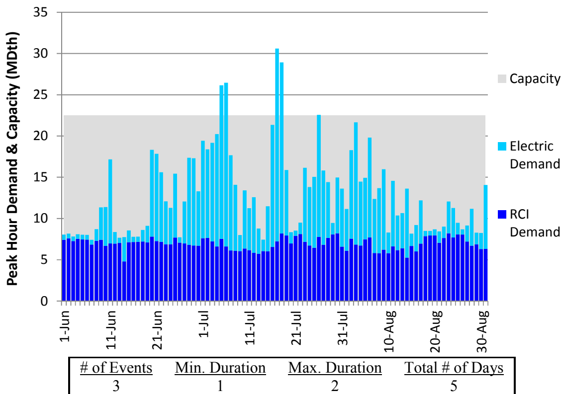
Figure J46. RGDS S5a Summer 2018 – Dominion Southeast – Descending Demand
