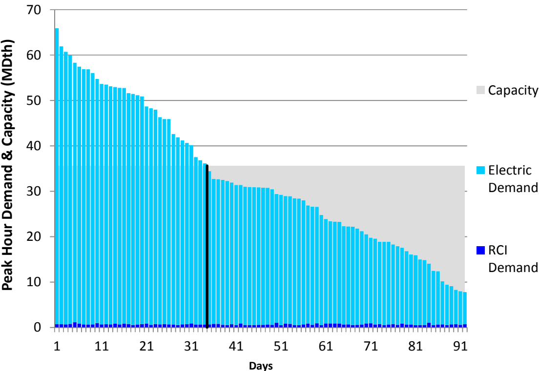
Figure J432. HGDS S0 Summer 2023 – Iroquois Z1 → Z2 – Descending Demand
