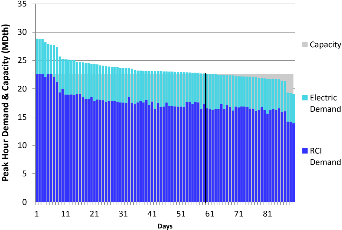
Figure J420. HGDS S0 Winter 2023 – Viking Zone 1 – Descending Demand
