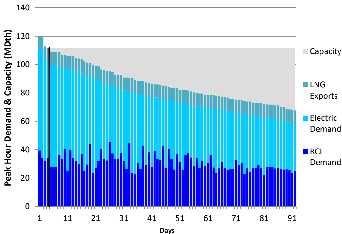
Figure J98. RGDS S5a Summer 2023 – Columbia Gas VA/MD – Descending Demand
