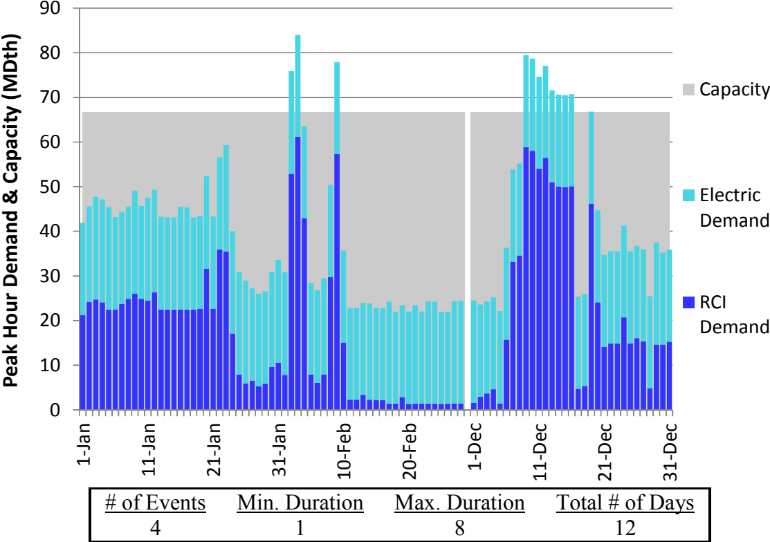
Figure J418. HGDS S0 Winter 2023 – Vector Zone 1 – Descending Demand
