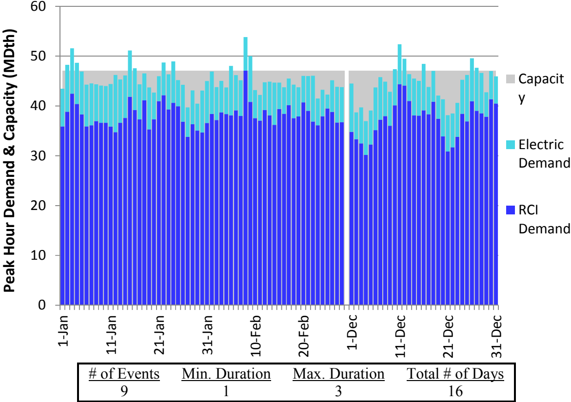
Figure J224. RGDS S5c Winter 2023 – Columbia Gas W PA/NY – Descending Demand
