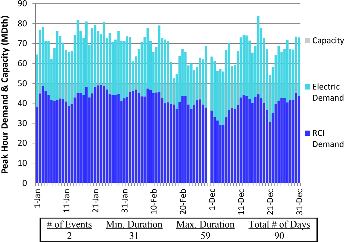
Figure J194. RGDS S5c Winter 2018 – Tennessee Z5 NY – Descending Demand
