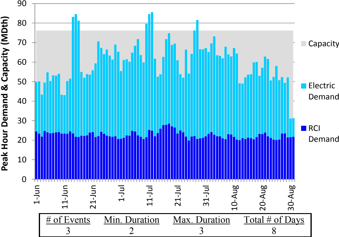
Figure J340. HGDS S9 Summer 2018 – Algonquin CT – Descending Demand
