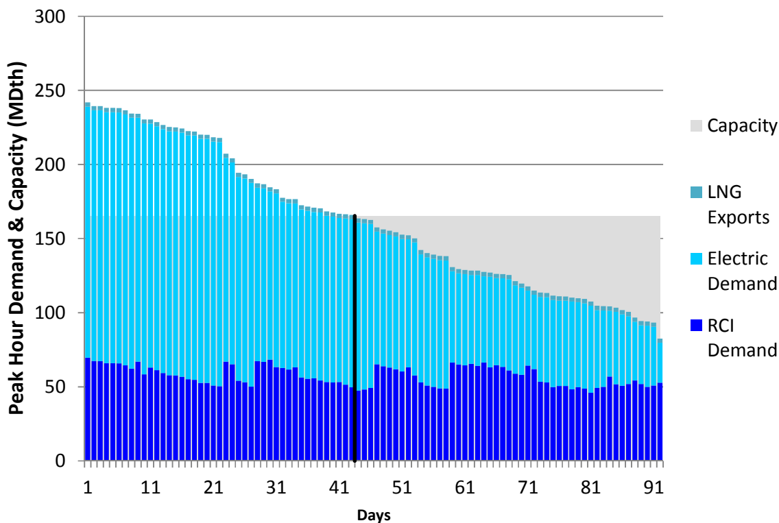
Figure J442. HGDS S0 Summer 2023 – Transco Z5 – Descending Demand
