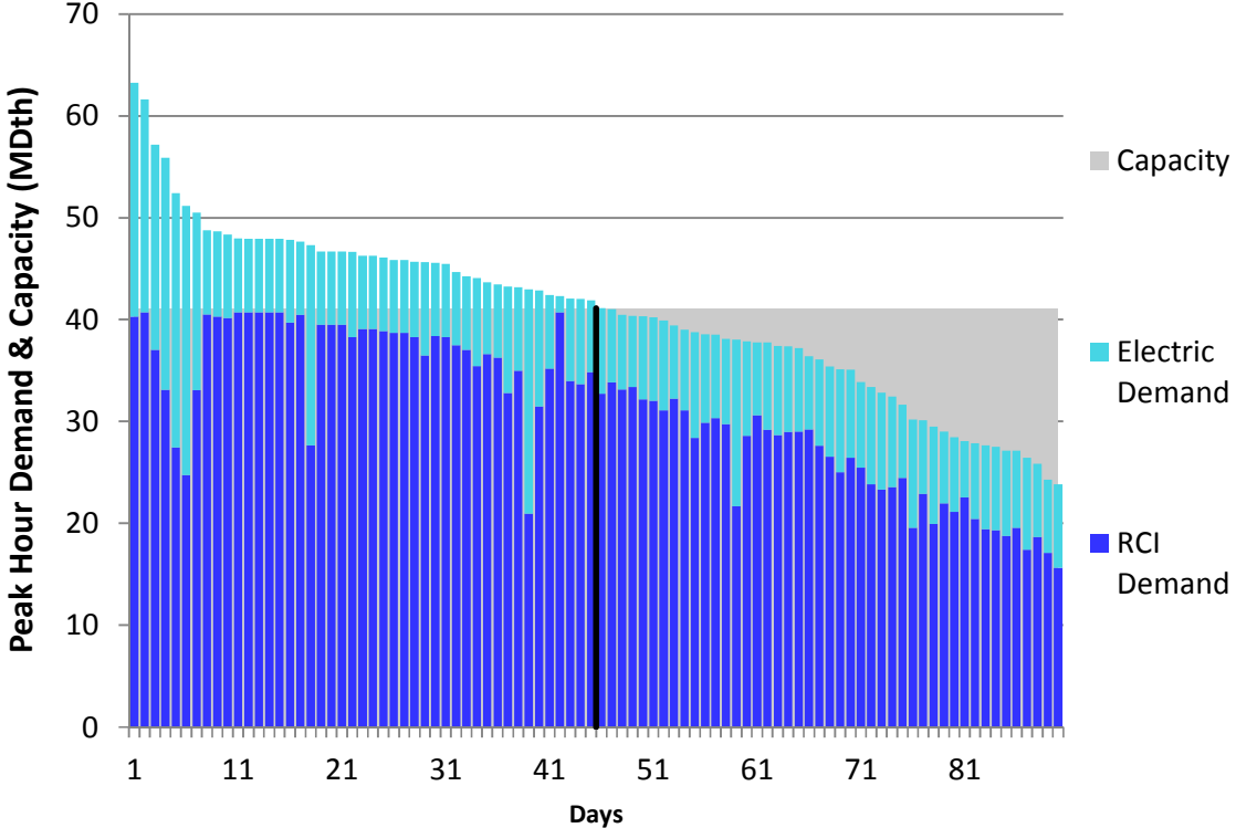
Figure J314. HGDS S9 Winter 2018 – Northern Border Chicago – Descending Demand
