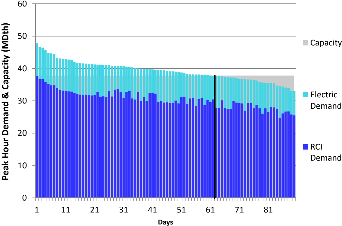
Figure J118. RGDS S5b Winter 2023 – Dominion Eastern NY– Descending Demand
