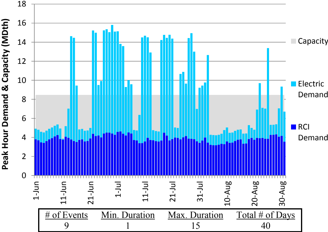
Figure J428. HGDS S0 Summer 2023 – Eastern Shore – Descending Demand
