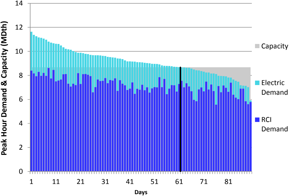
Figure J298. HGDS S9 Winter 2018 – Eastern Shore – Descending Demand
