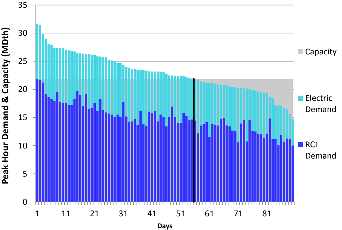
Figure J70. RGDS S5a Winter 2023 – Empire – Descending Demand
