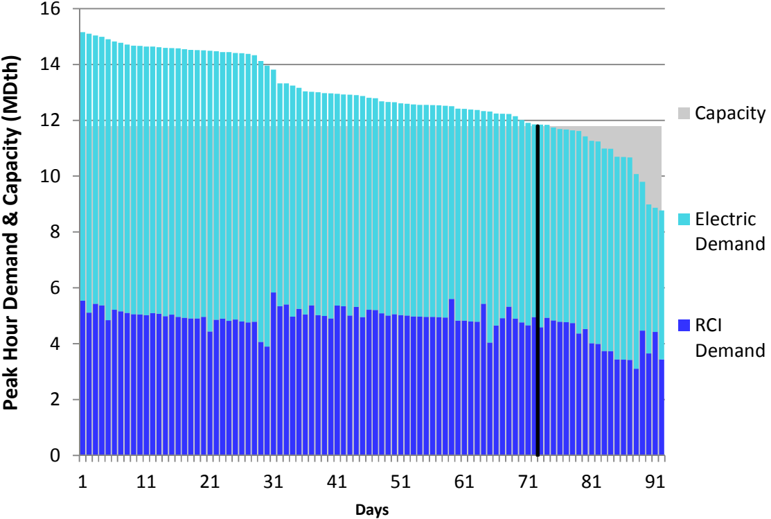
Figure J162. RGDS S5b Summer 2023 – NB/NS – Descending Demand
