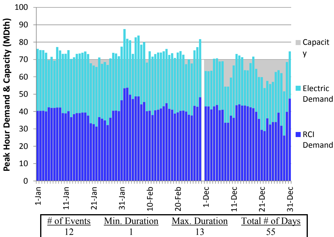
Figure J310. HGDS S9 Winter 2018 – NGPL IA/IL North – Descending Demand
