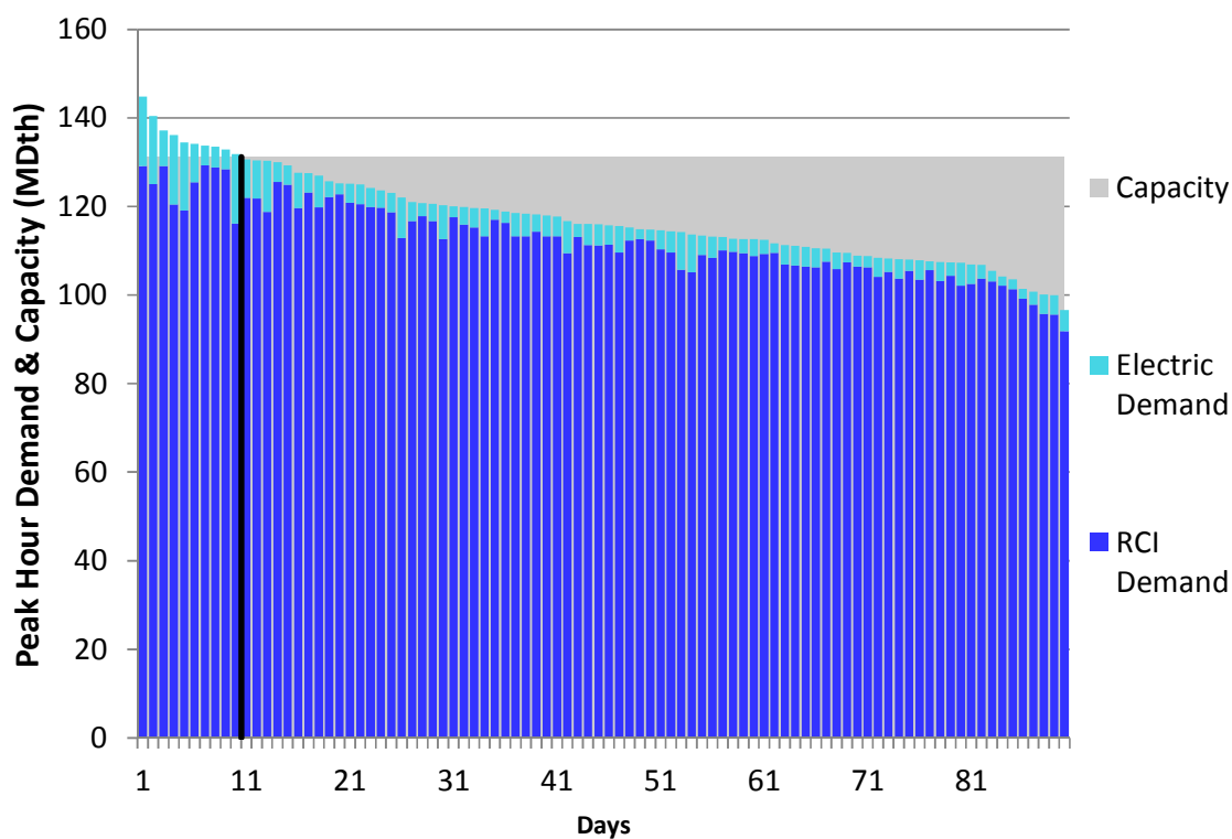
Figure J200. RGDS S5c Winter 2018 – TransCanada Ontario West – Descending Demand
