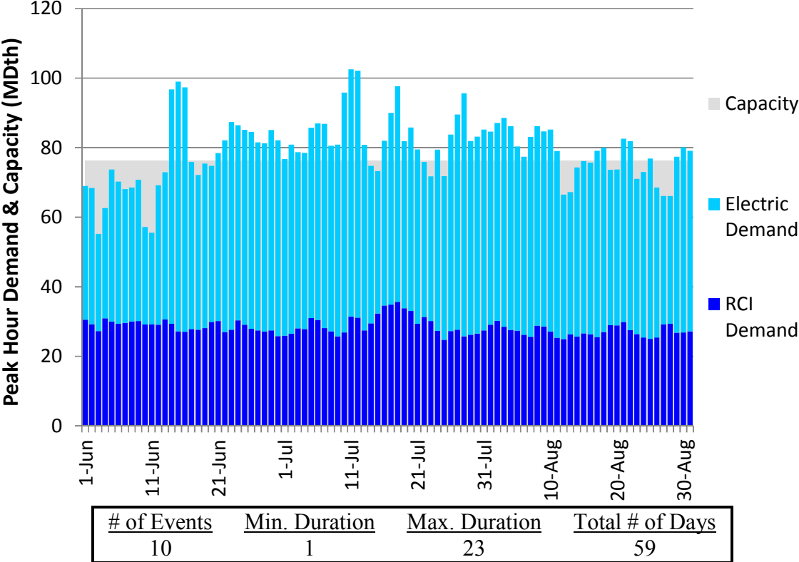
Figure J422. HGDS S0 Summer 2023 – Algonquin CT – Descending Demand
