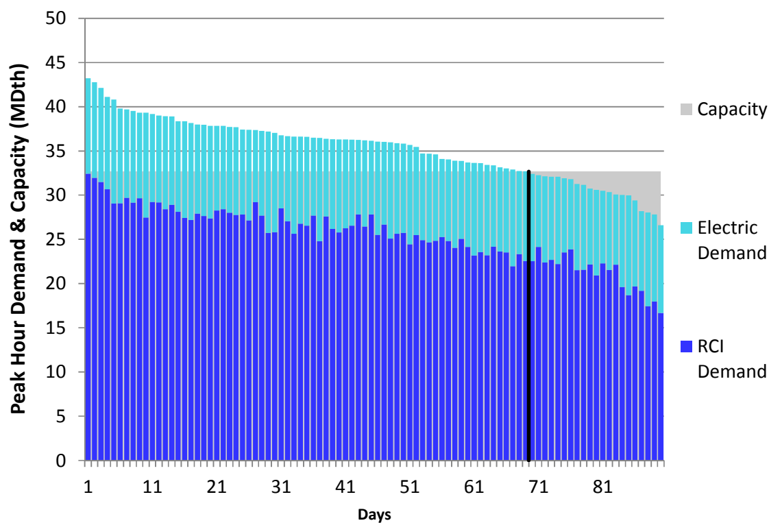
Figure J188. RGDS S5c Winter 2018 – Millennium – Descending Demand
