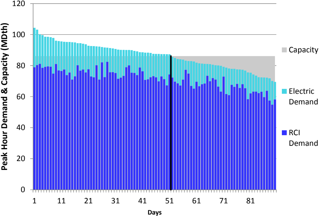
Figure J196. RGDS S5c Winter 2018 – Texas Eastern M2 PA South – Descending Demand
