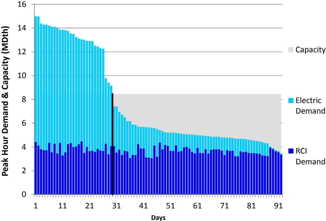
Figure J160. RGDS S5b Summer 2023 – Eastern Shore – Descending Demand
