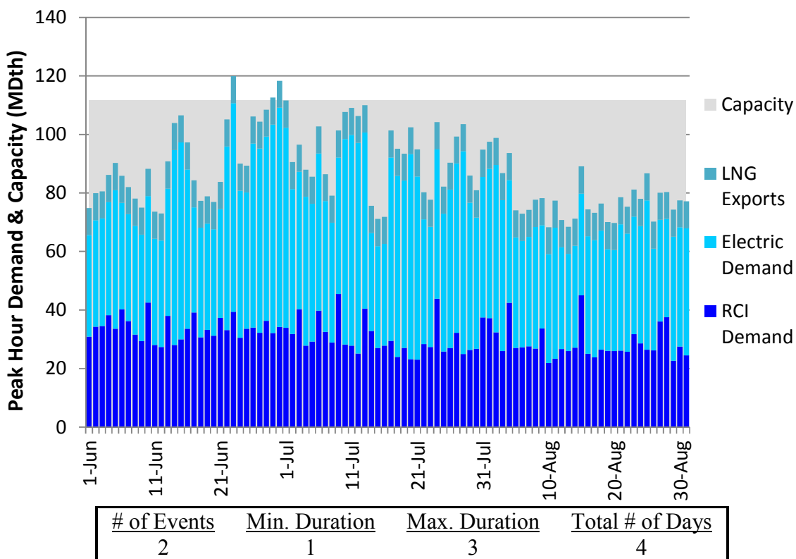
Figure J156. RGDS S5b Summer 2023 – Columbia Gas VA/MD – Descending Demand
