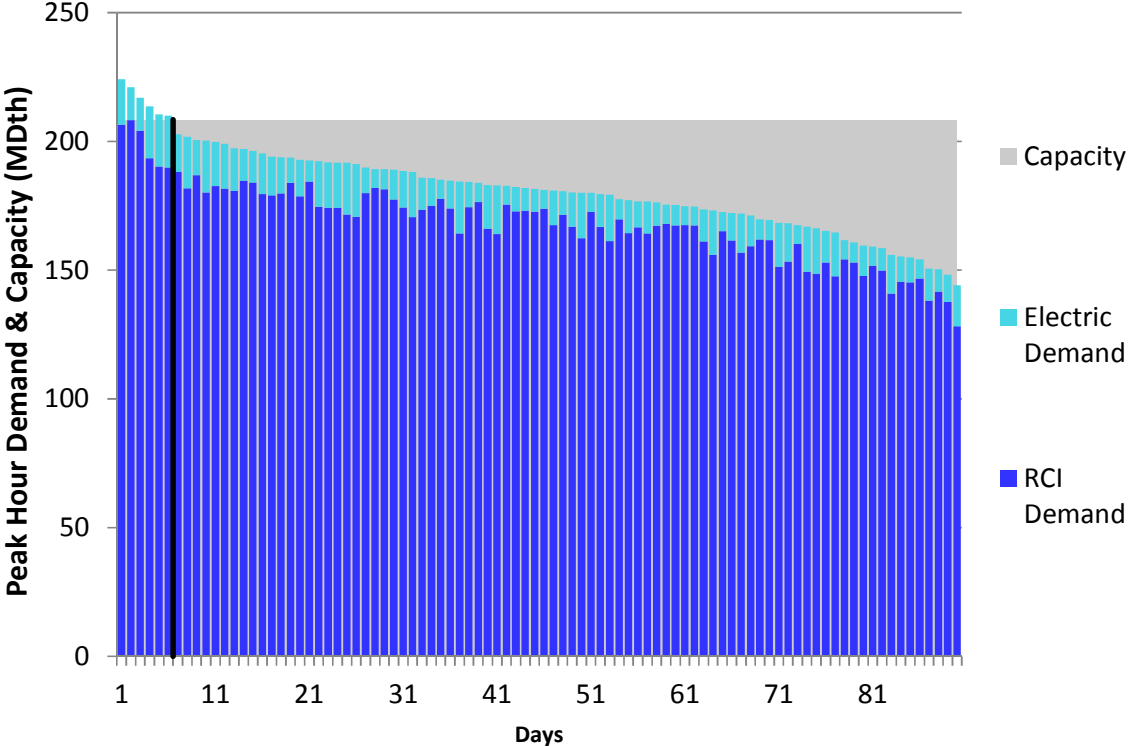
Figure J336. HGDS S9 Winter 2018 – Union Gas Dawn – Descending Demand
