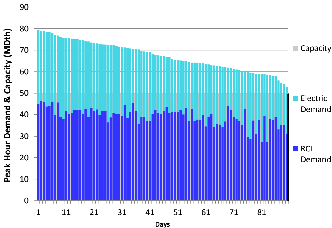
Figure J246. RGDS S5c Winter 2023 – Tennessee Z5 NY – Descending Demand
