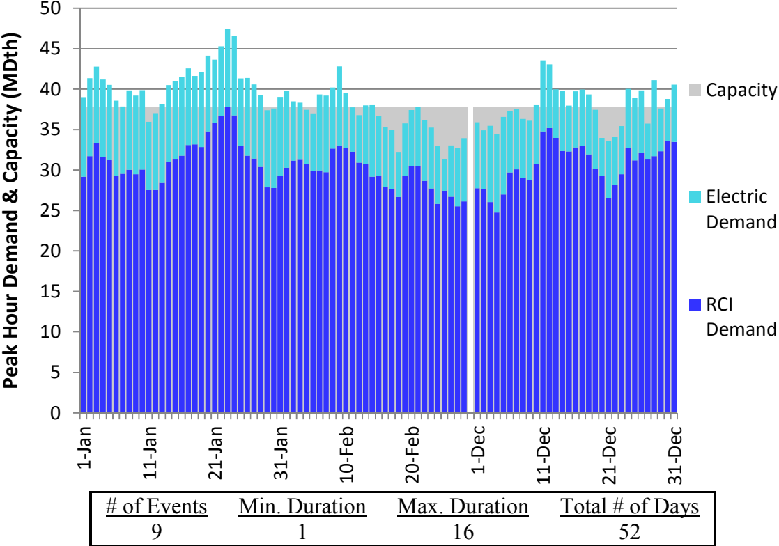
Figure J60. RGDS S5a Winter 2023 – Dominion Eastern NY– Descending Demand
