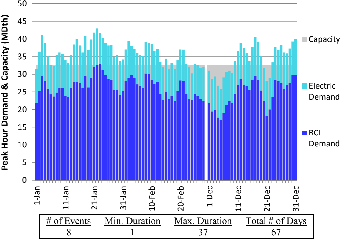
Figure J306. HGDS S9 Winter 2018 – Millennium – Descending Demand
