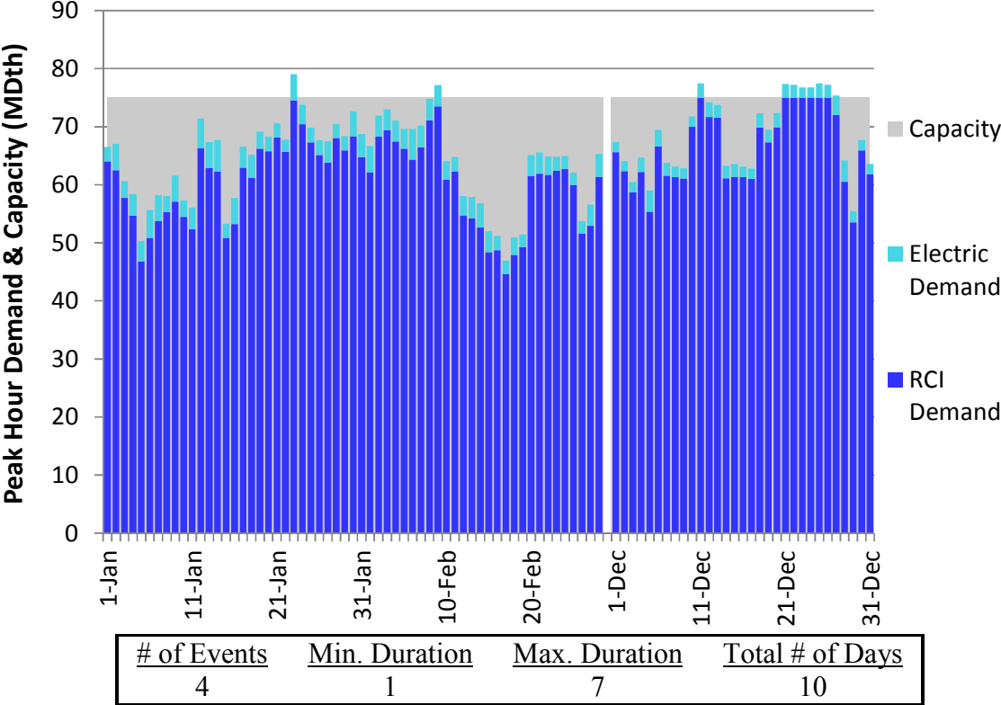
Figure J356. HGDS S0 Winter 2023 – Alliance – Descending Demand
