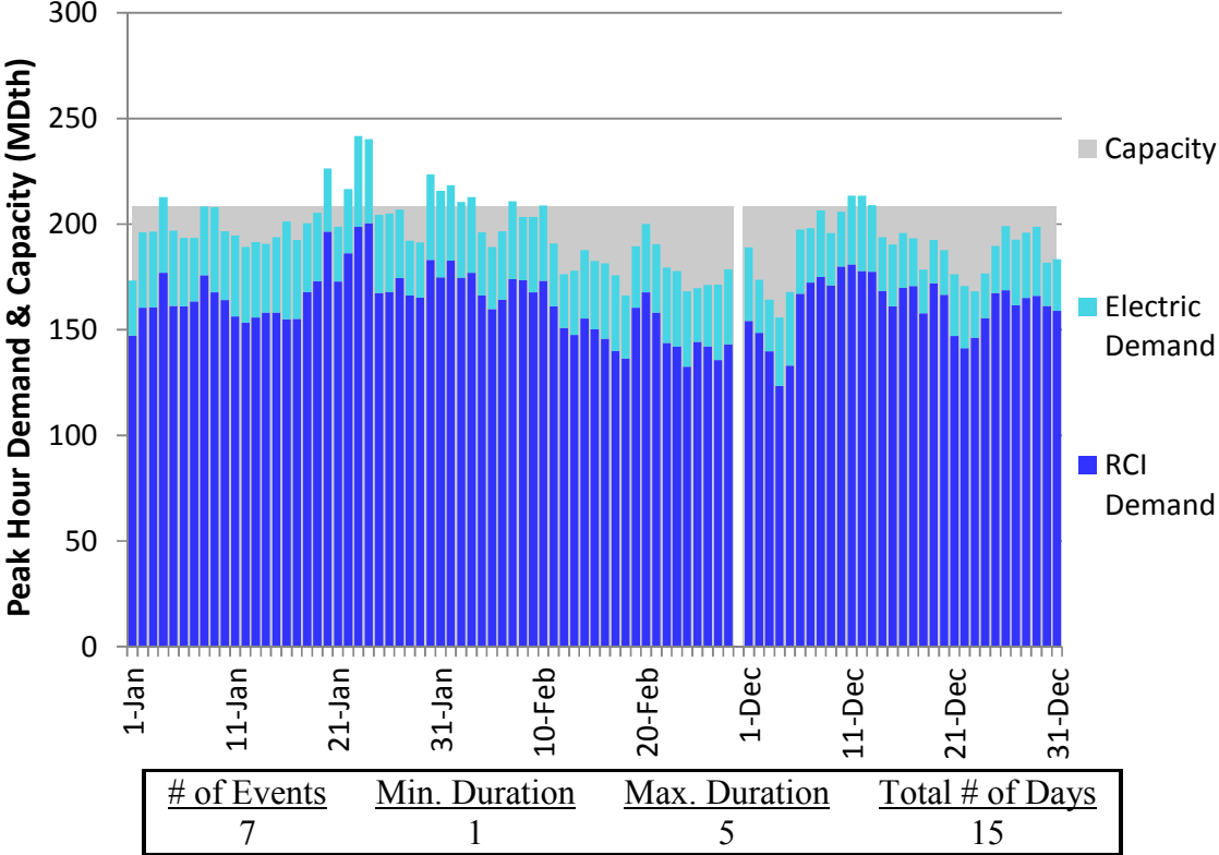
Figure J416. HGDS S0 Winter 2023 – Union Gas Dawn – Descending Demand
