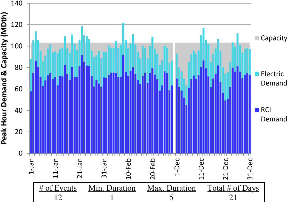
Figure J2. RGDS S5a Winter 2018 – Columbia Gas VA/MD – Descending Demand
