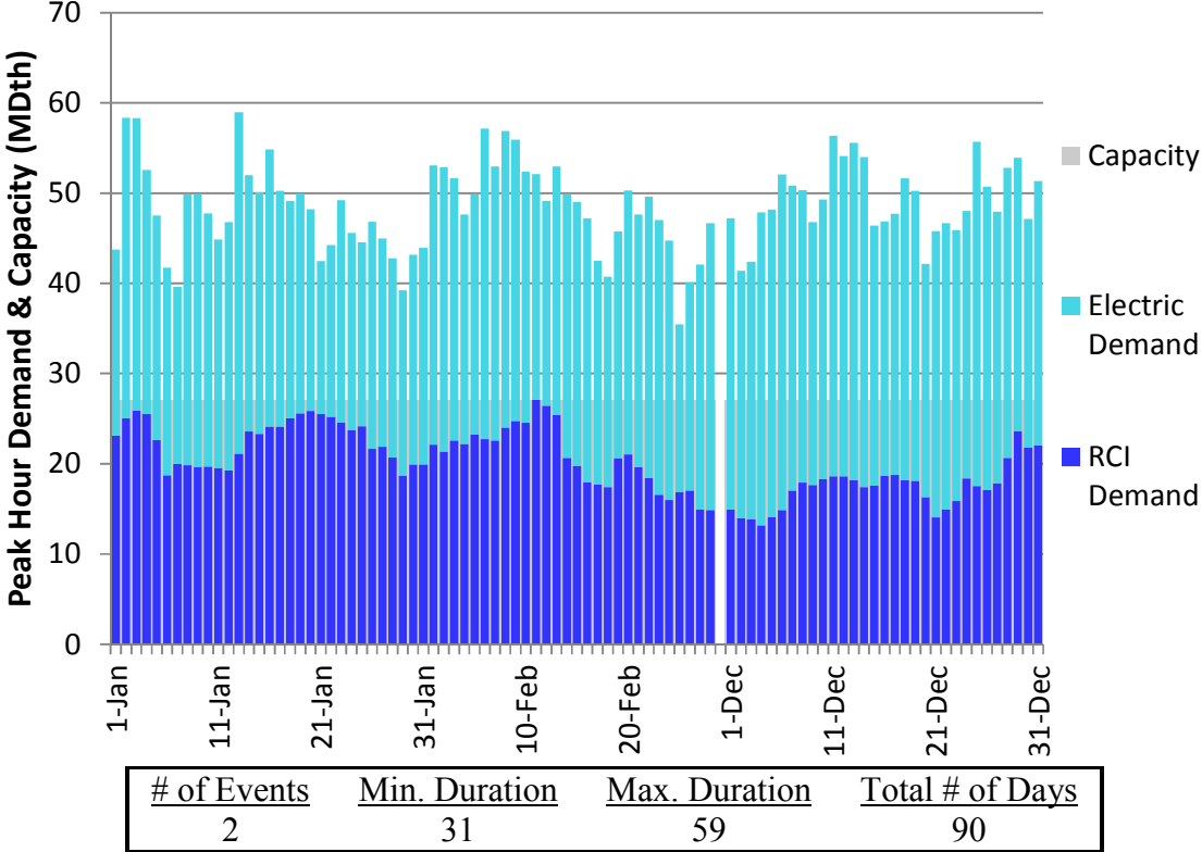
Figure J58. RGDS S5a Winter 2023 – Constitution – Descending Demand
