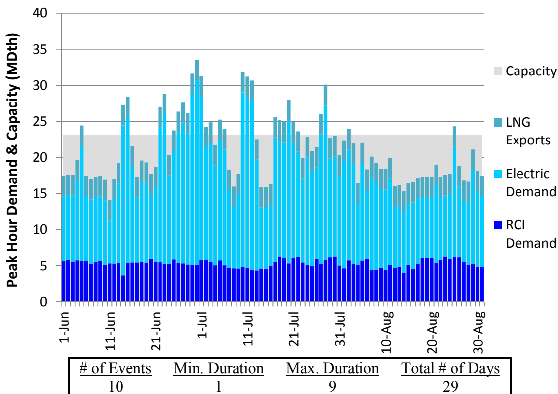
Figure J267. RGDS S5c Summer 2023 – Dominion Southeast – Chronological Demand
