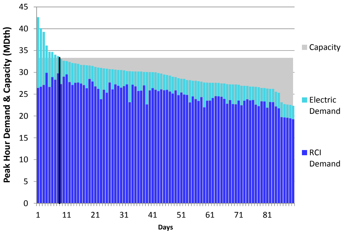
Figure J316. HGDS S9 Winter 2018 – Northern Natural Zone D – Descending Demand
