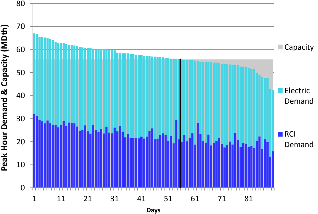
Figure J358. HGDS S0 Winter 2023 – ANR Northern IL – Descending Demand
