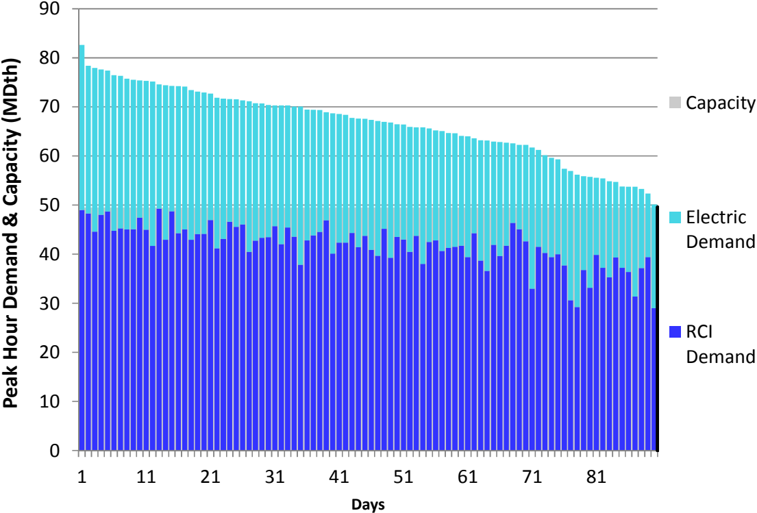
Figure J26. RGDS S5a Winter 2018 – Tennessee Z5 NY – Descending Demand
