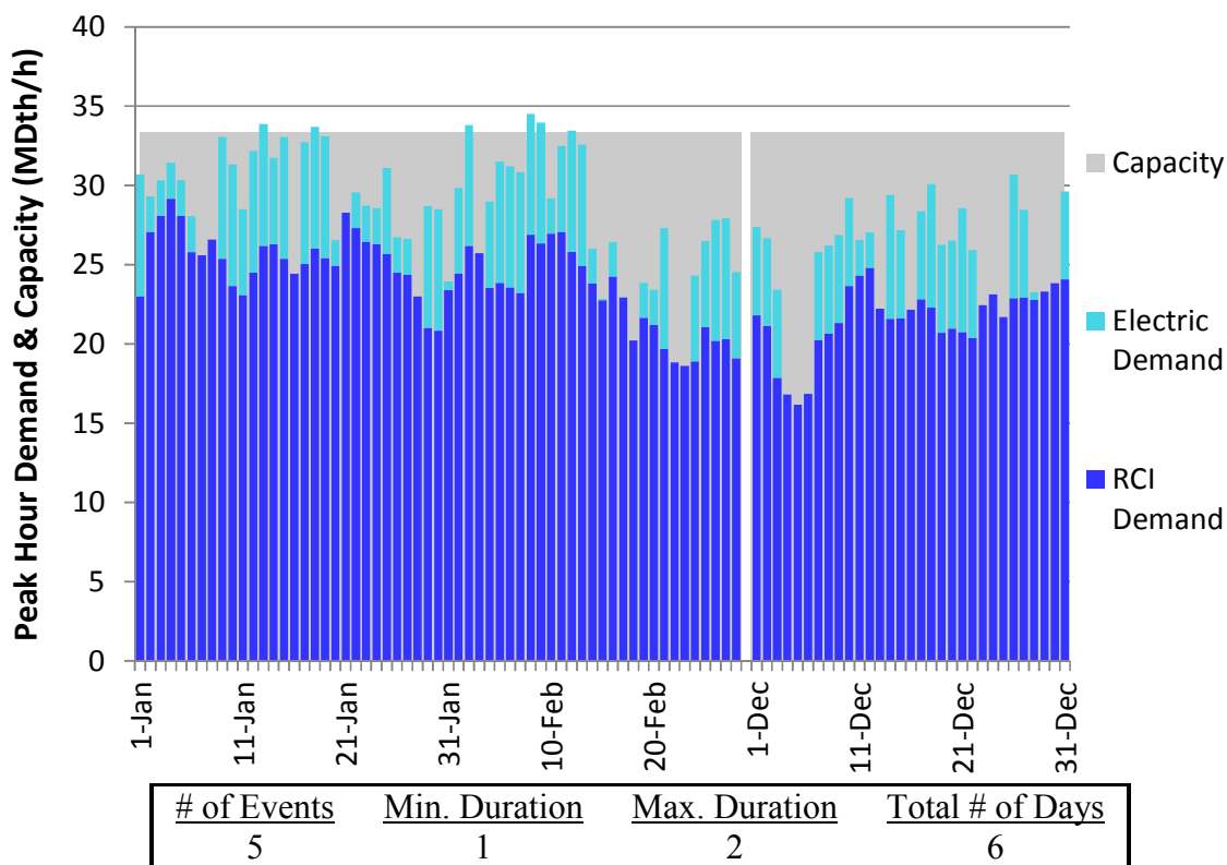
Figure J182. RGDS S5c Winter 2018 – East Tennessee – Descending Demand
