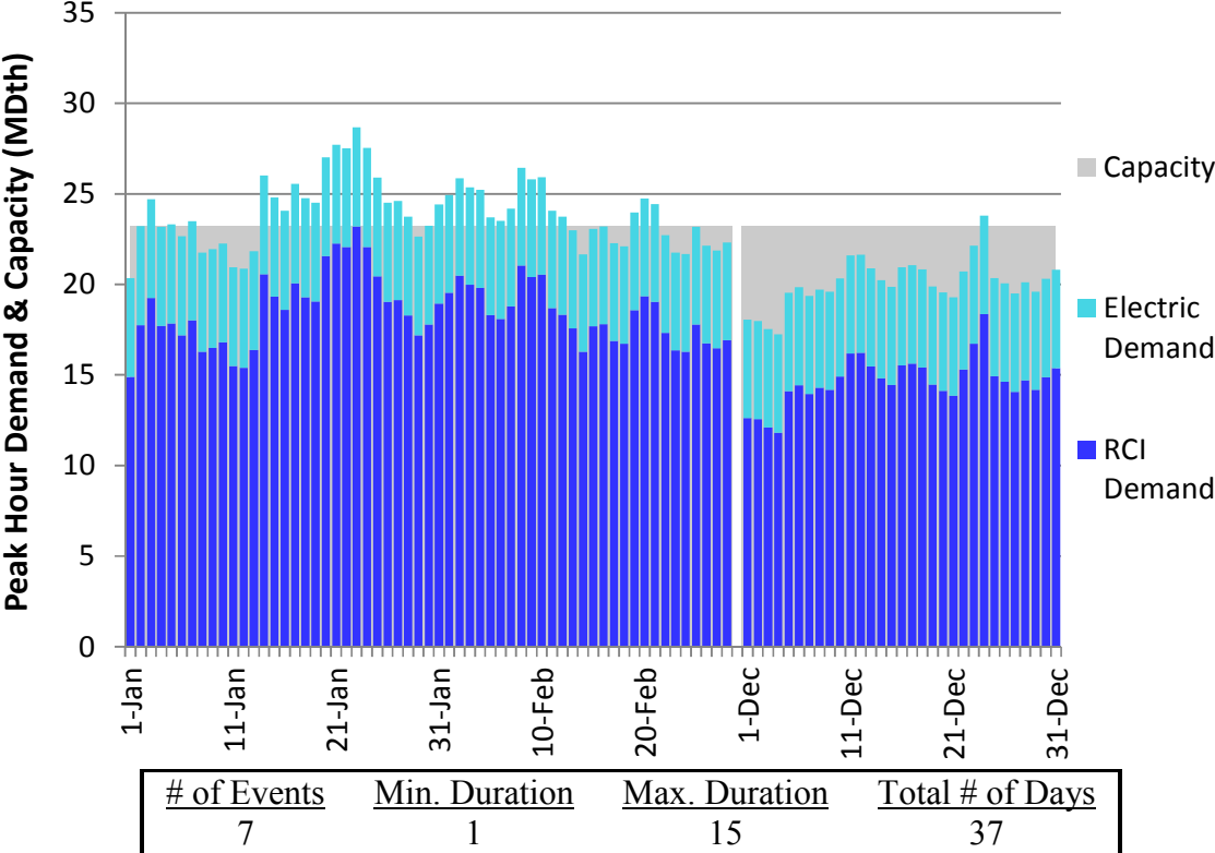
Figure J368. HGDS S0 Winter 2023 – Dominion Western NY– Descending Demand
