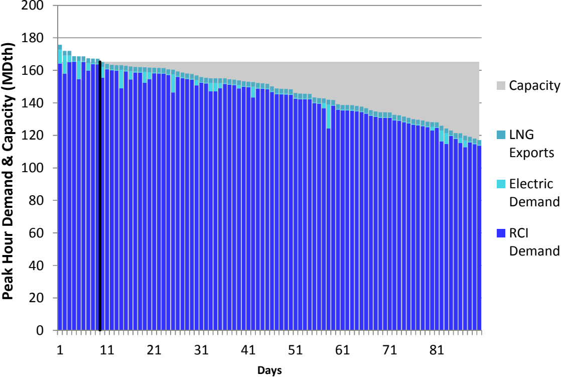
Figure J90. RGDS S5a Winter 2023 – Transco Z5 – Descending Demand
