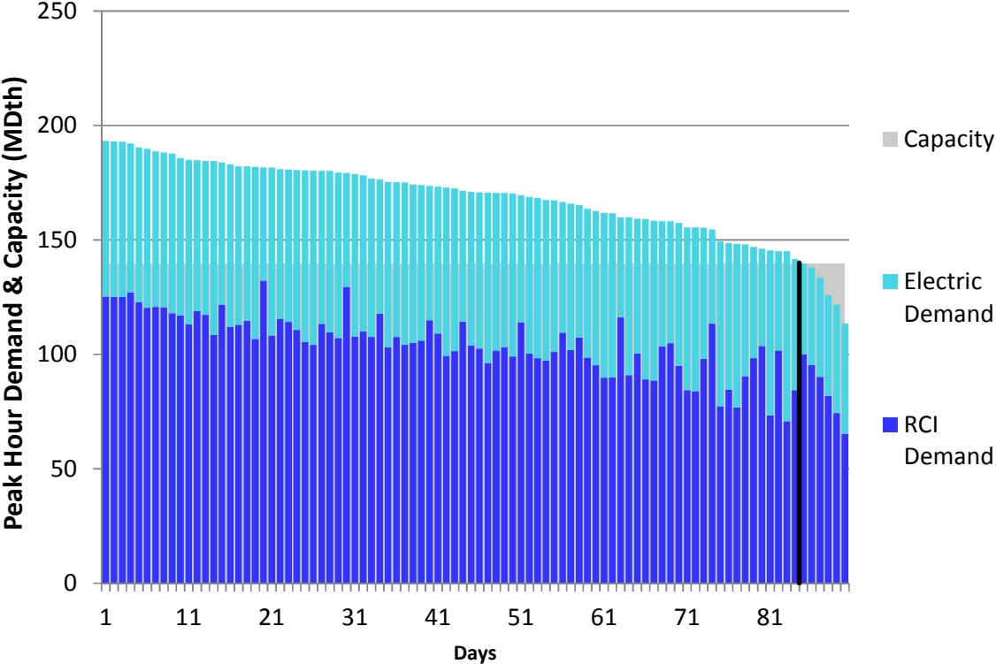
Figure J404. HGDS S0 Winter 2023 – Texas Eastern M3 North – Descending Demand
