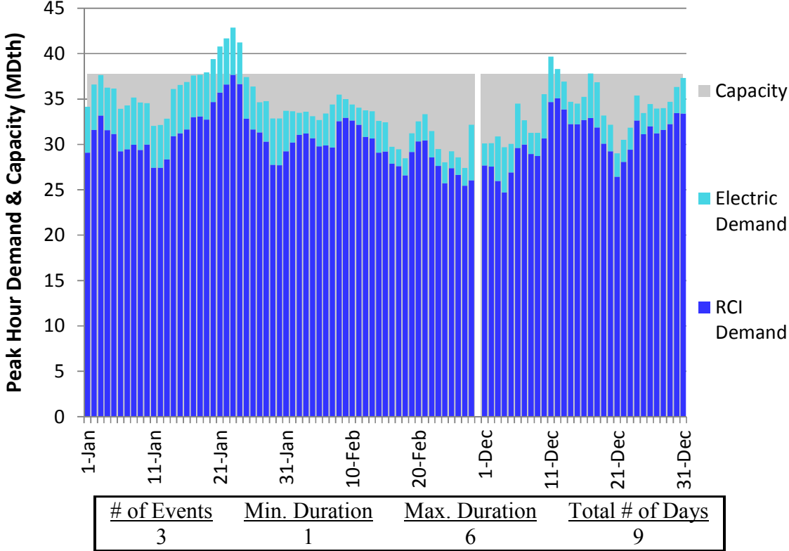
Figure J8. RGDS S5a Winter 2018 – Dominion Eastern NY– Descending Demand
