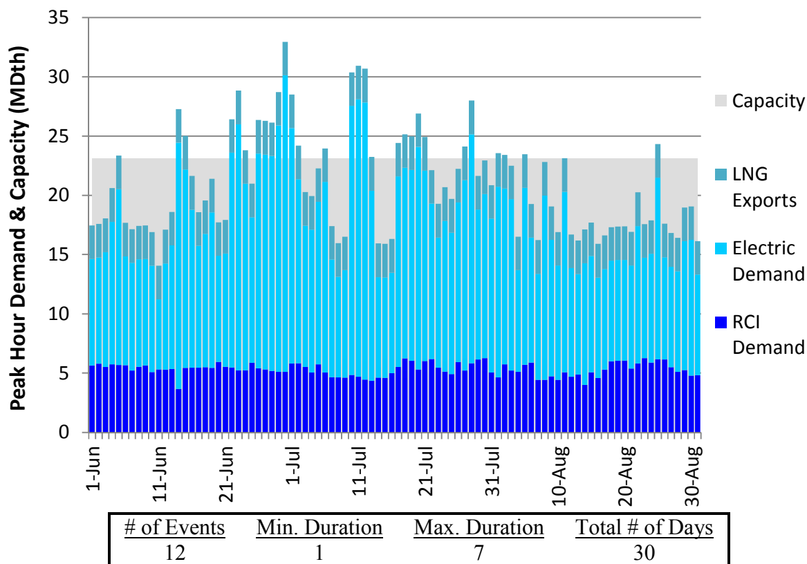
Figure J100. RGDS S5a Summer 2023 – Dominion Southeast – Descending Demand
