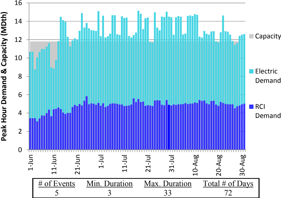
Figure J162. RGDS S5b Summer 2023 – NB/NS – Descending Demand
