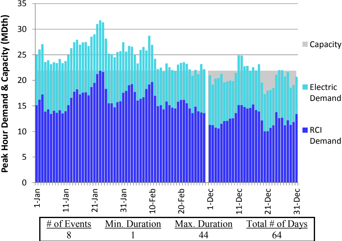
Figure J238. RGDS S5c Winter 2023 – Empire – Descending Demand
