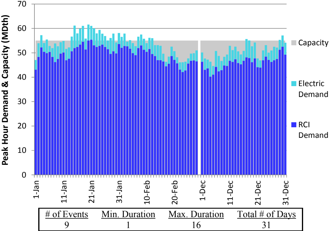
Figure J202. RGDS S5c Winter 2018 – TransCanada Quebec – Descending Demand
