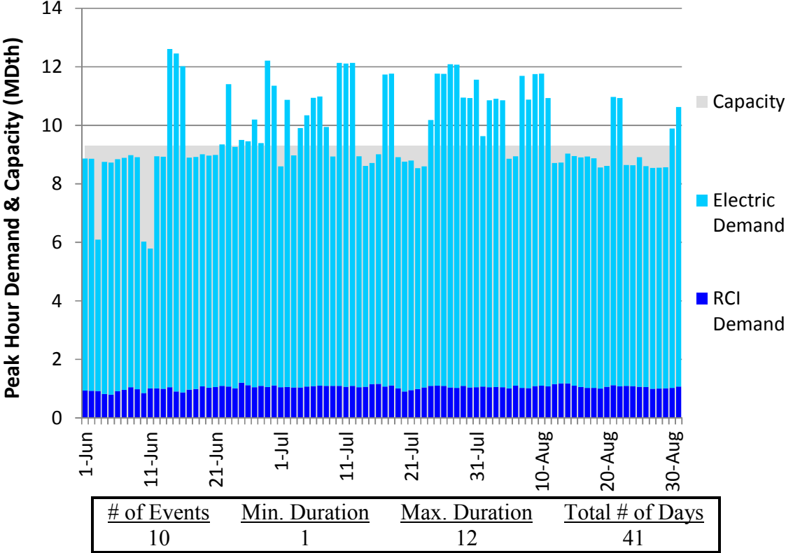
Figure J274. RGDS S5c Summer 2023 – PNGTS N of Westbrook – Descending Demand
