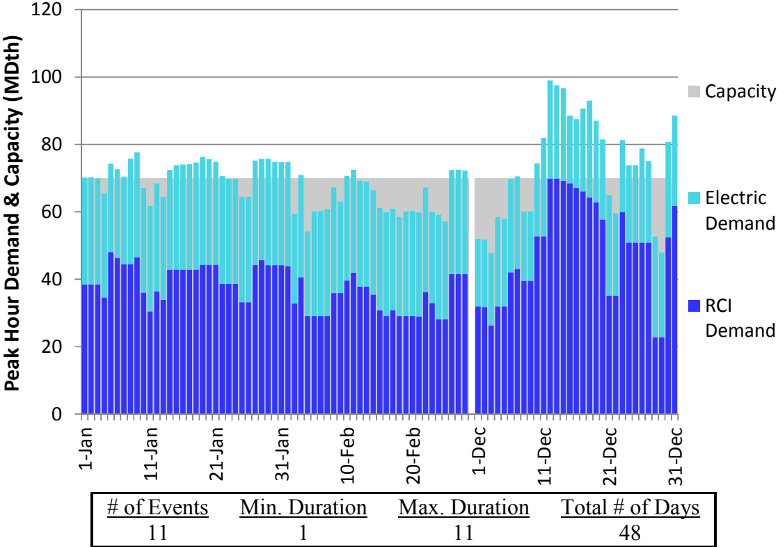
Figure J312. HGDS S9 Winter 2018 – NGPL IA/IL South – Descending Demand
