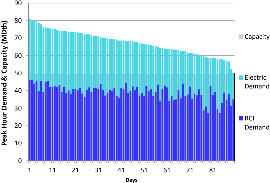
Figure J136. RGDS S5b Winter 23 – Tennessee Z5 NY – Descending Demand
