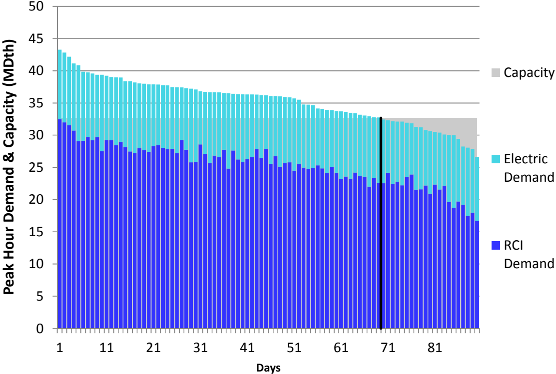
Figure J72. RGDS S5a Winter 2023 – Millennium – Descending Demand
