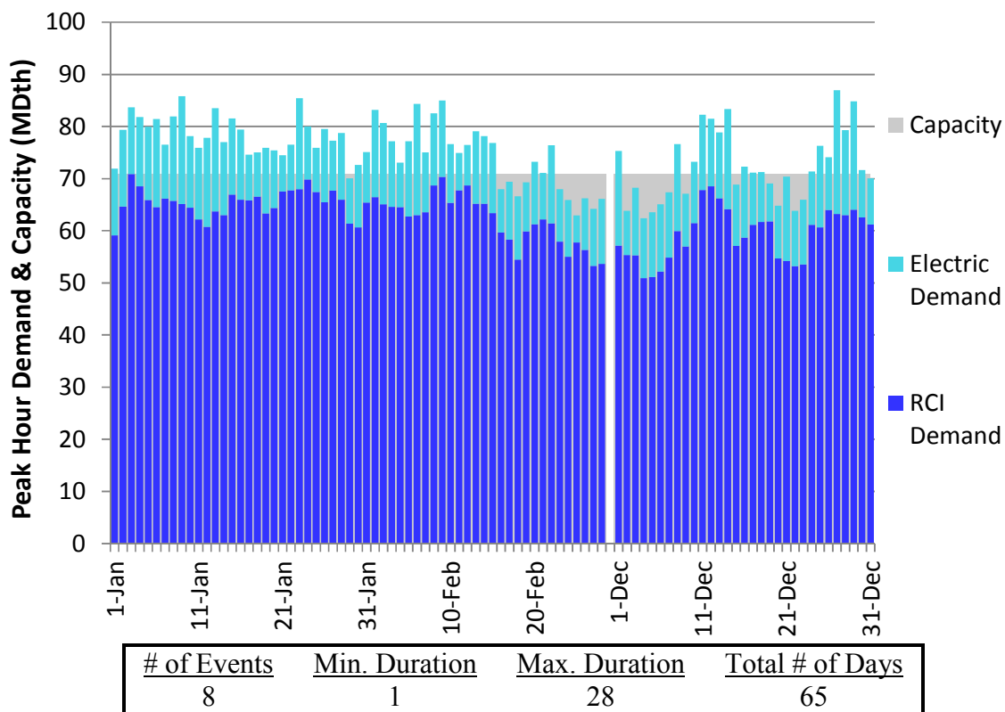
Figure J256. RGDS S5c Winter 2023 – Transco Leidy Atlantic – Descending Demand
