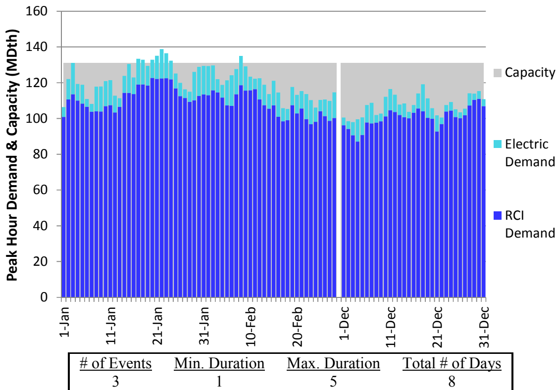
Figure J326. HGDS S9 Winter 2018 – TransCanada Ontario West – Descending Demand
