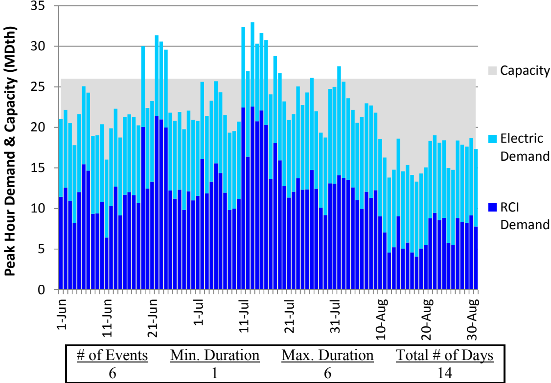
Figure J50. RGDS S5a Summer 2018 – Texas Eastern ETX – Descending Demand
