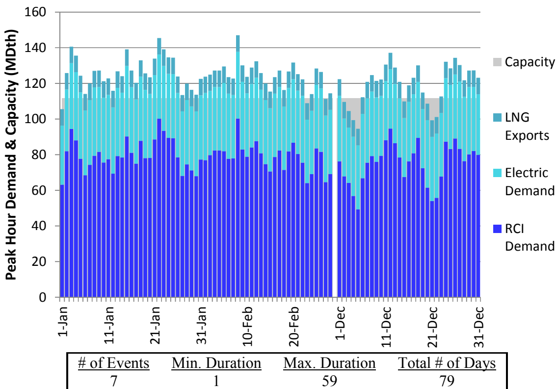
Figure J54. RGDS S5a Winter 2023 – Columbia Gas VA/MD – Descending Demand
