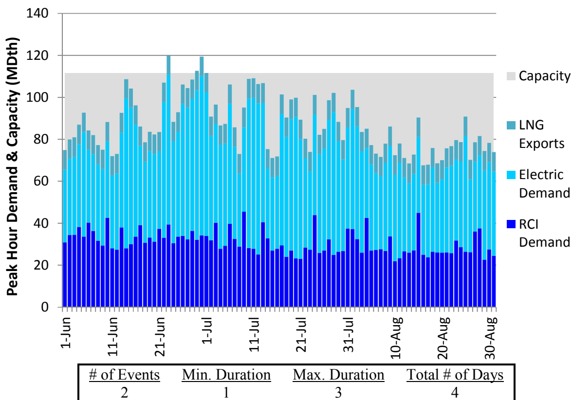
Figure J98. RGDS S5a Summer 2023 – Columbia Gas VA/MD – Descending Demand
