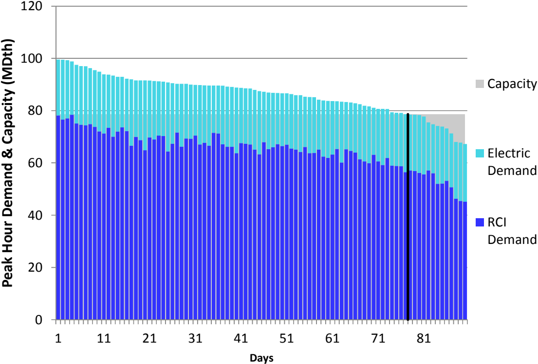
Figure J398. HGDS S0 Winter 2023 – Tennessee Z4 PA – Descending Demand
