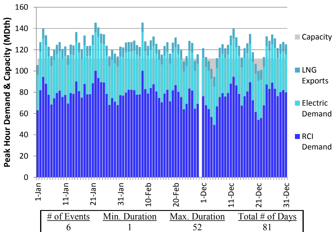
Figure J112. RGDS S5b Winter 2023 – Columbia Gas VA/MD – Descending Demand
