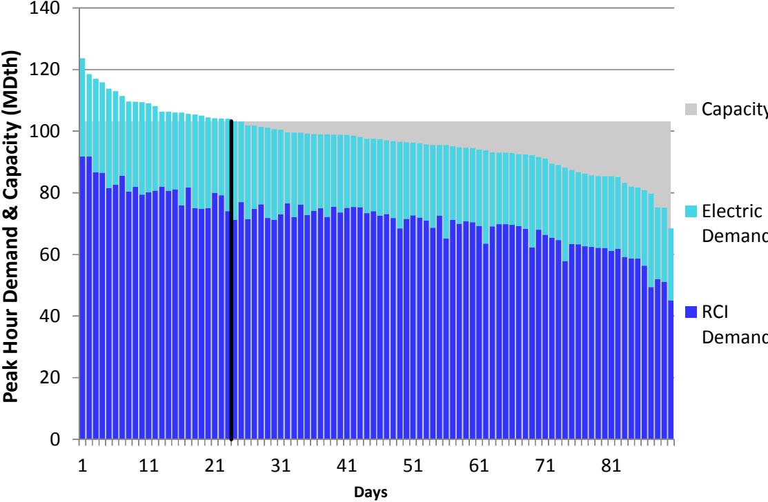
Figure J170. RGDS S5c Winter 2018 – Columbia Gas VA/MD – Descending Demand
