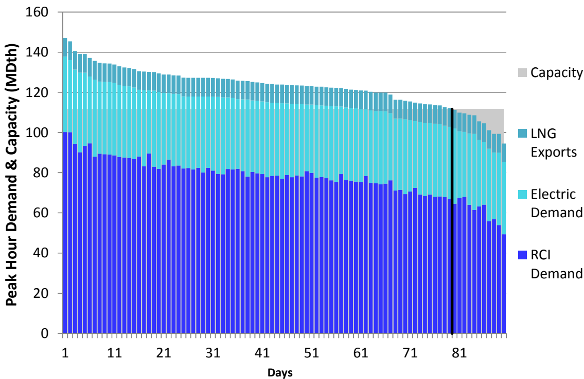
Figure J54. RGDS S5a Winter 2023 – Columbia Gas VA/MD – Descending Demand
