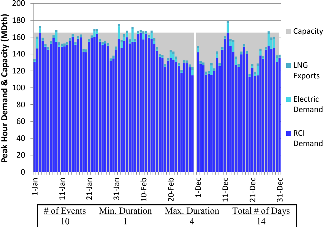
Figure J258. RGDS S5c Winter 2023 – Transco Z5 – Descending Demand
