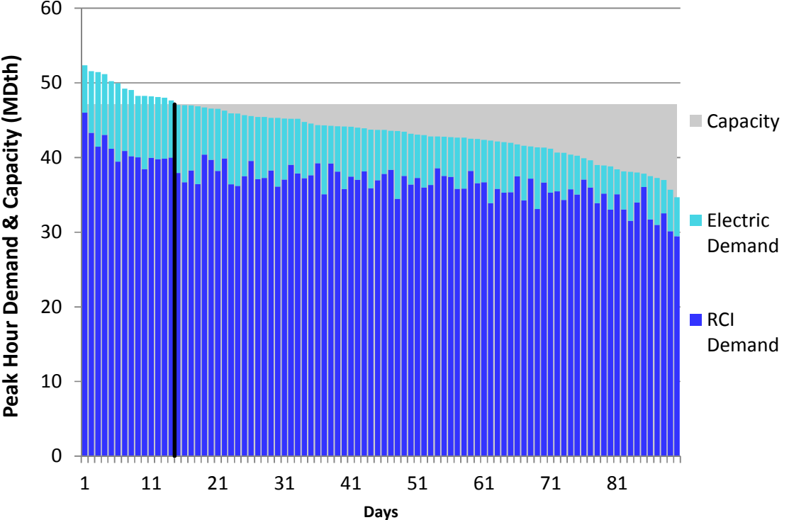
Figure J4. RGDS S5a Winter 2018 – Columbia Gas W PA/NY – Descending Demand
