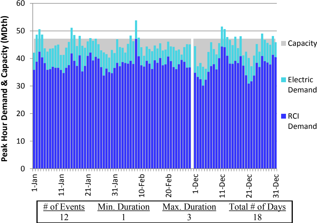
Figure J114. RGDS S5b Winter 2023 – Columbia Gas W PA/NY – Descending Demand
