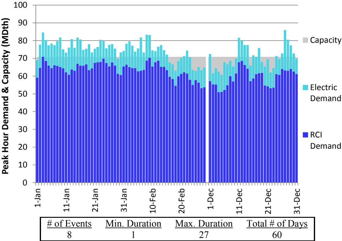
Figure J146. RGDS S5b Winter 2023 – Transco Leidy Atlantic – Descending Demand
