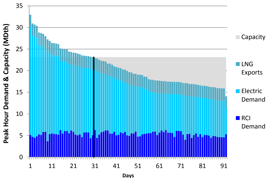
Figure J100. RGDS S5a Summer 2023 – Dominion Southeast – Descending Demand
