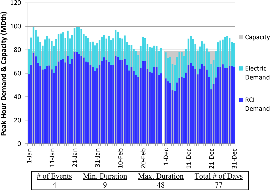
Figure J398. HGDS S0 Winter 2023 – Tennessee Z4 PA – Descending Demand
