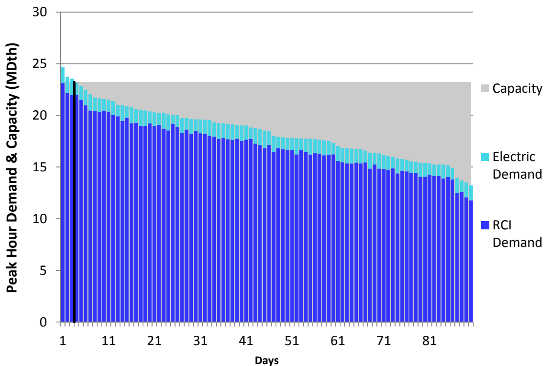
Figure J10. RGDS S5a Winter 2018 – Dominion Western NY– Descending Demand
