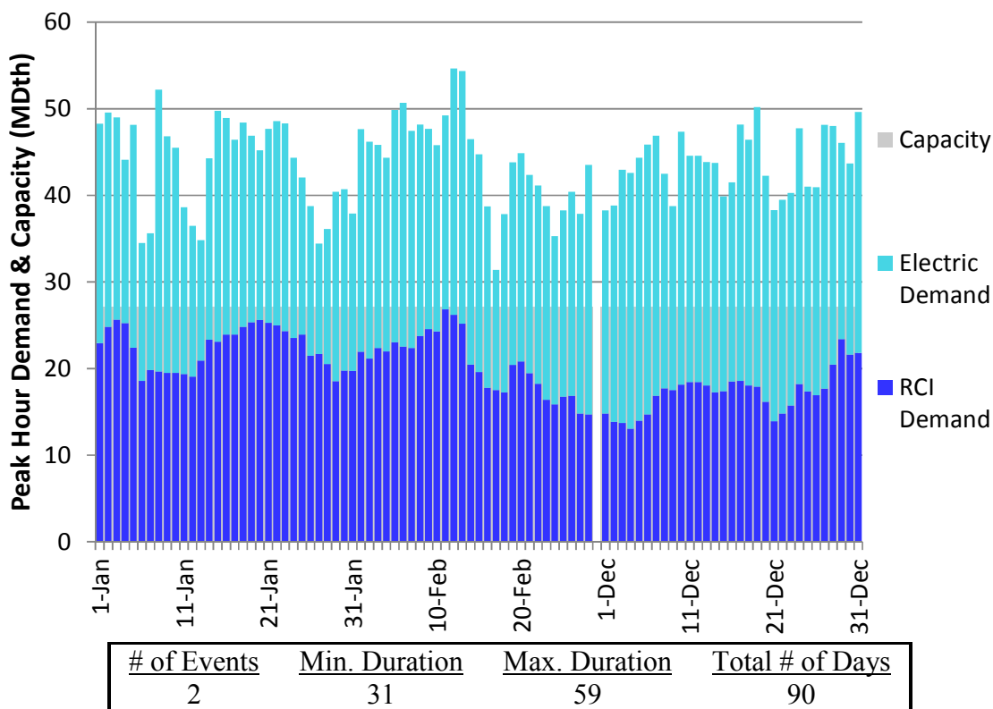
Figure J174. RGDS S5c Winter 2018 – Constitution – Descending Demand
