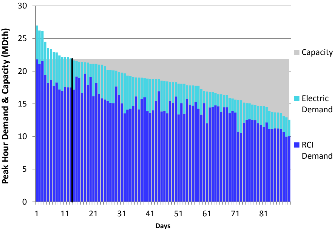
Figure J18. RGDS S5a Winter 2018 – Empire – Descending Demand
