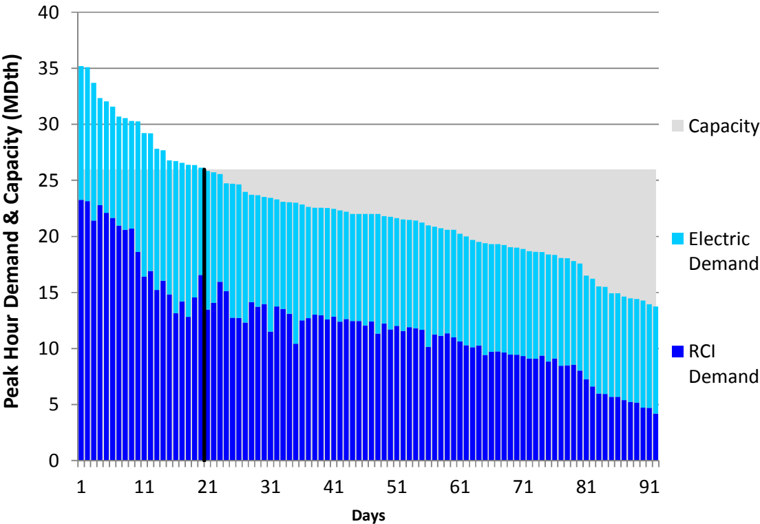
Figure J276. RGDS S5c Summer 2023 – Texas Eastern ETX – Descending Demand
