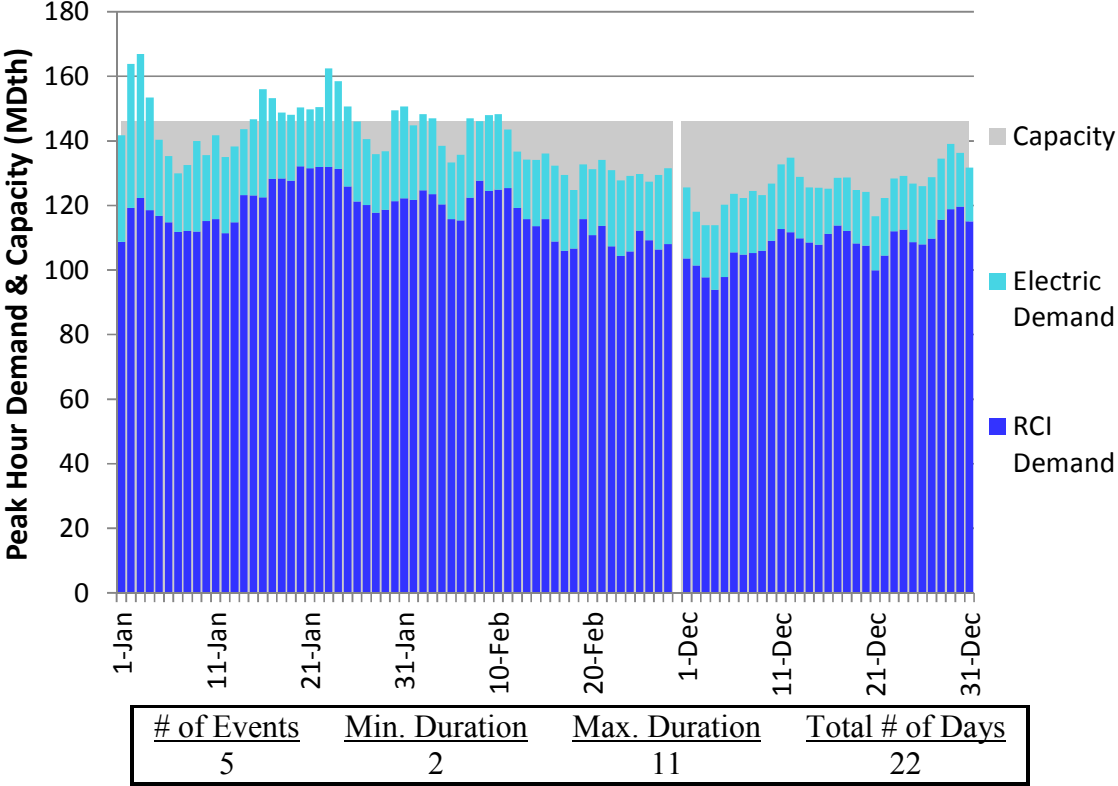
Figure J406. HGDS S0 Winter 2023 – TransCanada Ontario West – Descending Demand
