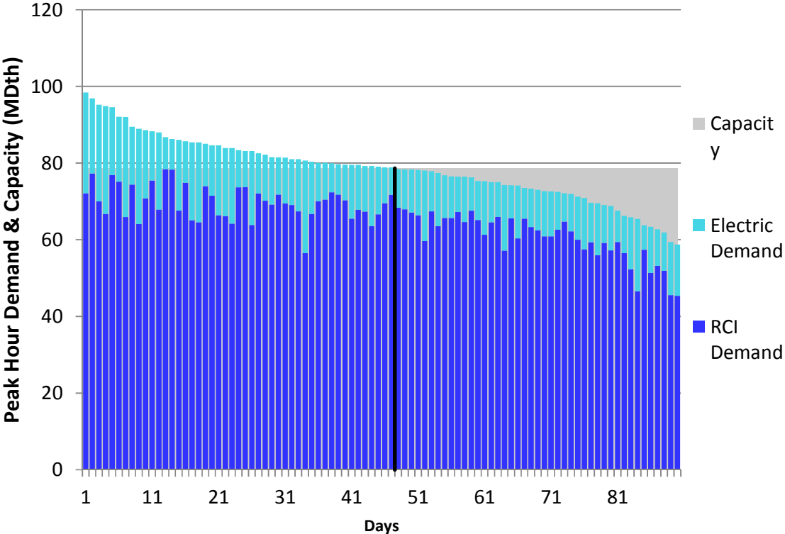
Figure J244. RGDS S5c Winter 2023 – Tennessee Z4 PA – Descending Demand
