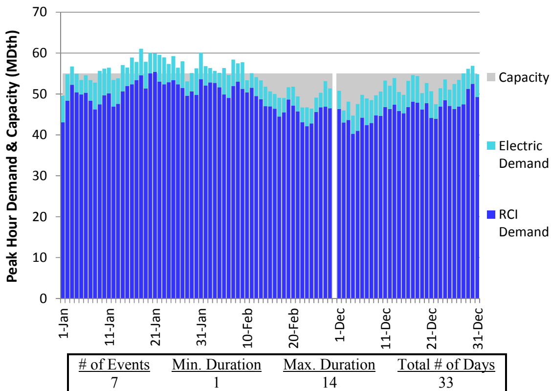
Figure J254. RGDS S5c Winter 2023 – TransCanada Quebec – Descending Demand
