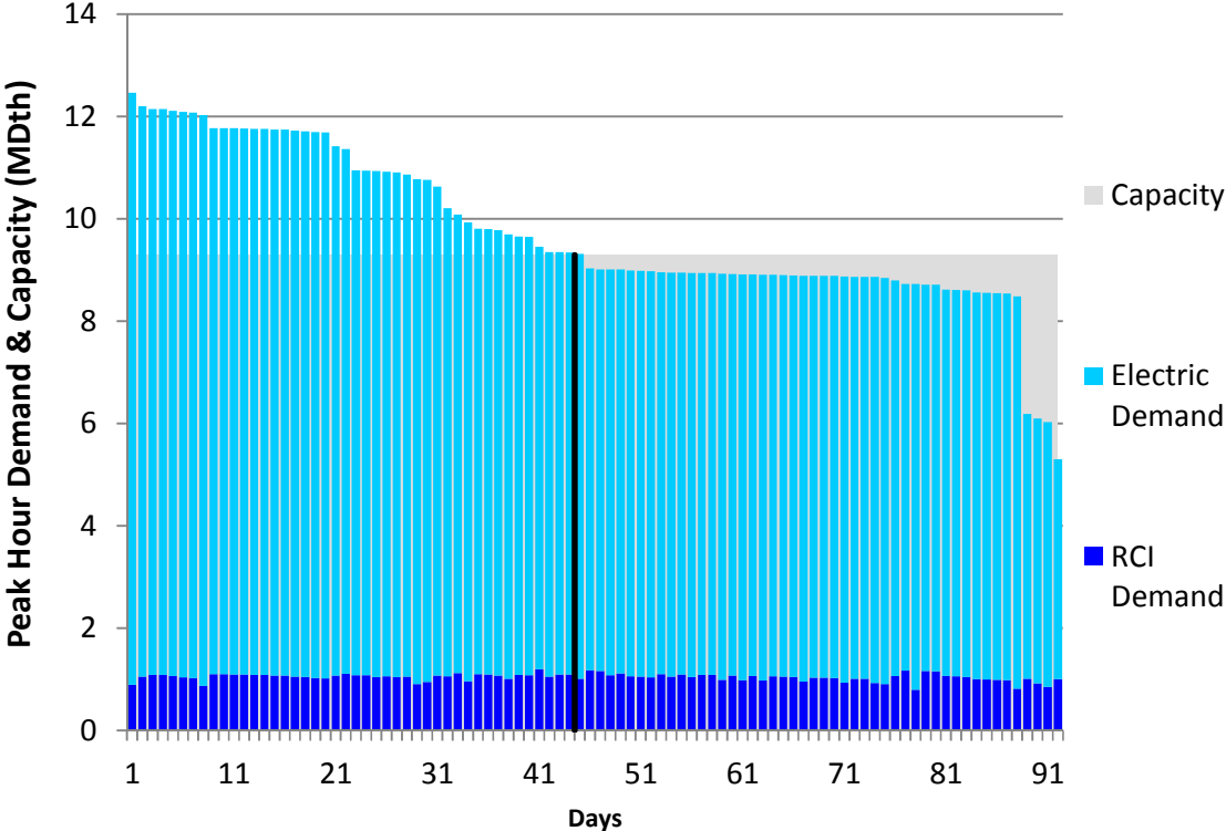
Figure J164. RGDS S5b Summer 2023 – PNGTS N of Westbrook – Descending Demand
