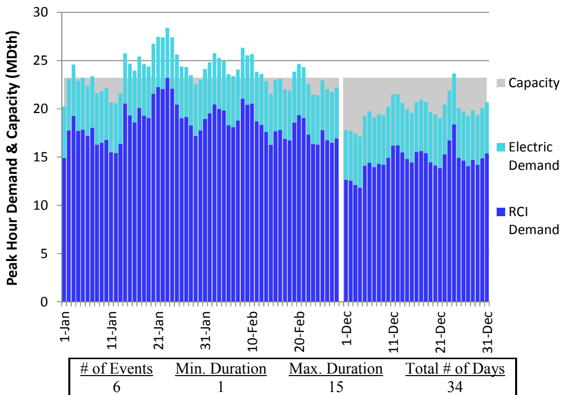
Figure J292. HGDS S9 Winter 2018 – Dominion Western NY– Descending Demand
