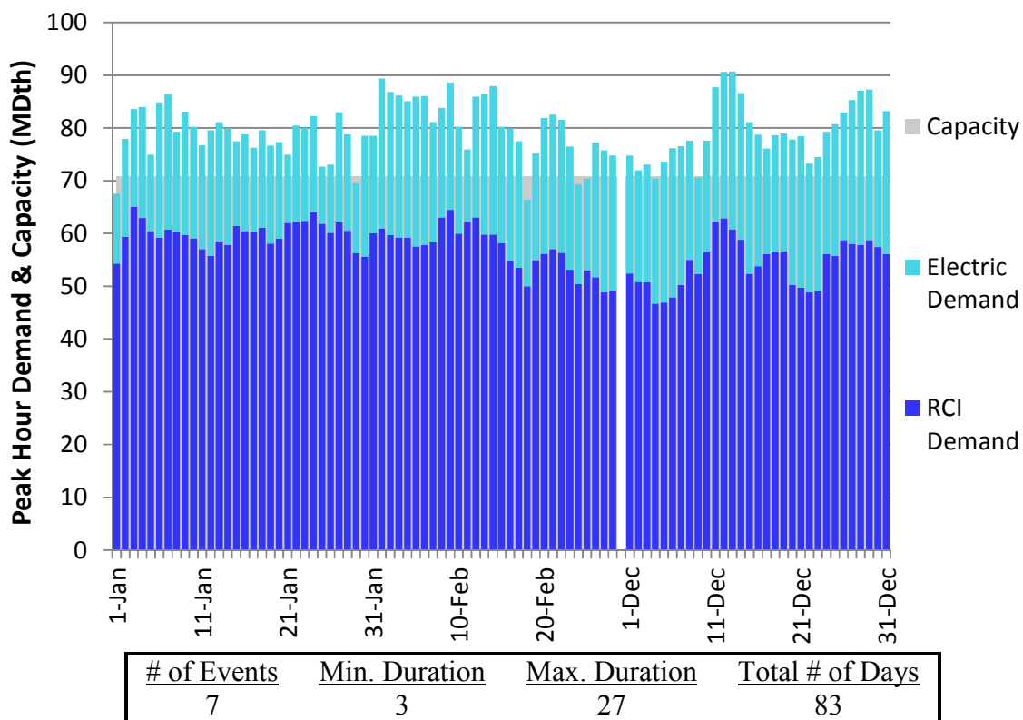
Figure J410. HGDS S0 Winter 2023 – Transco Leidy Atlantic – Descending Demand
