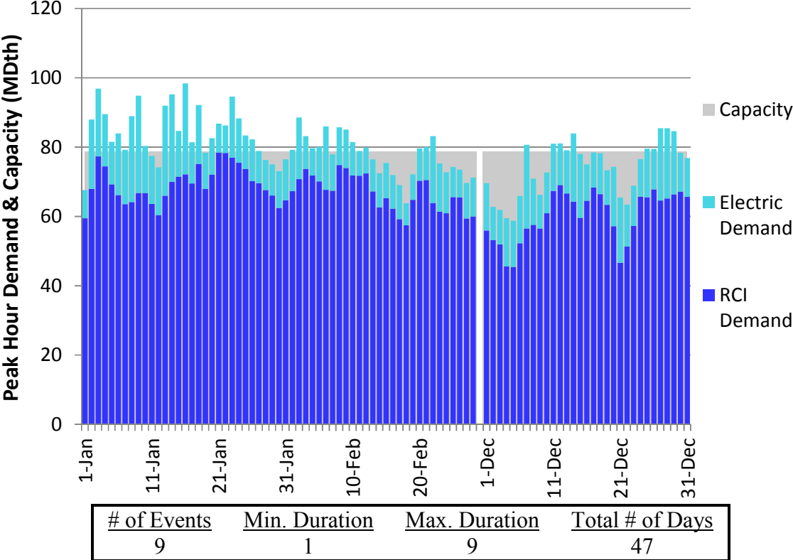
Figure J244. RGDS S5c Winter 2023 – Tennessee Z4 PA – Descending Demand
