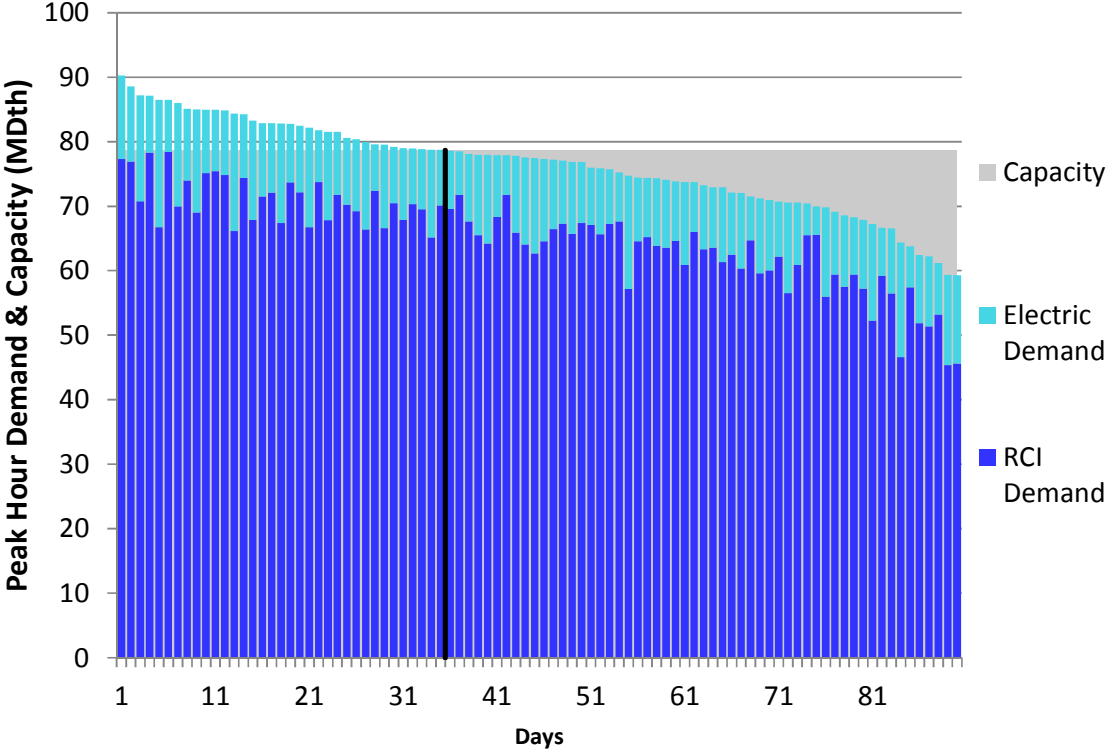
Figure J76. RGDS S5a Winter 2023 – Tennessee Z4 PA – Descending Demand
