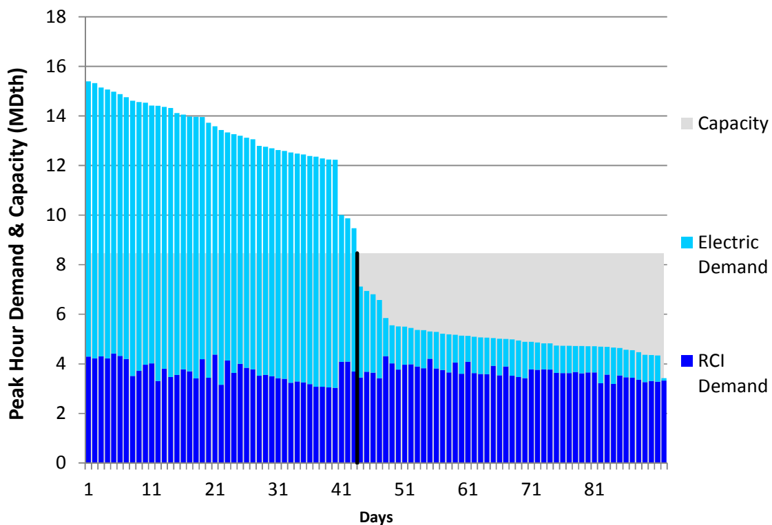
Figure J346. HGDS S9 Summer 2018 – Eastern Shore – Descending Demand
