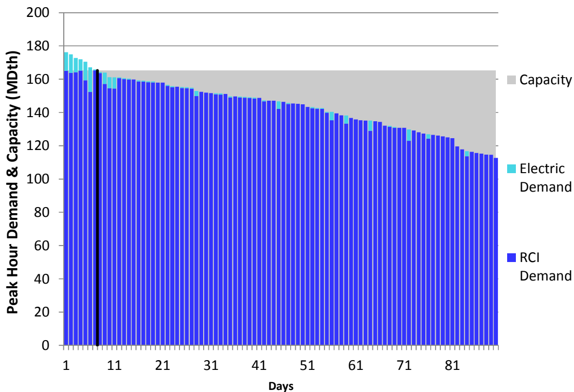
Figure J38. RGDS S5a Winter 2018 – Transco Z5 – Descending Demand
