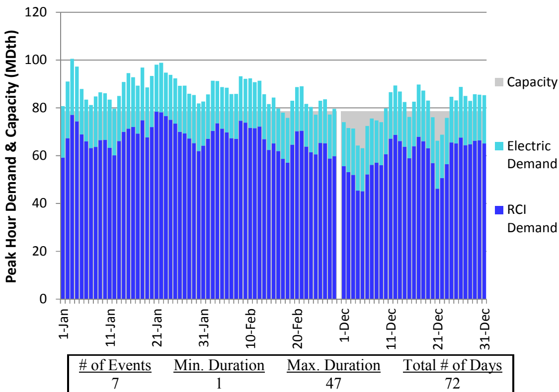
Figure J318. HGDS S9 Winter 2018 – Tennessee Z4 PA – Descending Demand
