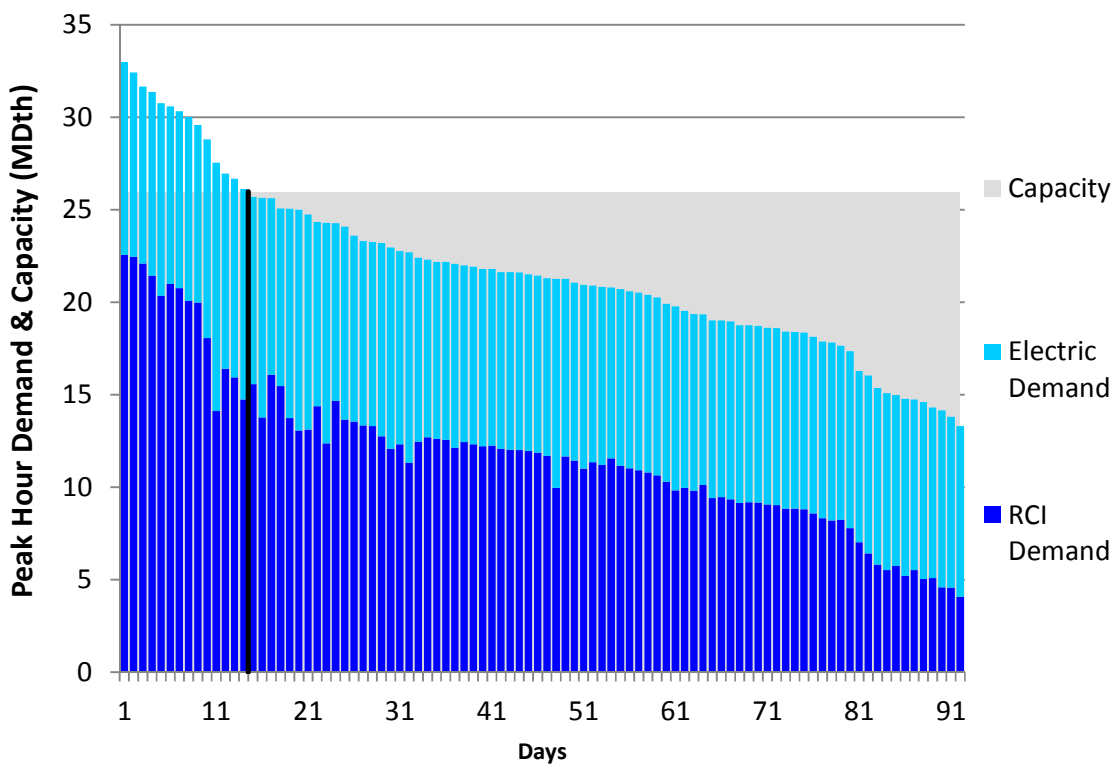
Figure J218. RGDS S5c Summer 2018 – Texas Eastern ETX – Descending Demand
