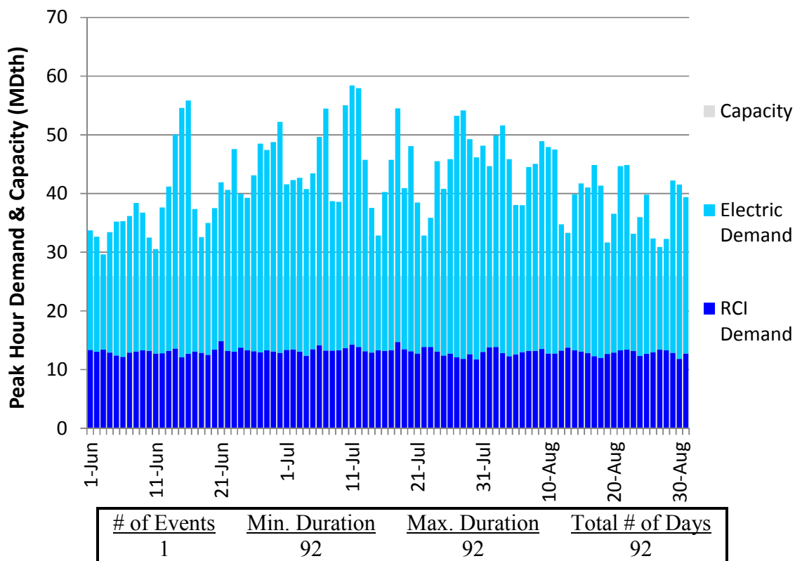
Figure J438. HGDS S0 Summer 2023 – Tennessee Z5 NY – Descending Demand
