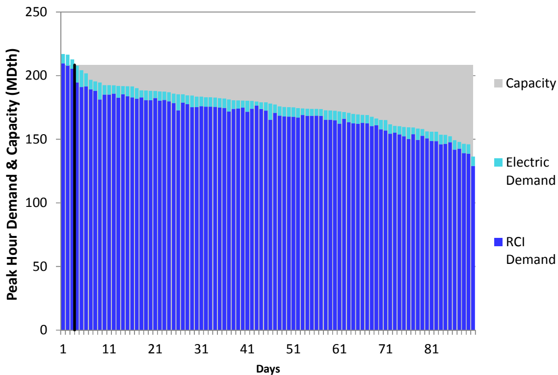
Figure J210. RGDS S5c Winter 2018 – Union Gas Dawn – Descending Demand
