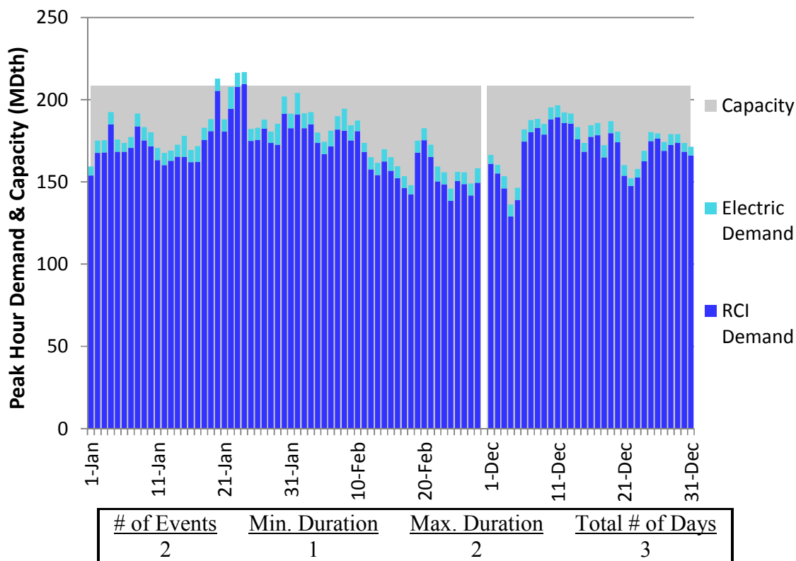
Figure J210. RGDS S5c Winter 2018 – Union Gas Dawn – Descending Demand
