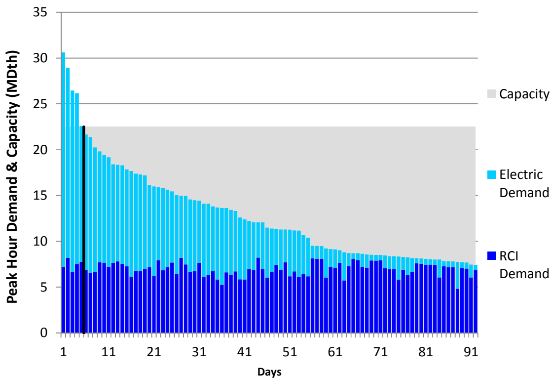
Figure J46. RGDS S5a Summer 2018 – Dominion Southeast – Descending Demand
