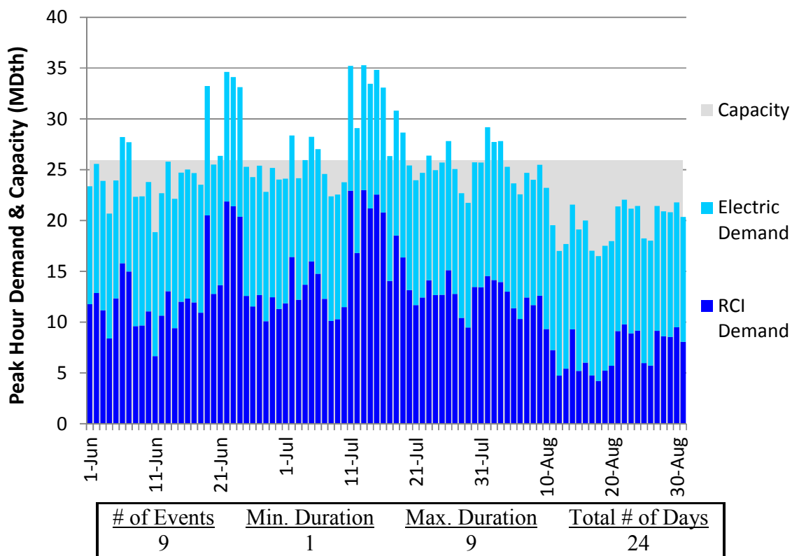
Figure J352. HGDS S9 Summer 2018 – Texas Eastern ETX – Descending Demand
