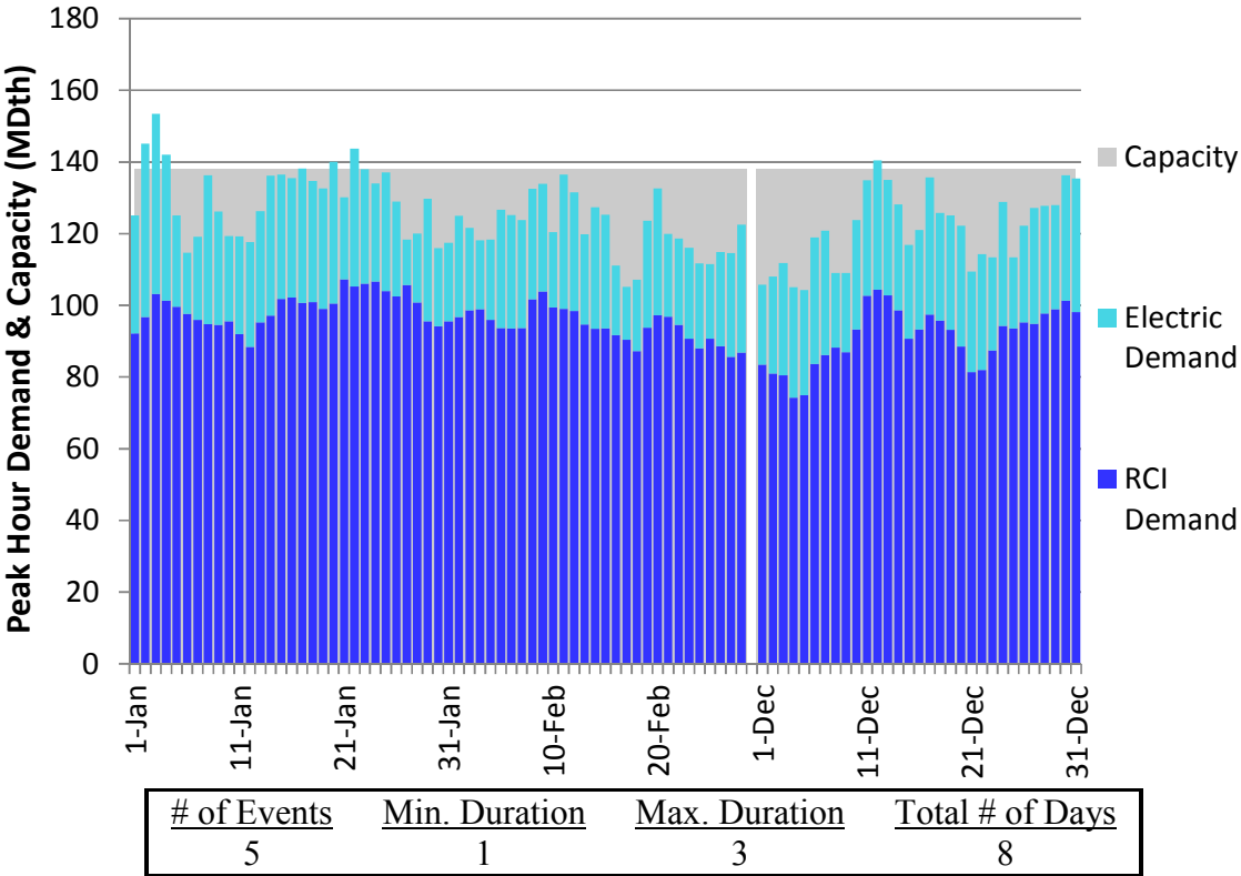
Figure J40. RGDS S5a Winter 2018 – Transco Leidy to Station 210 – Descending Demand
