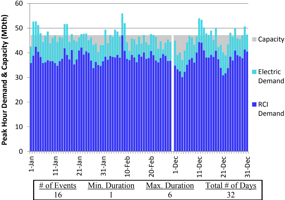
Figure J56. RGDS S5a Winter 2023 – Columbia Gas W PA/NY – Descending Demand
