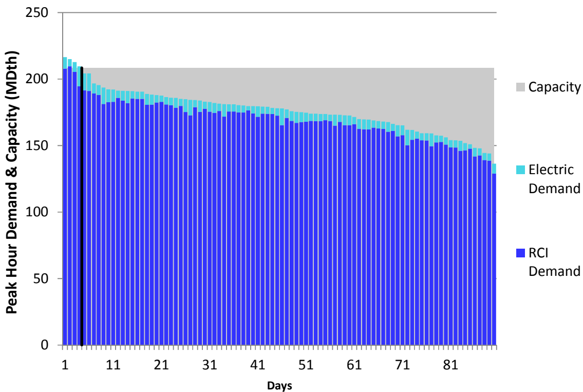
Figure J42. RGDS S5a Winter 2018 – Union Gas Dawn – Descending Demand
