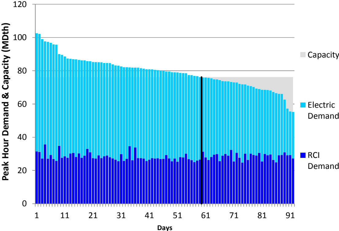
Figure J422. HGDS S0 Summer 2023 – Algonquin CT – Descending Demand
