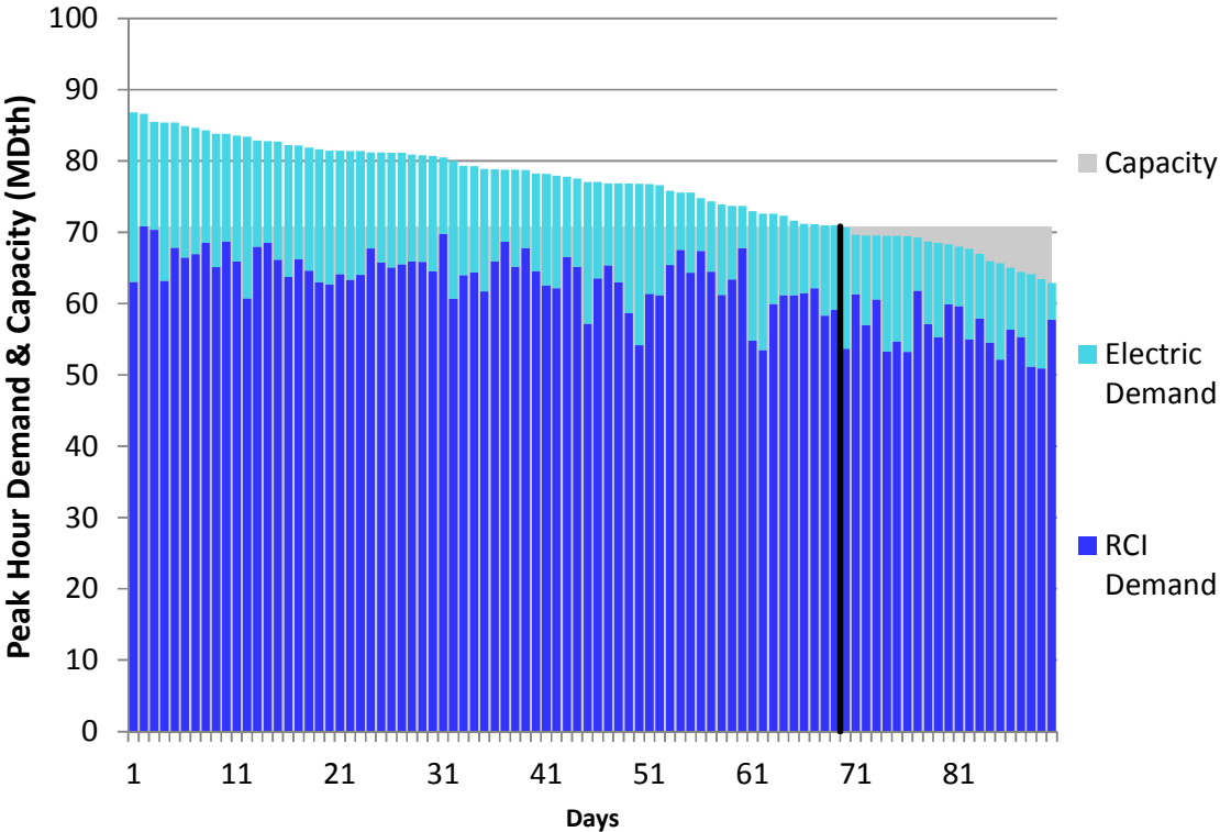
Figure J88. RGDS S5a Winter 2023 – Transco Leidy Atlantic – Descending Demand
