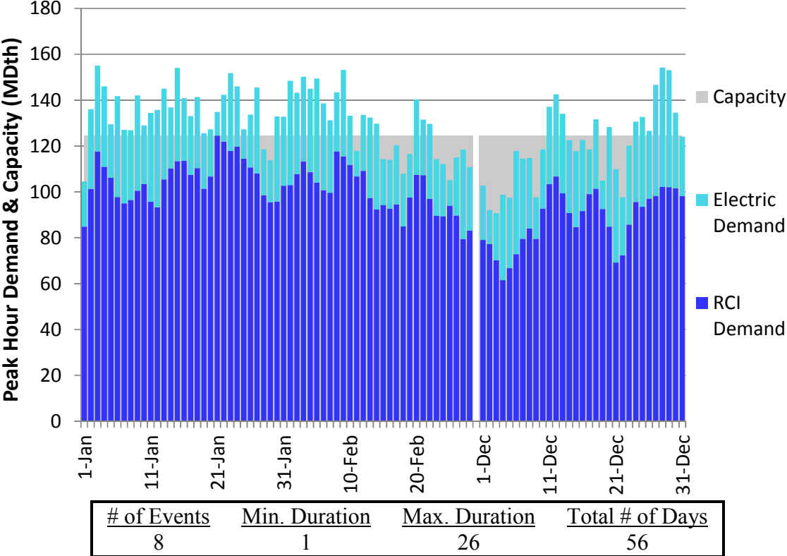
Figure J250. RGDS S5c Winter 2023 – Texas Eastern M3 North – Descending Demand
