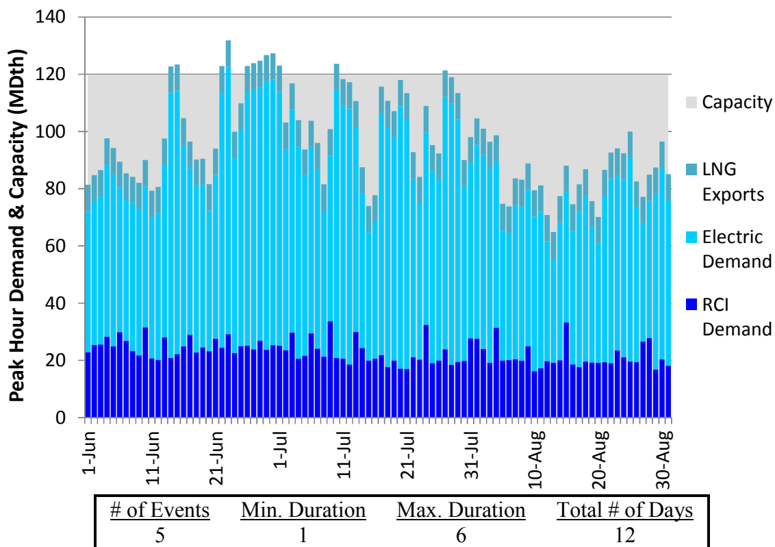
Figure J424. HGDS S0 Summer 2023 – Columbia Gas VA/MD – Descending Demand
