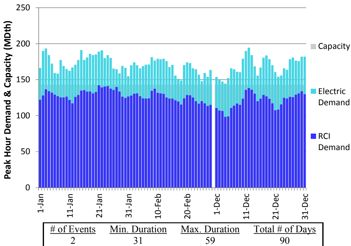
Figure J334. HGDS S9 Winter 2018 – Transco Leidy to Station 210 – Descending Demand
