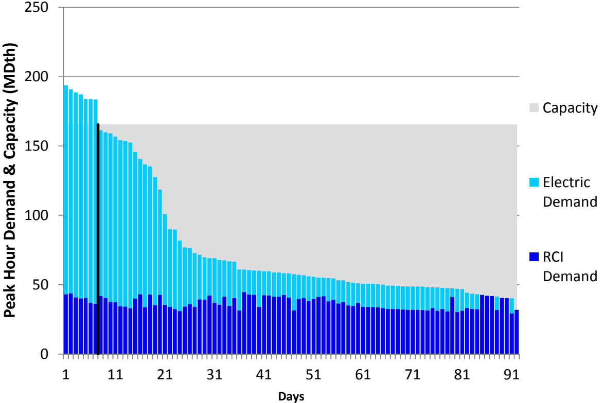
Figure H164. LGDS S2 Summer 2018 – Transco Z5 – Descending Demand
