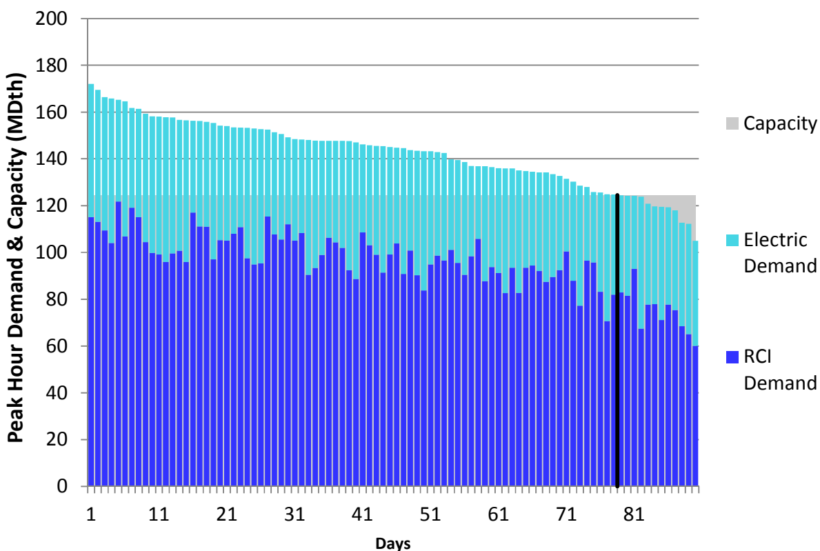
Figure H252. RGDS S3 Winter 2018 – Texas Eastern M3 North – Descending Demand
