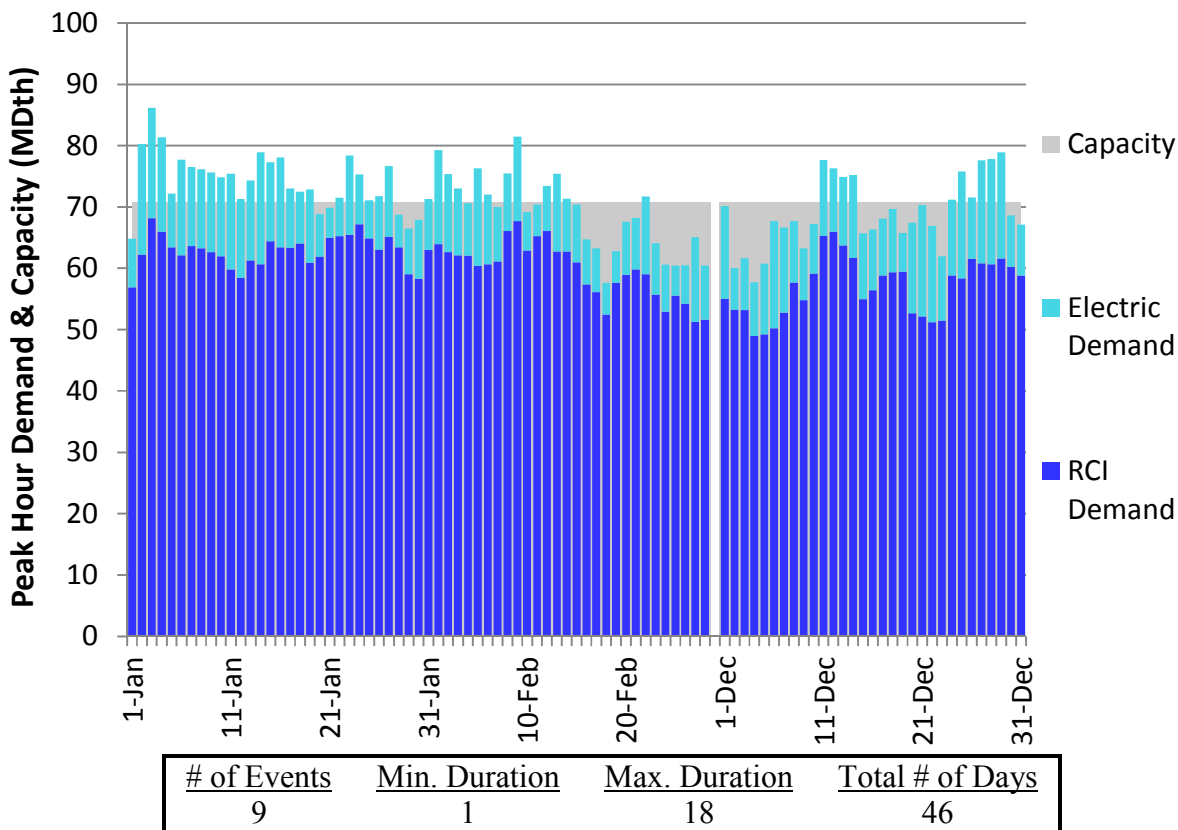
Figure H200. LGDS S2 Winter 2023 – Transco Leidy Atlantic – Descending Demand
