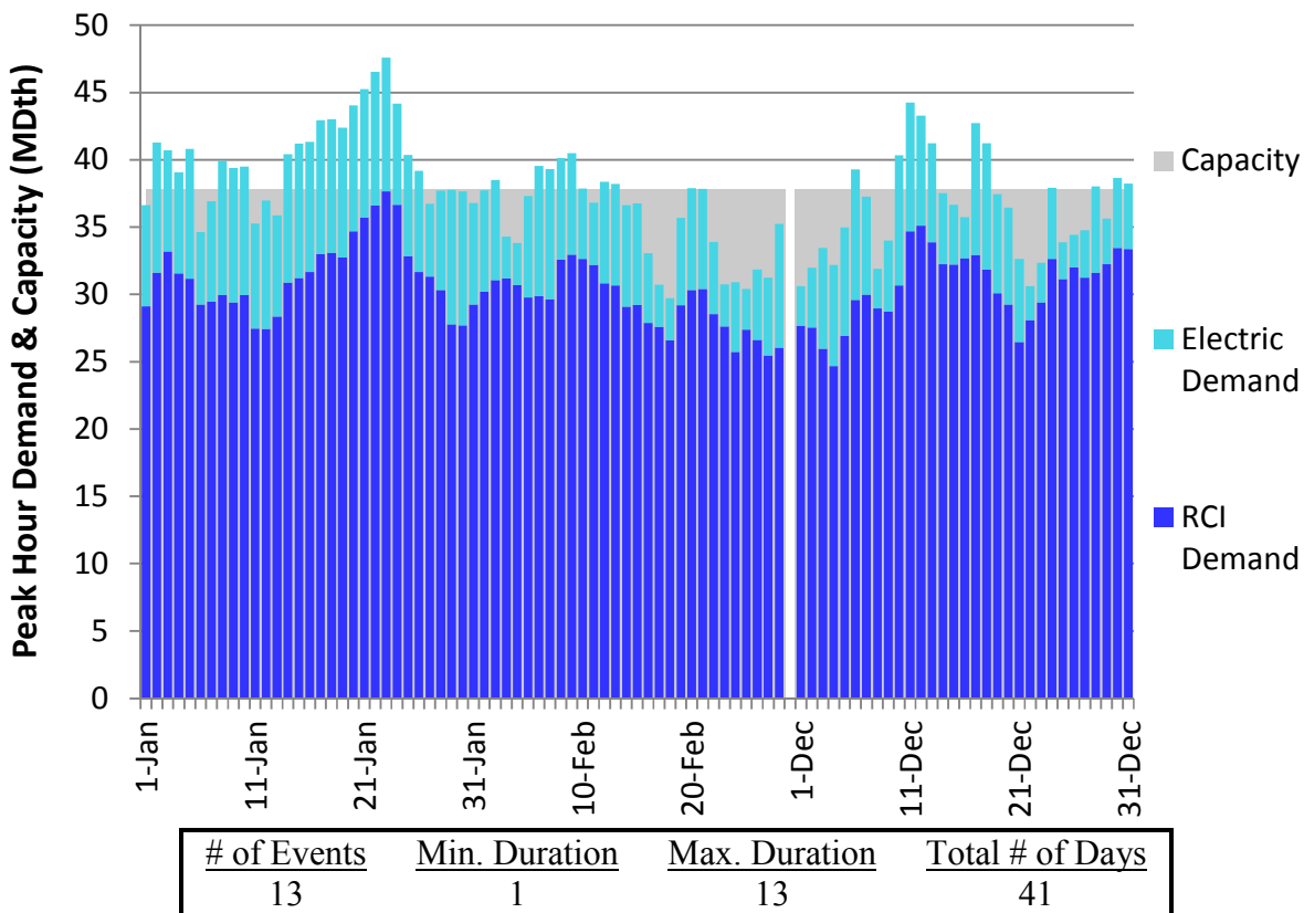
Figure H230. RGDS S3 Winter 2018 – Dominion Eastern NY– Descending Demand
