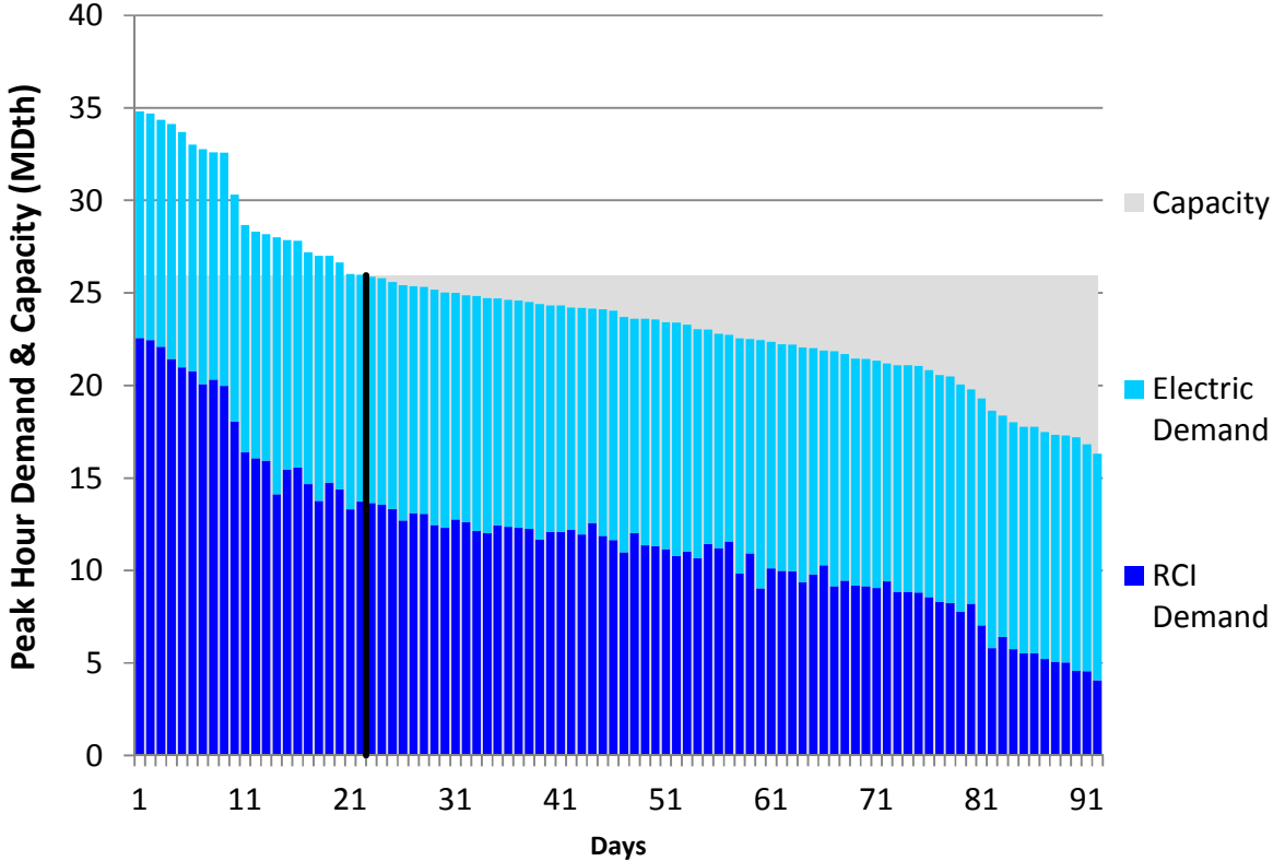
Figure H272. RGDS S3 Summer 2018 – Texas Eastern ETX – Descending Demand
