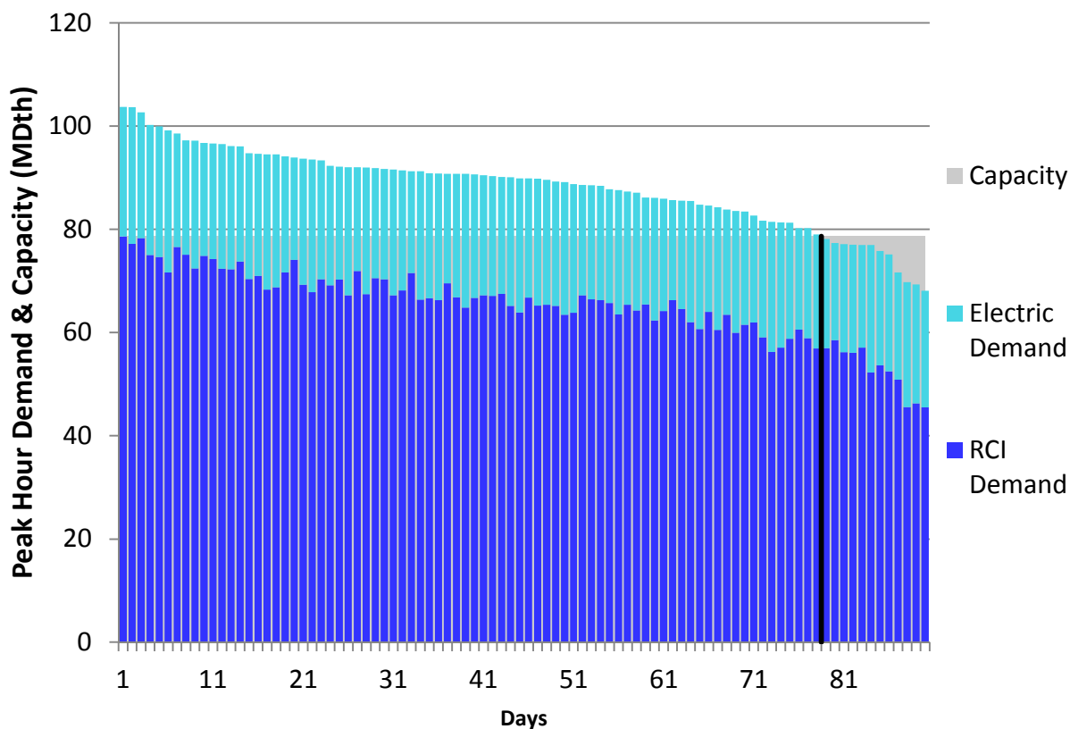
Figure H246. RGDS S3 Winter 2018 – Tennessee Z4 PA – Descending Demand
