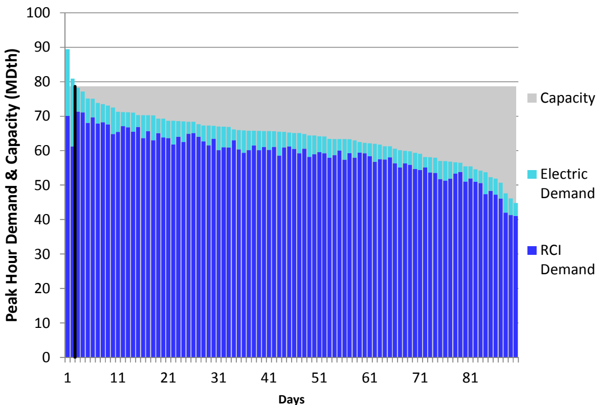
Figure H138. LGDS S2 Winter 2018 – Tennessee Z4 PA – Descending Demand
