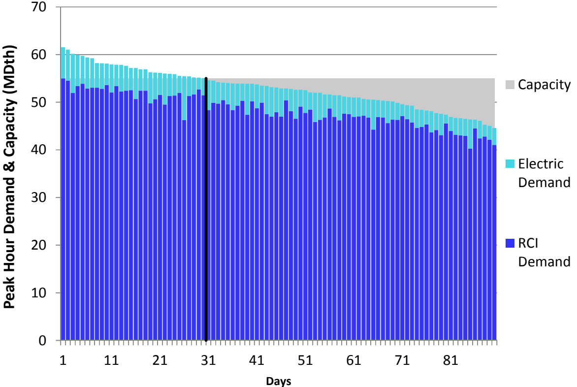
Figure H34. HGDS S2 Winter 2018 – TransCanada Quebec – Descending Demand
