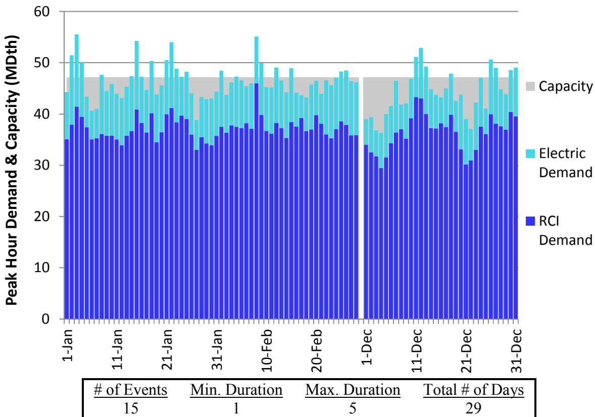
Figure H4. HGDS S2 Winter 2018 – Columbia Gas W PA/NY – Descending Demand
