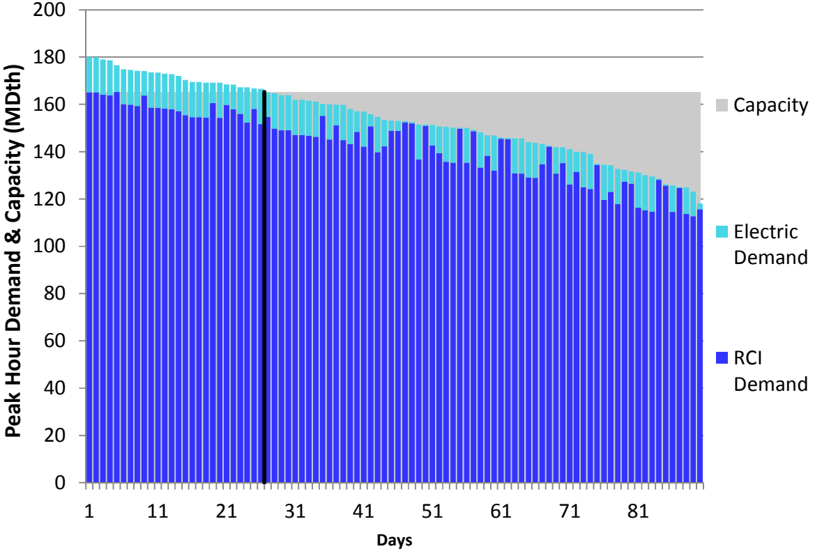
Figure H260. RGDS S3 Winter 2018 – Transco Z5 – Descending Demand
