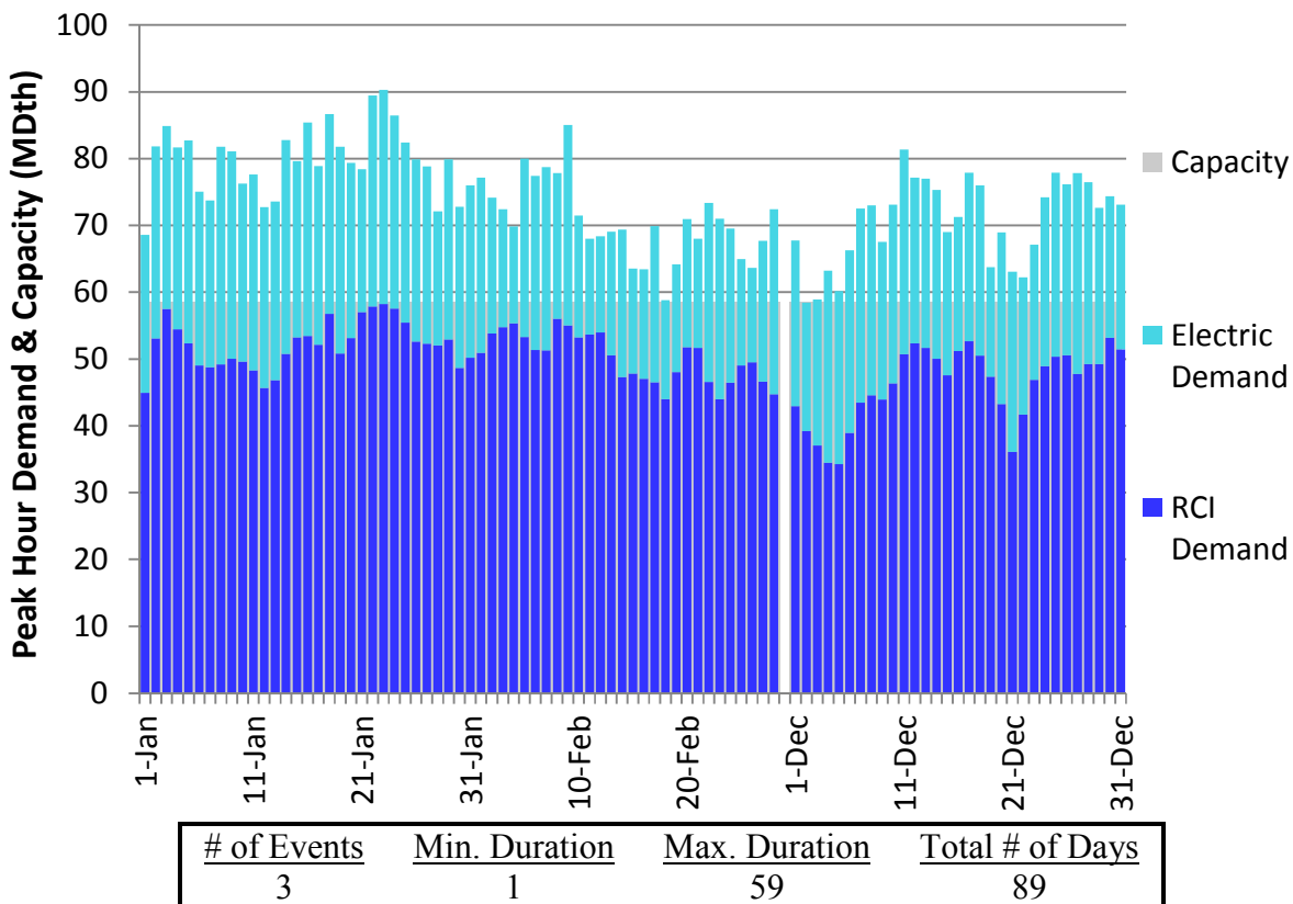
Figure H84. HGDS S2 Winter 2023 – Tennessee Z5 NY – Descending Demand
