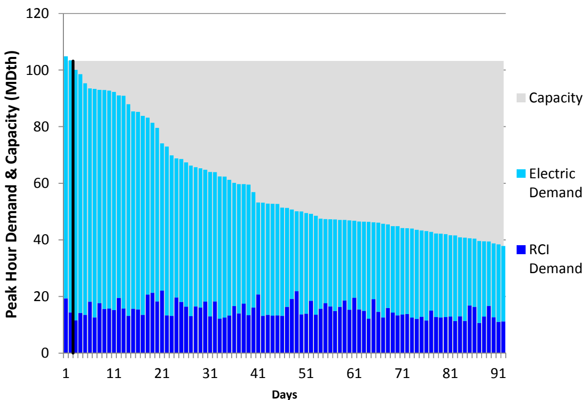
Figure H46. HGDS S2 Summer 2018 – Columbia Gas VA/MD – Descending Demand
