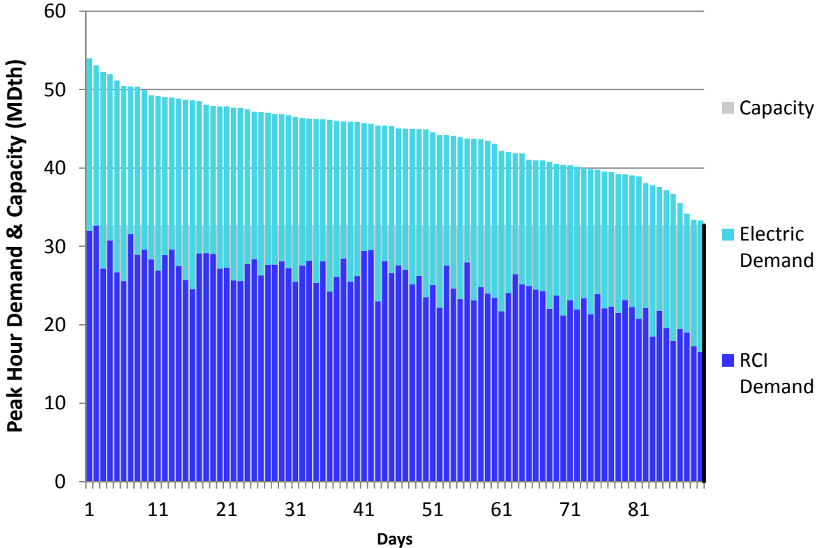
Figure H184. LGDS S2 Winter 2023 – Millennium – Descending Demand
