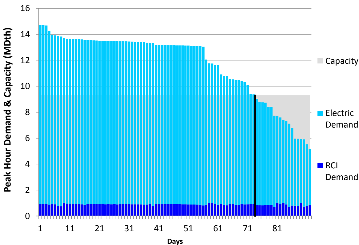
Figure H112. HGDS S2 Summer 2023 – PNGTS N of Westbrook – Descending Demand
