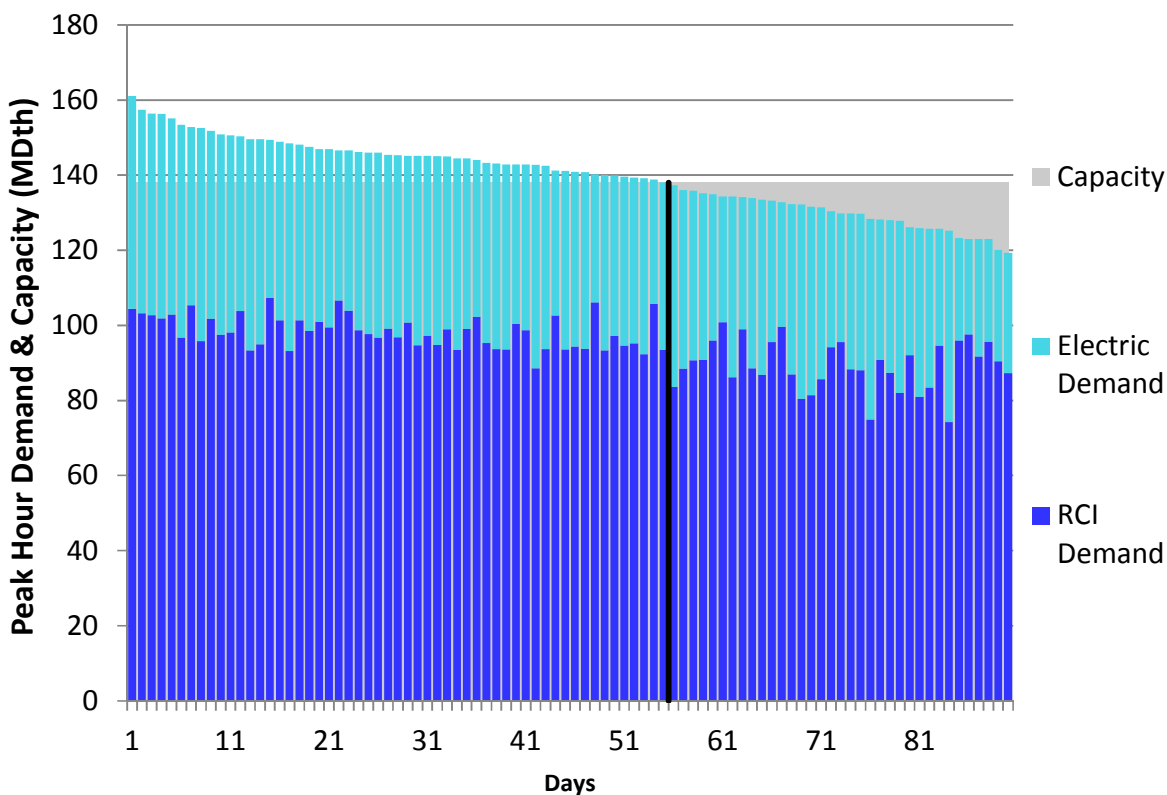
Figure H262. RGDS S3 Winter 2018 – Transco Leidy to Station 210 – Descending Demand
