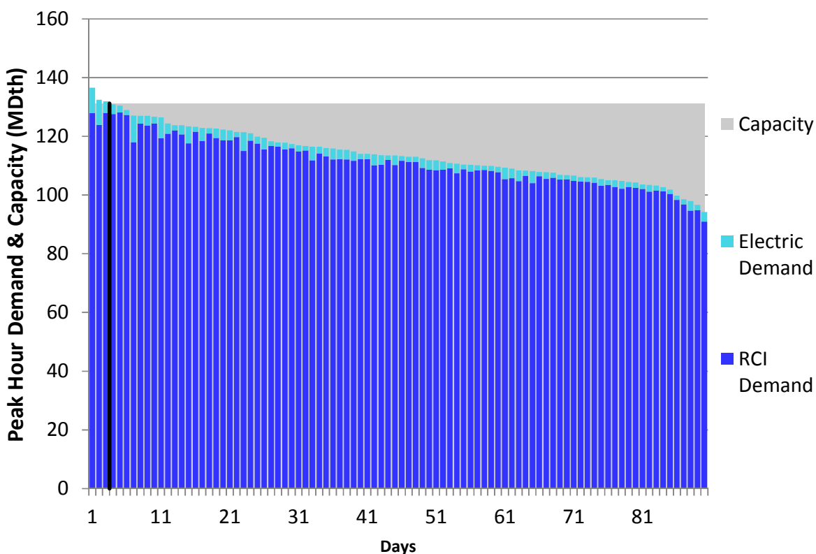
Figure H146. LGDS S2 Winter 2018 – TransCanada Ontario West – Descending Demand
