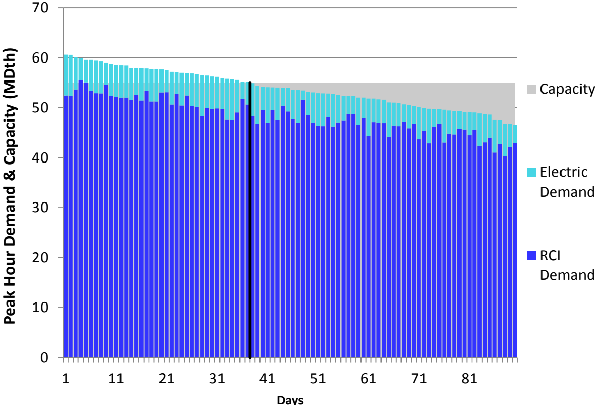
Figure H310. RGDS S3 Winter 2023 – TransCanada Quebec – Descending Demand
