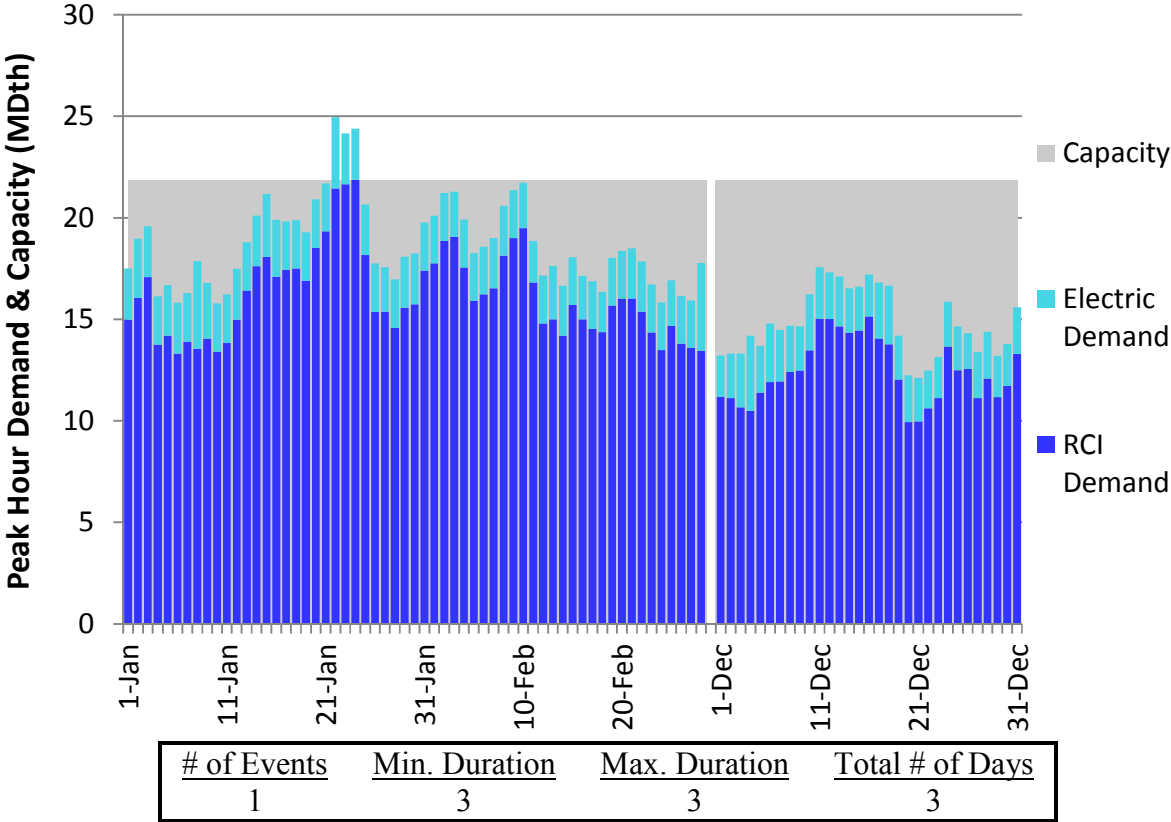
Figure H18. HGDS S2 Winter 2018 – Empire – Descending Demand
