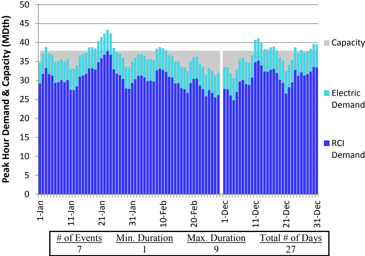
Figure H66. HGDS S2 Winter 2023 – Dominion Eastern NY– Descending Demand
