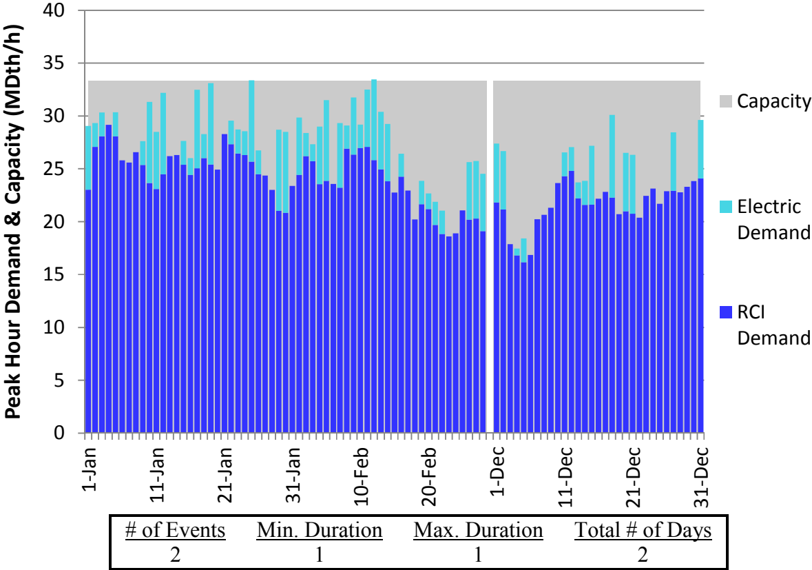
Figure H128. LGDS S2 Winter 2018 – East Tennessee – Descending Demand
