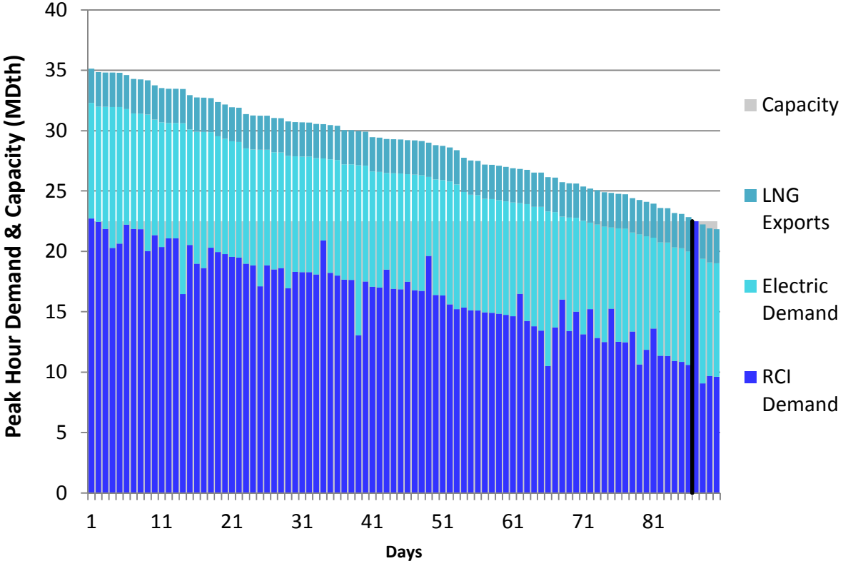
Figure H70. HGDS S2 Winter 2023 – Dominion Southeast – Descending Demand
