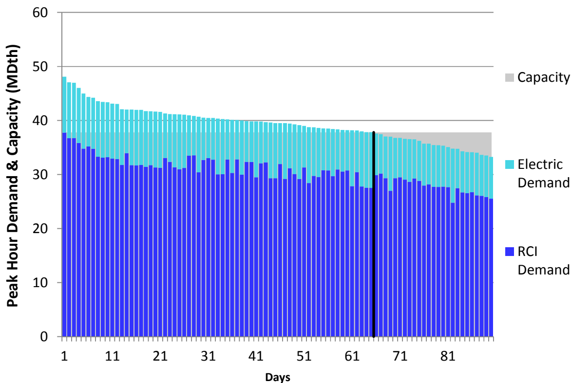
Figure H282. RGDS S3 Winter 2023 – Dominion Eastern NY– Descending Demand
