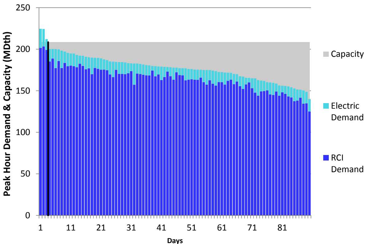
Figure H206. LGDS S2 Winter 2023 – Union Gas Dawn – Descending Demand
