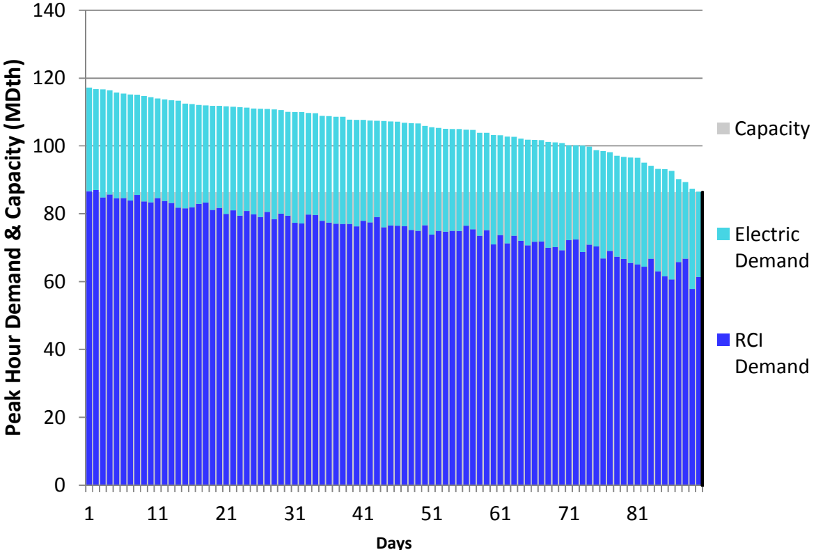
Figure H304. RGDS S3 Winter 23 – Texas Eastern M2 PA South – Descending Demand
