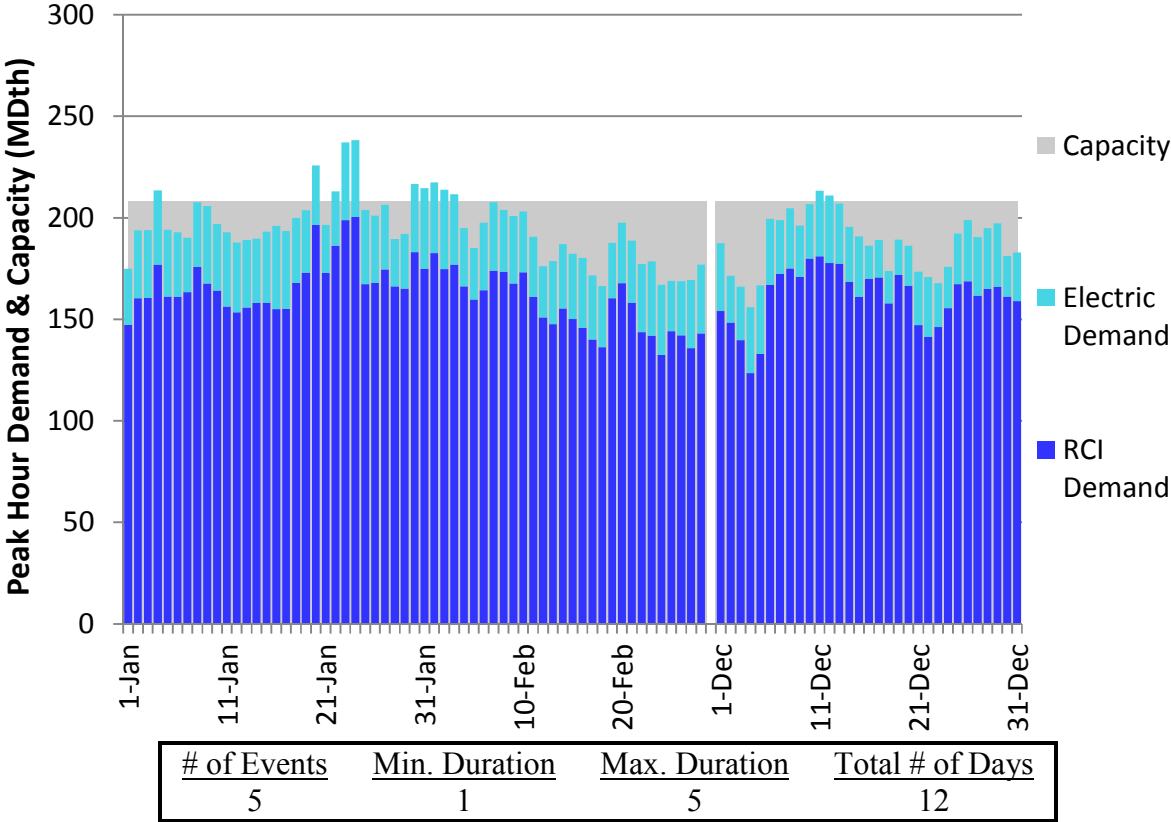
Figure H100. HGDS S2 Winter 2023 – Union Gas Dawn – Descending Demand
