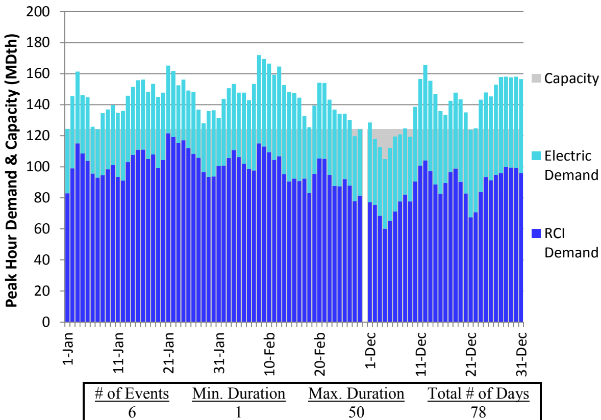
Figure H252. RGDS S3 Winter 2018 – Texas Eastern M3 North – Descending Demand
