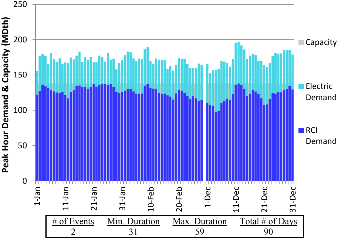
Figure H316. RGDS S3 Winter 2023 – Transco Leidy to Station 210 – Descending Demand
