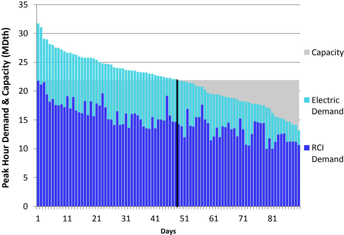
Figure H240. RGDS S3 Winter 2018 – Empire – Descending Demand
