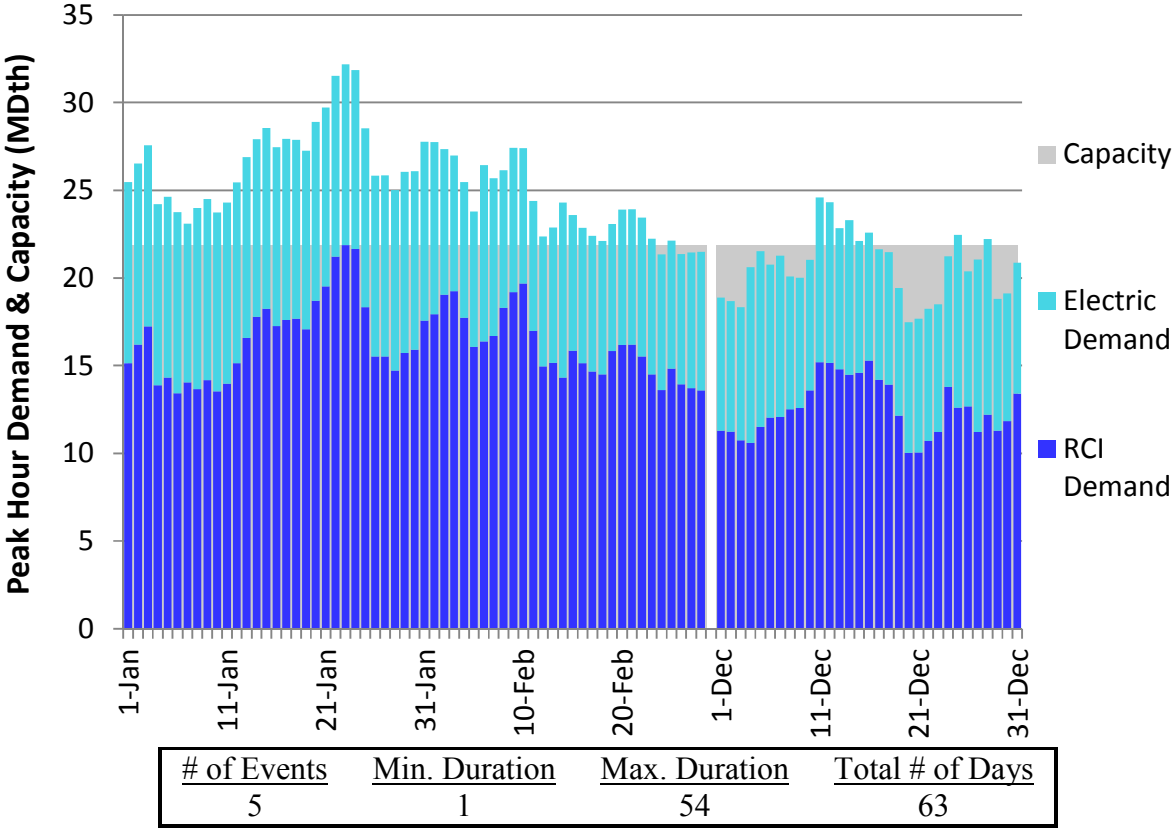
Figure H292. RGDS S3 Winter 23 – Empire – Descending Demand
