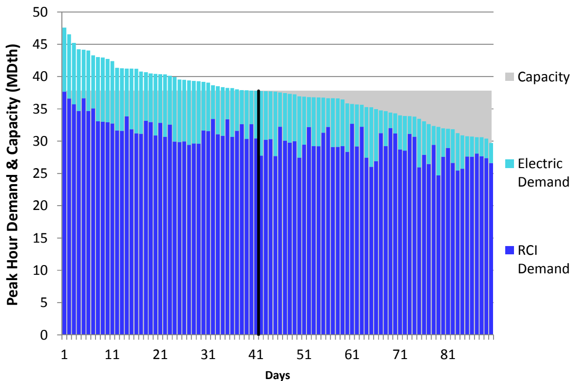
Figure H230. RGDS S3 Winter 2018 – Dominion Eastern NY– Descending Demand
