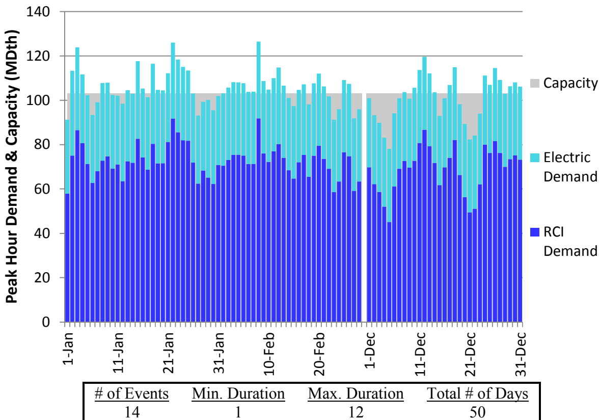
Figure H224. RGDS S3 Winter 2018 – Columbia Gas VA/MD – Descending Demand
