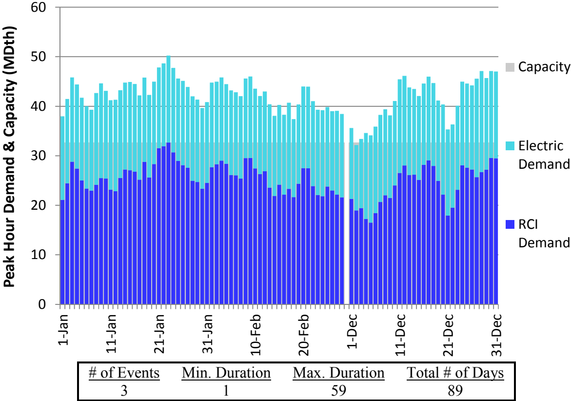
Figure H78. HGDS S2 Winter 2023 – Millennium – Descending Demand
