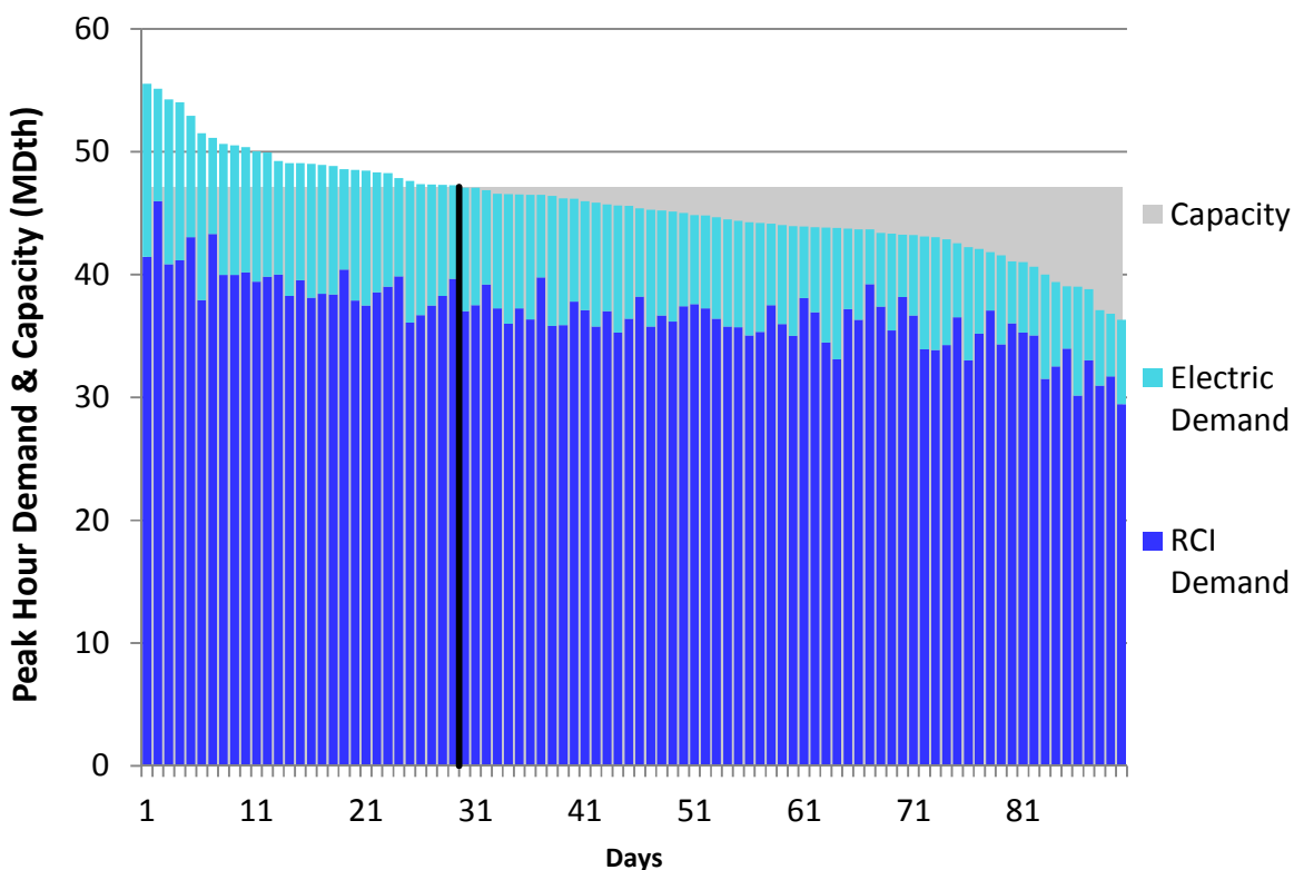
Figure H4. HGDS S2 Winter 2018 – Columbia Gas W PA/NY – Descending Demand
