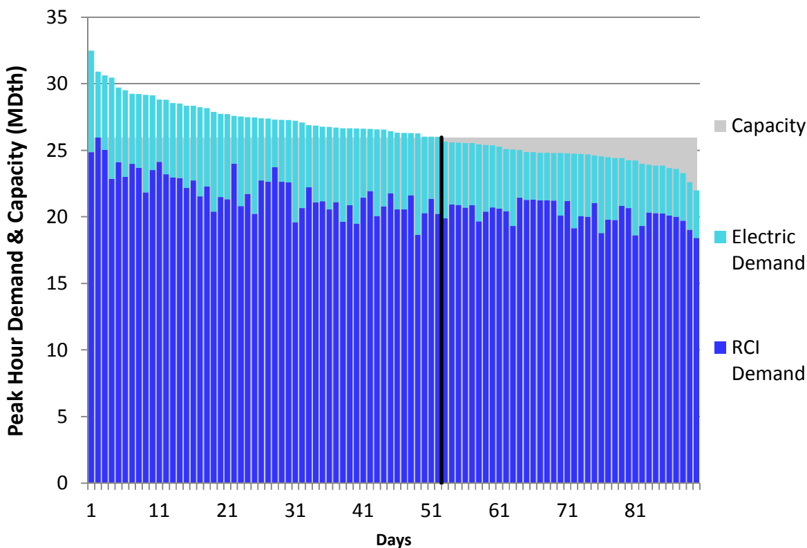
Figure H136. LGDS S2 Winter 2018 – NB/NS Supply – Descending Demand
