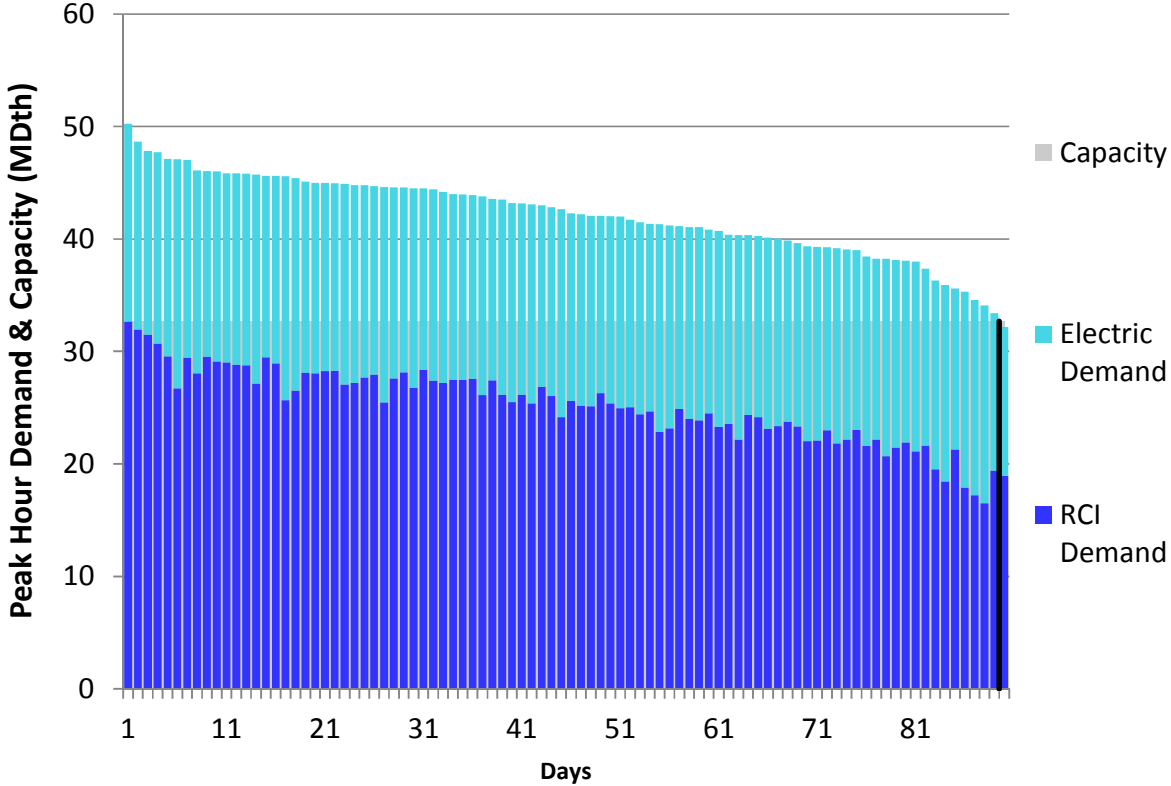
Figure H78. HGDS S2 Winter 2023 – Millennium – Descending Demand
