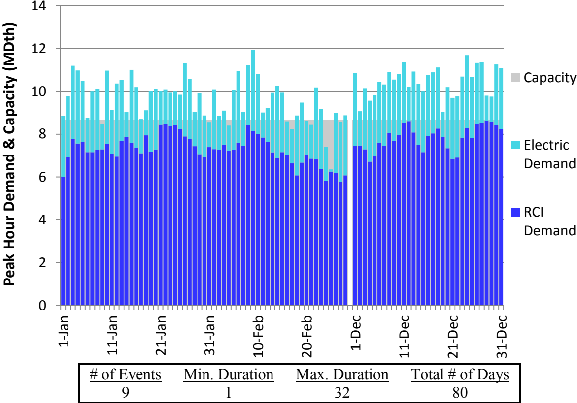
Figure H74. HGDS S2 Winter 2023 – Eastern Shore – Descending Demand
