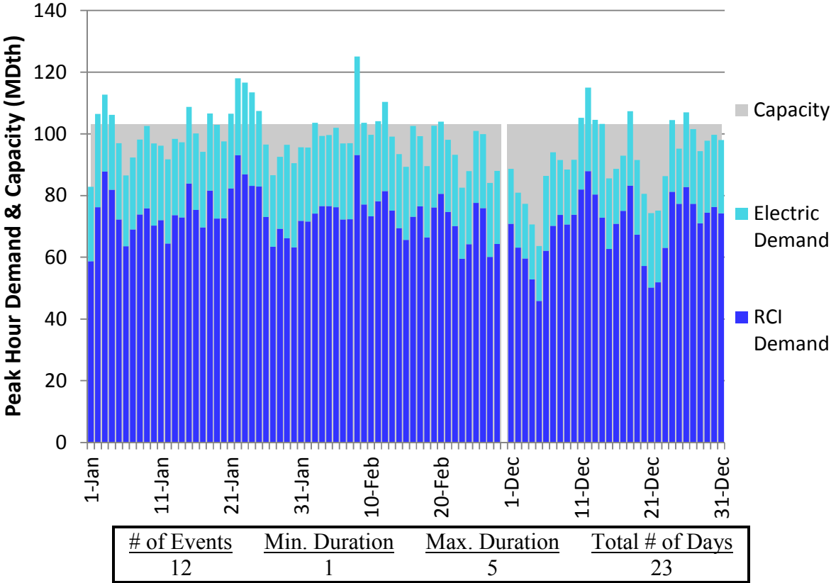
Figure H120. LGDS S2 Winter 2018 – Columbia Gas VA/MD – Descending Demand
