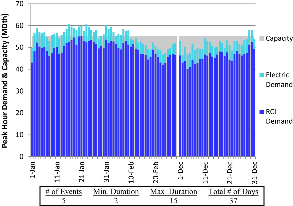
Figure H310. RGDS S3 Winter 2023 – TransCanada Quebec – Descending Demand
