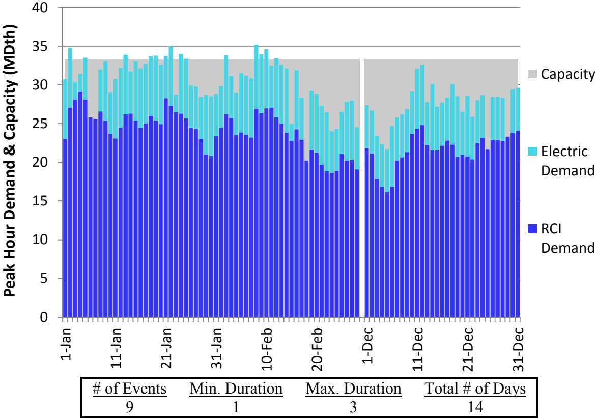
Figure H14. HGDS S2 Winter 2018 – East Tennessee – Descending Demand
