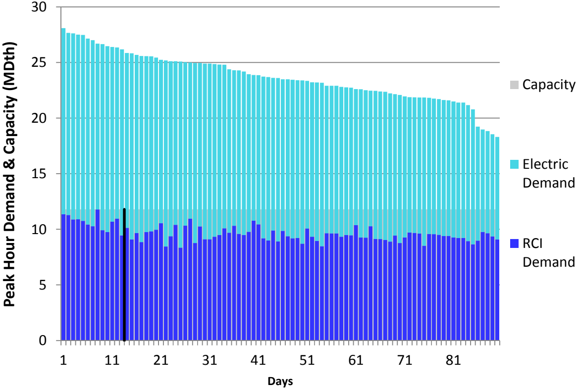
Figure H80. HGDS S2 Winter 2023 – NB/NS Supply – Descending Demand
