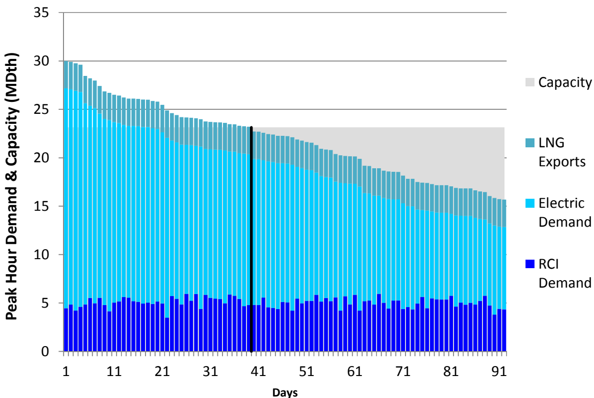
Figure H106. HGDS S2 Summer 2023 – Dominion Southeast – Descending Demand
