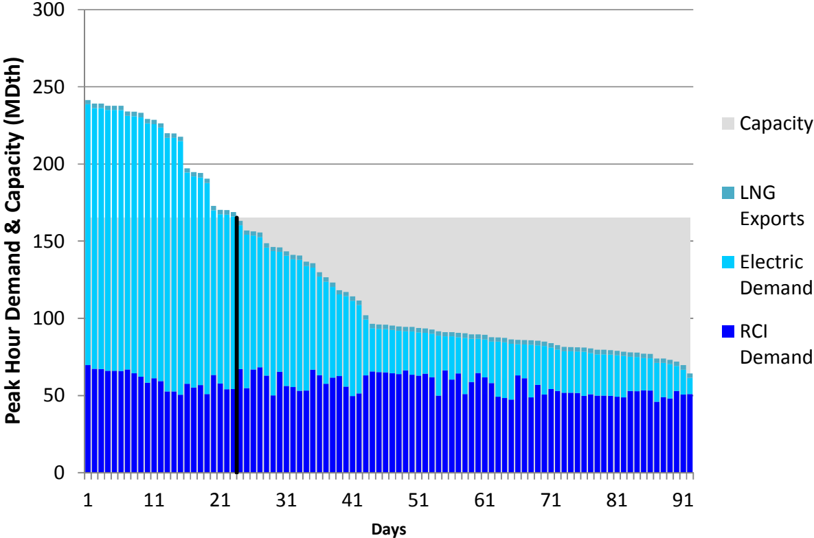
Figure H118. HGDS S2 Summer 2023 – Transco Z5 – Descending Demand
