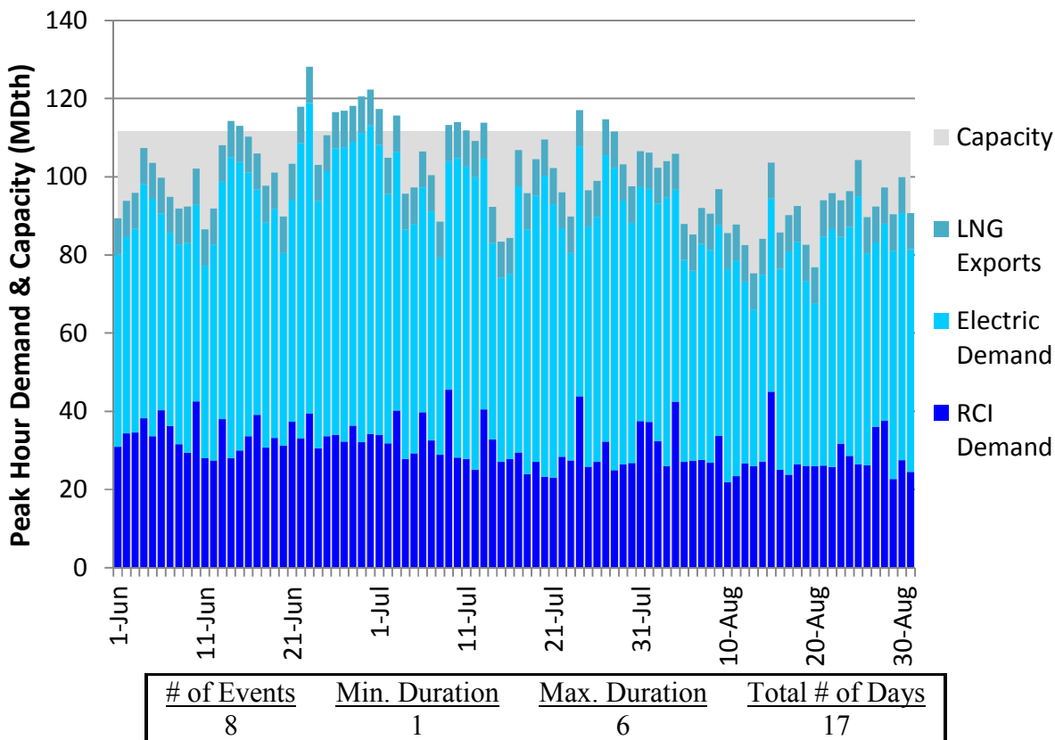
Figure H322. RGDS S3 Summer 2023 – Columbia Gas VA/MD – Descending Demand
