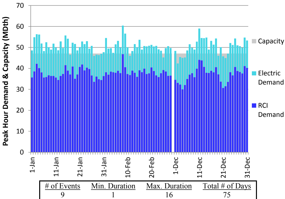
Figure H62. HGDS S2 Winter 2023 – Columbia Gas W PA/NY – Descending Demand
