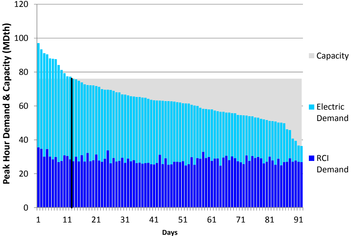
Figure H44. HGDS S2 Summer 2018 – Algonquin CT – Descending Demand
