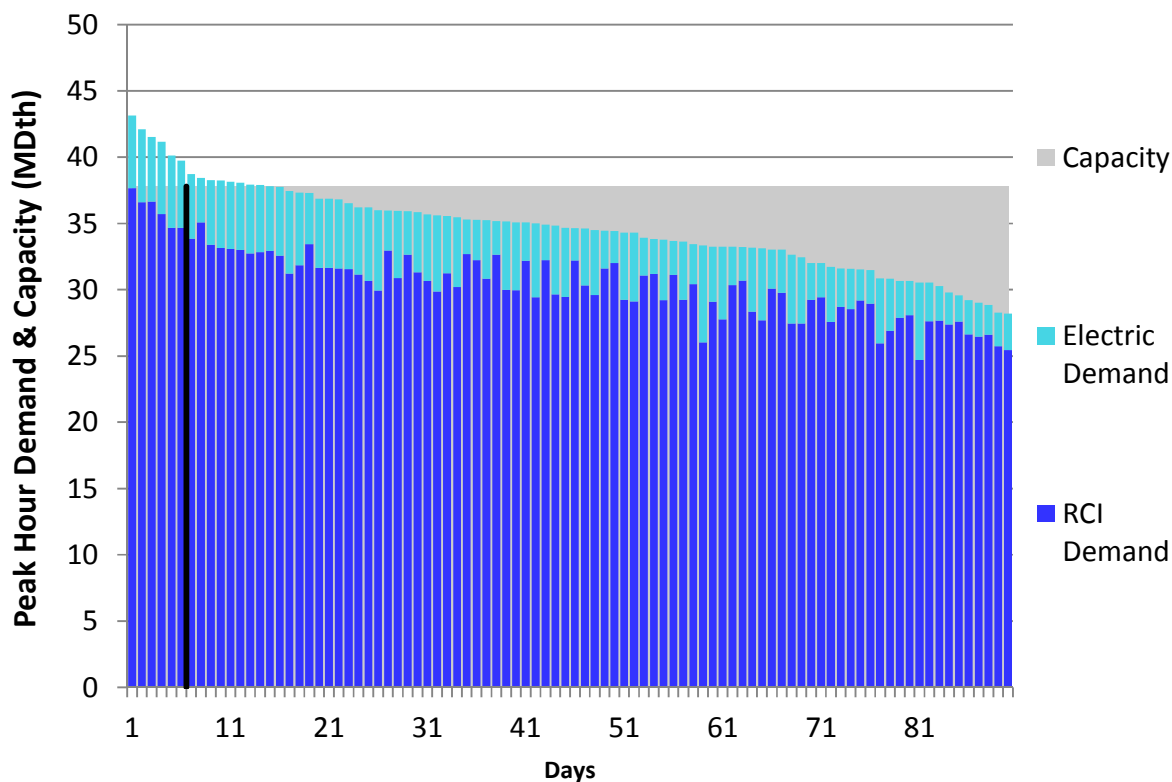
Figure H124. LGDS S2 Winter 2018 – Dominion Eastern NY– Descending Demand
