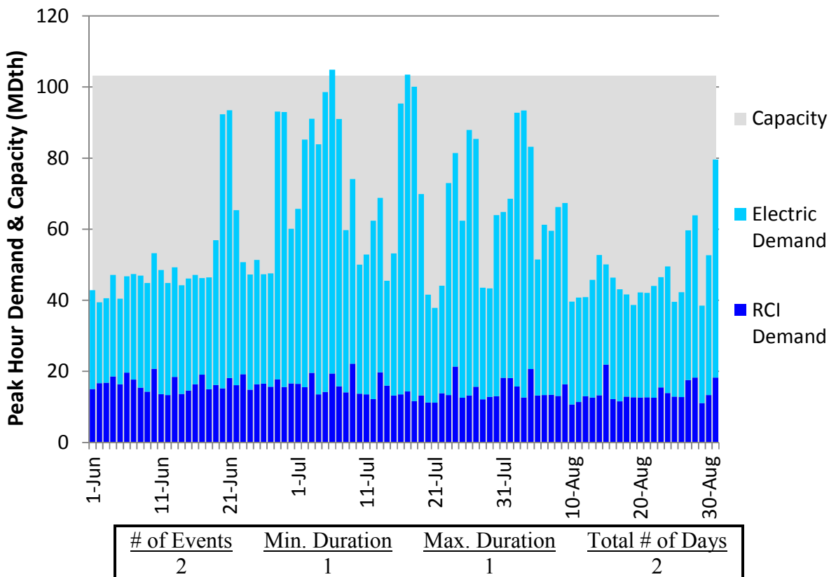
Figure H46. HGDS S2 Summer 2018 – Columbia Gas VA/MD – Descending Demand
