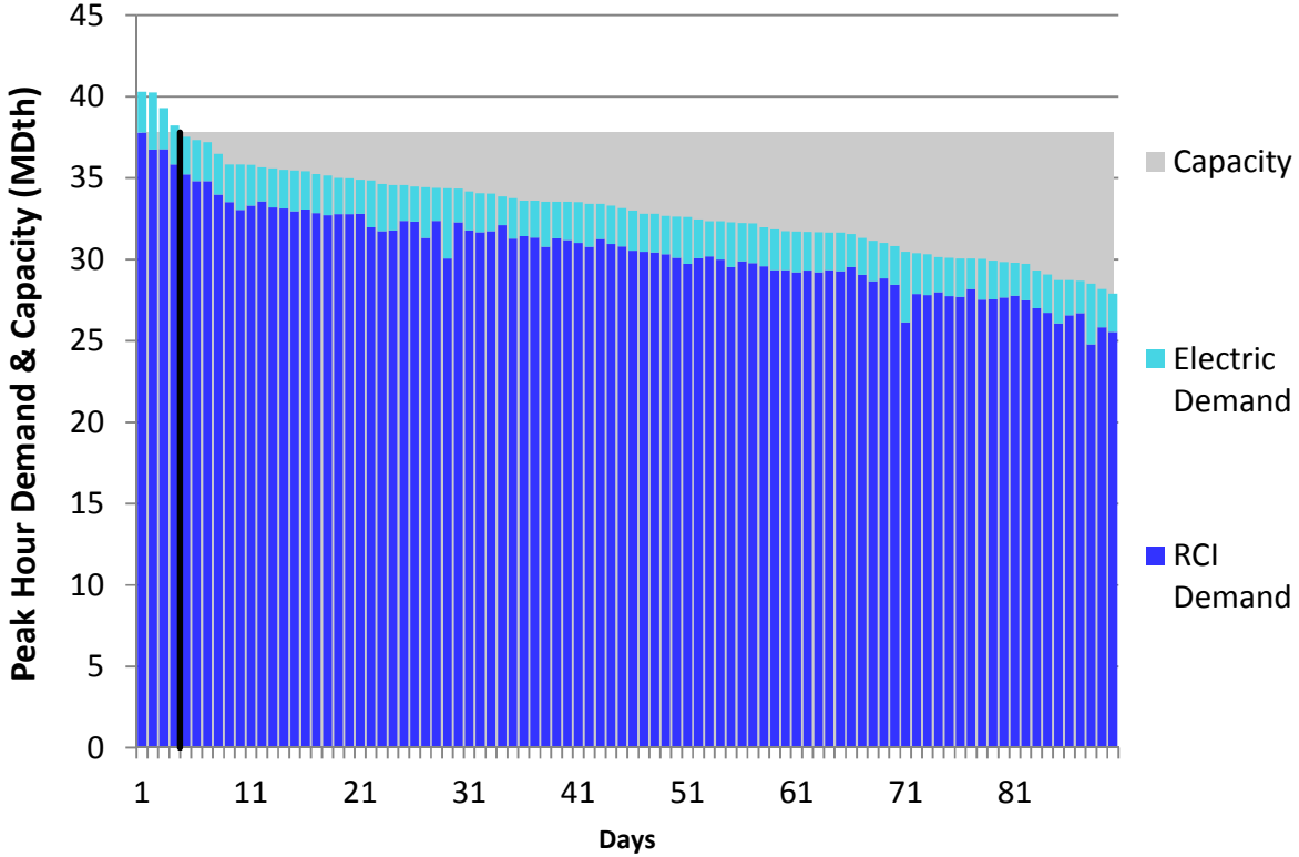
Figure H8. HGDS S2 Winter 2018 – Dominion Eastern NY– Descending Demand
