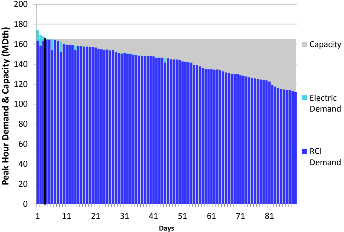
Figure H150. LGDS S2 Winter 2018 – Transco Z5 – Descending Demand
