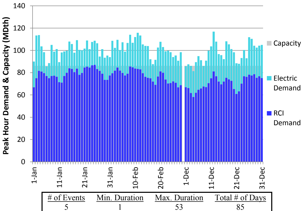
Figure H28. HGDS S2 Winter 2018 – Texas Eastern M2 PA South – Descending Demand
