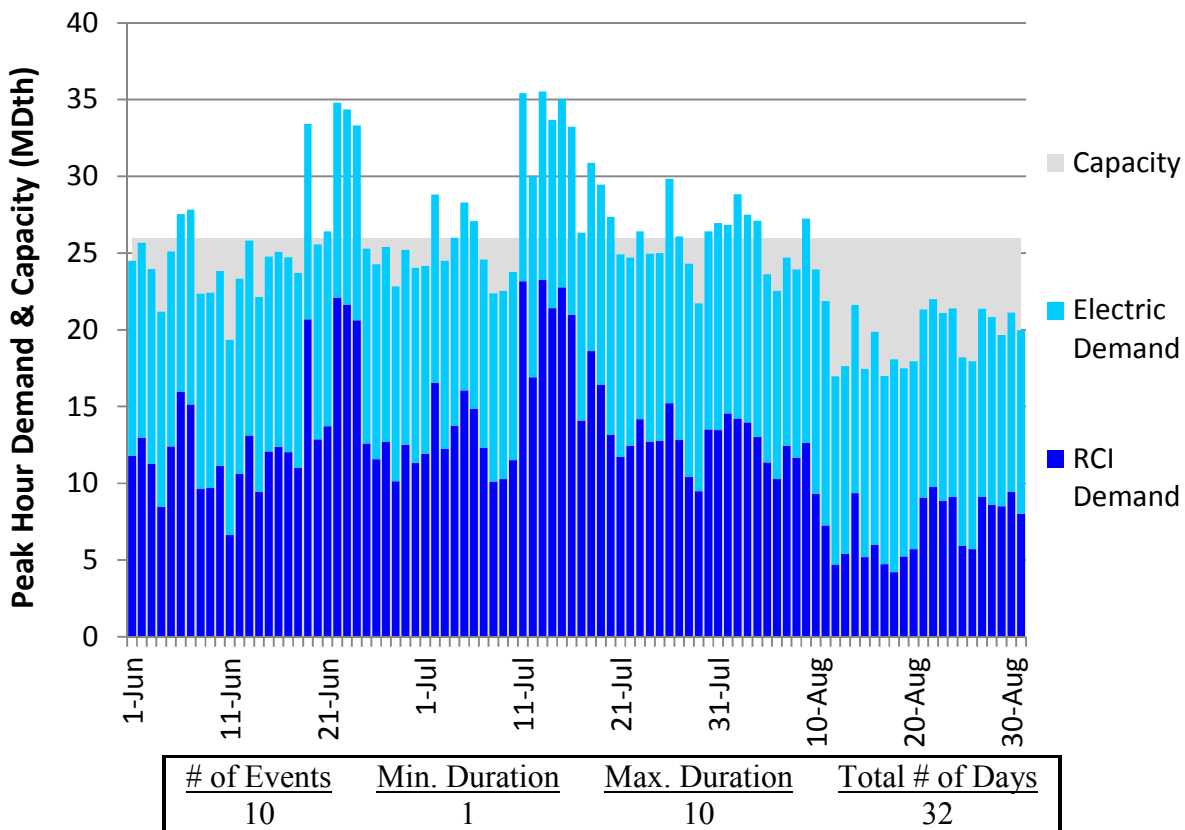
Figure H334. RGDS S3 Summer 2023 – Texas Eastern ETX – Descending Demand
