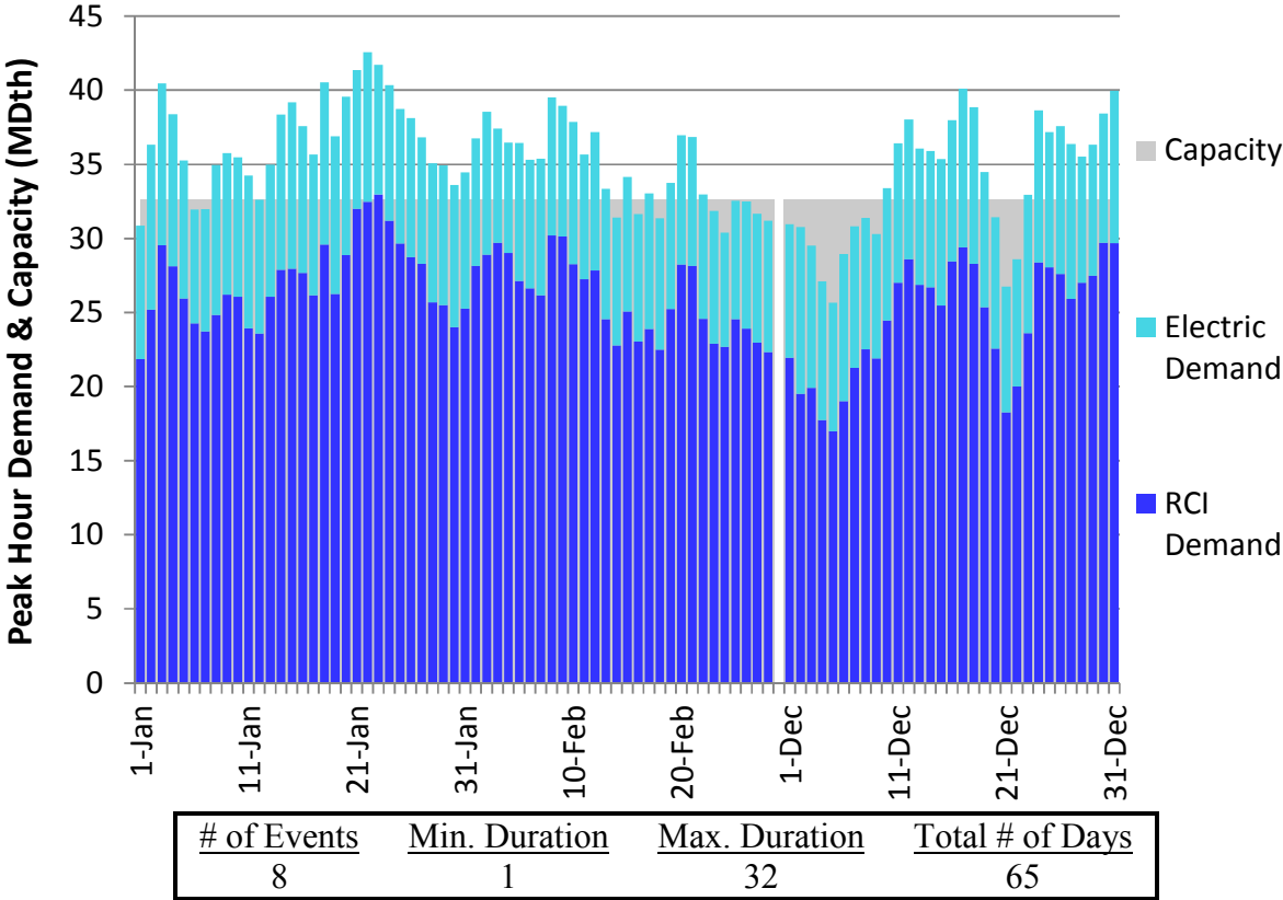
Figure H20. HGDS S2 Winter 2018 – Millennium – Descending Demand
