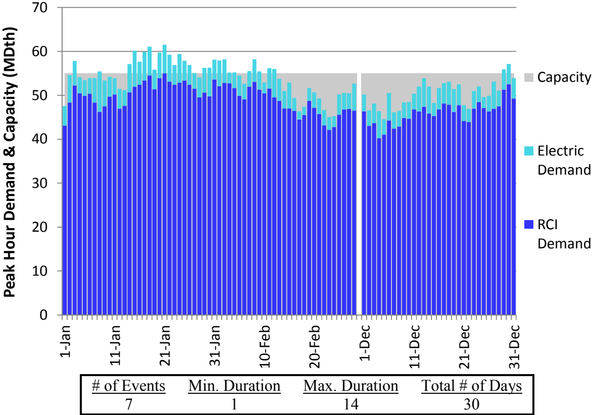
Figure H34. HGDS S2 Winter 2018 – TransCanada Quebec – Descending Demand
