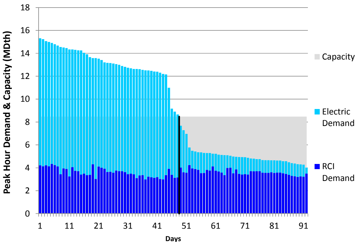
Figure H270. RGDS S3 Summer 2018 – Eastern Shore – Descending Demand
