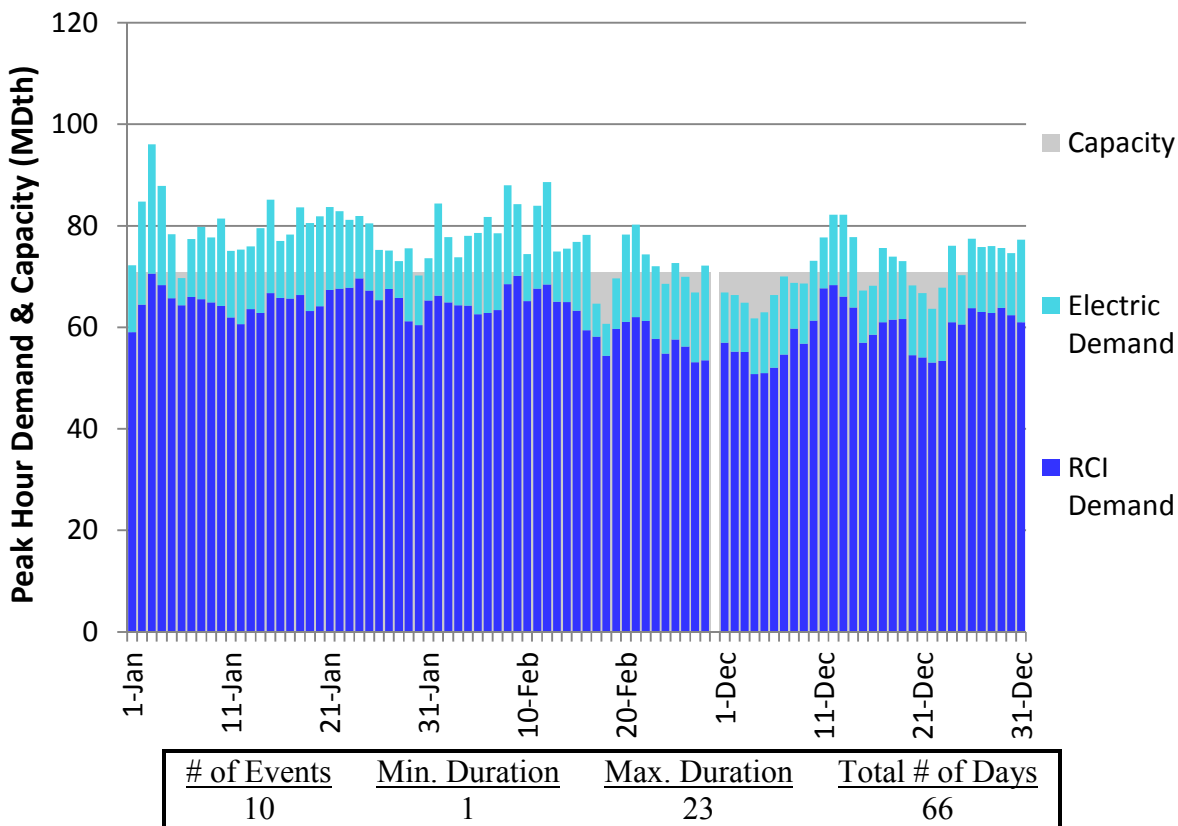
Figure H36. HGDS S2 Winter 2018 – Transco Leidy Atlantic – Descending Demand
