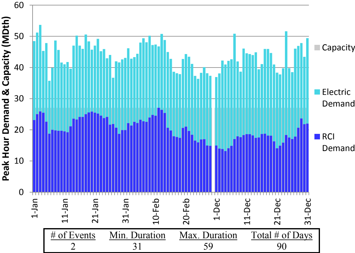
Figure H6. HGDS S2 Winter 2018 – Constitution – Descending Demand
