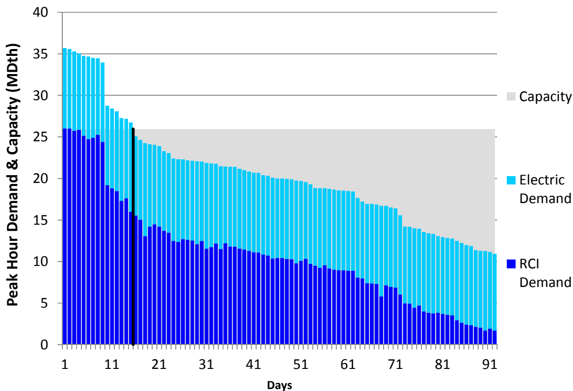
Figure H162. LGDS S2 Summer 2018 – Texas Eastern ETX – Descending Demand
