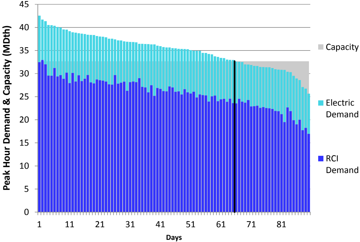
Figure H20. HGDS S2 Winter 2018 – Millennium – Descending Demand
