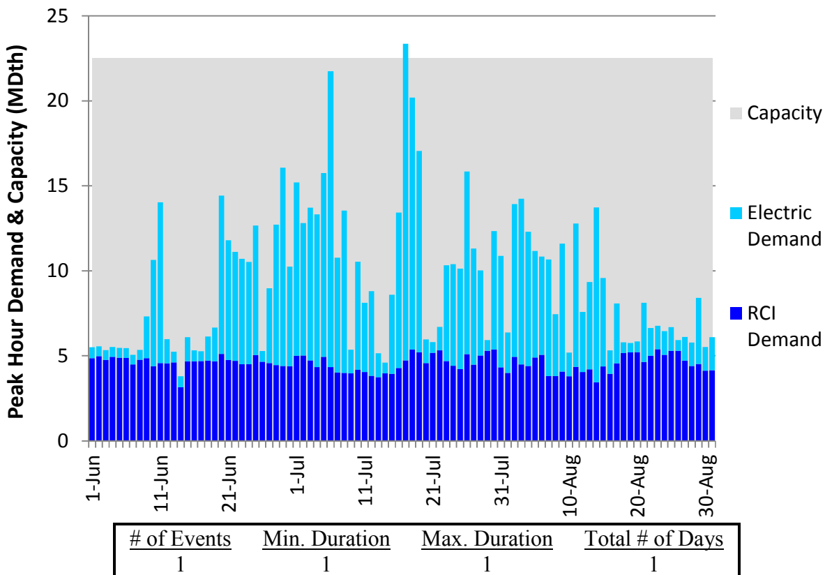
Figure H158. LGDS S2 Summer 2018 – Dominion Southeast – Descending Demand
