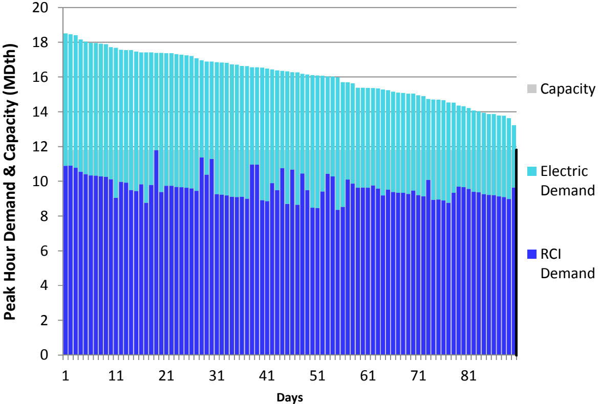
Figure H298. RGDS S3 Winter 2023 – NB/NS Supply – Descending Demand
