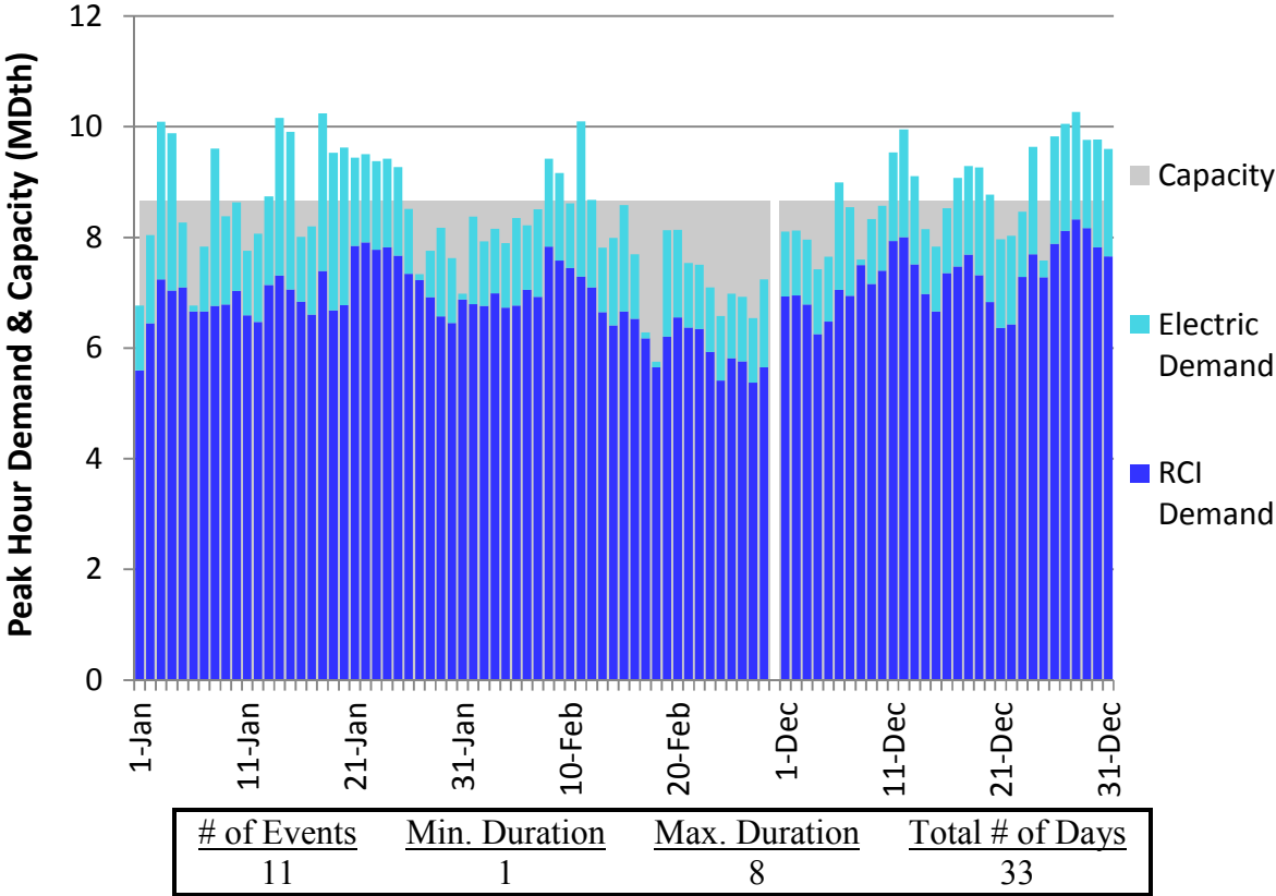
Figure H130. LGDS S2 Winter 2018 – Eastern Shore – Descending Demand
