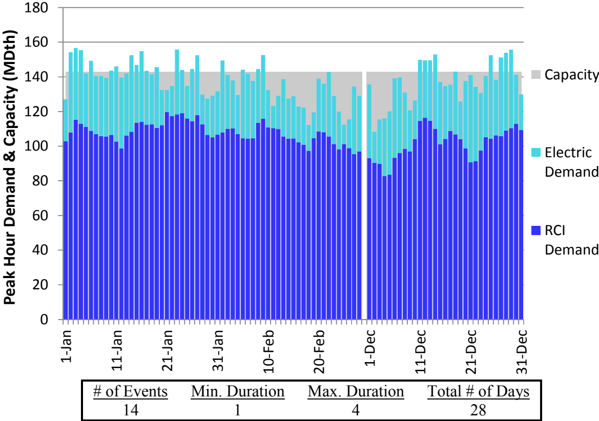
Figure H204. LGDS S2 Winter 2023 – Transco Leidy to Station 210 – Descending Demand
