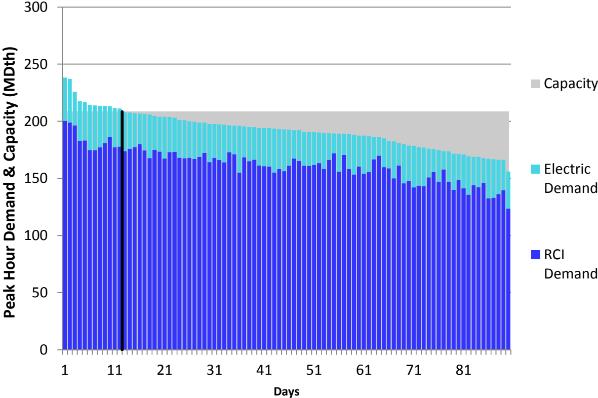
Figure H100. HGDS S2 Winter 2023 – Union Gas Dawn – Descending Demand
