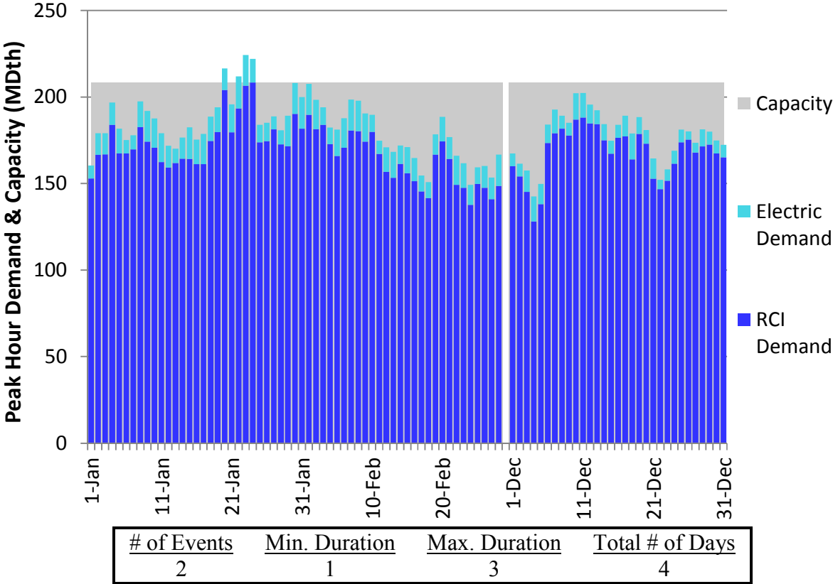
Figure H42. HGDS S2 Winter 2018 – Union Gas Dawn – Descending Demand
