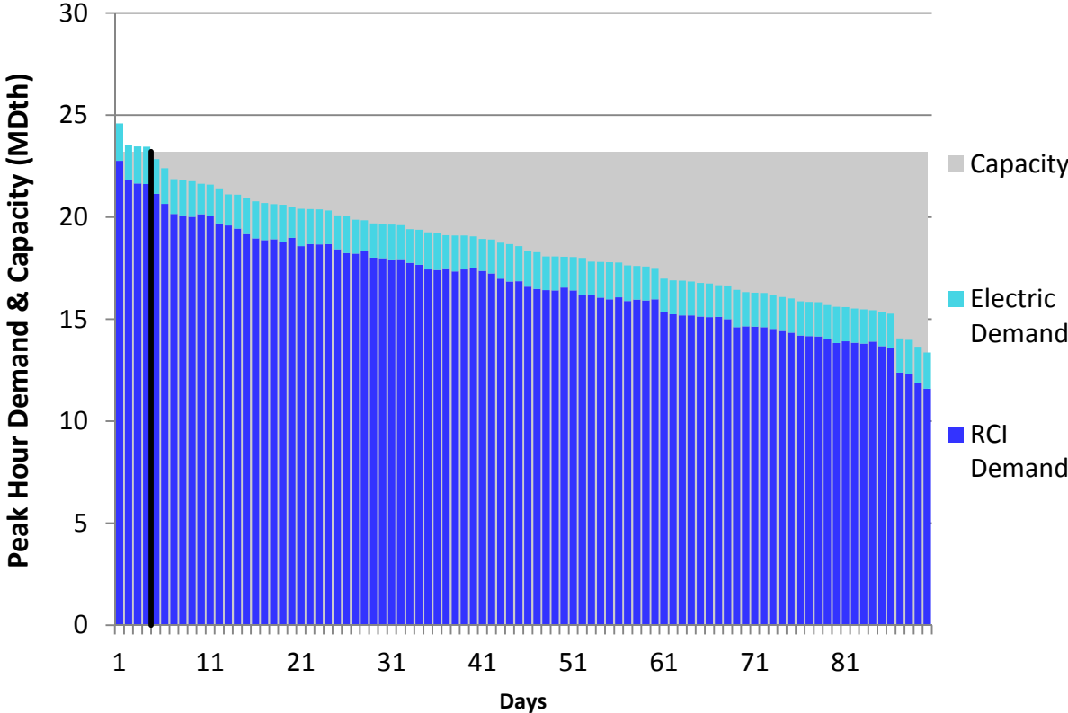
Figure H174. LGDS S2 Winter 2023 – Dominion Western NY– Descending Demand
