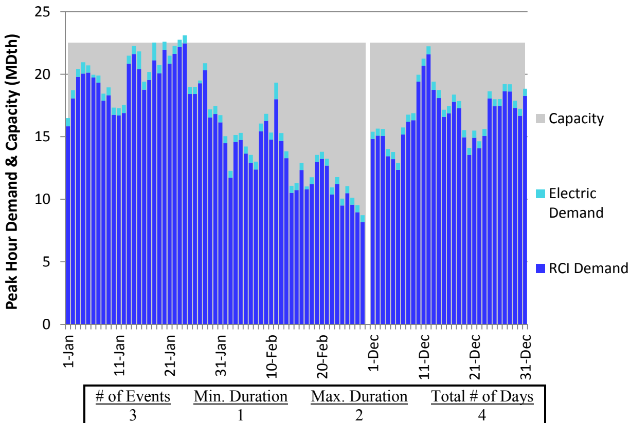
Figure H126. LGDS S2 Winter 2018 – Dominion Southeast – Descending Demand
