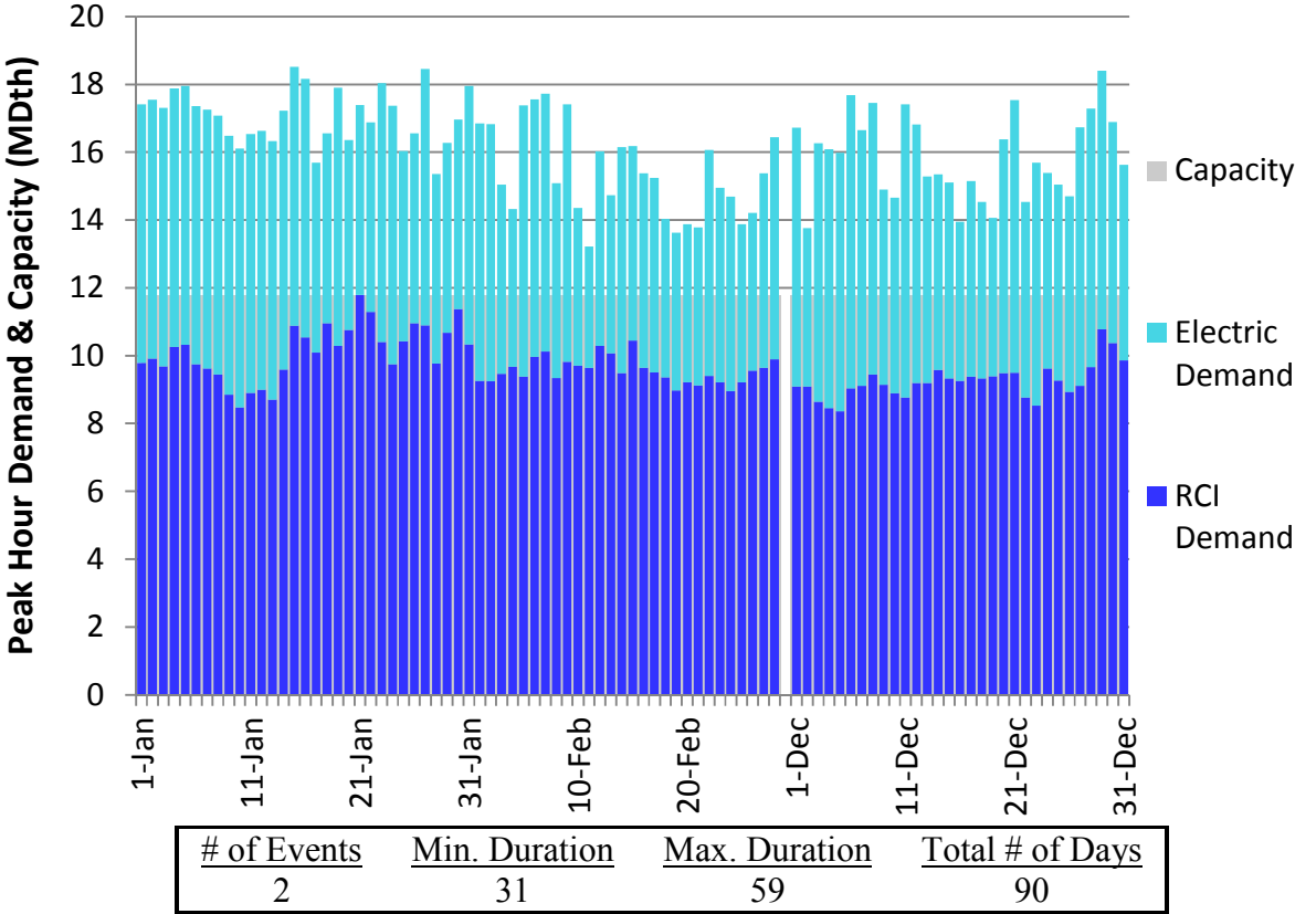
Figure H298. RGDS S3 Winter 2023 – NB/NS Supply – Descending Demand
