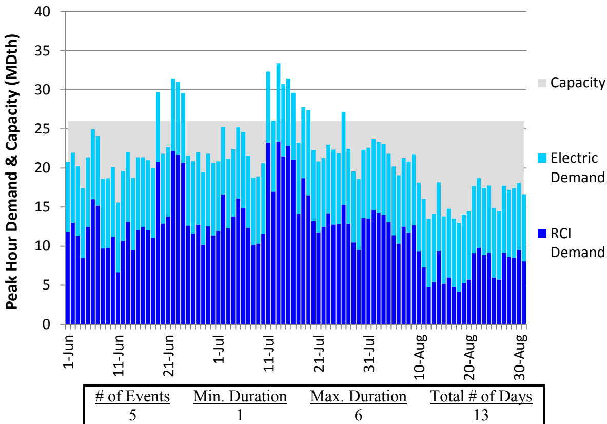
Figure H220. LGDS S2 Summer 2023 – Texas Eastern ETX – Descending Demand
