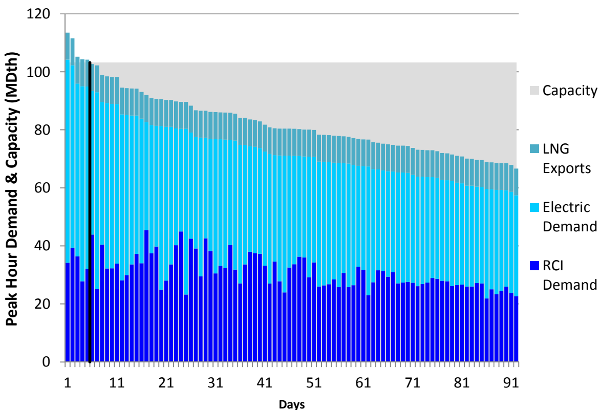
Figure H210. LGDS S2 Summer 2023 – Columbia Gas VA/MD – Descending Demand
