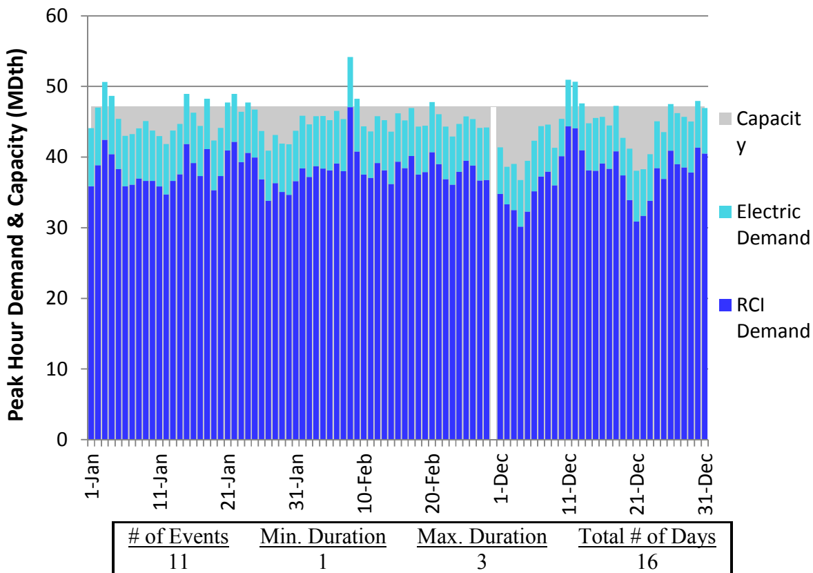
Figure H278. RGDS S3 Winter 2023 – Columbia Gas W PA/NY – Descending Demand
