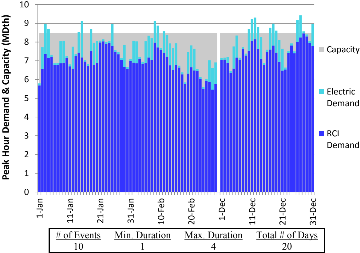
Figure H238. RGDS S3 Winter 2018 – Eastern Shore – Descending Demand
