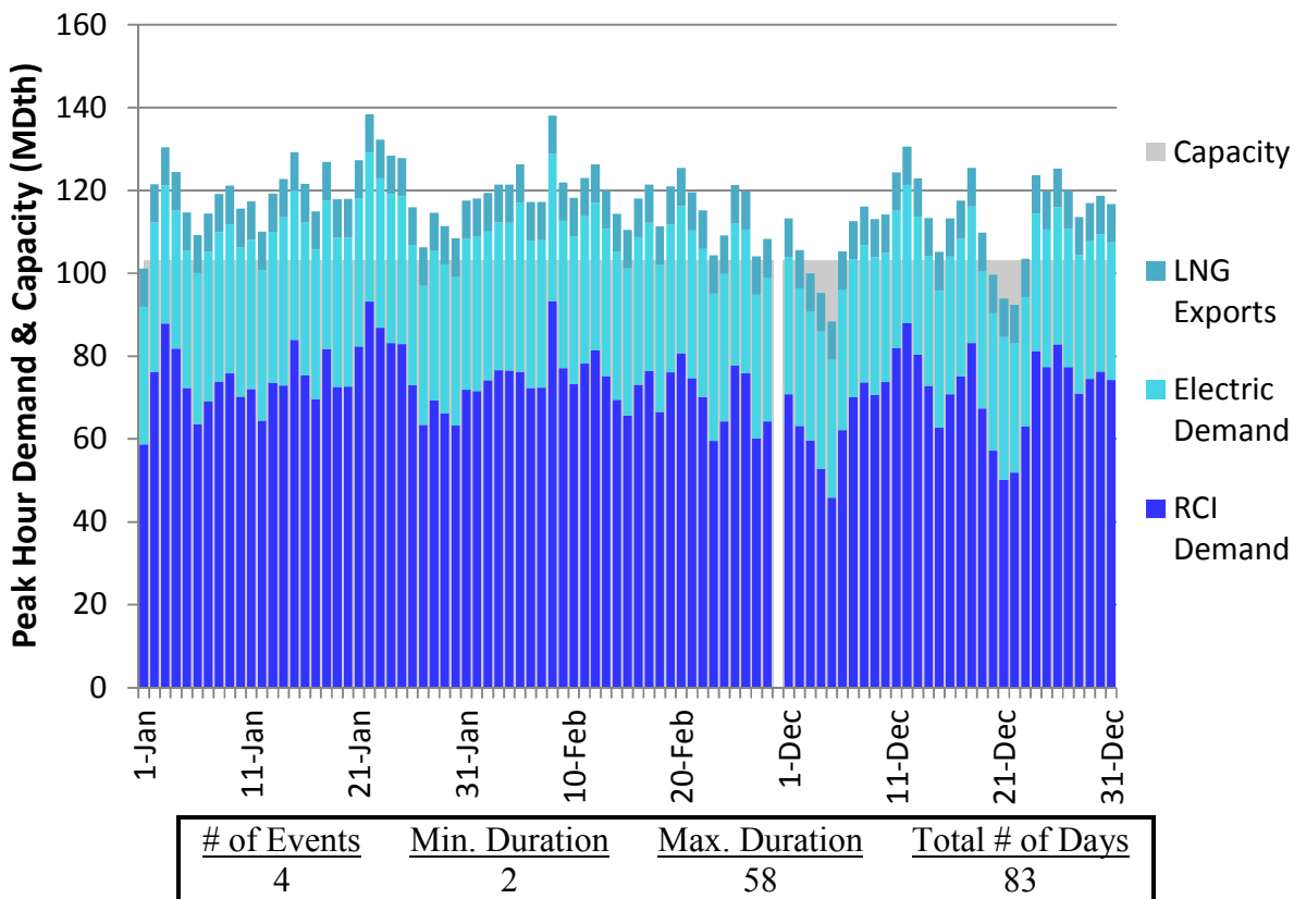
Figure H166. LGDS S2 Winter 2023 – Columbia Gas VA/MD – Descending Demand
