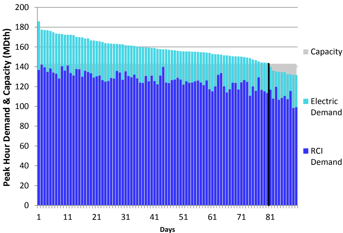
Figure H40. HGDS S2 Winter 2018 – Transco Leidy to Station 210 – Descending Demand
