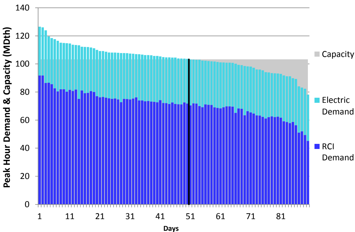
Figure H224. RGDS S3 Winter 2018 – Columbia Gas VA/MD – Descending Demand
