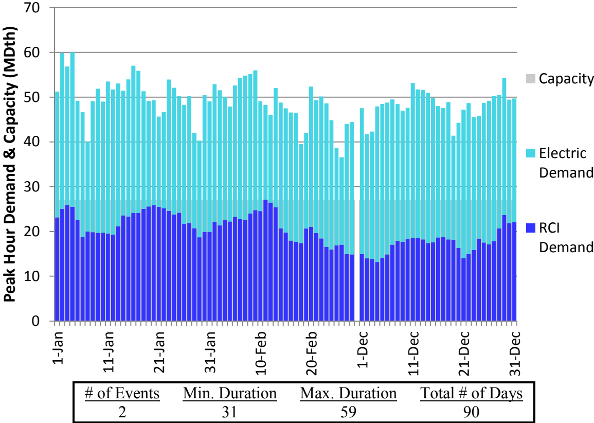
Figure H280. RGDS S3 Winter 2023 – Constitution – Descending Demand
