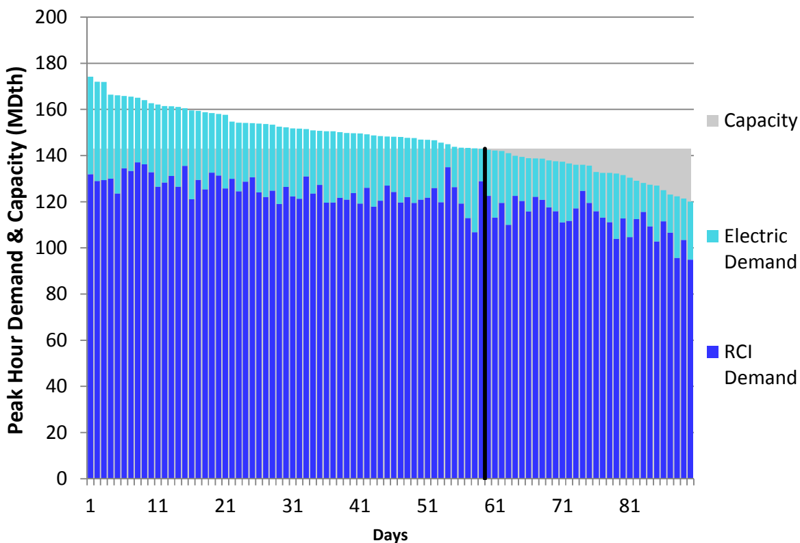
Figure H152. LGDS S2 Winter 2018 – Transco Leidy to Station 210 – Descending Demand
