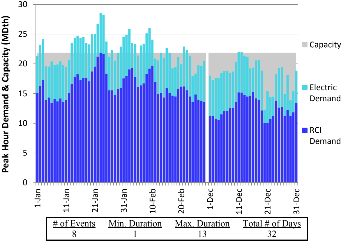
Figure H182. LGDS S2 Winter 2023 – Empire – Descending Demand
