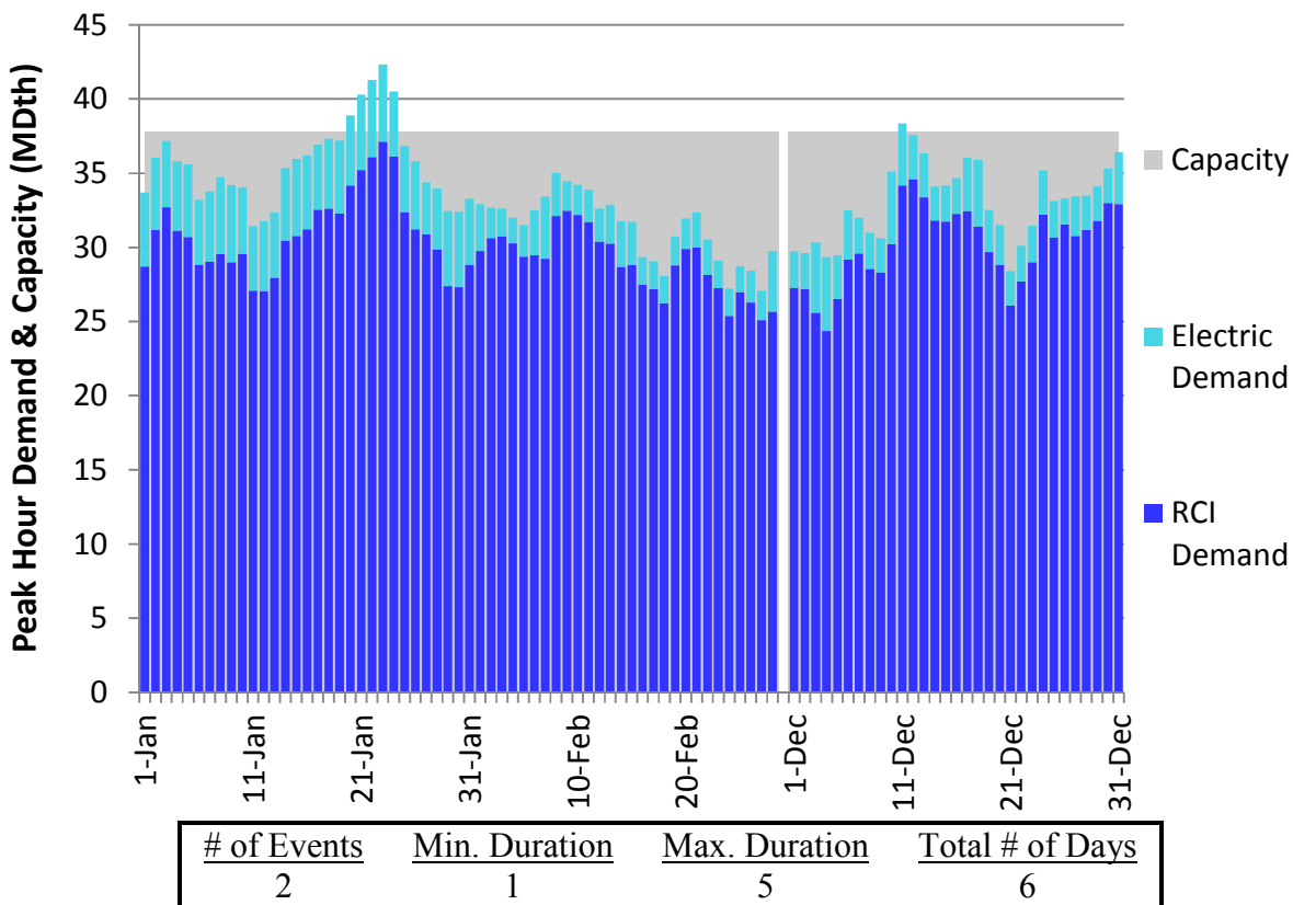
Figure H124. LGDS S2 Winter 2018 – Dominion Eastern NY– Descending Demand
