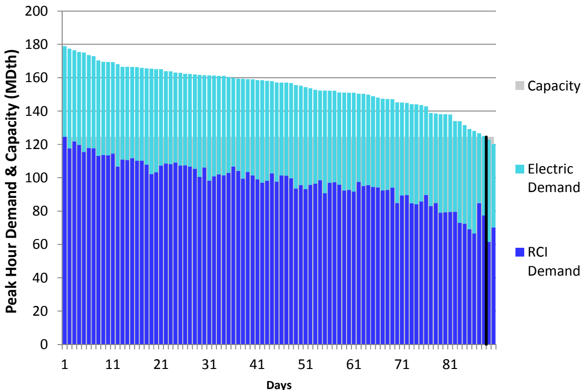
Figure H306. RGDS S3 Winter 2023 – Texas Eastern M3 North – Descending Demand
