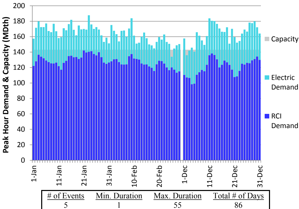
Figure H98. HGDS S2 Winter 2023 – Transco Leidy to Station 210 – Descending Demand
