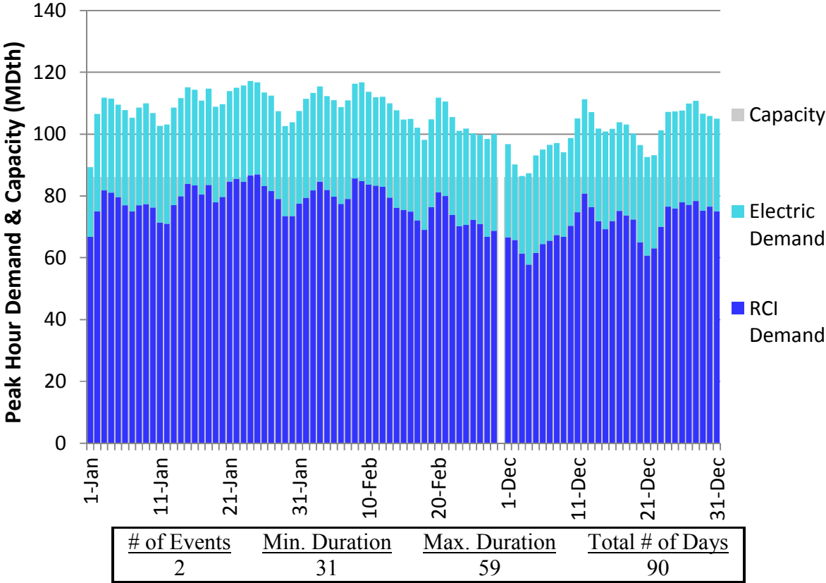
Figure H304. RGDS S3 Winter 23 – Texas Eastern M2 PA South – Descending Demand
