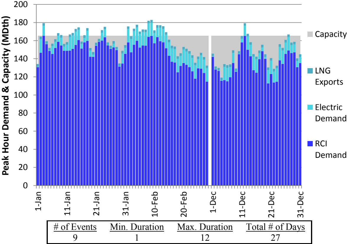
Figure H314. RGDS S3 Winter 2023 – Transco Z5 – Descending Demand
