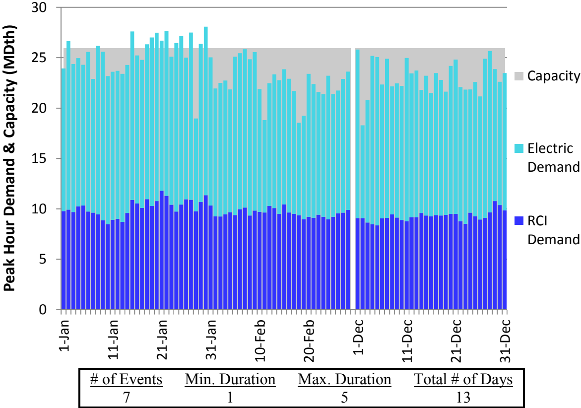
Figure H80. HGDS S2 Winter 2023 – NB/NS Supply – Descending Demand
