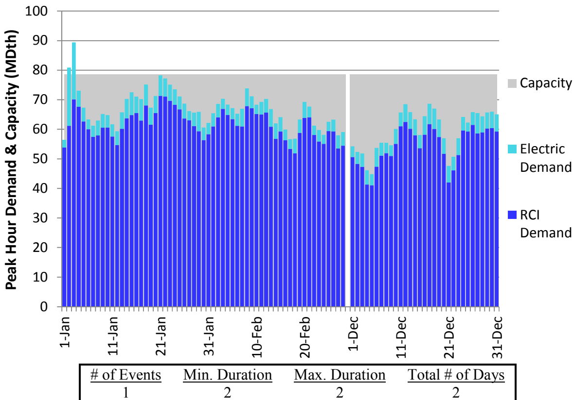
Figure H138. LGDS S2 Winter 2018 – Tennessee Z4 PA – Descending Demand
