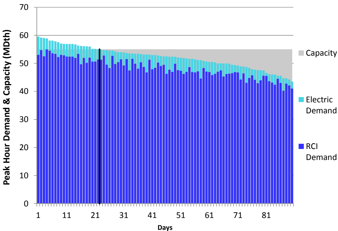
Figure H148. LGDS S2 Winter 2018 – TransCanada Quebec – Descending Demand
