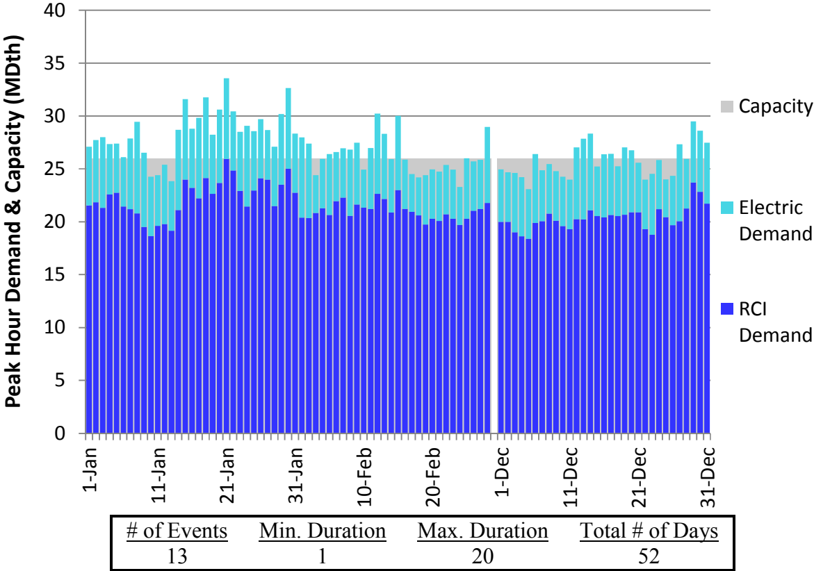
Figure H22. HGDS S2 Winter 2018 – NB/NS Supply – Descending Demand
