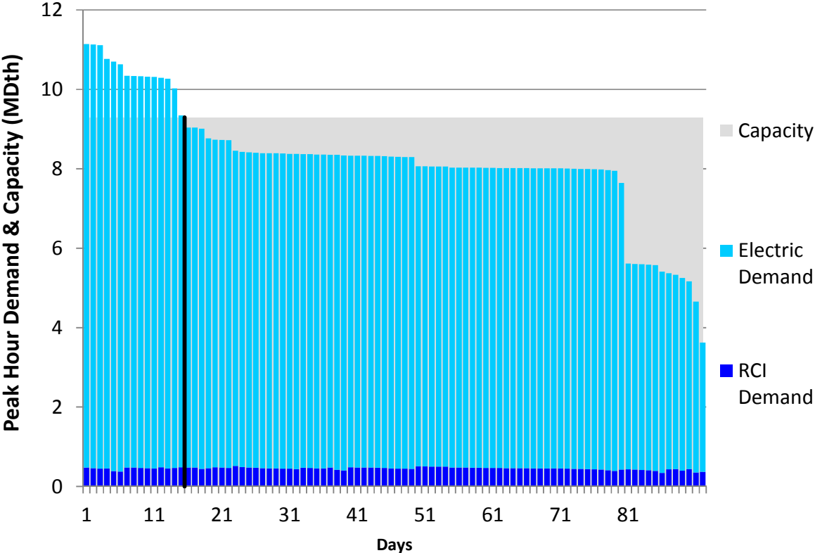
Figure H218. LGDS S2 Summer 2023 – PNGTS N of Westbrook – Descending Demand
