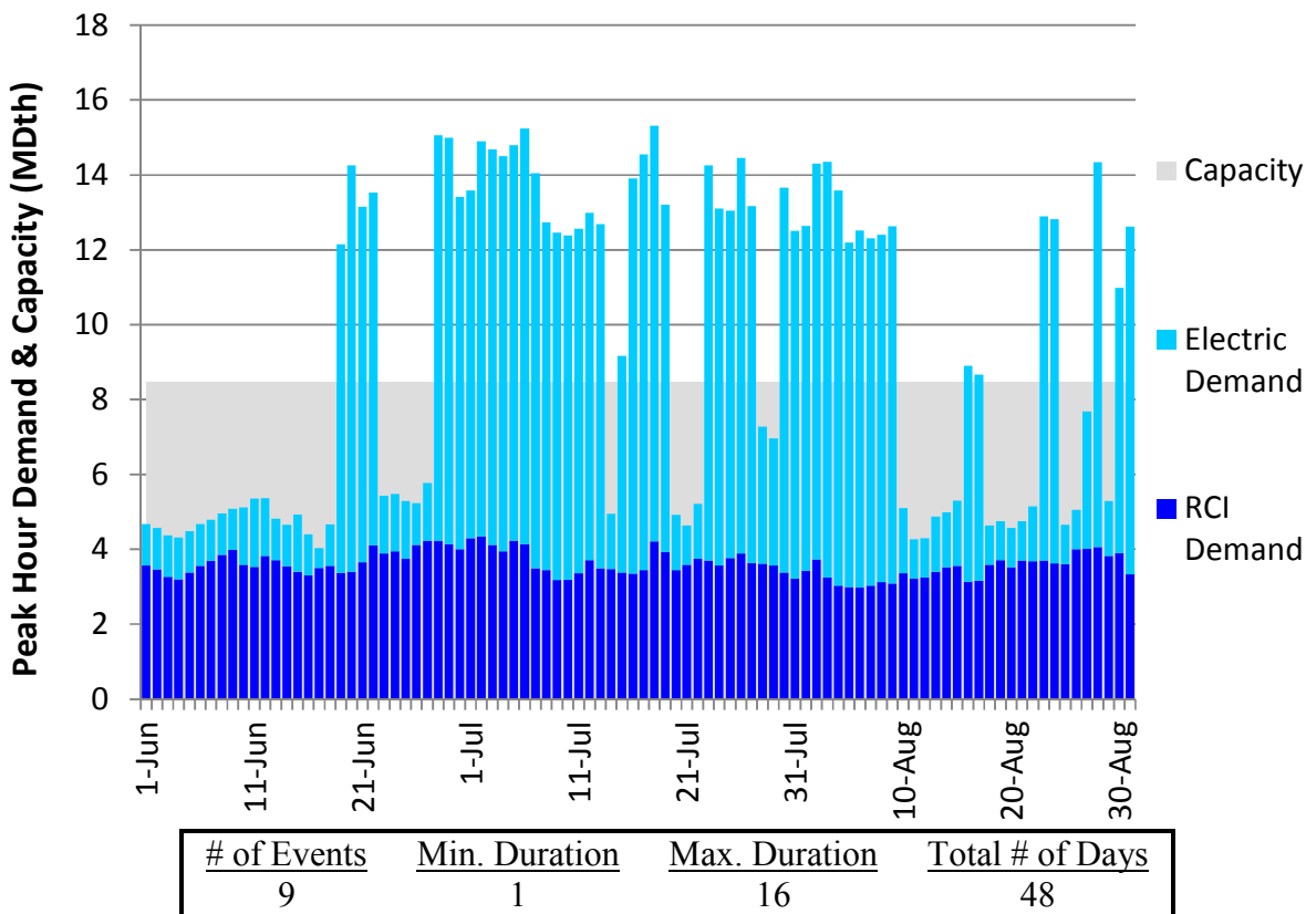
Figure H270. RGDS S3 Summer 2018 – Eastern Shore – Descending Demand
