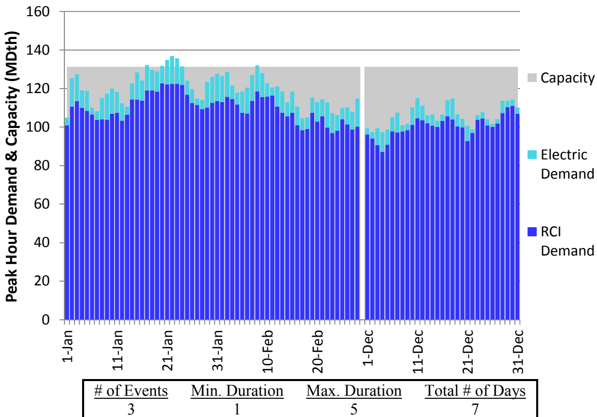
Figure H32. HGDS S2 Winter 2018 – TransCanada Ontario West – Descending Demand
