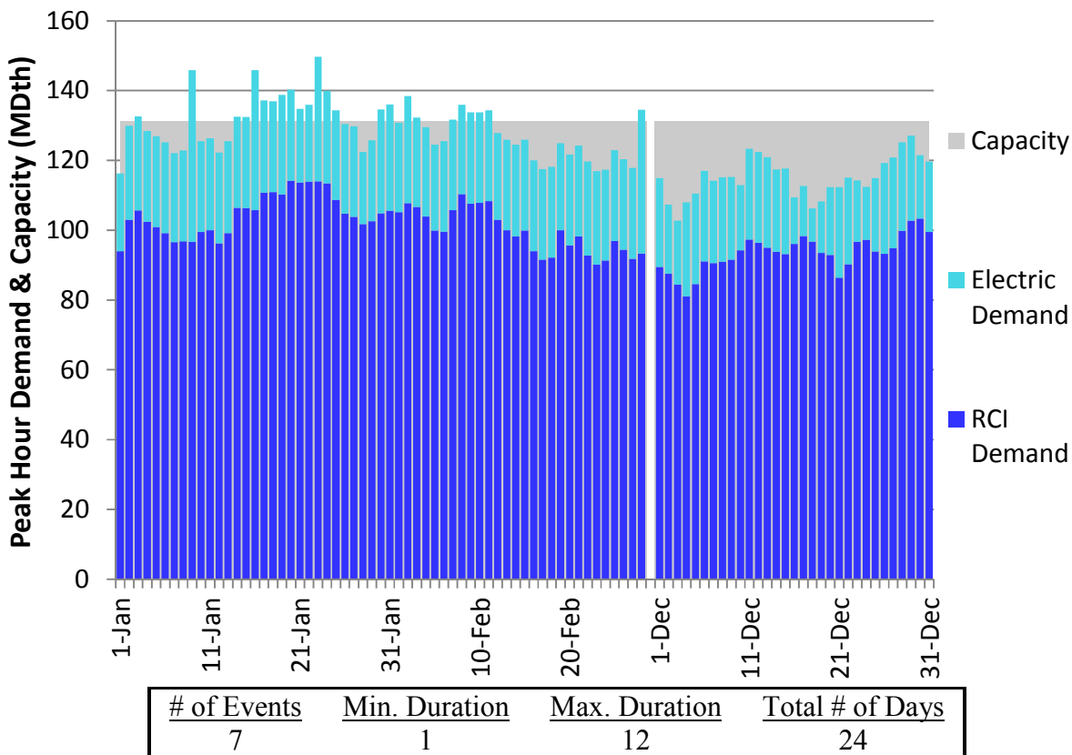
Figure H308. RGDS S3 Winter 2023 – TransCanada Ontario West – Descending Demand
