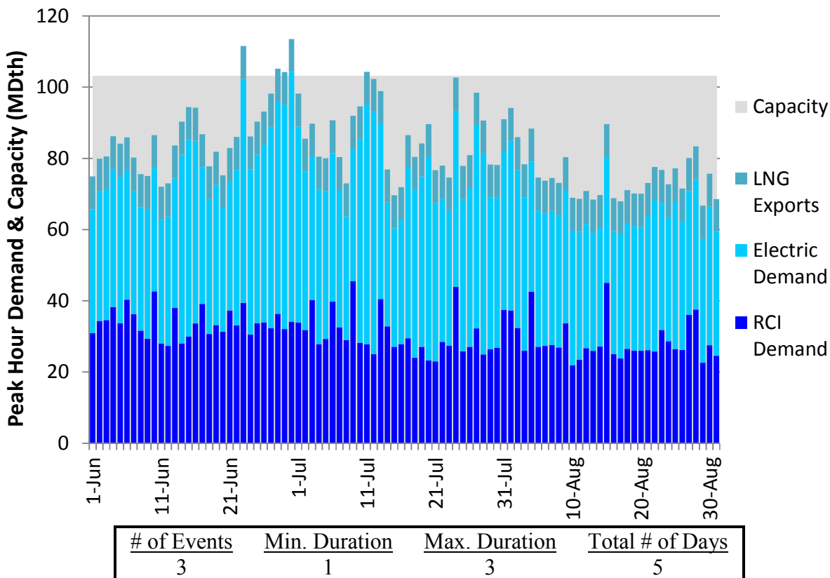
Figure H210. LGDS S2 Summer 2023 – Columbia Gas VA/MD – Descending Demand
