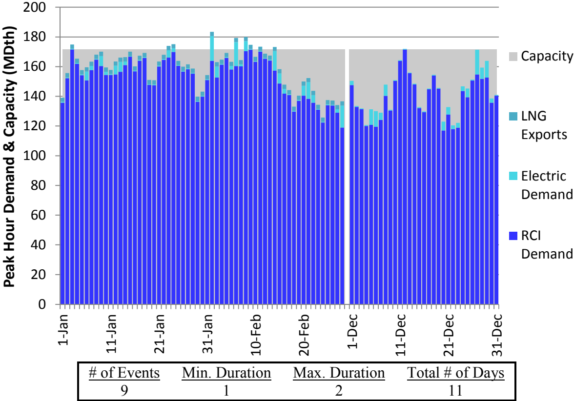
Figure H96. HGDS S2 Winter 2023 – Transco Z5 – Descending Demand
