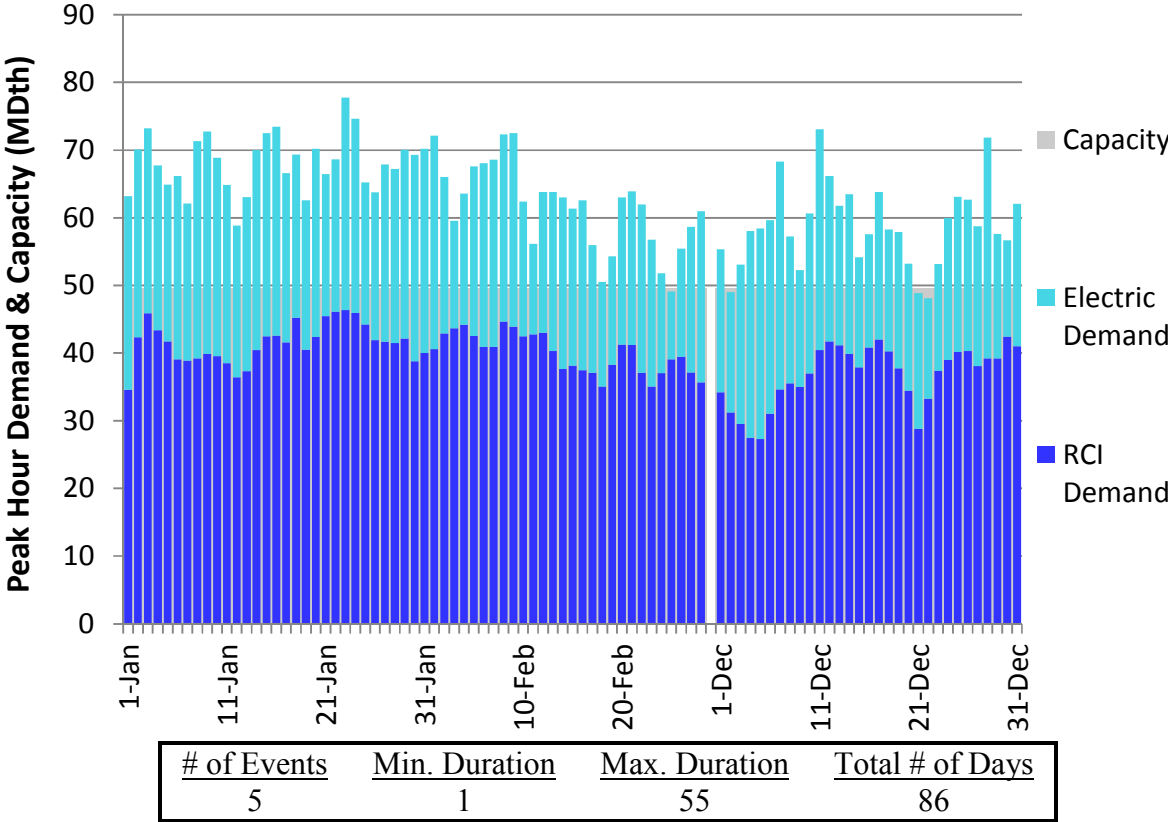
Figure H190. LGDS S2 Winter 2023 – Tennessee Z5 NY – Descending Demand
