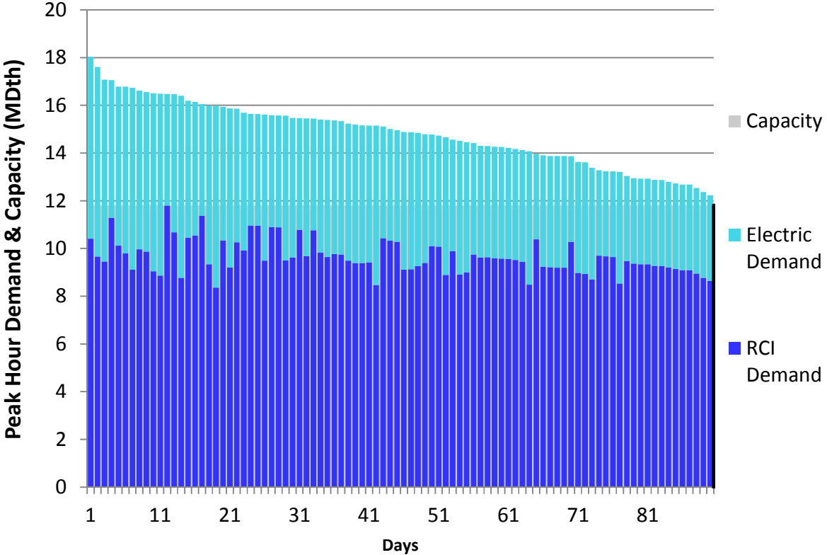
Figure H186. LGDS S2 Winter 2023 – NB/NS Supply – Descending Demand
