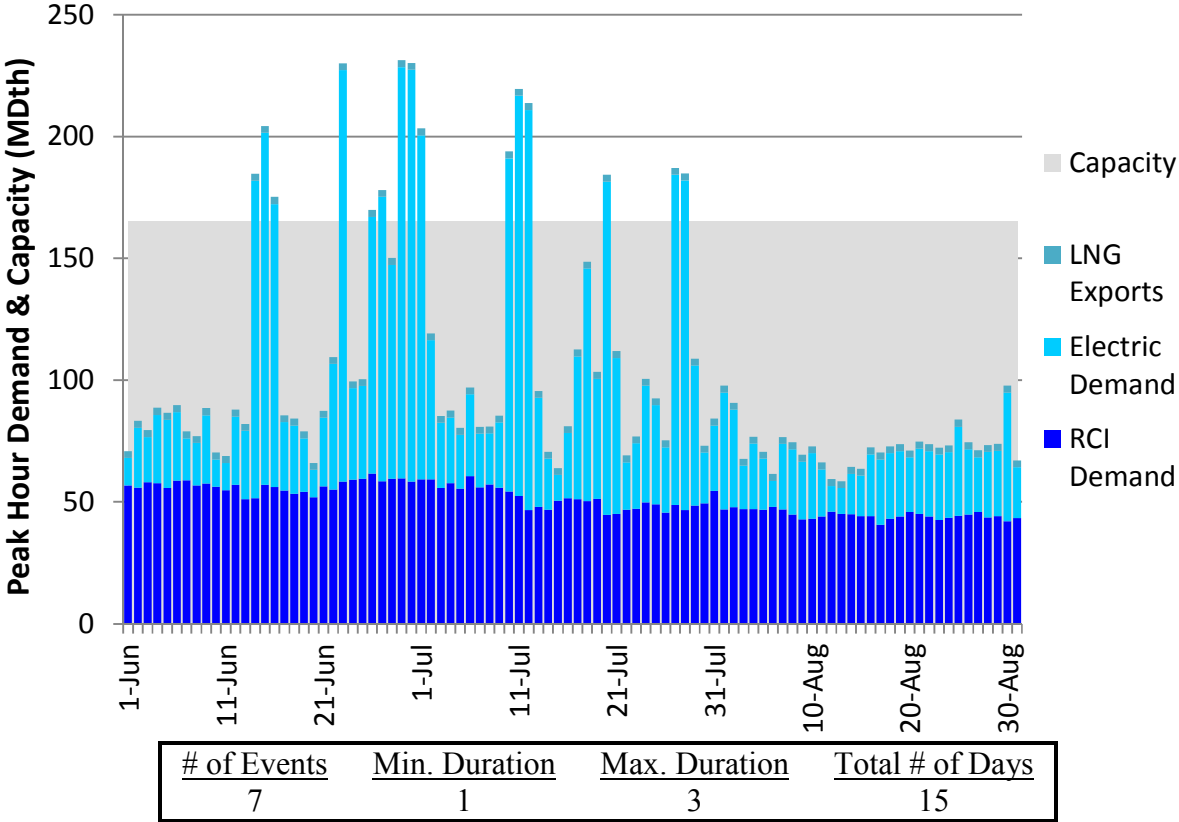
Figure H222. LGDS S2 Summer 2023 – Transco Z5 – Descending Demand
