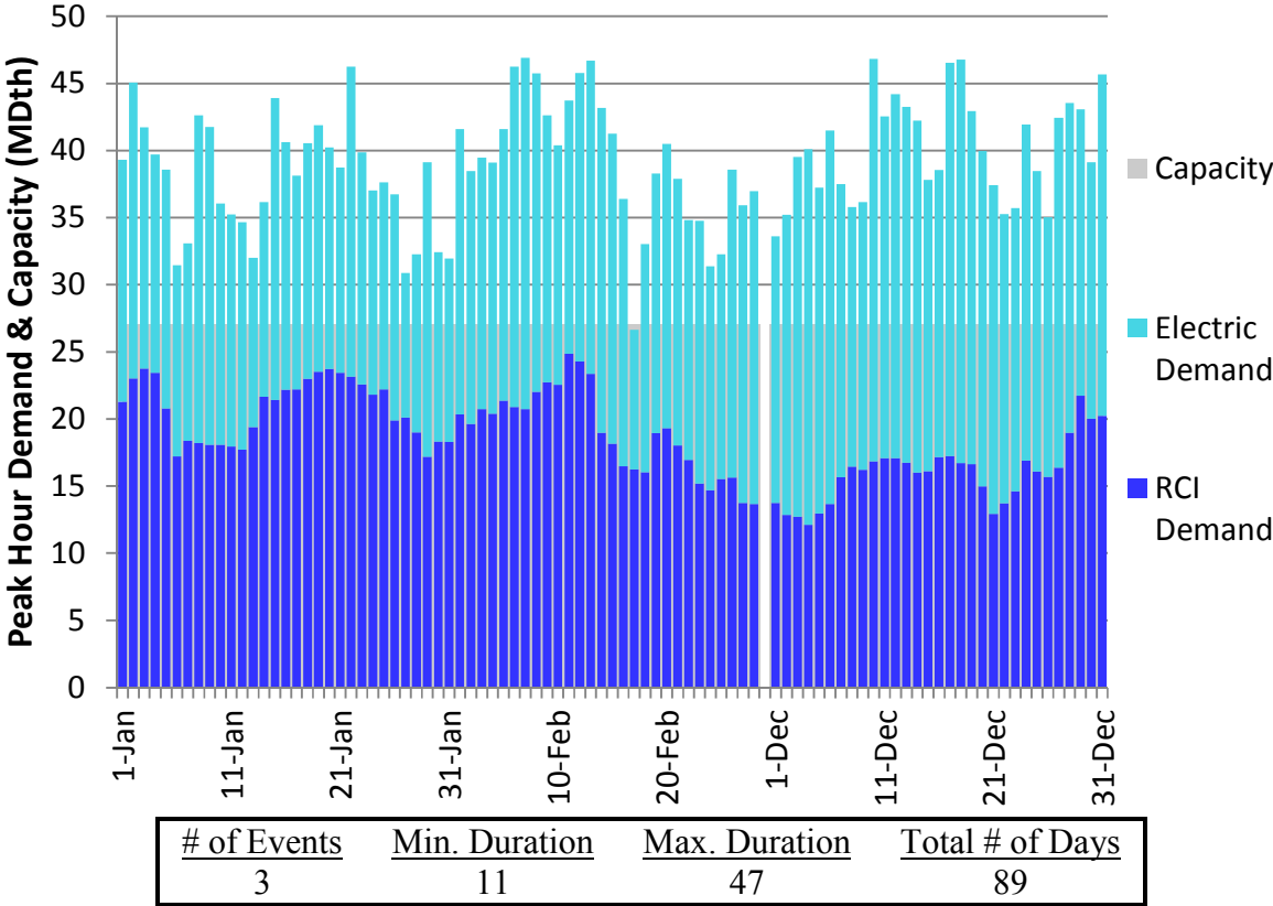
Figure H122. LGDS S2 Winter 2018 – Constitution – Descending Demand
