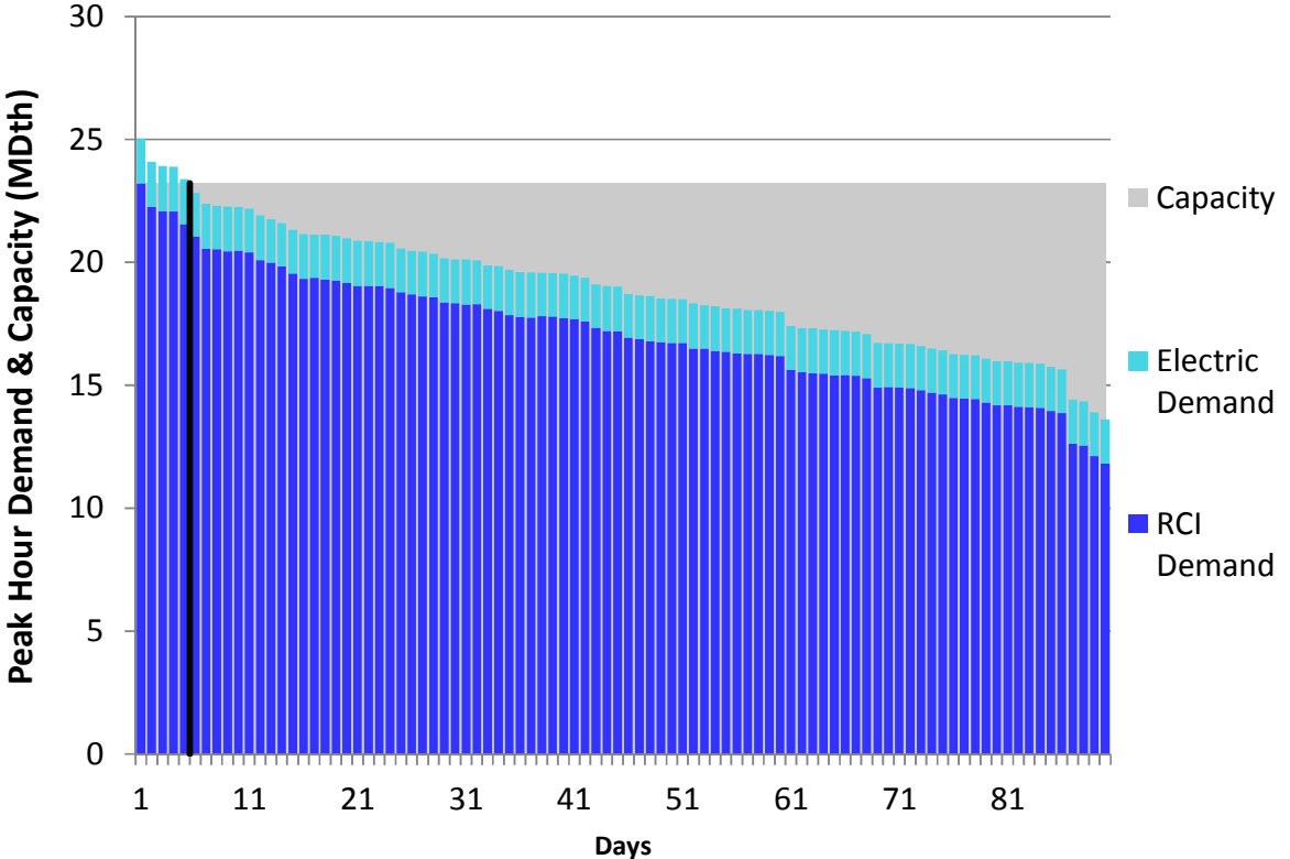
Figure H284. RGDS S3 Winter 2023 – Dominion Western NY– Descending Demand
