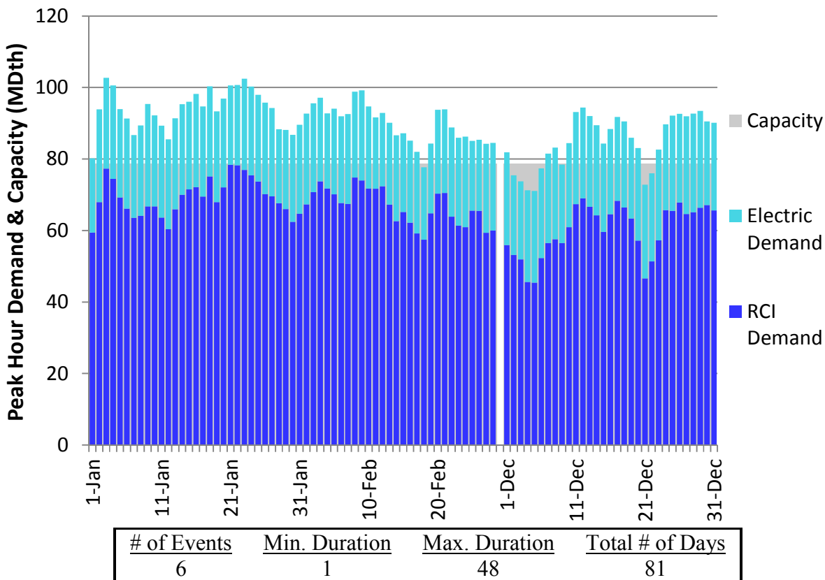
Figure H300. RGDS S3 Winter 2023 – Tennessee Z4 PA – Descending Demand
