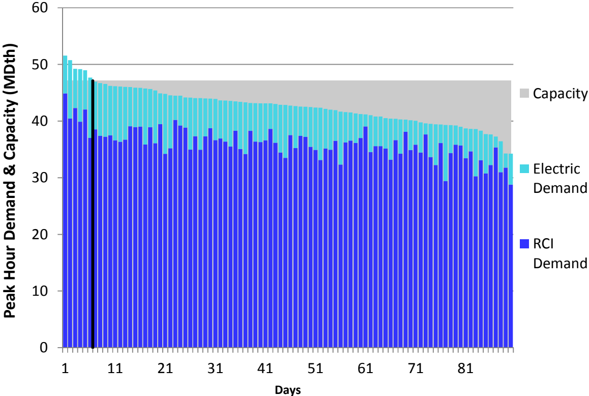
Figure H168. LGDS S2 Winter 2023 – Columbia Gas W PA/NY – Descending Demand
