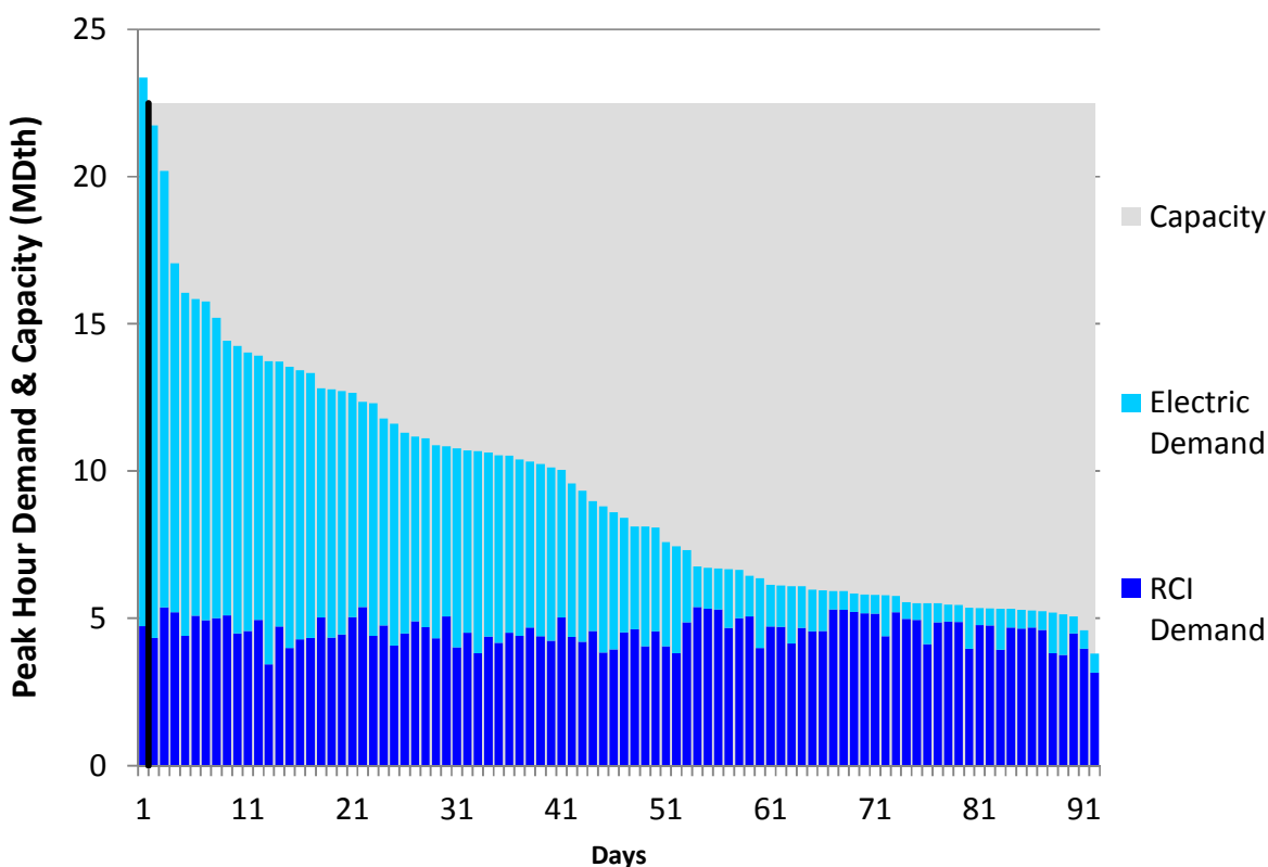
Figure H158. LGDS S2 Summer 2018 – Dominion Southeast – Descending Demand
