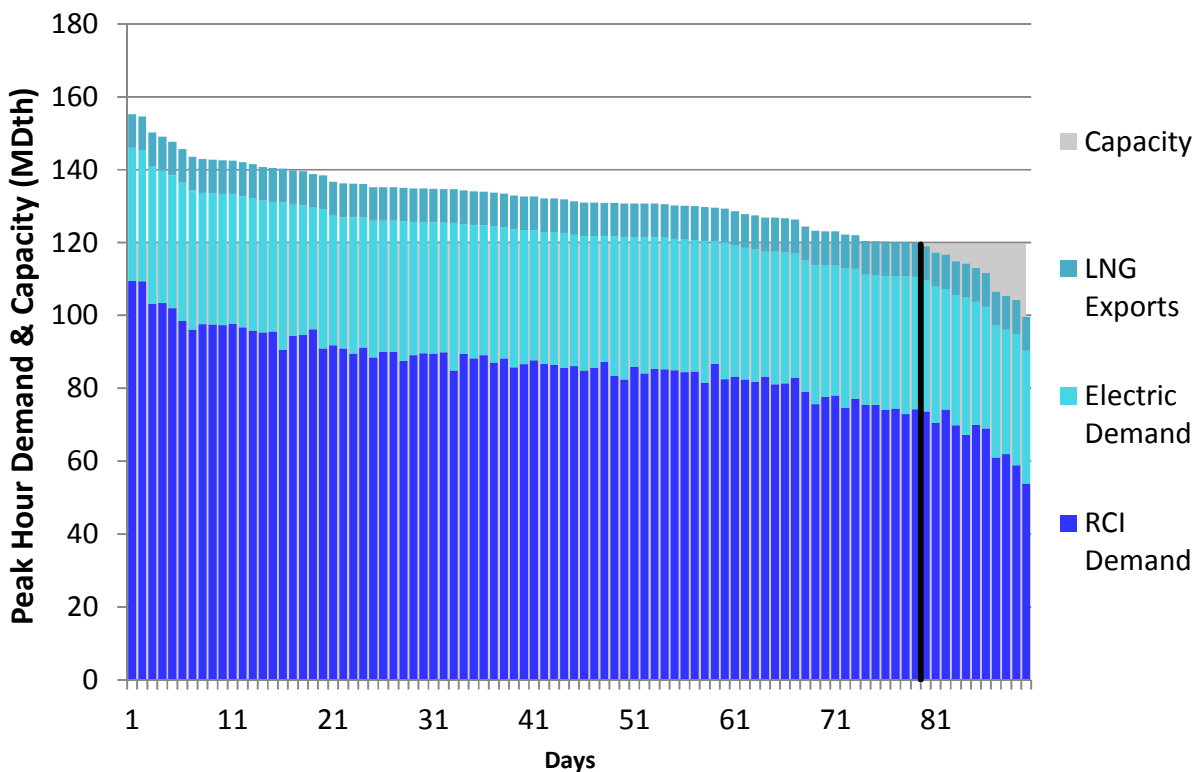
Figure H60. HGDS S2 Winter 2023 – Columbia Gas VA/MD – Descending Demand
