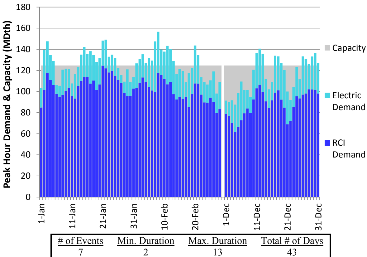
Figure H144. LGDS S2 Winter 2018 – Texas Eastern M3 North – Descending Demand
