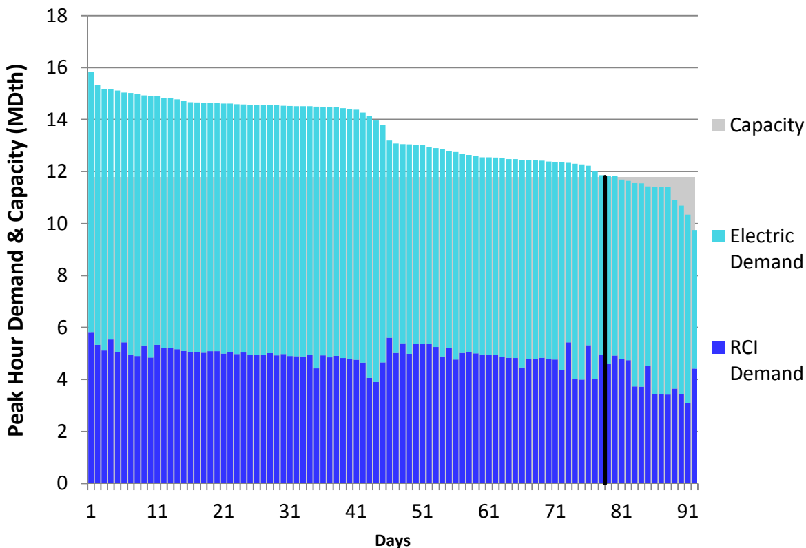
Figure H328. RGDS S3 Summer 2023 – NB/NS Supply – Descending Demand
