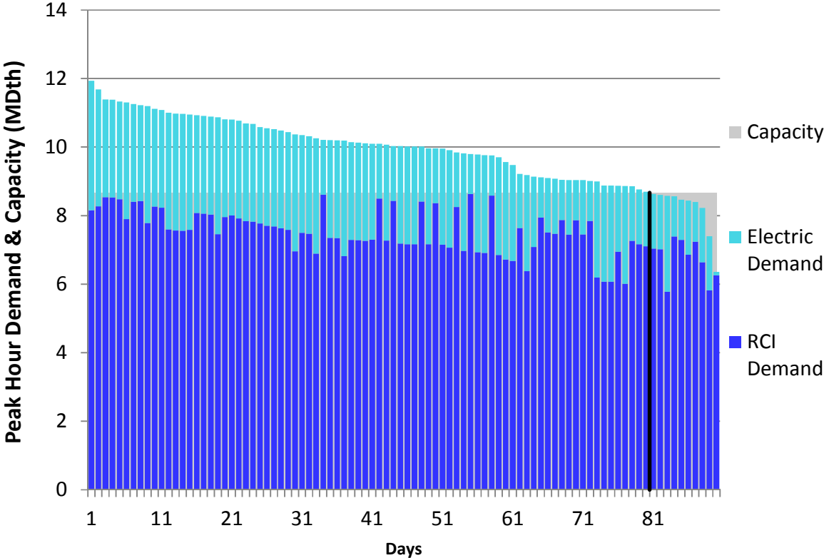
Figure H74. HGDS S2 Winter 2023 – Eastern Shore – Descending Demand
