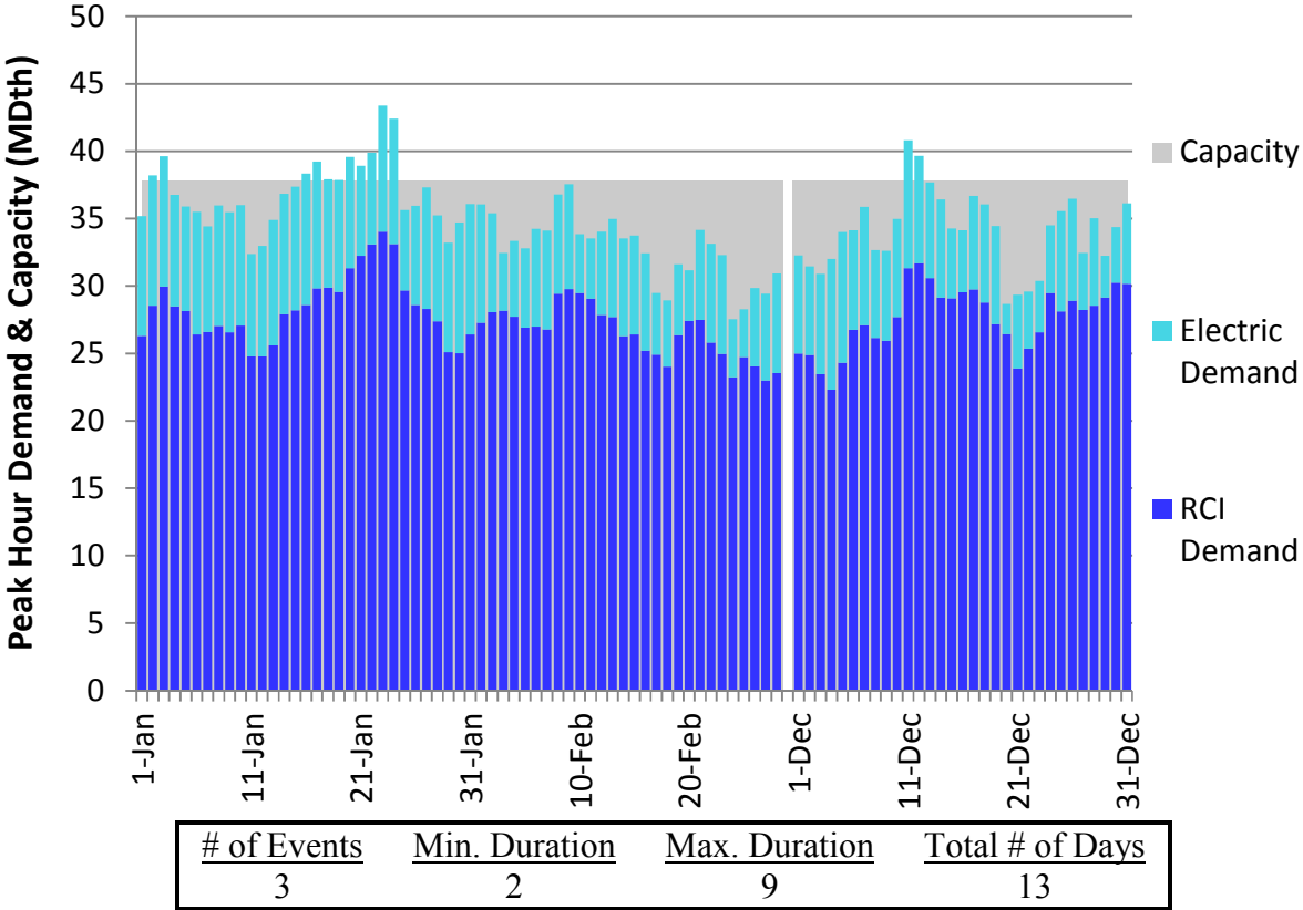
Figure H172. LGDS S2 Winter 2023 – Dominion Eastern NY– Descending Demand
