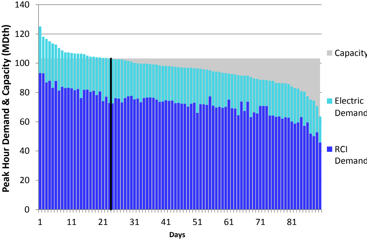
Figure H120. LGDS S2 Winter 2018 – Columbia Gas VA/MD – Descending Demand
