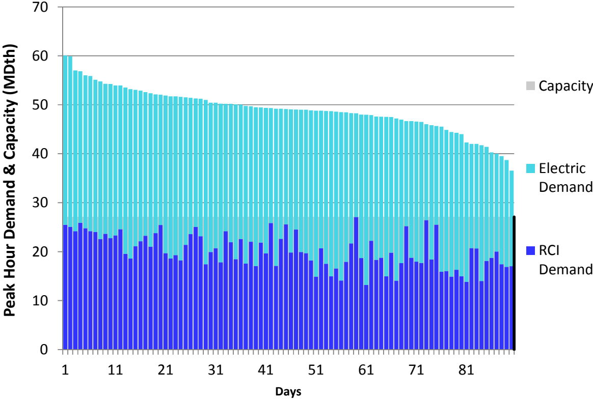
Figure H280. RGDS S3 Winter 2023 – Constitution – Descending Demand
