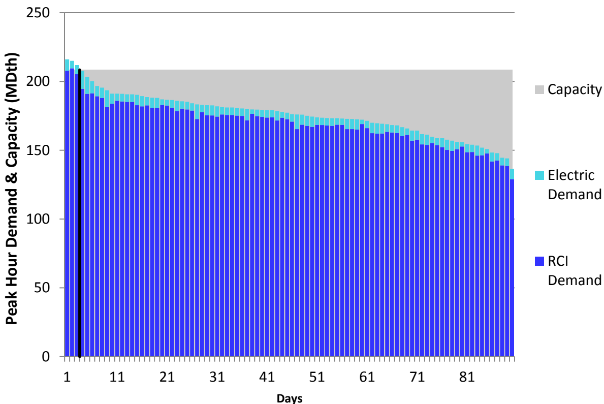
Figure H154. LGDS S2 Winter 2018 – Union Gas Dawn – Descending Demand
