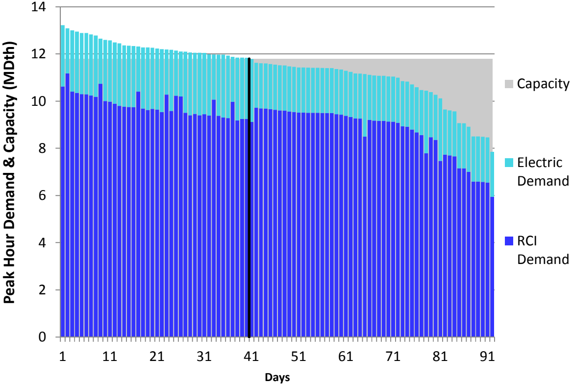
Figure H216. LGDS S2 Summer 2023 – NB/NS Supply – Descending Demand
