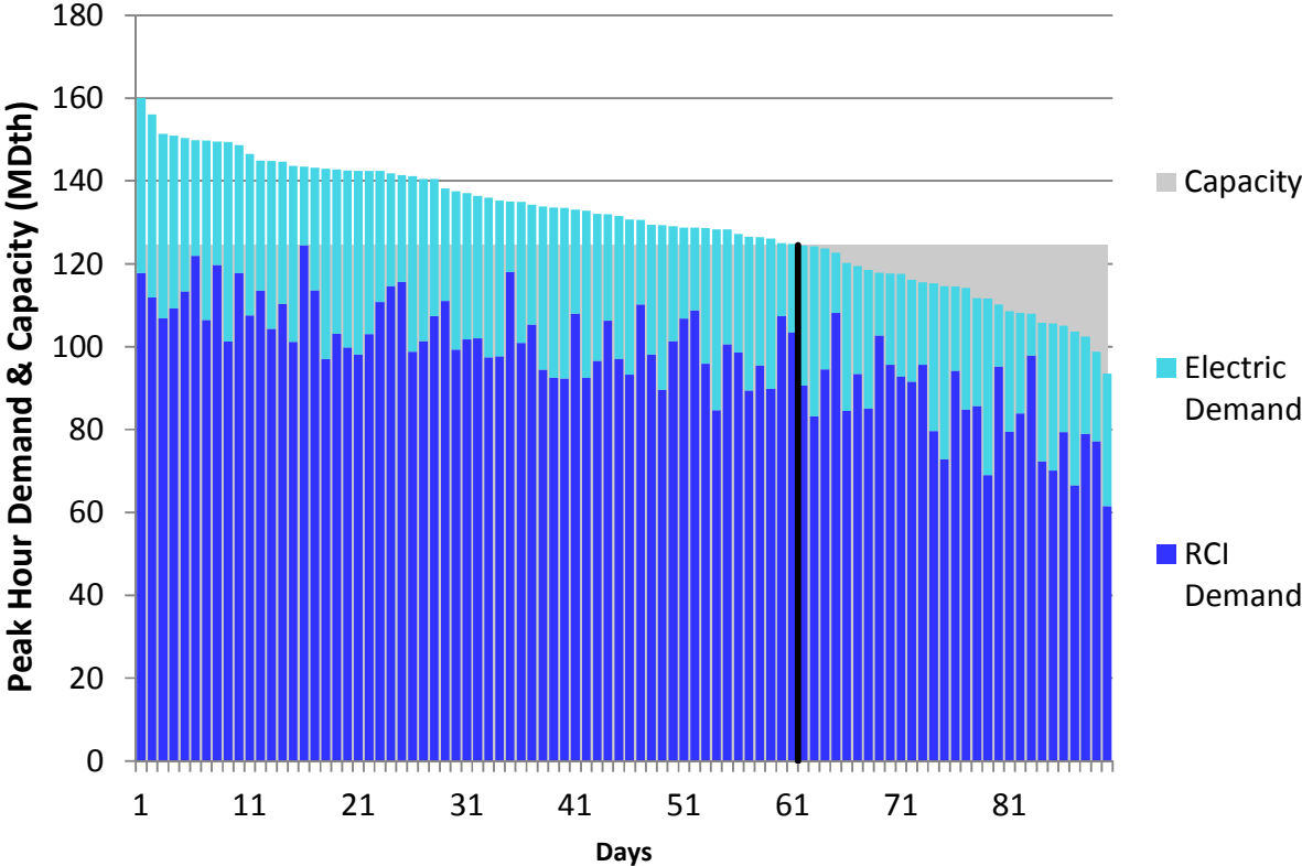
Figure H30. HGDS S2 Winter 2018 – Texas Eastern M3 North – Descending Demand
