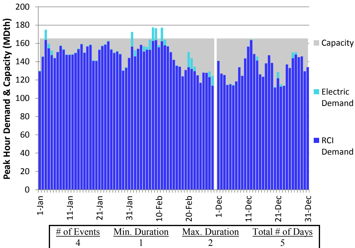
Figure H38. HGDS S2 Winter 2018 – Transco Z5 – Descending Demand
