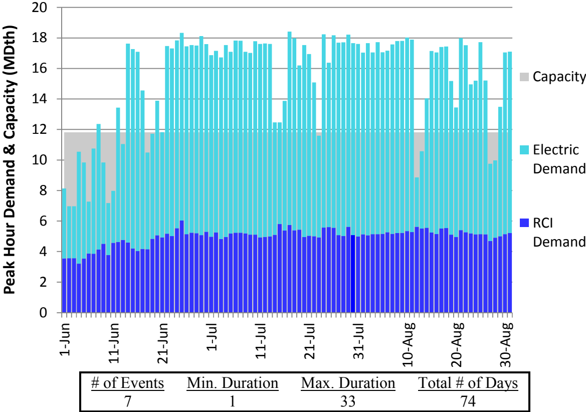
Figure H110. HGDS S2 Summer 2023 – NB/NS Supply – Descending Demand
