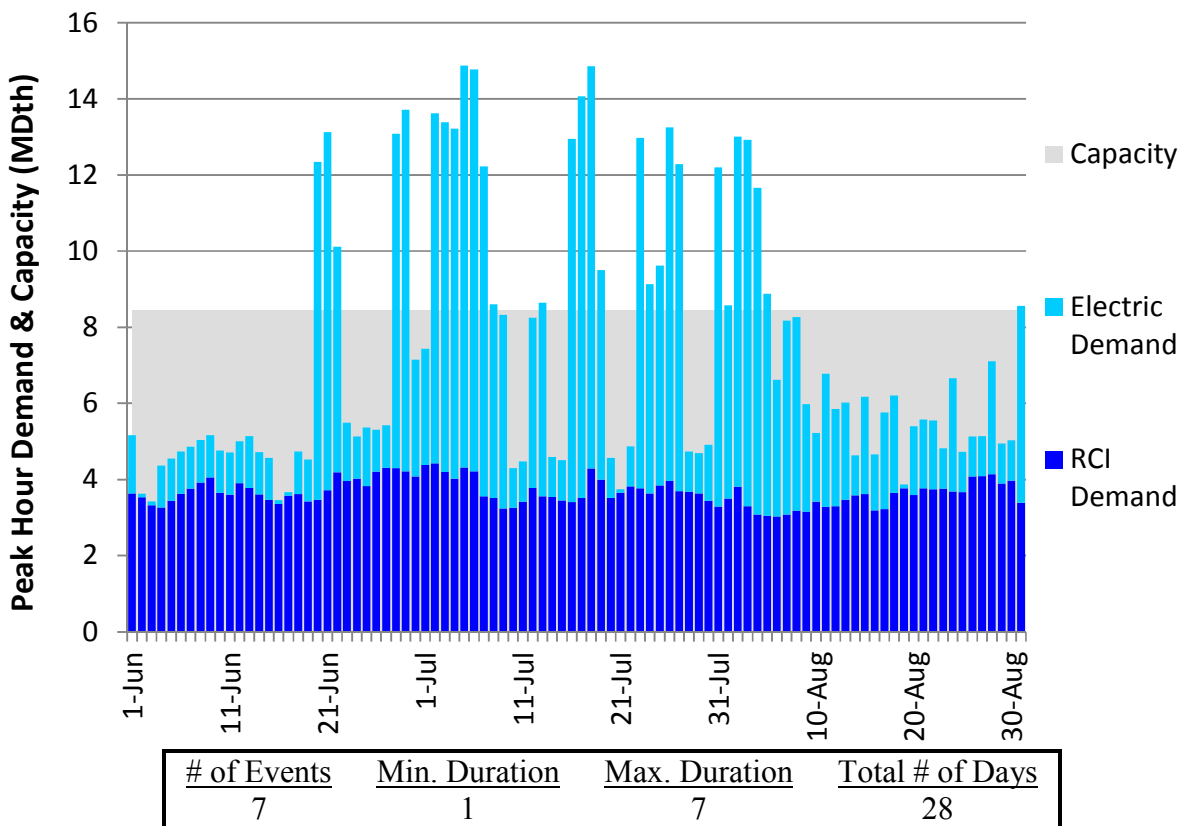
Figure H50. HGDS S2 Summer 2018 – Eastern Shore – Descending Demand
