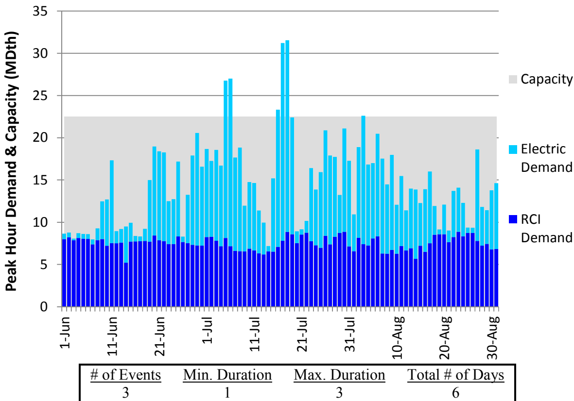
Figure H48. HGDS S2 Summer 2018 – Dominion Southeast – Descending Demand
