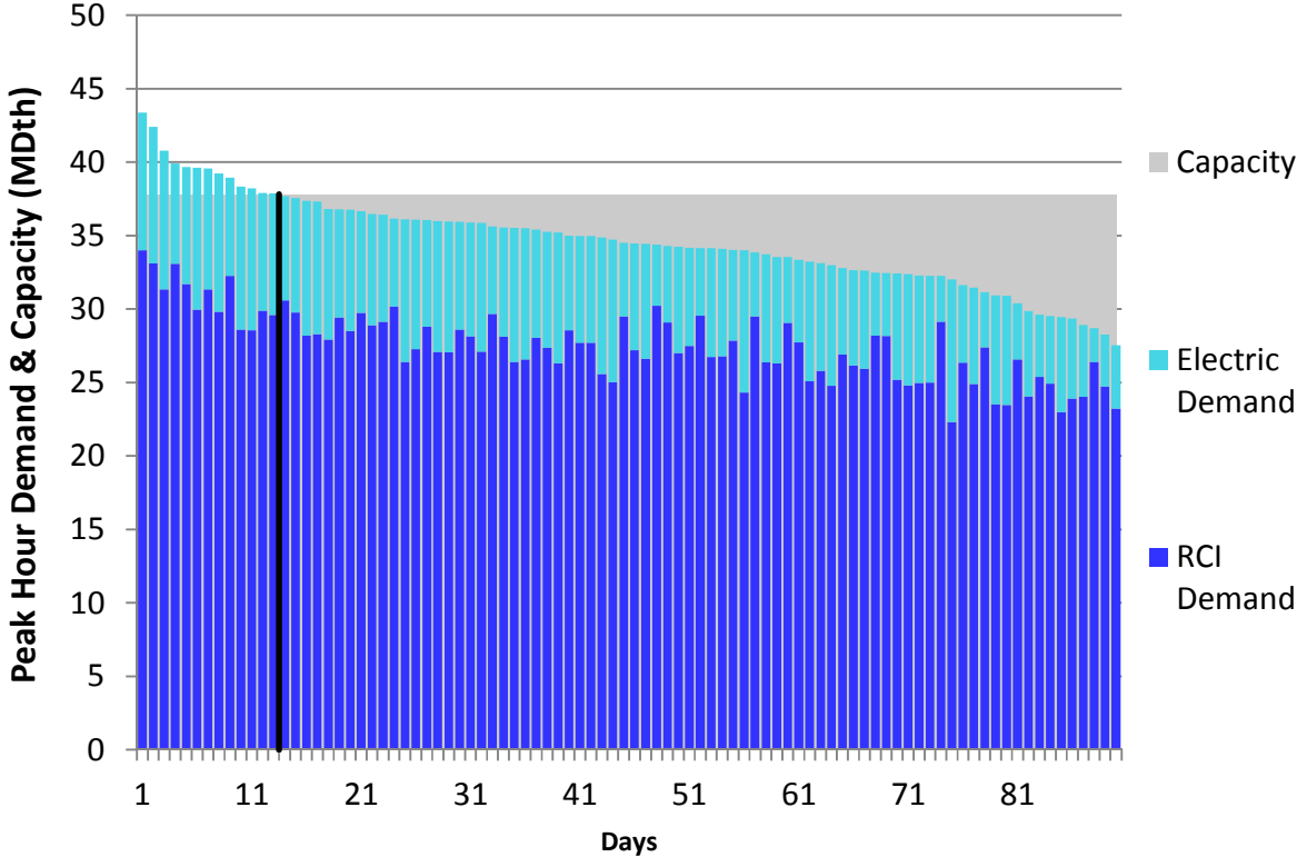
Figure H172. LGDS S2 Winter 2023 – Dominion Eastern NY– Descending Demand
