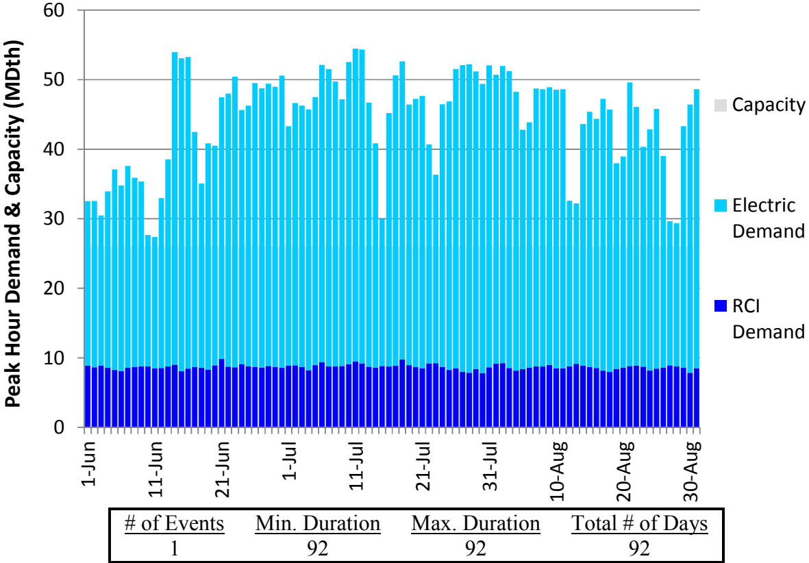
Figure H332. RGDS S3 Summer 2023 – Tennessee Z5 NY – Descending Demand
