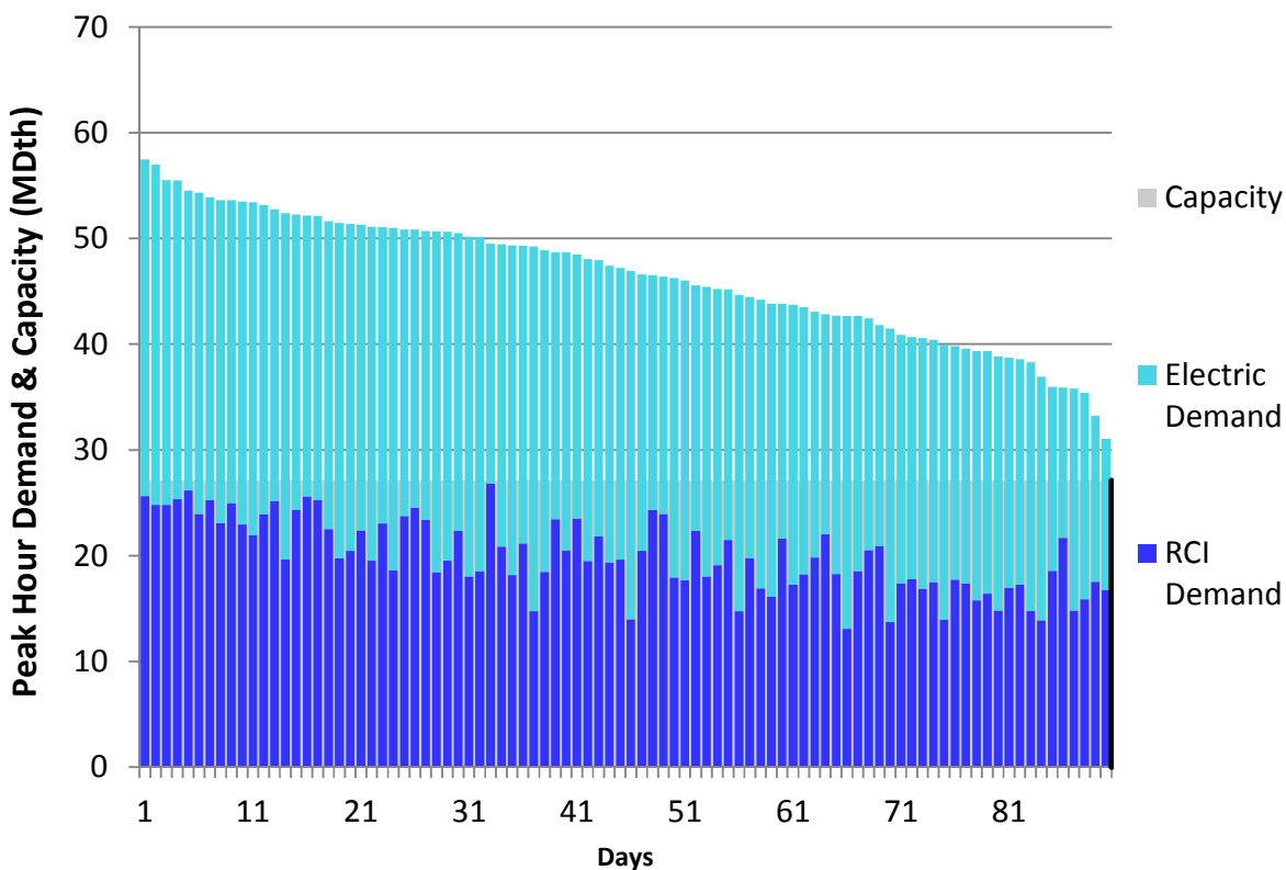
Figure H228. RGDS S3 Winter 2018 – Constitution – Descending Demand
