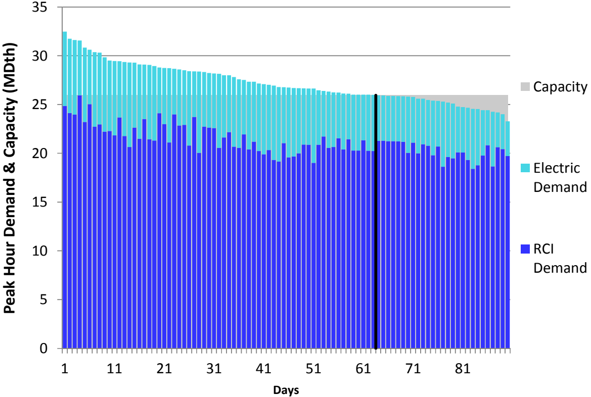
Figure H244. RGDS S3 Winter 2018 – NB/NS Supply – Descending Demand
