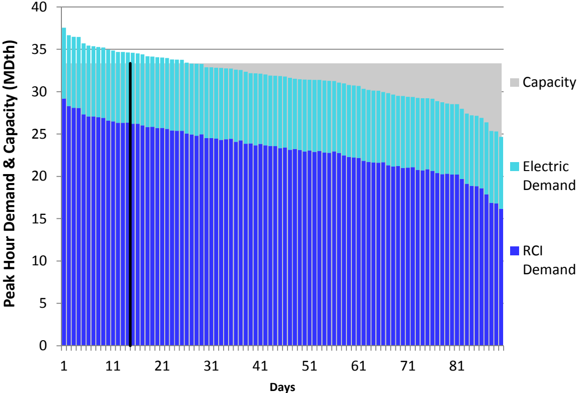
Figure H14. HGDS S2 Winter 2018 – East Tennessee – Descending Demand
