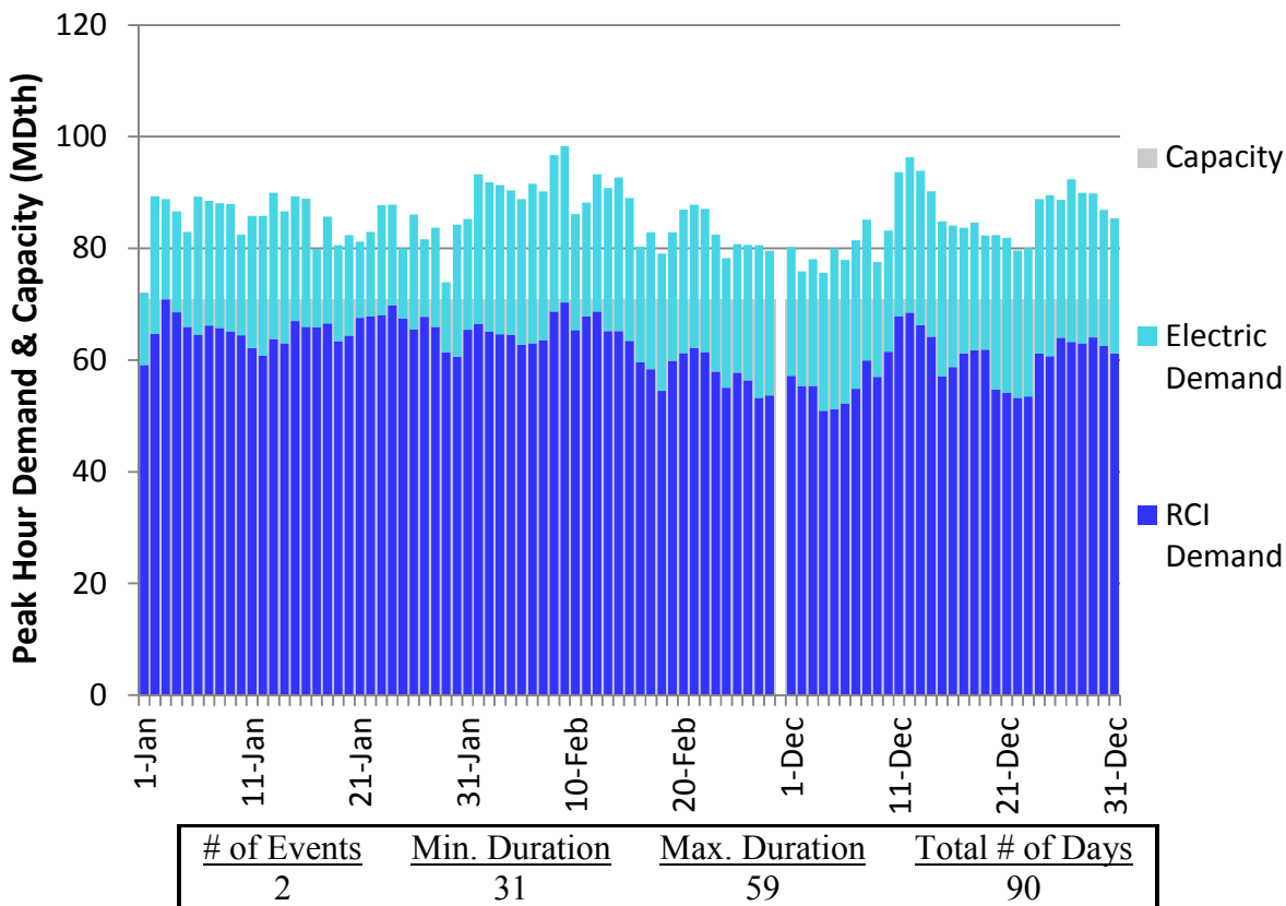
Figure H312. RGDS S3 Winter 2023 – Transco Leidy Atlantic – Descending Demand
