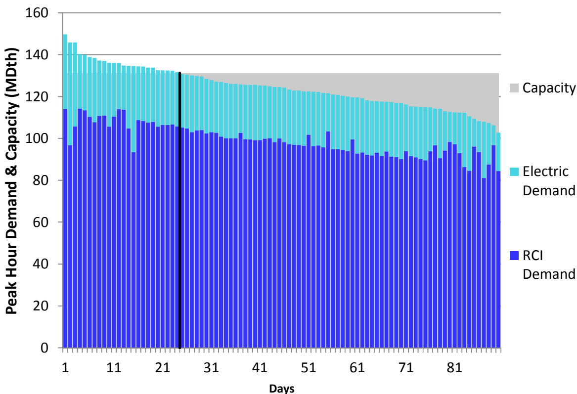
Figure H308. RGDS S3 Winter 2023 – TransCanada Ontario West – Descending Demand
