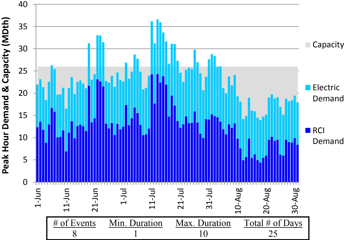
Figure H116. HGDS S2 Summer 2023 – Texas Eastern ETX – Descending Demand
