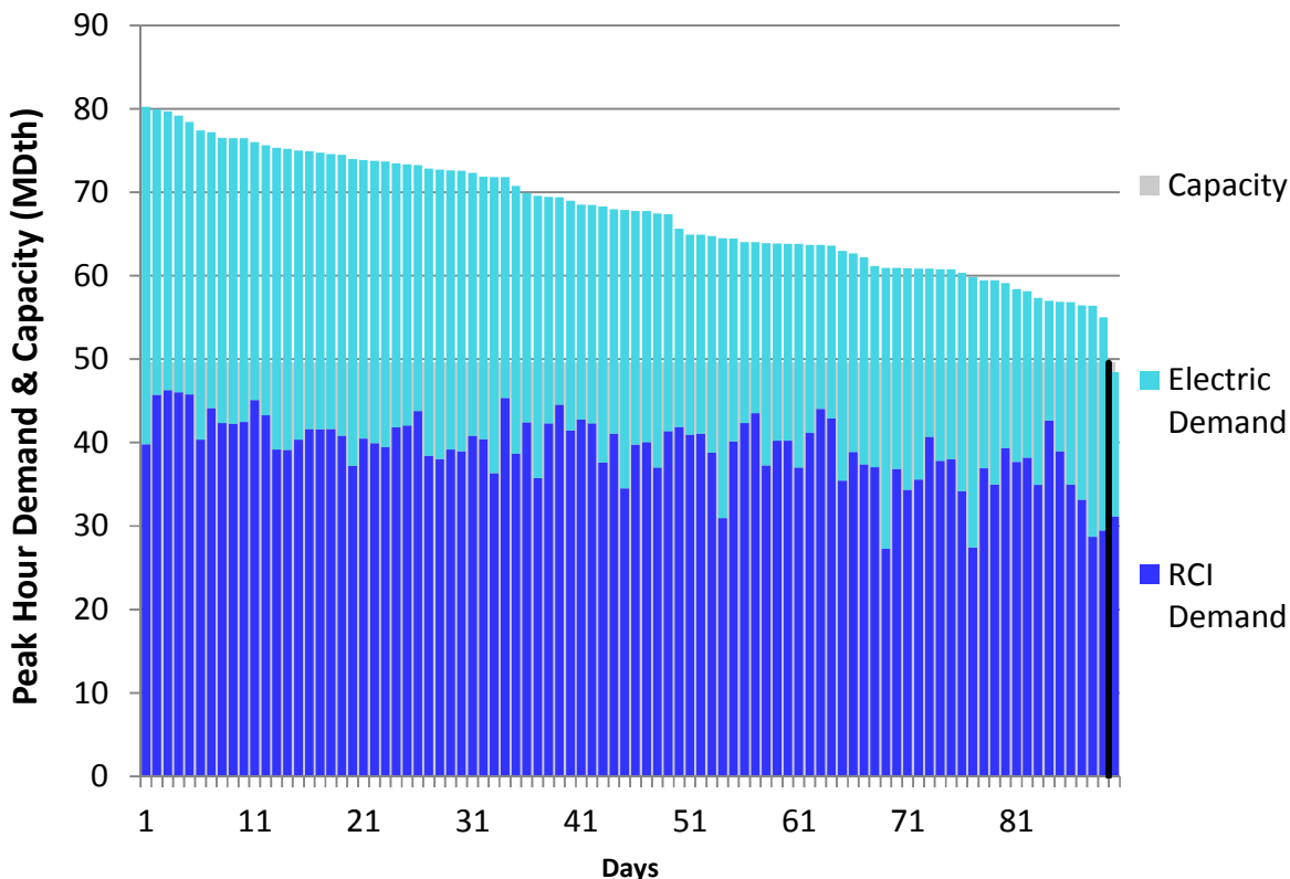
Figure H302. RGDS S3 Winter 2023 – Tennessee Z5 NY – Descending Demand
