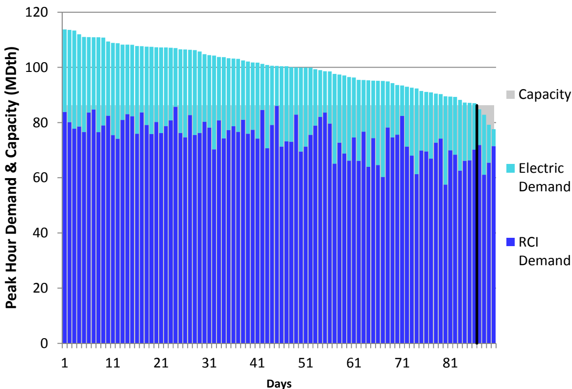
Figure H86. HGDS S2 Winter 2023 – Texas Eastern M2 PA South – Descending Demand
