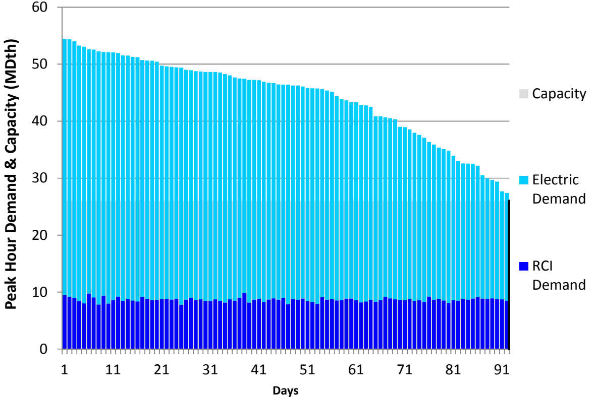
Figure H332. RGDS S3 Summer 2023 – Tennessee Z5 NY – Descending Demand
