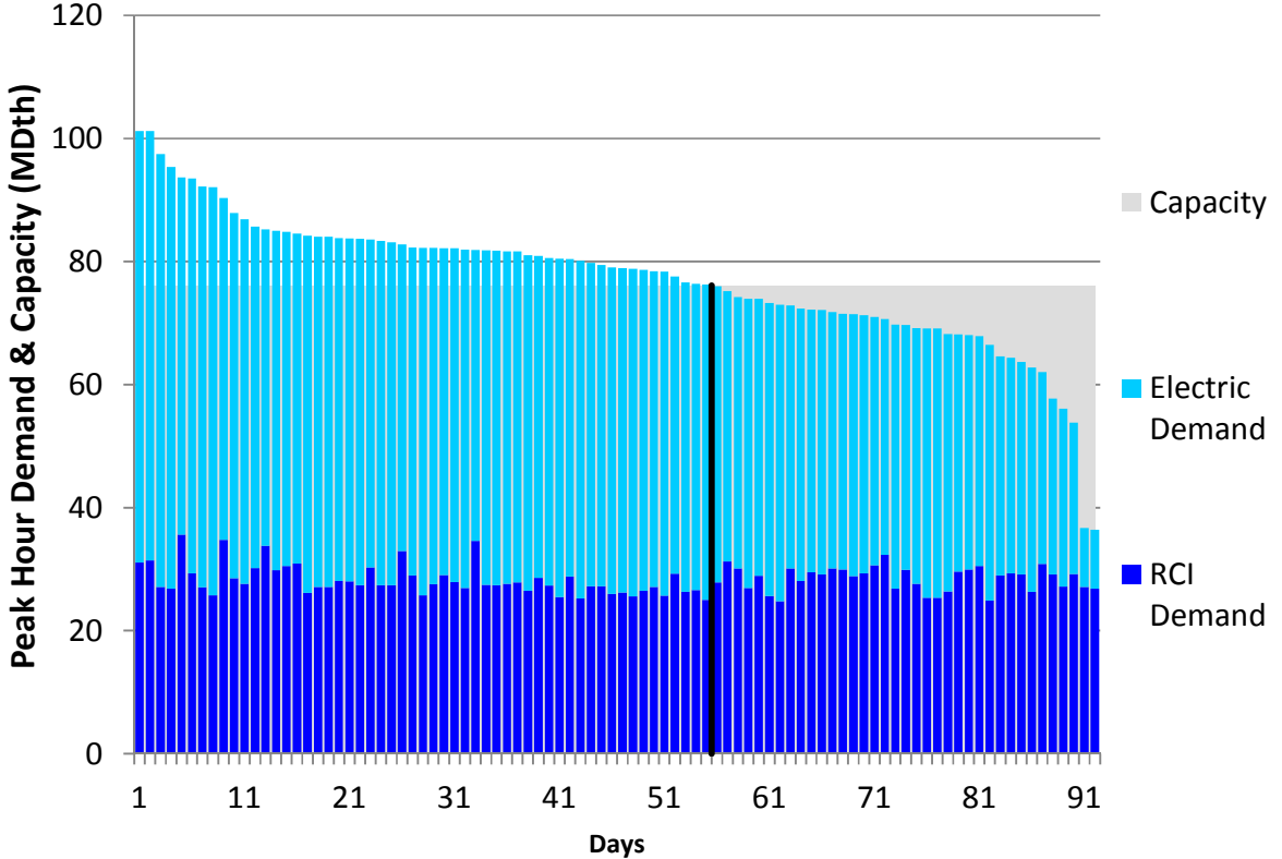
Figure H102. HGDS S2 Summer 2023 – Algonquin CT – Descending Demand
