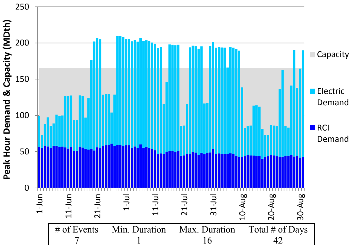
Figure H274. RGDS S3 Summer 2018 – Transco Z5 – Descending Demand
