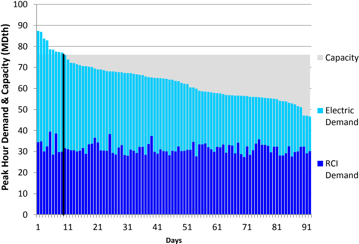
Figure H208. LGDS S2 Summer 2023 – Algonquin CT – Descending Demand
