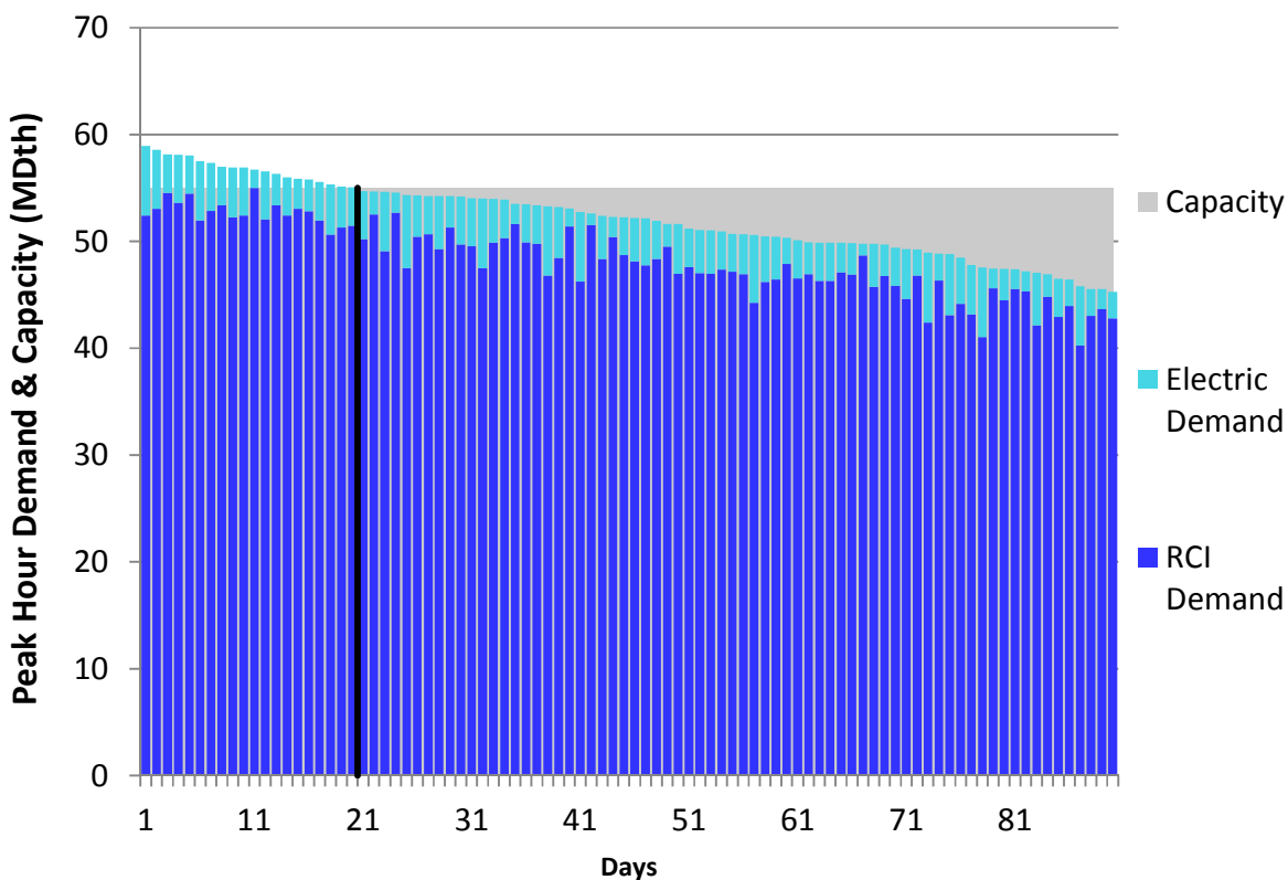
Figure H198. LGDS S2 Winter 2023 – TransCanada Quebec – Descending Demand
