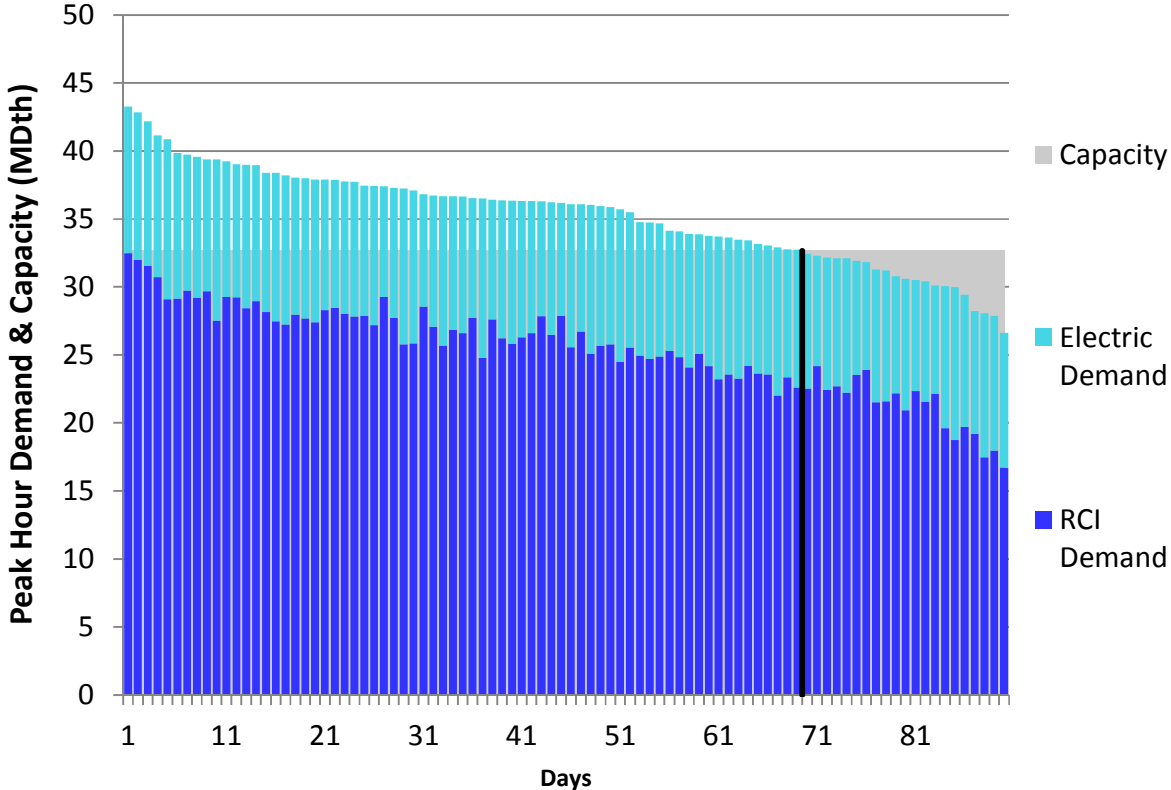
Figure H296. RGDS S3 Winter 2023 – Millennium – Descending Demand
