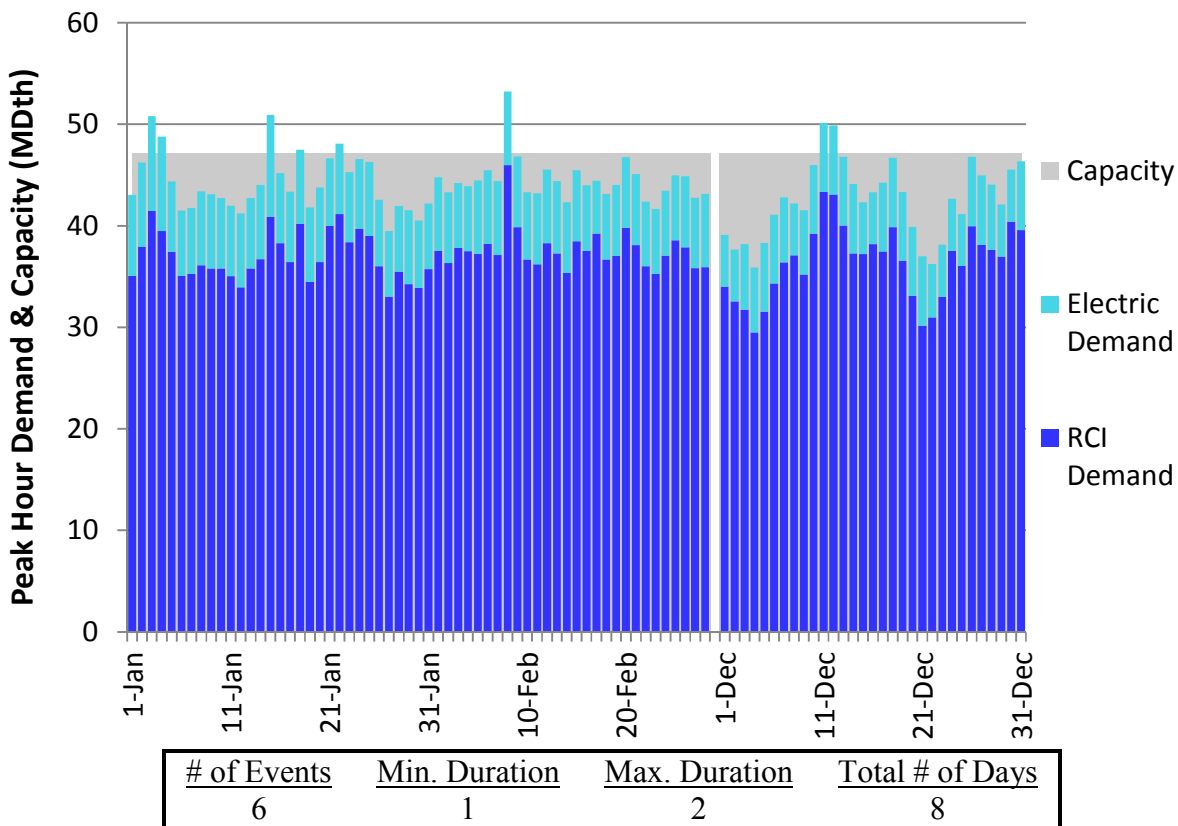
Figure H226. RGDS S3 Winter 2018 – Columbia Gas W PA/NY – Descending Demand
