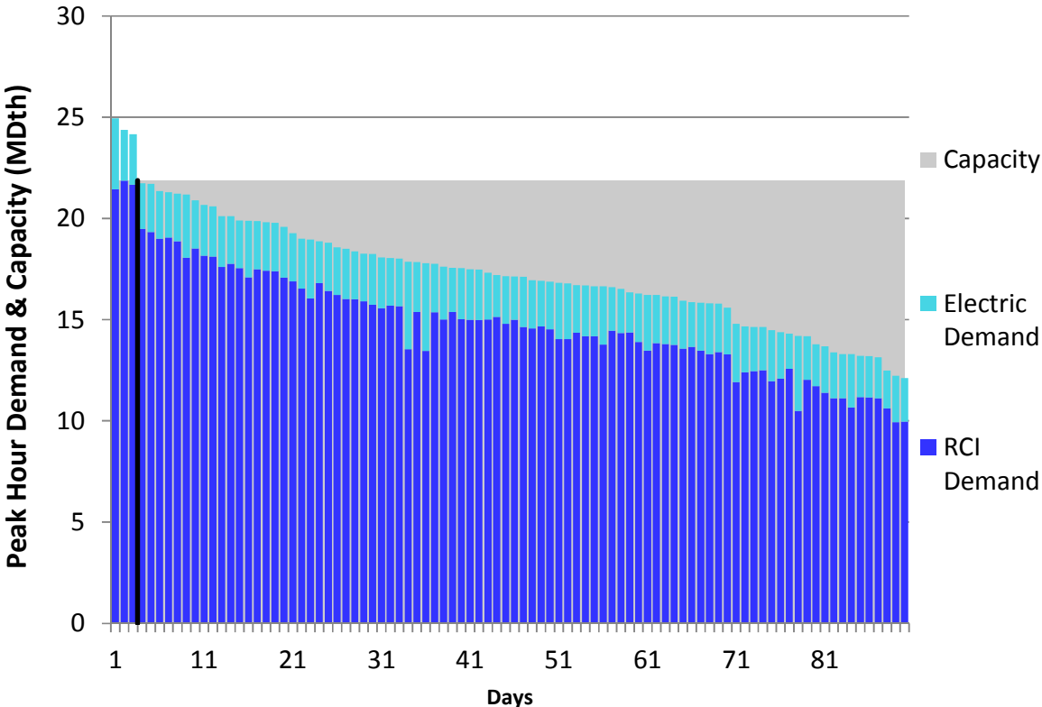
Figure H18. HGDS S2 Winter 2018 – Empire – Descending Demand
