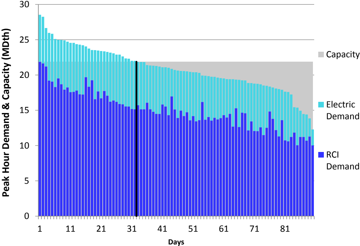
Figure H182. LGDS S2 Winter 2023 – Empire – Descending Demand
