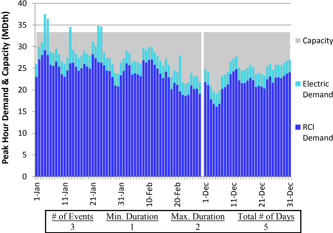
Figure H178. LGDS S2 Winter 2023 – East Tennessee – Descending Demand
