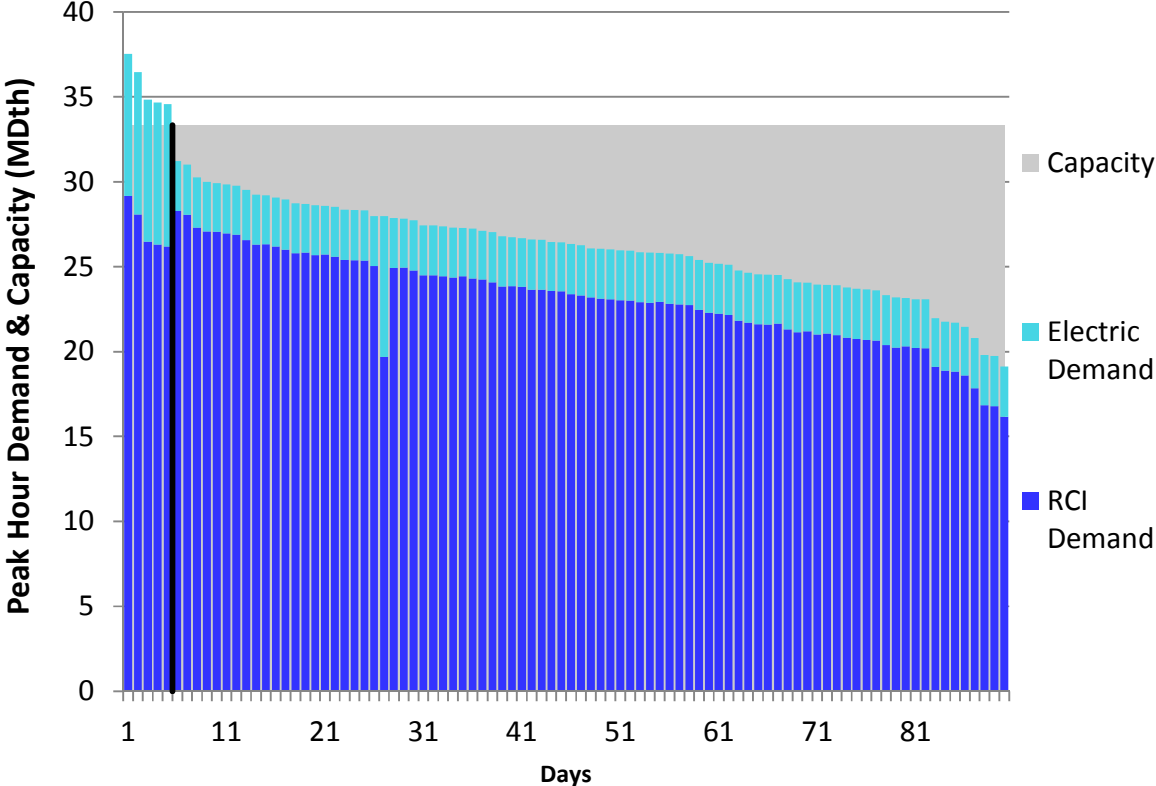
Figure H178. LGDS S2 Winter 2023 – East Tennessee – Descending Demand
