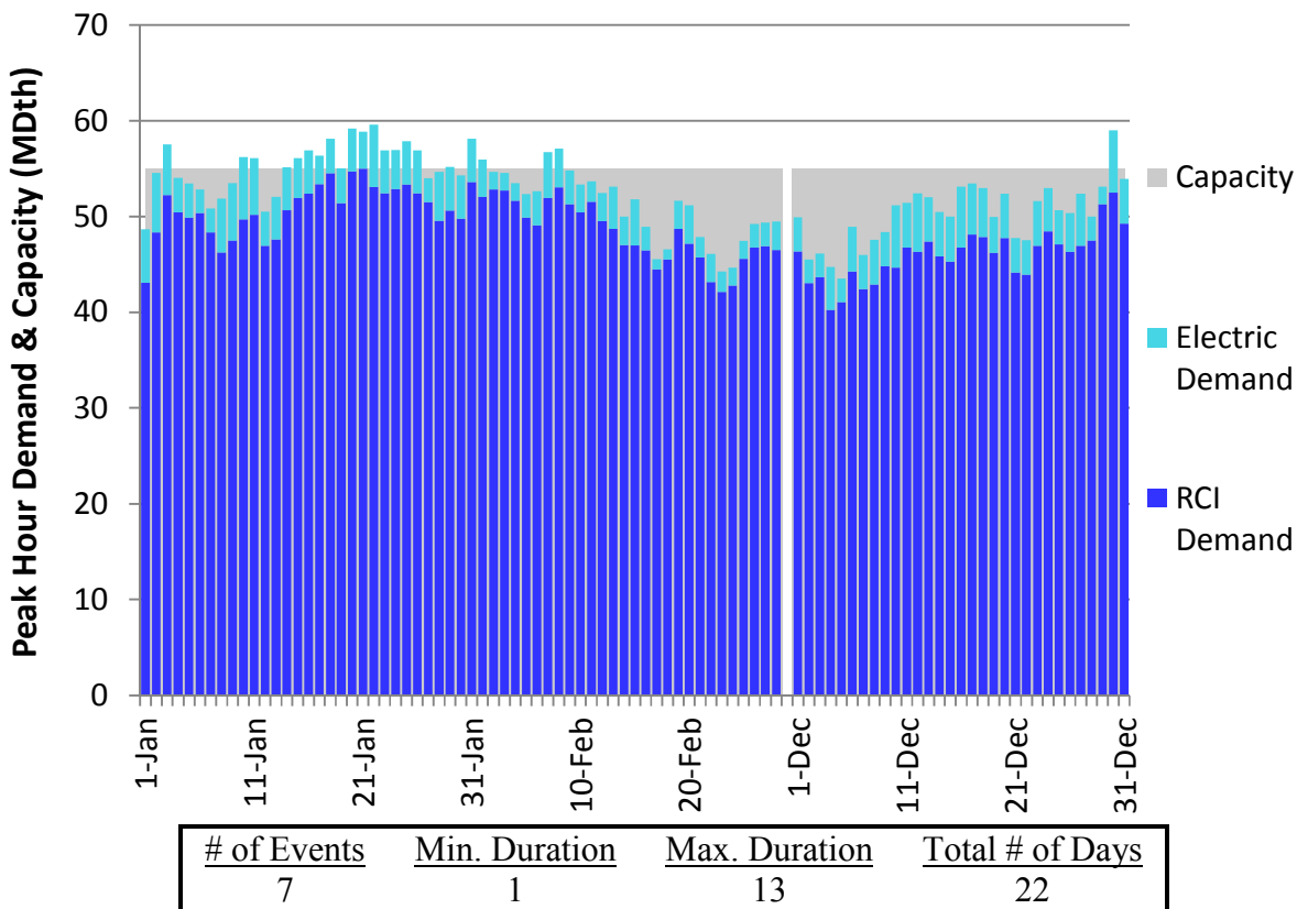
Figure H148. LGDS S2 Winter 2018 – TransCanada Quebec – Descending Demand
