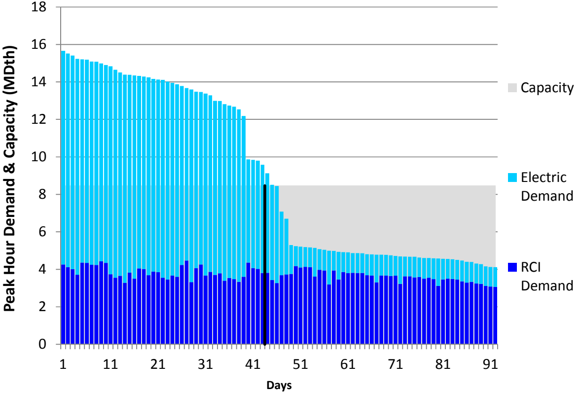
Figure H326. RGDS S3 Summer 2023 – Eastern Shore – Descending Demand
