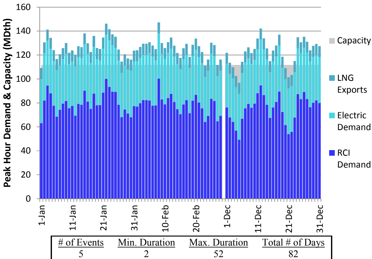
Figure H276. RGDS S3 Winter 2023 – Columbia Gas VA/MD – Descending Demand
