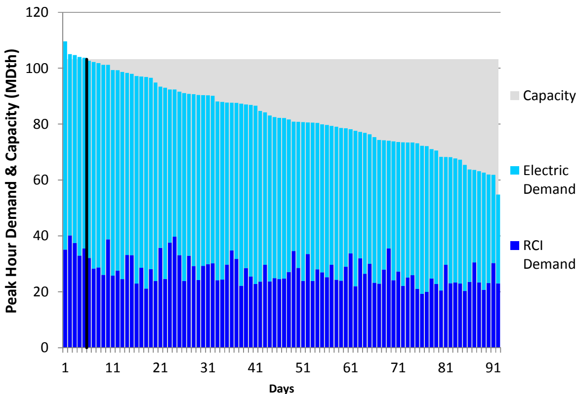
Figure H266. RGDS S3 Summer 2018 – Columbia Gas VA/MD – Descending Demand
