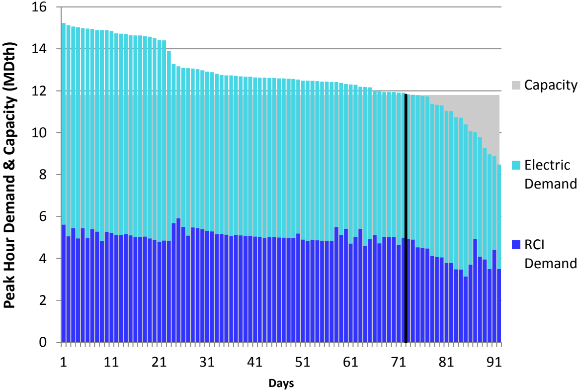
Figure H52. HGDS S2 Summer 2018 – NB/NS Supply – Descending Demand
