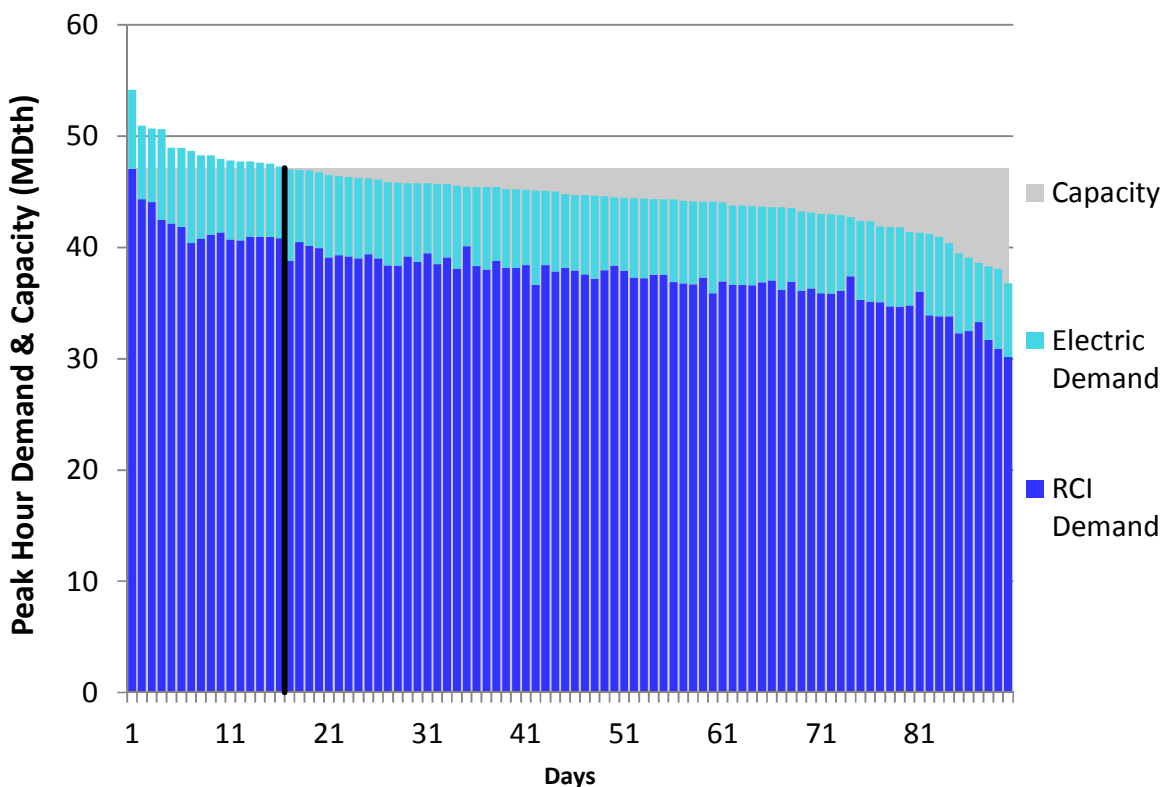
Figure H278. RGDS S3 Winter 2023 – Columbia Gas W PA/NY – Descending Demand
