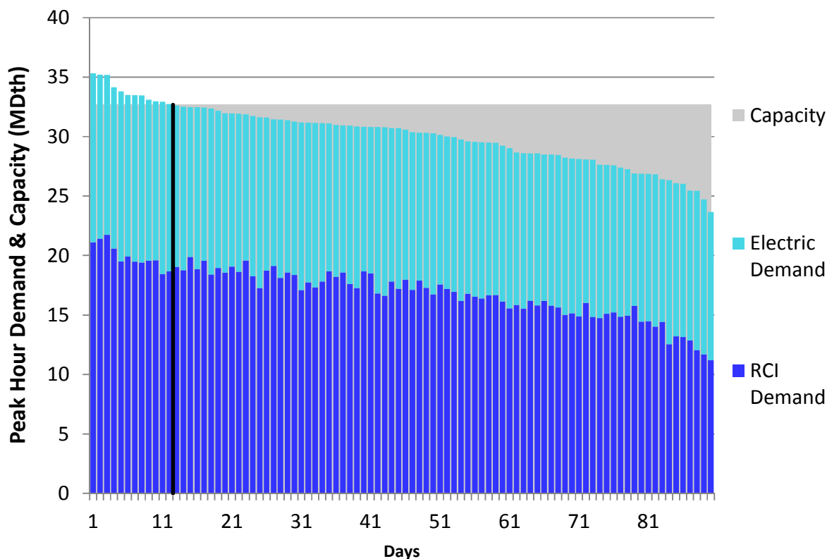
Figure H134. LGDS S2 Winter 2018 – Millennium – Descending Demand
