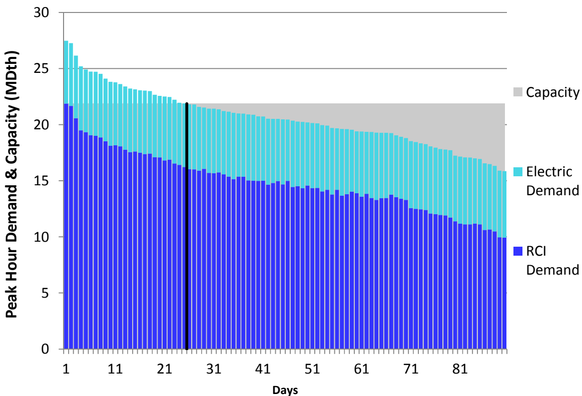
Figure H76. HGDS S2 Winter 2023 – Empire – Descending Demand
