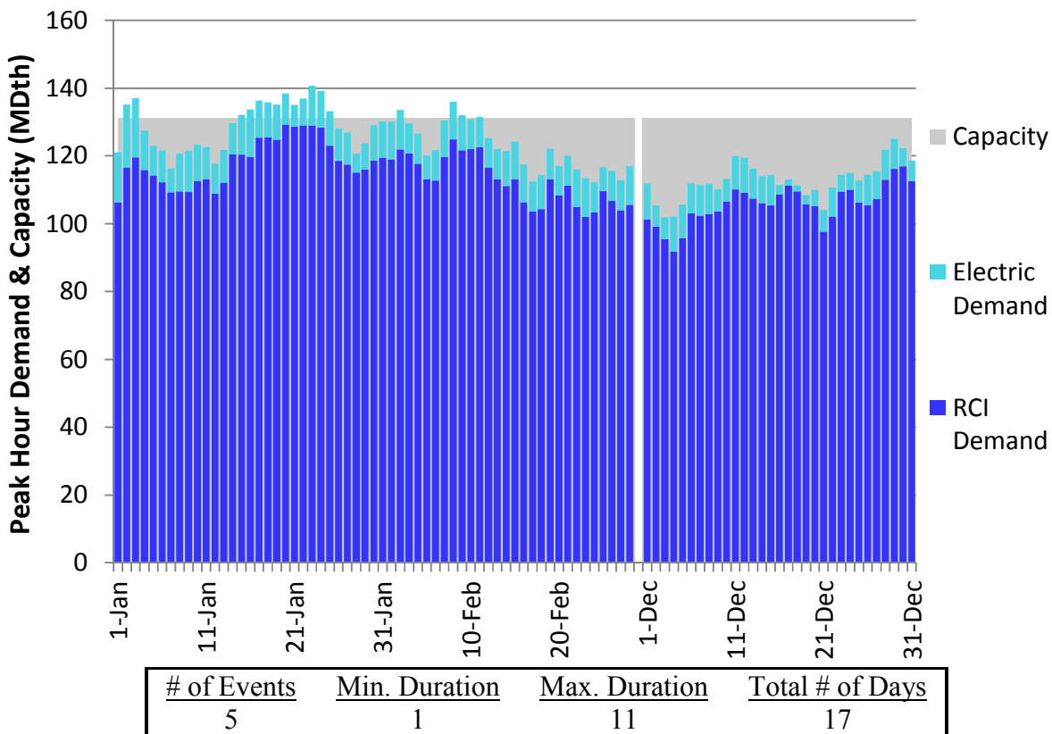
Figure H196. LGDS S2 Winter 2023 – TransCanada Ontario West – Descending Demand
