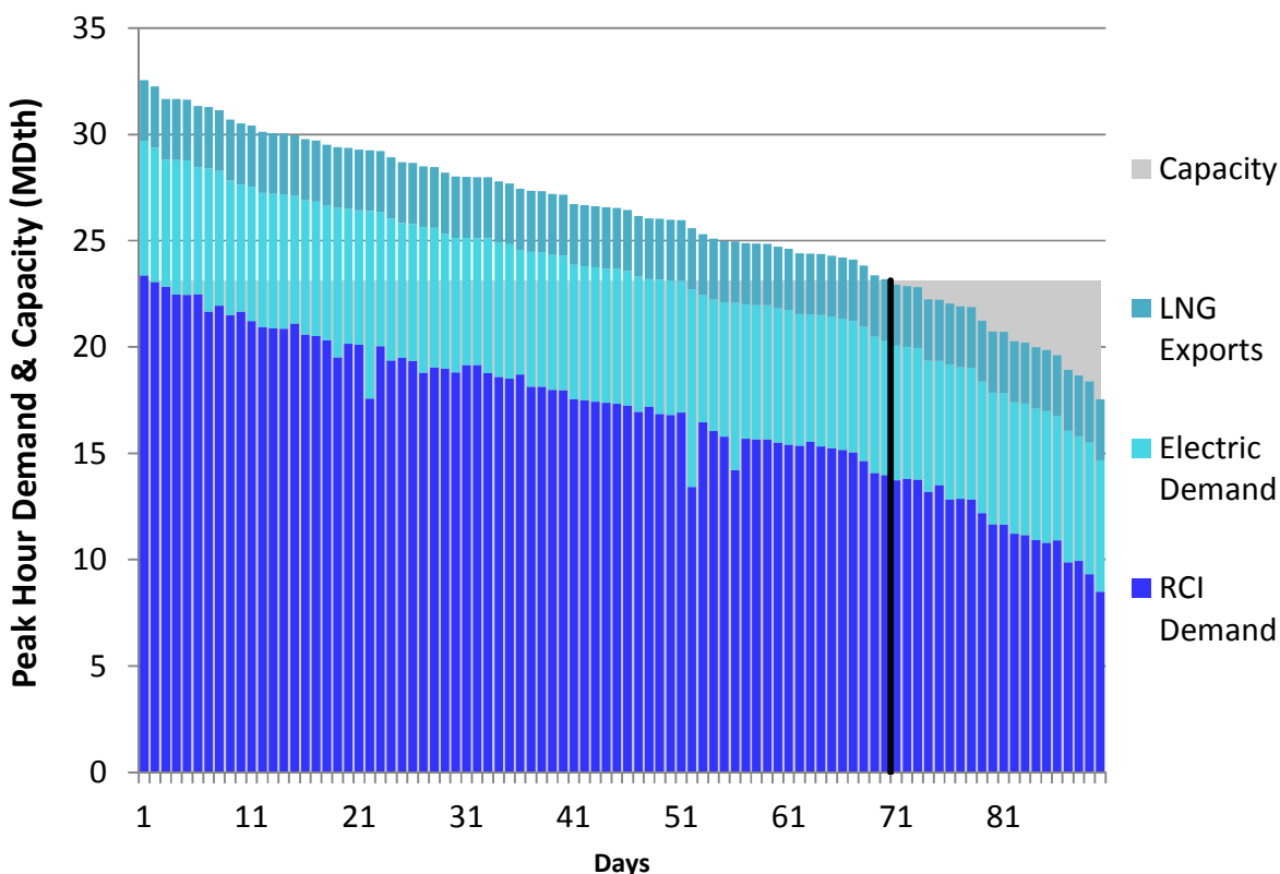
Figure H286. RGDS S3 Winter 2023 – Dominion Southeast – Descending Demand
