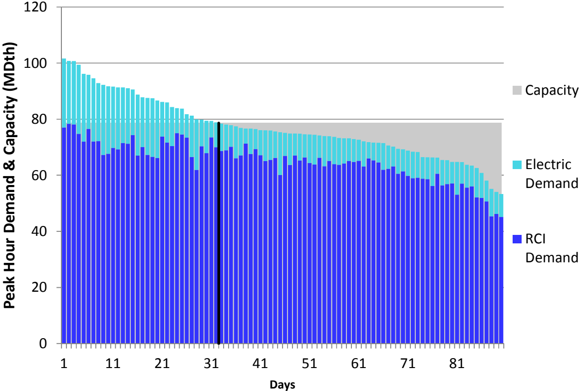
Figure H24. HGDS S2 Winter 2018 – Tennessee Z4 PA – Descending Demand
