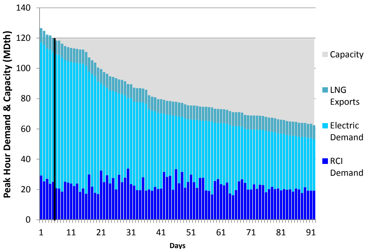
Figure H104. HGDS S2 Summer 2023 – Columbia Gas VA/MD – Descending Demand
