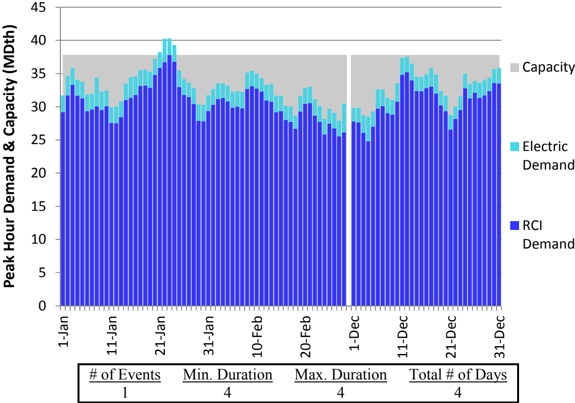
Figure H8. HGDS S2 Winter 2018 – Dominion Eastern NY– Descending Demand
