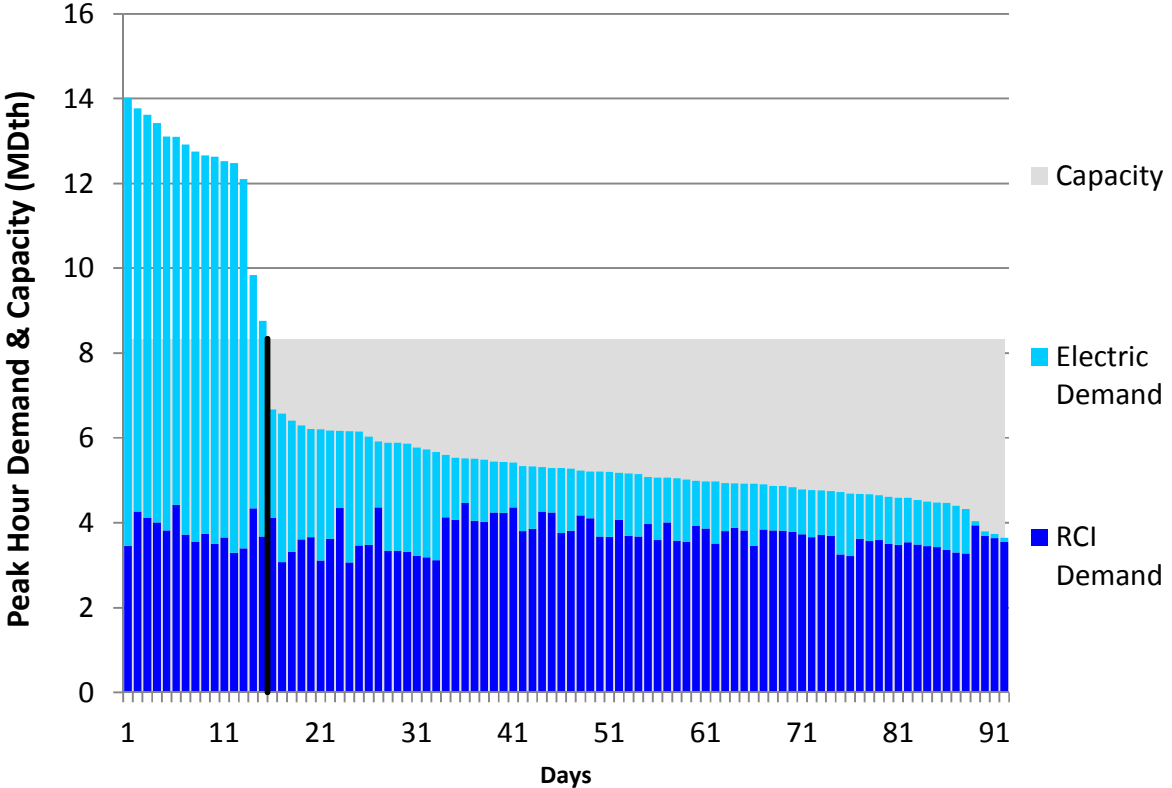
Figure H214. LGDS S2 Summer 2023 – Eastern Shore – Descending Demand
