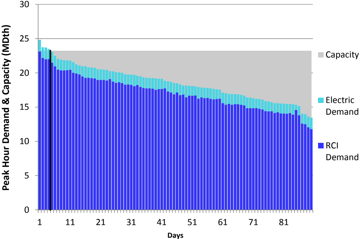
Figure H232. RGDS S3 Winter 2018 – Dominion Western NY– Descending Demand
