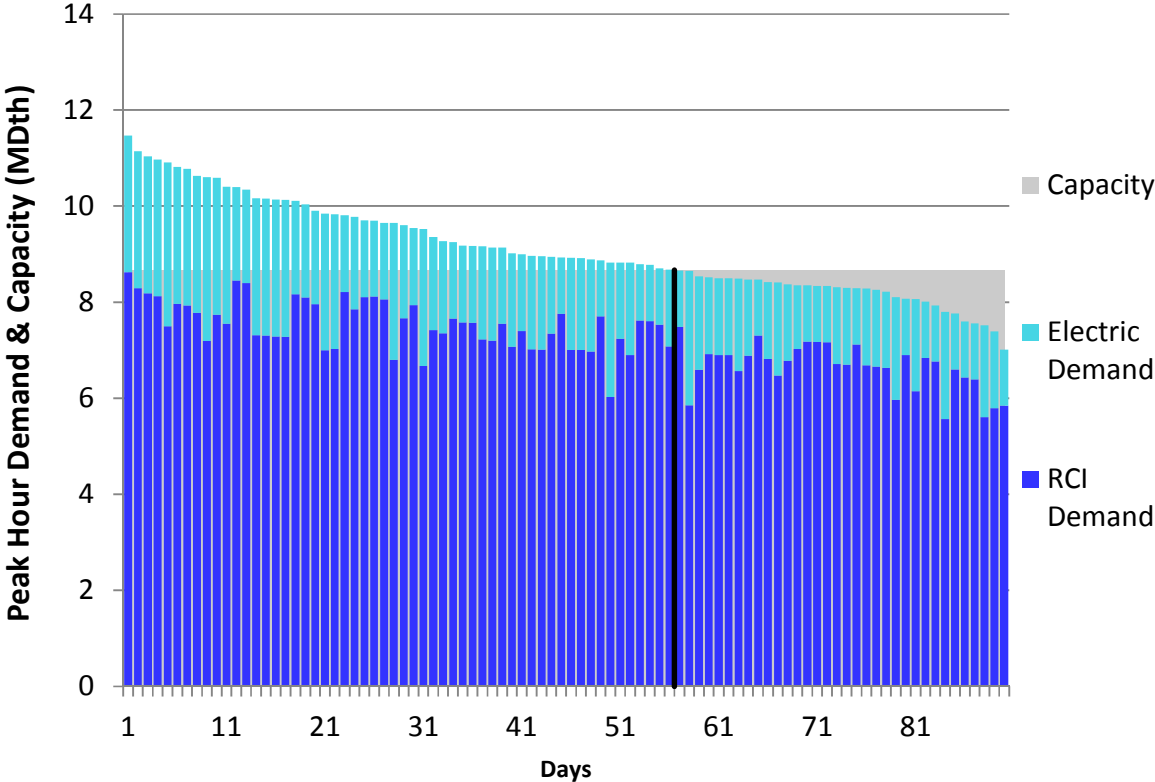
Figure H16. HGDS S2 Winter 2018 – Eastern Shore – Descending Demand
