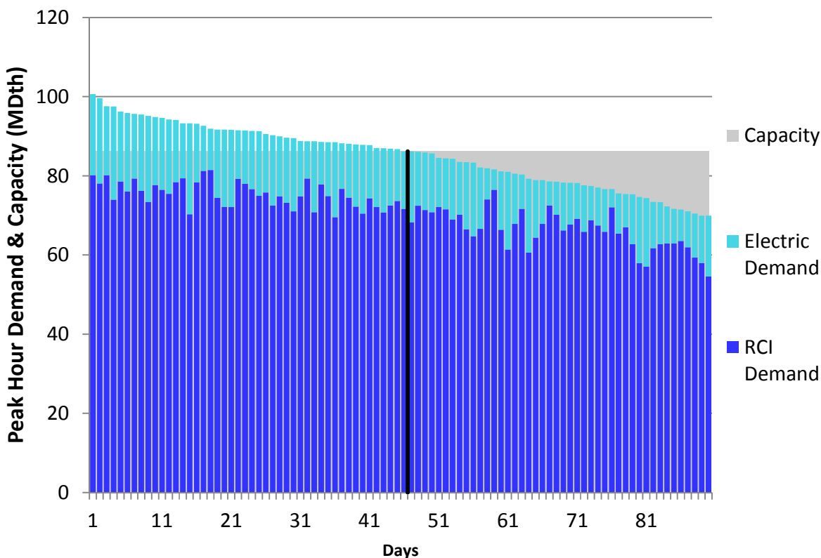
Figure H142. LGDS S2 Winter 2018 – Texas Eastern M2 PA South – Descending Demand
