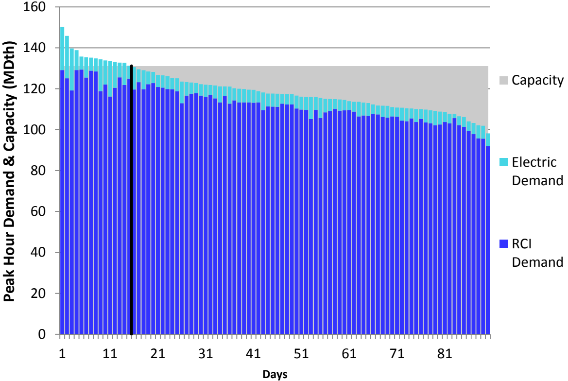
Figure H254. RGDS S3 Winter 2018 – TransCanada Ontario West – Descending Demand
