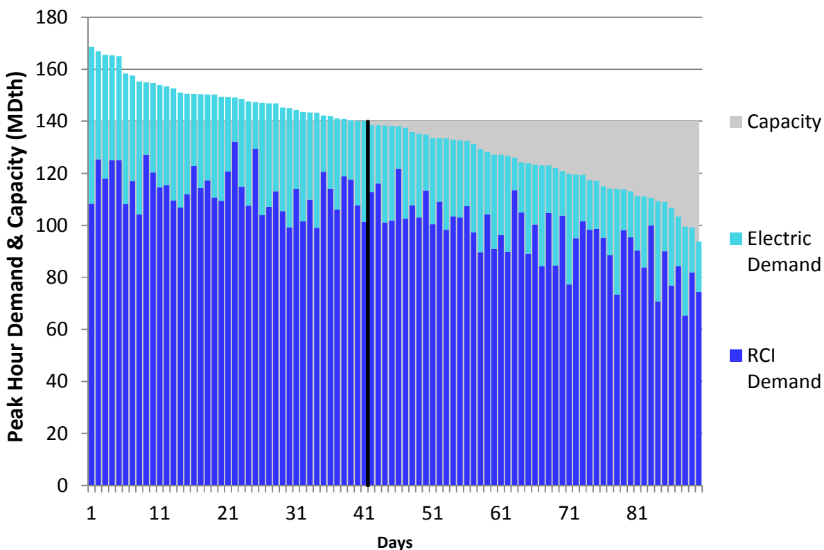
Figure H88. HGDS S2 Winter 2023 – Texas Eastern M3 North – Descending Demand
