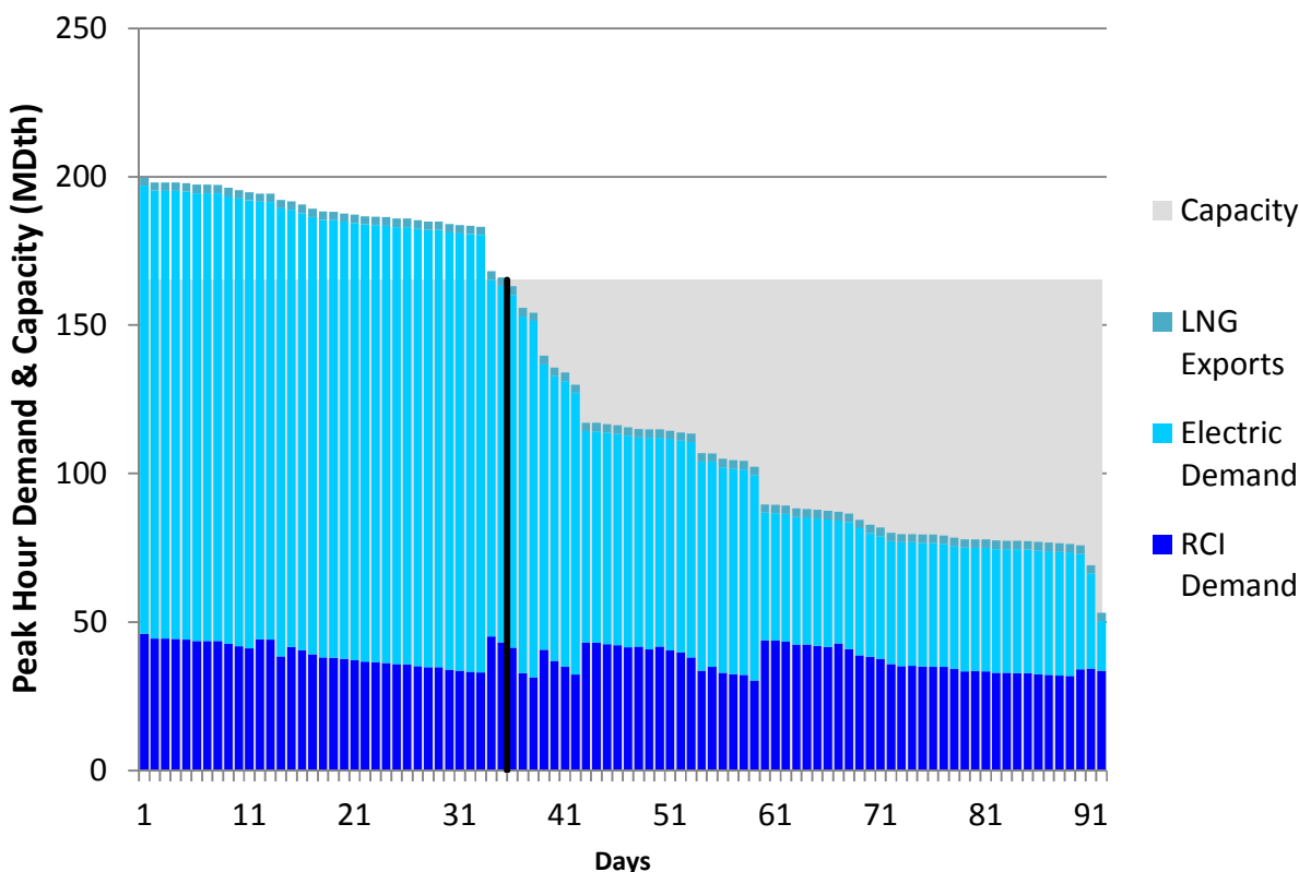
Figure H336. RGDS S3 Summer 2023 – Transco Z5 – Descending Demand
