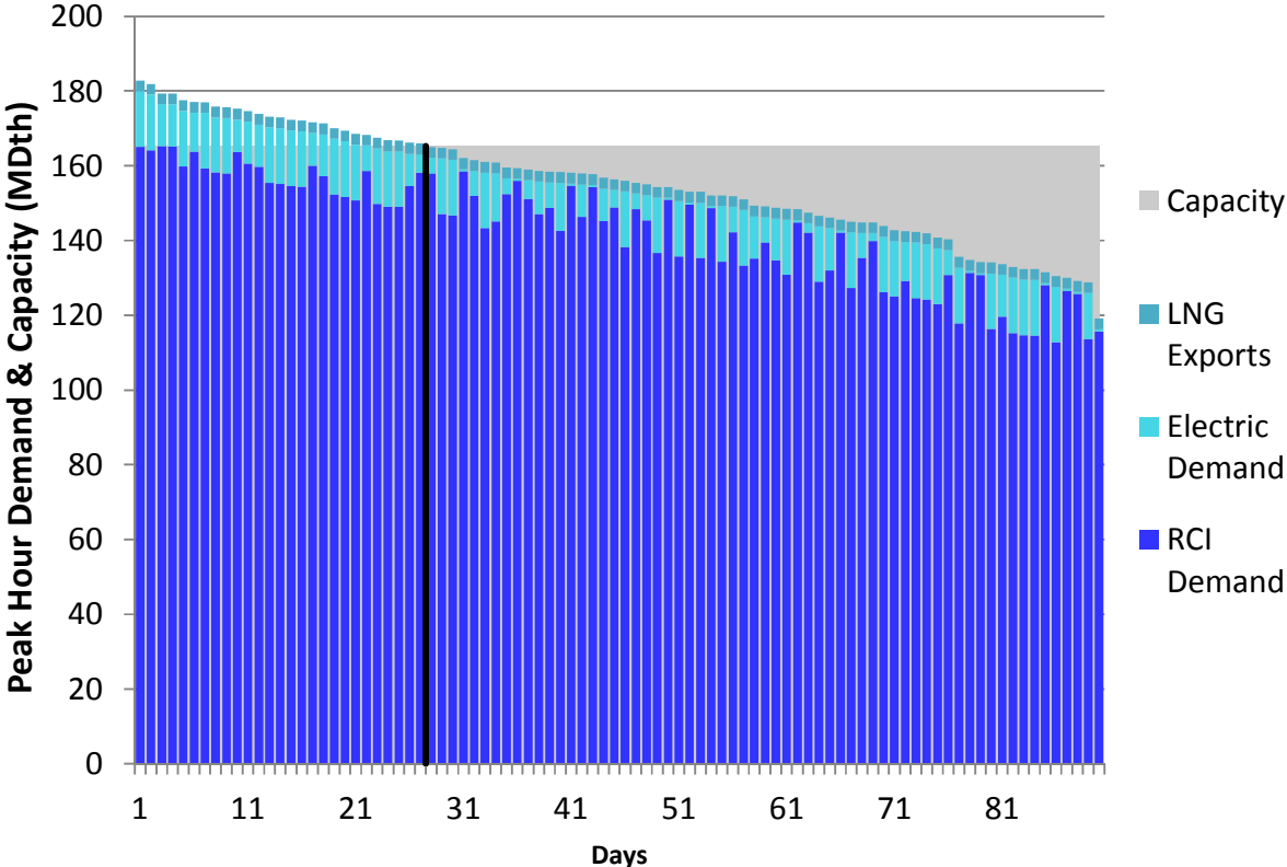
Figure H314. RGDS S3 Winter 2023 – Transco Z5 – Descending Demand
