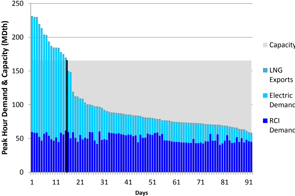
Figure H222. LGDS S2 Summer 2023 – Transco Z5 – Descending Demand
