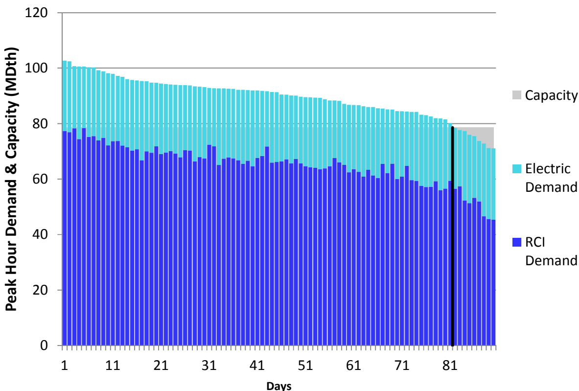
Figure H300. RGDS S3 Winter 2023 – Tennessee Z4 PA – Descending Demand
