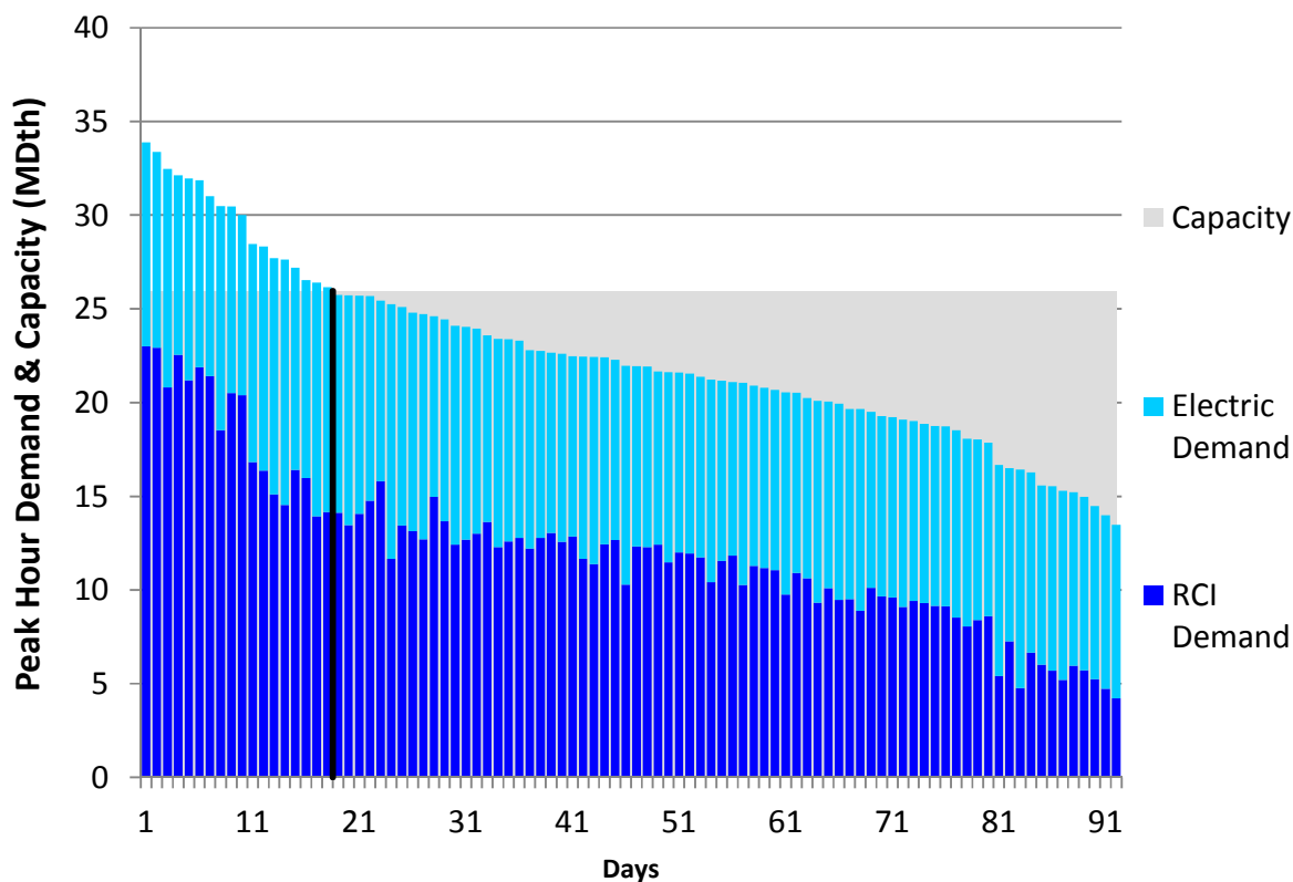
Figure H56. HGDS S2 Summer 2018 – Texas Eastern ETX – Descending Demand
