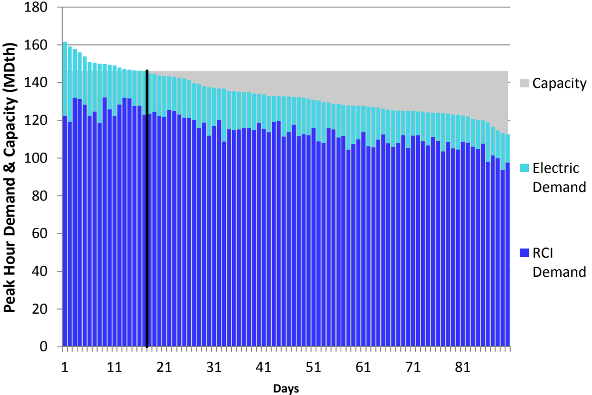
Figure H90. HGDS S2 Winter 2023 – TransCanada Ontario West – Descending Demand
