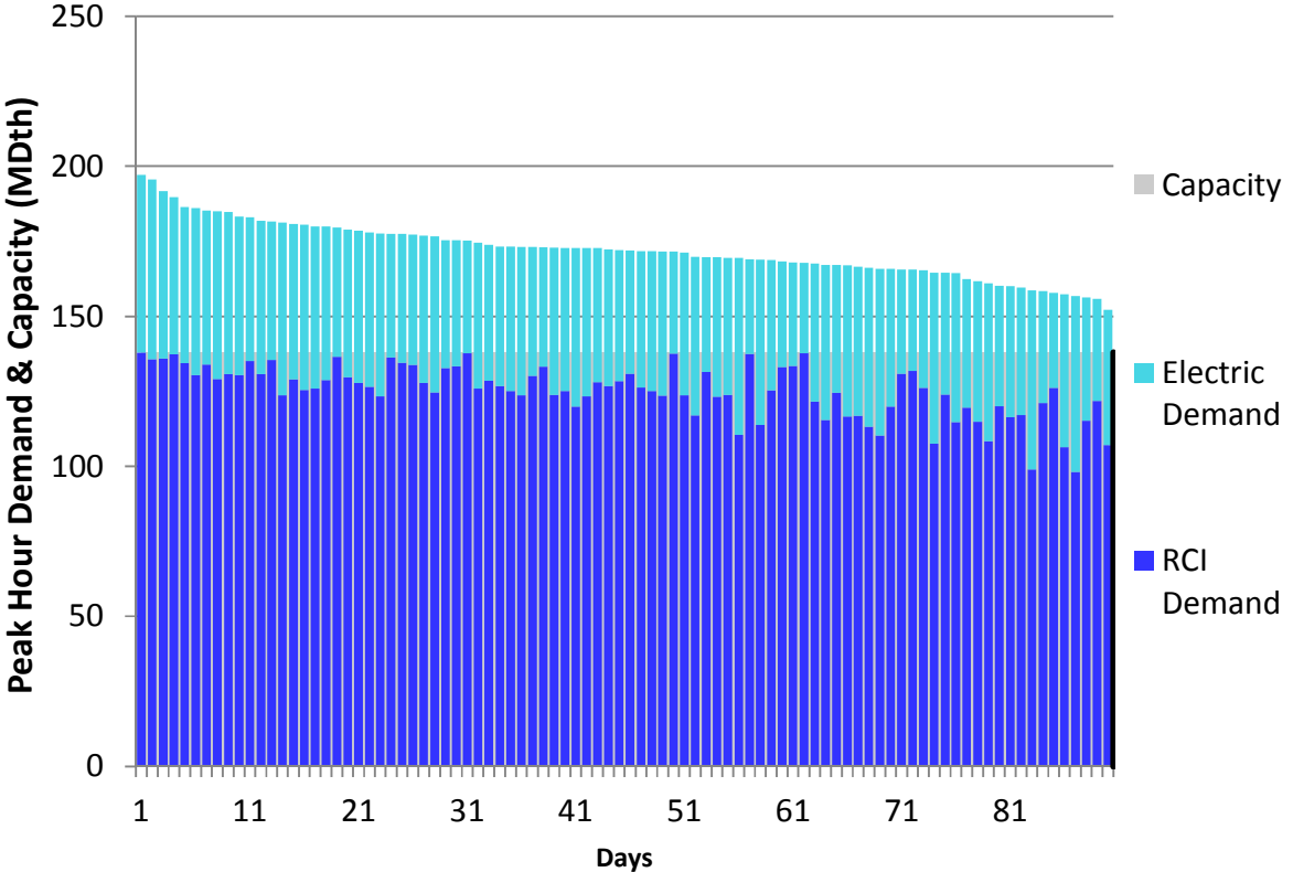
Figure H316. RGDS S3 Winter 2023 – Transco Leidy to Station 210 – Descending Demand
