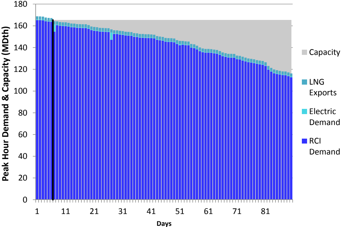
Figure H202. LGDS S2 Winter 2023 – Transco Z5 – Descending Demand
