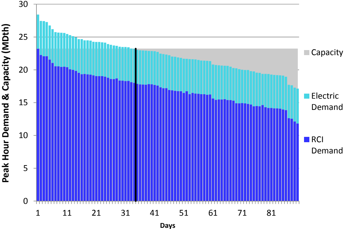
Figure H10. HGDS S2 Winter 2018 – Dominion Western NY– Descending Demand
