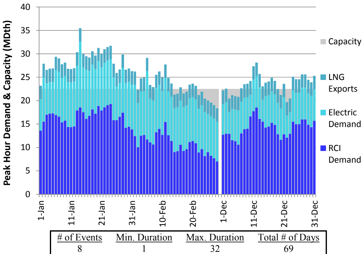
Figure H176. LGDS S2 Winter 2023 – Dominion Southeast – Descending Demand
