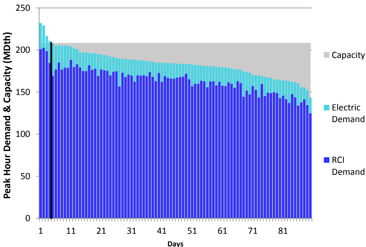
Figure H318. RGDS S3 Winter 2023 – Union Gas Dawn – Descending Demand
