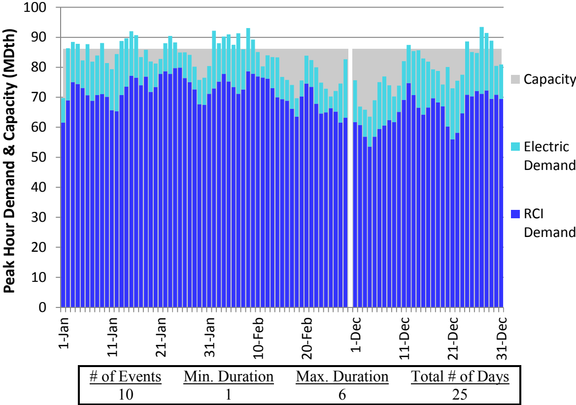
Figure H192. LGDS S2 Winter 2023 – Texas Eastern M2 PA South – Descending Demand
