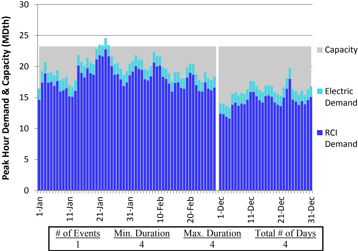
Figure H174. LGDS S2 Winter 2023 – Dominion Western NY– Descending Demand
