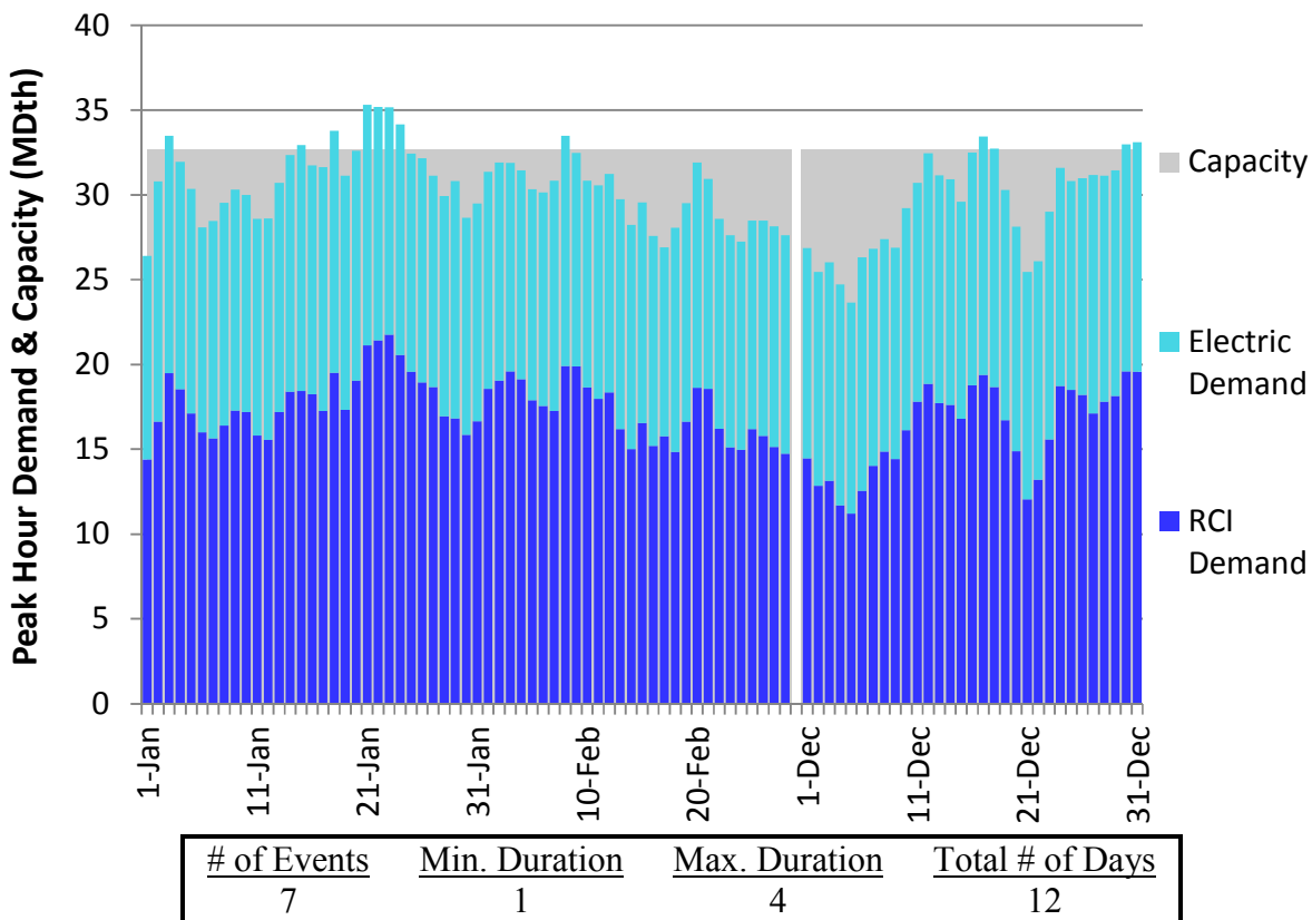
Figure H134. LGDS S2 Winter 2018 – Millennium – Descending Demand
