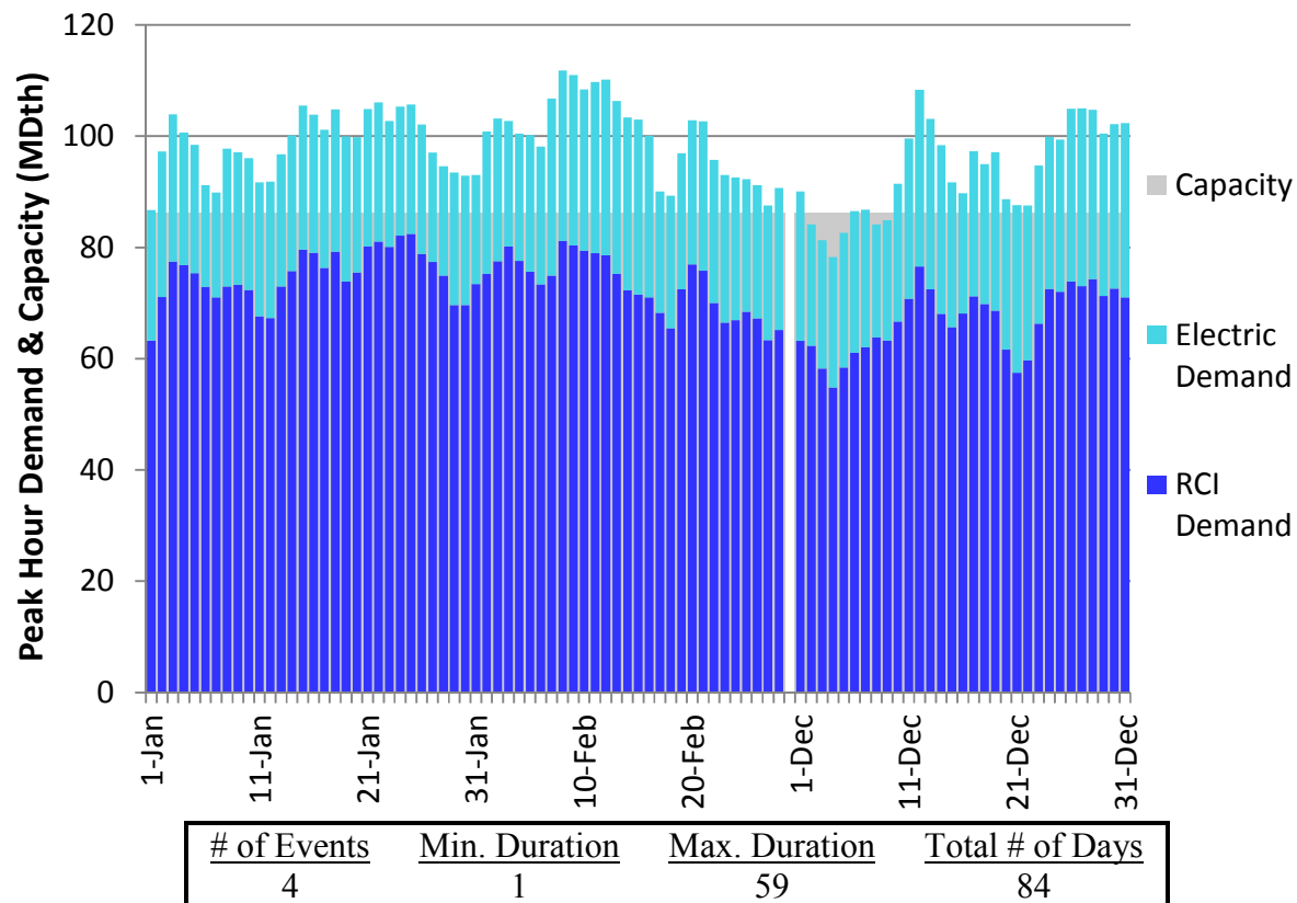
Figure H250. RGDS S3 Winter 2018 – Texas Eastern M2 PA South – Descending Demand
