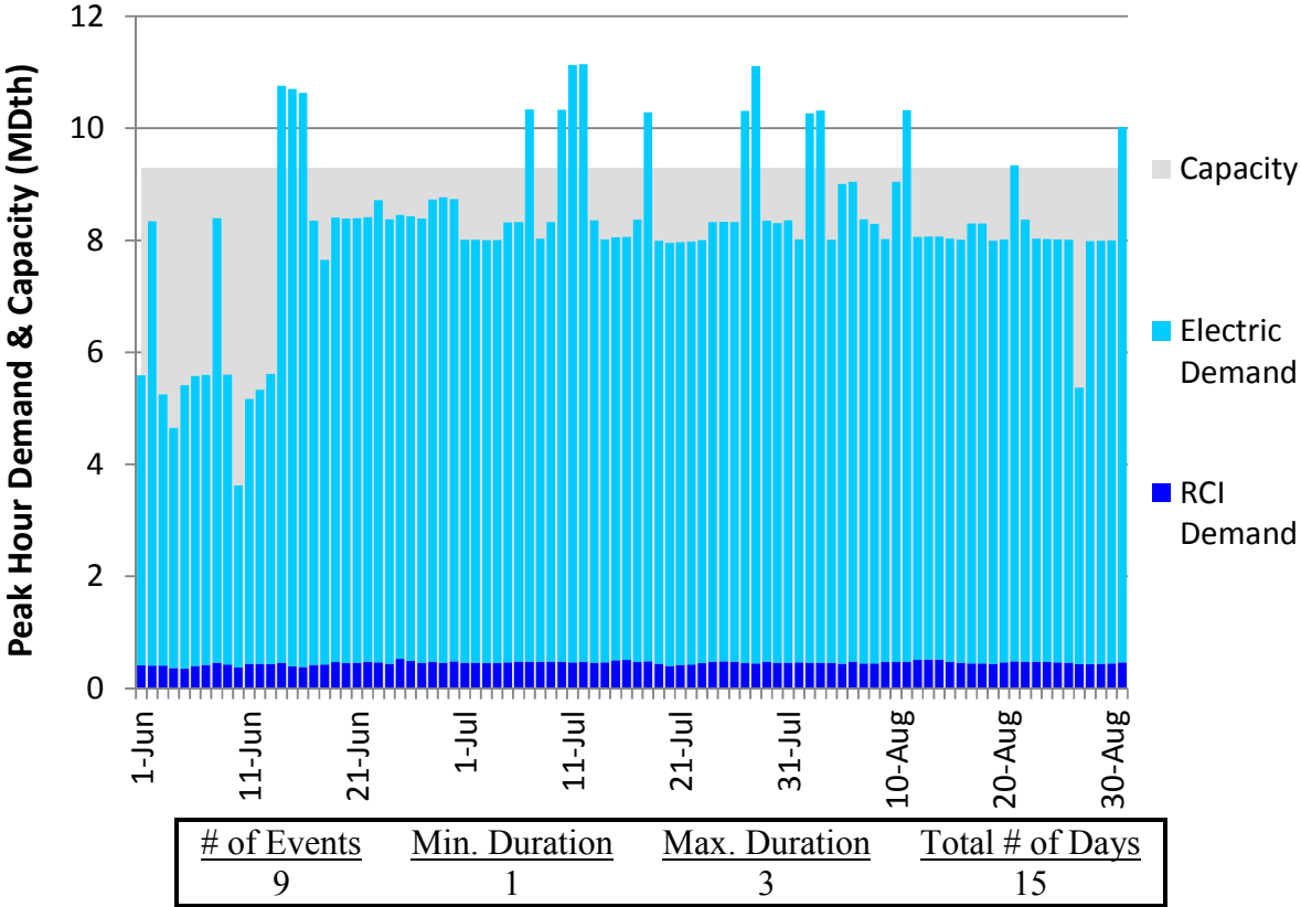
Figure H218. LGDS S2 Summer 2023 – PNGTS N of Westbrook – Descending Demand
