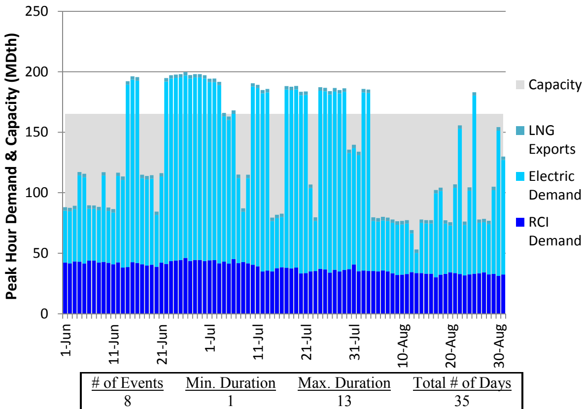
Figure H336. RGDS S3 Summer 2023 – Transco Z5 – Descending Demand
