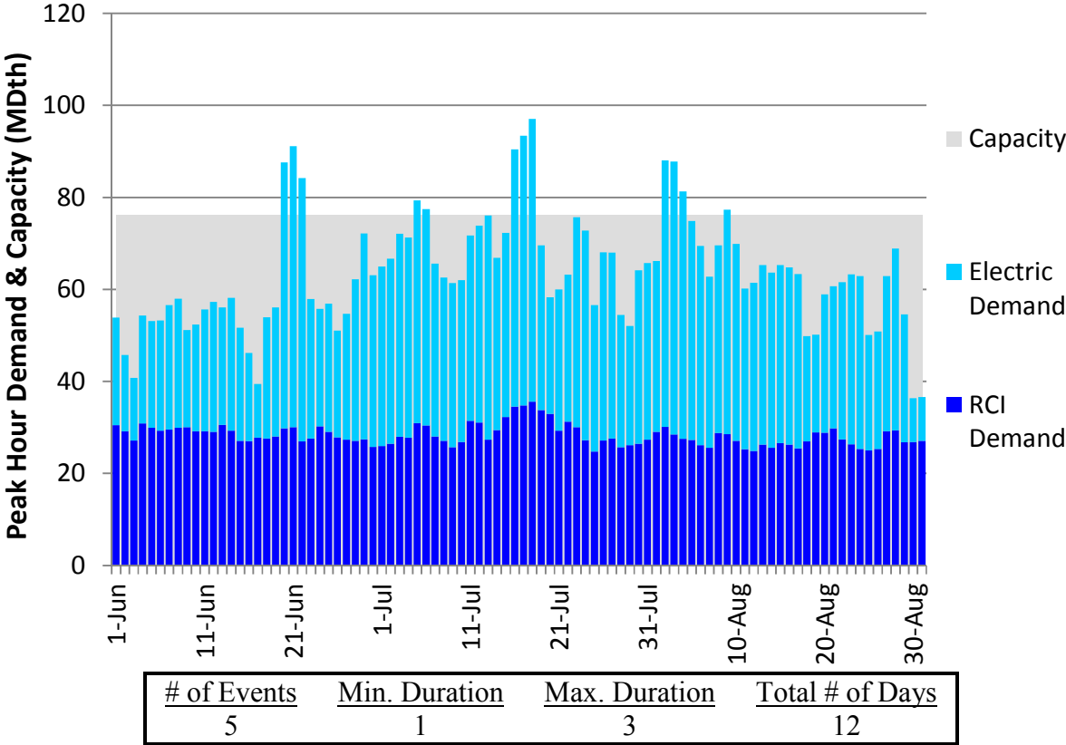
Figure H44. HGDS S2 Summer 2018 – Algonquin CT – Descending Demand
