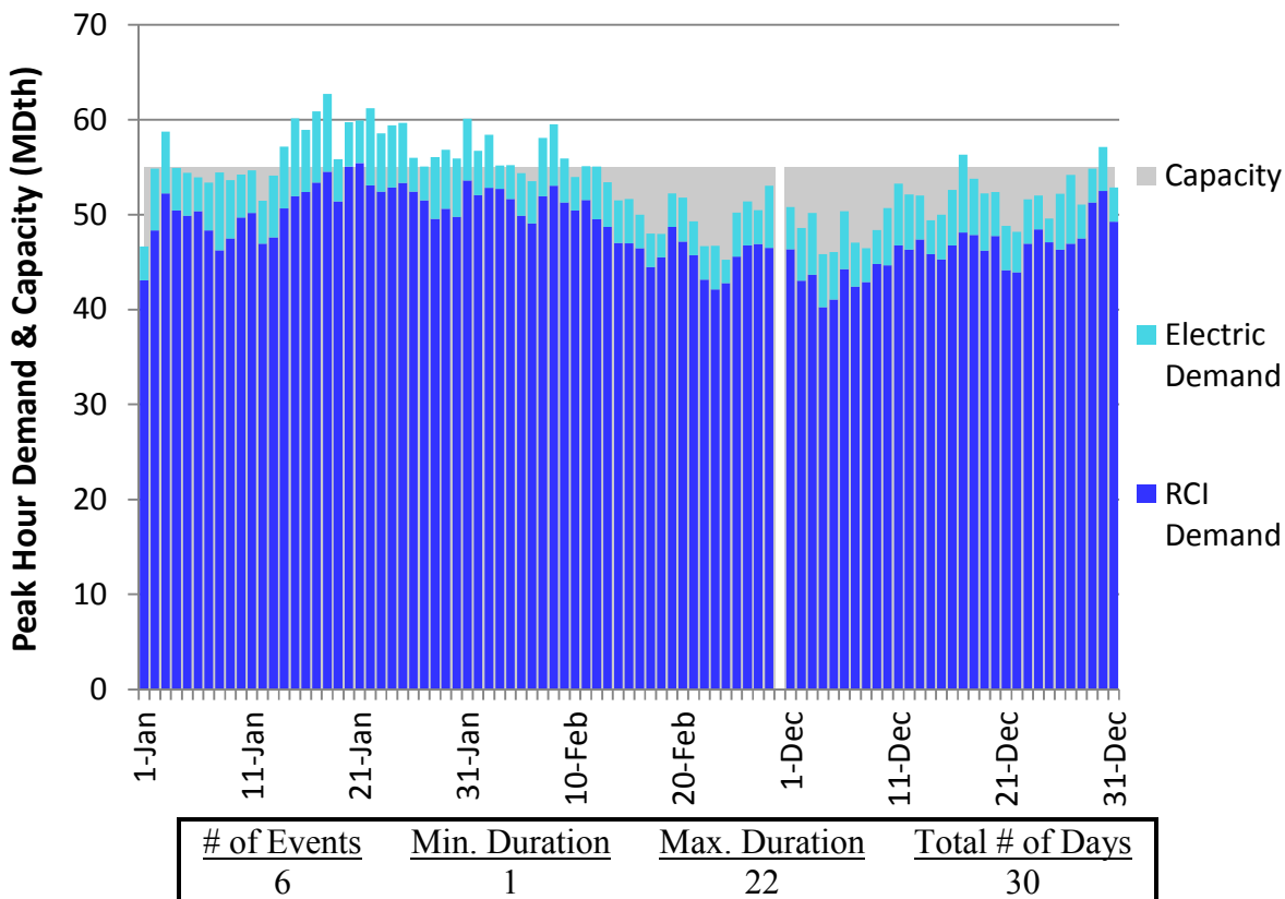
Figure H256. RGDS S3 Winter 2018 – TransCanada Quebec – Descending Demand
