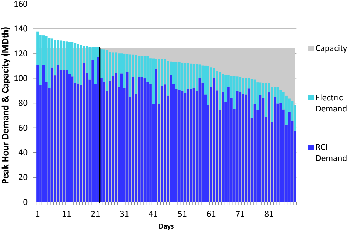
Figure H194. LGDS S2 Winter 2023 – Texas Eastern M3 North – Descending Demand
