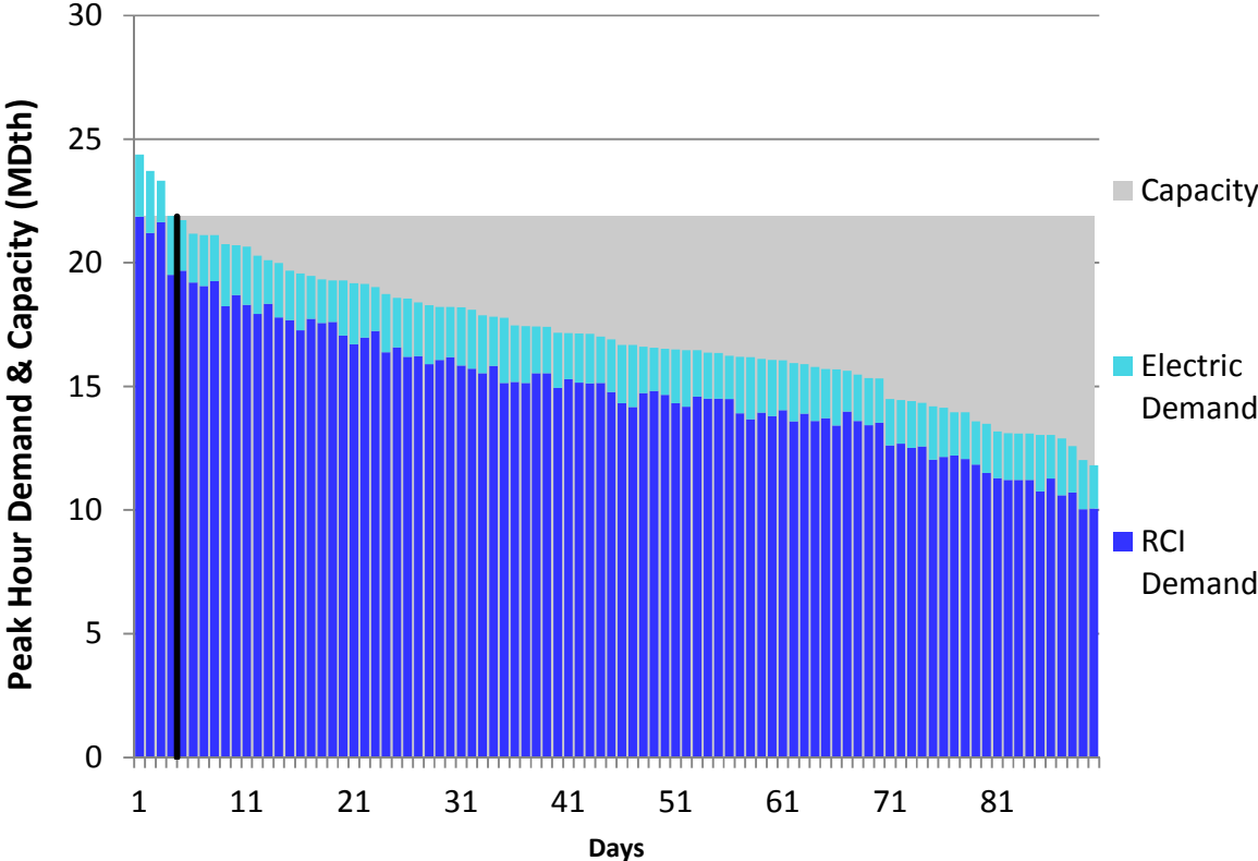
Figure H132. LGDS S2 Winter 2018 – Empire – Descending Demand
