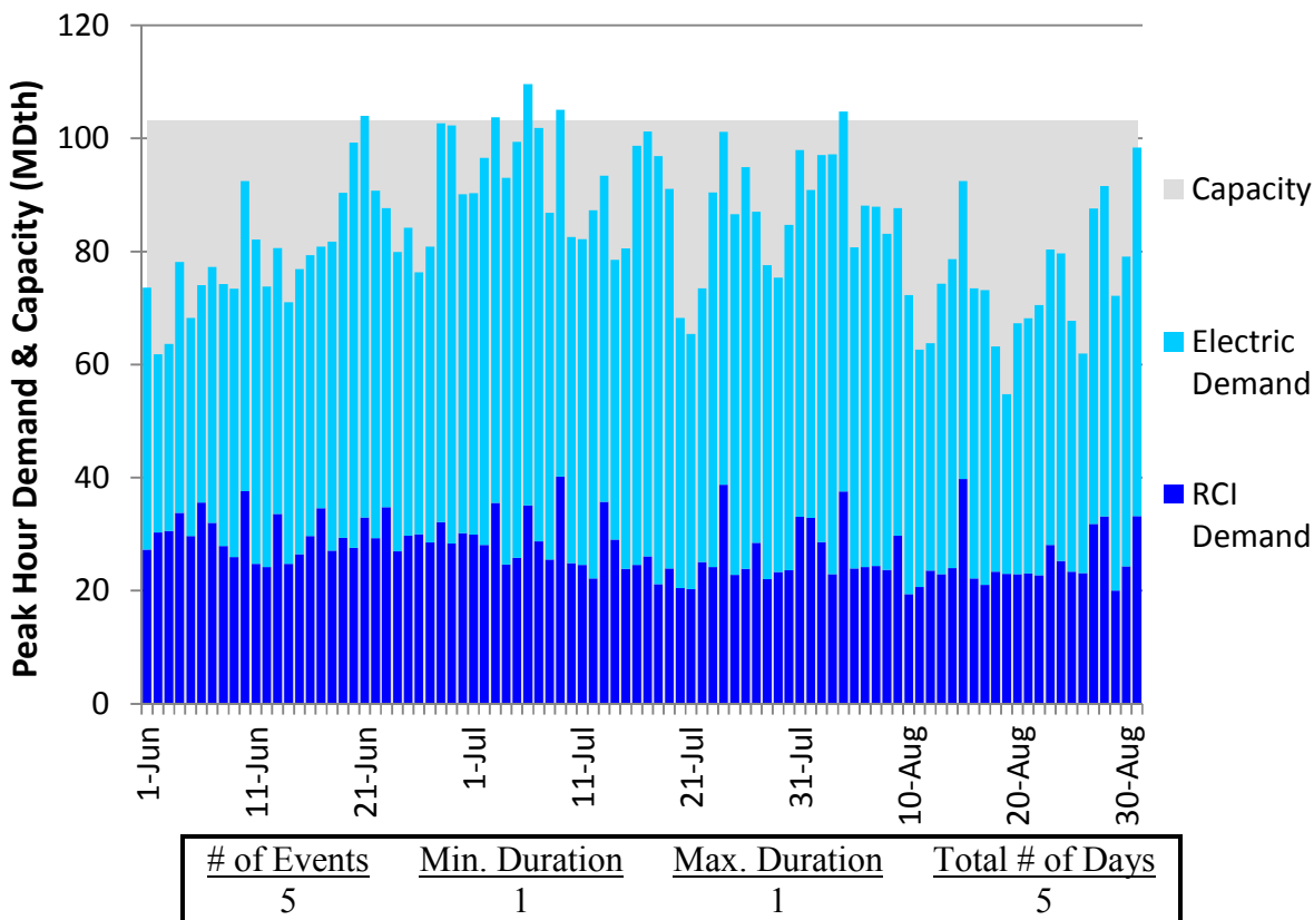
Figure H266. RGDS S3 Summer 2018 – Columbia Gas VA/MD – Descending Demand
