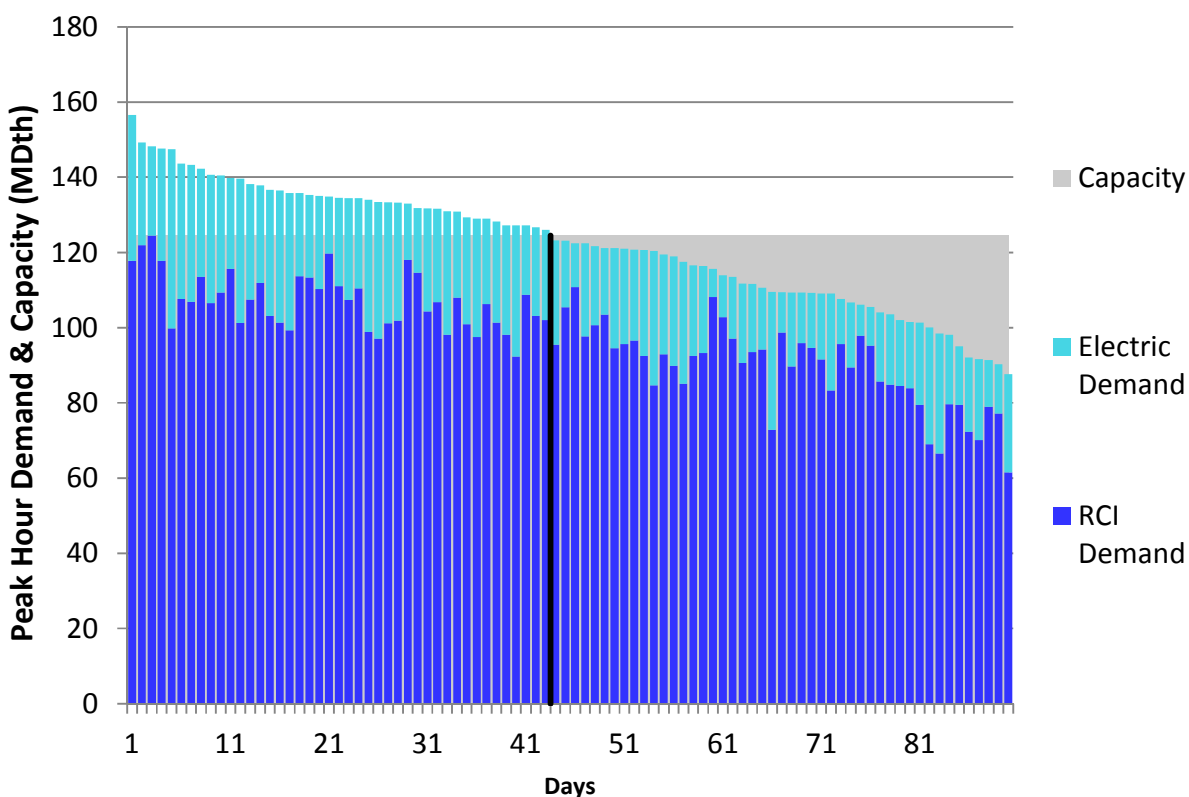
Figure H144. LGDS S2 Winter 2018 – Texas Eastern M3 North – Descending Demand
