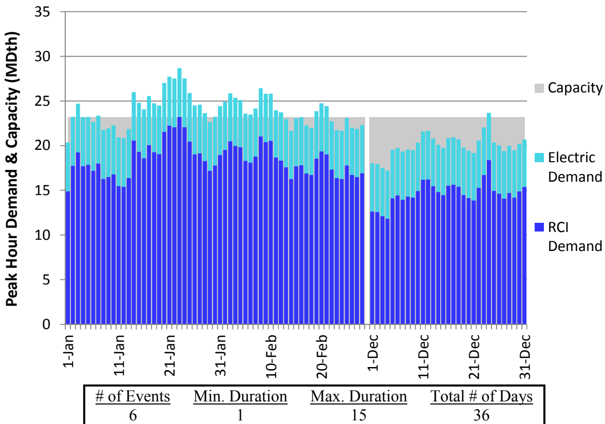
Figure H68. HGDS S2 Winter 2023 – Dominion Western NY– Descending Demand
