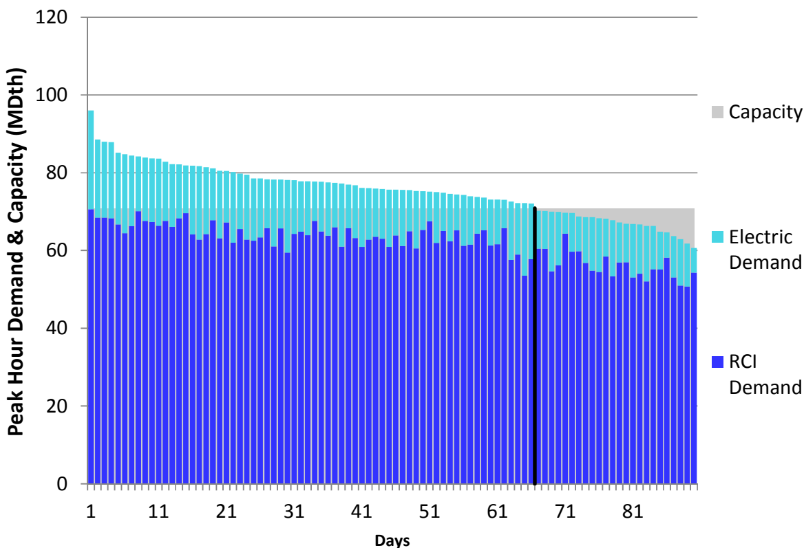
Figure H36. HGDS S2 Winter 2018 – Transco Leidy Atlantic – Descending Demand
