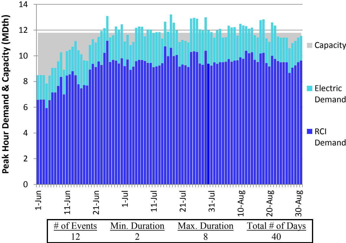
Figure H216. LGDS S2 Summer 2023 – NB/NS Supply – Descending Demand
