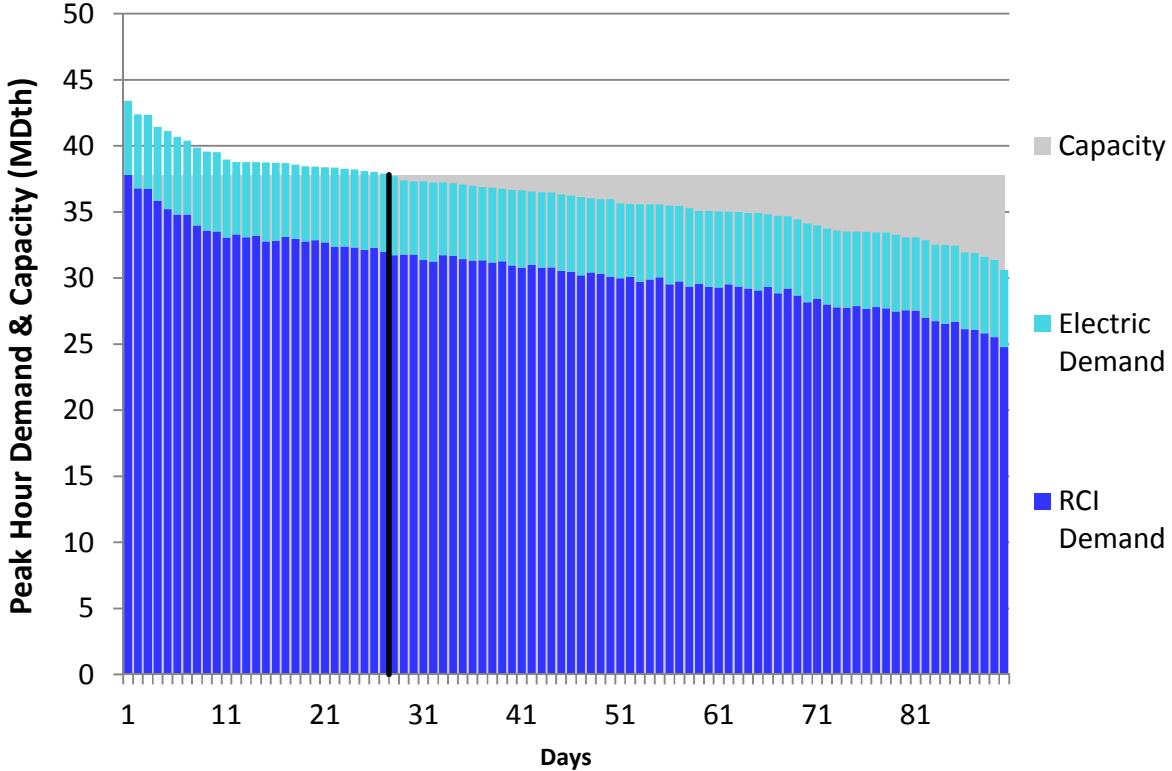
Figure H66. HGDS S2 Winter 2023 – Dominion Eastern NY– Descending Demand
