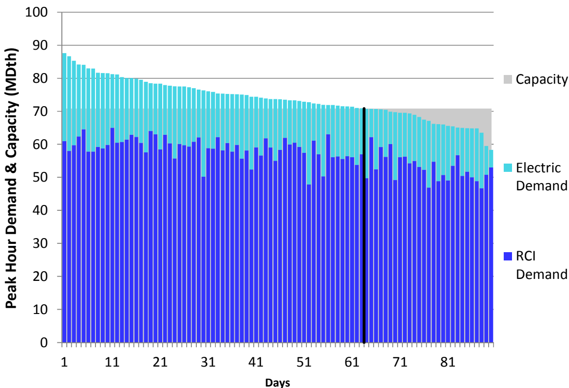
Figure H94. HGDS S2 Winter 2023 – Transco Leidy Atlantic – Descending Demand
