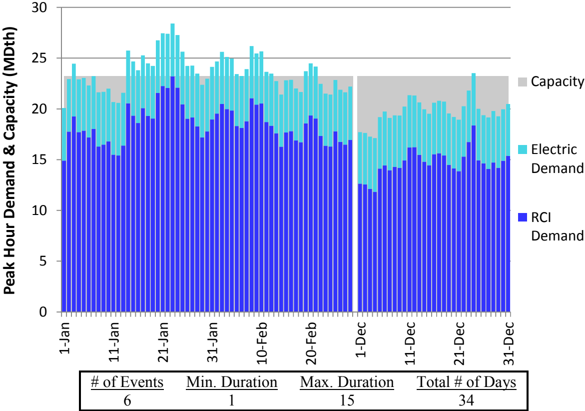
Figure H10. HGDS S2 Winter 2018 – Dominion Western NY– Descending Demand
