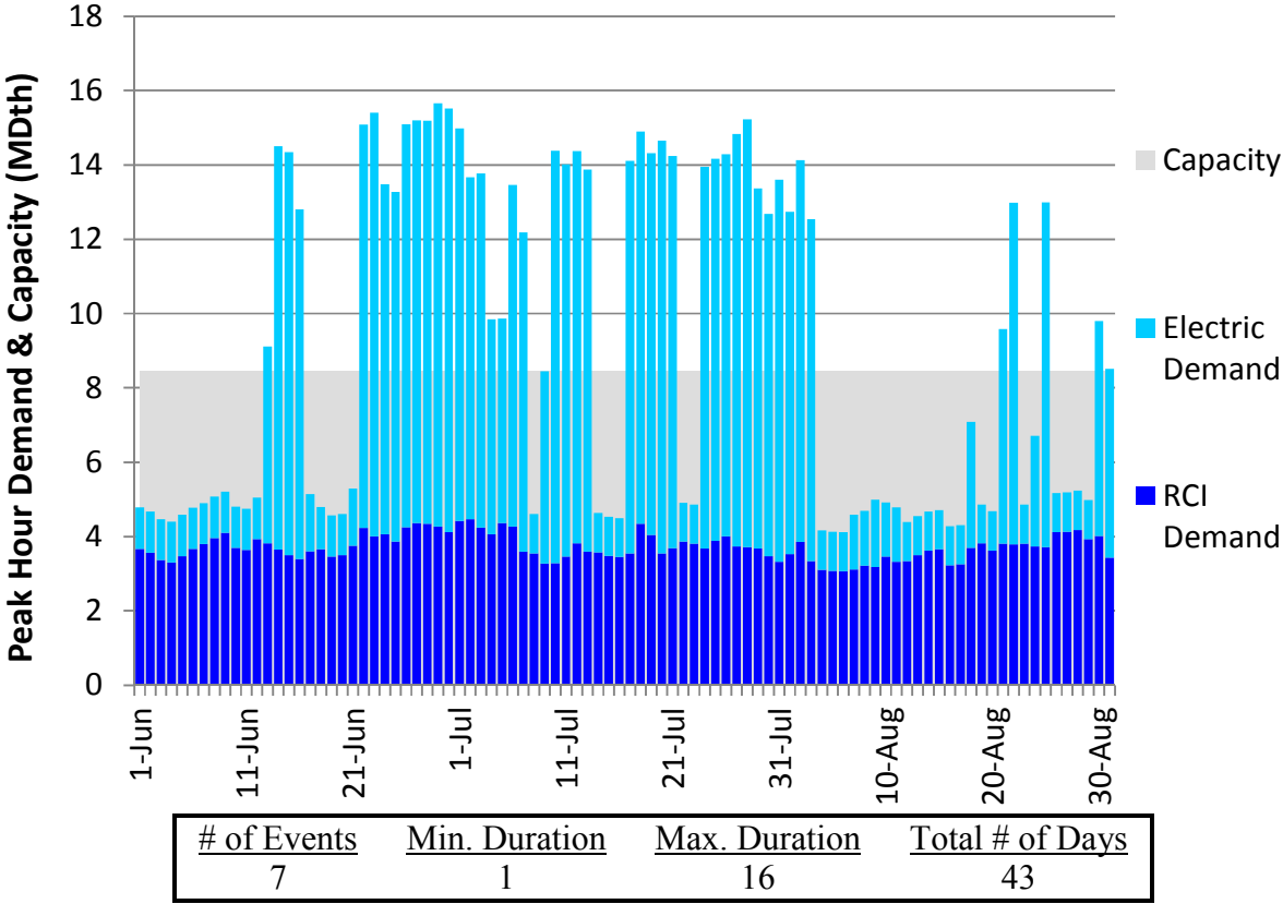
Figure H326. RGDS S3 Summer 2023 – Eastern Shore – Descending Demand
