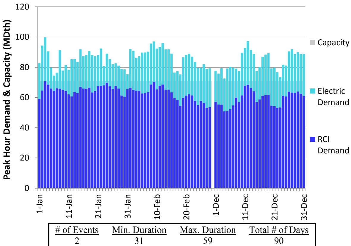
Figure H258. RGDS S3 Winter 2018 – Transco Leidy Atlantic – Descending Demand
