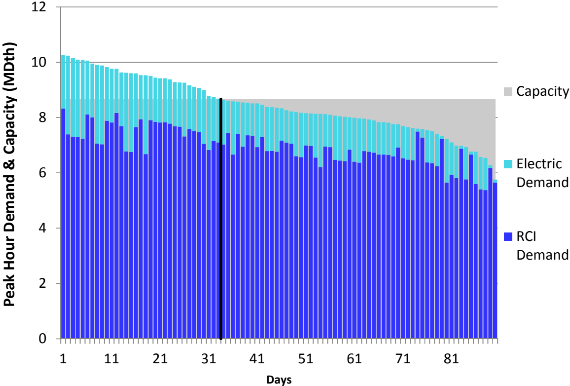
Figure H130. LGDS S2 Winter 2018 – Eastern Shore – Descending Demand
