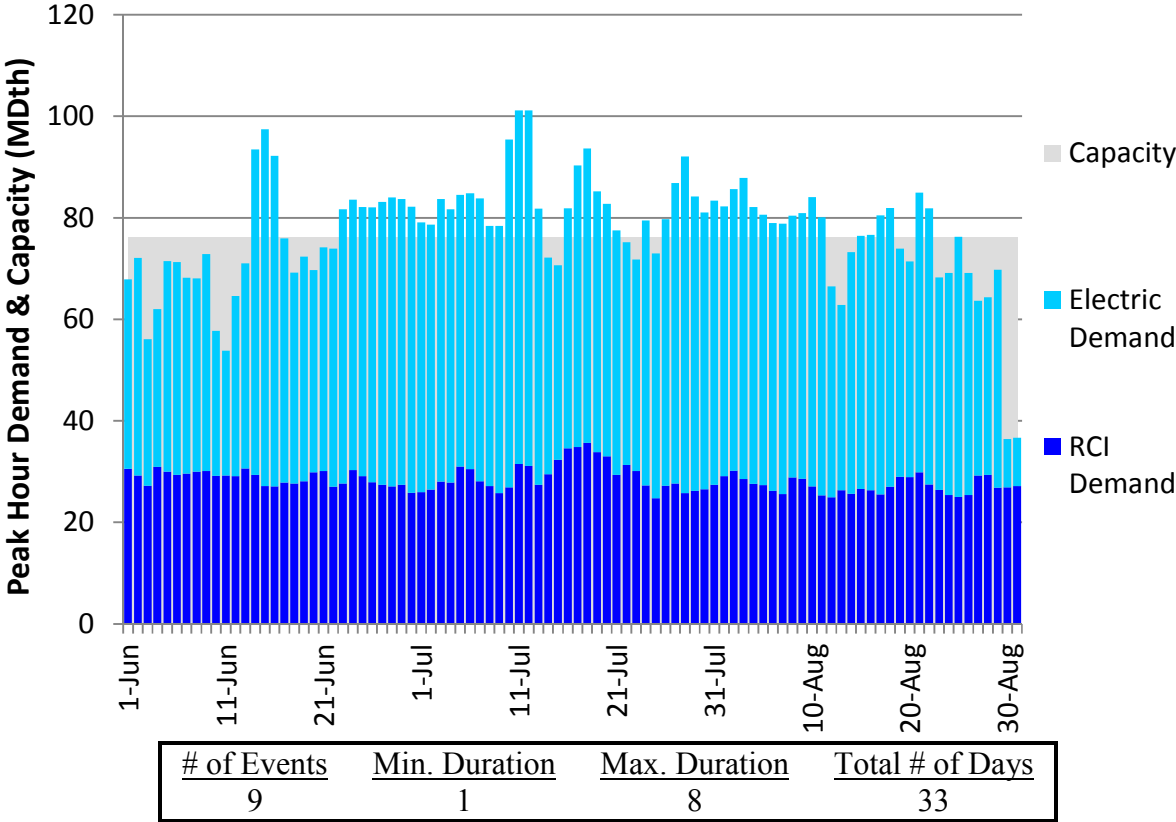
Figure H102. HGDS S2 Summer 2023 – Algonquin CT – Descending Demand
