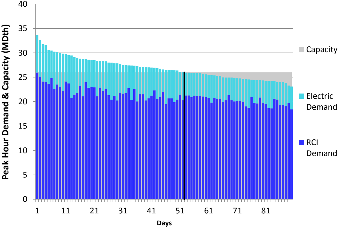
Figure H22. HGDS S2 Winter 2018 – NB/NS Supply – Descending Demand
