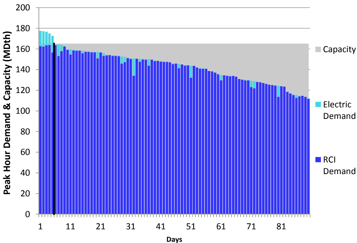
Figure H38. HGDS S2 Winter 2018 – Transco Z5 – Descending Demand
