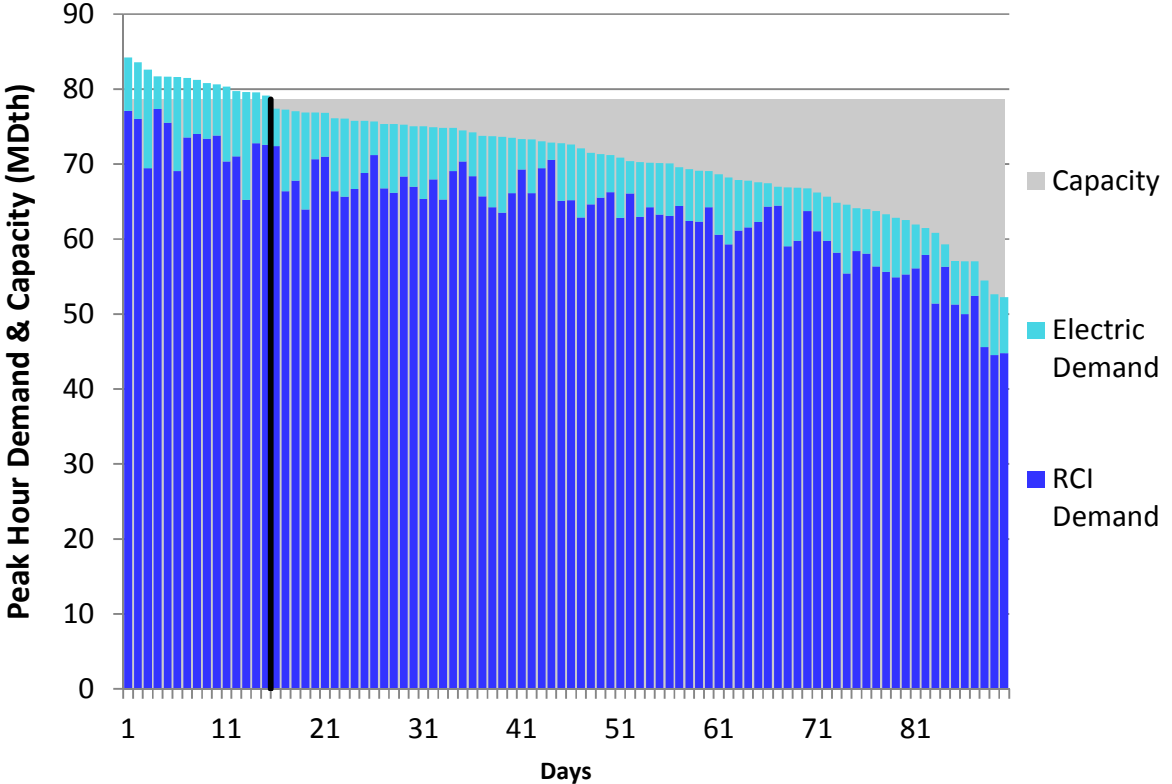
Figure H188. LGDS S2 Winter 2023 – Tennessee Z4 PA – Descending Demand
