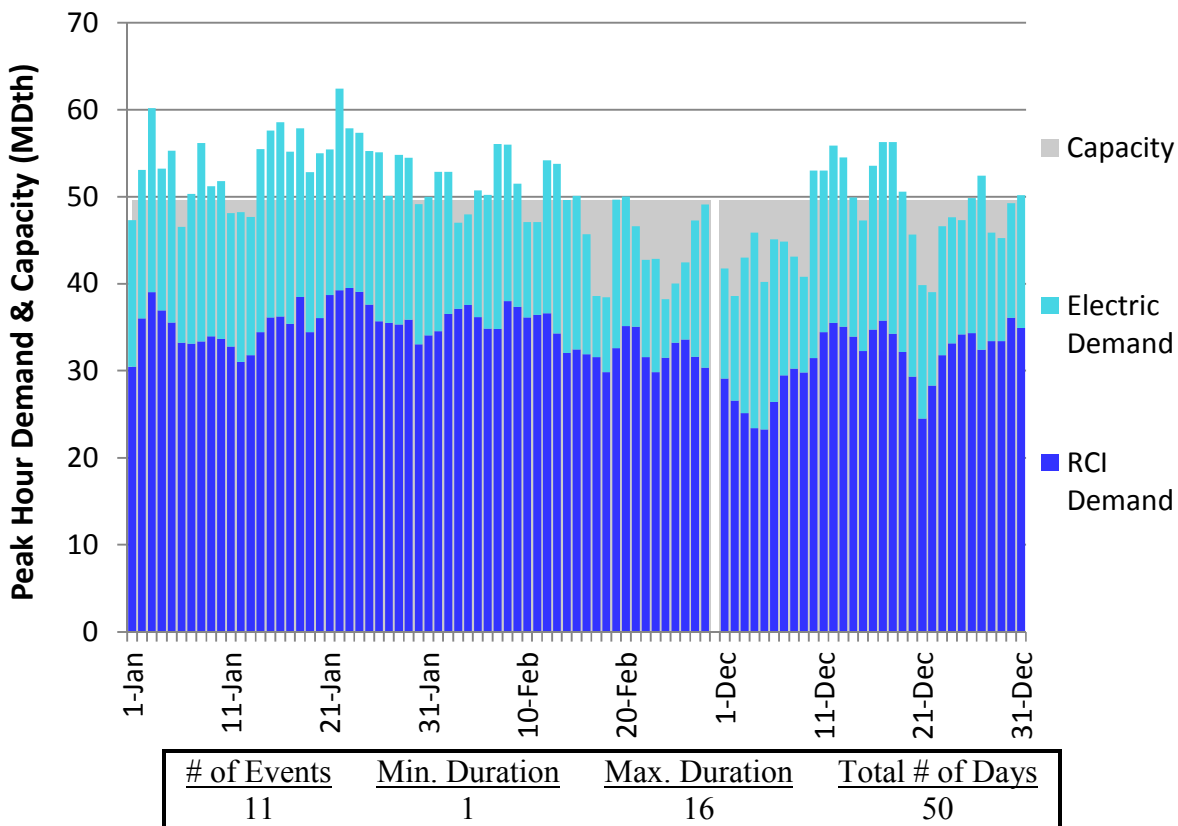
Figure H140. LGDS S2 Winter 2018 – Tennessee Z5 NY – Descending Demand
