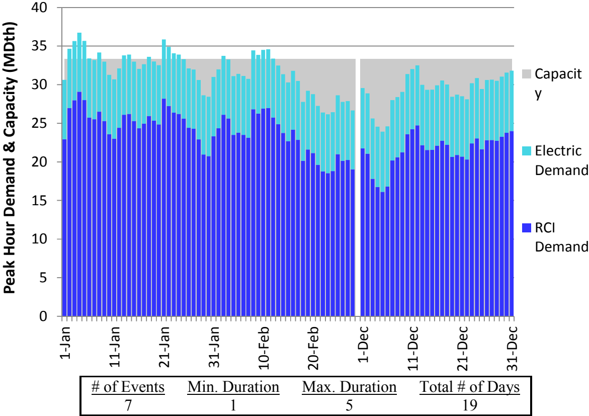
Figure H288. RGDS S3 Winter 2023 – East Tennessee – Descending Demand
