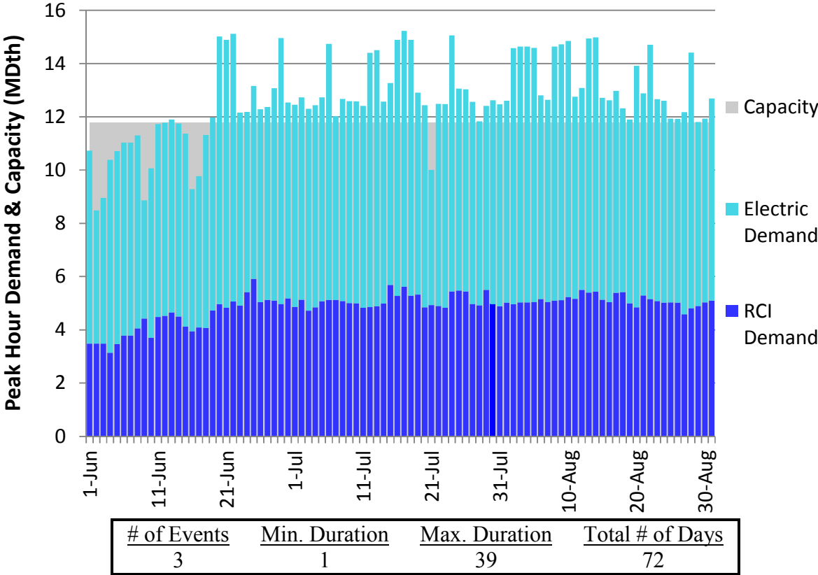
Figure H52. HGDS S2 Summer 2018 – NB/NS Supply – Descending Demand
