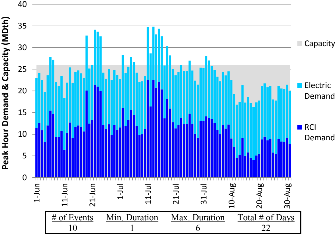
Figure H272. RGDS S3 Summer 2018 – Texas Eastern ETX – Descending Demand
