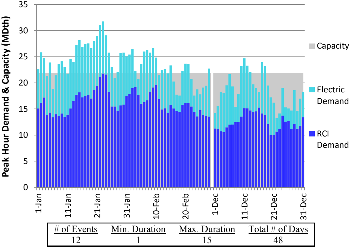
Figure H240. RGDS S3 Winter 2018 – Empire – Descending Demand
