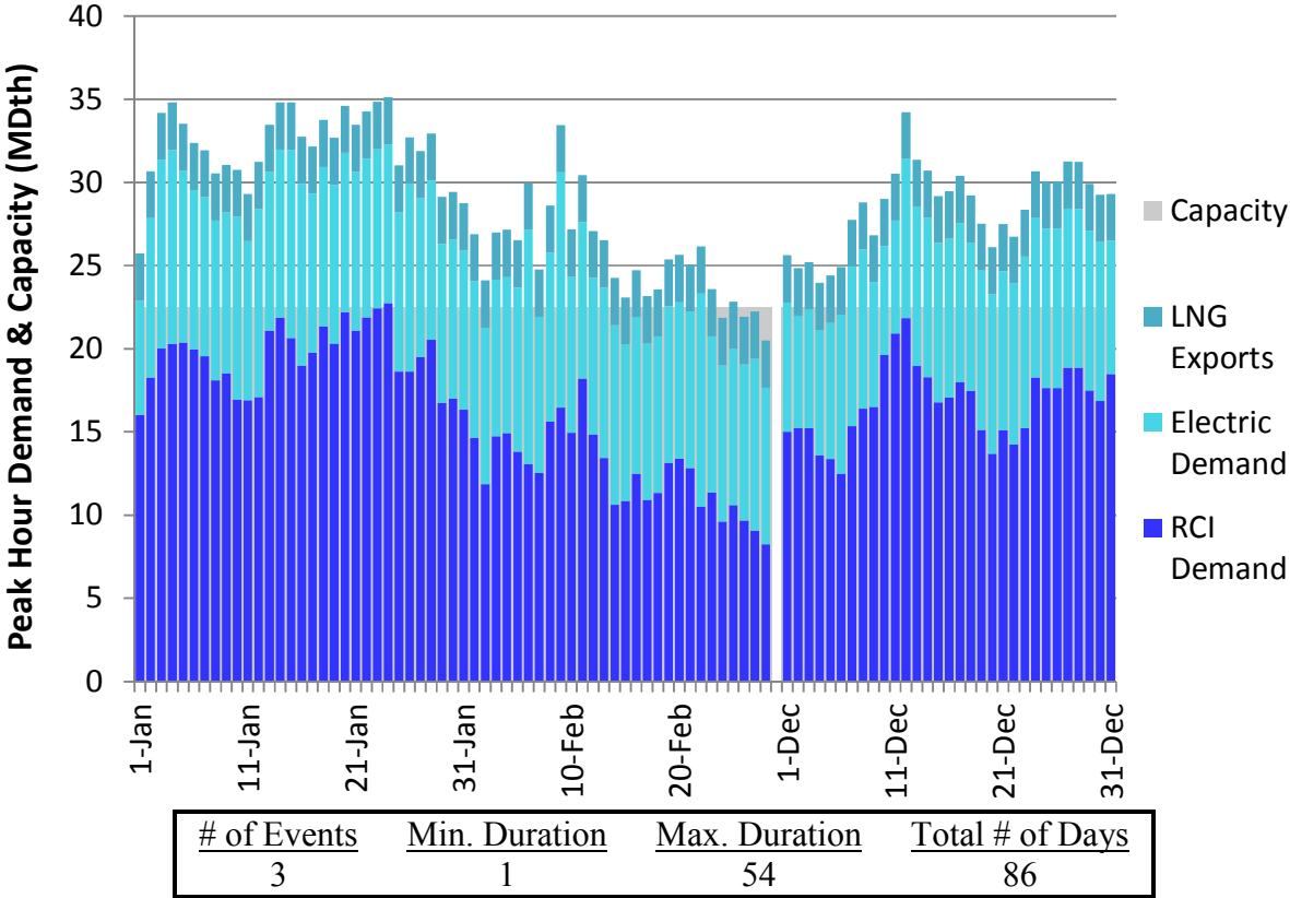
Figure H70. HGDS S2 Winter 2023 – Dominion Southeast – Descending Demand
