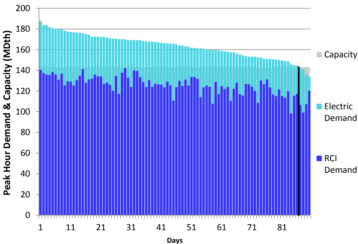
Figure H98. HGDS S2 Winter 2023 – Transco Leidy to Station 210 – Descending Demand
