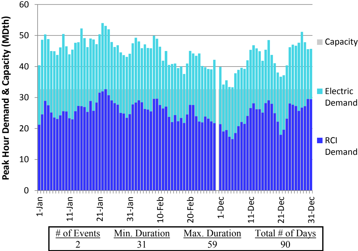
Figure H184. LGDS S2 Winter 2023 – Millennium – Descending Demand
