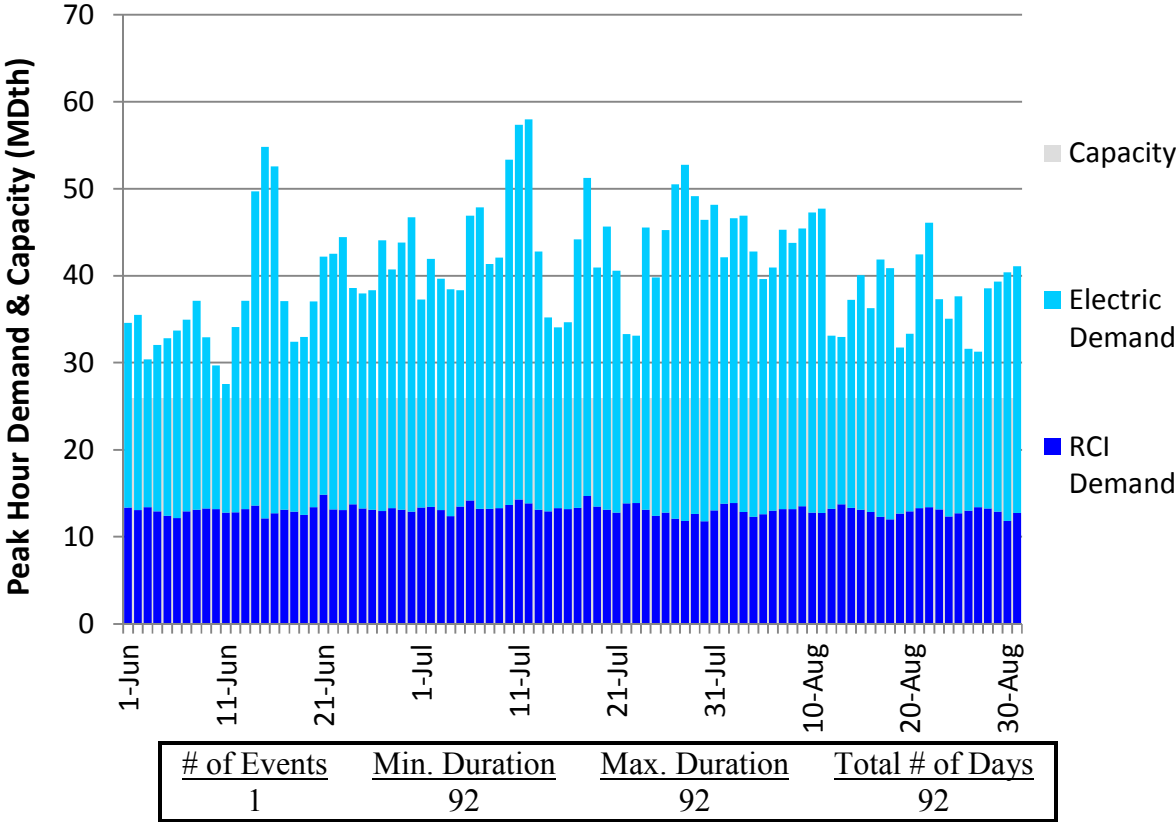
Figure H114. HGDS S2 Summer 2023 – Tennessee Z5 NY – Descending Demand
