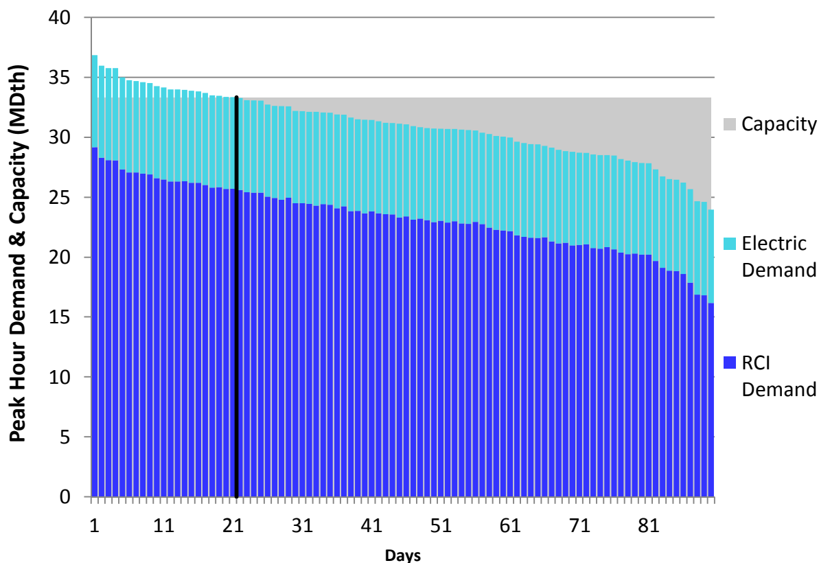
Figure H236. RGDS S3 Winter 2018 – East Tennessee – Descending Demand
