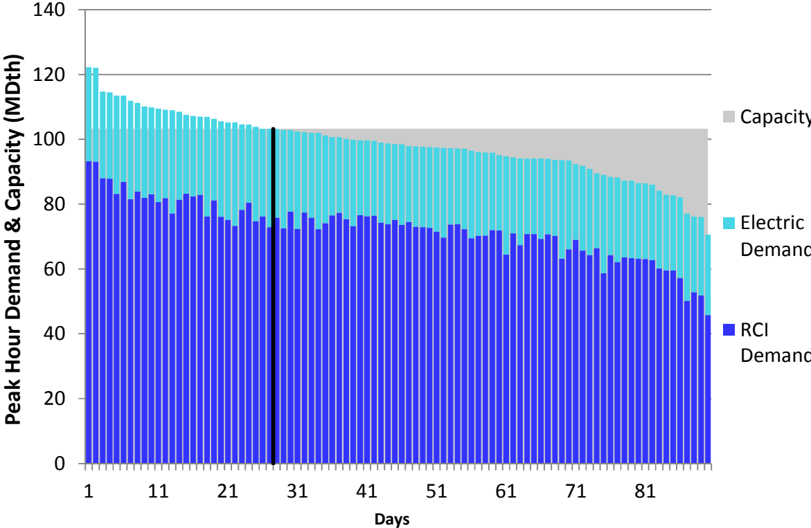
Figure H2. HGDS S2 Winter 2018 – Columbia Gas VA/MD – Descending Demand
