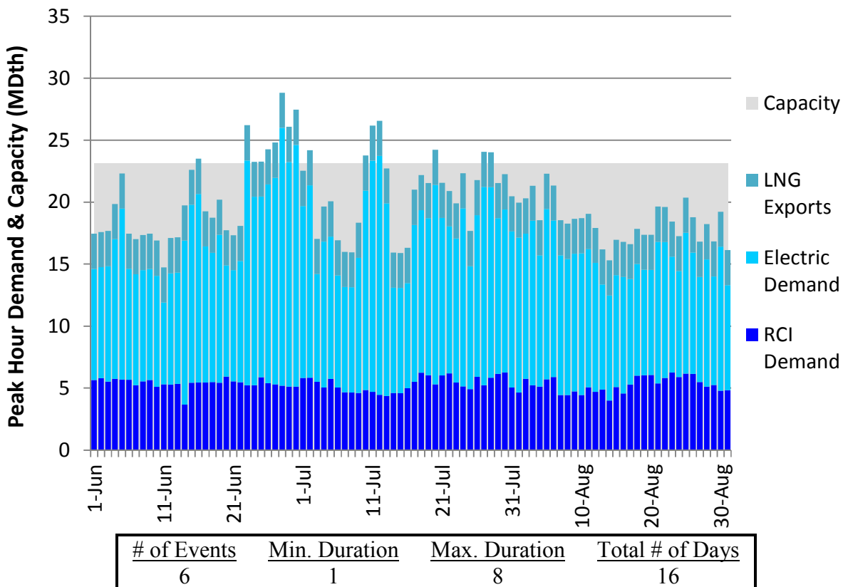
Figure H212. LGDS S2 Summer 2023 – Dominion Southeast – Descending Demand
