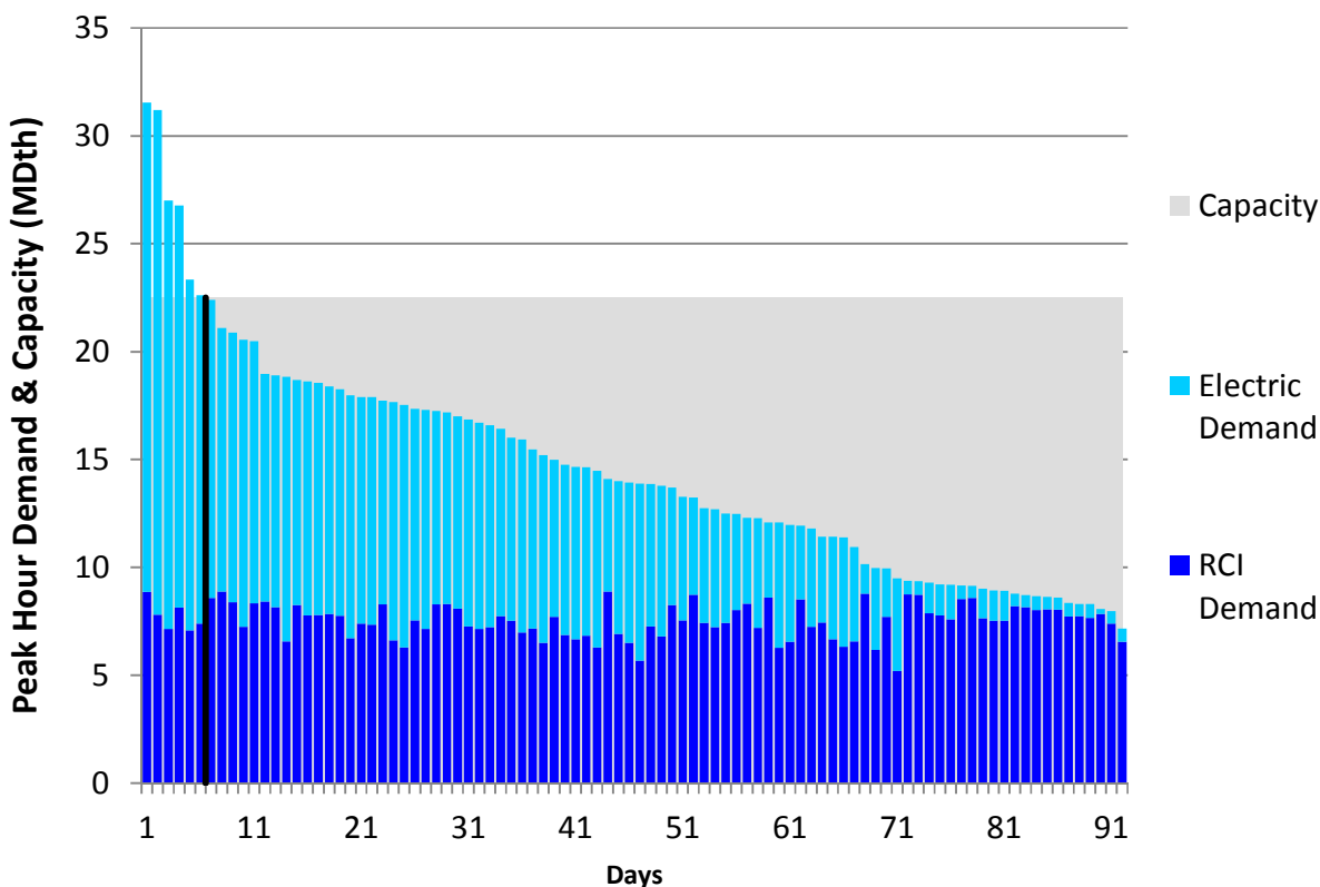
Figure H48. HGDS S2 Summer 2018 – Dominion Southeast – Descending Demand
