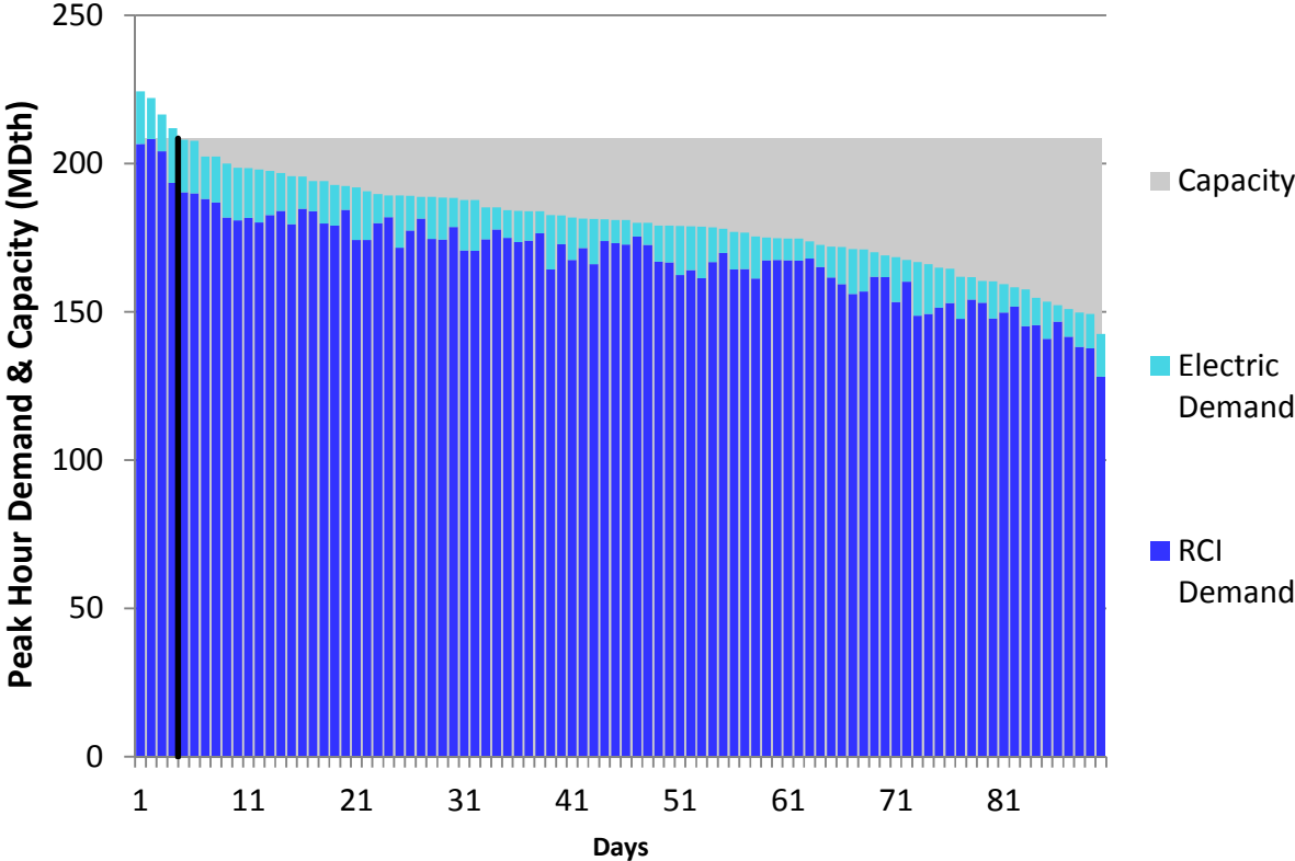
Figure H42. HGDS S2 Winter 2018 – Union Gas Dawn – Descending Demand
