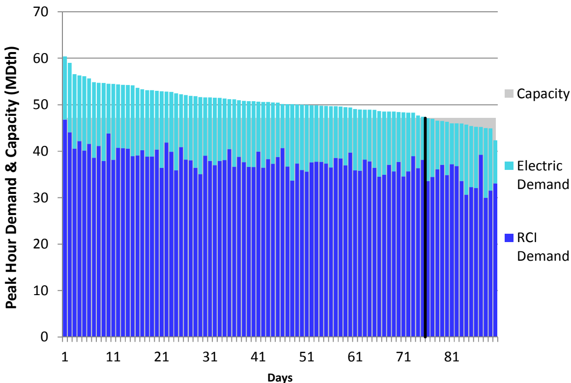
Figure H62. HGDS S2 Winter 2023 – Columbia Gas W PA/NY – Descending Demand
