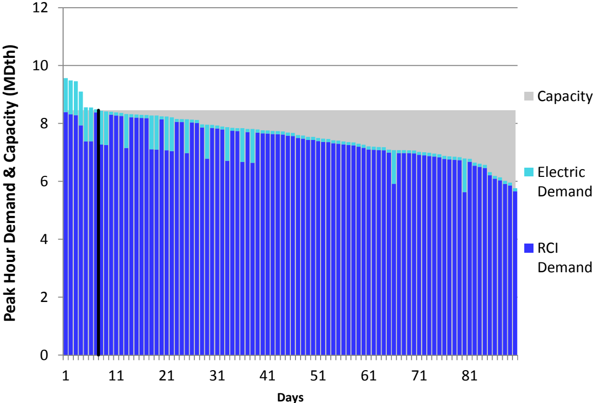
Figure H290. RGDS S3 Winter 23 – Eastern Shore – Descending Demand
