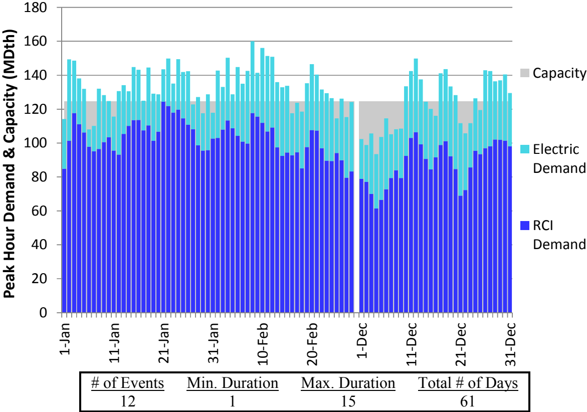
Figure H30. HGDS S2 Winter 2018 – Texas Eastern M3 North – Descending Demand
