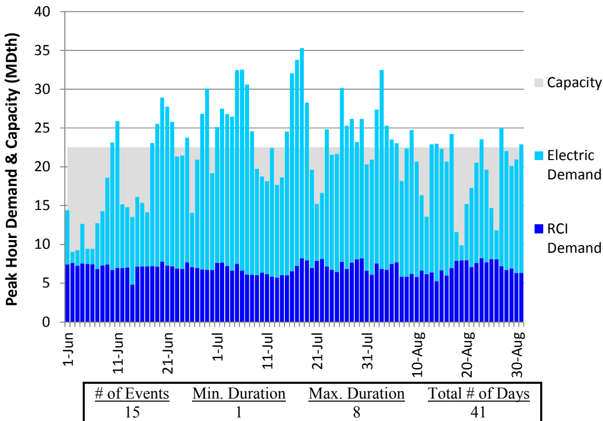
Figure H268. RGDS S3 Summer 2018 – Dominion Southeast – Descending Demand
