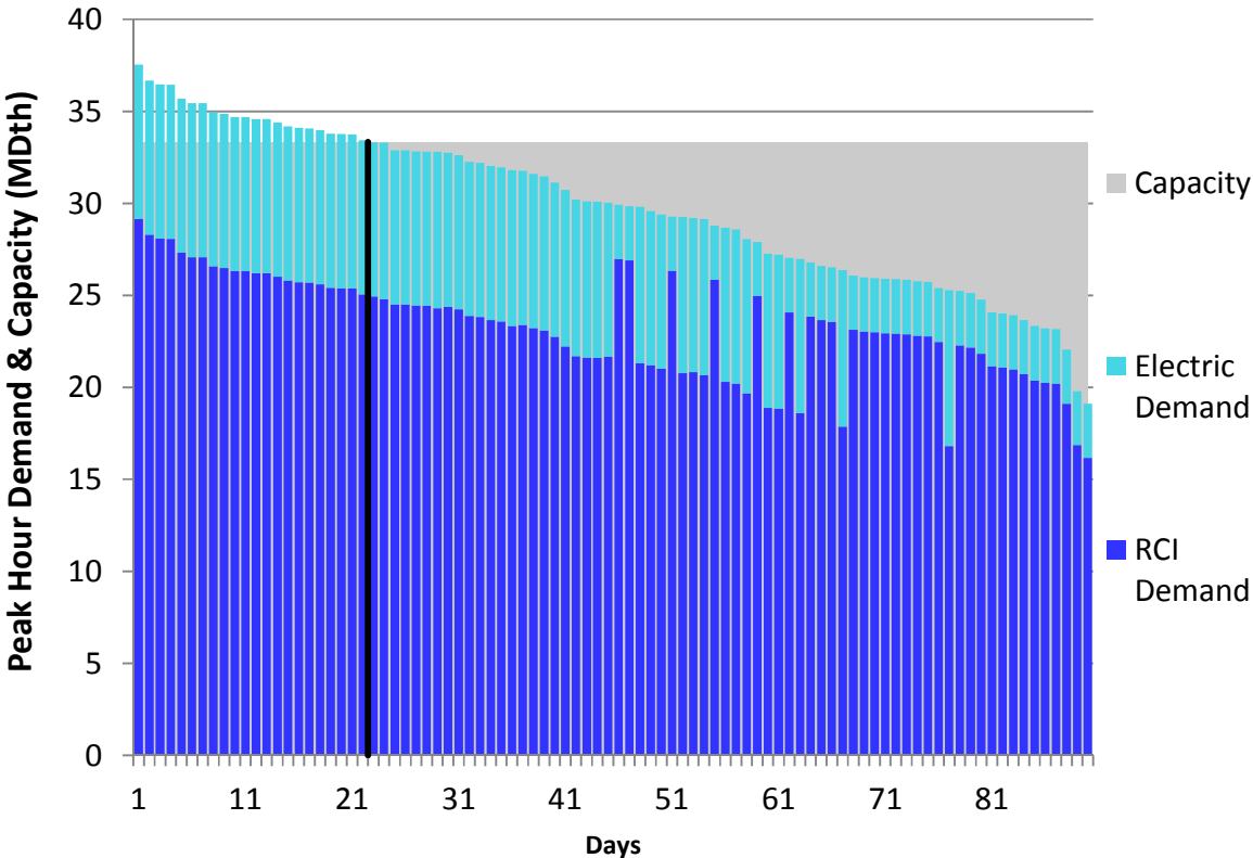
Figure H72. HGDS S2 Winter 2023 – East Tennessee – Descending Demand
