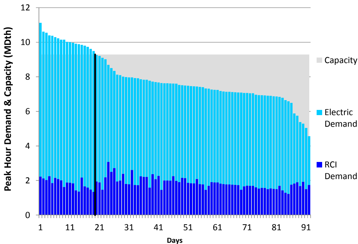
Figure H54. HGDS S2 Summer 2018 – PNGTS N of Westbrook – Descending Demand
