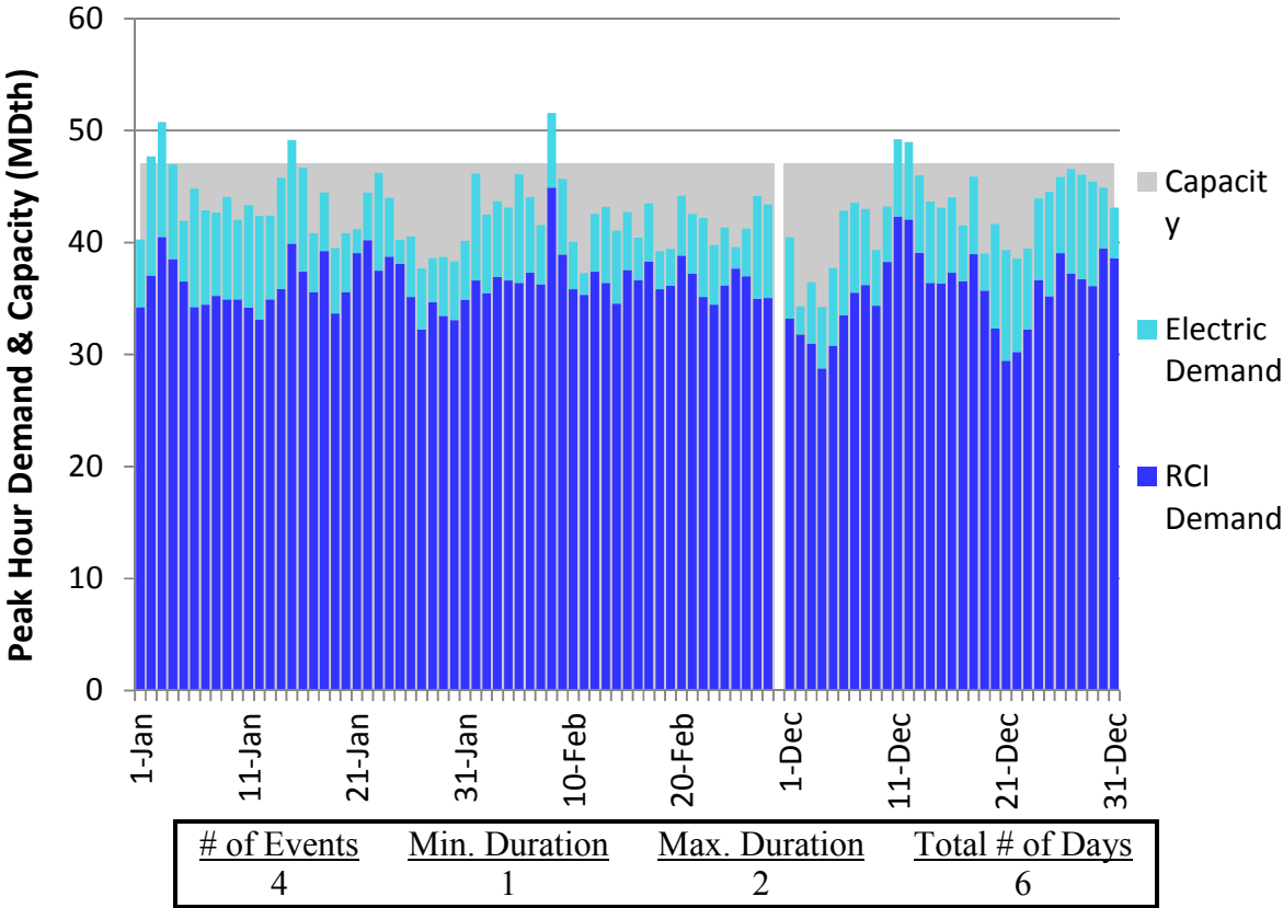
Figure H168. LGDS S2 Winter 2023 – Columbia Gas W PA/NY – Descending Demand
