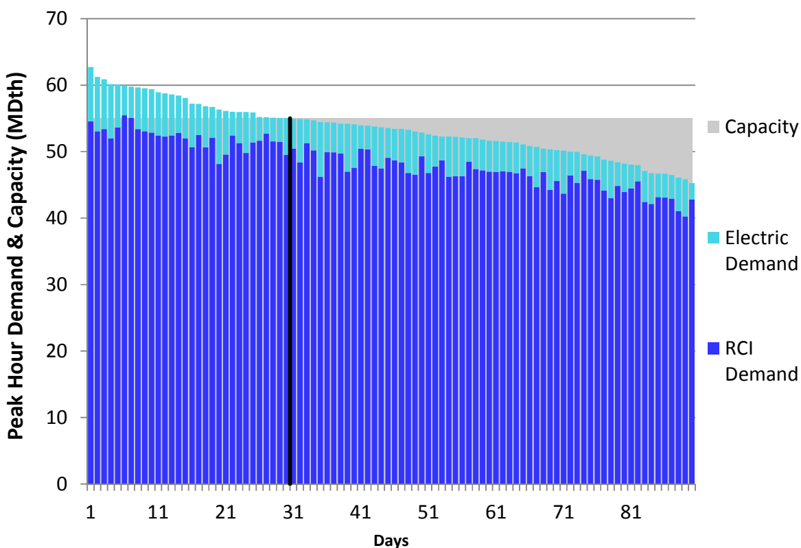
Figure H256. RGDS S3 Winter 2018 – TransCanada Quebec – Descending Demand
