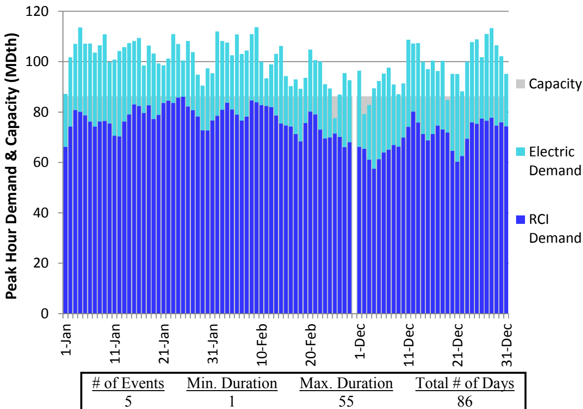
Figure H86. HGDS S2 Winter 2023 – Texas Eastern M2 PA South – Descending Demand
