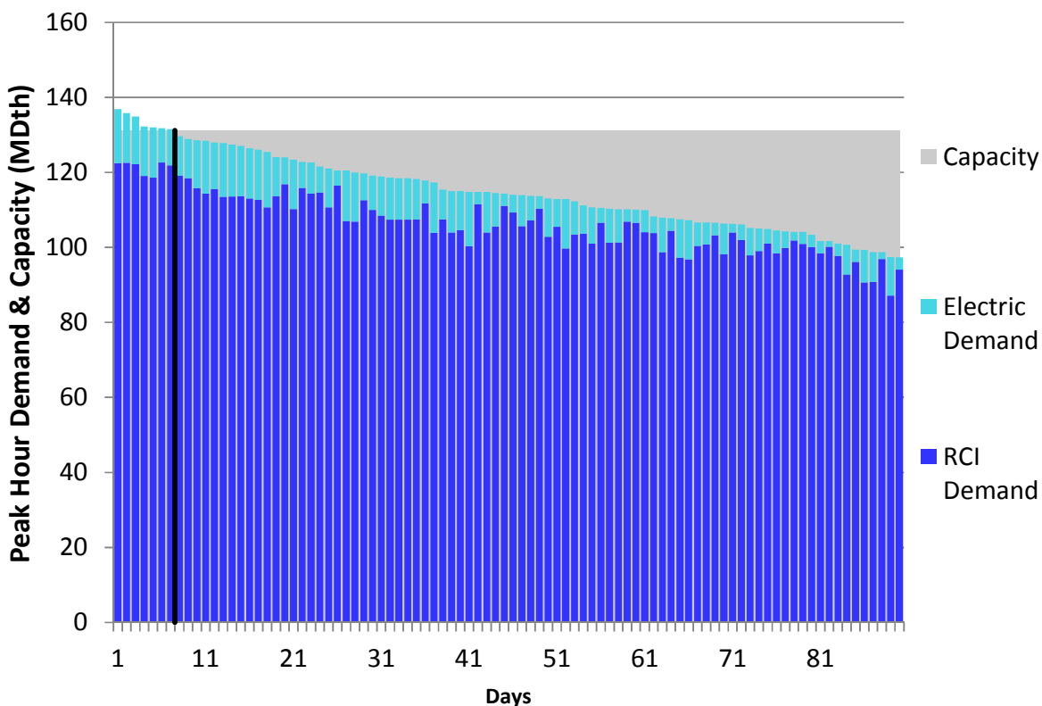
Figure H32. HGDS S2 Winter 2018 – TransCanada Ontario West – Descending Demand
