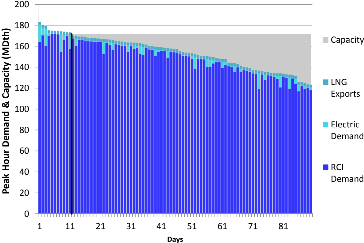
Figure H96. HGDS S2 Winter 2023 – Transco Z5 – Descending Demand
