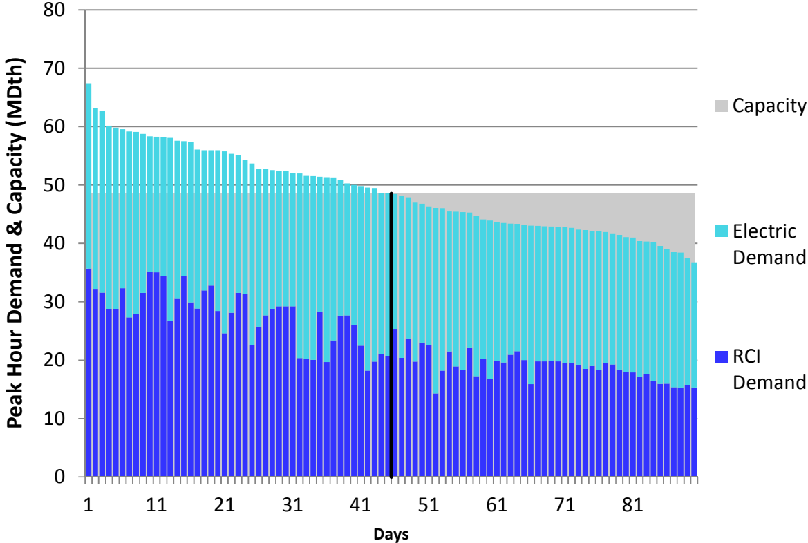
Figure H294. RGDS S3 Winter 2023 – Great Lakes East – Descending Demand
