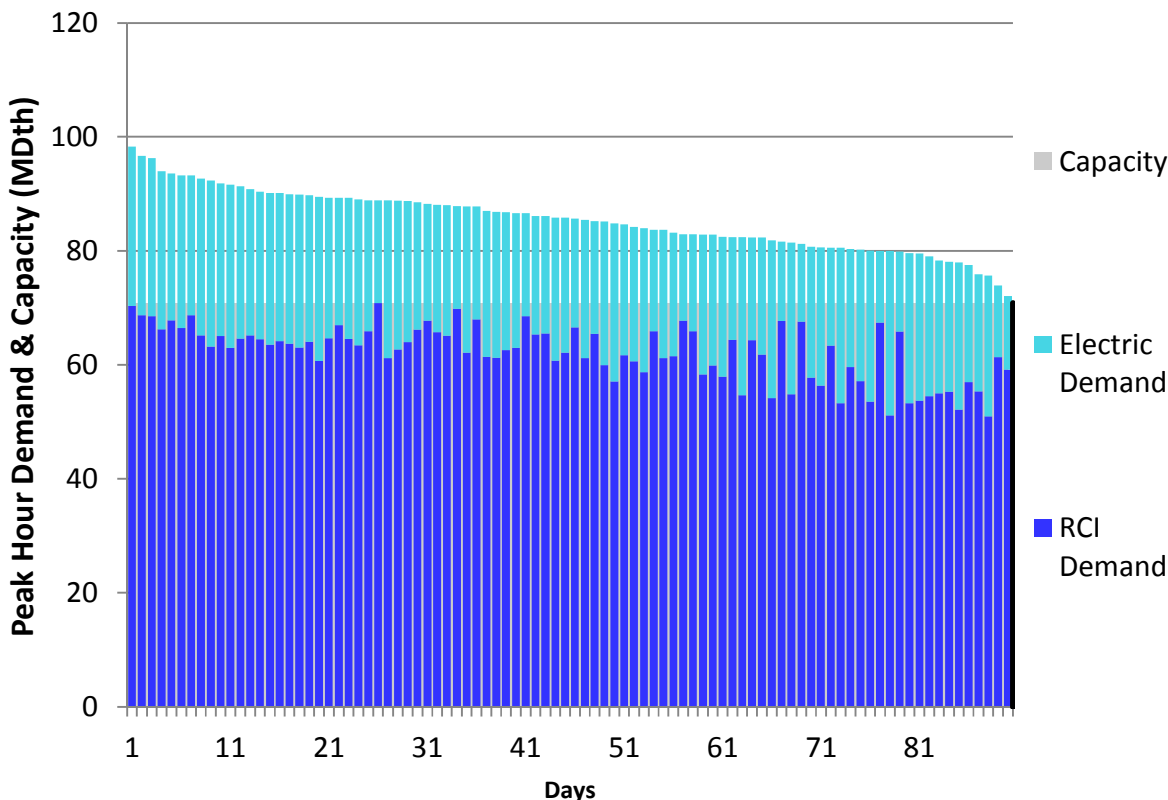
Figure H312. RGDS S3 Winter 2023 – Transco Leidy Atlantic – Descending Demand
