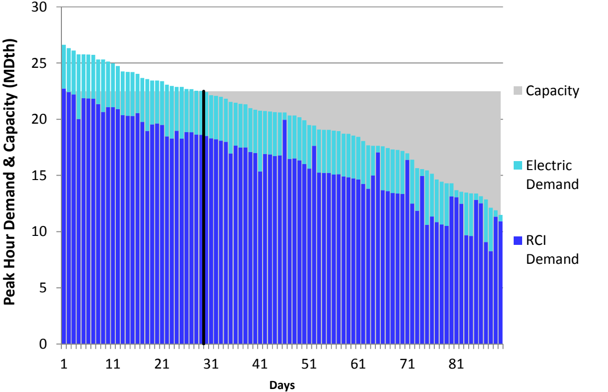
Figure H12. HGDS S2 Winter 2018 – Dominion Southeast – Descending Demand
