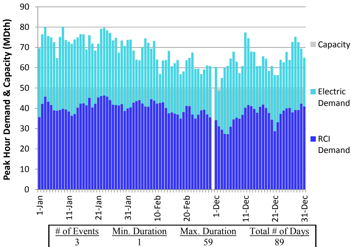
Figure H302. RGDS S3 Winter 2023 – Tennessee Z5 NY – Descending Demand
