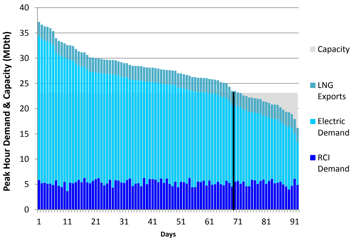
Figure H324. RGDS S3 Summer 23 – Dominion Southeast – Descending Demand
