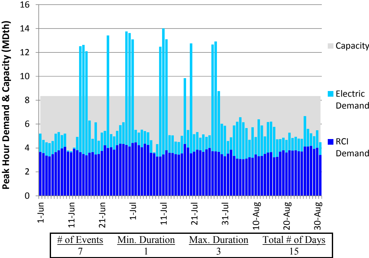
Figure H214. LGDS S2 Summer 2023 – Eastern Shore – Descending Demand
