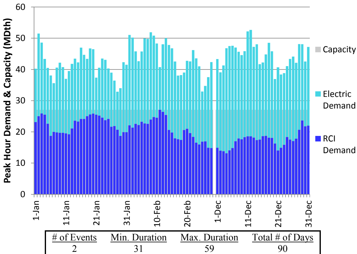
Figure H170. LGDS S2 Winter 2023 – Constitution – Descending Demand
