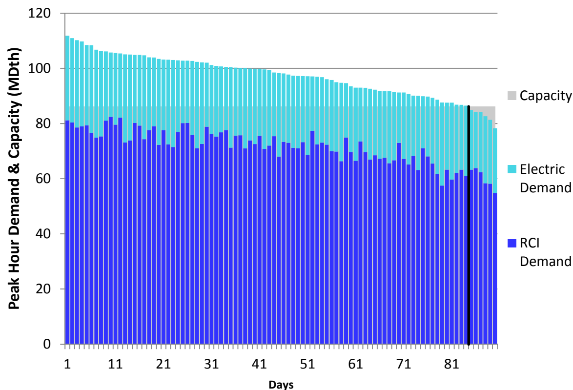
Figure H250. RGDS S3 Winter 2018 – Texas Eastern M2 PA South – Descending Demand
