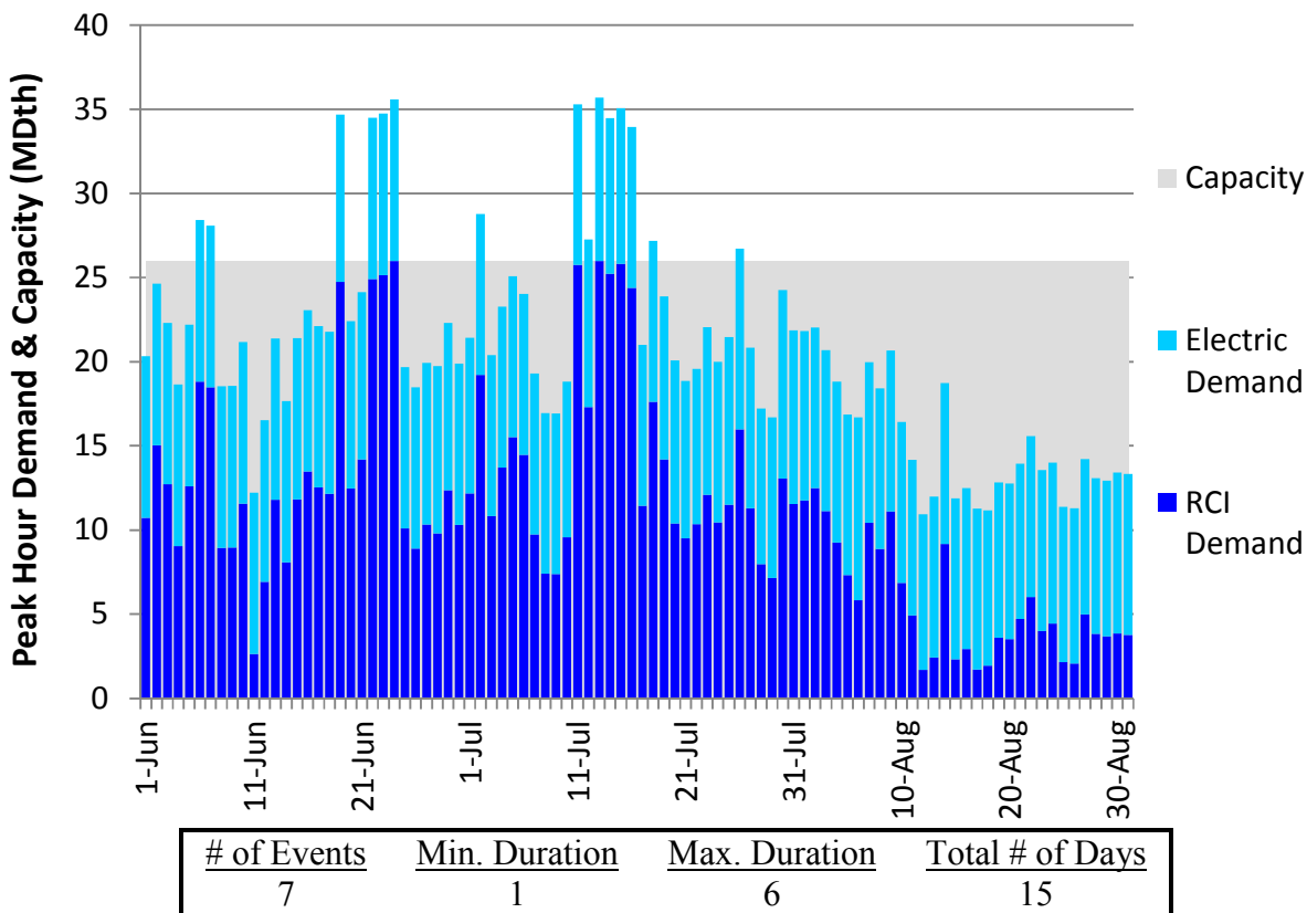
Figure H162. LGDS S2 Summer 2018 – Texas Eastern ETX – Descending Demand
