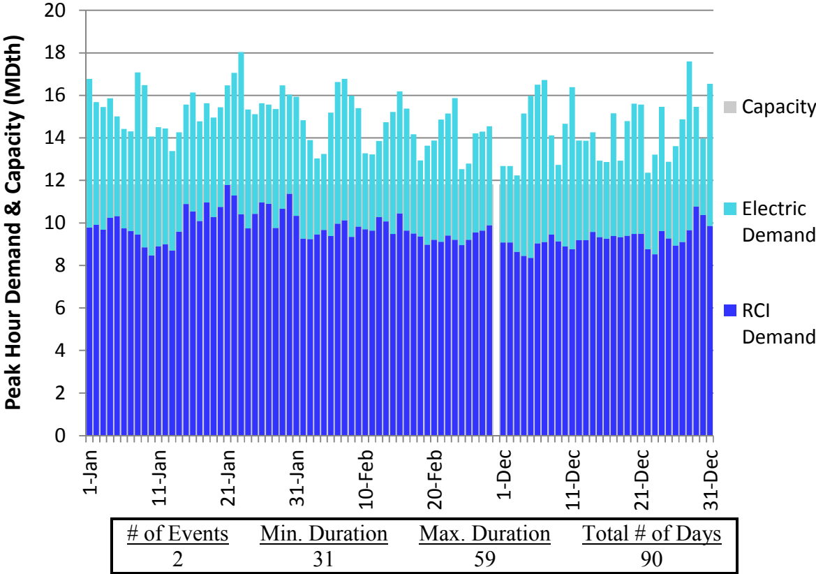
Figure H186. LGDS S2 Winter 2023 – NB/NS Supply – Descending Demand
