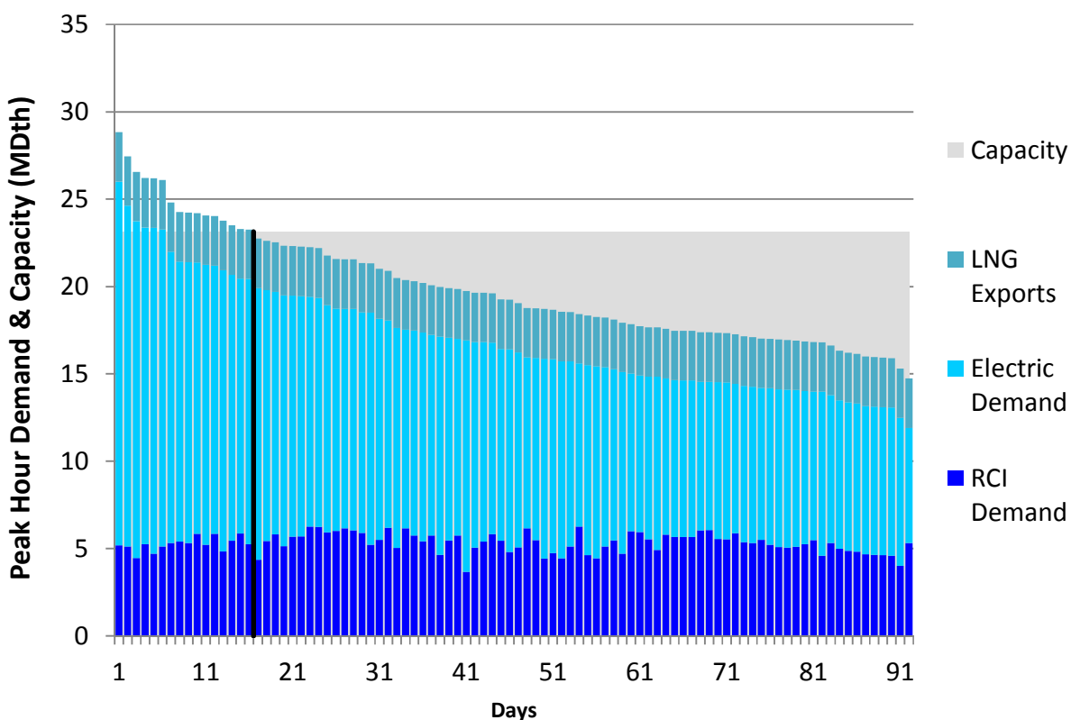
Figure H212. LGDS S2 Summer 2023 – Dominion Southeast – Descending Demand
