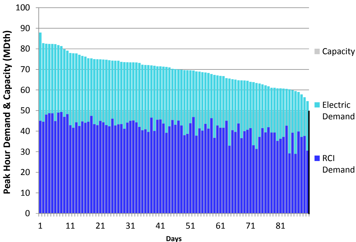
Figure H248. RGDS S3 Winter 2018 – Tennessee Z5 NY – Descending Demand
