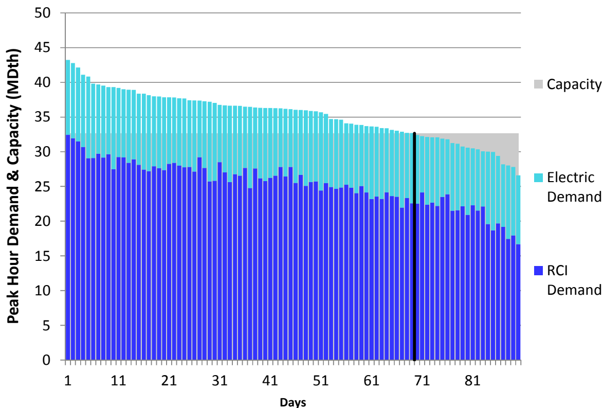
Figure H242. RGDS S3 Winter 2018 – Millennium – Descending Demand
