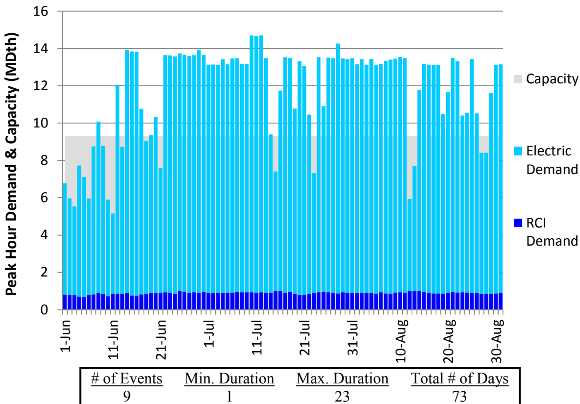
Figure H112. HGDS S2 Summer 2023 – PNGTS N of Westbrook – Descending Demand
