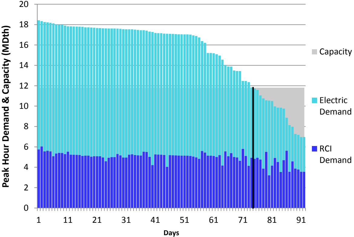
Figure H110. HGDS S2 Summer 2023 – NB/NS Supply – Descending Demand
