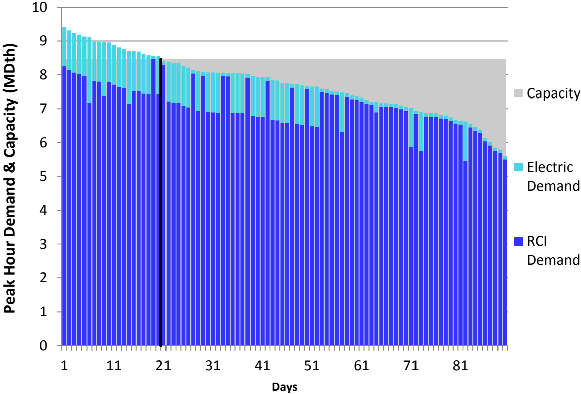
Figure H238. RGDS S3 Winter 2018 – Eastern Shore – Descending Demand
