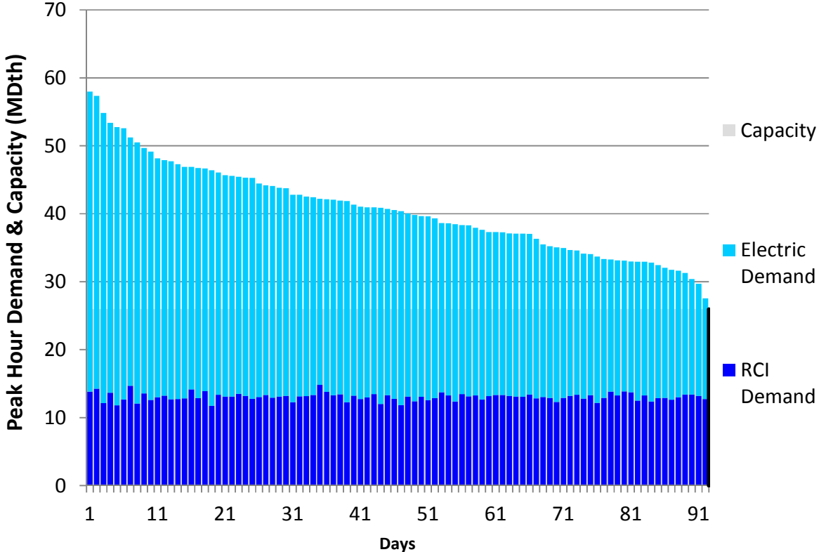
Figure H114. HGDS S2 Summer 2023 – Tennessee Z5 NY – Descending Demand
