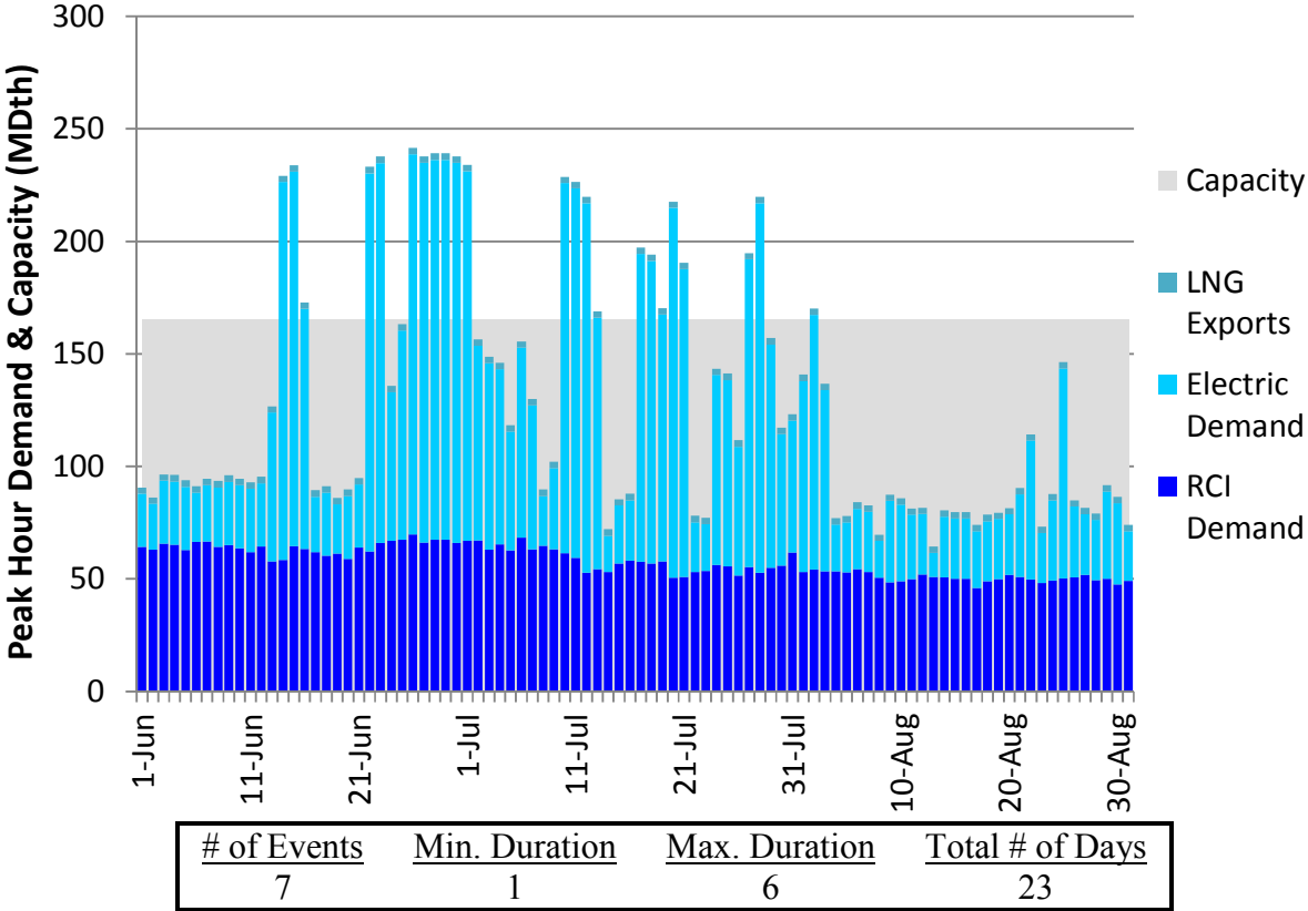
Figure H118. HGDS S2 Summer 2023 – Transco Z5 – Descending Demand
