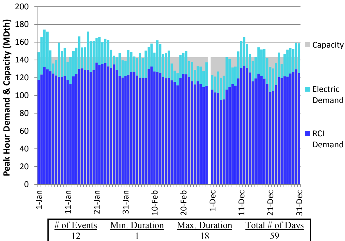
Figure H152. LGDS S2 Winter 2018 – Transco Leidy to Station 210 – Descending Demand
