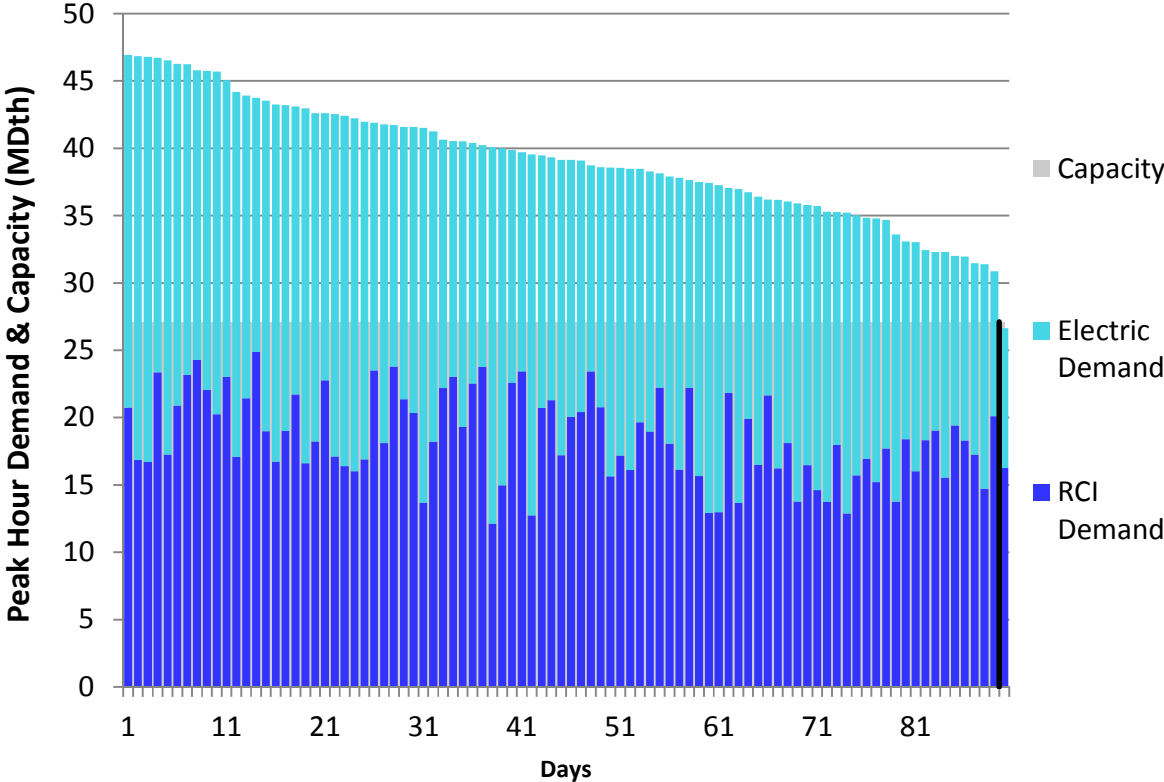
Figure H122. LGDS S2 Winter 2018 – Constitution – Descending Demand
