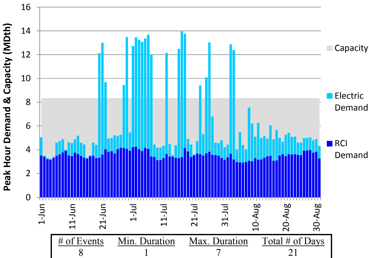
Figure H160. LGDS S2 Summer 2018 – Eastern Shore – Descending Demand
