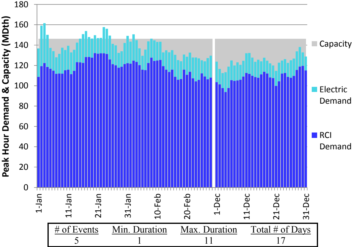
Figure H90. HGDS S2 Winter 2023 – TransCanada Ontario West – Descending Demand
