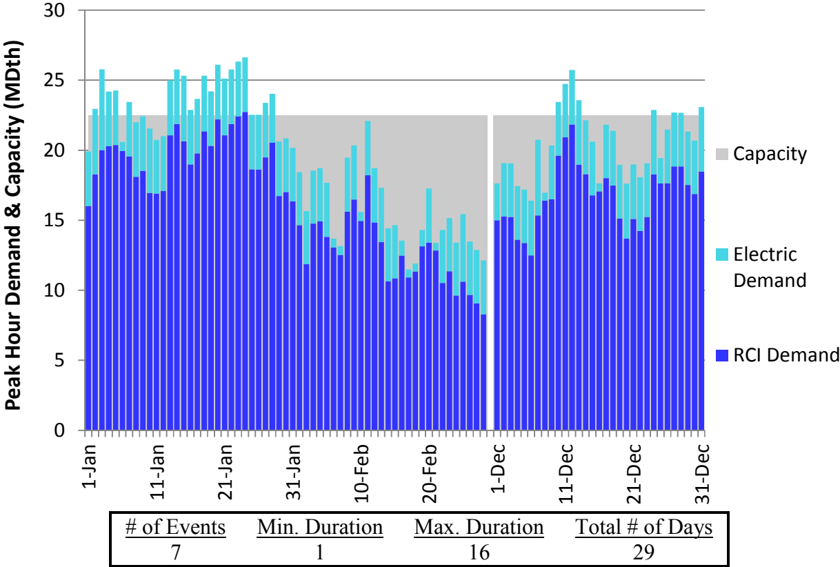
Figure H12. HGDS S2 Winter 2018 – Dominion Southeast – Descending Demand
