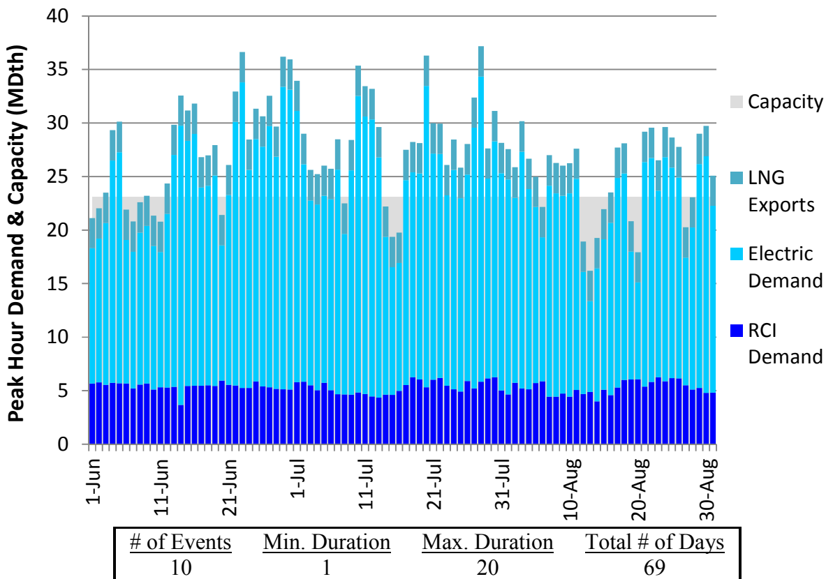
Figure H324. RGDS S3 Summer 23 – Dominion Southeast – Descending Demand
