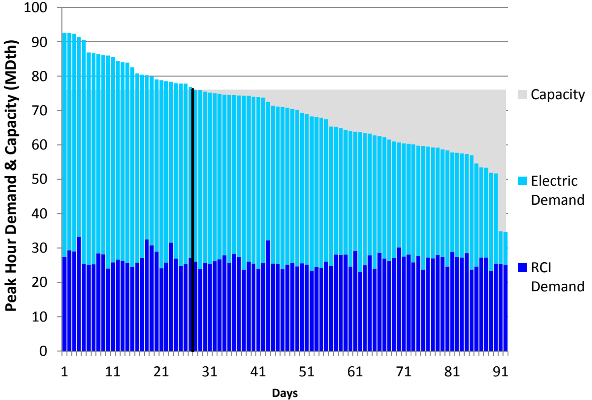
Figure H320. RGDS S3 Summer 2023 – Algonquin CT – Descending Demand
