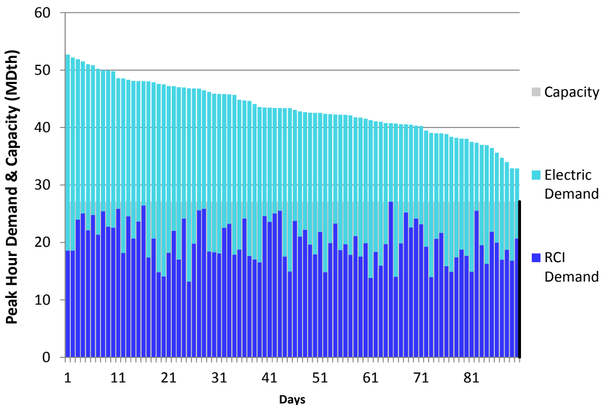
Figure H170. LGDS S2 Winter 2023 – Constitution – Descending Demand
