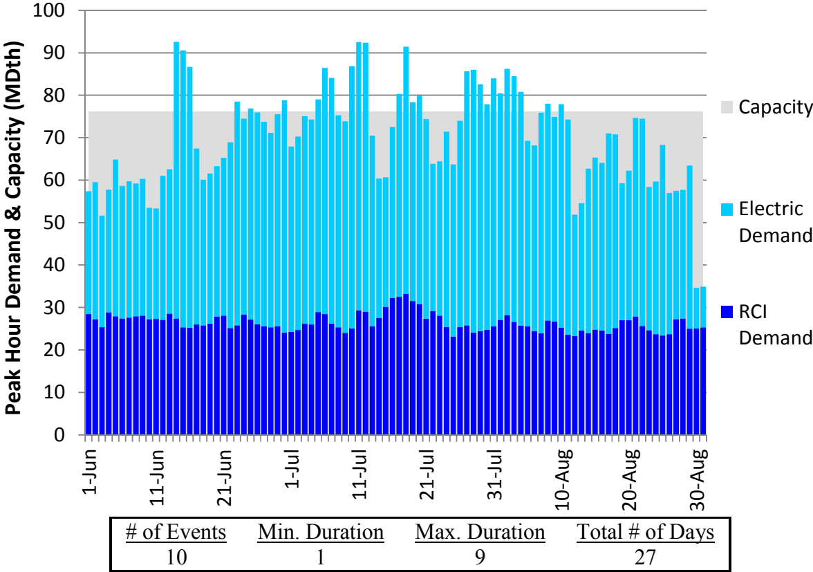
Figure H320. RGDS S3 Summer 2023 – Algonquin CT – Descending Demand
