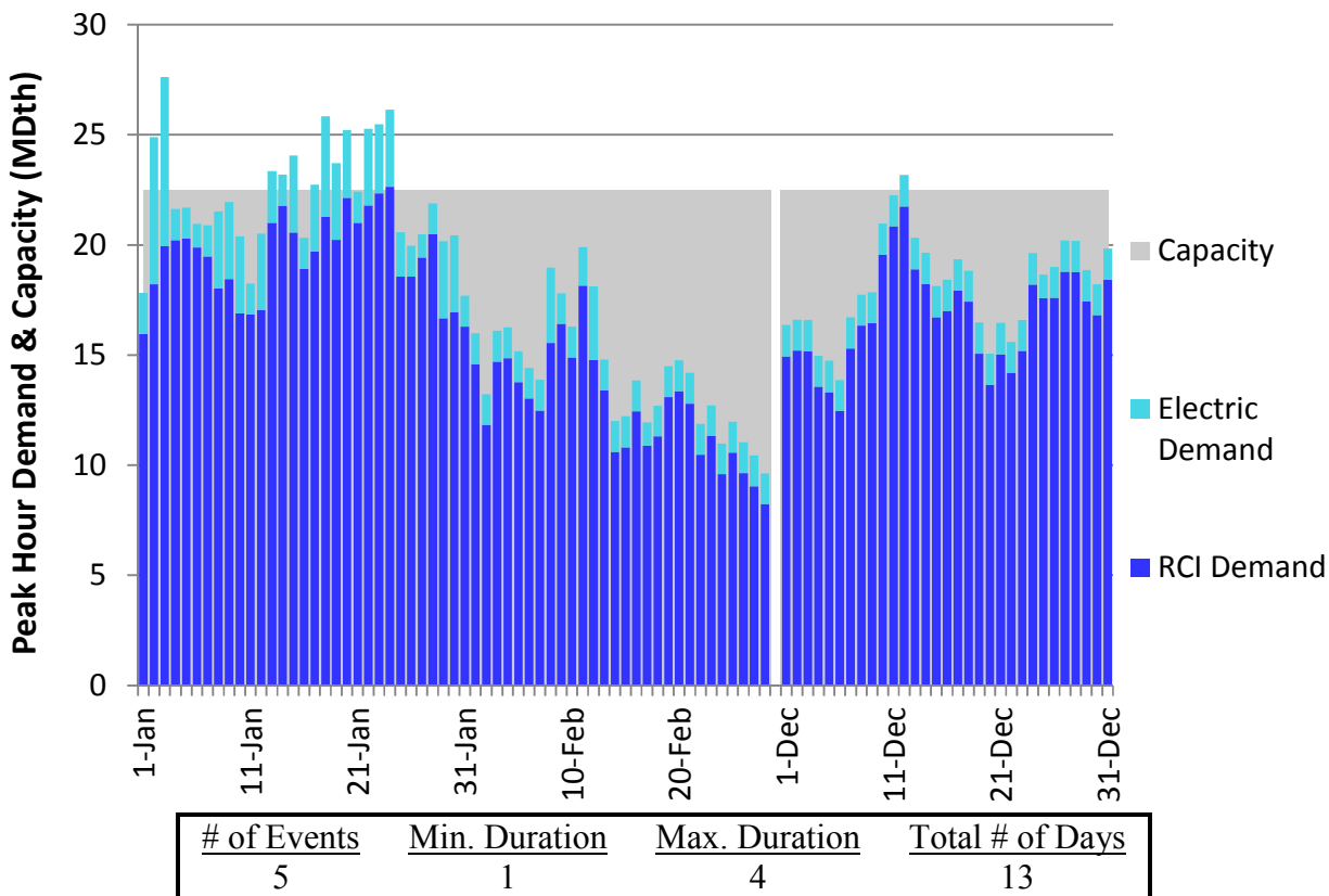
Figure H234. RGDS S3 Winter 2018 – Dominion Southeast – Descending Demand
