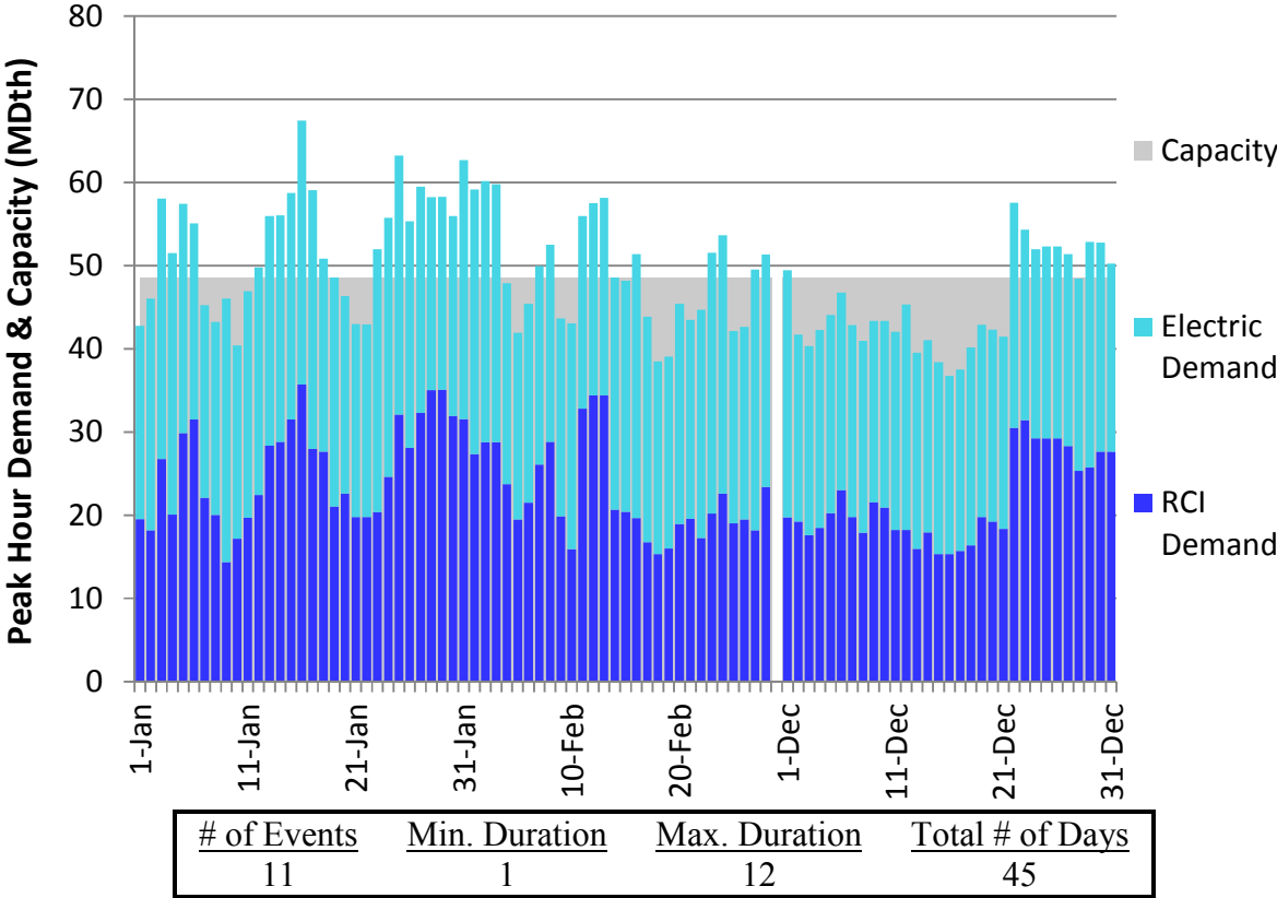
Figure H294. RGDS S3 Winter 2023 – Great Lakes East – Descending Demand
