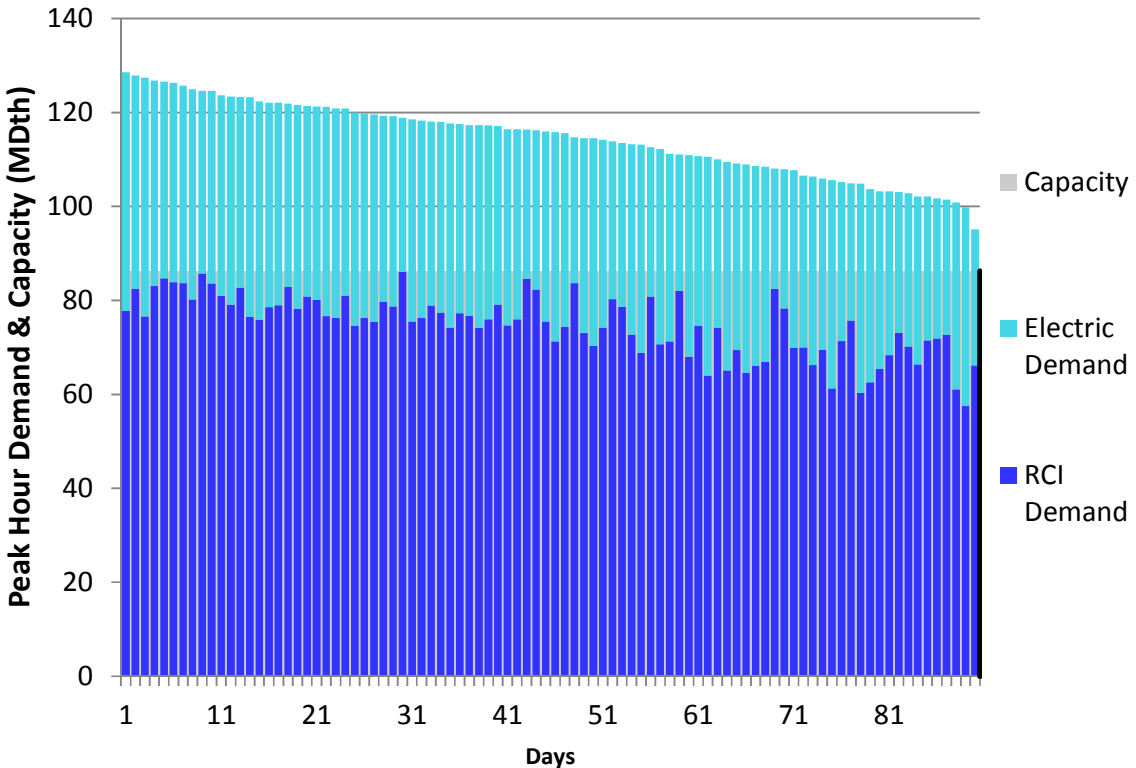
Figure E124. HGDS S0 Winter 2023 – Texas Eastern M2 PA South – Descending Demand
