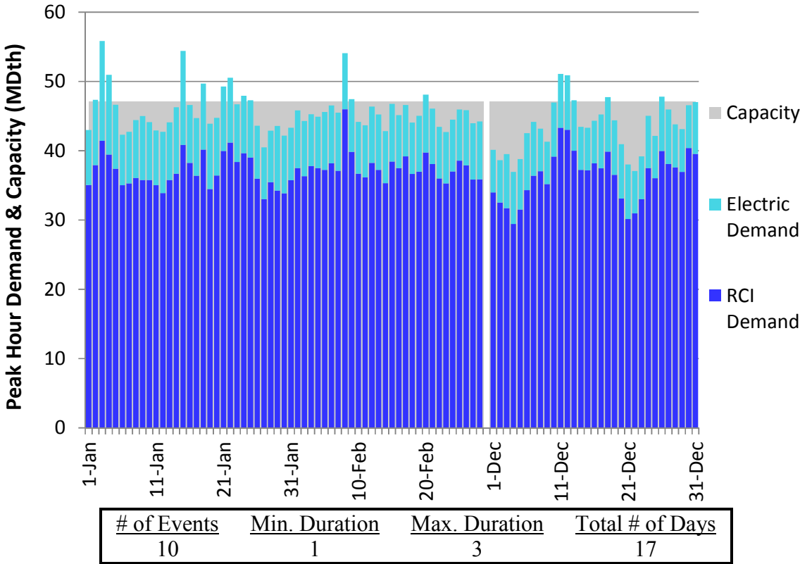
Figure E8. HGDS S0 Winter 2018 – Columbia Gas W PA/NY – Descending Demand
