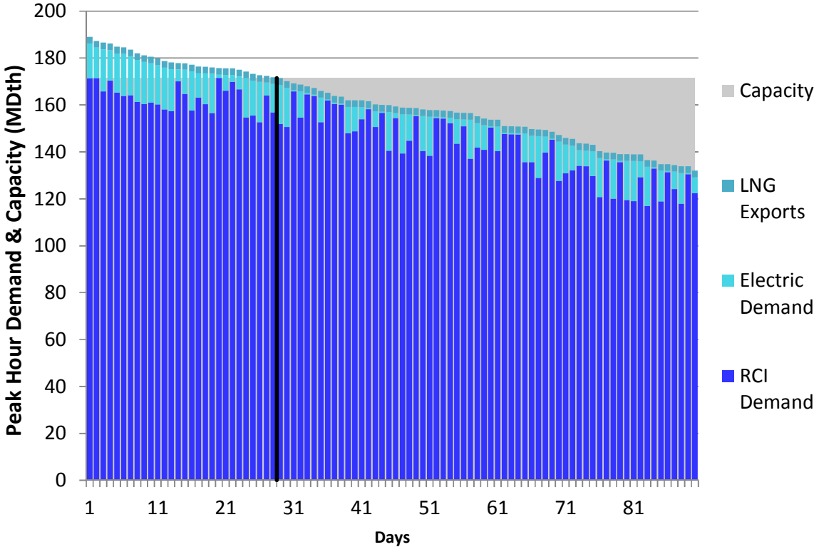
Figure E134. HGDS S0 Winter 2023 – Transco Z5 – Descending Demand
