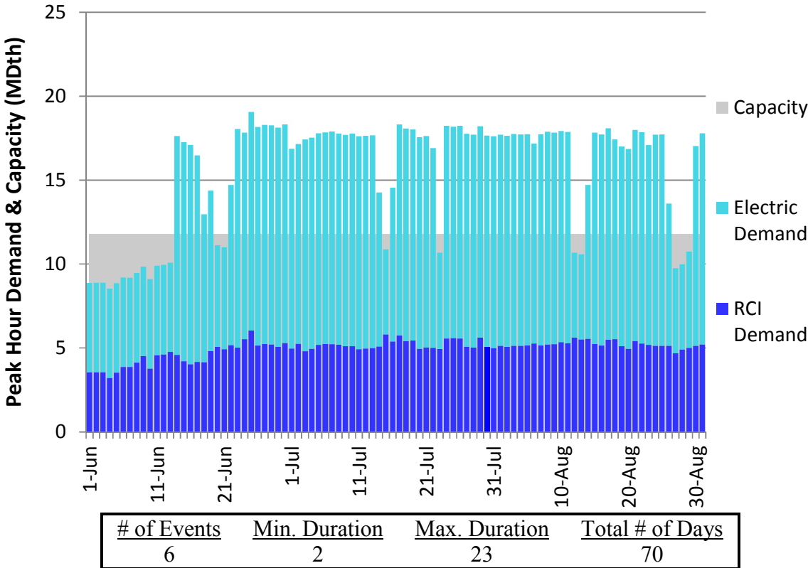
Figure E156. HGDS S0 Summer 2023 – NB/NS – Descending Demand
