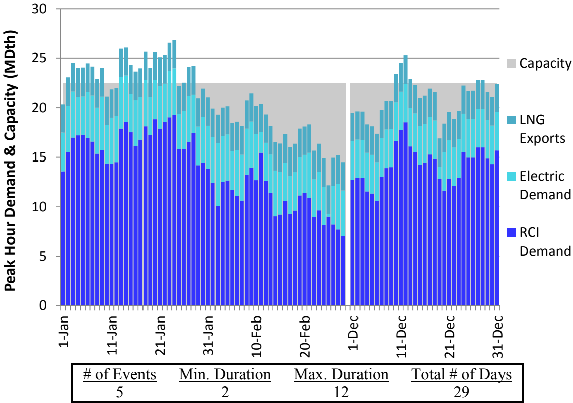
Figure E214. LGDS S0 Winter 2023 – Dominion Southeast – Descending Demand
