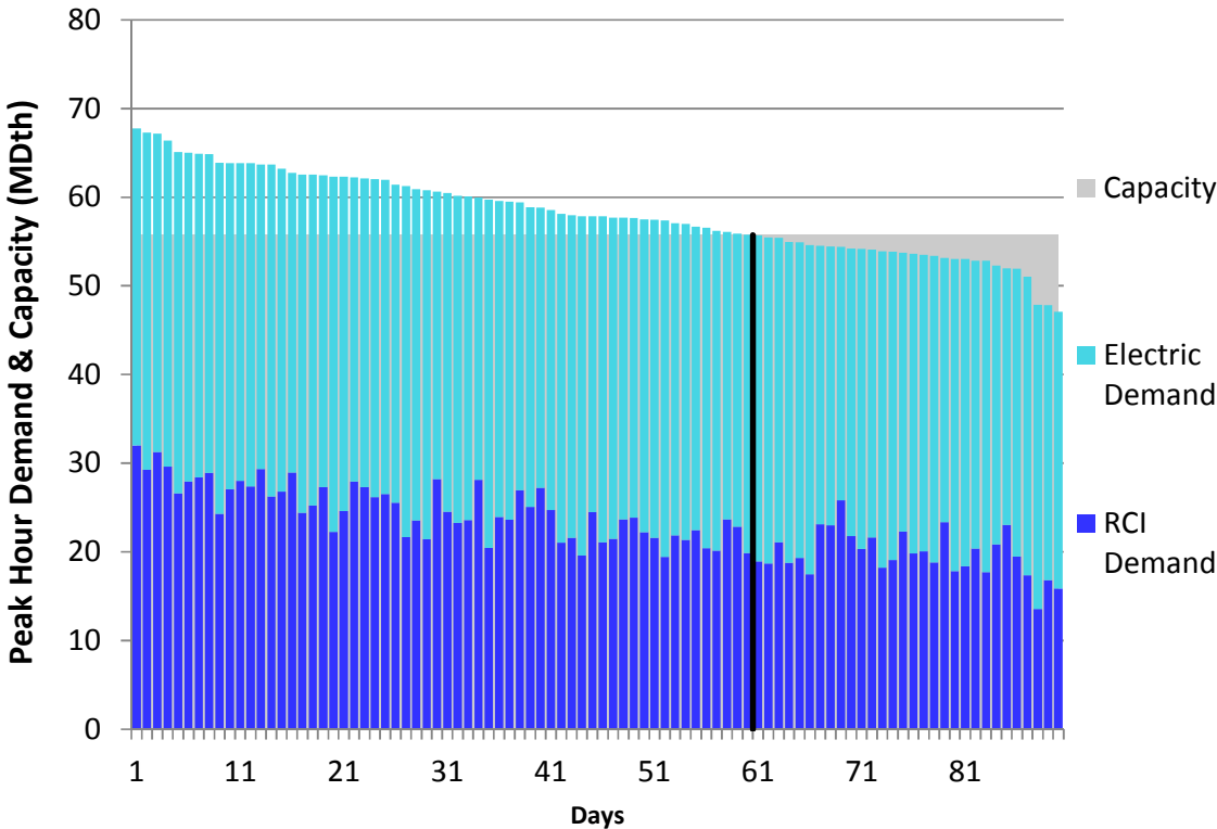
Figure E4. HGDS S0 Winter 2018 – ANR Northern IL – Descending Demand
