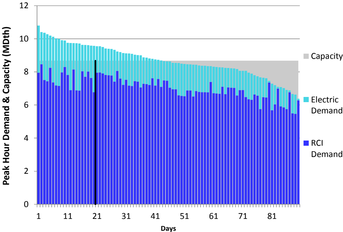
Figure E20. HGDS S0 Winter 2018 – Eastern Shore – Descending Demand
