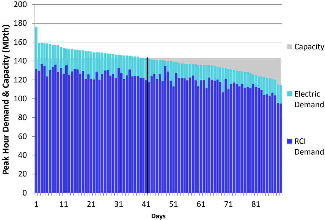
Figure E190. LGDS S0 Winter 2018 – Transco Leidy to 210 – Descending Demand
