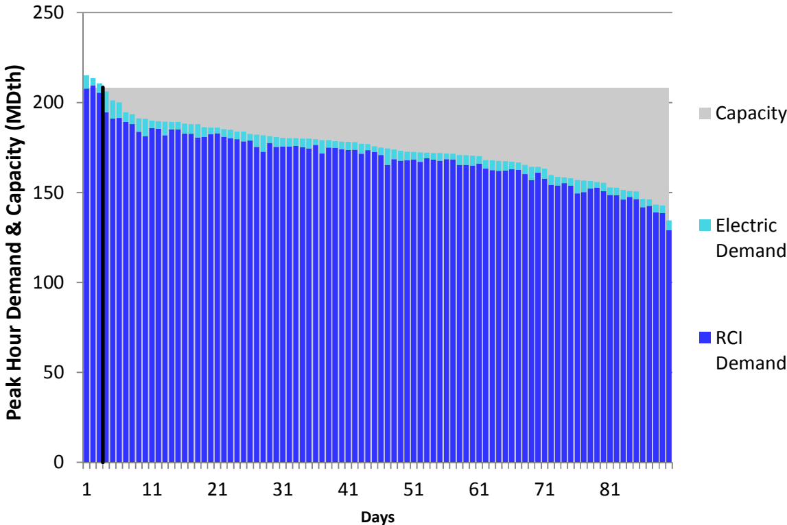
Figure E192. LGDS S0 Winter 2018 – Union Gas Dawn – Descending Demand
