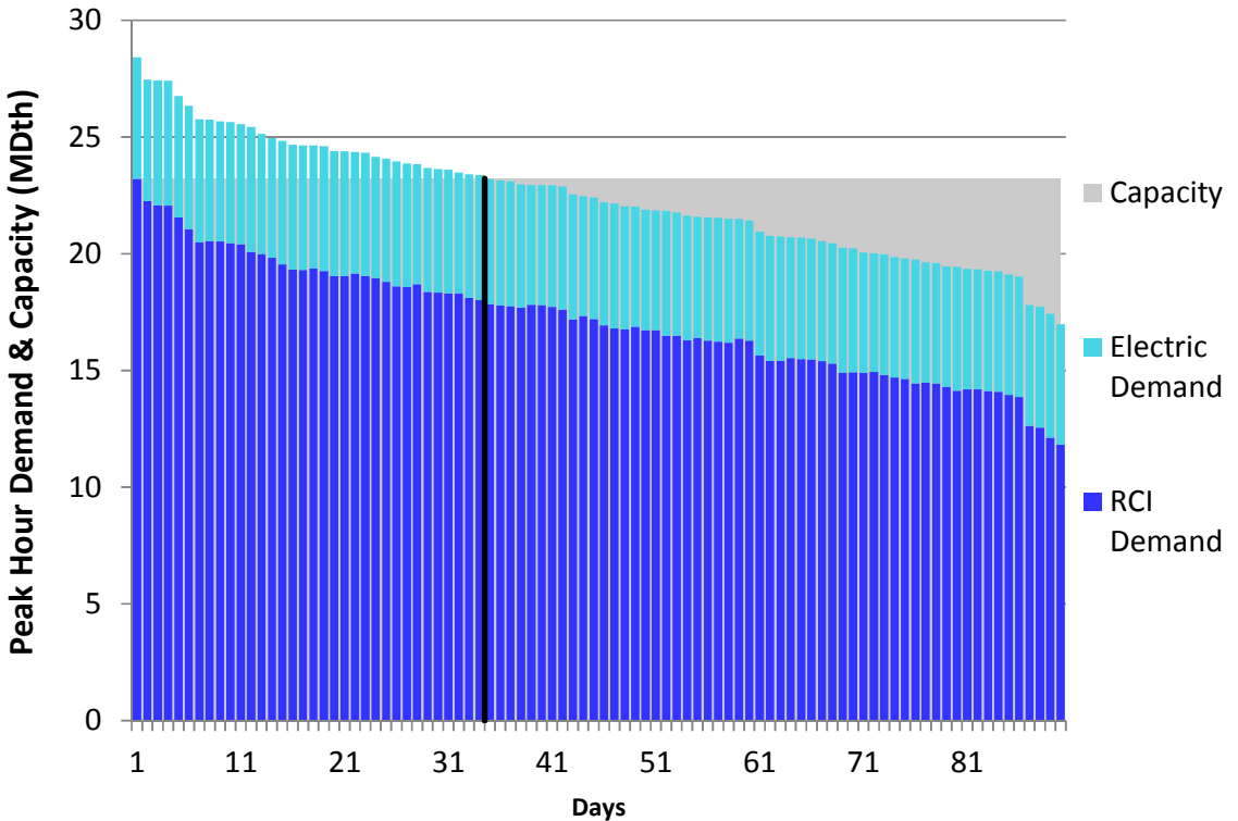
Figure E14. HGDS S0 Winter 2018 – Dominion Western NY– Descending Demand
