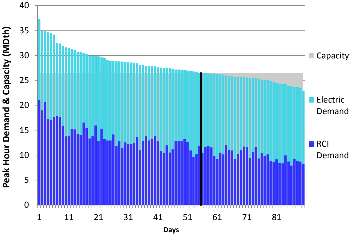
Figure E26. HGDS S0 Winter 2018 – Midwestern – Descending Demand
