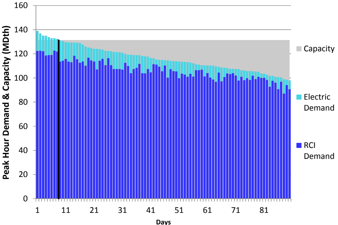
Figure E48. HGDS S0 Winter 2018 – TransCanada Ontario West – Descending Demand
