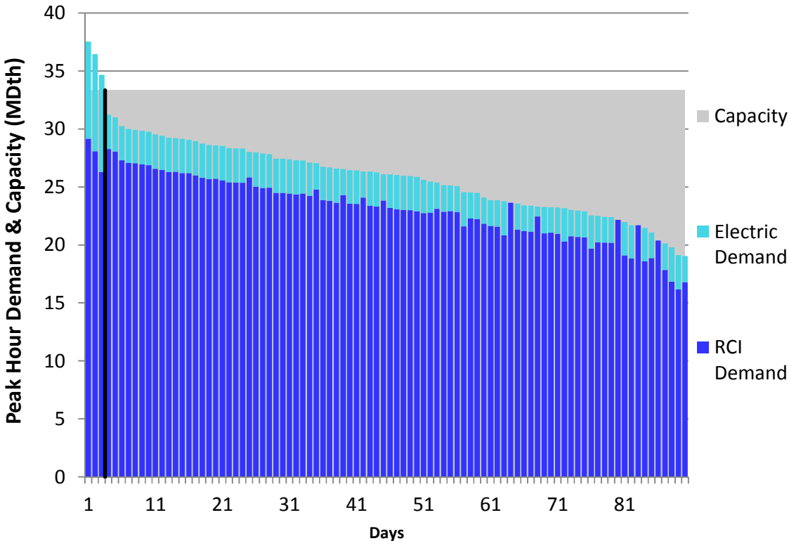
Figure E216. LGDS S0 Winter 2023 – East Tennessee – Descending Demand
