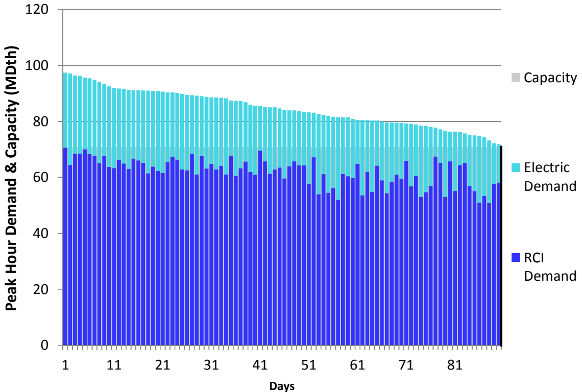
Figure E52. HGDS S0 Winter 2018 – Transco Leidy Atlantic – Descending Demand
