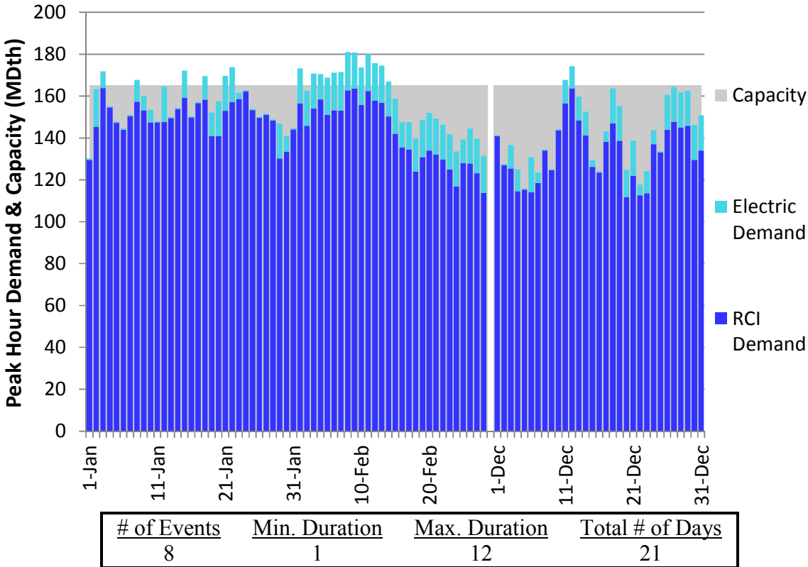
Figure E54. HGDS S0 Winter 2018 – Transco Z5 – Descending Demand
