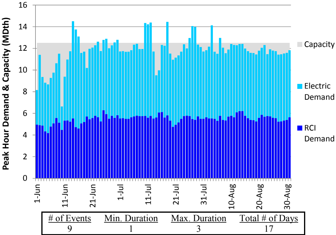
Figure E252. LGDS S0 Summer 2023 – PNGTS S of Westbrook – Descending Demand
