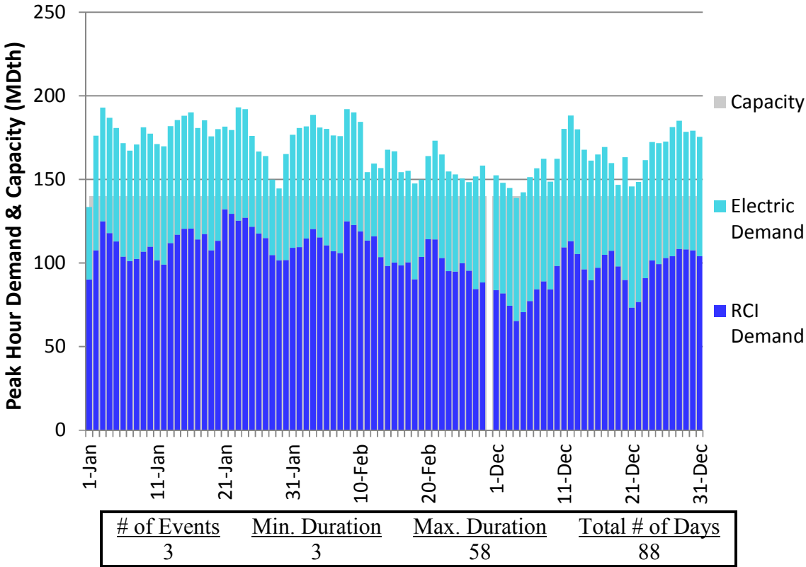
Figure E126. HGDS S0 Winter 2023 – Texas Eastern M3 North – Descending Demand
