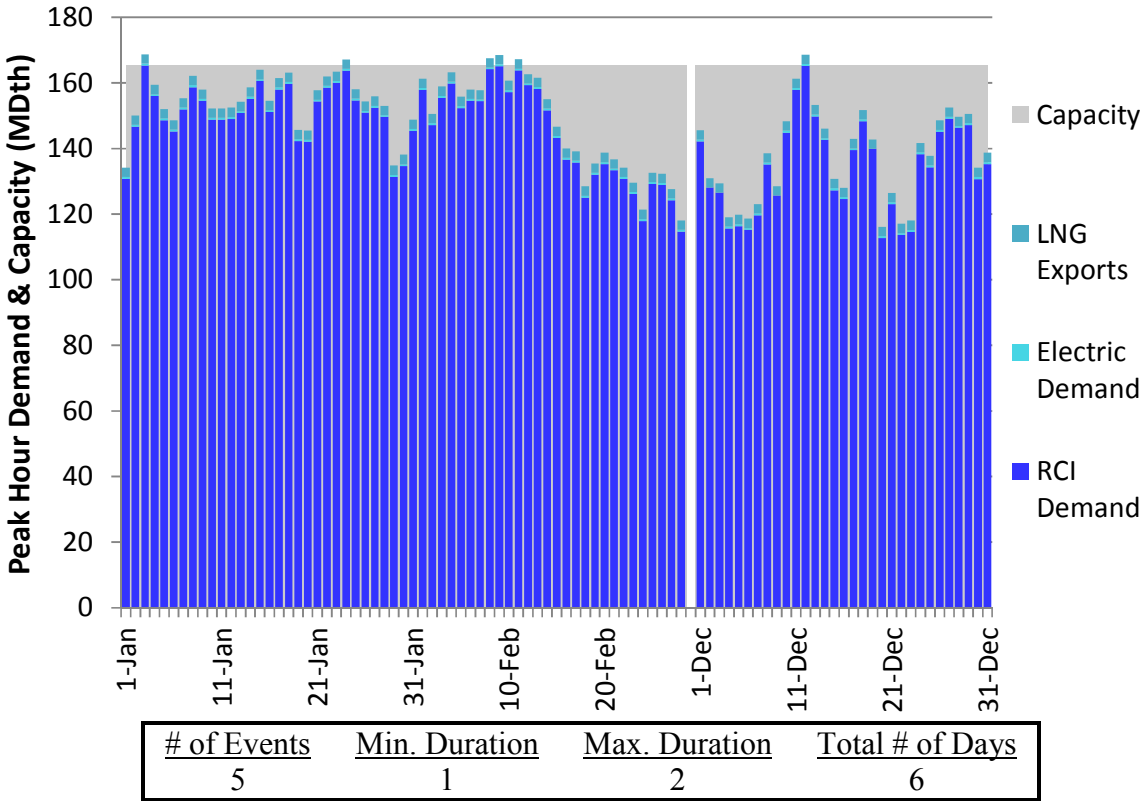
Figure E236. LGDS S0 Winter 2023 – Transco Z5 – Descending Demand
