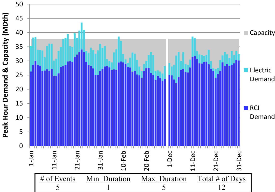
Figure E210. LGDS S0 Winter 2023 – Dominion Eastern NY– Descending Demand
