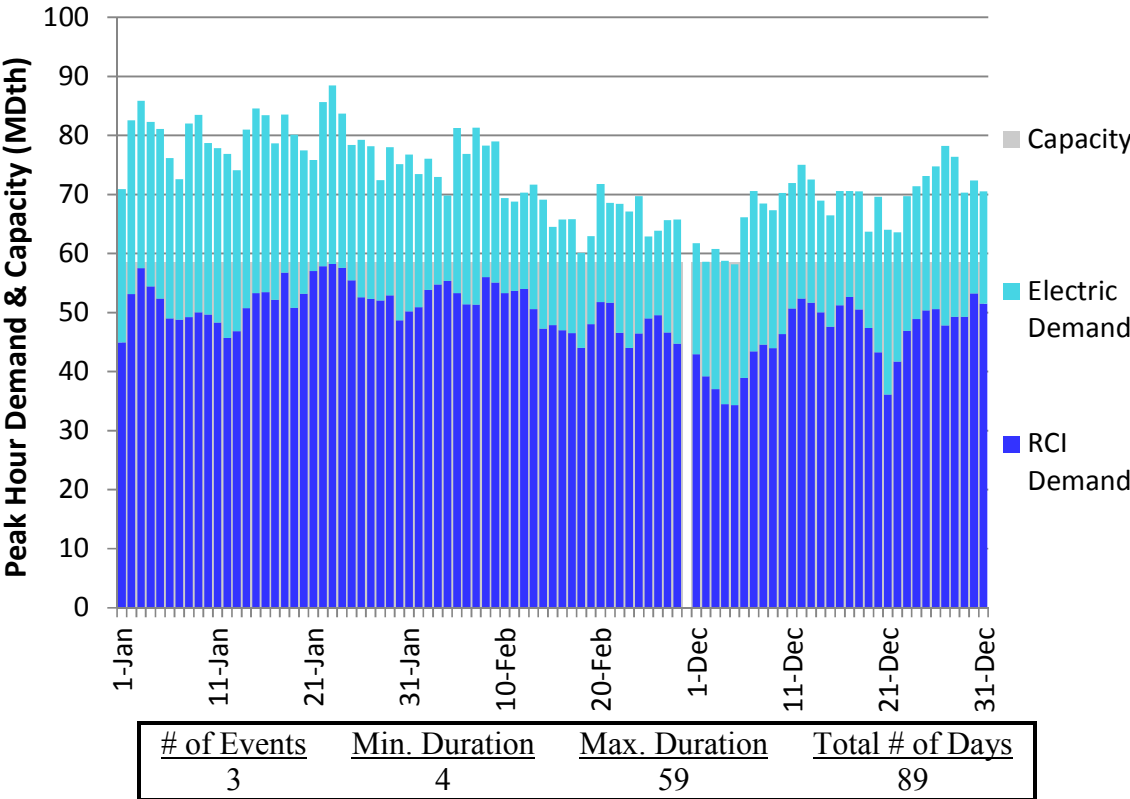
Figure E122. HGDS S0 Winter 2023 – Tennessee Z5 NY – Descending Demand
