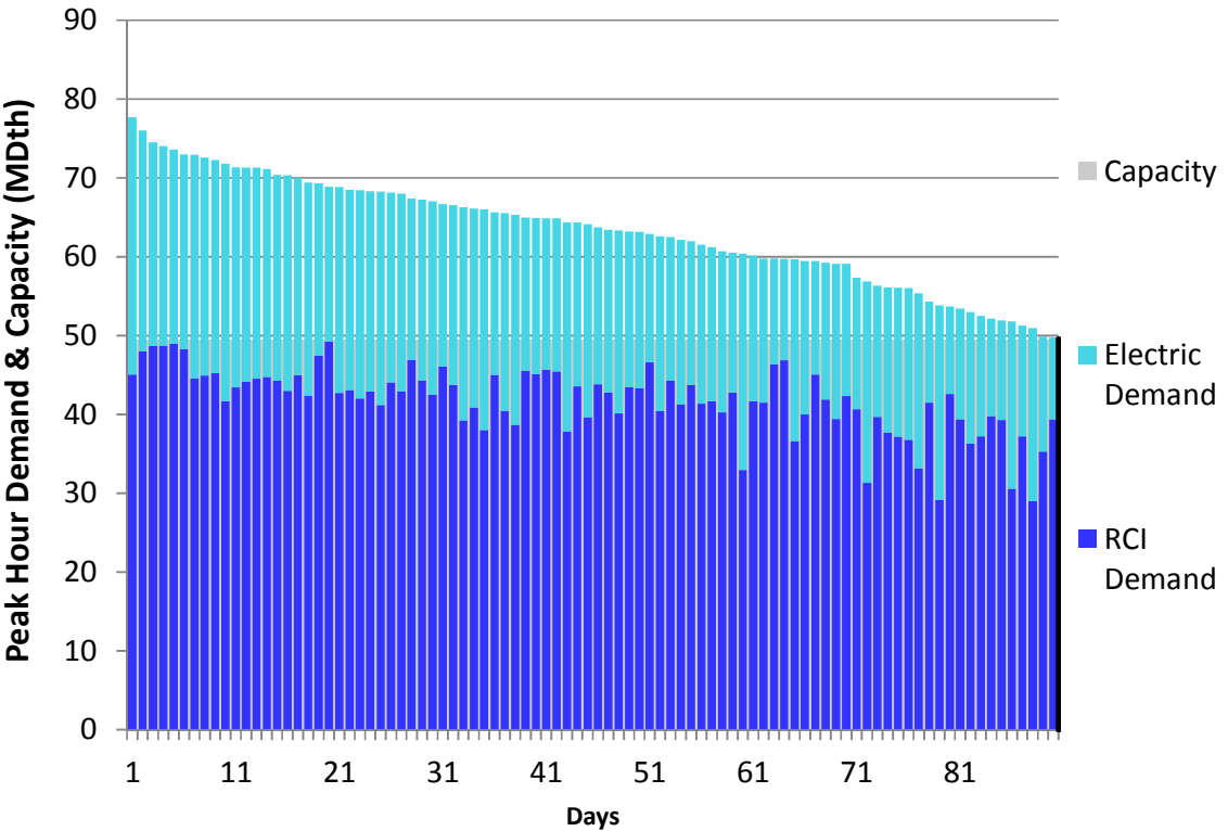
Figure E42. HGDS S0 Winter 2018 – Tennessee Z5 NY – Descending Demand
