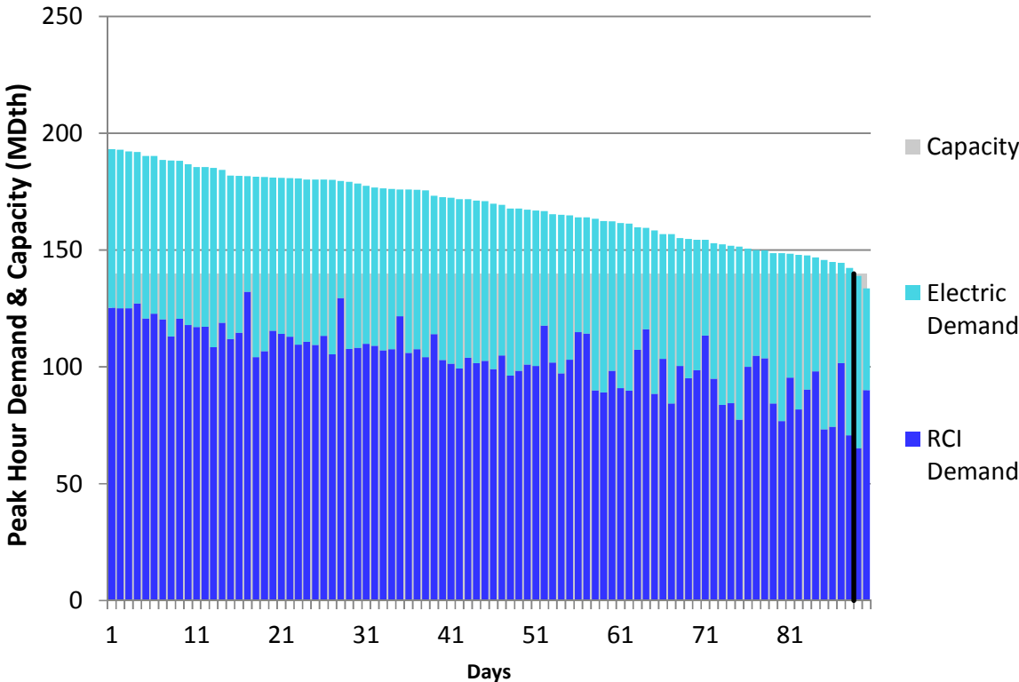
Figure E126. HGDS S0 Winter 2023 – Texas Eastern M3 North – Descending Demand
