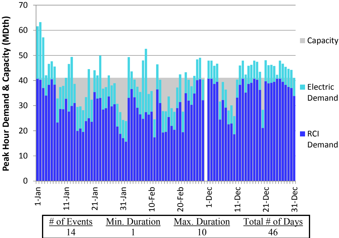
Figure E36. HGDS S0 Winter 2018 – Northern Border Chicago – Descending Demand
