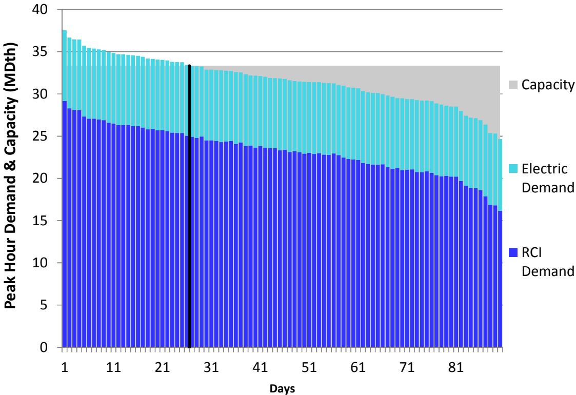
Figure E18. HGDS S0 Winter 2018 – East Tennessee – Descending Demand
