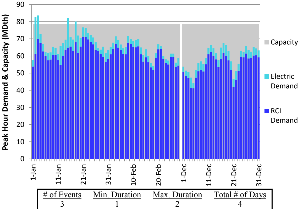
Figure E178. LGDS S0 Winter 2018 – Tennessee Z4 PA – Descending Demand
