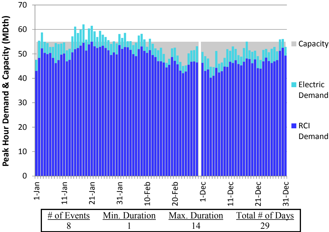
Figure E50. HGDS S0 Winter 2018 – TransCanada Quebec – Descending Demand
