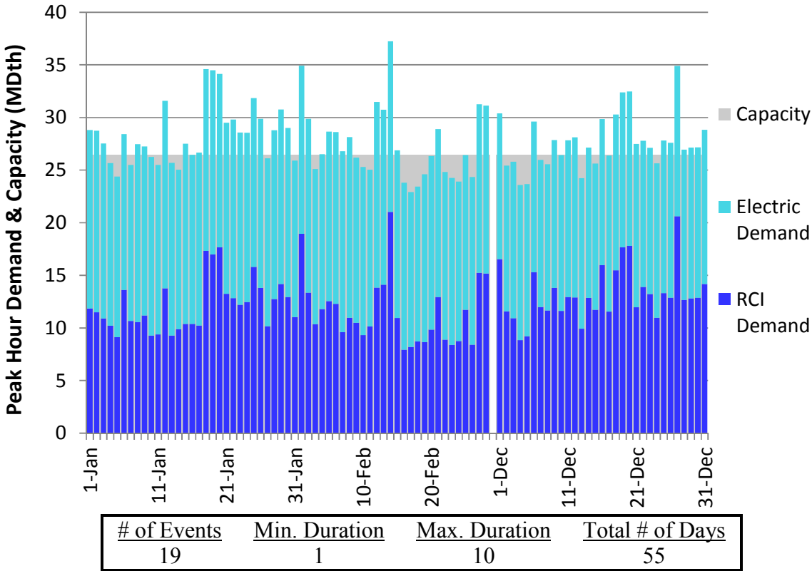
Figure E26. HGDS S0 Winter 2018 – Midwestern – Descending Demand
