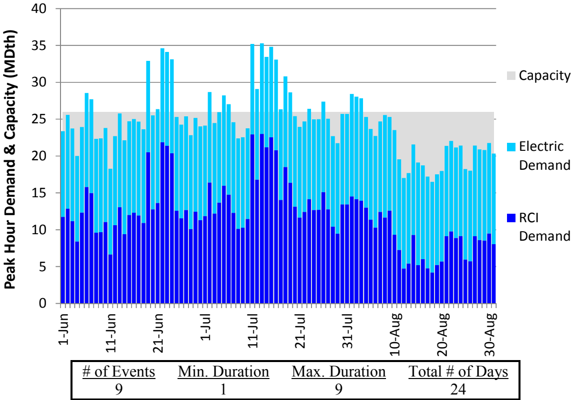
Figure E76. HGDS S0 Summer 2018 – Texas Eastern ETX – Descending Demand
