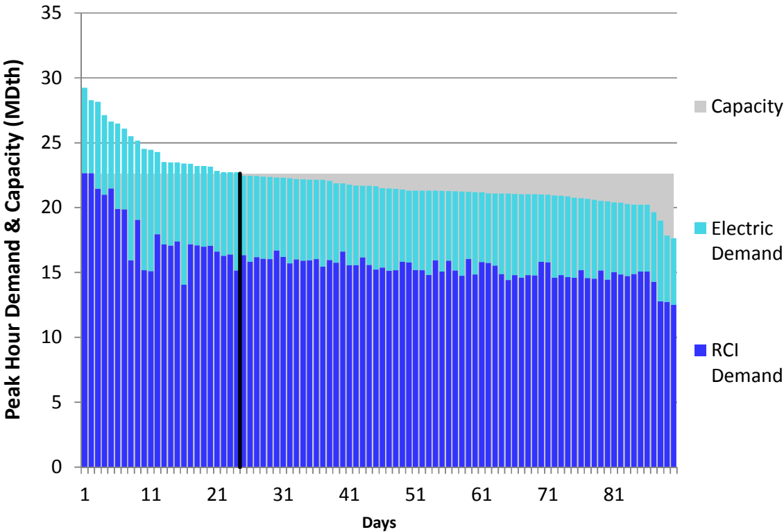
Figure E60. HGDS S0 Winter 2018 – Viking Zone 1 – Descending Demand
