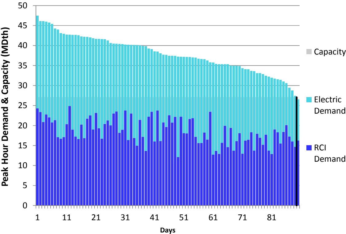
Figure E170. LGDS S0 Winter 2018 – Constitution – Descending Demand
