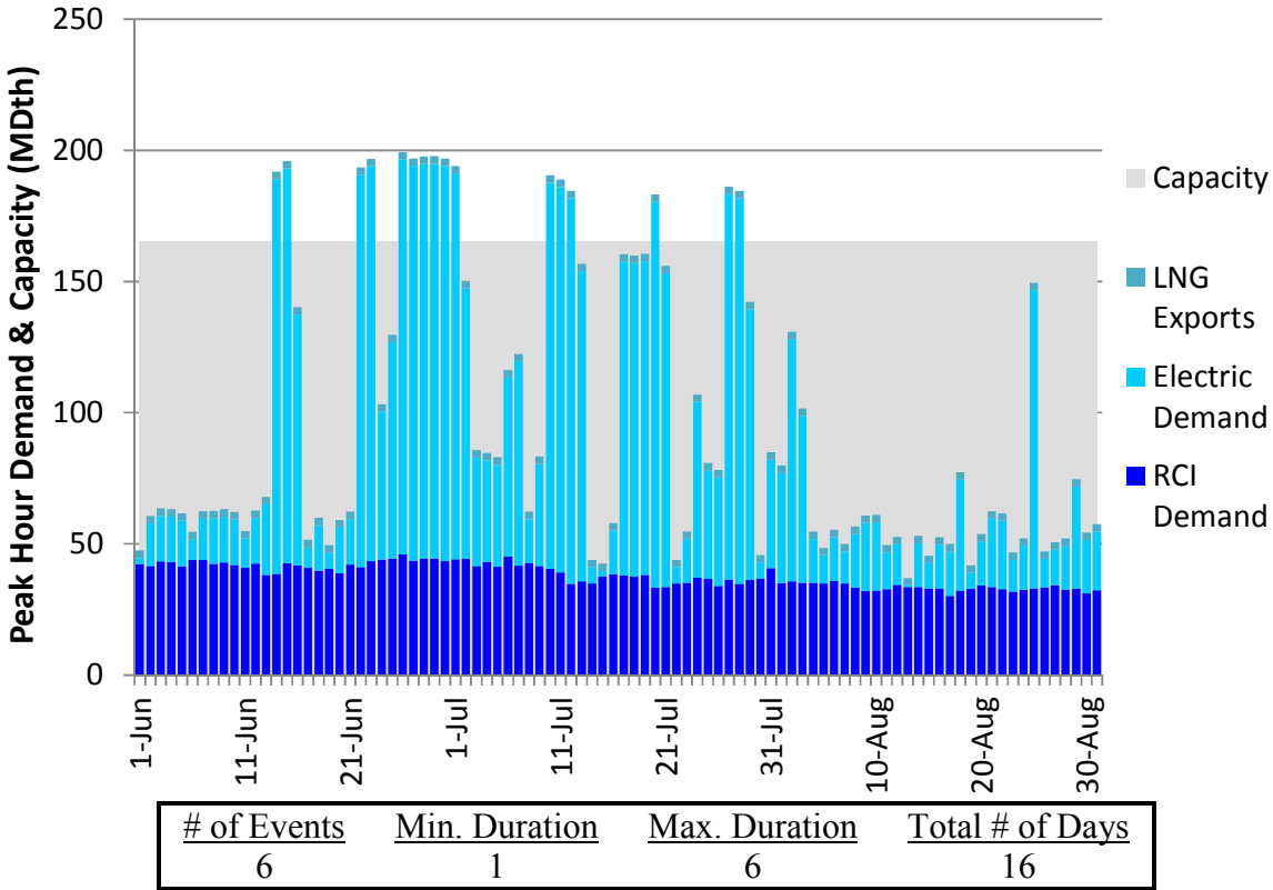
Figure E78. HGDS S0 Summer 2018 – Transco Z5 – Descending Demand
