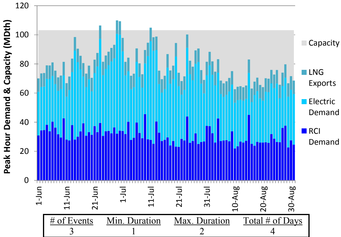
Figure E244. LGDS S0 Summer 2023 – Columbia Gas VA/MD – Descending Demand
