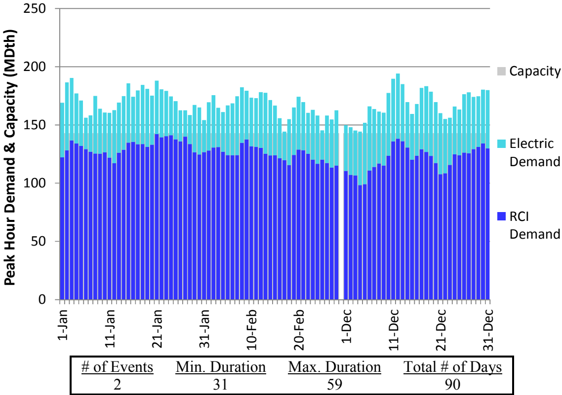
Figure E56. HGDS S0 Winter 2018 – Transco Leidy to 210 – Descending Demand
