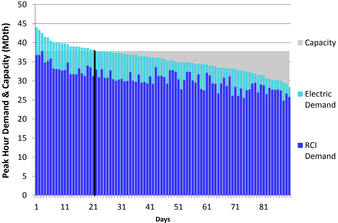
Figure E12. HGDS S0 Winter 2018 – Dominion Eastern NY– Descending Demand
