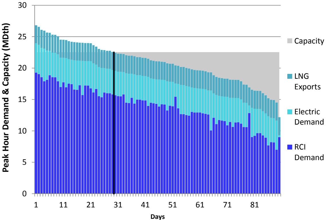
Figure E214. LGDS S0 Winter 2023 – Dominion Southeast – Descending Demand
