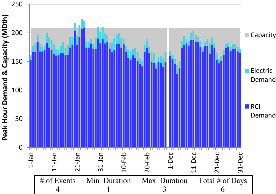
Figure E58. HGDS S0 Winter 2018 – Union Gas Dawn – Descending Demand
