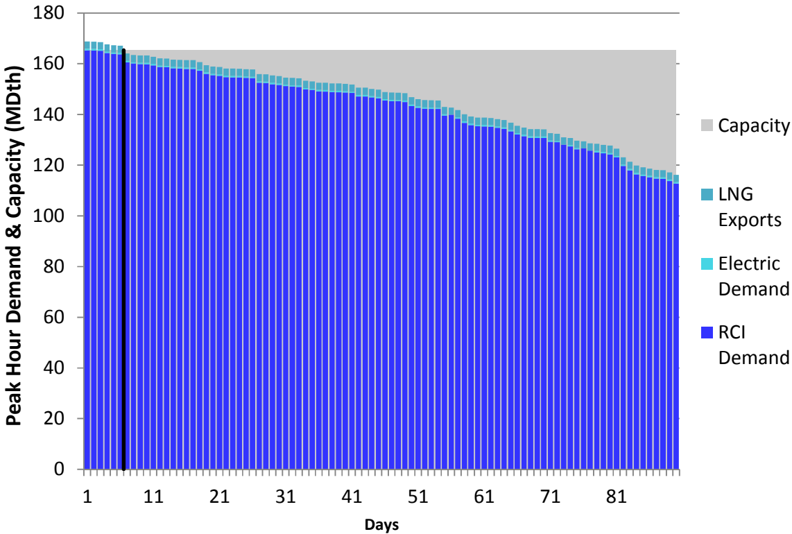
Figure E236. LGDS S0 Winter 2023 – Transco Z5 – Descending Demand
