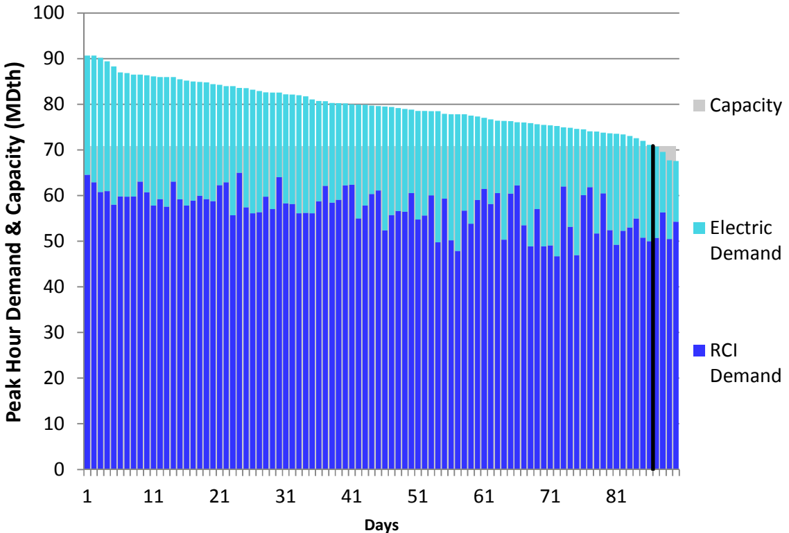
Figure E132. HGDS S0 Winter 2023 – Transco Leidy Atlantic – Descending Demand
