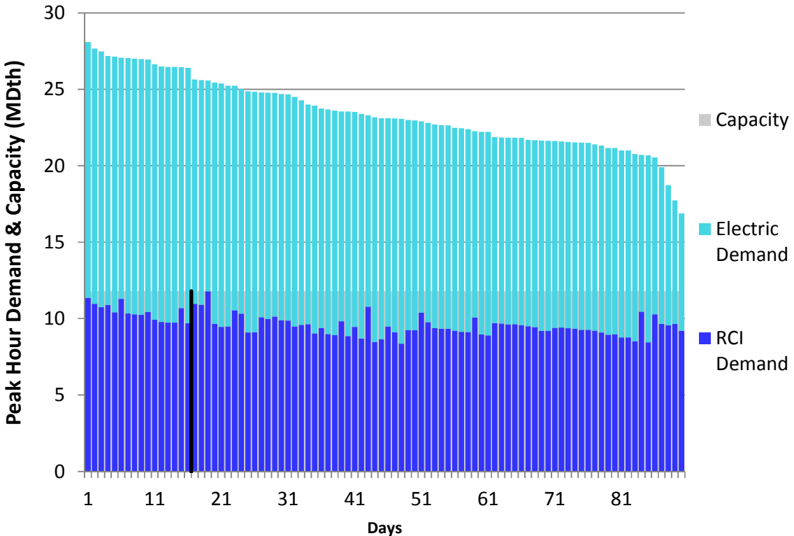
Figure E110. HGDS S0 Winter 2023 – NB/NS – Descending Demand
