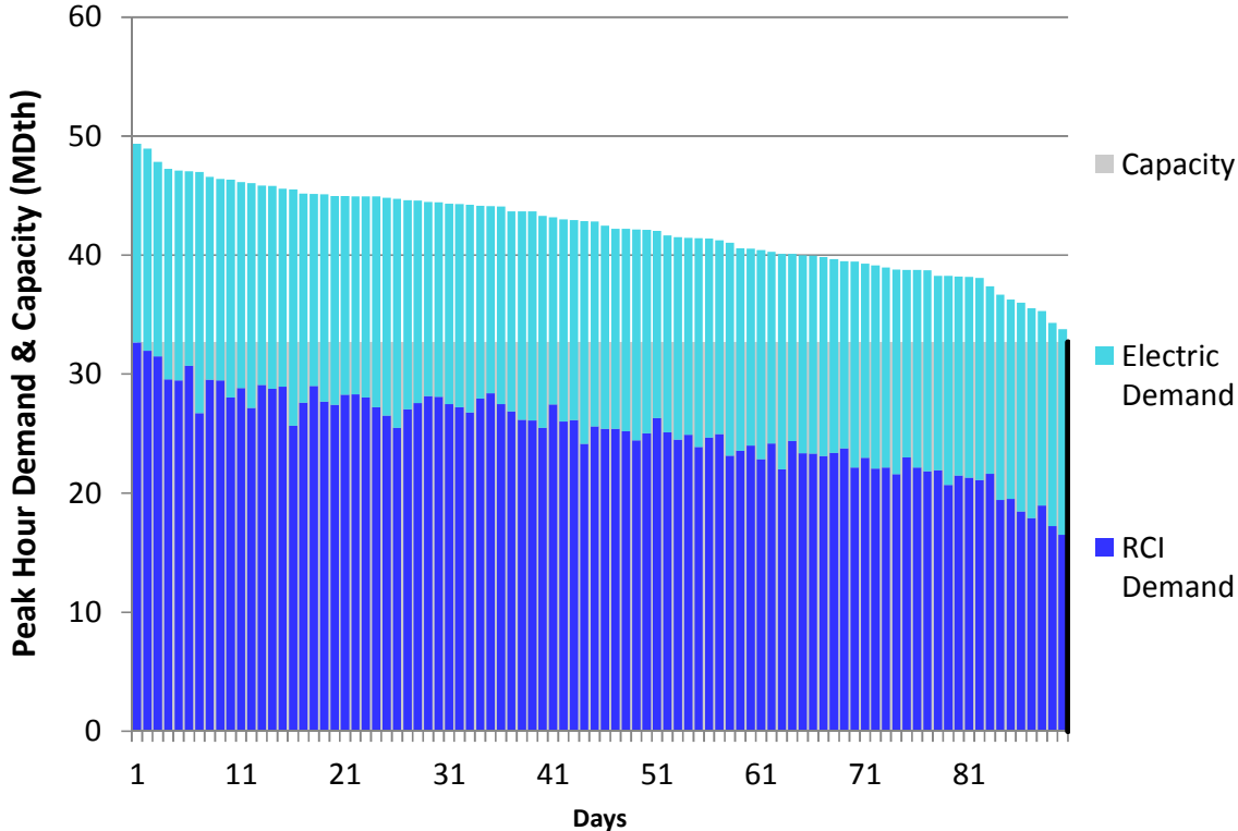
Figure E108. HGDS S0 Winter 2023 – Millennium – Descending Demand
