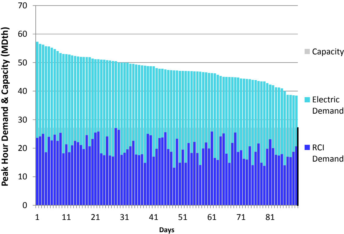
Figure E88. HGDS S0 Winter 2018 – Constitution – Descending Demand
