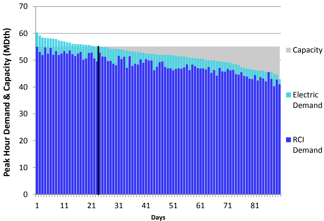
Figure E188. LGDS S0 Winter 2018 – TransCanada Quebec – Descending Demand
