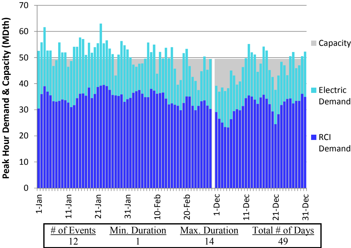
Figure E180. LGDS S0 Winter 2018 – Tennessee Z5 NY – Descending Demand
