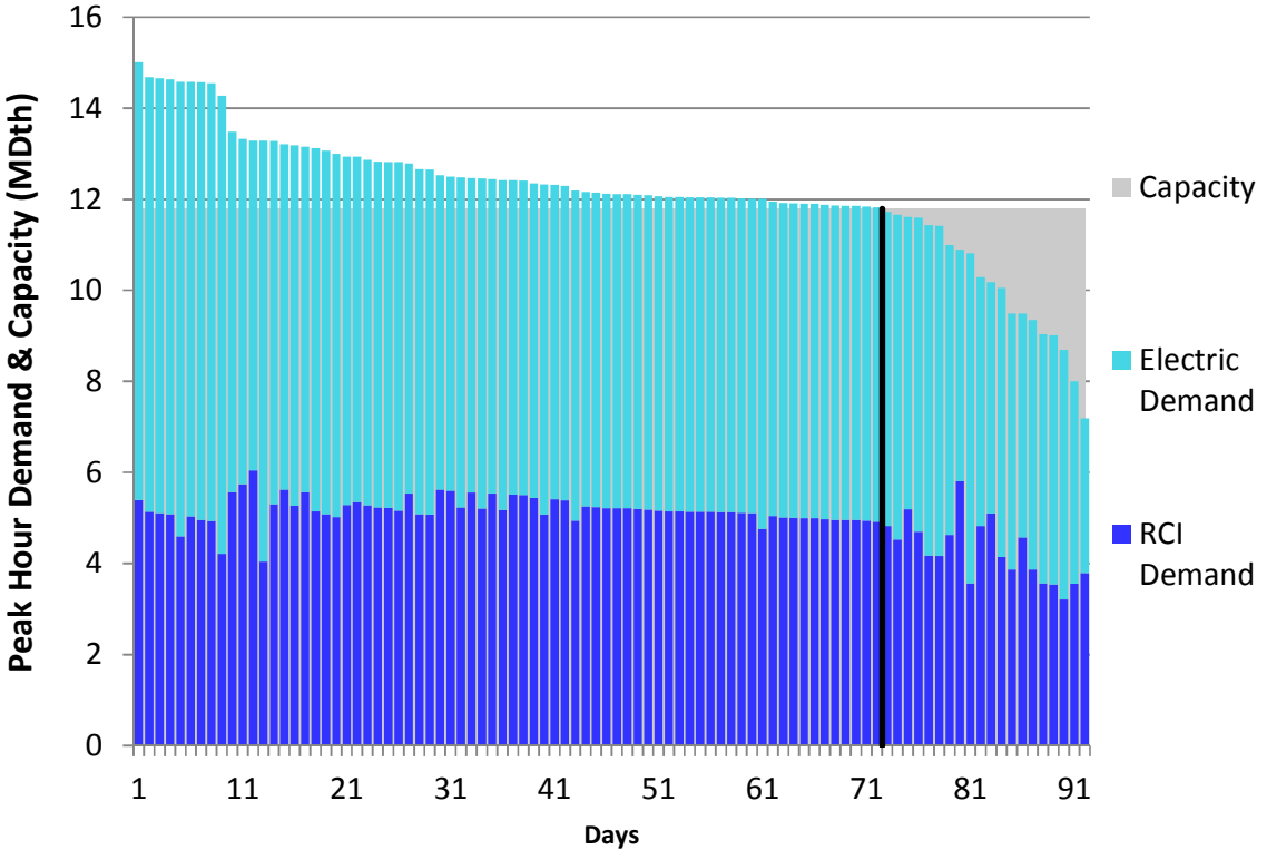
Figure E250. LGDS S0 Summer 2023 – NB/NS – Descending Demand
