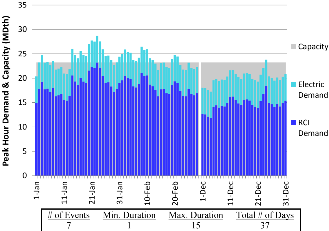
Figure E92. HGDS S0 Winter 2023 – Dominion Western NY– Descending Demand
