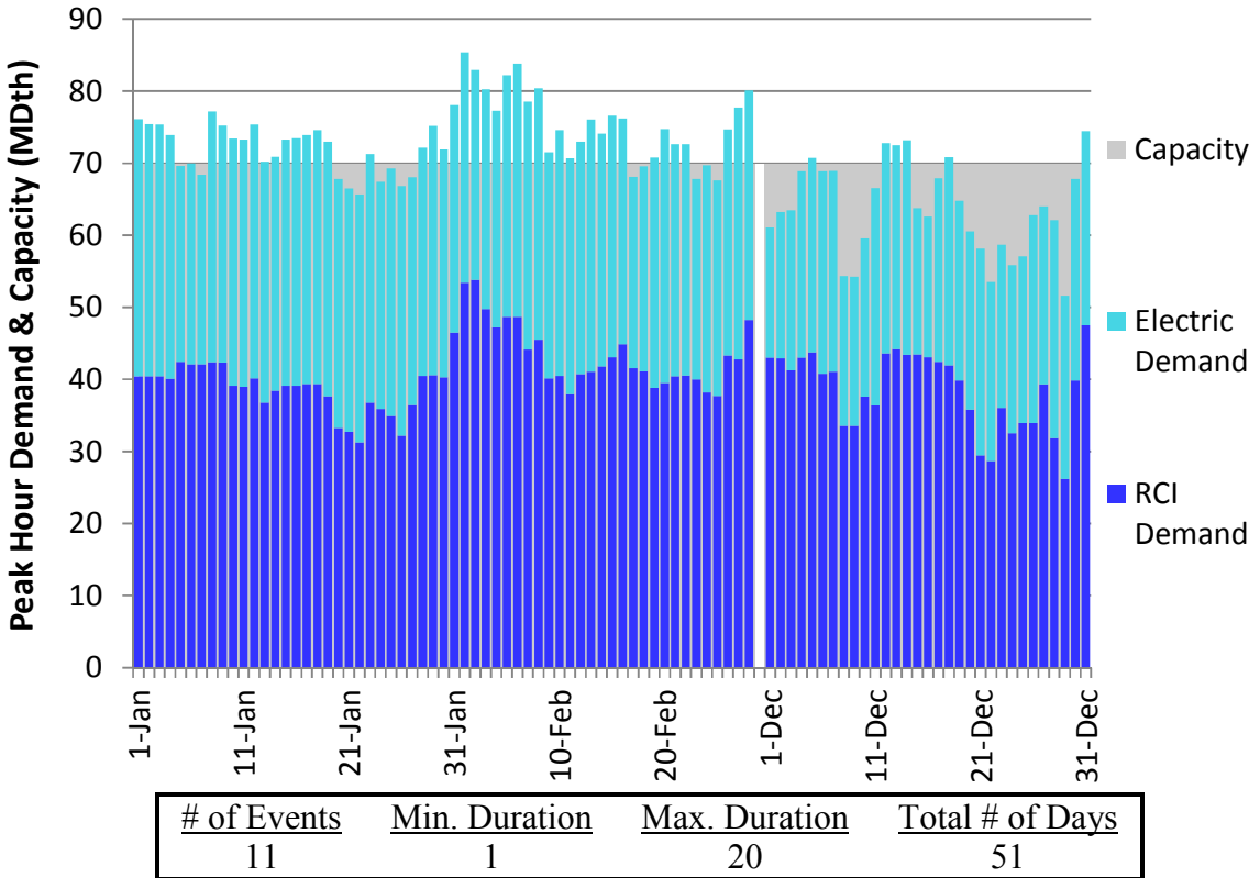
Figure E32. HGDS S0 Winter 2018 – NGPL IA/IL North – Descending Demand
