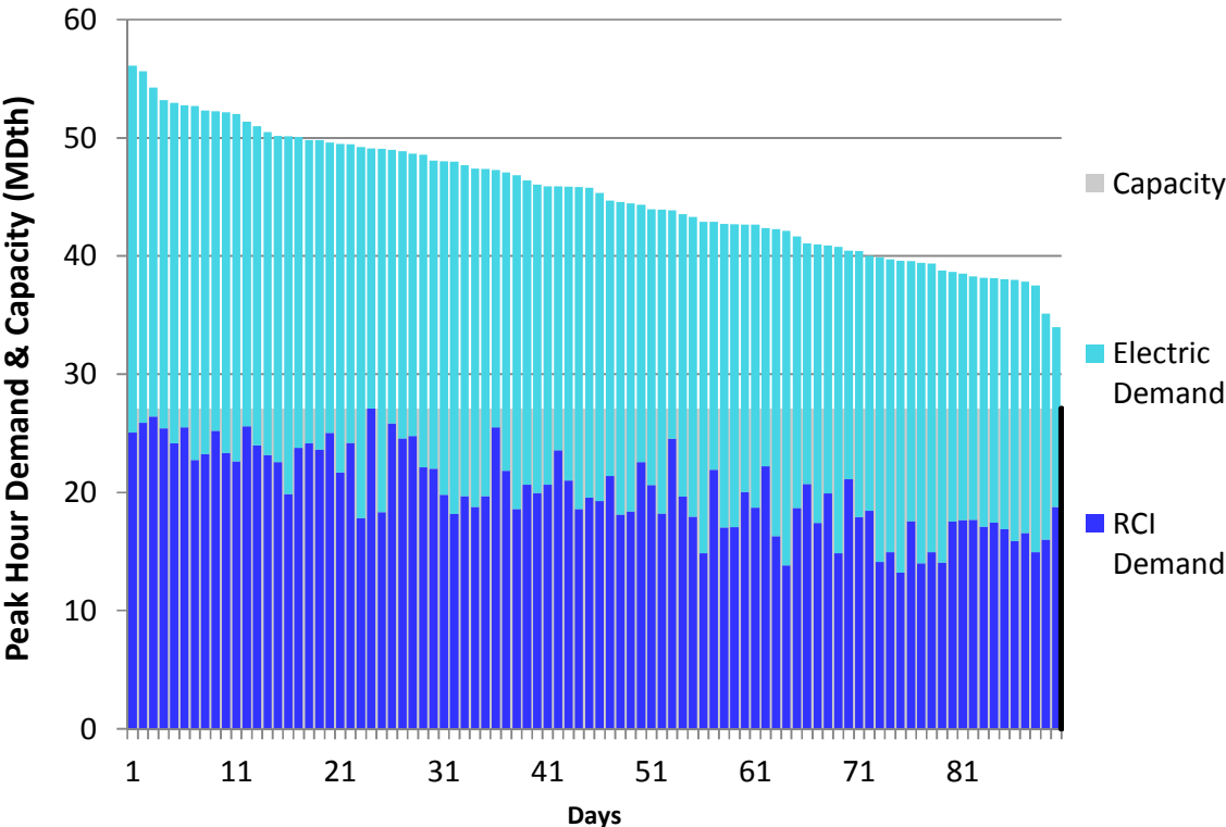
Figure E10. HGDS S0 Winter 2018 – Constitution – Descending Demand
