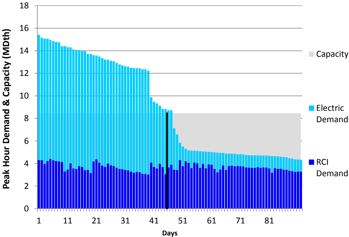
Figure E68. HGDS S0 Summer 2018 – Eastern Shore – Descending Demand
