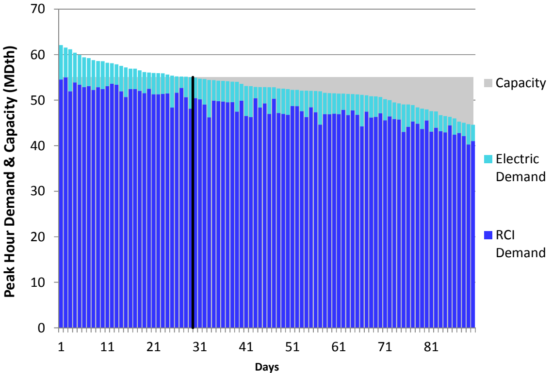
Figure E50. HGDS S0 Winter 2018 – TransCanada Quebec – Descending Demand
