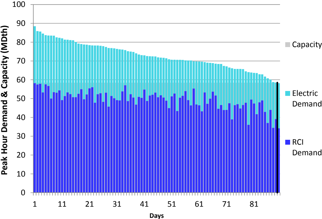
Figure E122. HGDS S0 Winter 2023 – Tennessee Z5 NY – Descending Demand
