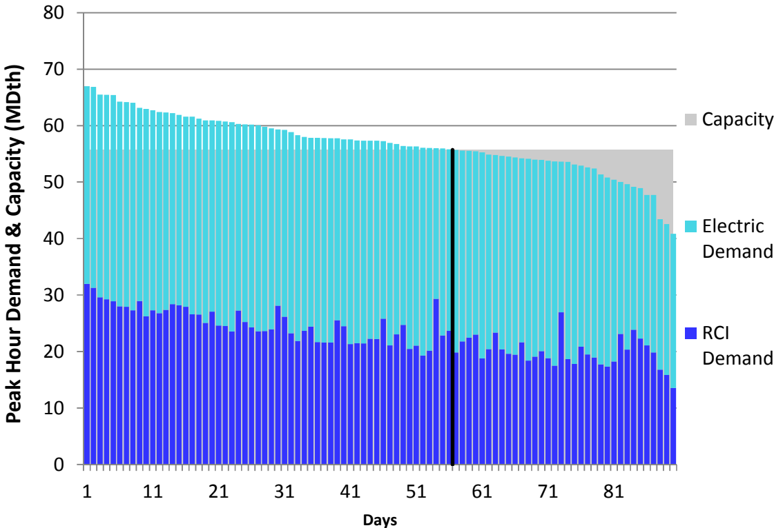
Figure E82. HGDS S0 Winter 2023 – ANR Northern IL – Descending Demand
