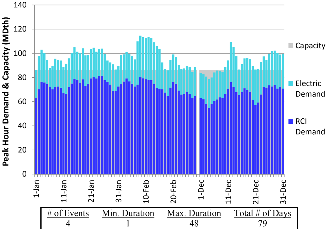
Figure E182. LGDS S0 Winter 2018 – Texas Eastern M2 PA South – Descending Demand
