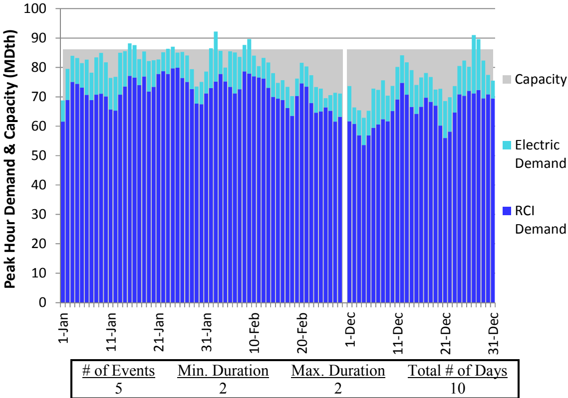
Figure E228. LGDS S0 Winter 2023 – Texas Eastern M2 PA South – Descending Demand
