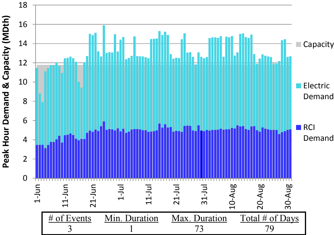
Figure E70. HGDS S0 Summer 2018 – NB/NS – Descending Demand
