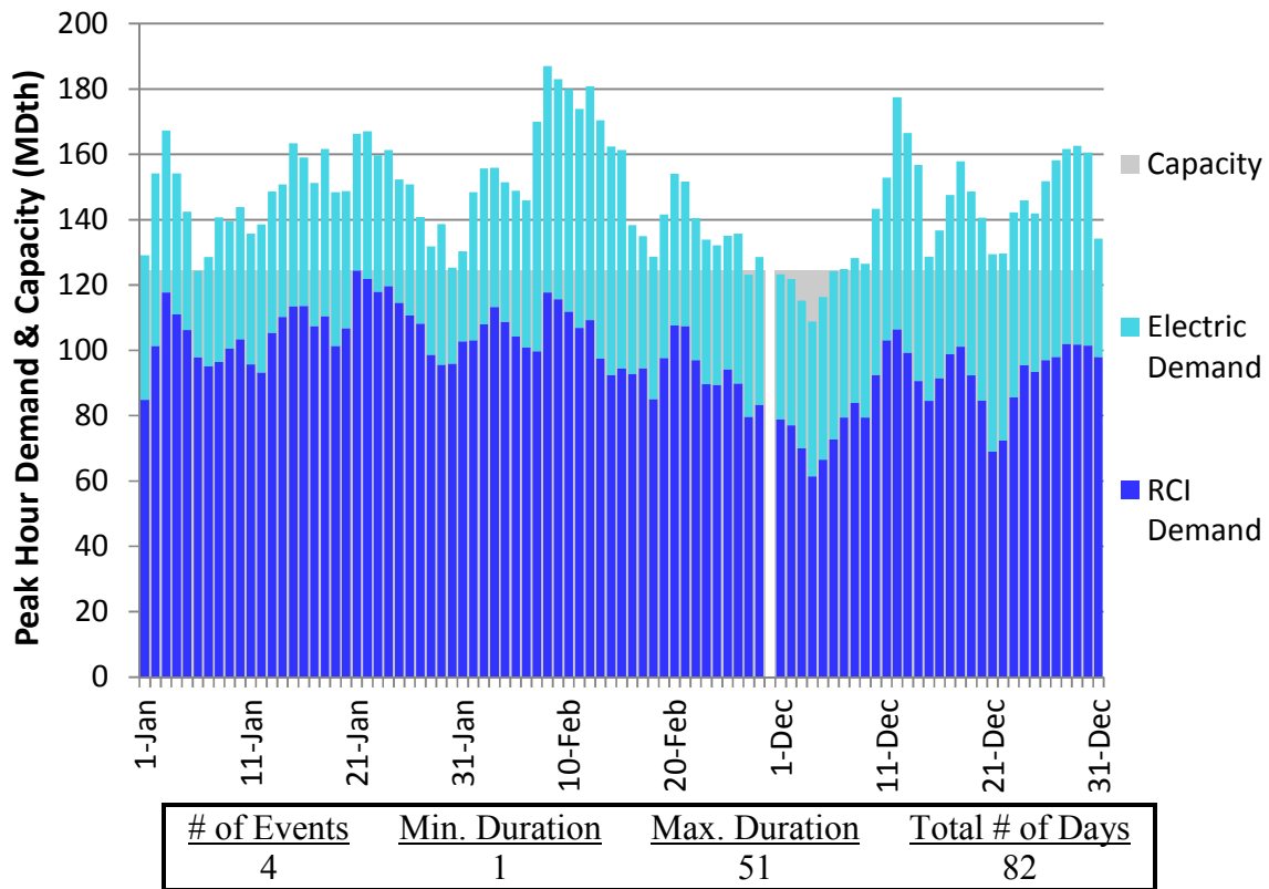
Figure E46. HGDS S0 Winter 2018 – Texas Eastern M3 North – Descending Demand
