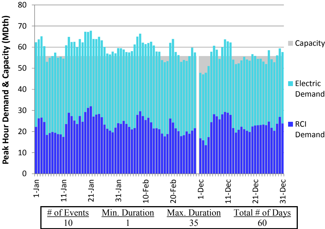
Figure E4. HGDS S0 Winter 2018 – ANR Northern IL – Descending Demand
