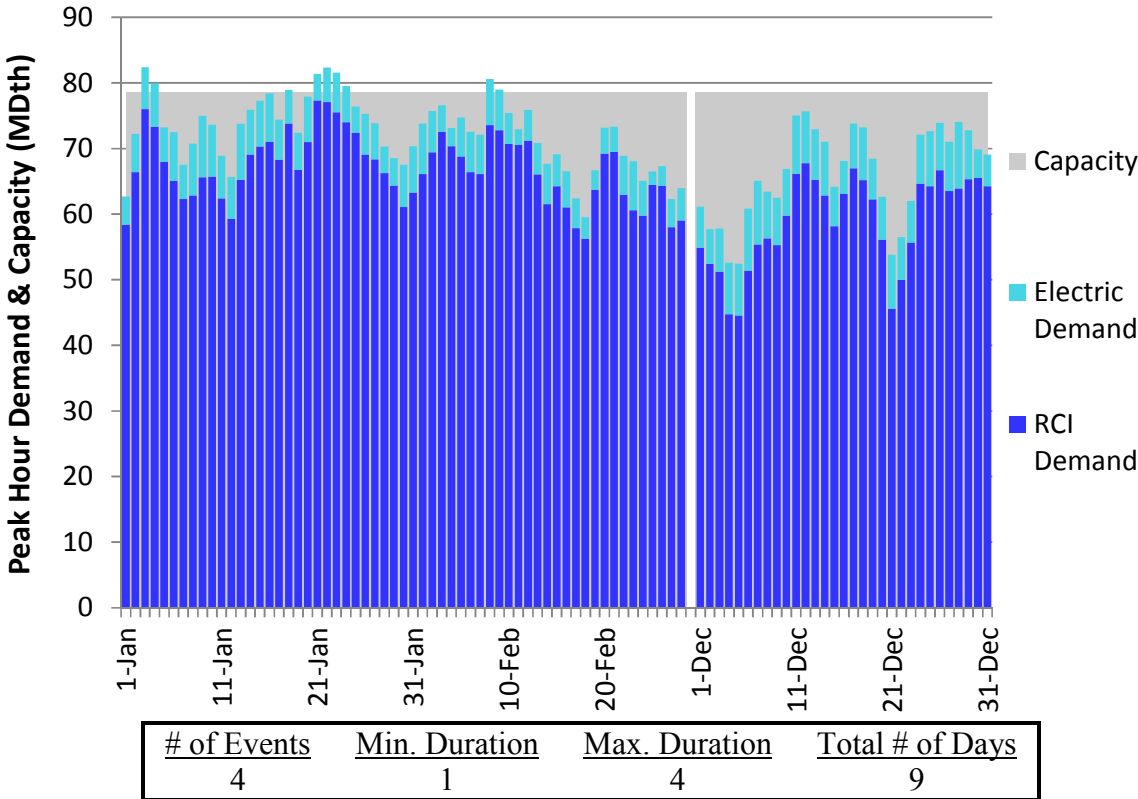
Figure E224. LGDS S0 Winter 2023 – Tennessee Z4 PA – Descending Demand
