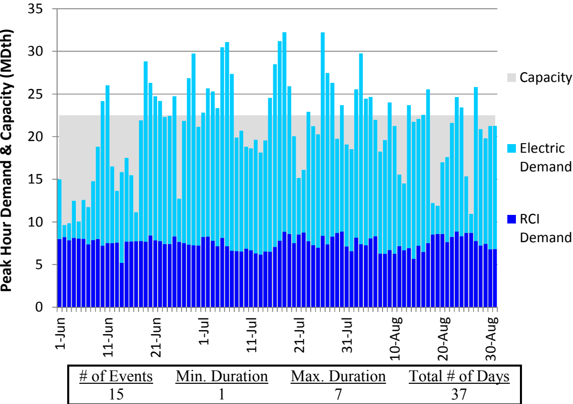
Figure E66. HGDS S0 Summer 2018 – Dominion Southeast – Descending Demand
