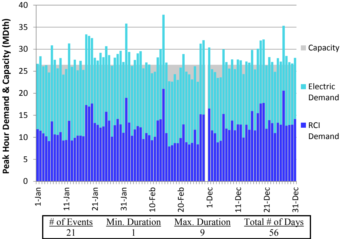
Figure E106. HGDS S0 Winter 2023 – Midwestern – Descending Demand
