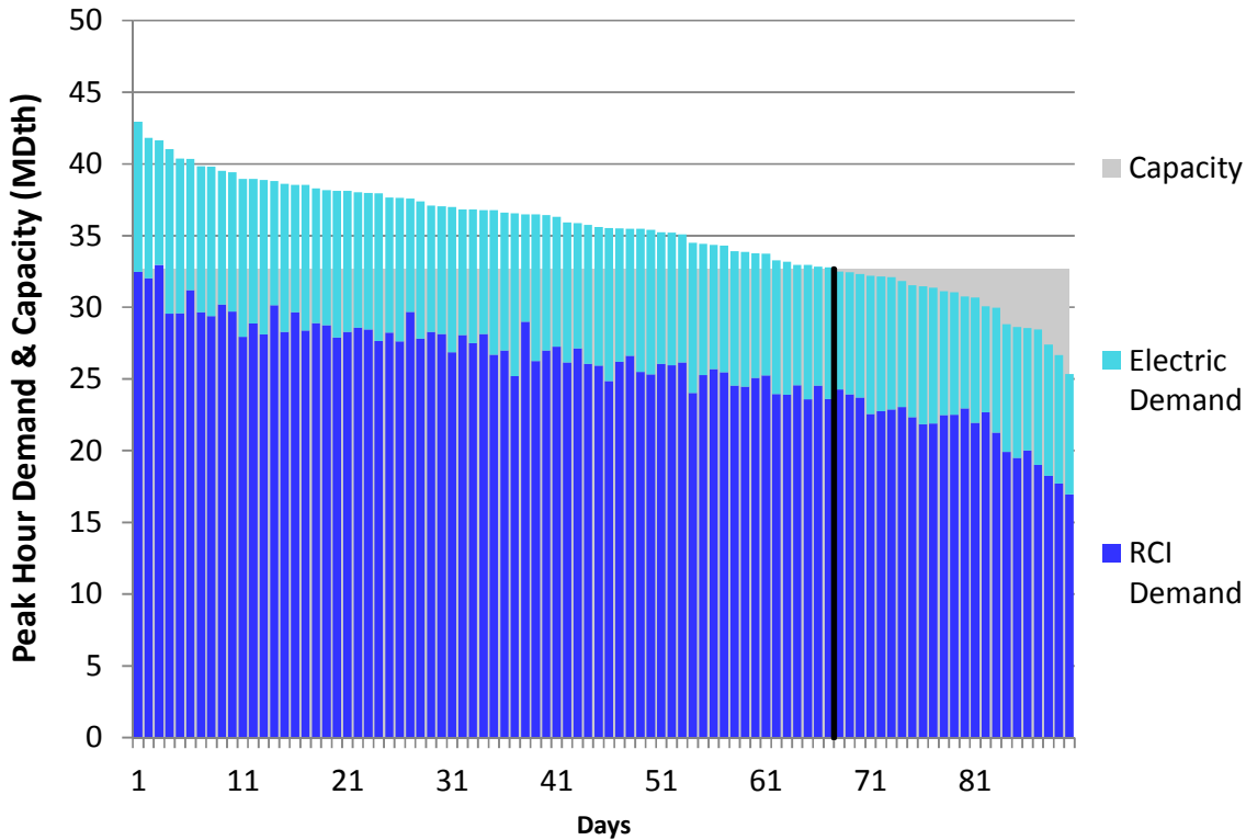
Figure E28. HGDS S0 Winter 2018 – Millennium – Descending Demand
