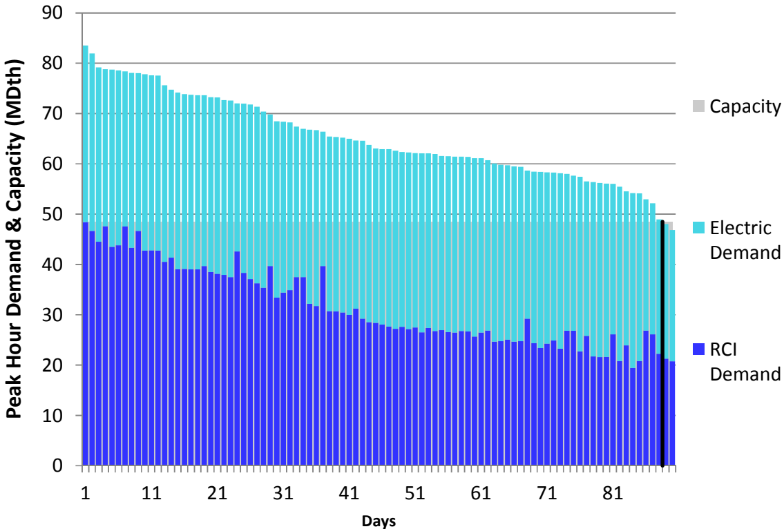
Figure E102. HGDS S0 Winter 2023 – Great Lakes East – Descending Demand
