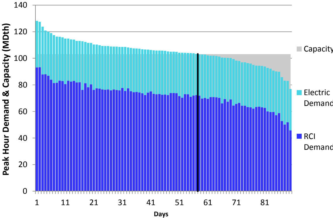
Figure E6. HGDS S0 Winter 2018 – Columbia Gas VA/MD – Descending Demand
