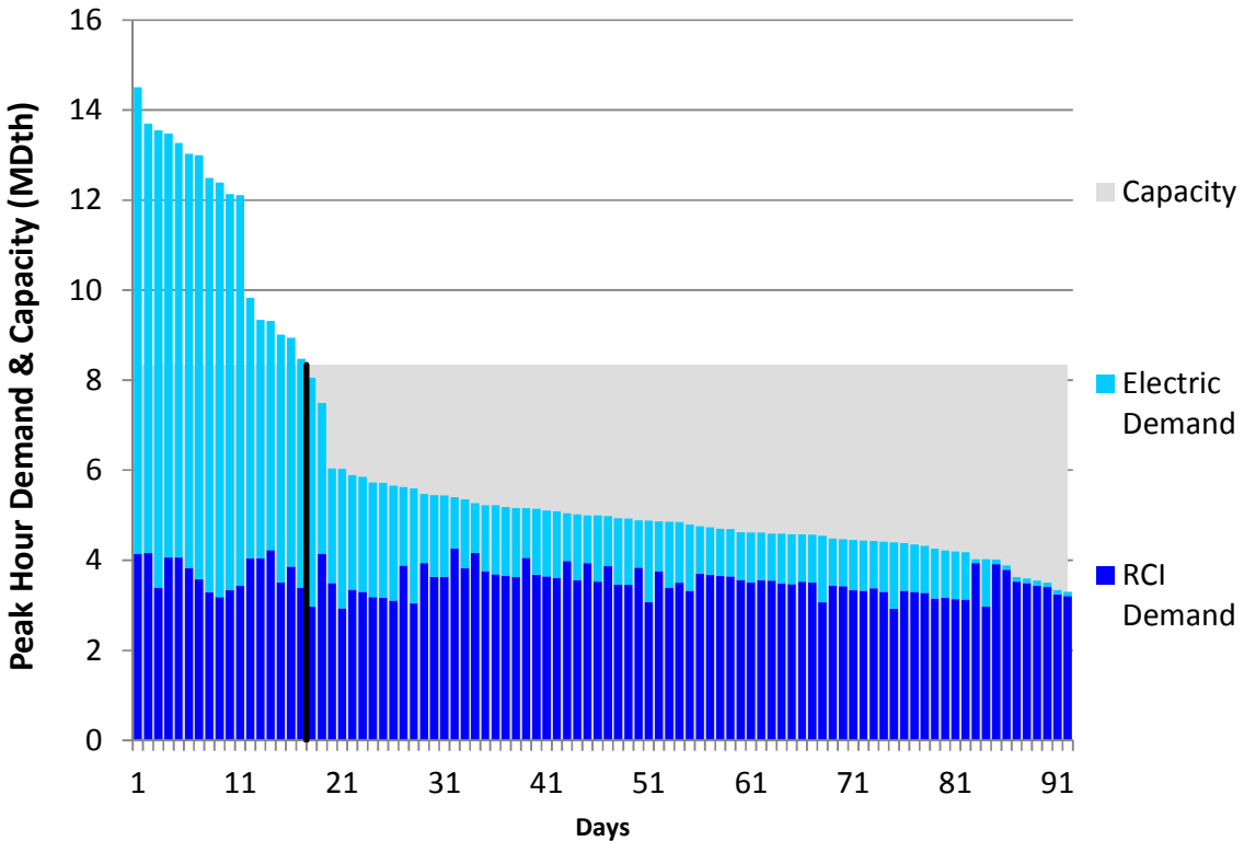
Figure E198. LGDS S0 Summer 2018 – Eastern Shore – Descending Demand
