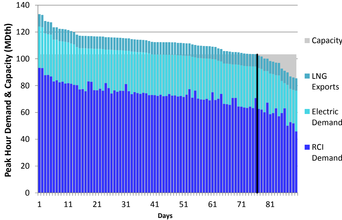
Figure E206. LGDS S0 Winter 2023 – Columbia Gas VA/MD – Descending Demand
