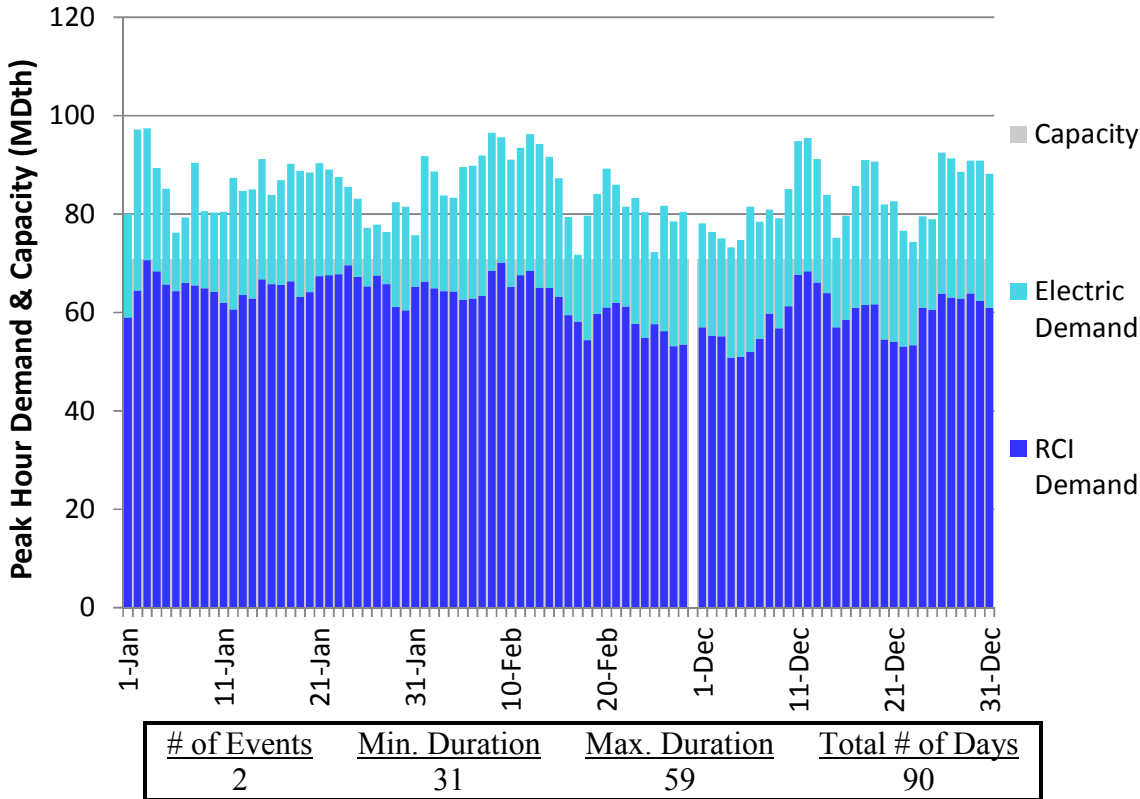
Figure E52. HGDS S0 Winter 2018 – Transco Leidy Atlantic – Descending Demand
