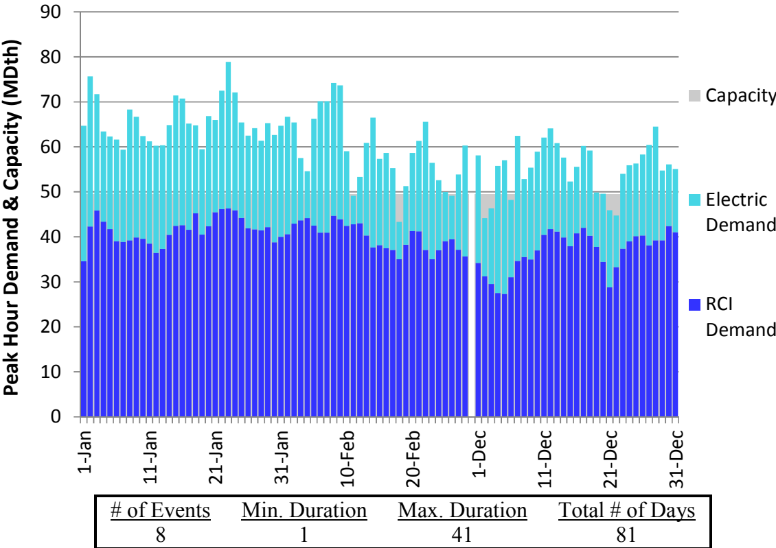
Figure E226. LGDS S0 Winter 2023 – Tennessee Z5 NY – Descending Demand
