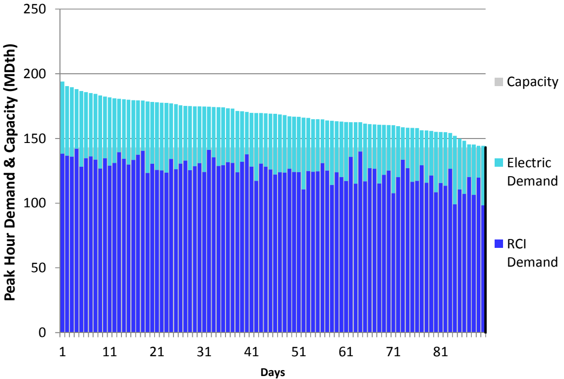
Figure E56. HGDS S0 Winter 2018 – Transco Leidy to 210 – Descending Demand
