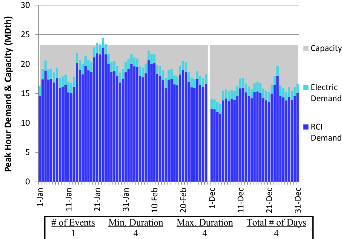
Figure E212. LGDS S0 Winter 2023 – Dominion Western NY– Descending Demand
