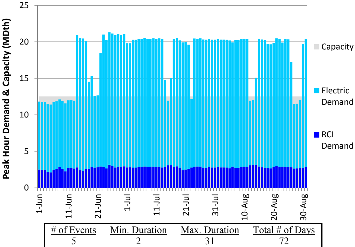
Figure E160. HGDS S0 Summer 2023 – PNGTS S of Westbrook – Descending Demand
