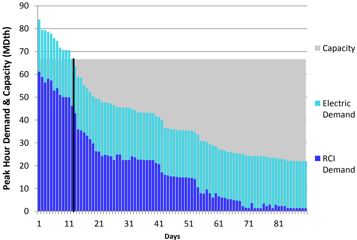
Figure E140. HGDS S0 Winter 2023 – Vector Zone 1 – Descending Demand
