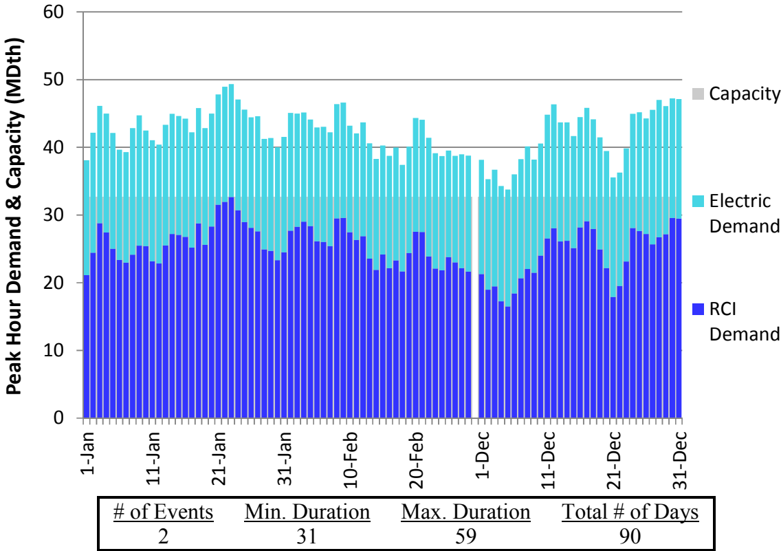
Figure E108. HGDS S0 Winter 2023 – Millennium – Descending Demand
