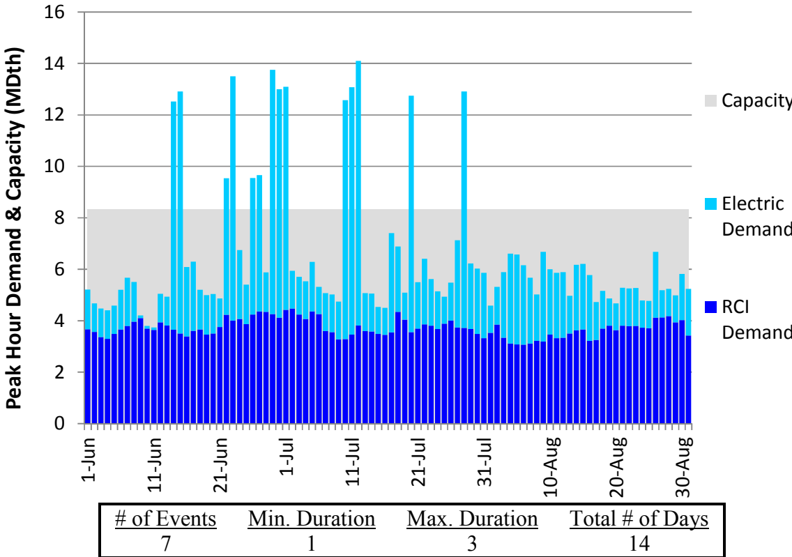
Figure E248. LGDS S0 Summer 2023 – Eastern Shore – Descending Demand
