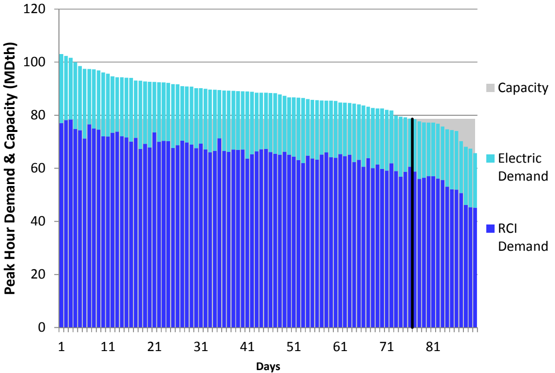
Figure E40. HGDS S0 Winter 2018 – Tennessee Z4 PA – Descending Demand
