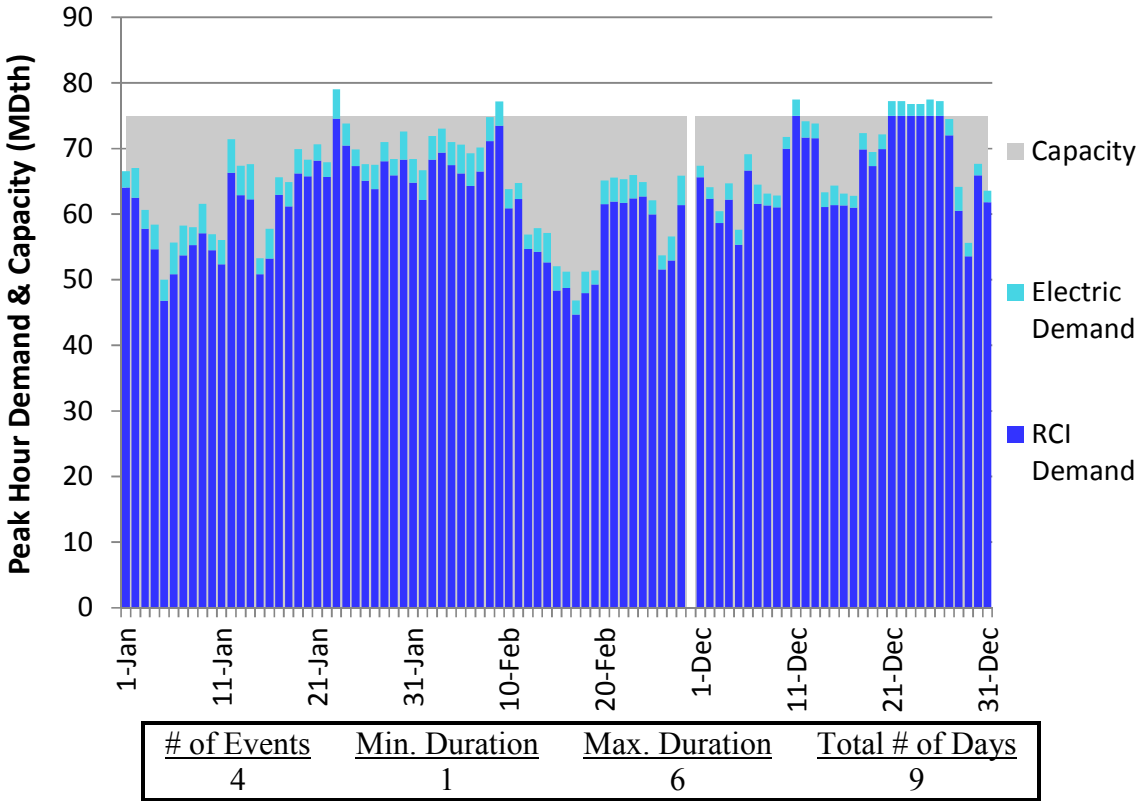
Figure E80. HGDS S0 Winter 2023 – Alliance – Descending Demand
