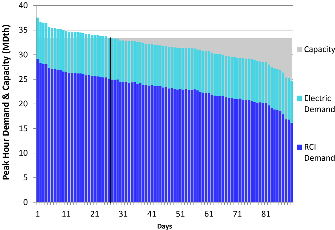
Figure E96. HGDS S0 Winter 2023 – East Tennessee – Descending Demand
