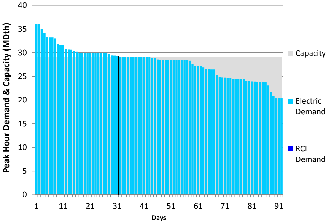
Figure E152. HGDS S0 Summer 2023 – Gulf South Z2 HH – Descending Demand
