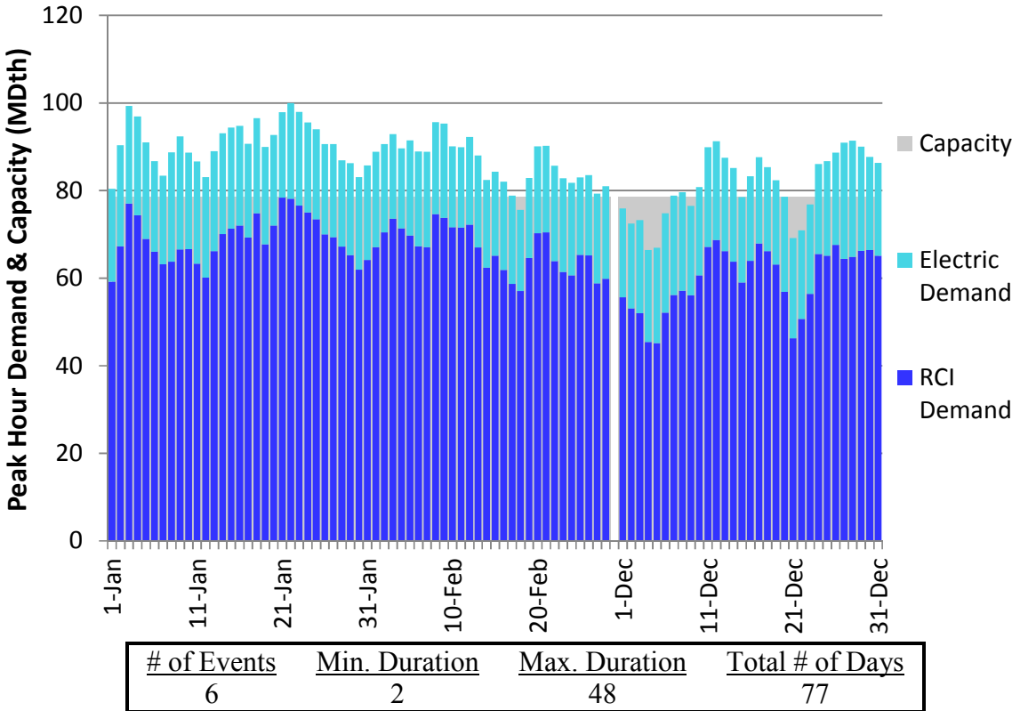
Figure E120. HGDS S0 Winter 2023 – Tennessee Z4 PA – Descending Demand
