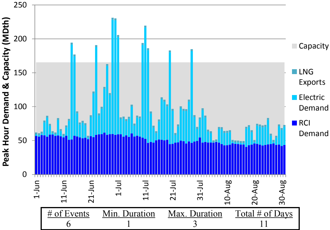
Figure E256. LGDS S0 Summer 2023 – Transco Z5 – Descending Demand
