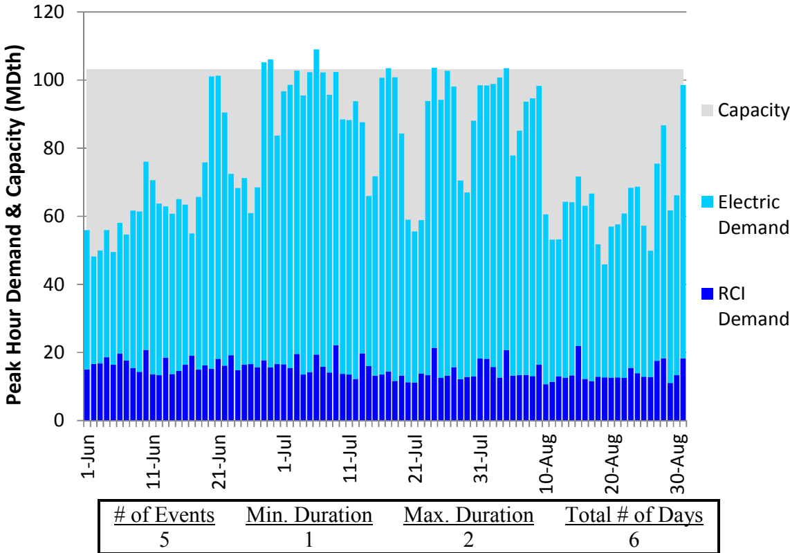
Figure E64. HGDS S0 Summer 2018 – Columbia Gas VA/MD – Descending Demand
