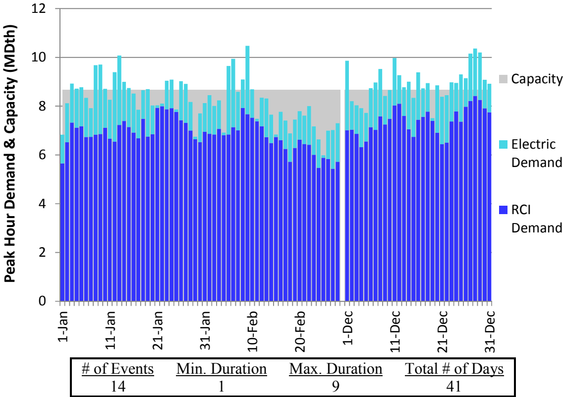
Figure E218. LGDS S0 Winter 2023 – Eastern Shore – Descending Demand
