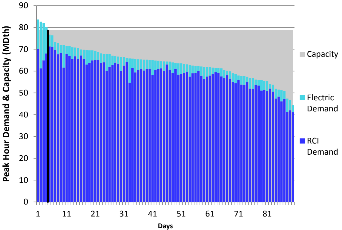
Figure E178. LGDS S0 Winter 2018 – Tennessee Z4 PA – Descending Demand
