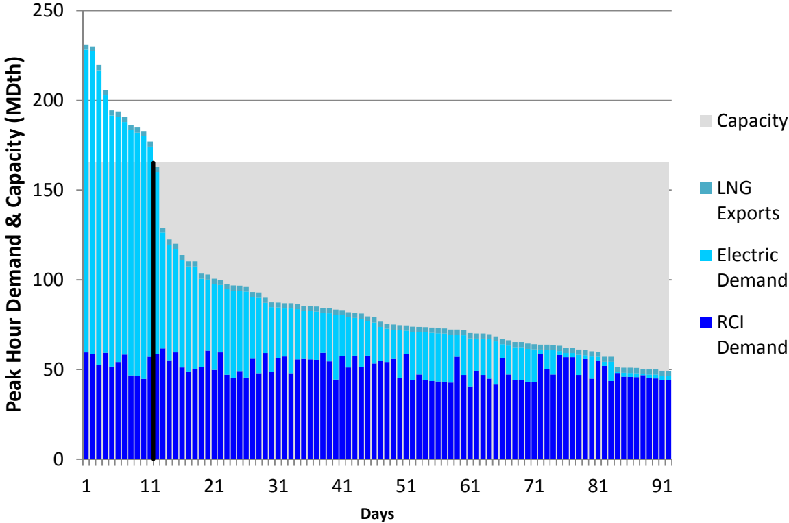
Figure E256. LGDS S0 Summer 2023 – Transco Z5 – Descending Demand
