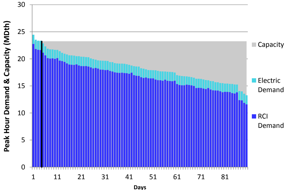
Figure E212. LGDS S0 Winter 2023 – Dominion Western NY– Descending Demand
