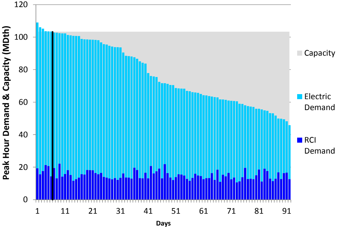
Figure E64. HGDS S0 Summer 2018 – Columbia Gas VA/MD – Descending Demand
