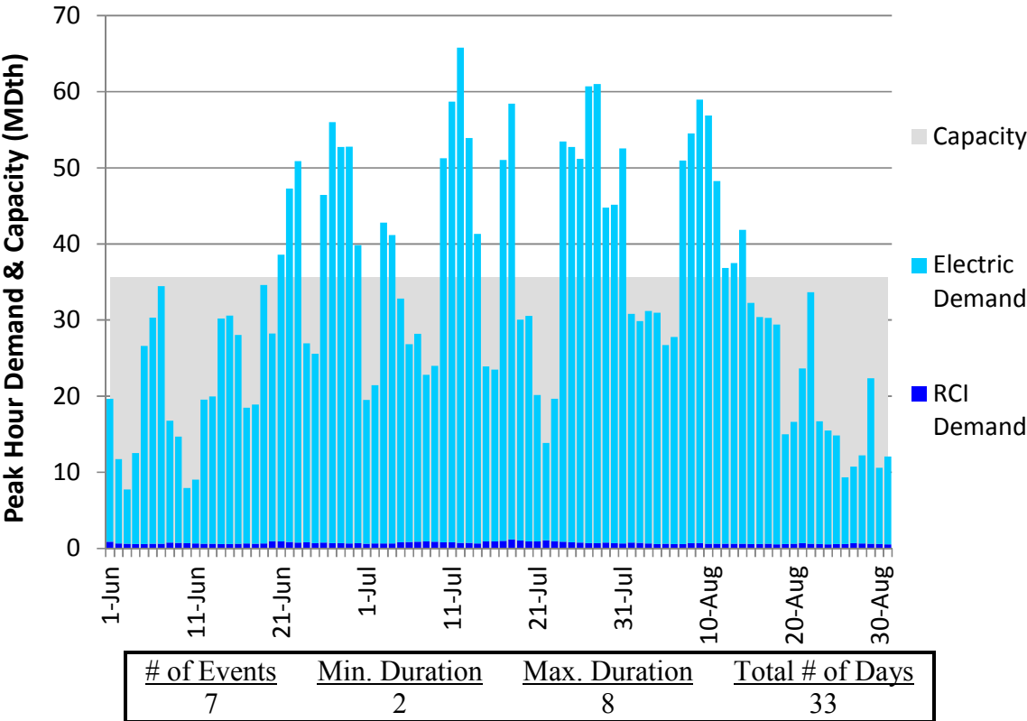
Figure E154. HGDS S0 Summer 2023 – Iroquois Z1 → Z2 – Descending Demand
