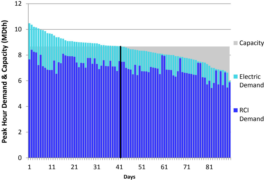
Figure E218. LGDS S0 Winter 2023 – Eastern Shore – Descending Demand
