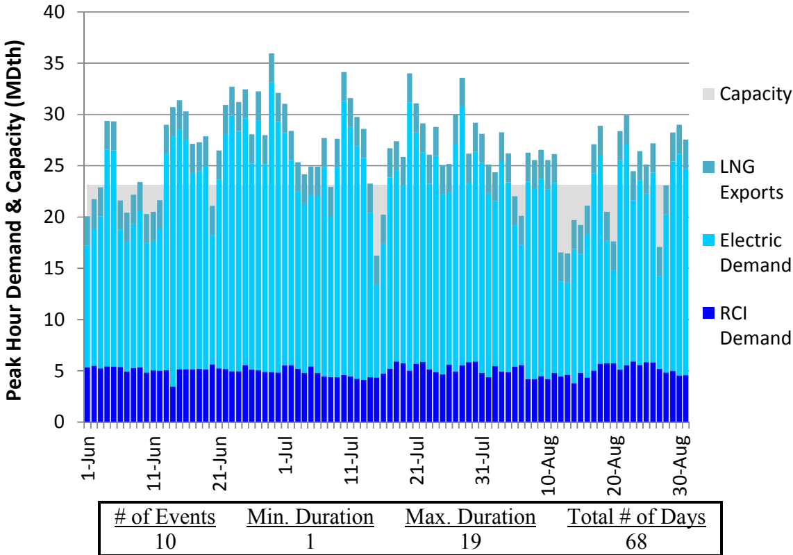
Figure E148. HGDS S0 Summer 23 – Dominion Southeast – Descending Demand
