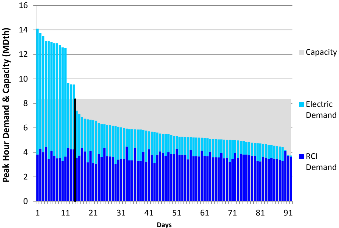
Figure E248. LGDS S0 Summer 2023 – Eastern Shore – Descending Demand
