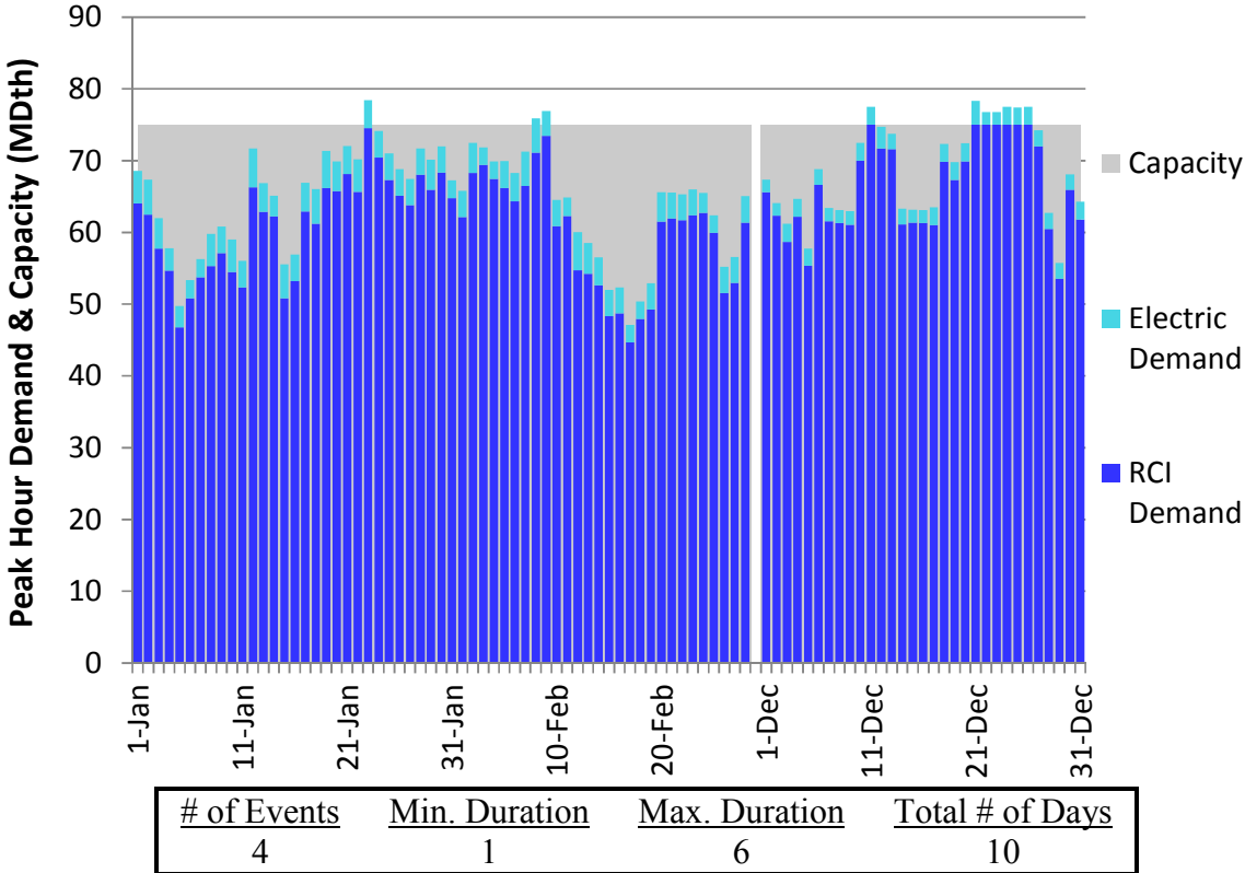
Figure E2. HGDS S0 Winter 2018 – Alliance – Descending Demand
