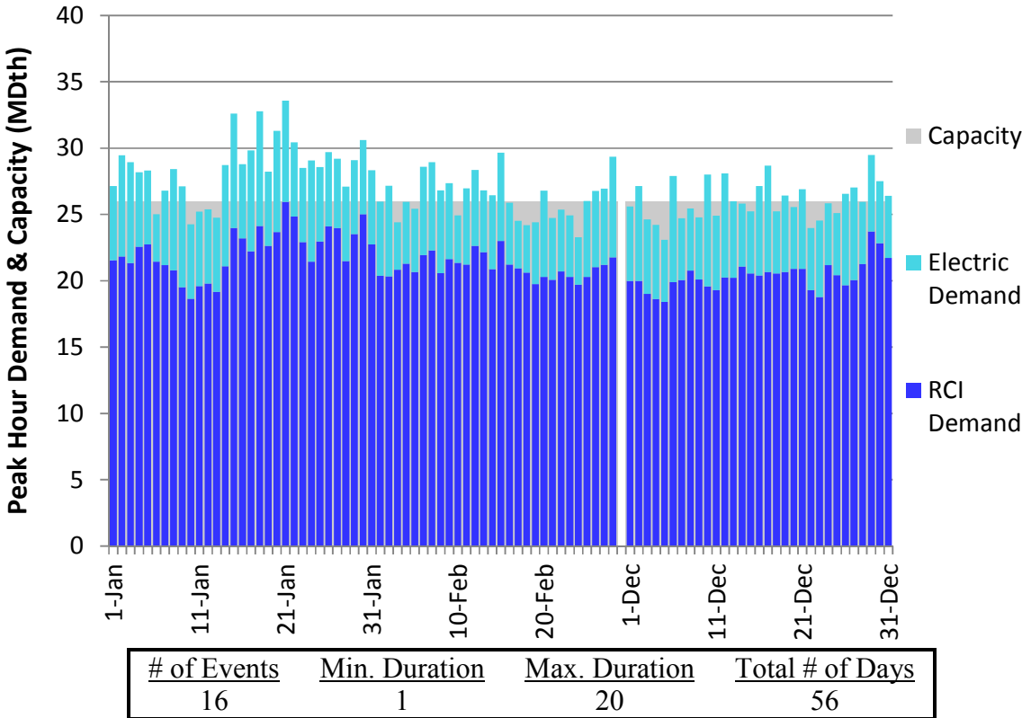
Figure E30. HGDS S0 Winter 2018 – NB/NS – Descending Demand
