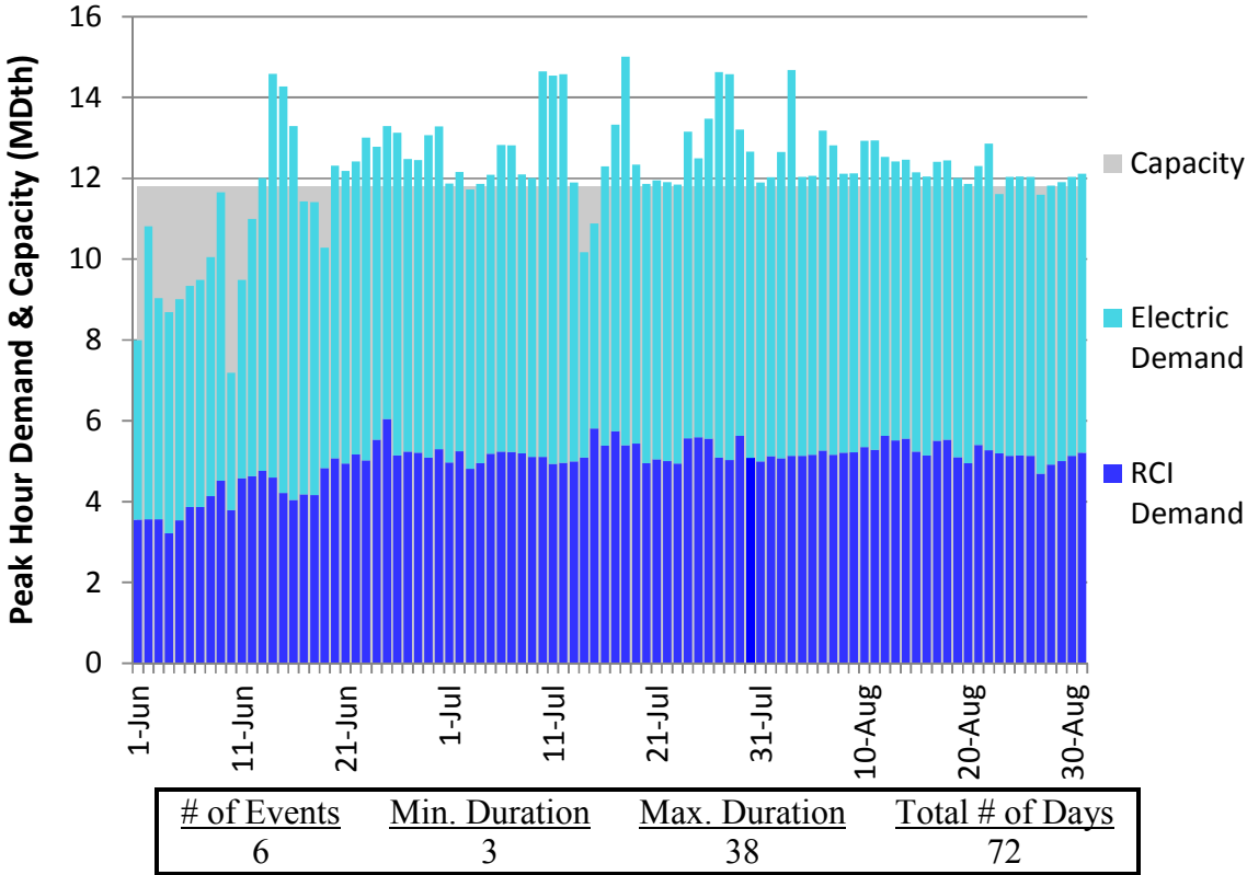
Figure E250. LGDS S0 Summer 2023 – NB/NS – Descending Demand
