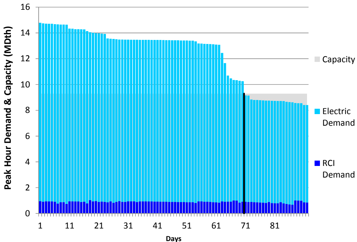
Figure E158. RGDS S0 Summer 2023 – PNGTS N of Westbrook – Descending Demand
