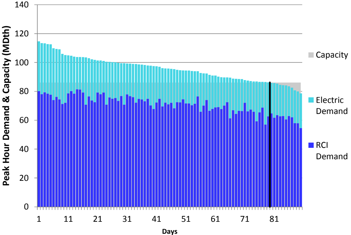
Figure E182. LGDS S0 Winter 2018 – Texas Eastern M2 PA South – Descending Demand
