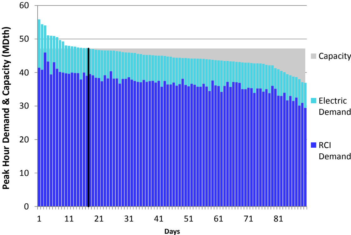
Figure E8. HGDS S0 Winter 2018 – Columbia Gas W PA/NY – Descending Demand
