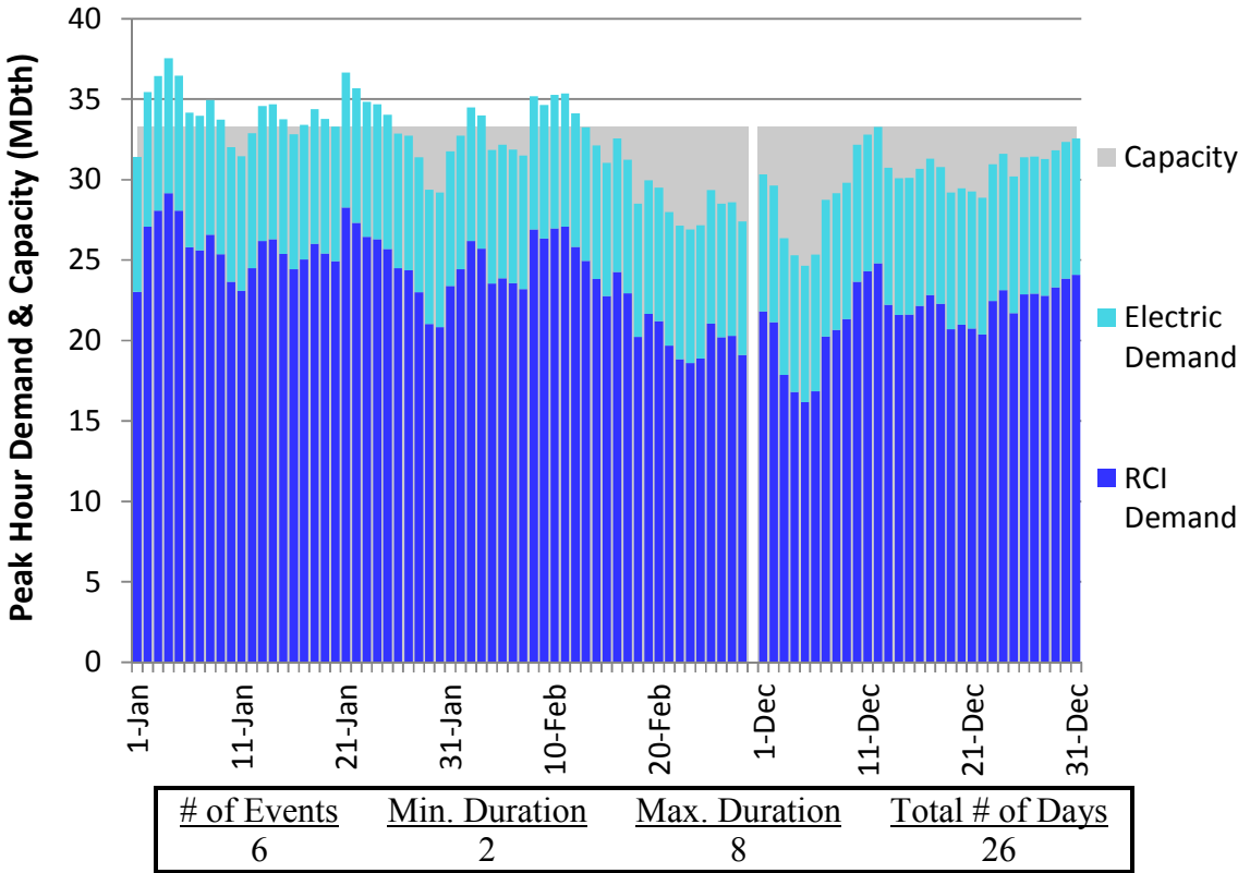
Figure E18. HGDS S0 Winter 2018 – East Tennessee – Descending Demand
