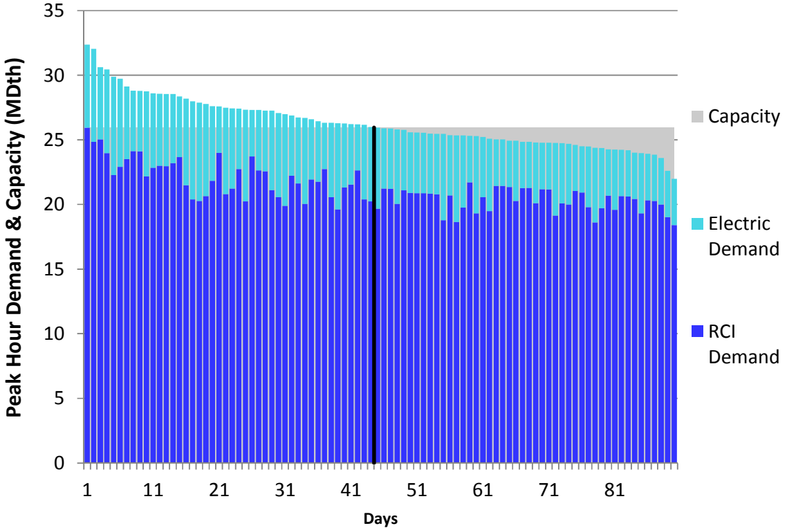
Figure E176. LGDS S0 Winter 2018 – NB/NS – Descending Demand
