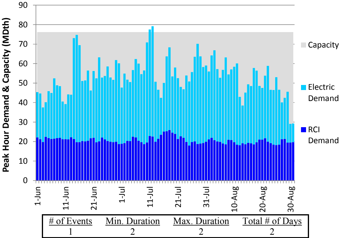
Figure E242. LGDS S0 Summer 2023 – Algonquin CT – Descending Demand
