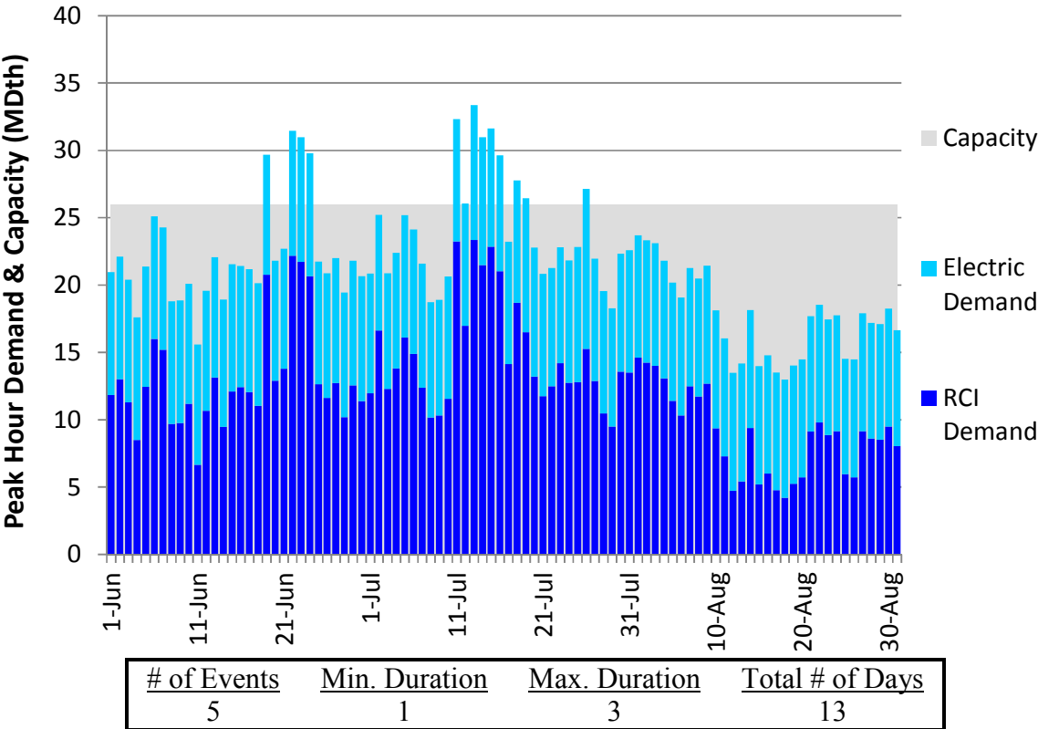
Figure E254. LGDS S0 Summer 2023 – Texas Eastern ETX – Descending Demand
